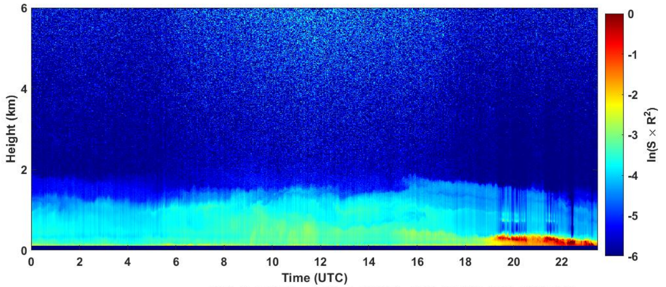
2024-09-28 RCS quick look CHM15k - ILVA LIDAR3 AGGLOMERATO
