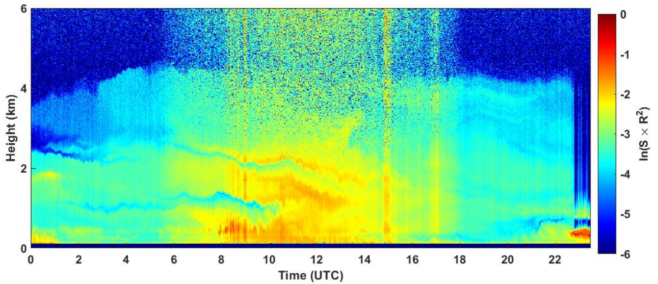
2024-09-08 RCS quick look CHM15k - ILVA LIDAR3 AGGLOMERATO
