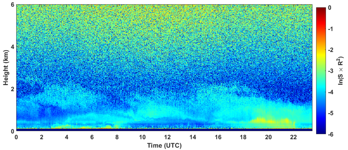
2024-09-26 RCS quick look CHM15k - ILVA LIDAR2 PARCHI
