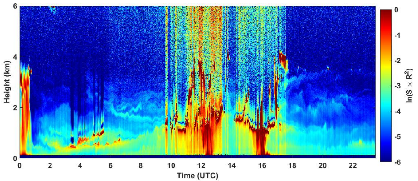
2024-09-20 RCS quick look CHM15k - ILVA LIDAR3 AGGLOMERATO
