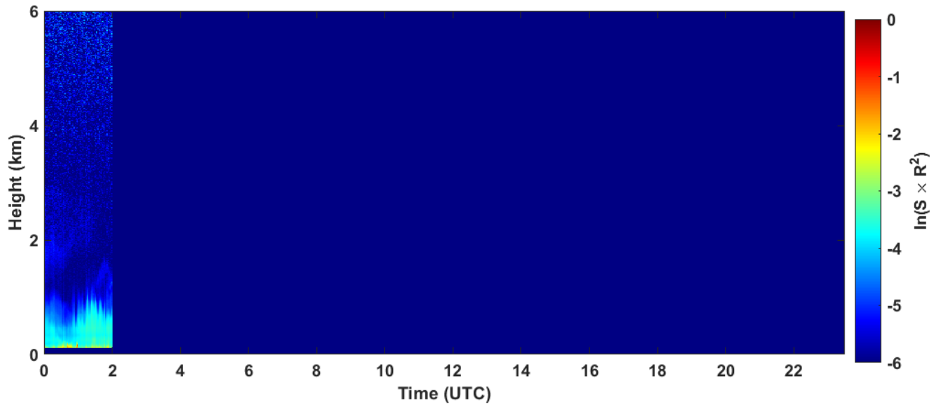
2024-09-30 RCS quick look CHM15k - ILVA LIDAR3 AGGLOMERATO
