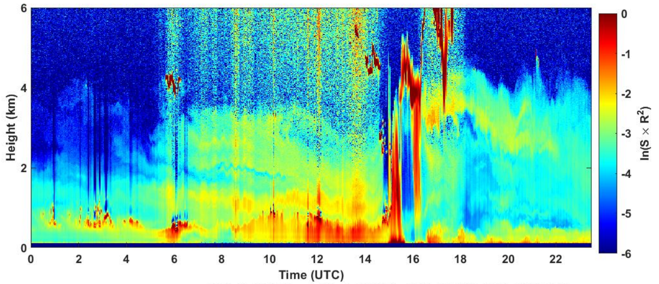
2024-09-06 RCS quick look CHM15k - ILVA LIDAR3 AGGLOMERATO
