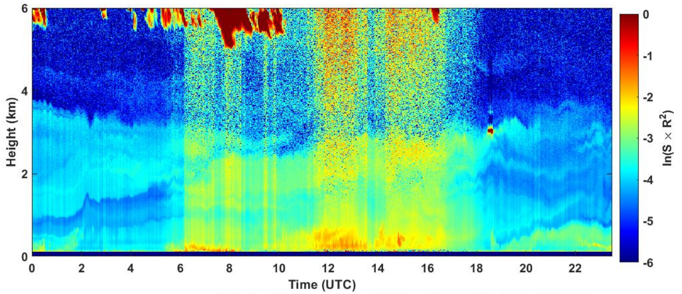
2024-09-04 RCS quick look CHM15k - ILVA LIDAR3 AGGLOMERATO
