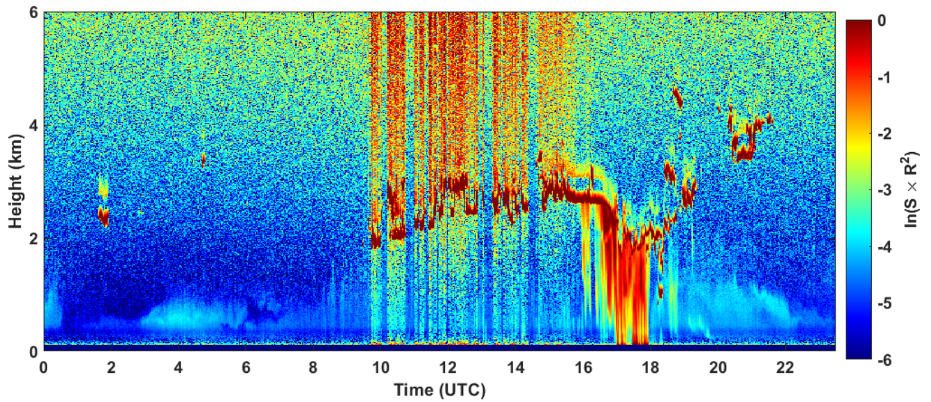
2024-09-14 RCS quick look CHM15k - ILVA LIDAR2 PARCHI
