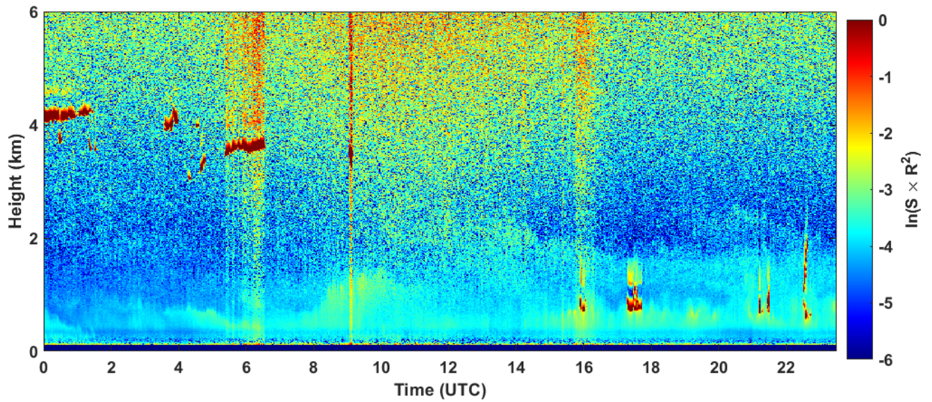
2024-09-04 RCS quick look CHM15k - ILVA LIDAR2 PARCHI
