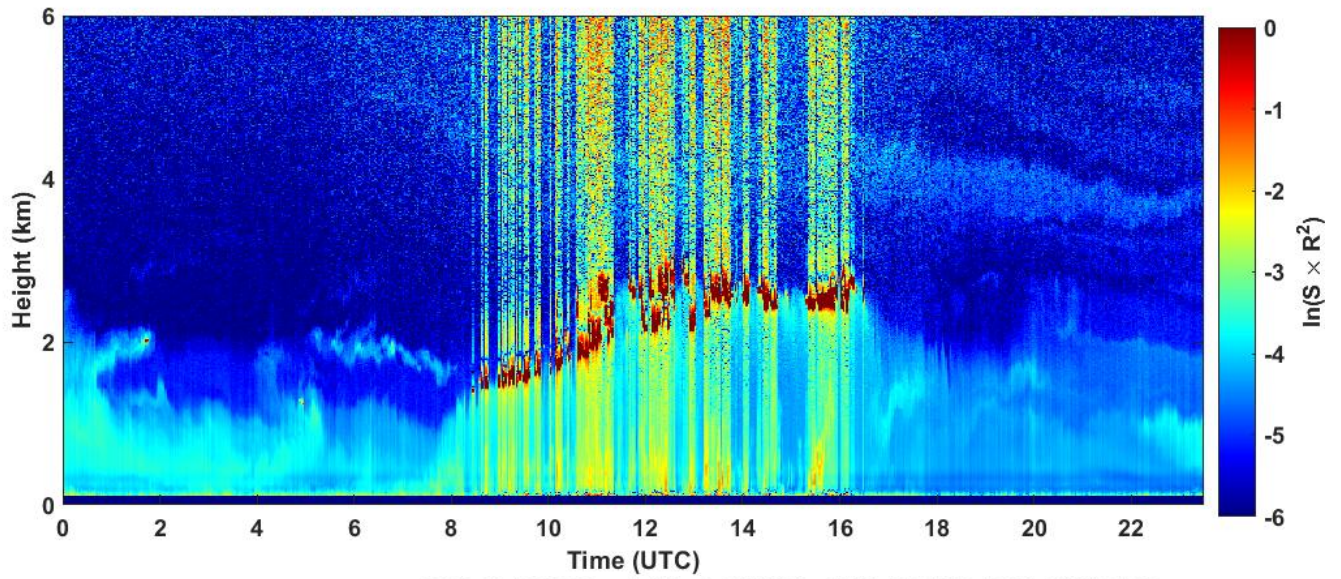
2024-09-12 RCS quick look CHM15k - ILVA LIDAR3 AGGLOMERATO
