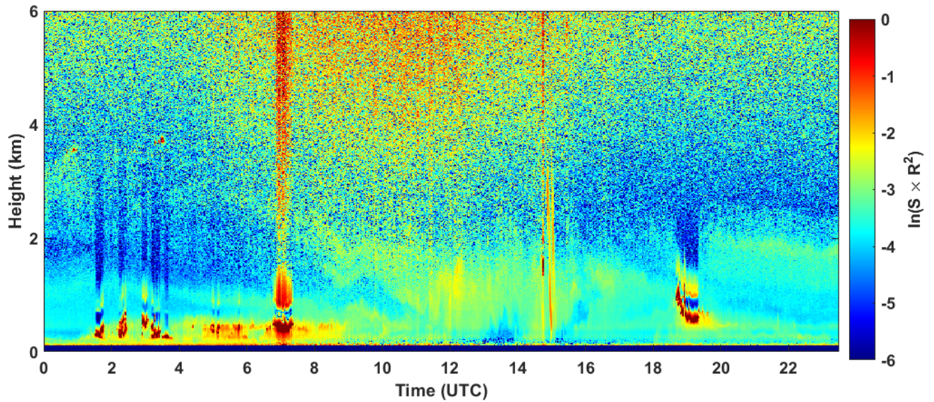
2024-09-08 RCS quick look CHM15k - ILVA LIDAR2 PARCHI
