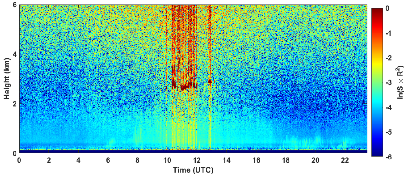
2024-09-02 RCS quick look CHM15k - ILVA LIDAR2 PARCHI
