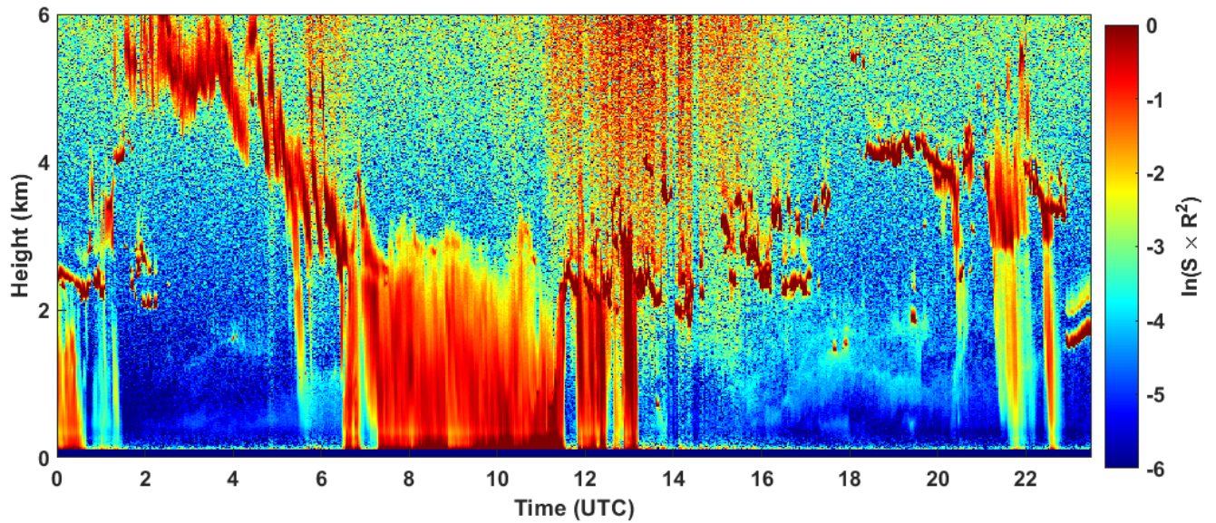
2024-09-18 RCS quick look CHM15k - ILVA LIDAR2 PARCHI
