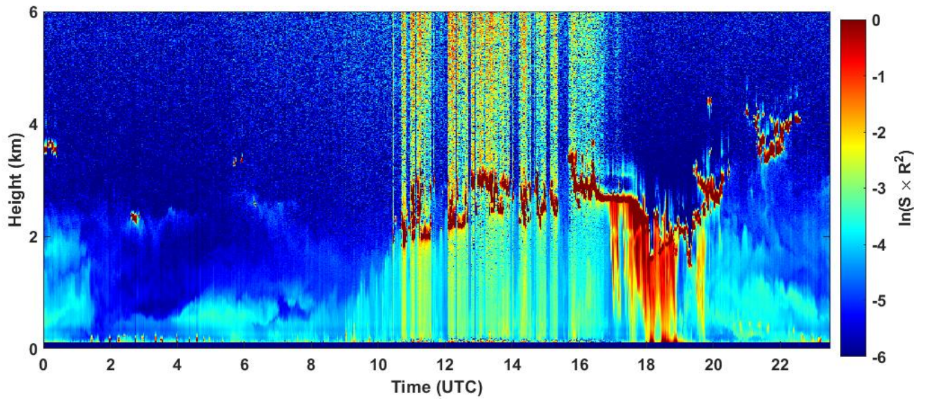
2024-09-14 RCS quick look CHM15k - ILVA LIDAR3 AGGLOMERATO
