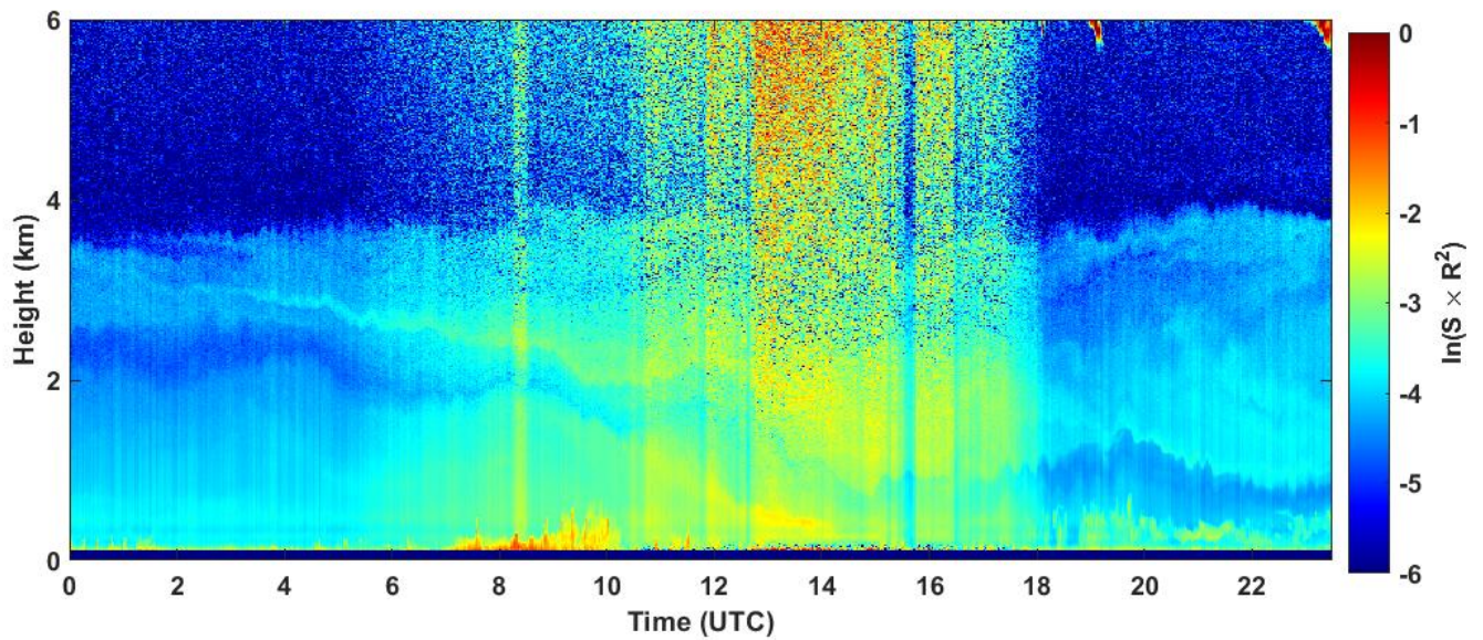
2024-09-02 RCS quick look CHM15k - ILVA LIDAR3 AGGLOMERATO
