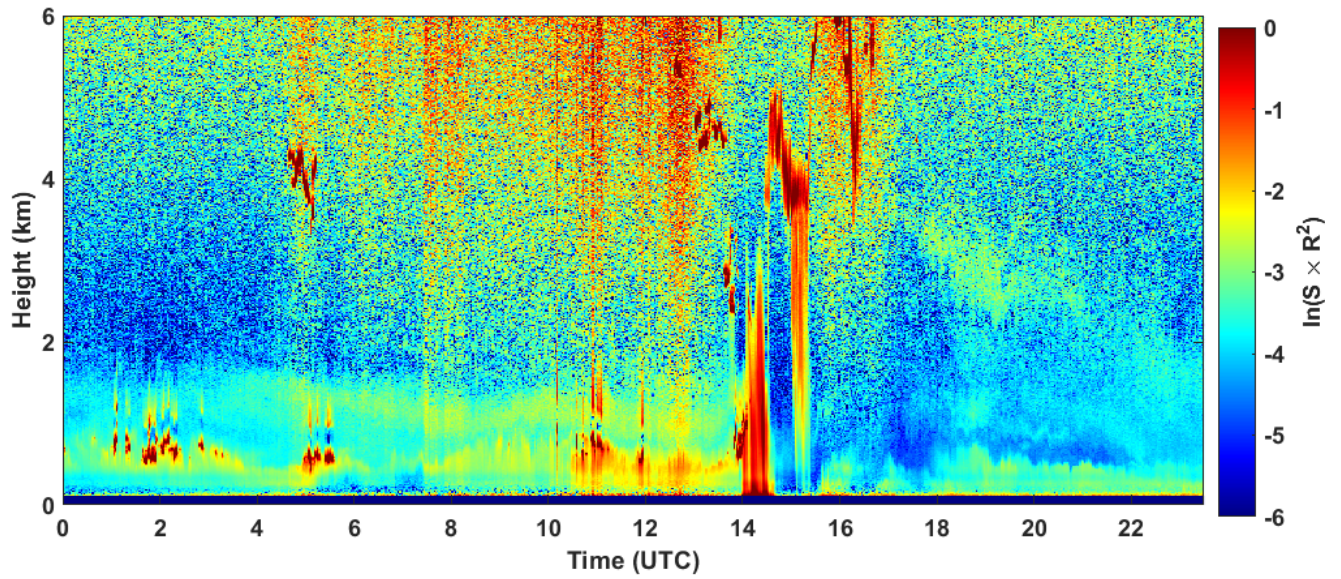
2024-09-06 RCS quick look CHM15k - ILVA LIDAR2 PARCHI
