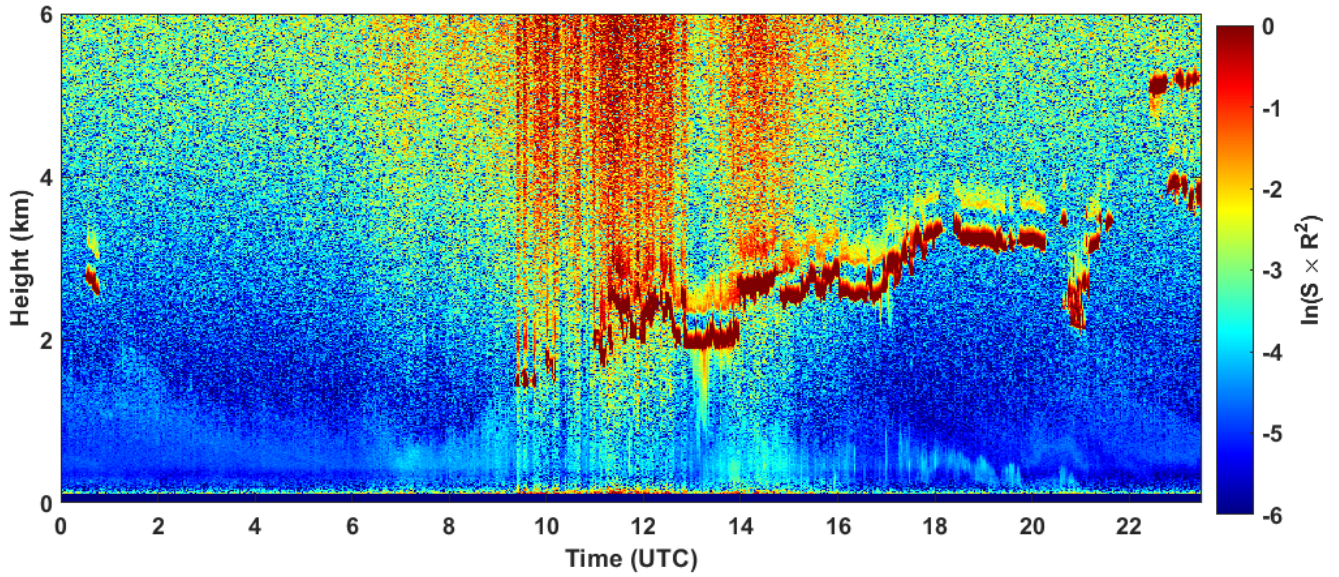
2024-09-16 RCS quick look CHM15k - ILVA LIDAR2 PARCHI
