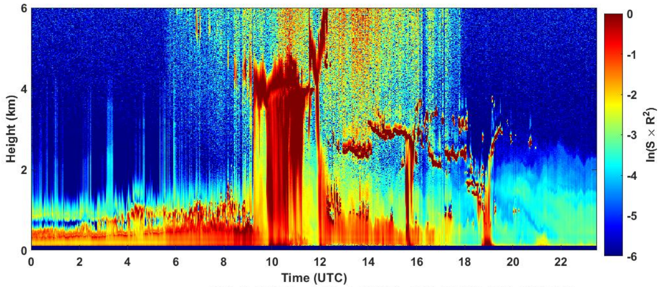
2024-09-10 RCS quick look CHM15k - ILVA LIDAR3 AGGLOMERATO
