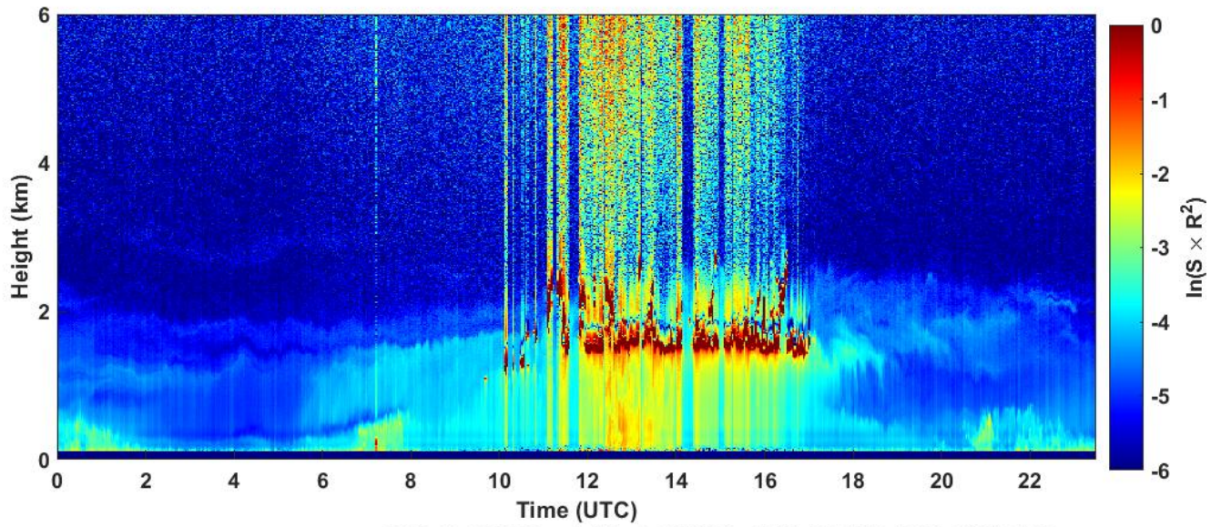
2024-09-22 RCS quick look CHM15k - ILVA LIDAR3 AGGLOMERATO
