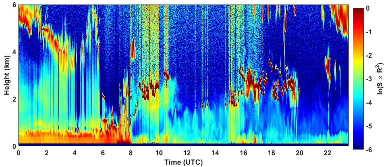
2024-03-12 RCS quick look CHM15k - ILVA LIDAR3 AGGLOMERATO
