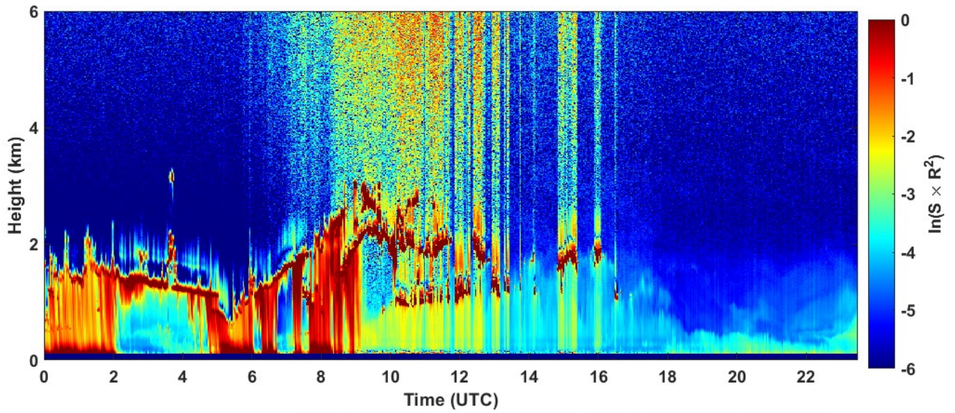
2024-03-20 RCS quick look CHM15k - ILVA LIDAR3 AGGLOMERATO
