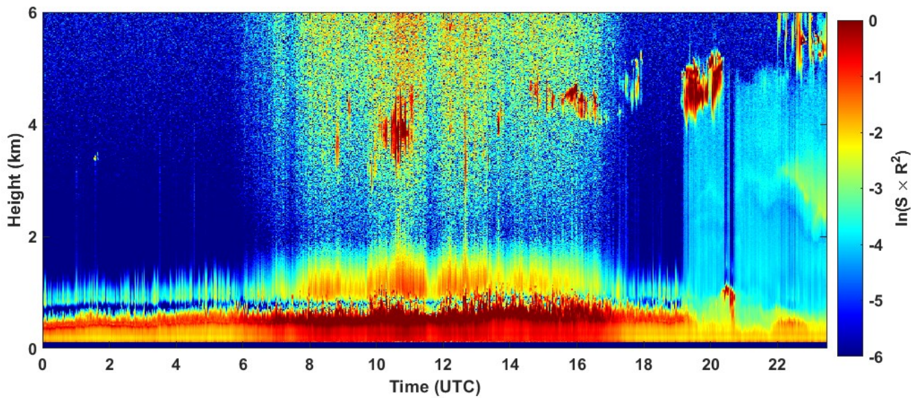
2024-03-10 RCS quick look CHM15k - ILVA LIDAR3 AGGLOMERATO
