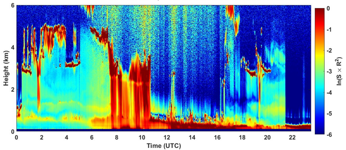
2024-03-26 RCS quick look CHM15k - ILVA LIDAR3 AGGLOMERATO
