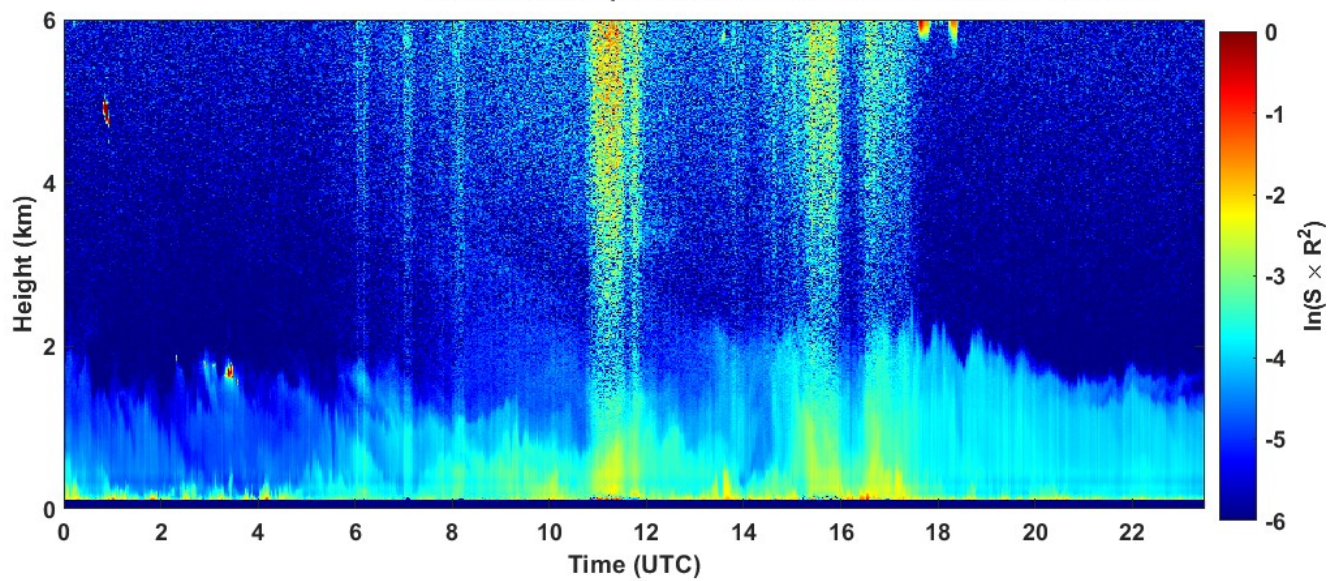
2024-03-28 RCS quick look CHM15k - ILVA LIDAR3 AGGLOMERATO
