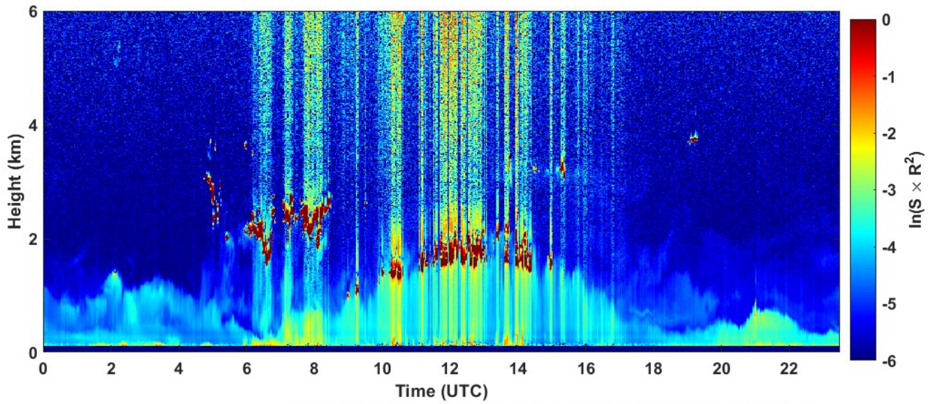
2024-03-14 RCS quick look CHM15k - ILVA LIDAR3 AGGLOMERATO
