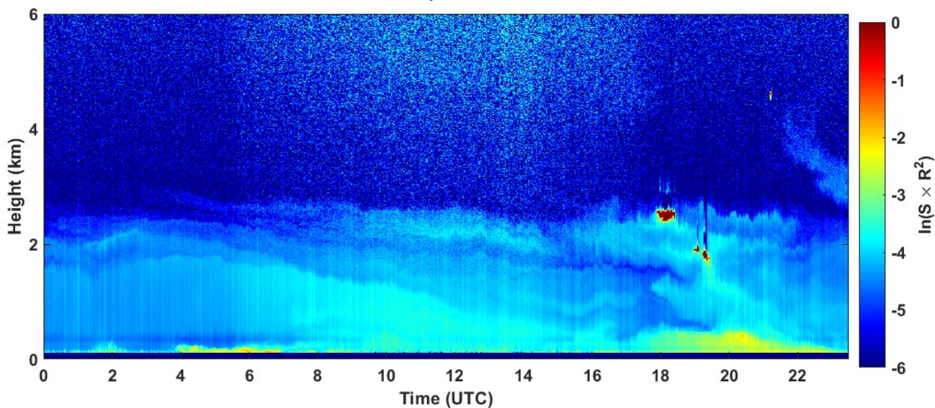
2024-03-24 RCS quick look CHM15k - ILVA LIDAR3 AGGLOMERATO
