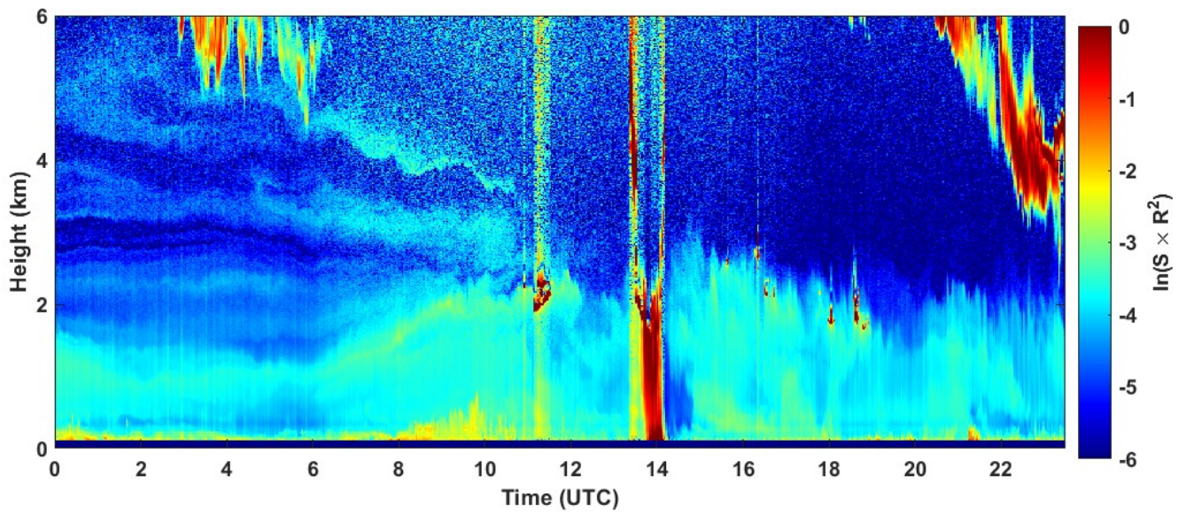
2024-03-06 RCS quick look CHM15k - ILVA LIDAR3 AGGLOMERATO
