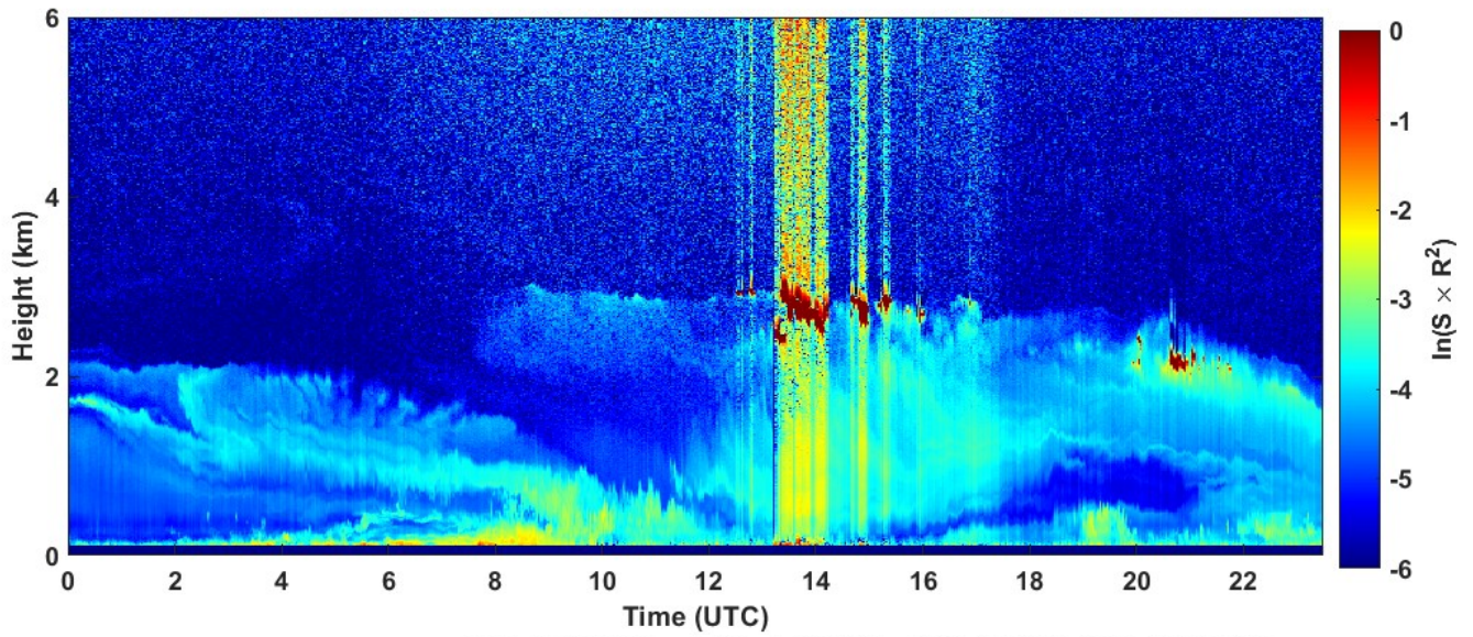
2024-03-16 RCS quick look CHM15k - ILVA LIDAR3 AGGLOMERATO
