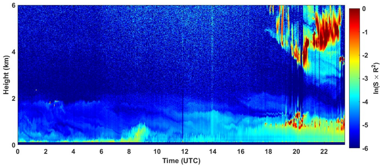
2024-03-08 RCS quick look CHM15k - ILVA LIDAR3 AGGLOMERATO
