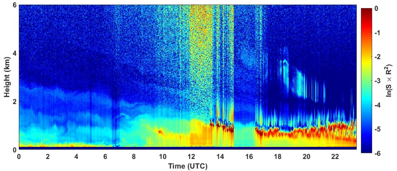
2024-03-04 RCS quick look CHM15k - ILVA LIDAR3 AGGLOMERATO
