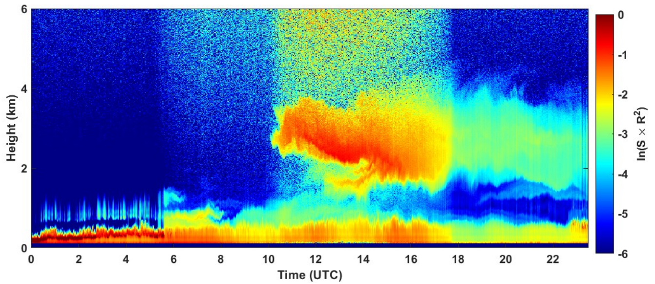
2024-03-30 RCS quick look CHM15k - ILVA LIDAR3 AGGLOMERATO
