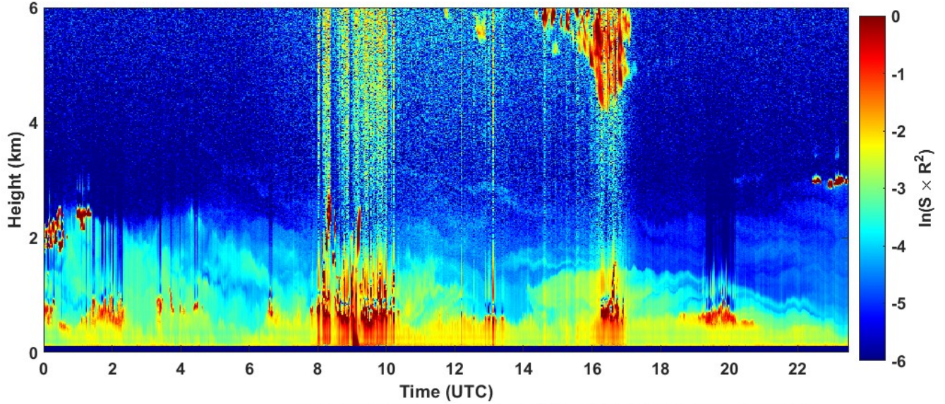
2024-03-02 RCS quick look CHM15k - ILVA LIDAR3 AGGLOMERATO
