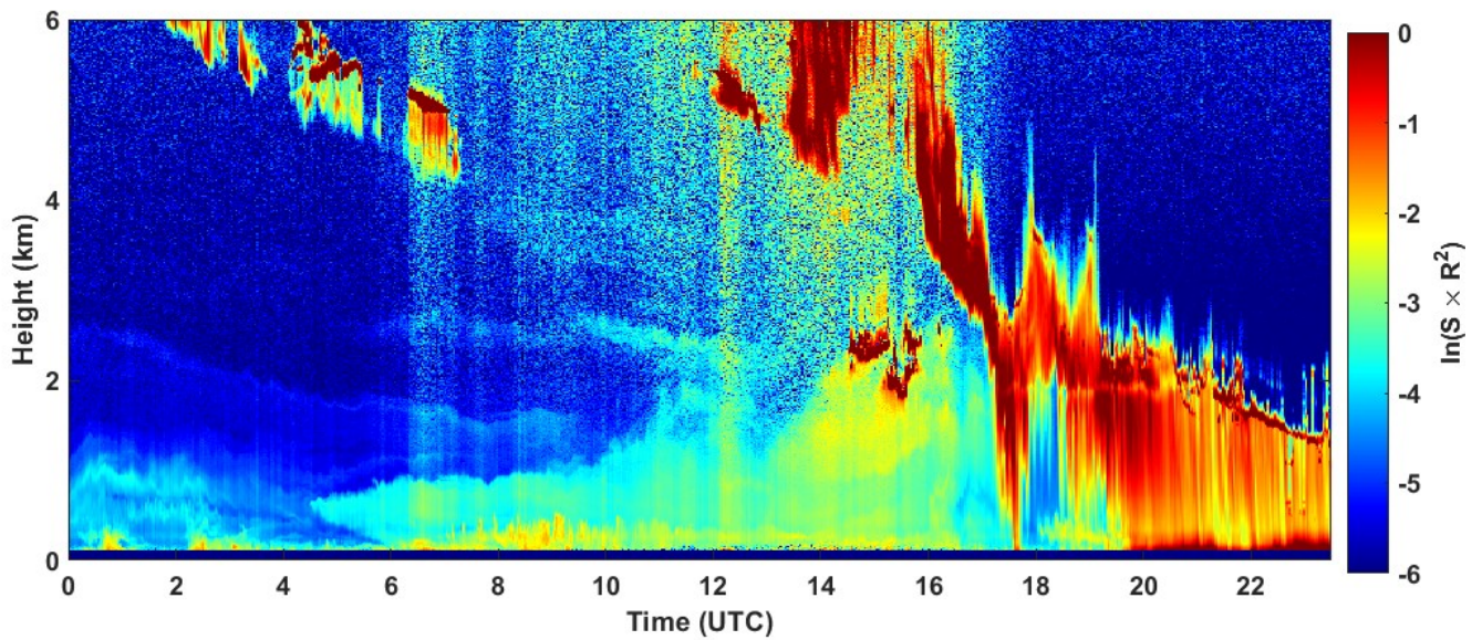
2024-03-18 RCS quick look CHM15k - ILVA LIDAR3 AGGLOMERATO
