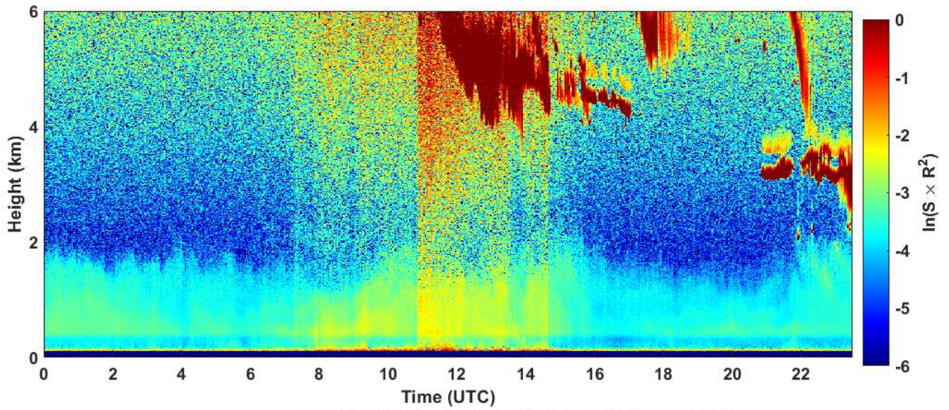
2024-01-20 RCS quick look CHM15k - ILVA LIDAR2 PARCHI
