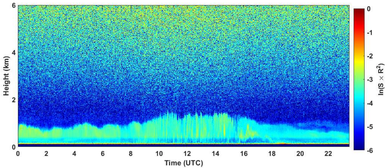
2024-01-22 RCS quick look CHM15k - ILVA LIDAR2 PARCHI
