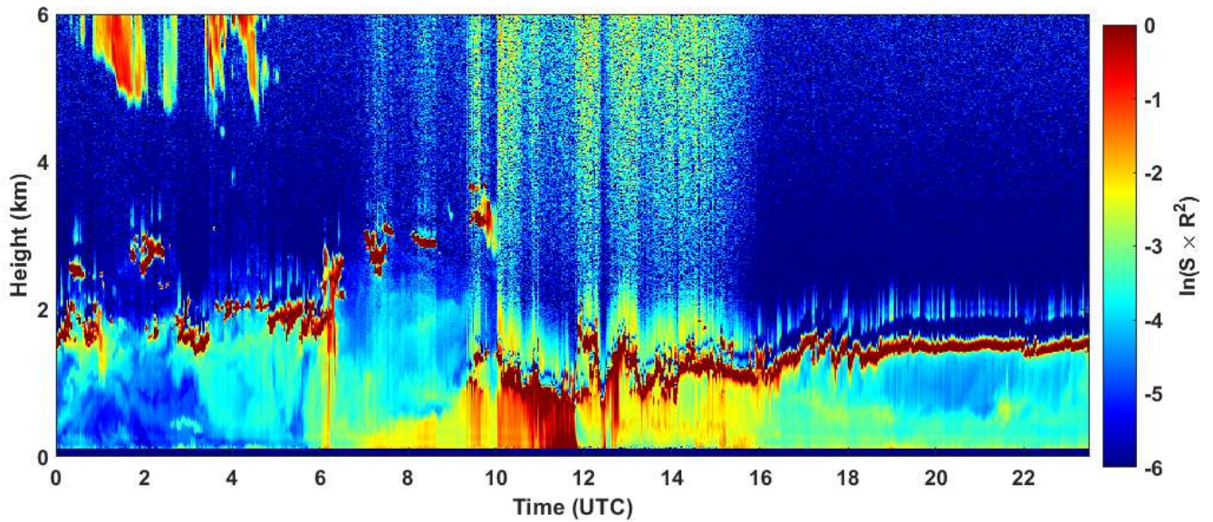
2024-01-10 RCS quick look CHM15k - ILVA LIDAR3 AGGLOMERATO
