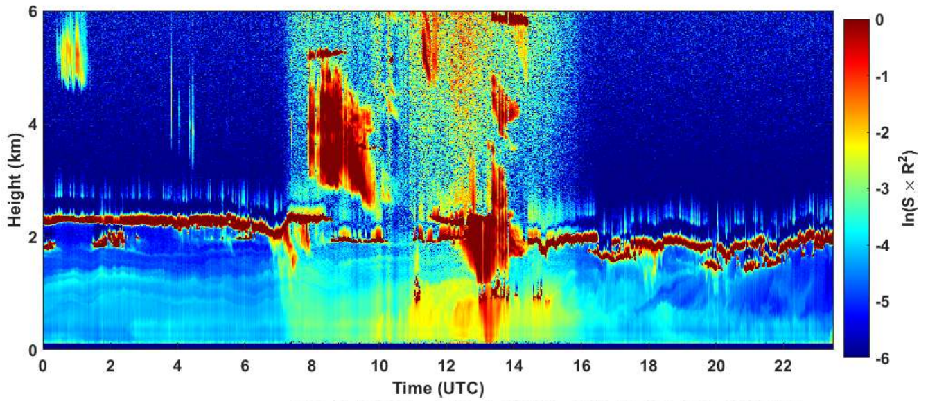
2024-01-12 RCS quick look CHM15k - ILVA LIDAR3 AGGLOMERATO
