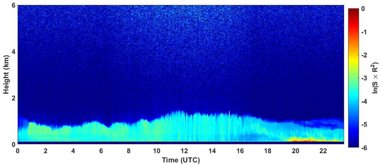
2024-01-22 RCS quick look CHM15k - ILVA LIDAR3 AGGLOMERATO
