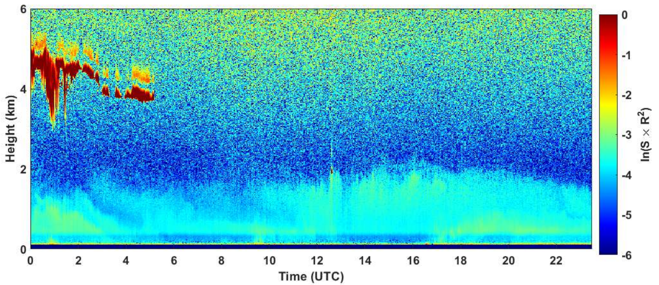
2024-01-04 RCS quick look CHM15k - ILVA LIDAR2 PARCHI
