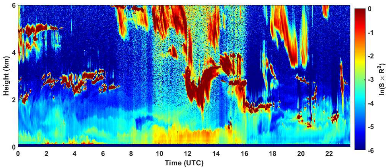
2024-01-08 RCS quick look CHM15k - ILVA LIDAR3 AGGLOMERATO
