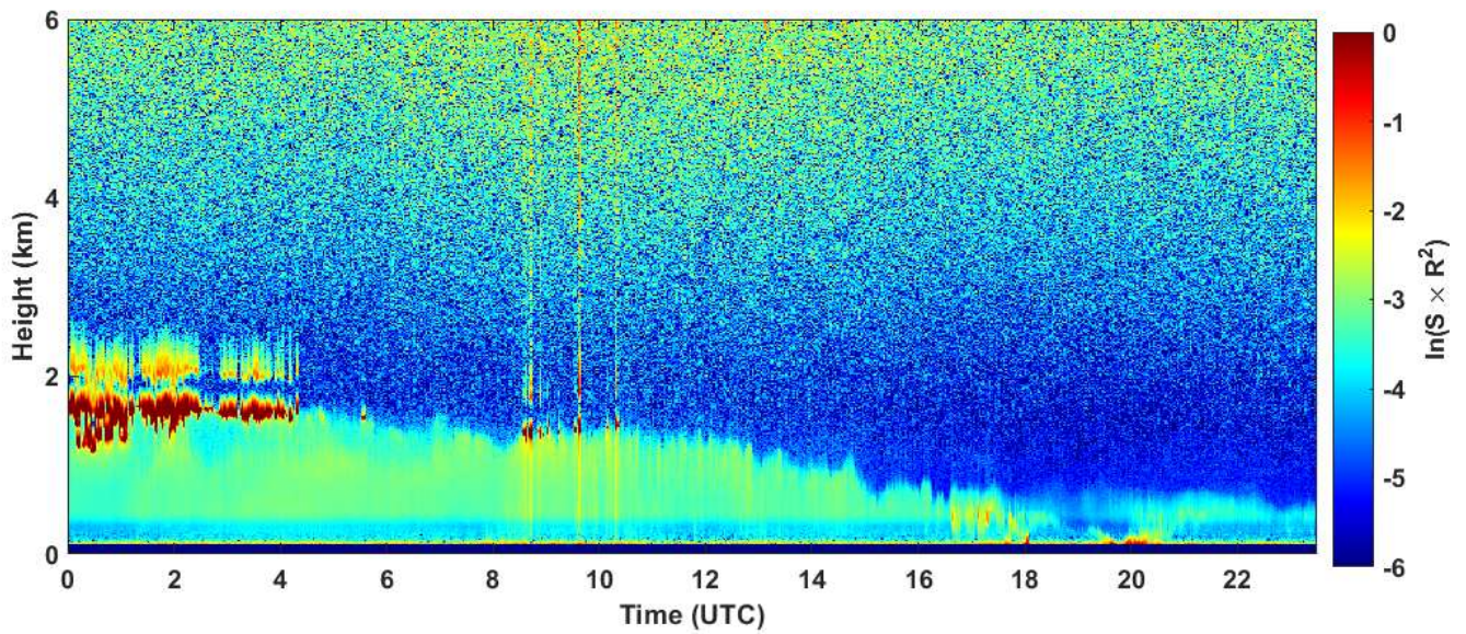
2024-01-30 RCS quick look CHM15k - ILVA LIDAR2 PARCHI
