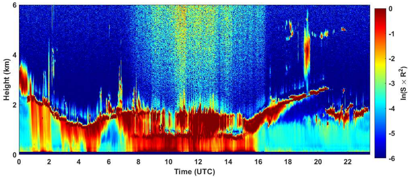
2024-01-20 RCS quick look CHM15k - ILVA LIDAR3 AGGLOMERATO
