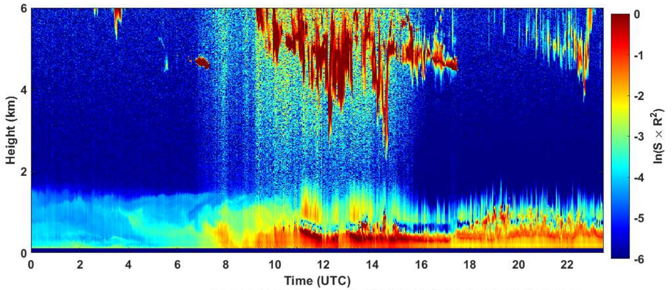
2024-01-06 RCS quick look CHM15k - ILVA LIDAR3 AGGLOMERATO
