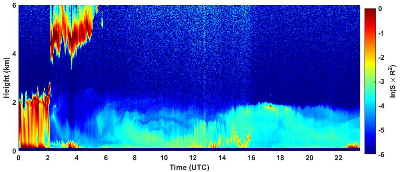
2024-01-02 RCS quick look CHM15k - ILVA LIDAR3 AGGLOMERATO
