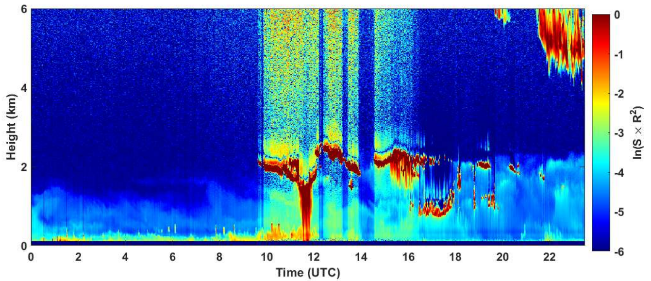
2024-01-14 RCS quick look CHM15k - ILVA LIDAR3 AGGLOMERATO
