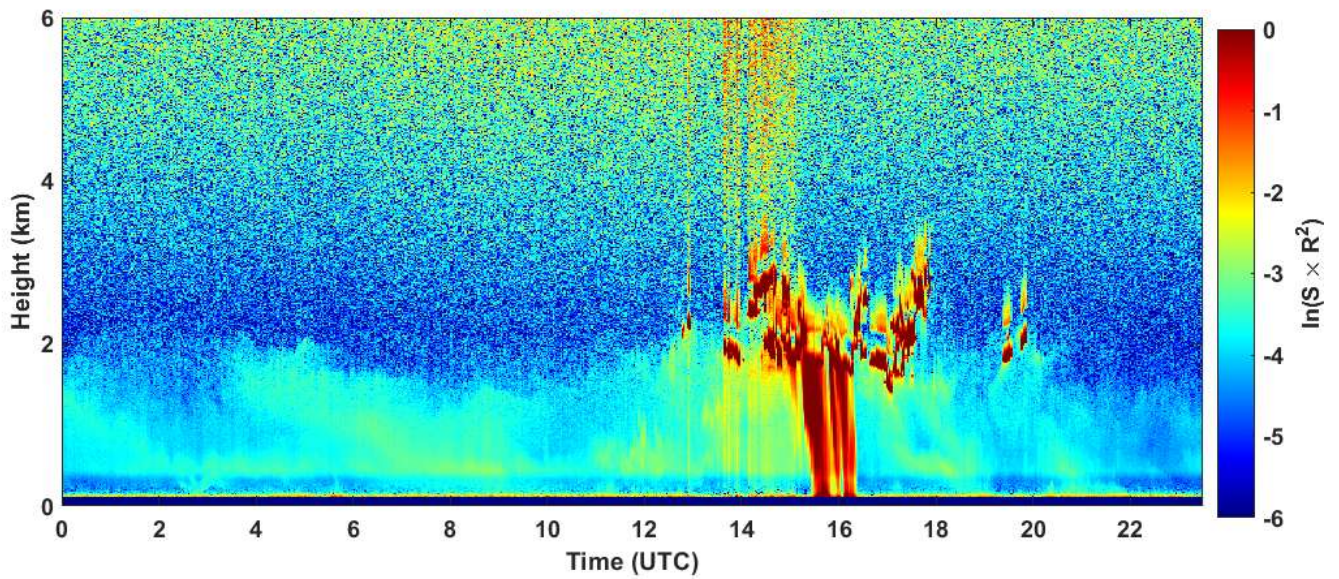
2024-01-16 RCS quick look CHM15k - ILVA LIDAR2 PARCHI
