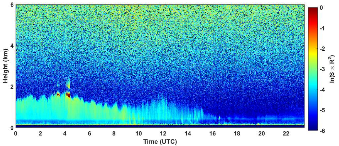
2024-01-24 RCS quick look CHM15k - ILVA LIDAR2 PARCHI
