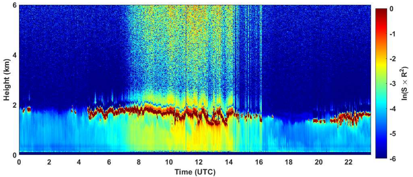
2024-01-30 RCS quick look CHM15k - ILVA LIDAR3 AGGLOMERATO
