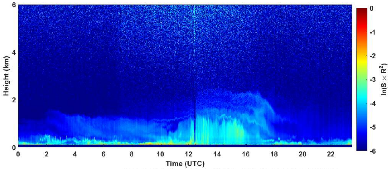
2024-01-26 RCS quick look CHM15k - ILVA LIDAR3 AGGLOMERATO
