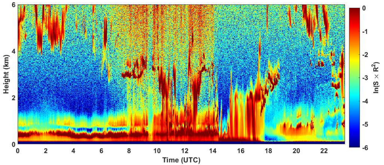
2024-01-06 RCS quick look CHM15k - ILVA LIDAR2 PARCHI
