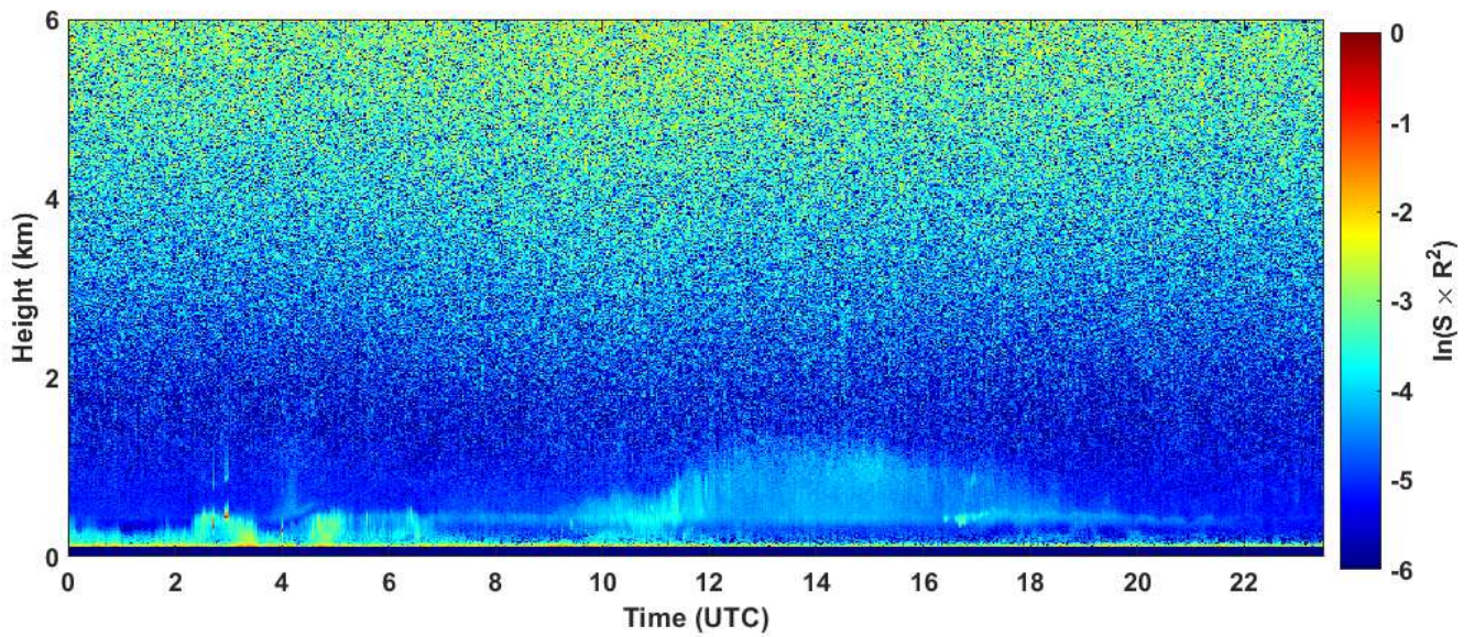
2024-01-26 RCS quick look CHM15k - ILVA LIDAR2 PARCHI
