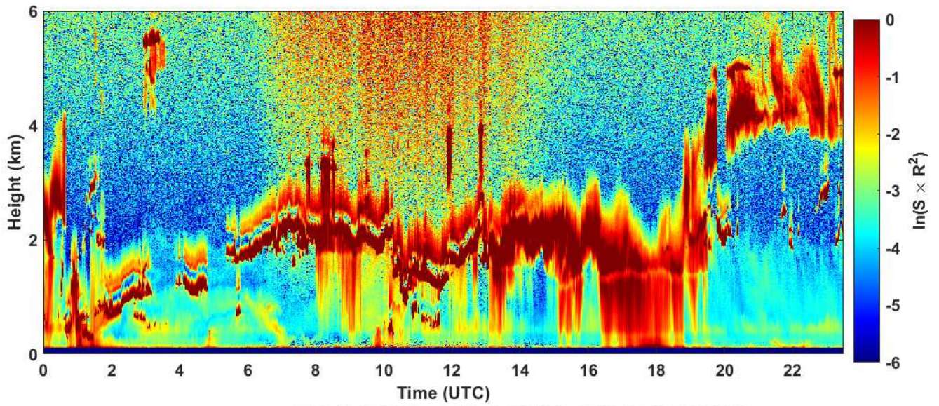
2024-01-08 RCS quick look CHM15k - ILVA LIDAR2 PARCHI
