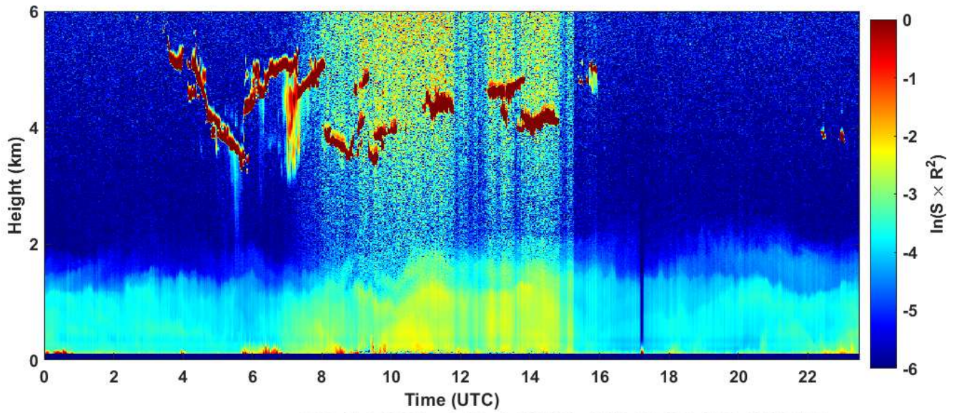
2024-01-04 RCS quick look CHM15k - ILVA LIDAR3 AGGLOMERATO
