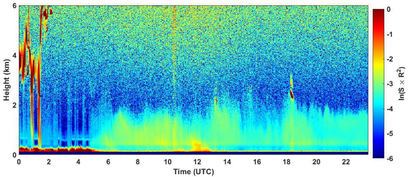
2024-01-18 RCS quick look CHM15k - ILVA LIDAR2 PARCHI
