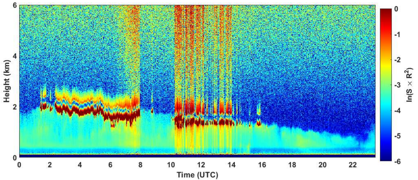
2024-01-14 RCS quick look CHM15k - ILVA LIDAR2 PARCHI
