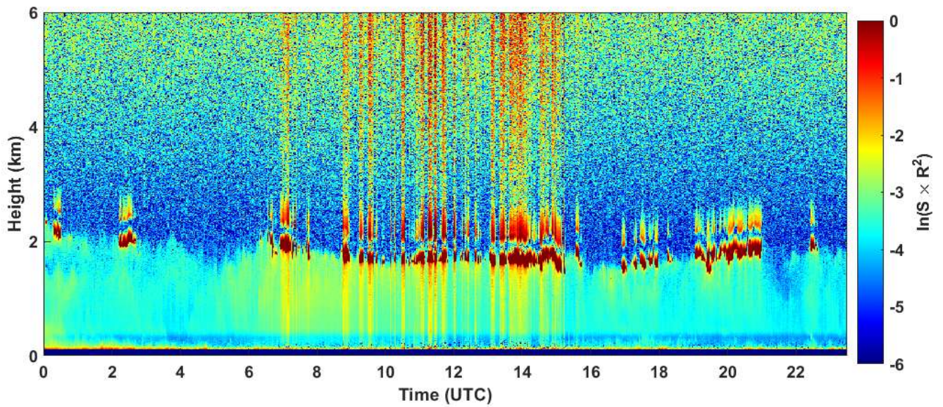
2024-01-28 RCS quick look CHM15k - ILVA LIDAR2 PARCHI
