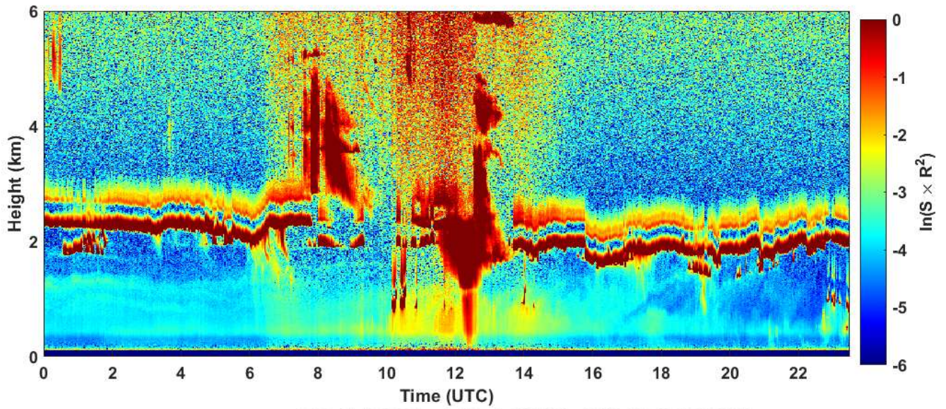
2024-01-12 RCS quick look CHM15k - ILVA LIDAR2 PARCHI
