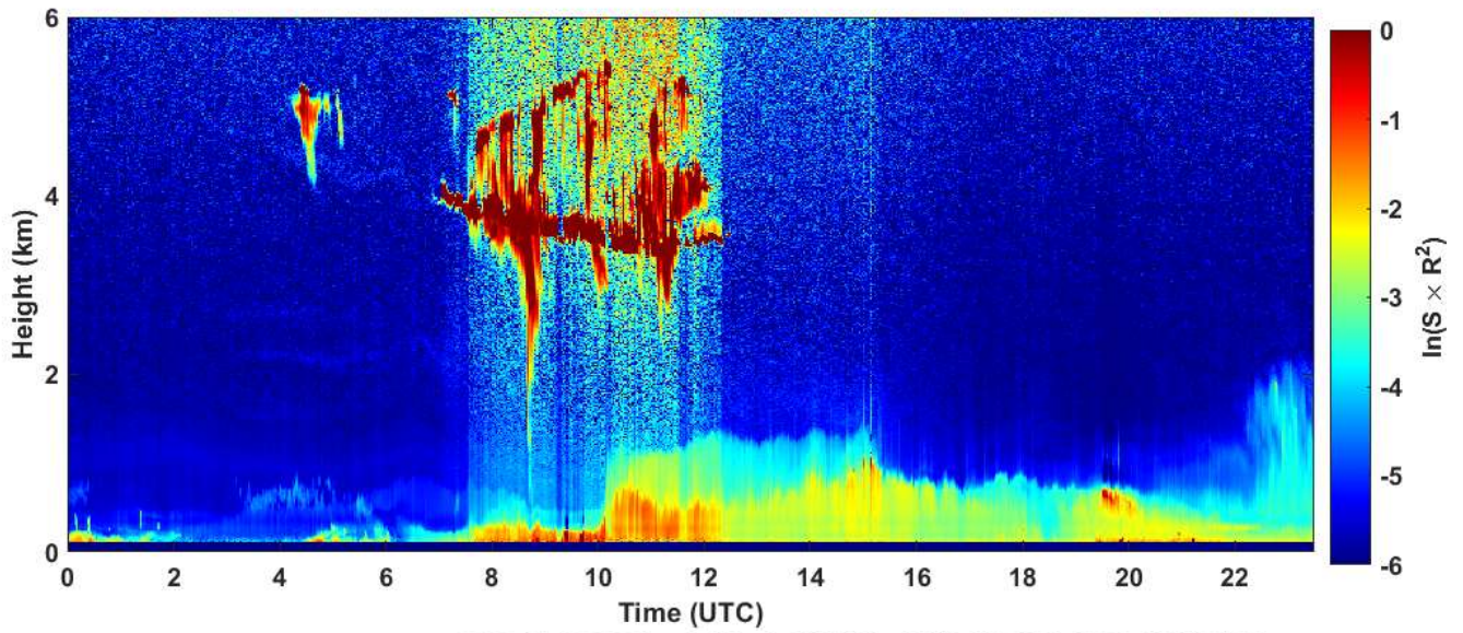
2024-01-28 RCS quick look CHM15k - ILVA LIDAR3 AGGLOMERATO
