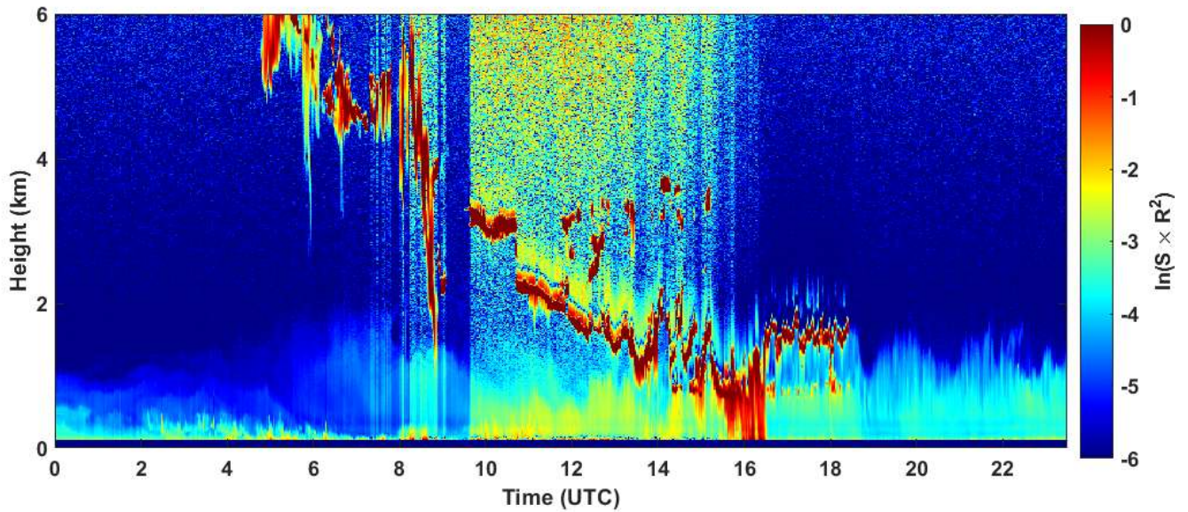
2024-01-24 RCS quick look CHM15k - ILVA LIDAR3 AGGLOMERATO
