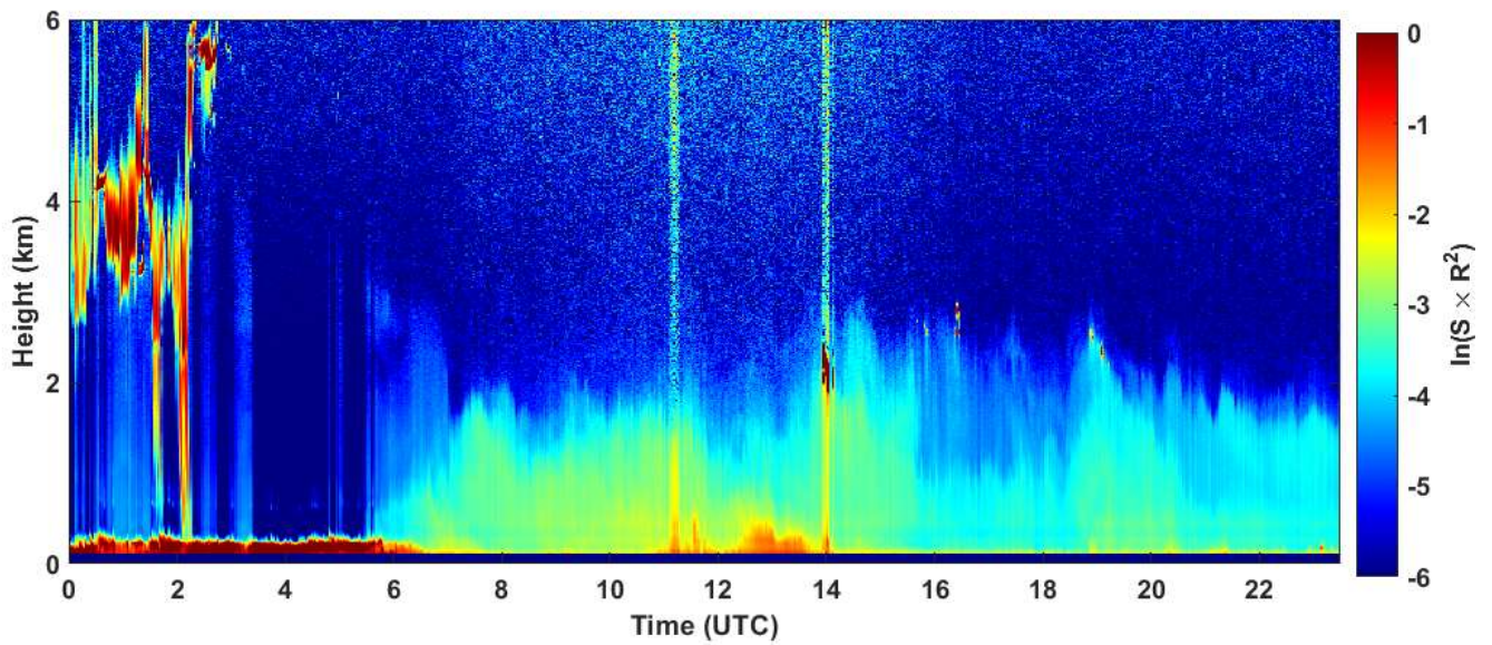
2024-01-18 RCS quick look CHM15k - ILVA LIDAR3 AGGLOMERATO
