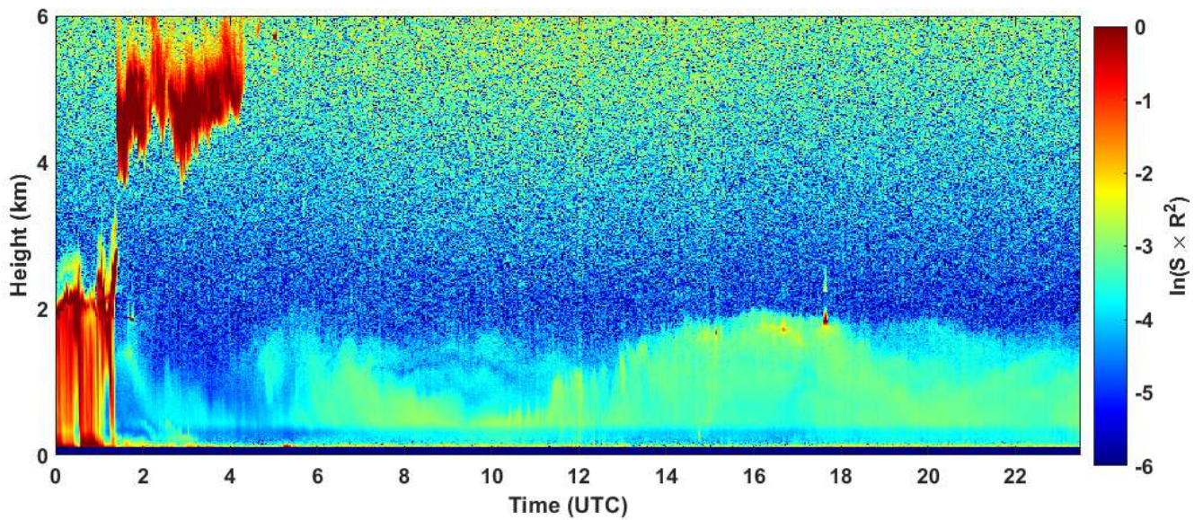
2024-01-02 RCS quick look CHM15k - ILVA LIDAR2 PARCHI
