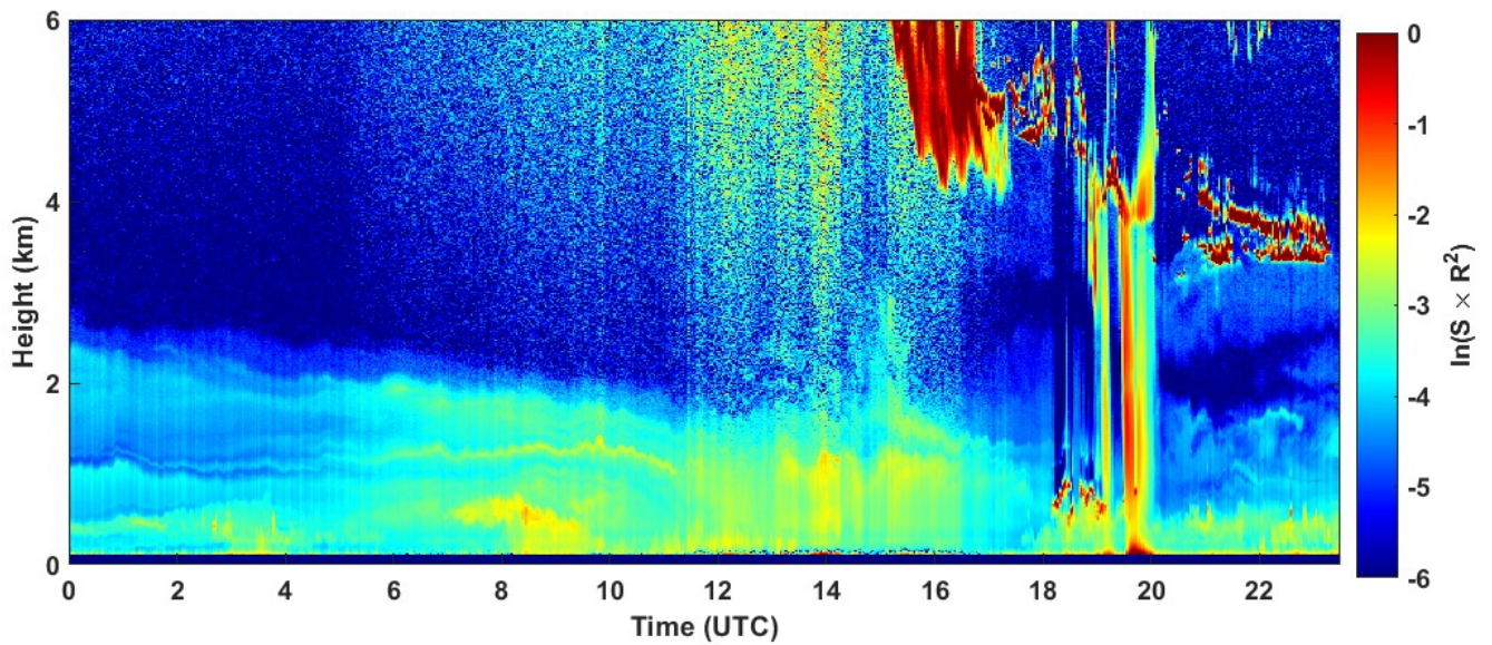
2023-09-16 RCS quick look CHM15k - ILVA LIDAR3 AGGLOMERATO
