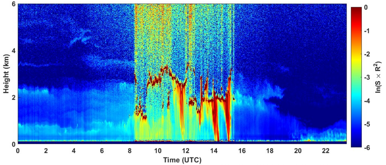
2023-09-02 RCS quick look CHM15k - ILVA LIDAR3 AGGLOMERATO
