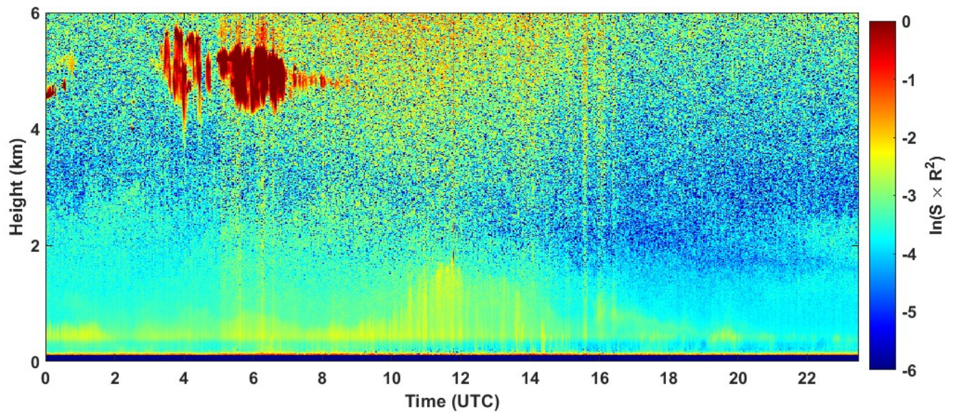
2023-09-28 RCS quick look CHM15k - ILVA LIDAR2 PARCHI
