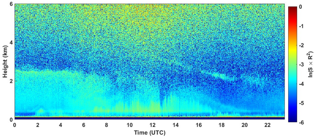
2023-09-10 RCS quick look CHM15k - ILVA LIDAR2 PARCHI
