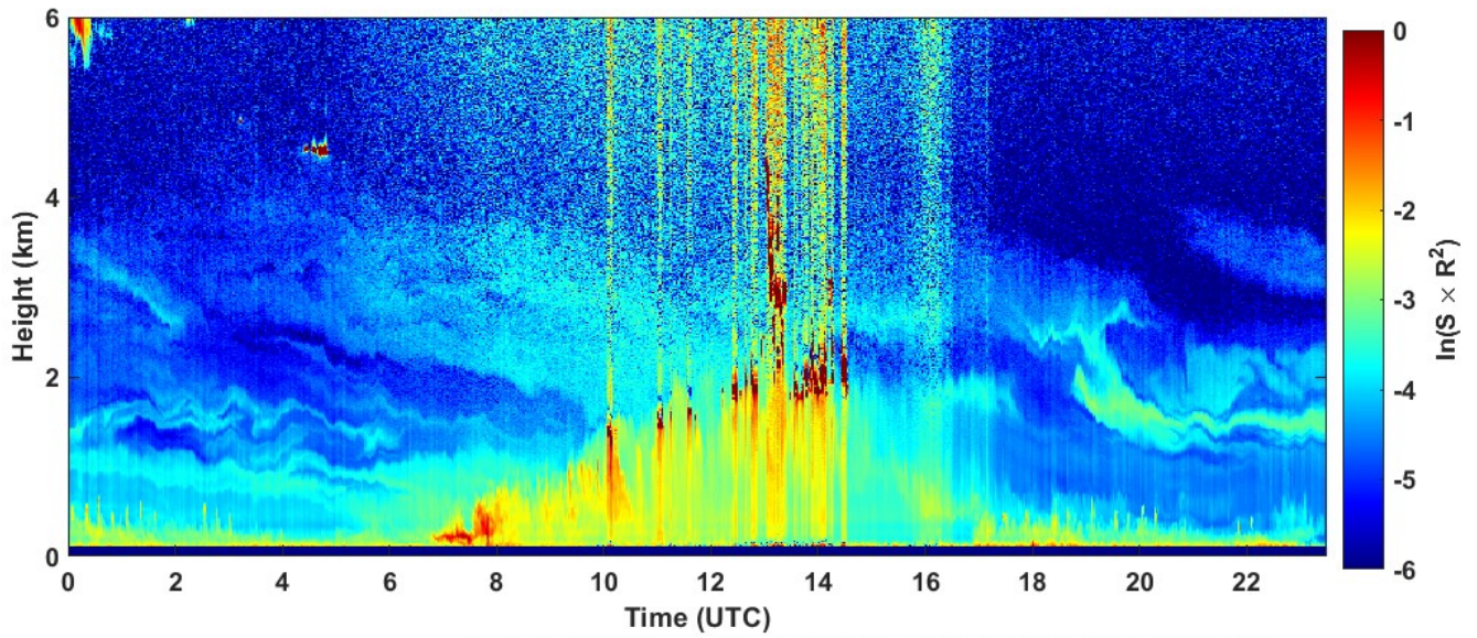
2023-09-18 RCS quick look CHM15k - ILVA LIDAR3 AGGLOMERATO
