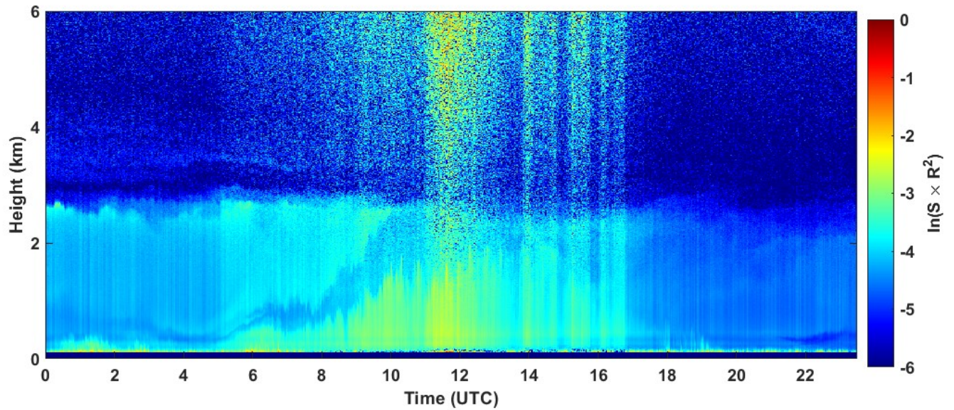
2023-09-10 RCS quick look CHM15k - ILVA LIDAR3 AGGLOMERATO
