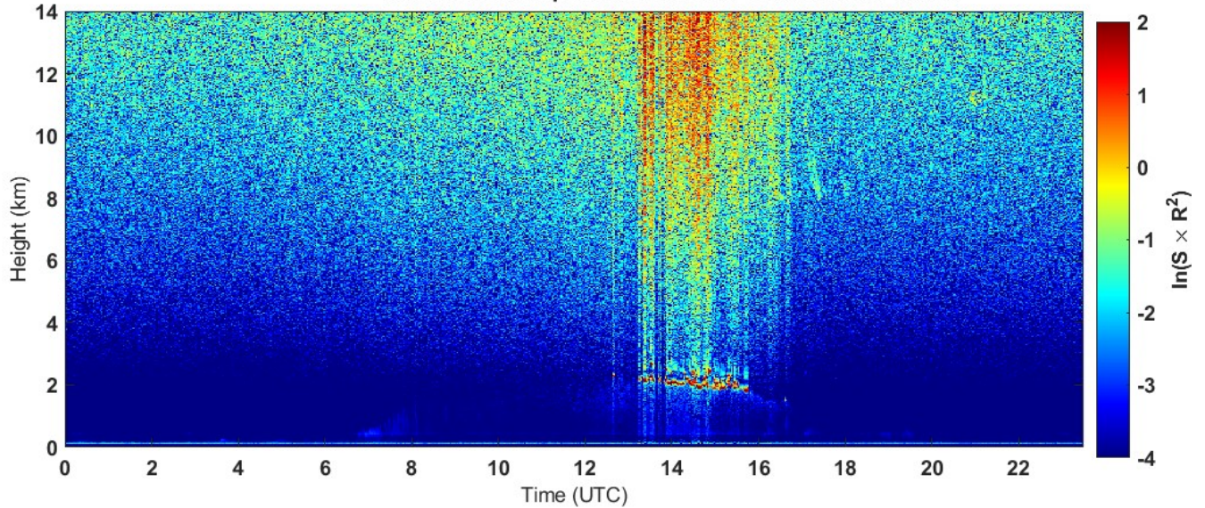
2023-09-02 RCS quick look CHM15k - ILVA LIDAR2 PARCHI
