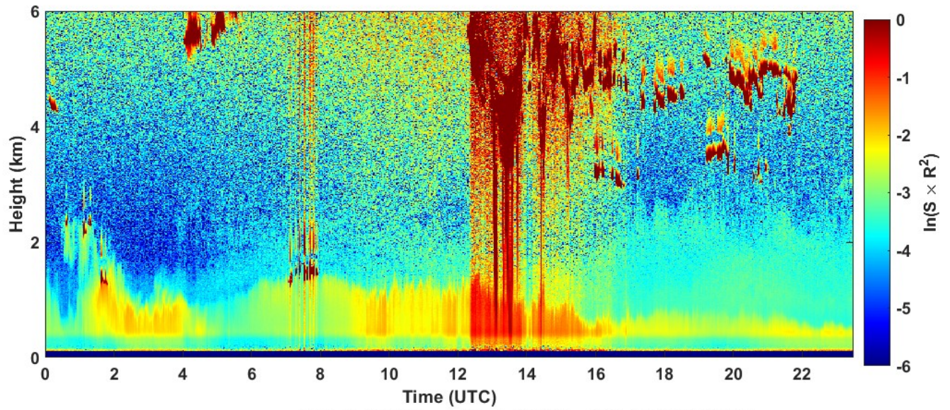
2023-09-06 RCS quick look CHM15k - ILVA LIDAR2 PARCHI
