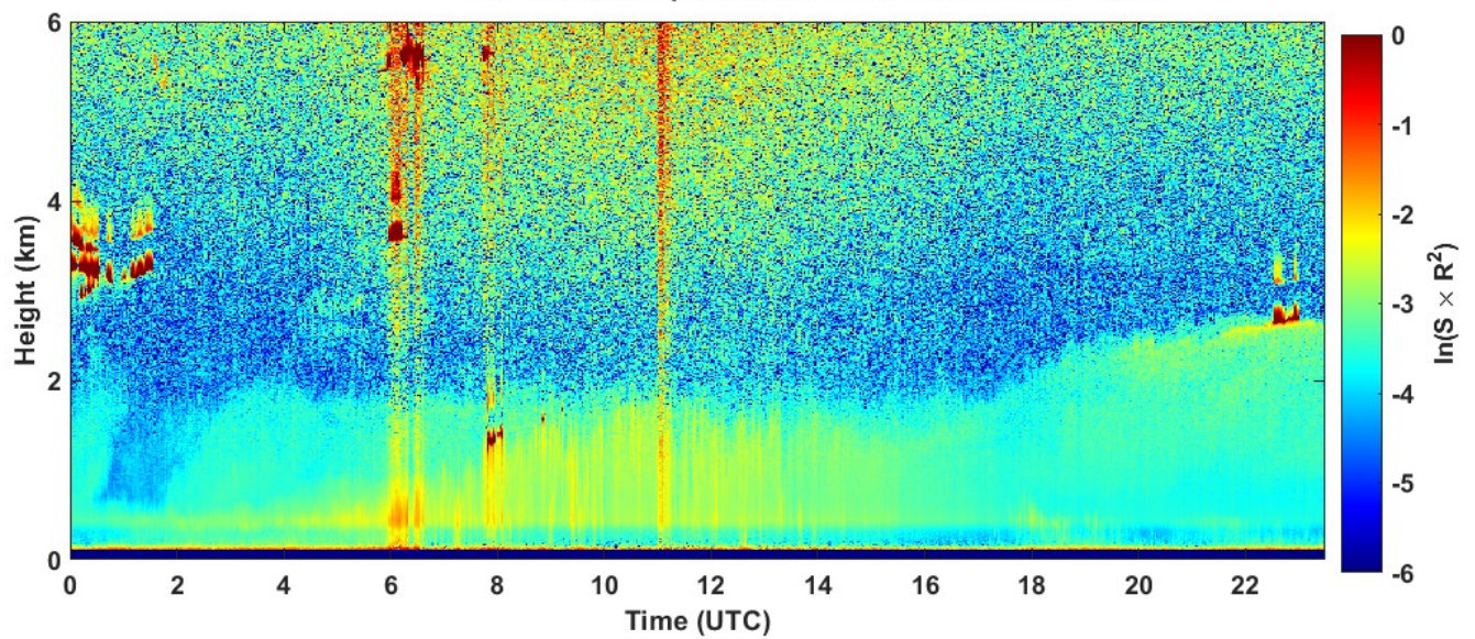
2023-09-08 RCS quick look CHM15k - ILVA LIDAR2 PARCHI
