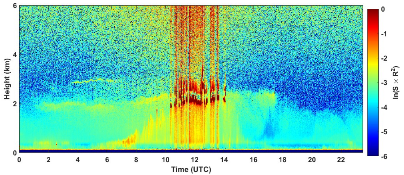
2023-09-30 RCS quick look CHM15k - ILVA LIDAR2 PARCHI
