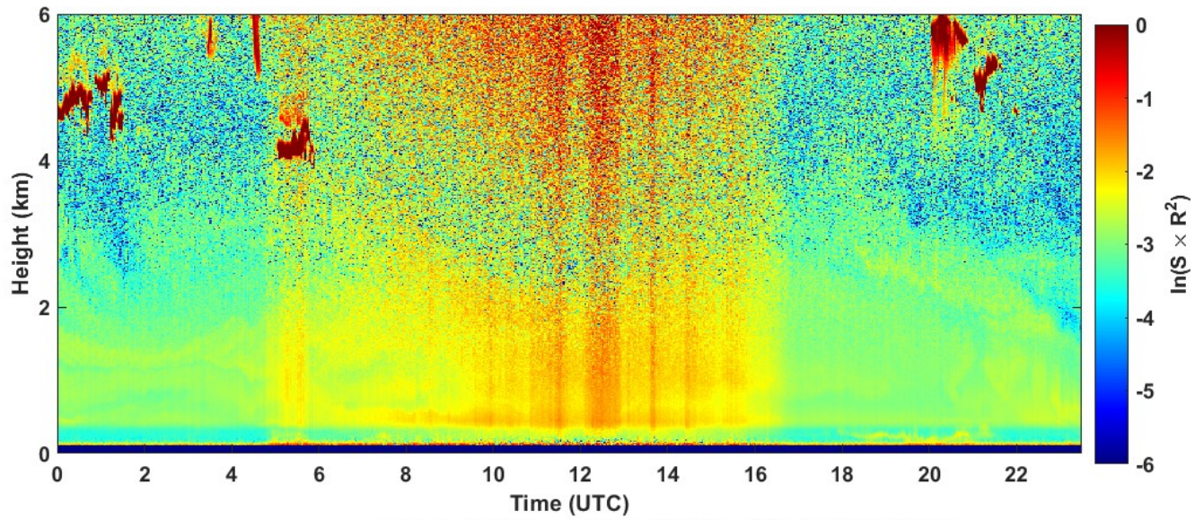
2023-09-20 RCS quick look CHM15k - ILVA LIDAR2 PARCHI
