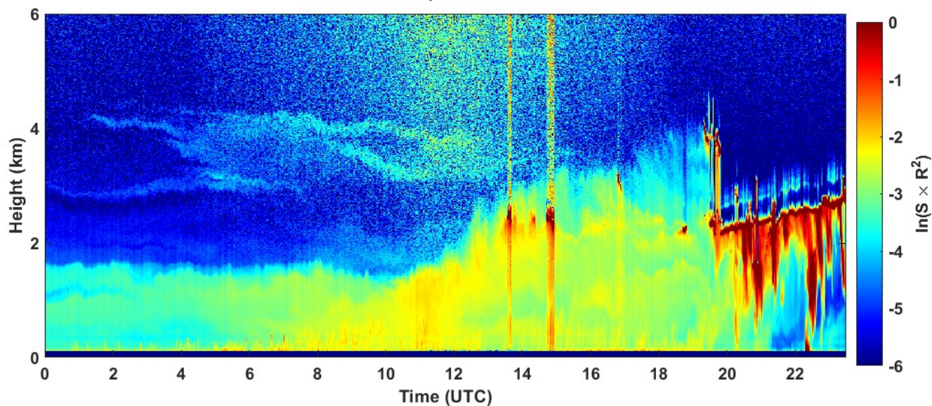
2023-08-08 RCS quick look CHM15k - ILVA LIDAR3 AGGLOMERATO
