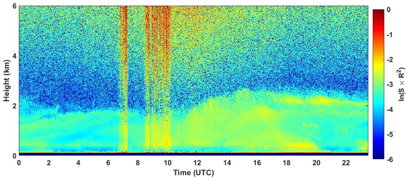
2023-08-02 RCS quick look CHM15k - ILVA LIDAR2 PARCHI
