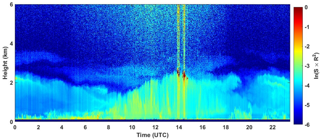
2023-08-16 RCS quick look CHM15k - ILVA LIDAR3 AGGLOMERATO
