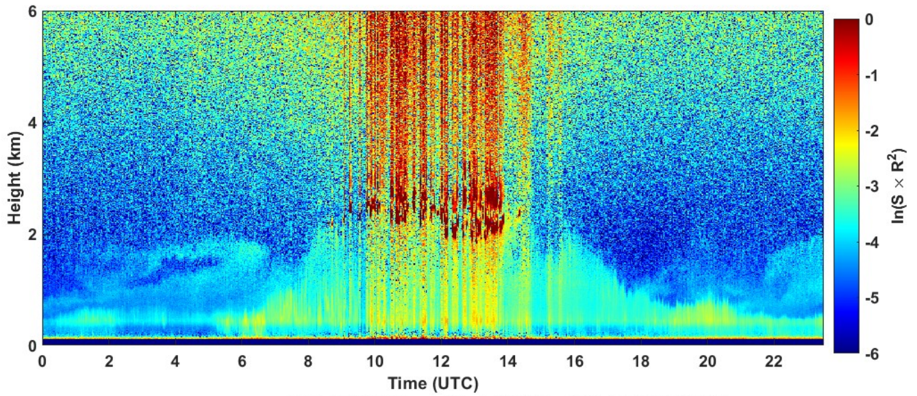
2023-08-12 RCS quick look CHM15k - ILVA LIDAR2 PARCHI
