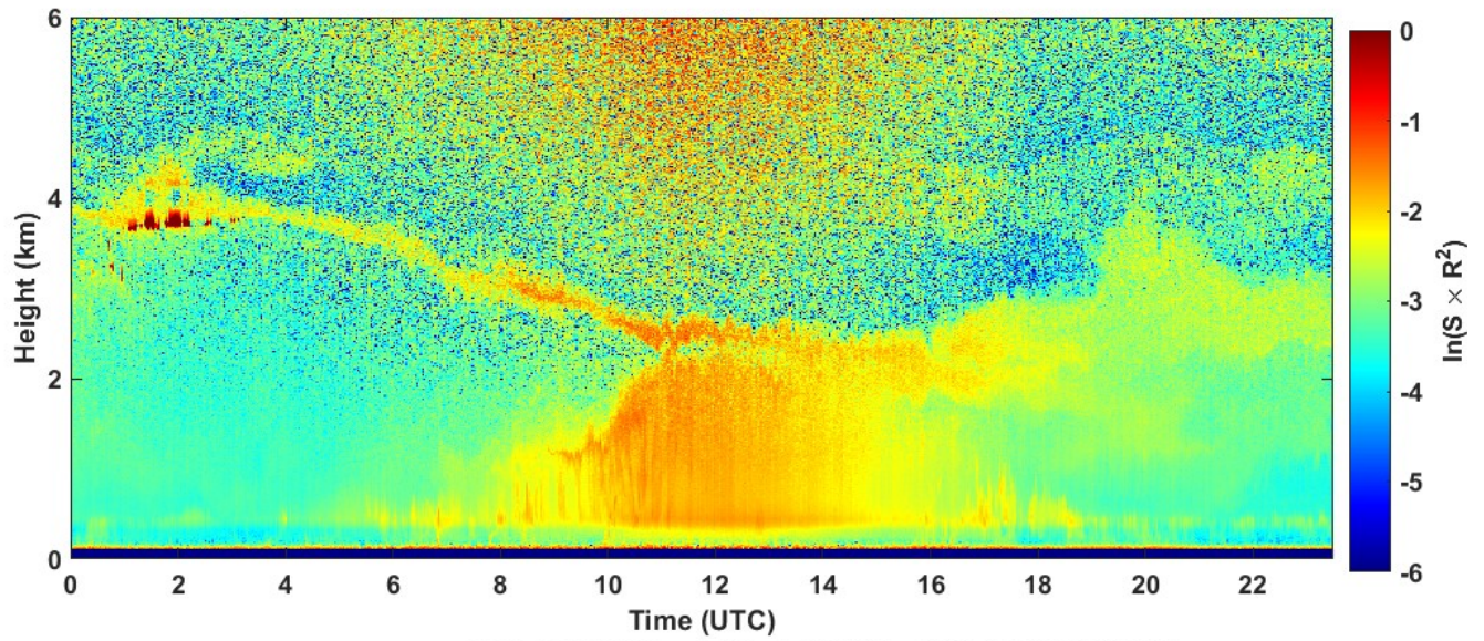
2023-08-24 RCS quick look CHM15k - ILVA LIDAR2 PARCHI
