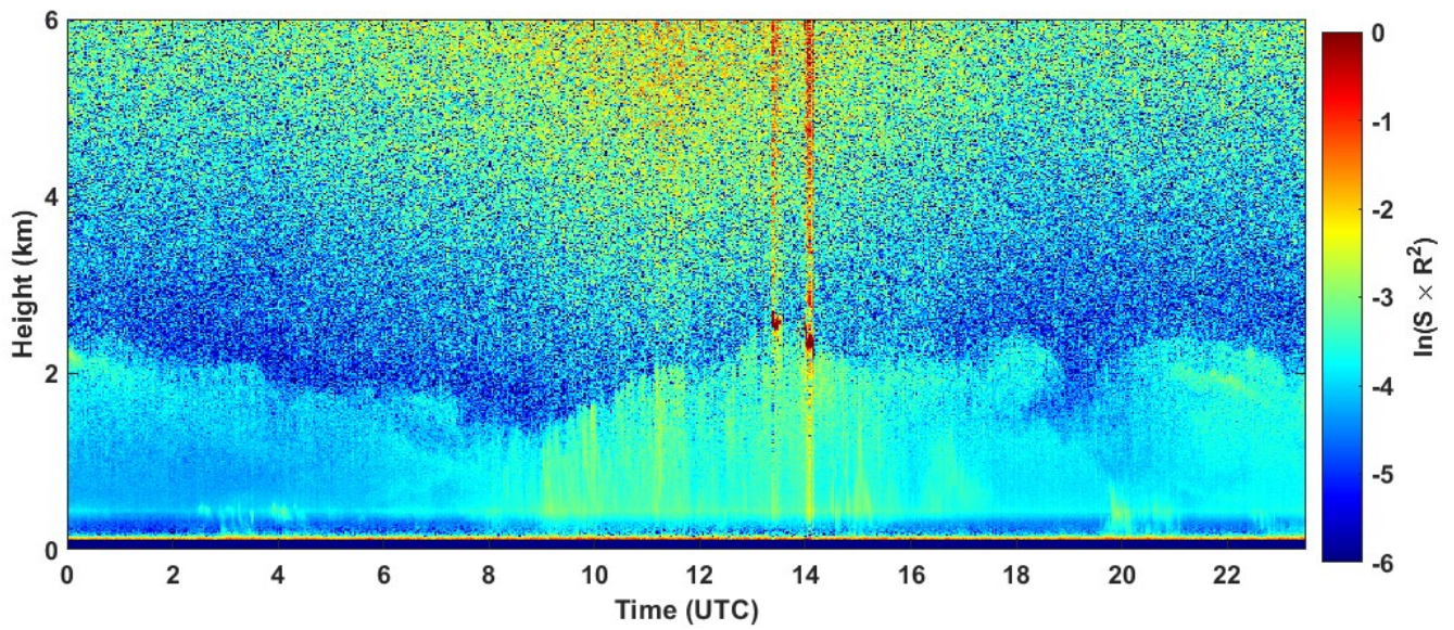
2023-08-16 RCS quick look CHM15k - ILVA LIDAR2 PARCHI
