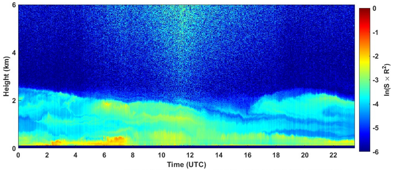
2023-08-04 RCS quick look CHM15k - ILVA LIDAR3 AGGLOMERATO
