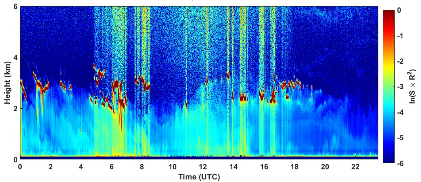
2023-08-30 RCS quick look CHM15k - ILVA LIDAR3 AGGLOMERATO
