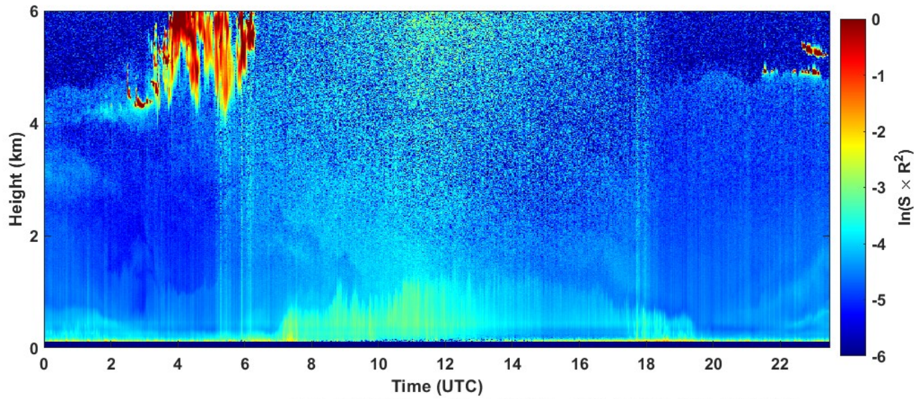
2023-08-22 RCS quick look CHM15k - ILVA LIDAR3 AGGLOMERATO
