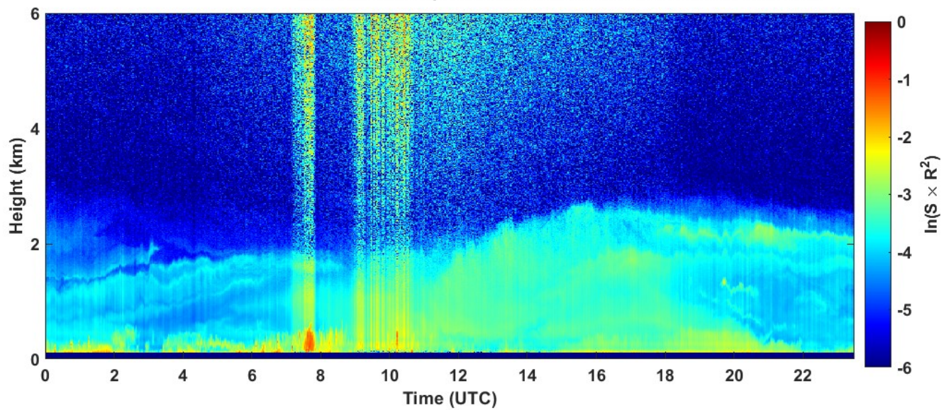
2023-08-02 RCS quick look CHM15k - ILVA LIDAR3 AGGLOMERATO
