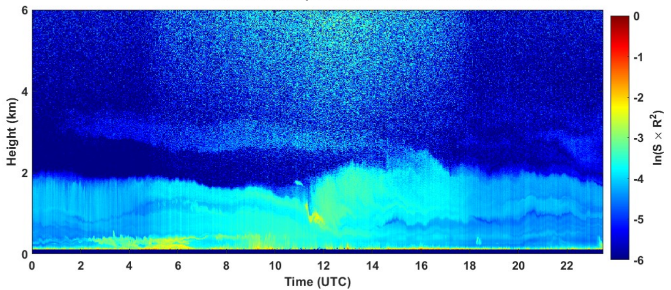
2023-08-26 RCS quick look CHM15k - ILVA LIDAR3 AGGLOMERATO
