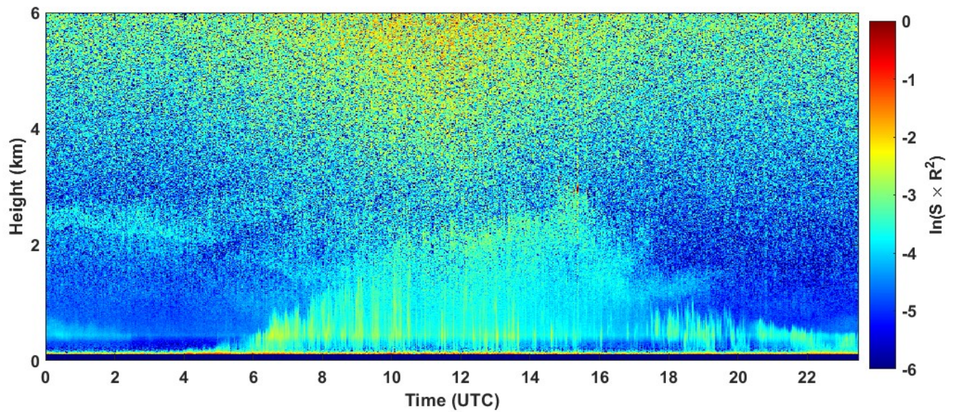
2023-08-10 RCS quick look CHM15k - ILVA LIDAR2 PARCHI
