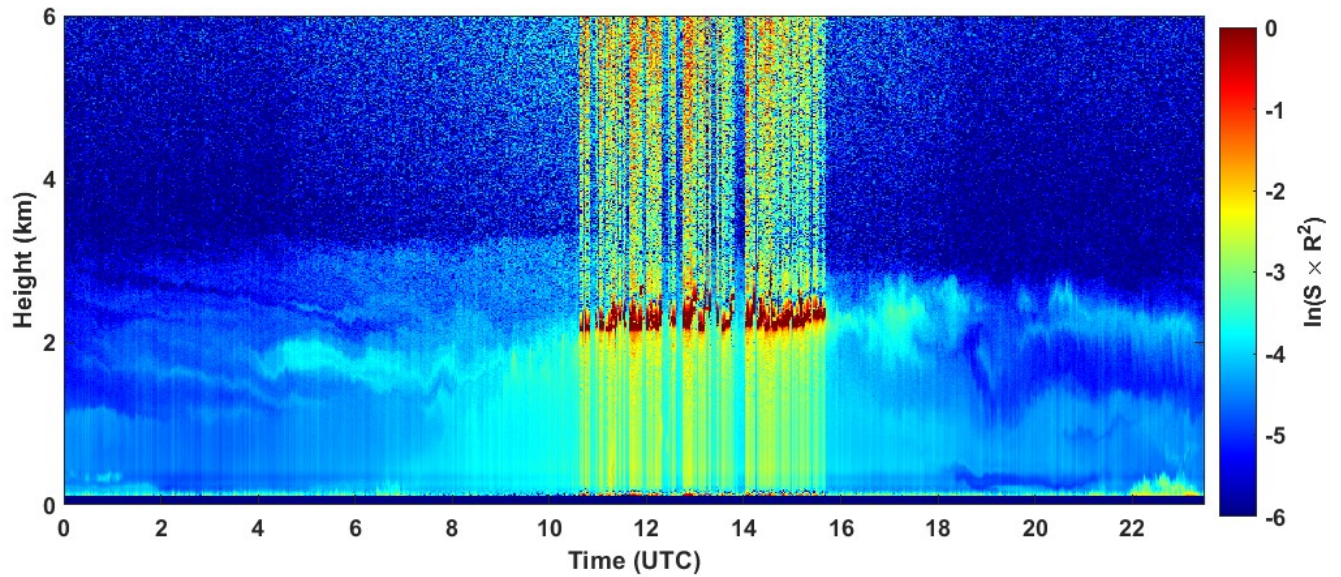
2023-08-14 RCS quick look CHM15k - ILVA LIDAR3 AGGLOMERATO
