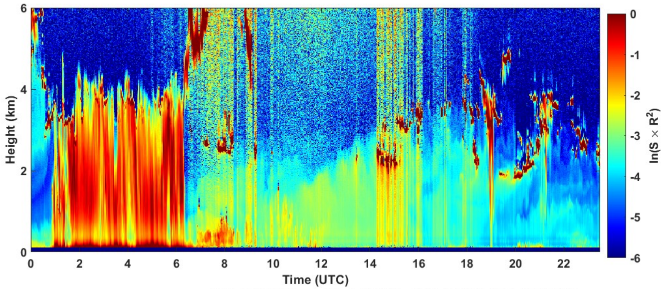
2023-08-06 RCS quick look CHM15k - ILVA LIDAR3 AGGLOMERATO
