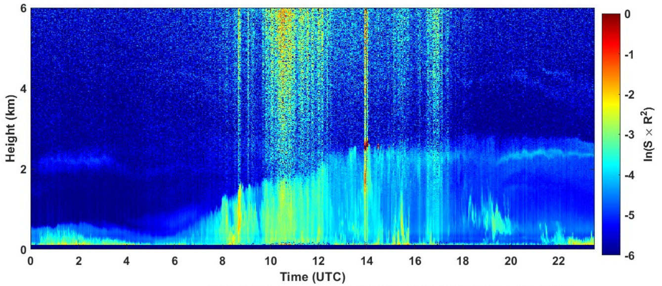
2023-08-10 RCS quick look CHM15k - ILVA LIDAR3 AGGLOMERATO
