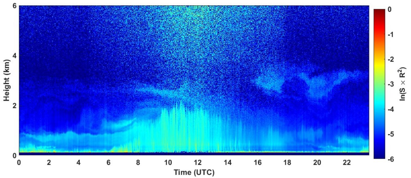
2023-08-18 RCS quick look CHM15k - ILVA LIDAR3 AGGLOMERATO
