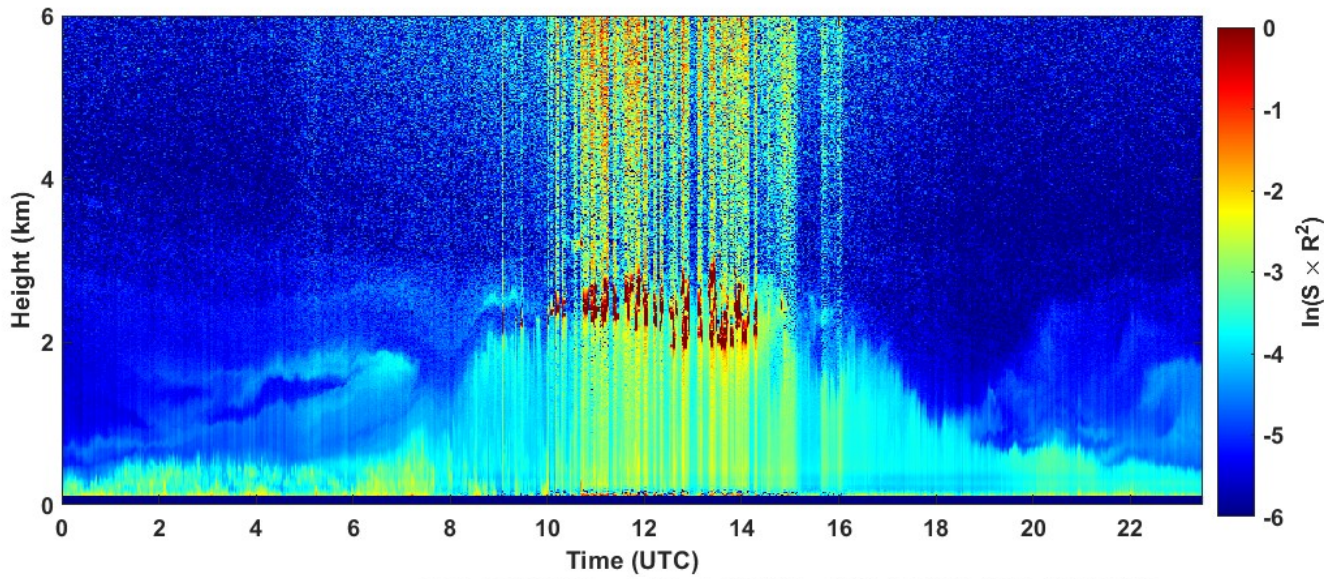
2023-08-12 RCS quick look CHM15k - ILVA LIDAR3 AGGLOMERATO
