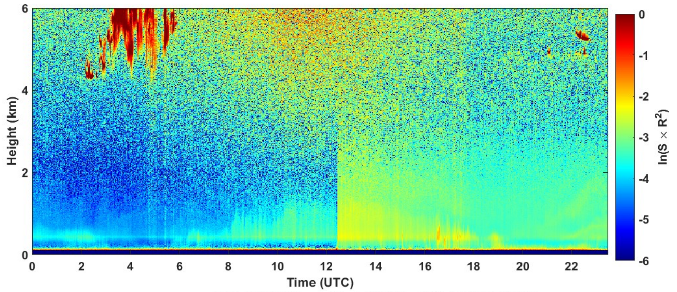
2023-08-22 RCS quick look CHM15k - ILVA LIDAR2 PARCHI
