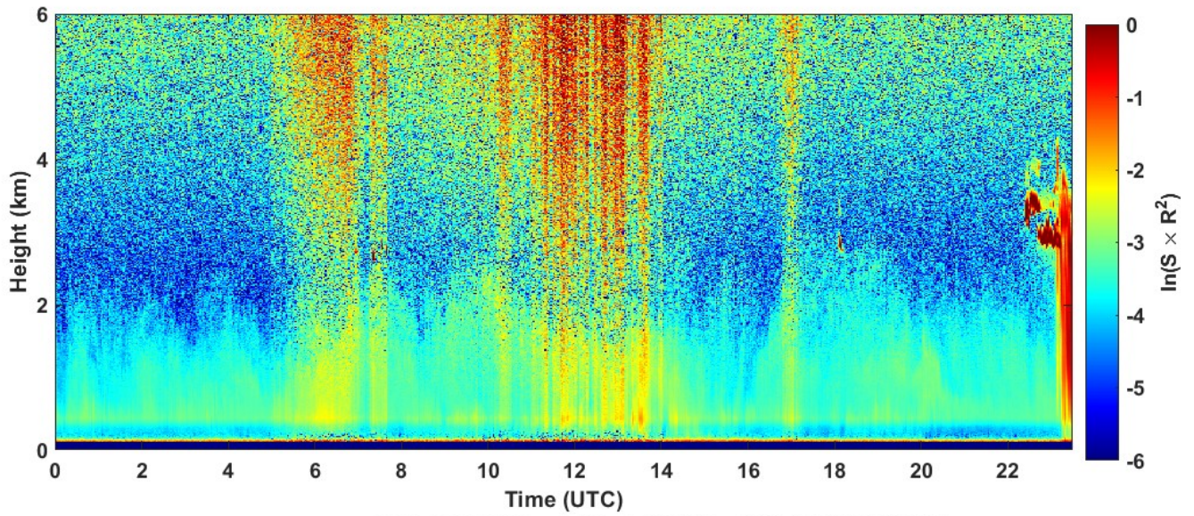
2023-08-30 RCS quick look CHM15k - ILVA LIDAR2 PARCHI
