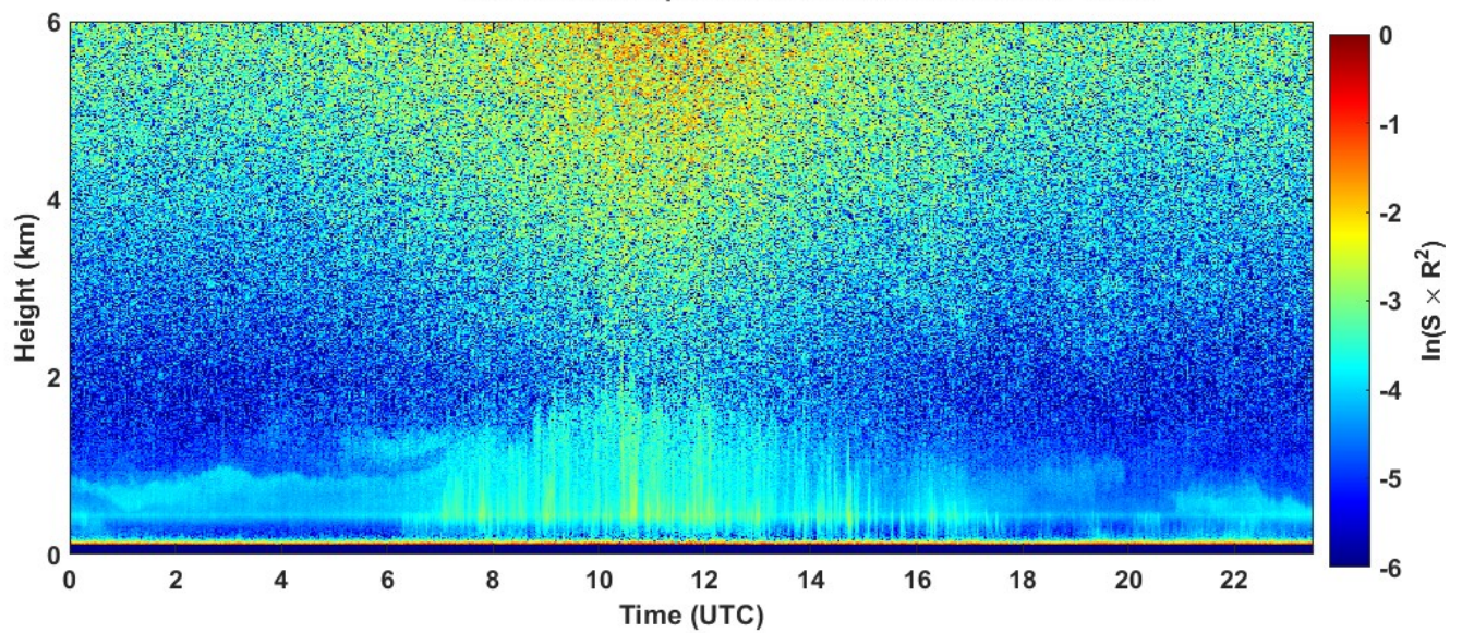
2023-08-18 RCS quick look CHM15k - ILVA LIDAR2 PARCHI
