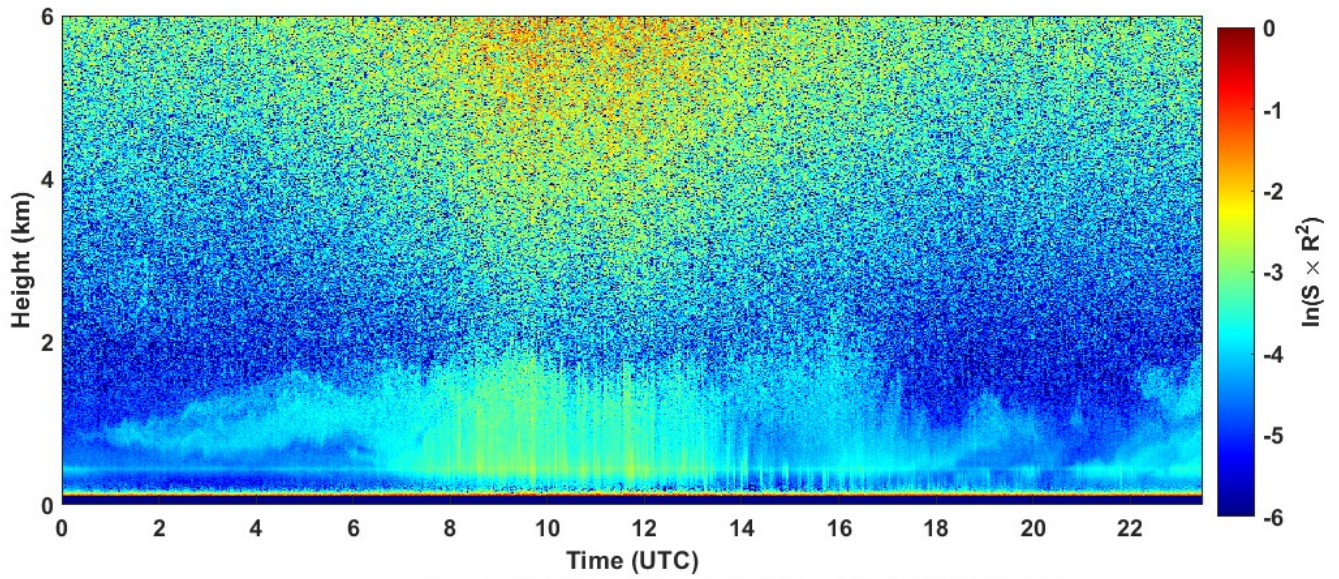
2023-08-20 RCS quick look CHM15k - ILVA LIDAR2 PARCHI
