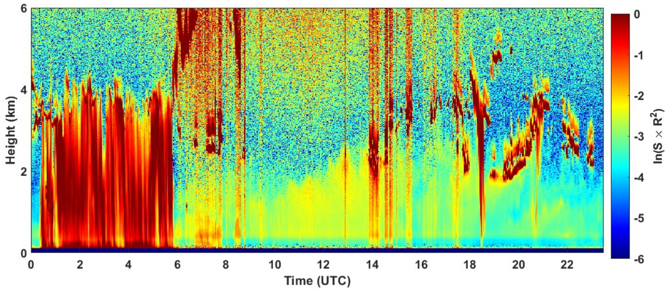
2023-08-06 RCS quick look CHM15k - ILVA LIDAR2 PARCHI
