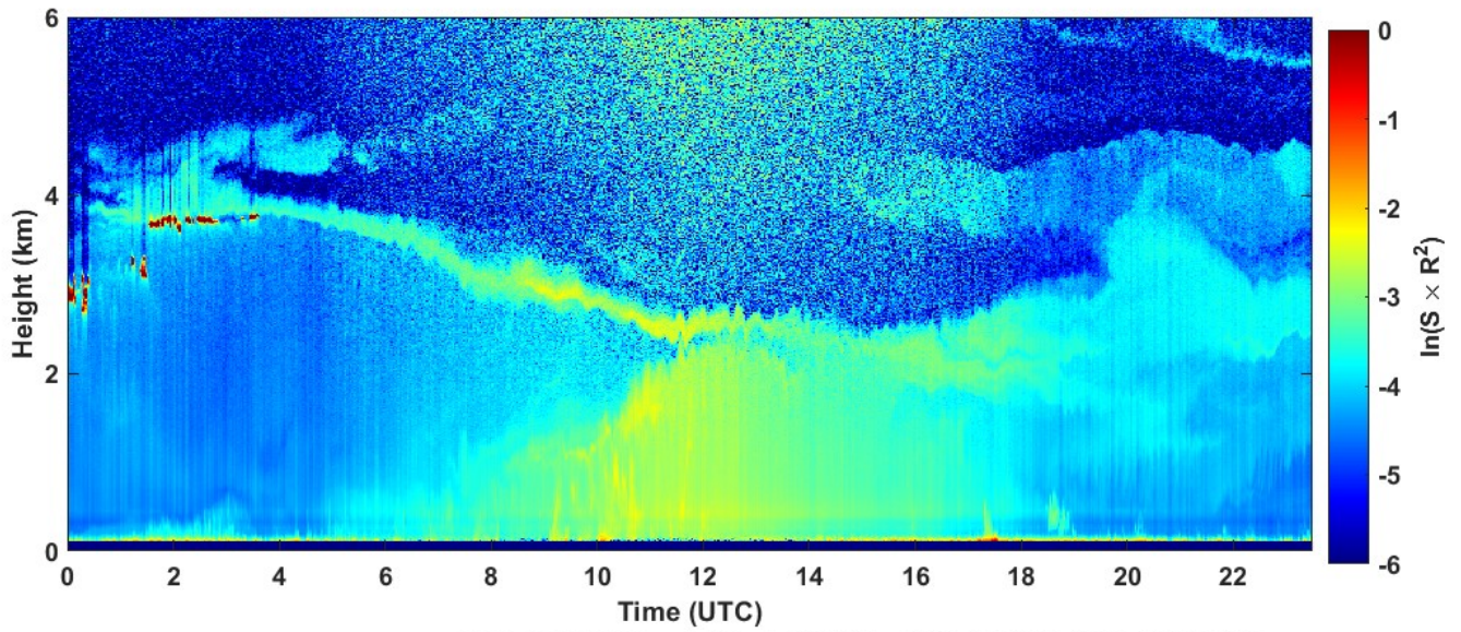
2023-08-24 RCS quick look CHM15k - ILVA LIDAR3 AGGLOMERATO
