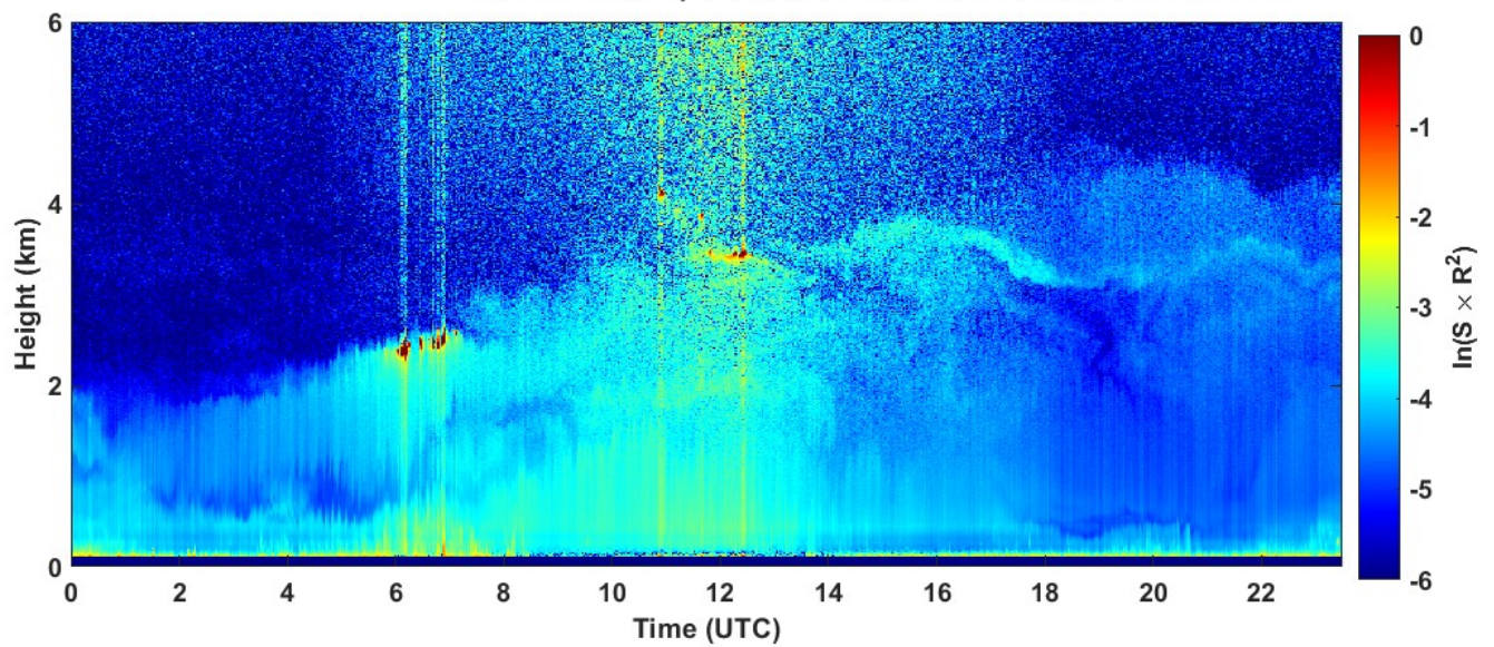
2023-08-20 RCS quick look CHM15k - ILVA LIDAR3 AGGLOMERATO
