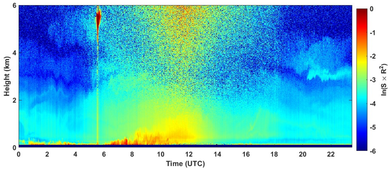
2023-07-20 RCS quick look CHM15k - ILVA LIDAR3 AGGLOMERATO
