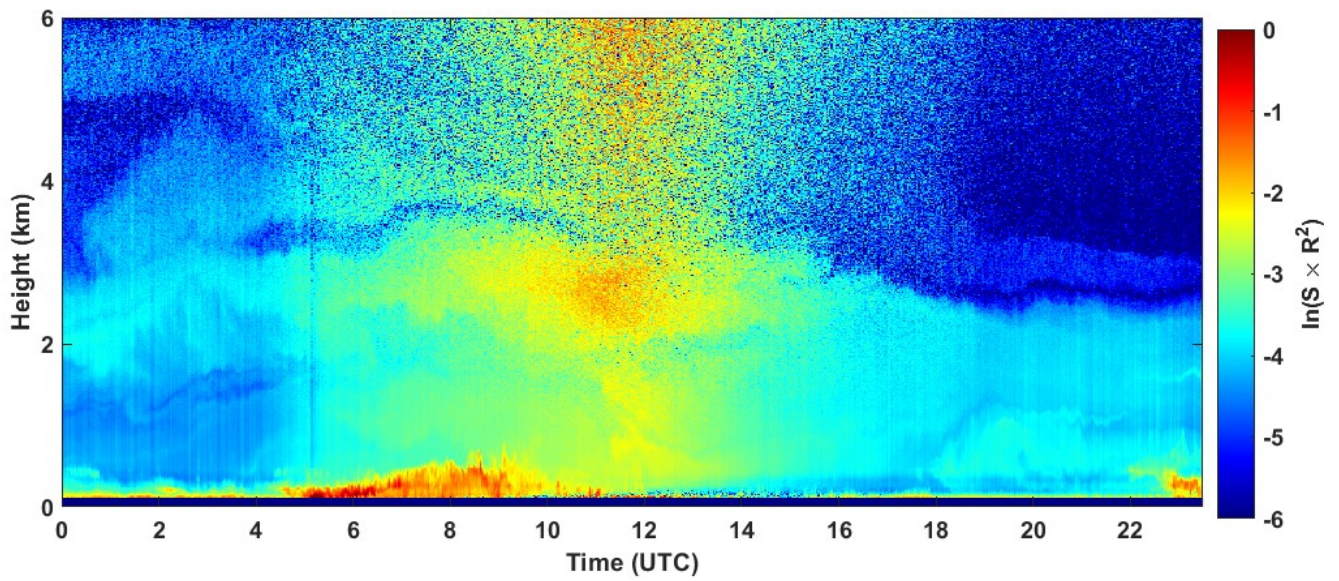
2023-07-14 RCS quick look CHM15k - ILVA LIDAR3 AGGLOMERATO
