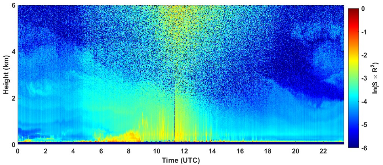
2023-07-18 RCS quick look CHM15k - ILVA LIDAR3 AGGLOMERATO
