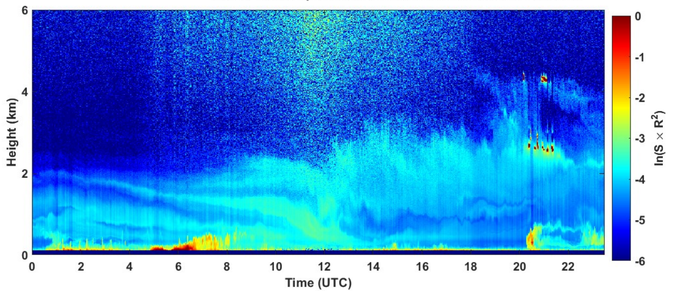
2023-07-30 RCS quick look CHM15k - ILVA LIDAR3 AGGLOMERATO
