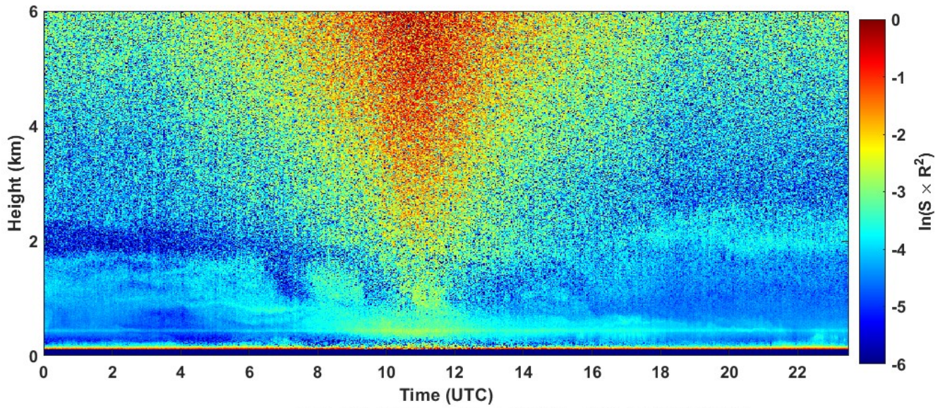
2023-07-14 RCS quick look CHM15k - ILVA LIDAR2 PARCHI
