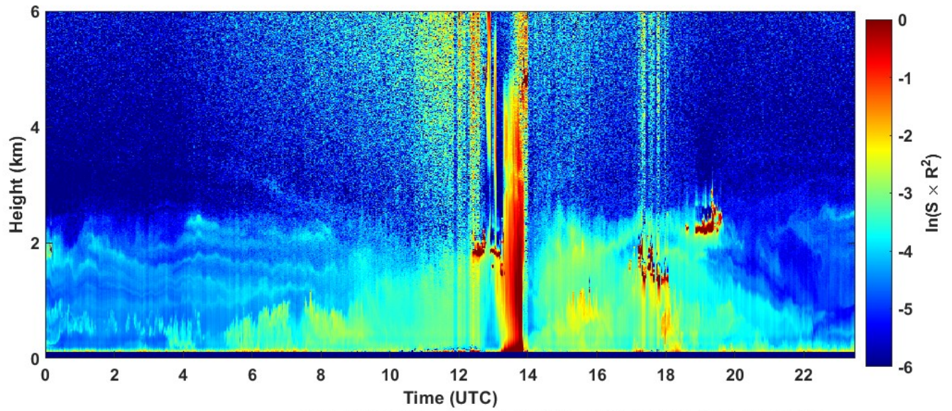
2023-07-06 RCS quick look CHM15k - ILVA LIDAR3 AGGLOMERATO
