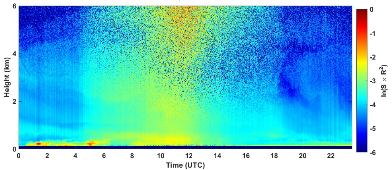
2023-07-24 RCS quick look CHM15k - ILVA LIDAR3 AGGLOMERATO
