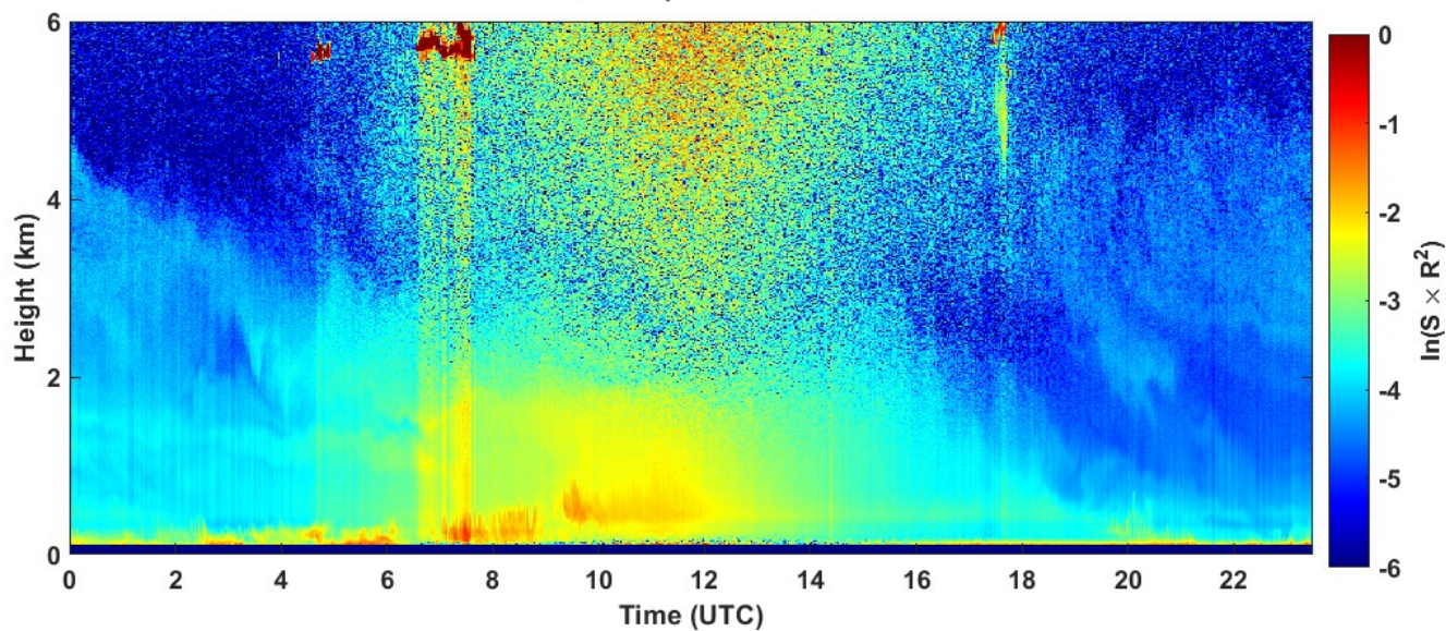
2023-07-22 RCS quick look CHM15k - ILVA LIDAR3 AGGLOMERATO
