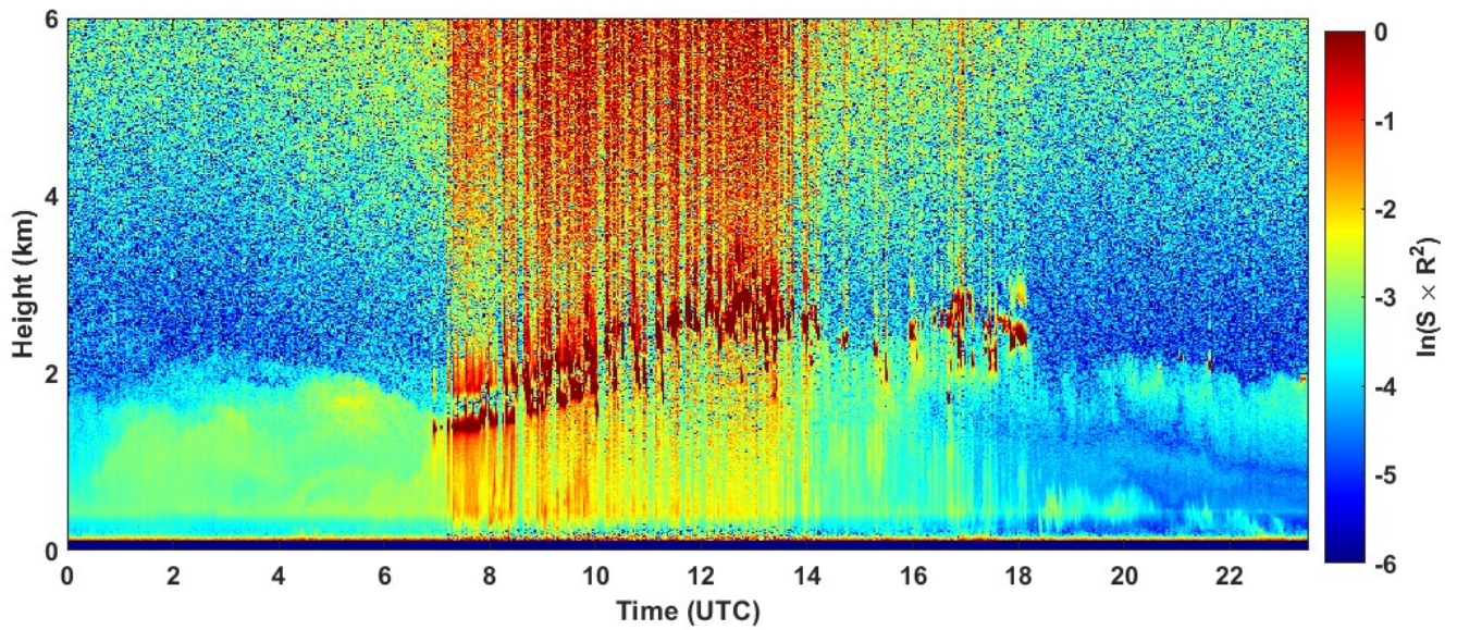
2023-07-02 RCS quick look CHM15k - ILVA LIDAR2 PARCHI
