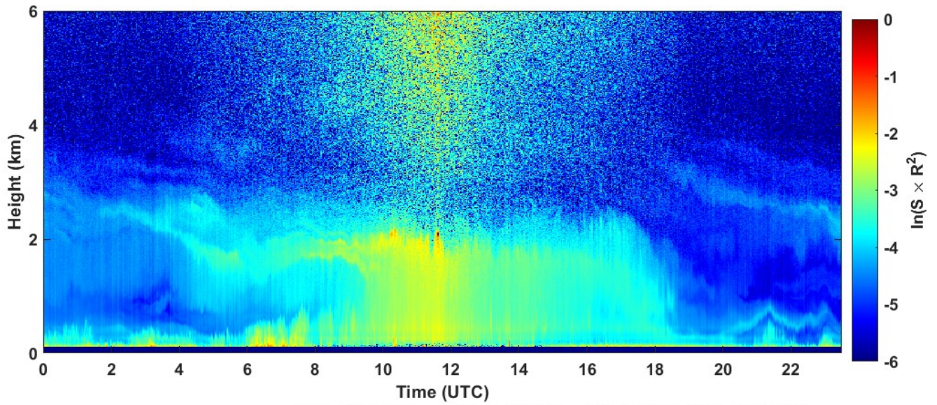
2023-07-08 RCS quick look CHM15k - ILVA LIDAR3 AGGLOMERATO
