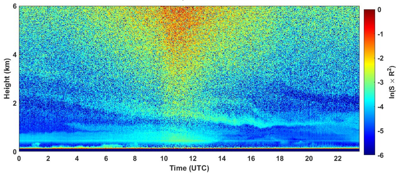
2023-07-12 RCS quick look CHM15k - ILVA LIDAR2 PARCHI
