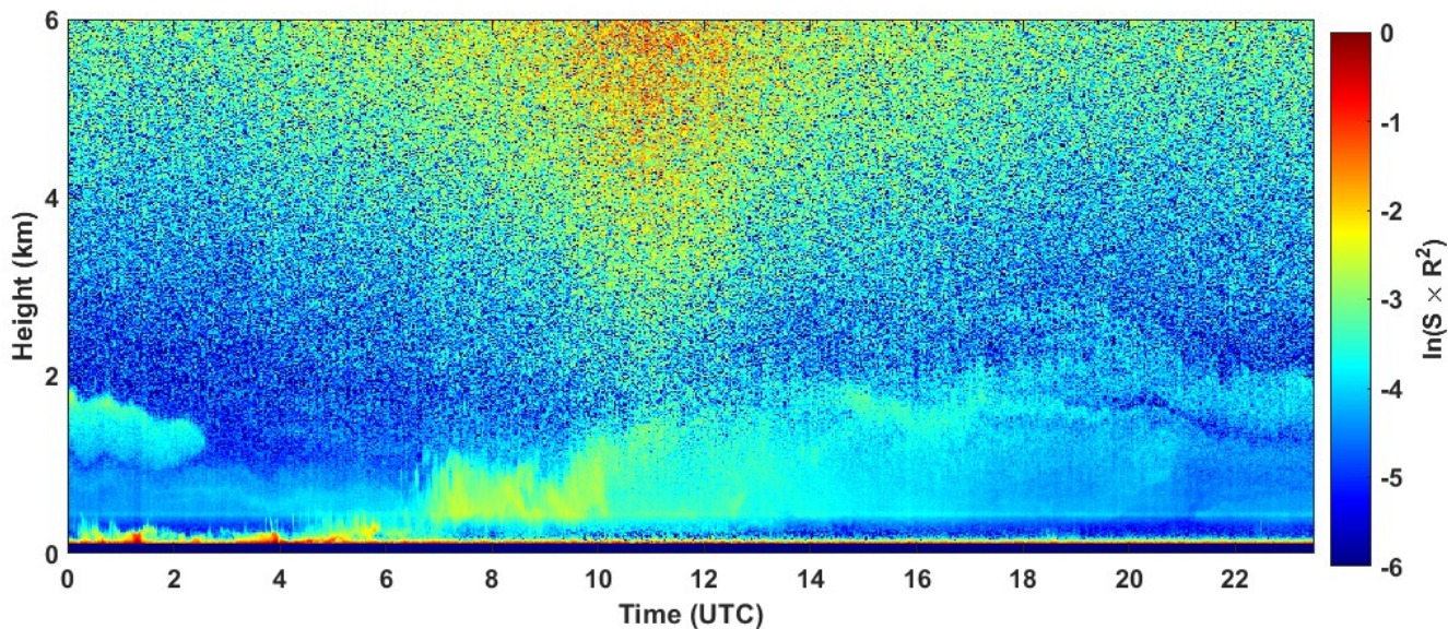
2023-07-04 RCS quick look CHM15k - ILVA LIDAR2 PARCHI
