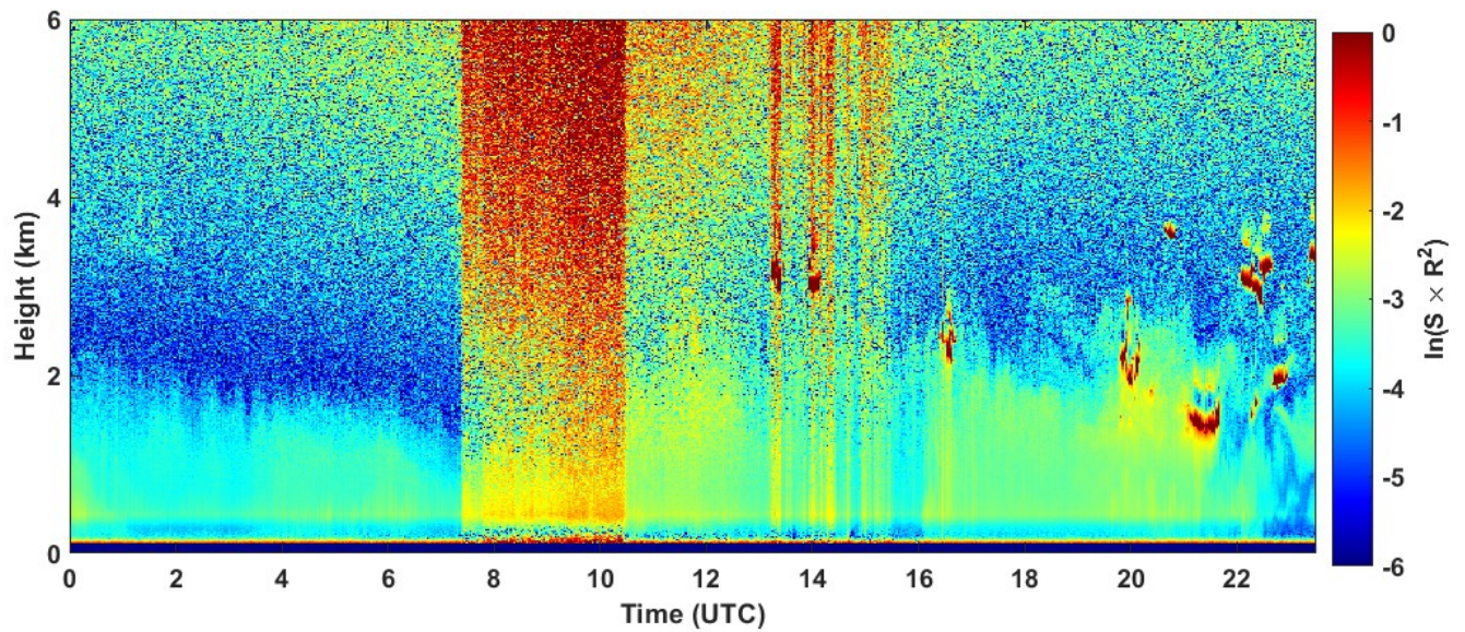
2023-07-27 RCS quick look CHM15k - ILVA LIDAR2 PARCHI
