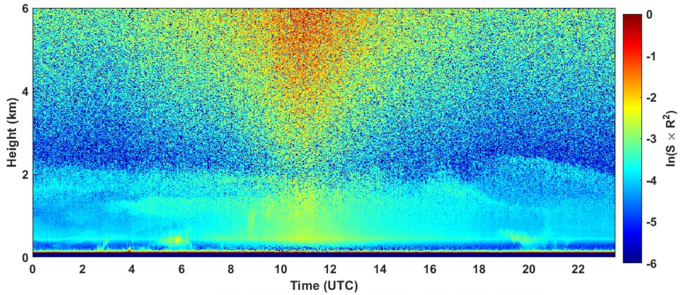
2023-07-16 RCS quick look CHM15k - ILVA LIDAR2 PARCHI
