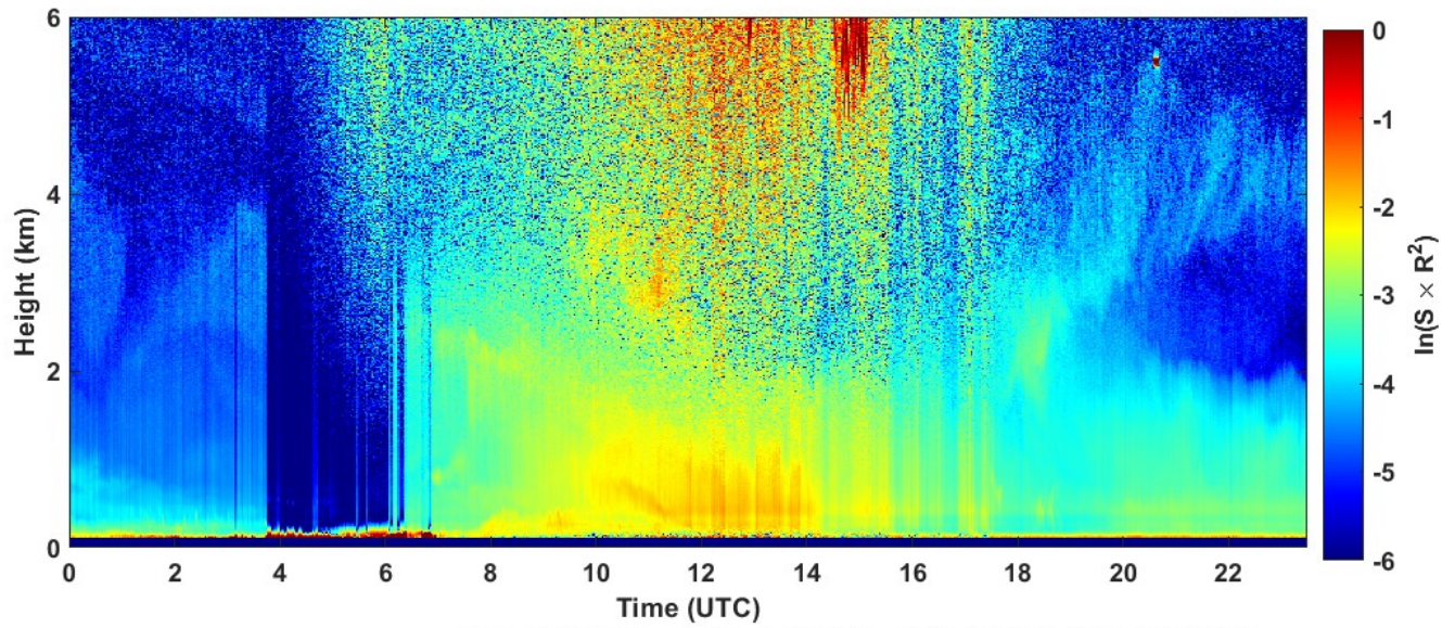
2023-07-26 RCS quick look CHM15k - ILVA LIDAR3 AGGLOMERATO
