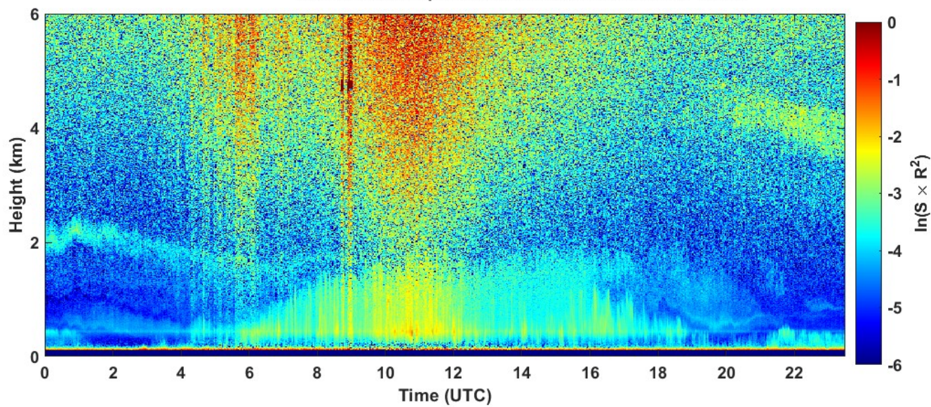
2023-07-08 RCS quick look CHM15k - ILVA LIDAR2 PARCHI
