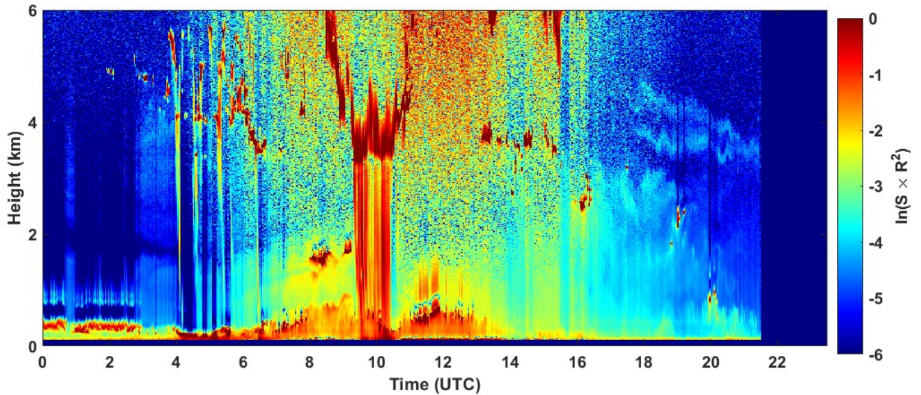
2023-07-02 RCS quick look CHM15k - ILVA LIDAR3 AGGLOMERATO
