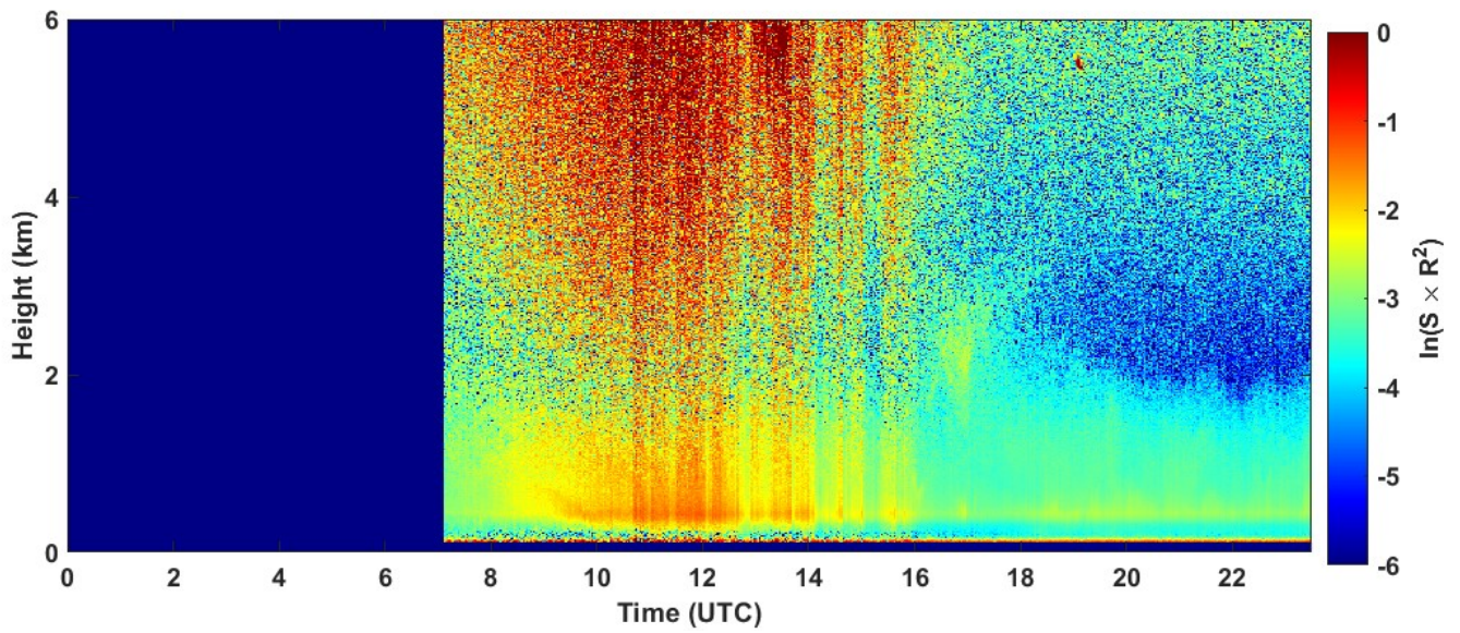
2023-07-25 RCS quick look CHM15k - ILVA LIDAR2 PARCHI
