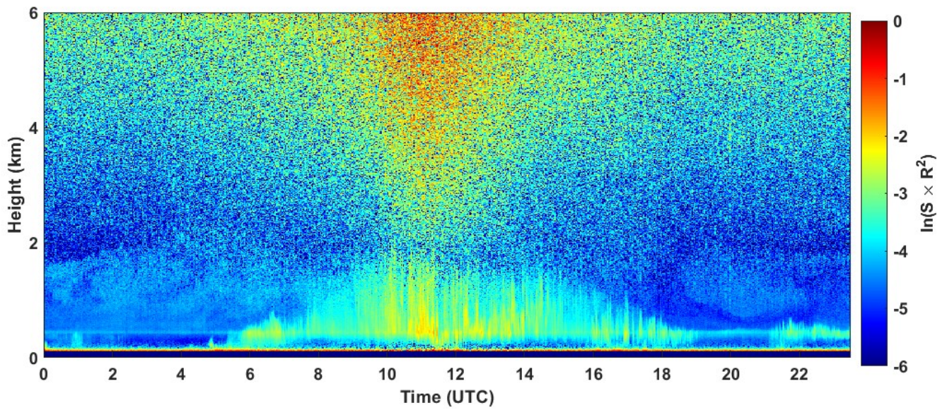
2023-07-10 RCS quick look CHM15k - ILVA LIDAR2 PARCHI
