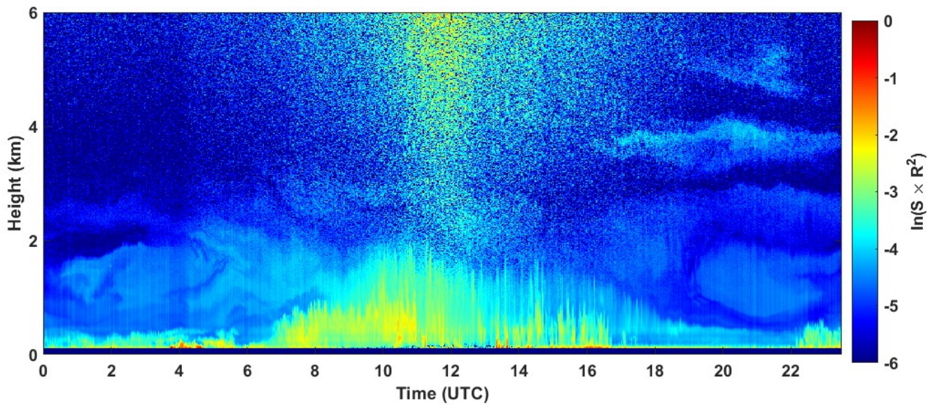
2023-07-10 RCS quick look CHM15k - ILVA LIDAR3 AGGLOMERATO
