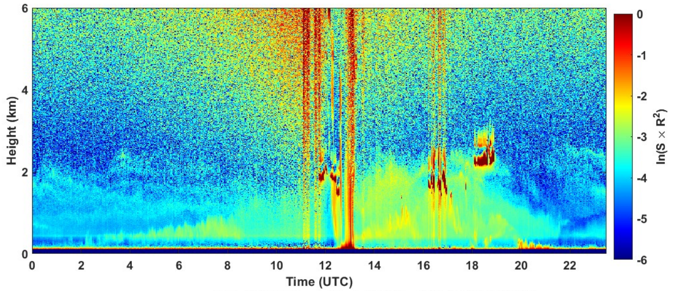
2023-07-06 RCS quick look CHM15k - ILVA LIDAR2 PARCHI
