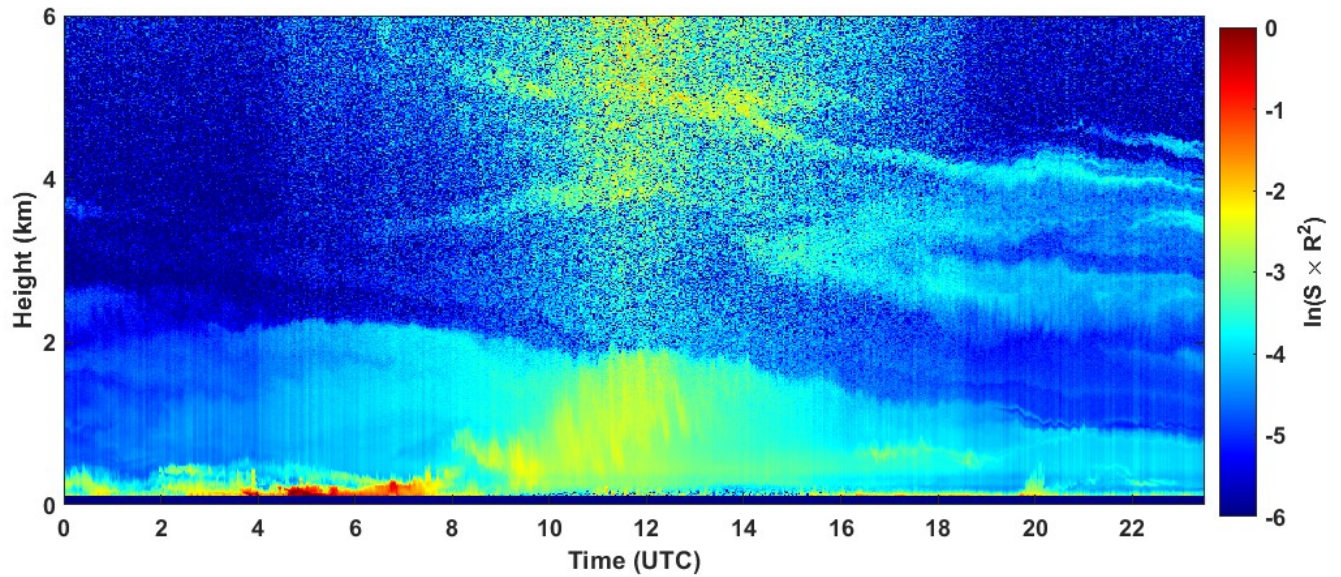
2023-07-12 RCS quick look CHM15k - ILVA LIDAR3 AGGLOMERATO
