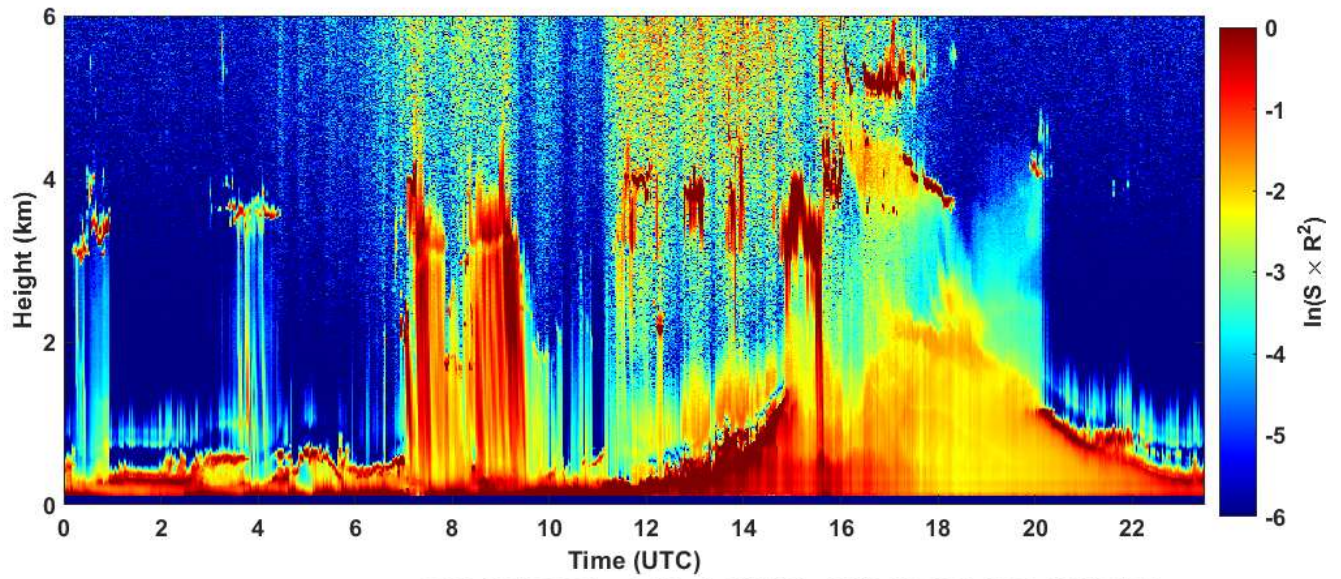
2023-05-16 RCS quick look CHM15k - ILVA LIDAR3 AGGLOMERATO
