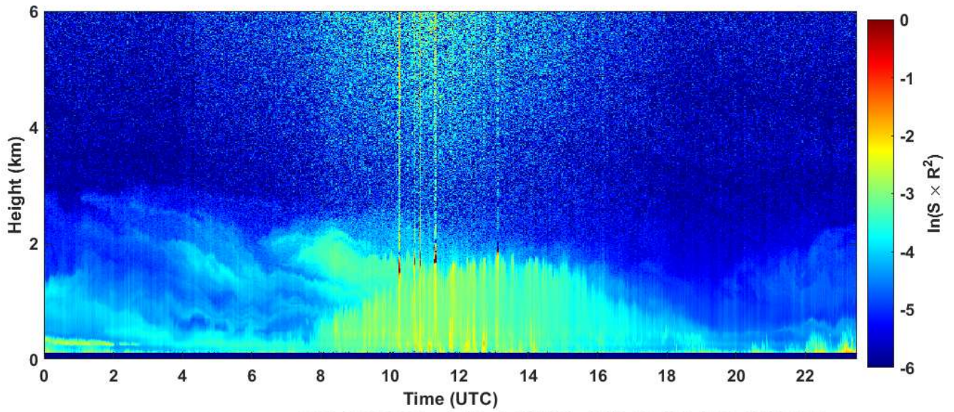
2023-05-06 RCS quick look CHM15k - ILVA LIDAR3 AGGLOMERATO
