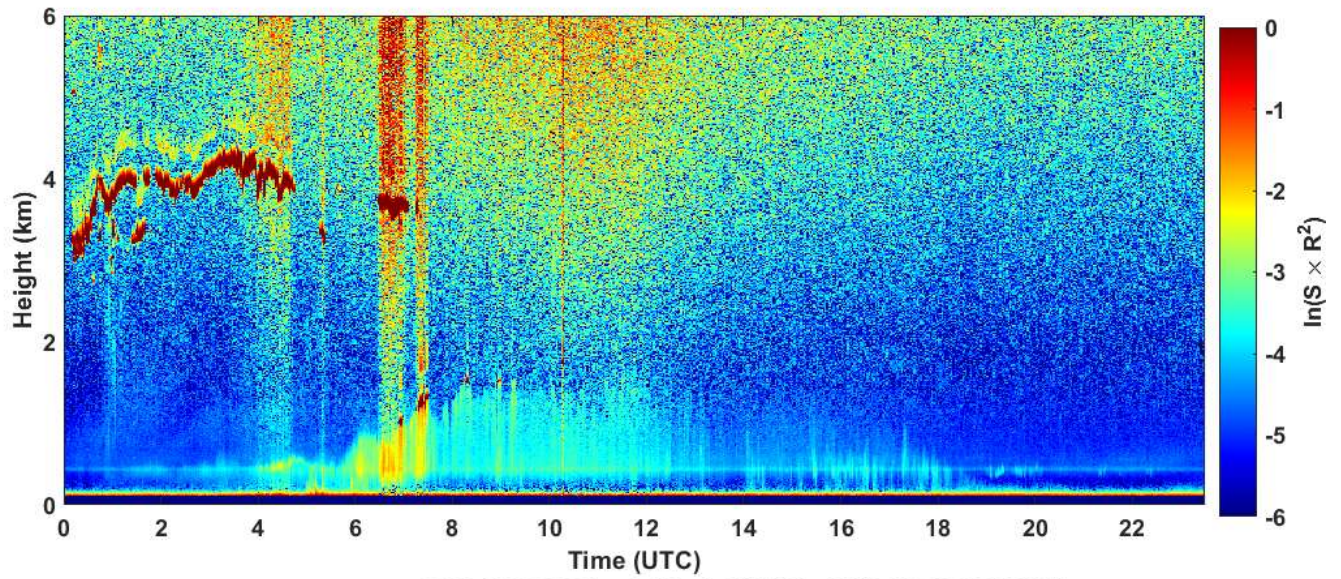
2023-05-28 RCS quick look CHM15k - ILVA LIDAR2 PARCHI
