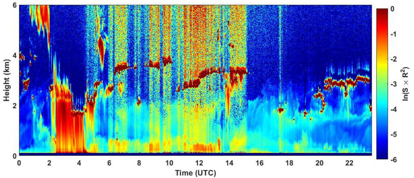
2023-05-18 RCS quick look CHM15k - ILVA LIDAR3 AGGLOMERATO
