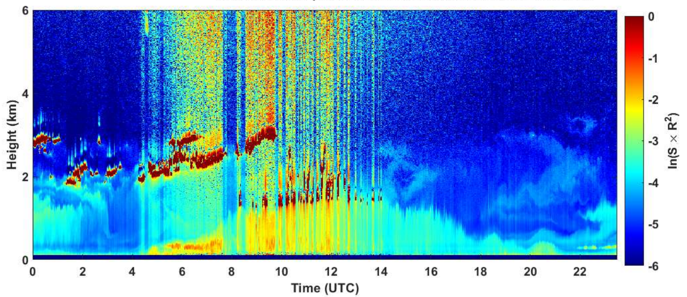
2023-05-04 RCS quick look CHM15k - ILVA LIDAR3 AGGLOMERATO
