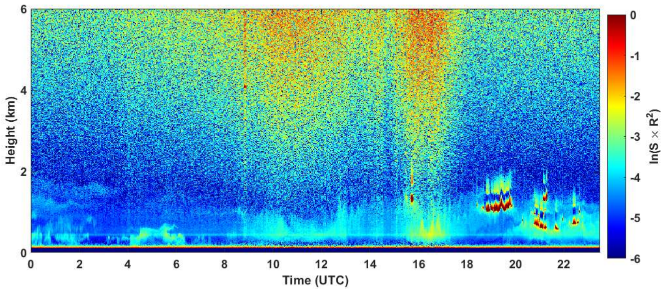
2023-05-30 RCS quick look CHM15k - ILVA LIDAR2 PARCHI
