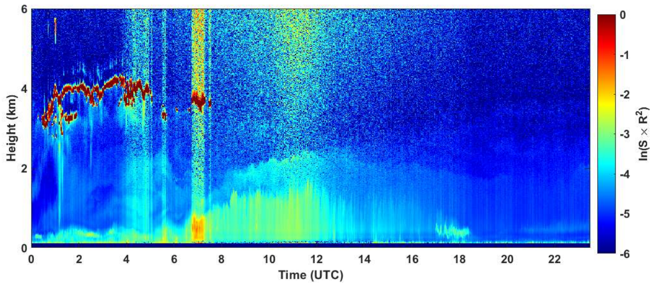
2023-05-28 RCS quick look CHM15k - ILVA LIDAR3 AGGLOMERATO
