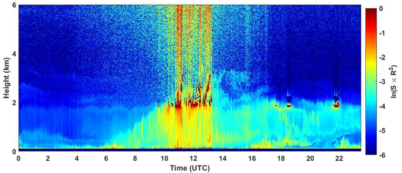
2023-05-30 RCS quick look CHM15k - ILVA LIDAR3 AGGLOMERATO
