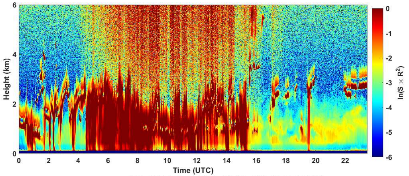
2023-05-04 RCS quick look CHM15k - ILVA LIDAR2 PARCHI
