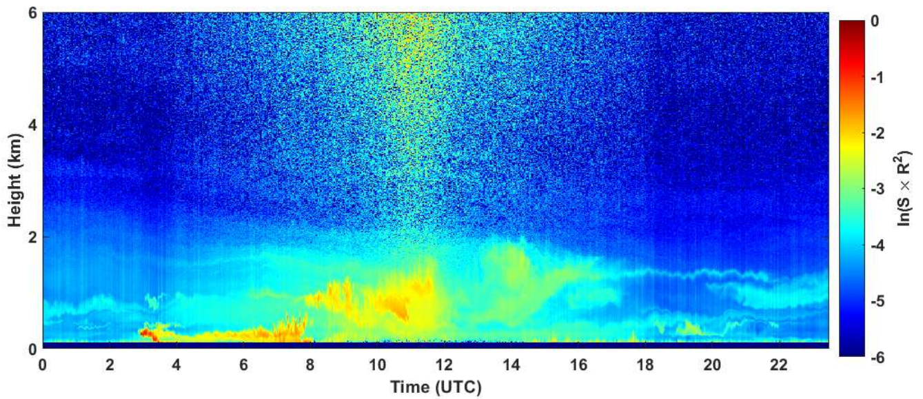
2023-05-24 RCS quick look CHM15k - ILVA LIDAR3 AGGLOMERATO
