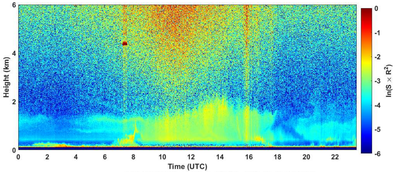
2023-05-26 RCS quick look CHM15k - ILVA LIDAR2 PARCHI
