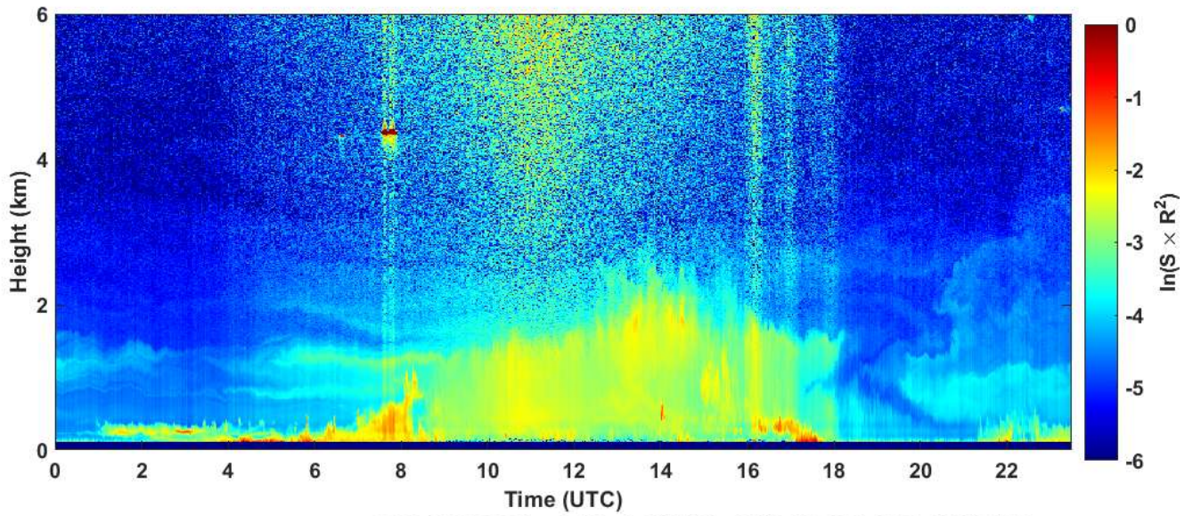
2023-05-26 RCS quick look CHM15k - ILVA LIDAR3 AGGLOMERATO
