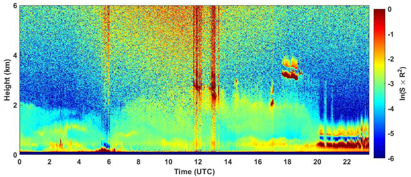
2023-05-12 RCS quick look CHM15k - ILVA LIDAR2 PARCHI
