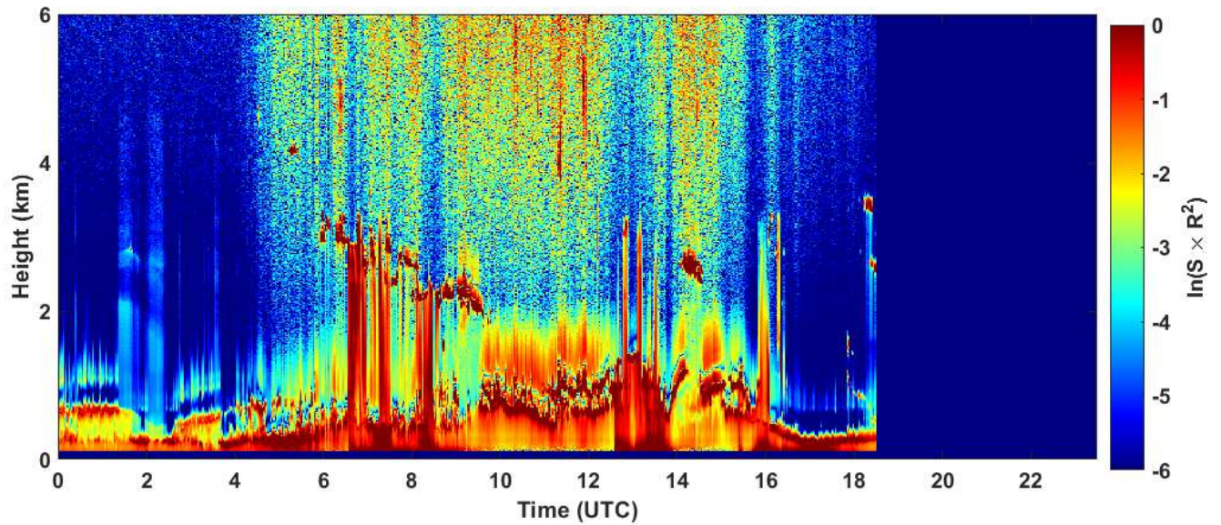
2023-05-14 RCS quick look CHM15k - ILVA LIDAR3 AGGLOMERATO
