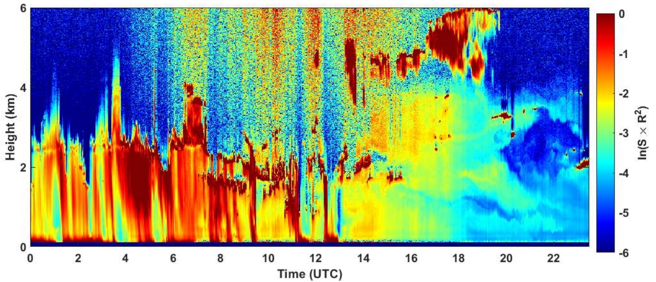
2023-05-22 RCS quick look CHM15k - ILVA LIDAR3 AGGLOMERATO
