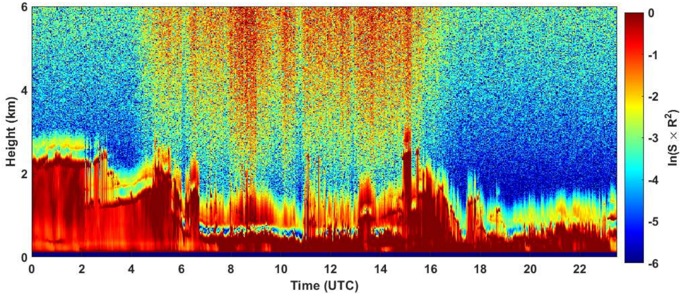
2023-05-02 RCS quick look CHM15k - ILVA LIDAR2 PARCHI
