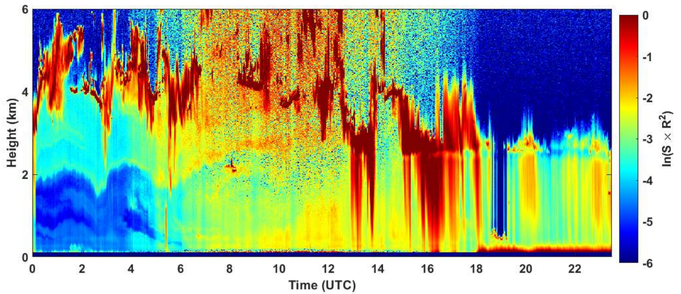
2023-05-20 RCS quick look CHM15k - ILVA LIDAR3 AGGLOMERATO
