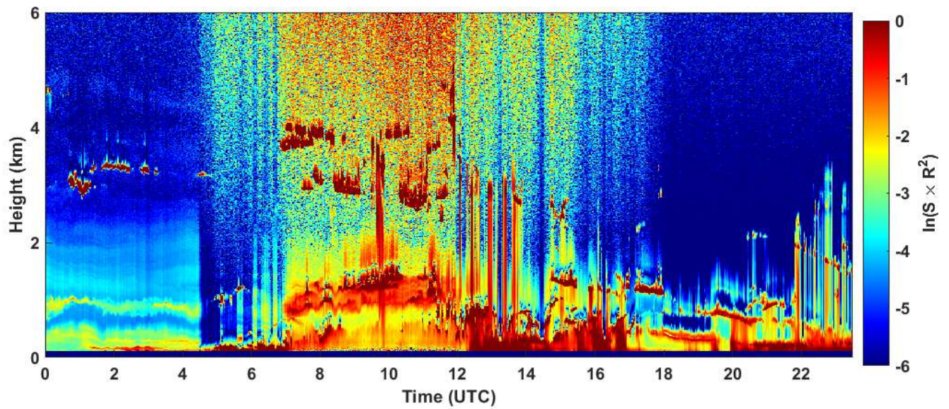
2023-05-10 RCS quick look CHM15k - ILVA LIDAR3 AGGLOMERATO
