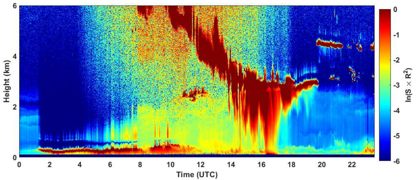
2023-05-08 RCS quick look CHM15k - ILVA LIDAR3 AGGLOMERATO
