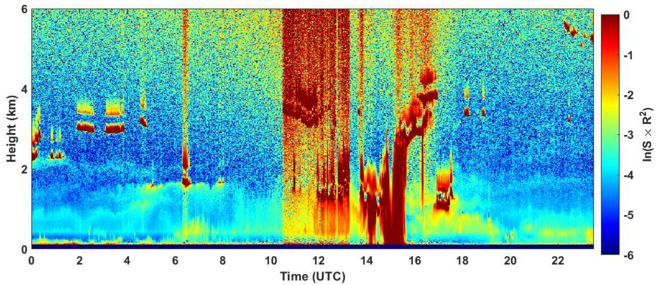
2023-05-18 RCS quick look CHM15k - ILVA LIDAR2 PARCHI
