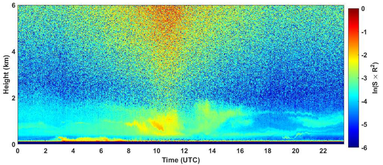
2023-05-24 RCS quick look CHM15k - ILVA LIDAR2 PARCHI
