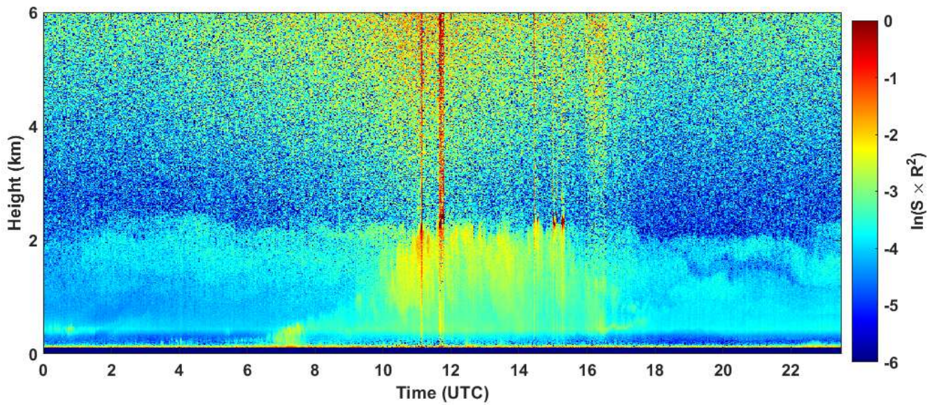
2023-05-06 RCS quick look CHM15k - ILVA LIDAR2 PARCHI
