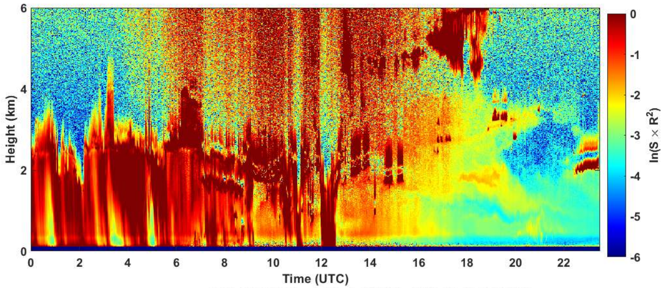
2023-05-22 RCS quick look CHM15k - ILVA LIDAR2 PARCHI
