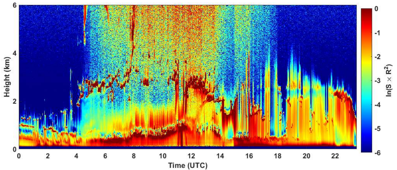
2023-05-02 RCS quick look CHM15k - ILVA LIDAR3 AGGLOMERATO
