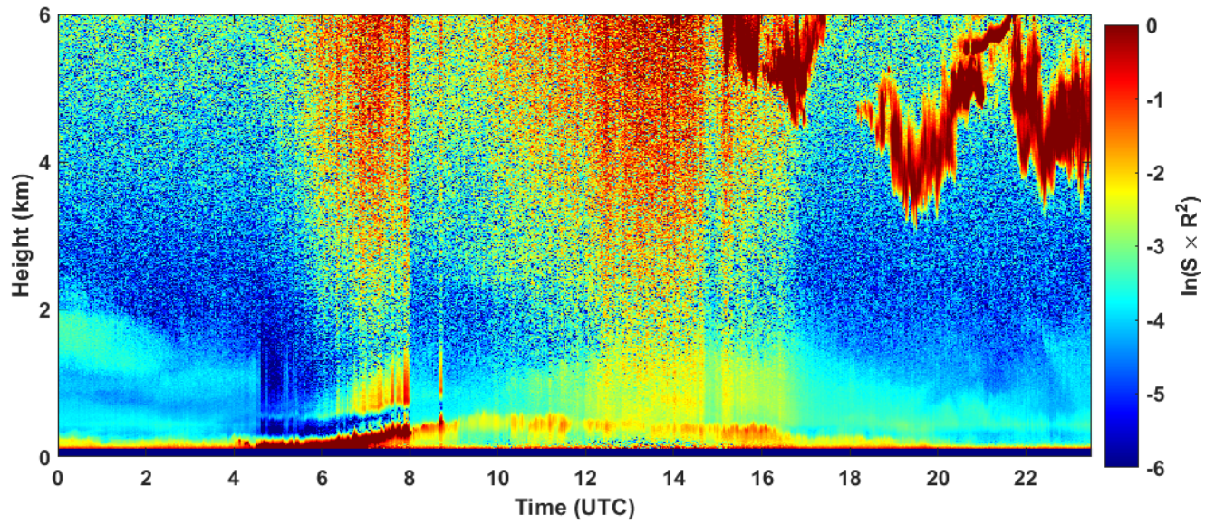
2023-03-31 RCS quick look CHM15k - ILVA LIDAR2 PARCHI
