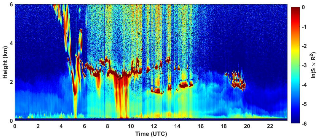
2023-03-08 RCS quick look CHM15k - ILVA LIDAR3 AGGLOMERATO
