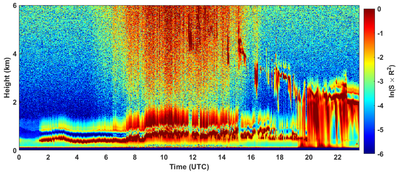
2023-03-20 RCS quick look CHM15k - ILVA LIDAR2 PARCHI
