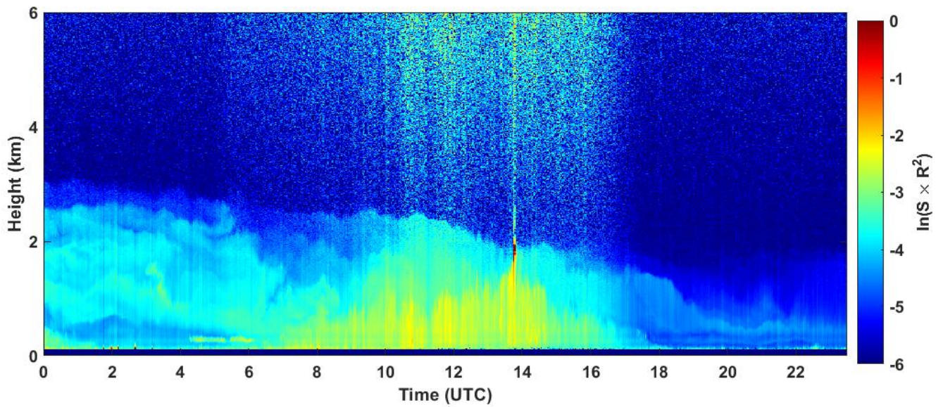
2023-03-22 RCS quick look CHM15k - ILVA LIDAR3 AGGLOMERATO
