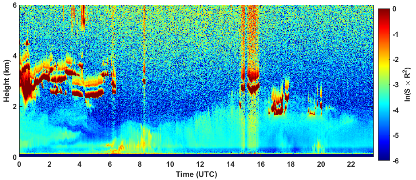
2023-03-08 RCS quick look CHM15k - ILVA LIDAR2 PARCHI
