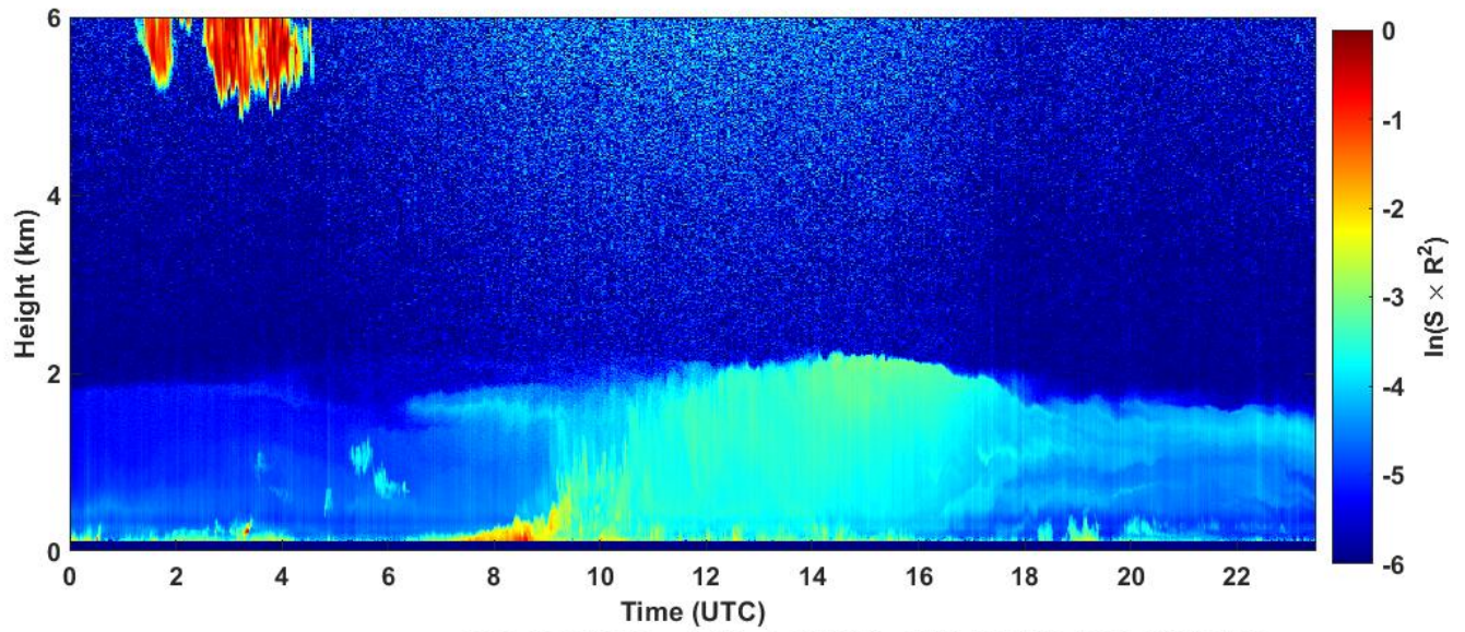
2023-03-24 RCS quick look CHM15k - ILVA LIDAR3 AGGLOMERATO
