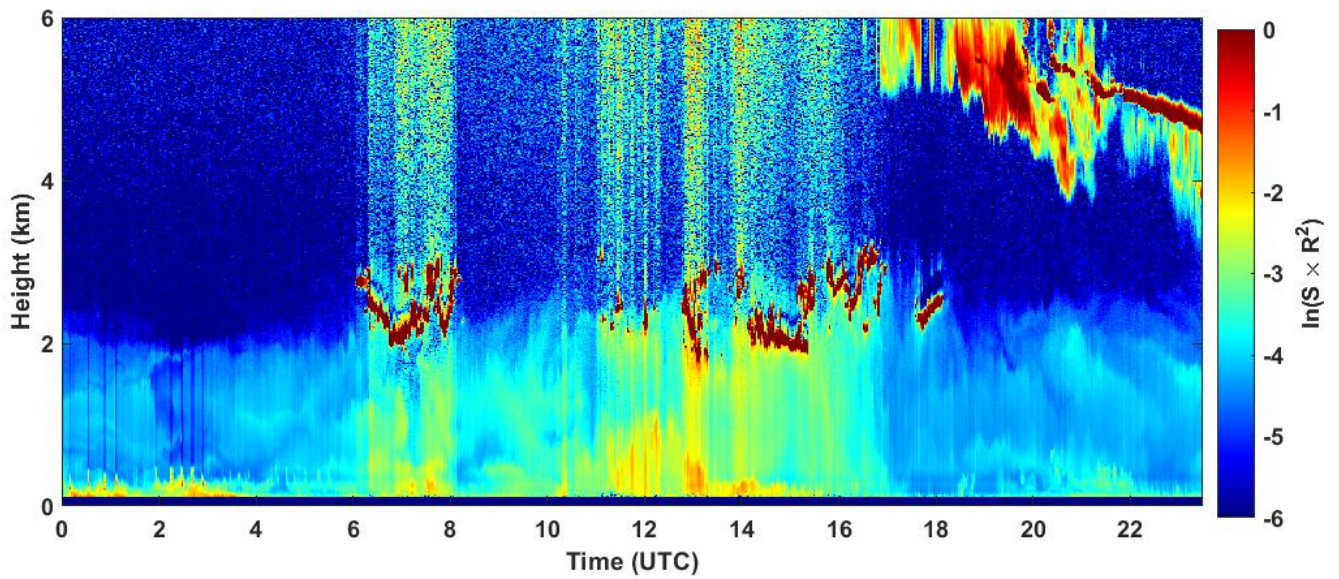
2023-03-06 RCS quick look CHM15k - ILVA LIDAR3 AGGLOMERATO
