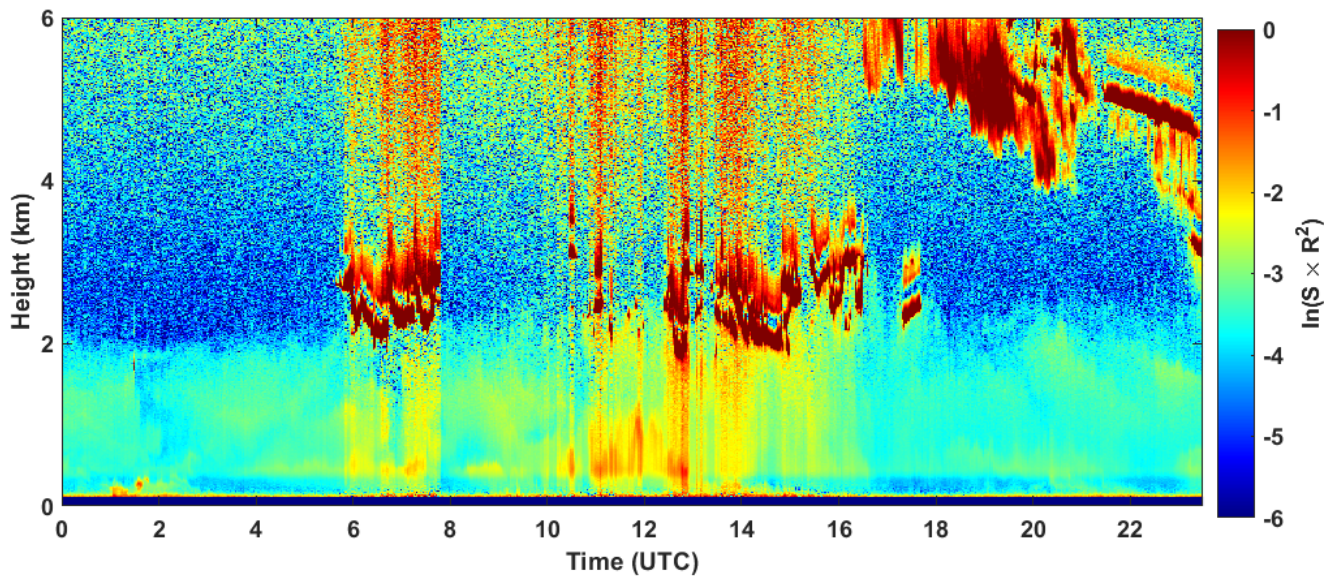
2023-03-06 RCS quick look CHM15k - ILVA LIDAR2 PARCHI
