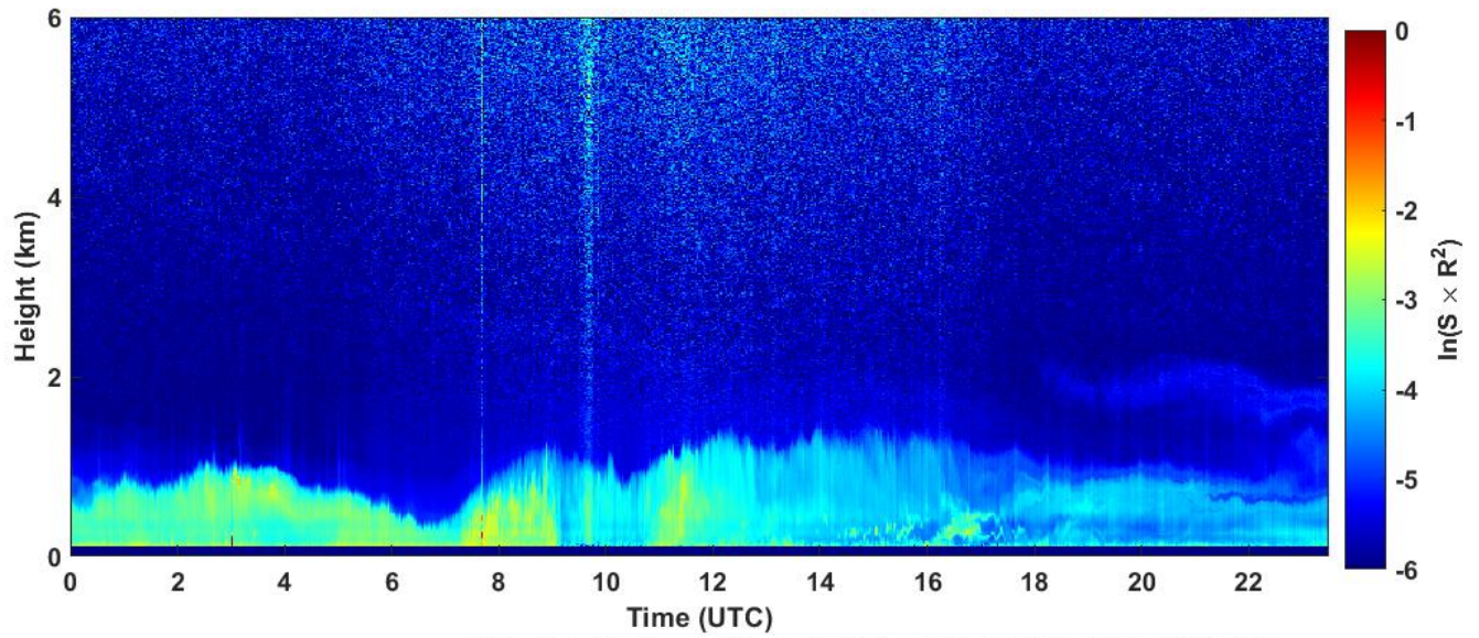
2023-03-14 RCS quick look CHM15k - ILVA LIDAR3 AGGLOMERATO
