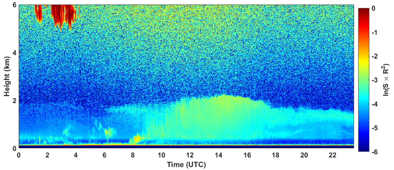
2023-03-24 RCS quick look CHM15k - ILVA LIDAR2 PARCHI
