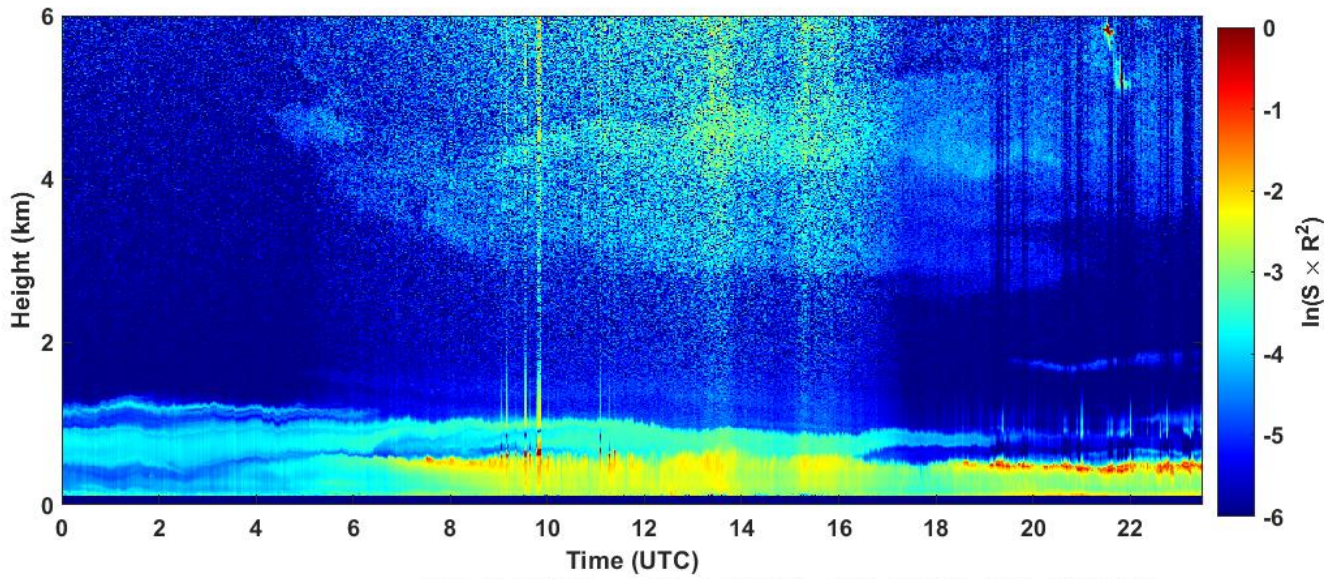
2023-03-20 RCS quick look CHM15k - ILVA LIDAR3 AGGLOMERATO
