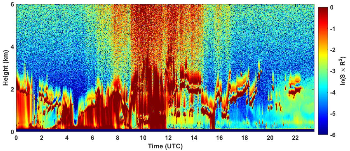
2023-03-22 RCS quick look CHM15k - ILVA LIDAR2 PARCHI
