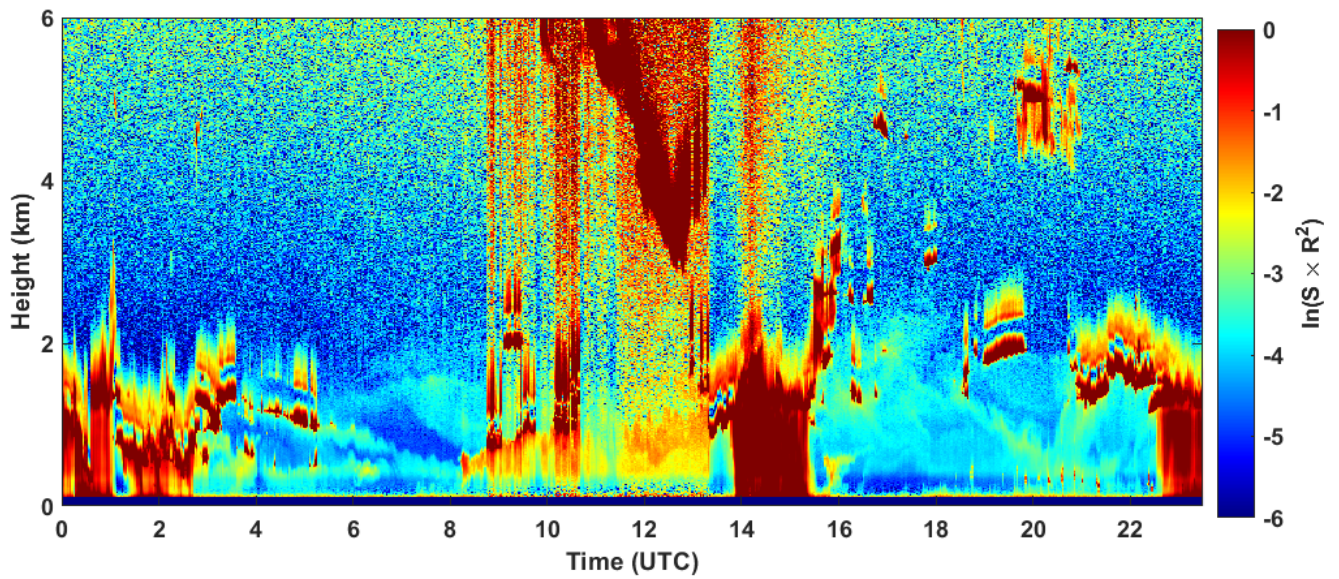
2023-03-04 RCS quick look CHM15k - ILVA LIDAR2 PARCHI
