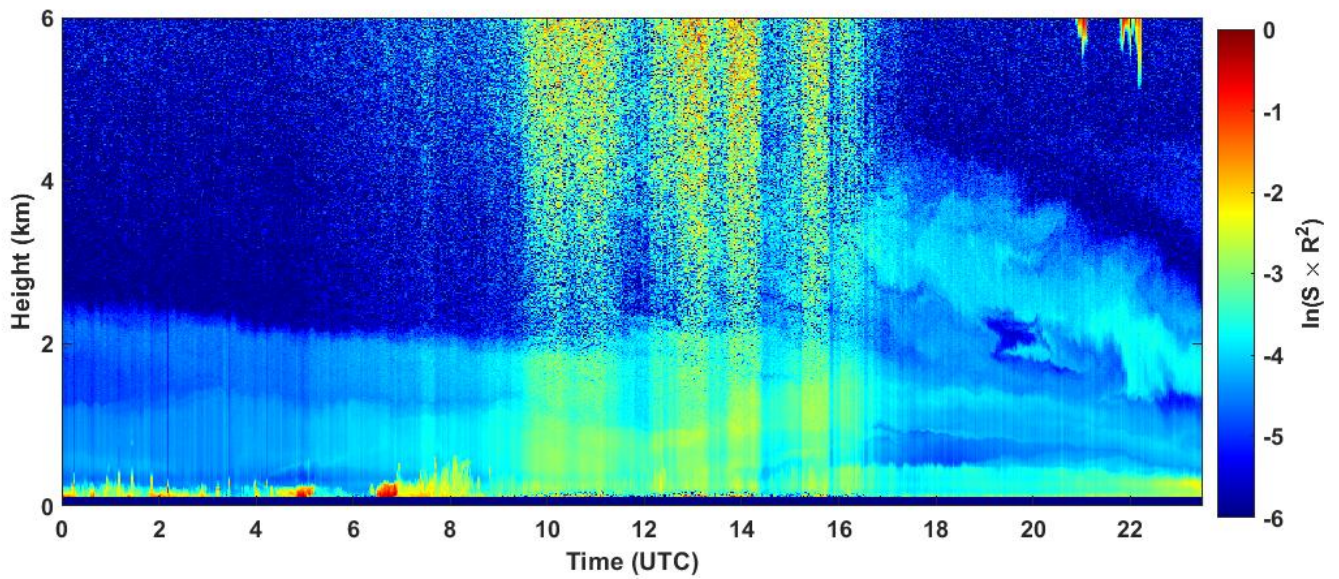
2023-03-30 RCS quick look CHM15k - ILVA LIDAR3 AGGLOMERATO
