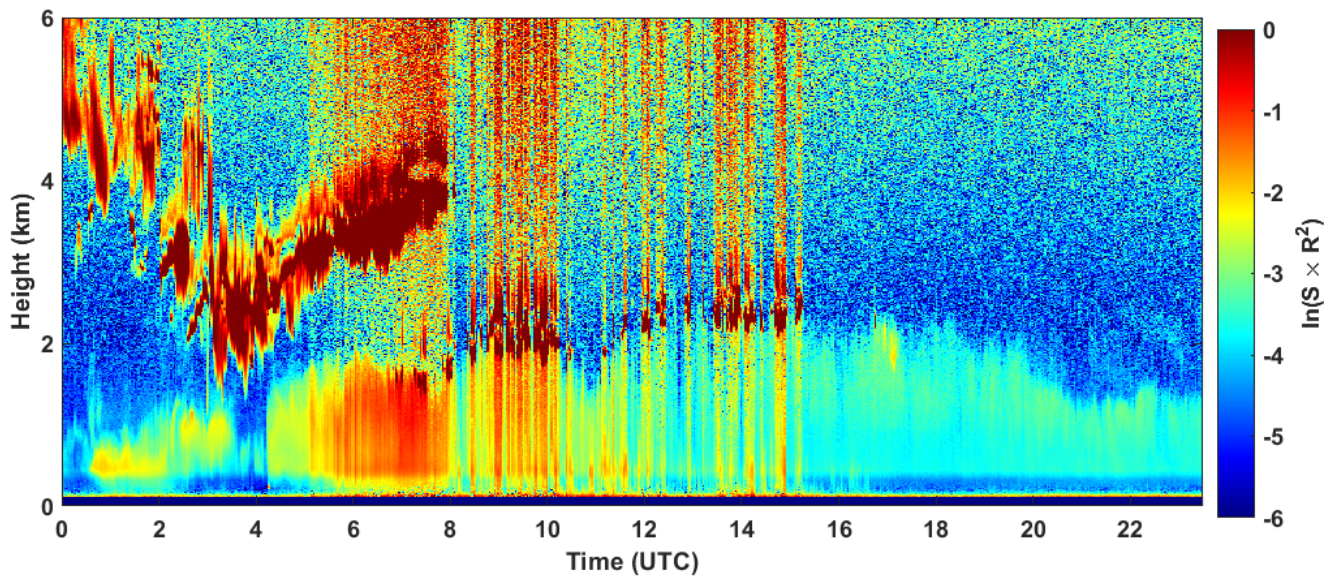
2023-03-28 RCS quick look CHM15k - ILVA LIDAR2 PARCHI
