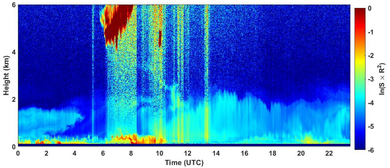
2023-03-26 RCS quick look CHM15k - ILVA LIDAR3 AGGLOMERATO
