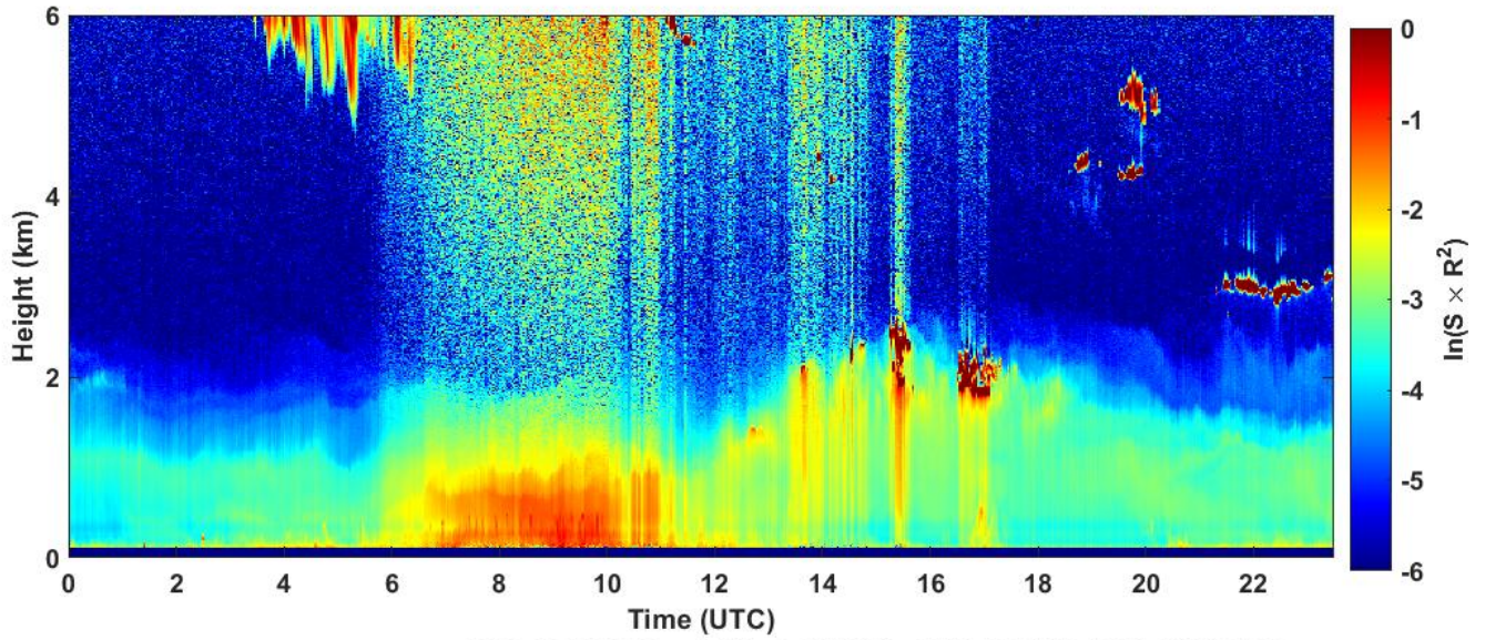
2023-03-12 RCS quick look CHM15k - ILVA LIDAR3 AGGLOMERATO
