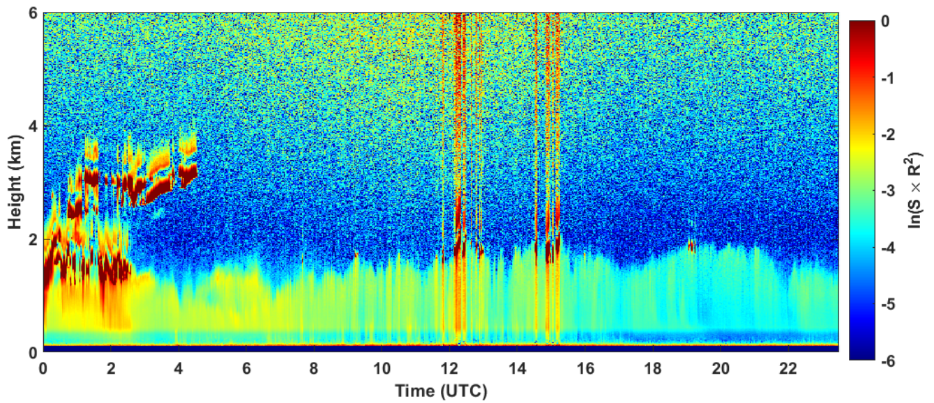
2023-03-16 RCS quick look CHM15k - ILVA LIDAR2 PARCHI
