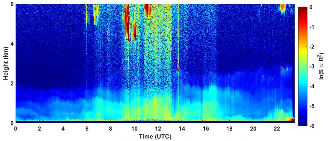
2023-03-10 RCS quick look CHM15k - ILVA LIDAR3 AGGLOMERATO
