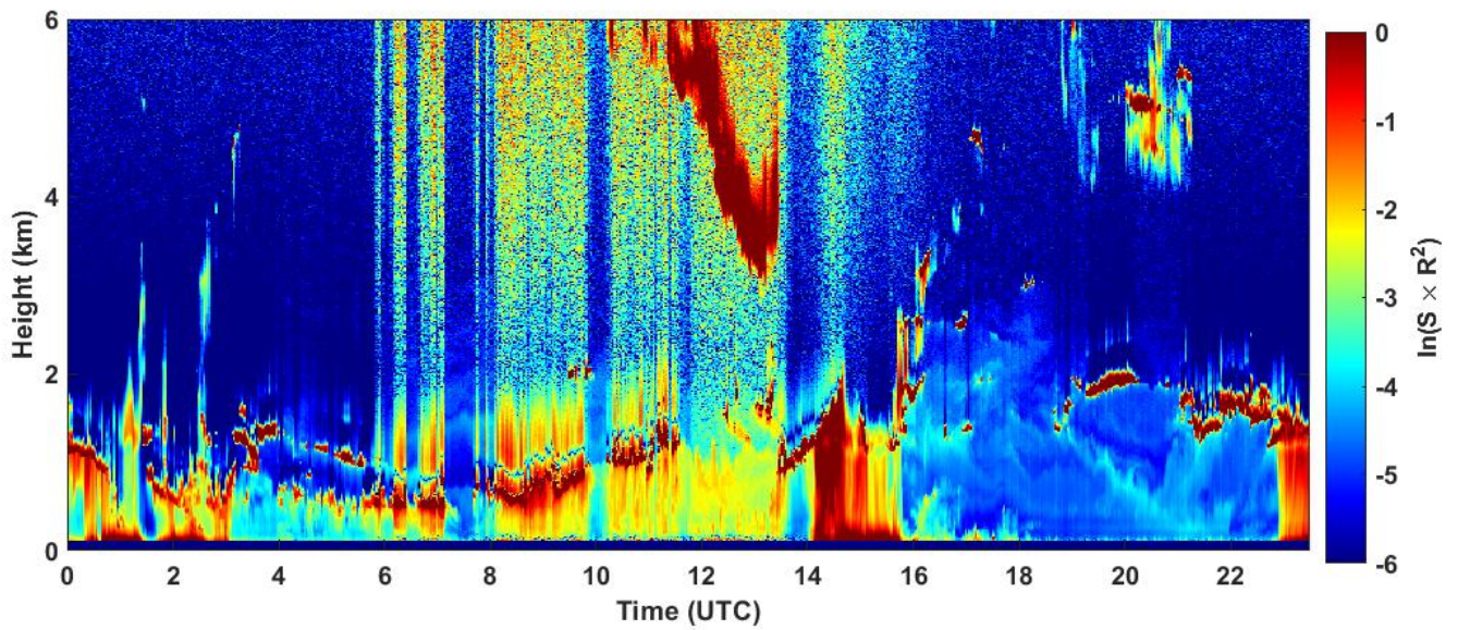
2023-03-04 RCS quick look CHM15k - ILVA LIDAR3 AGGLOMERATO
