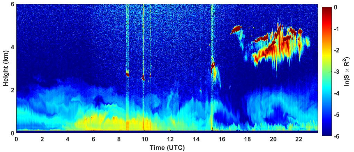
2023-03-02 RCS quick look CHM15k - ILVA LIDAR3 AGGLOMERATO
