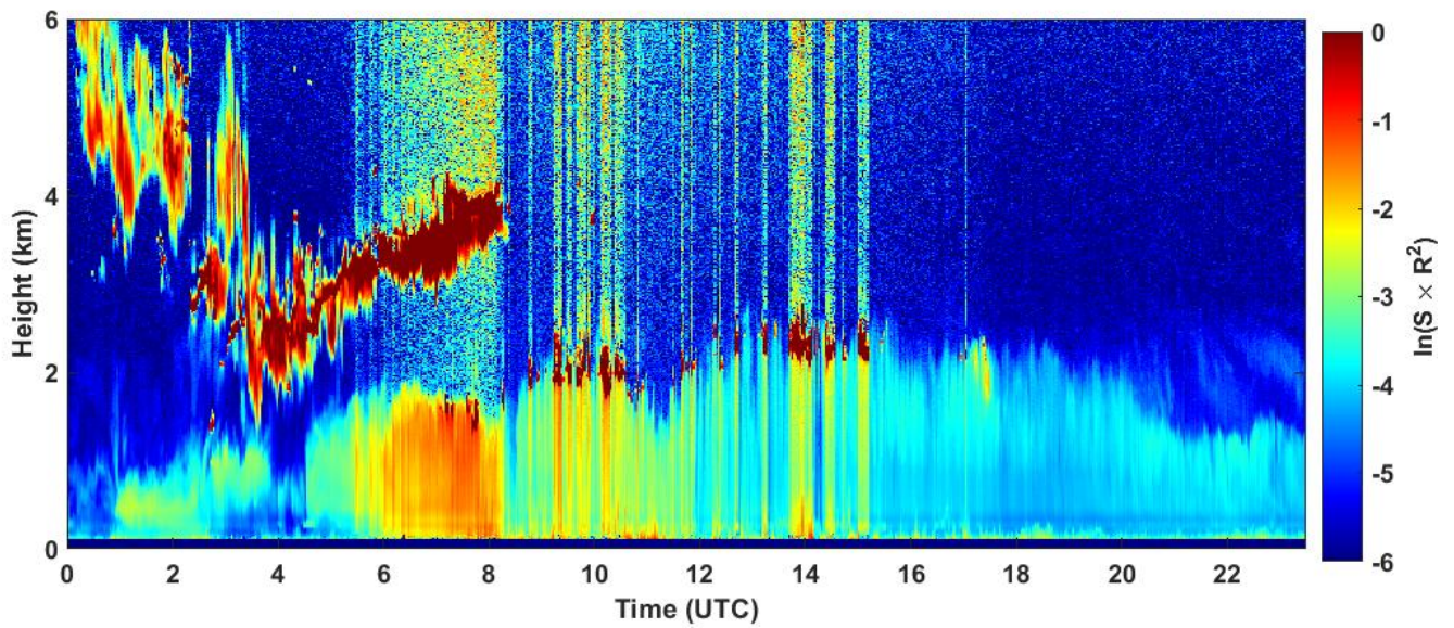
2023-03-28 RCS quick look CHM15k - ILVA LIDAR3 AGGLOMERATO
