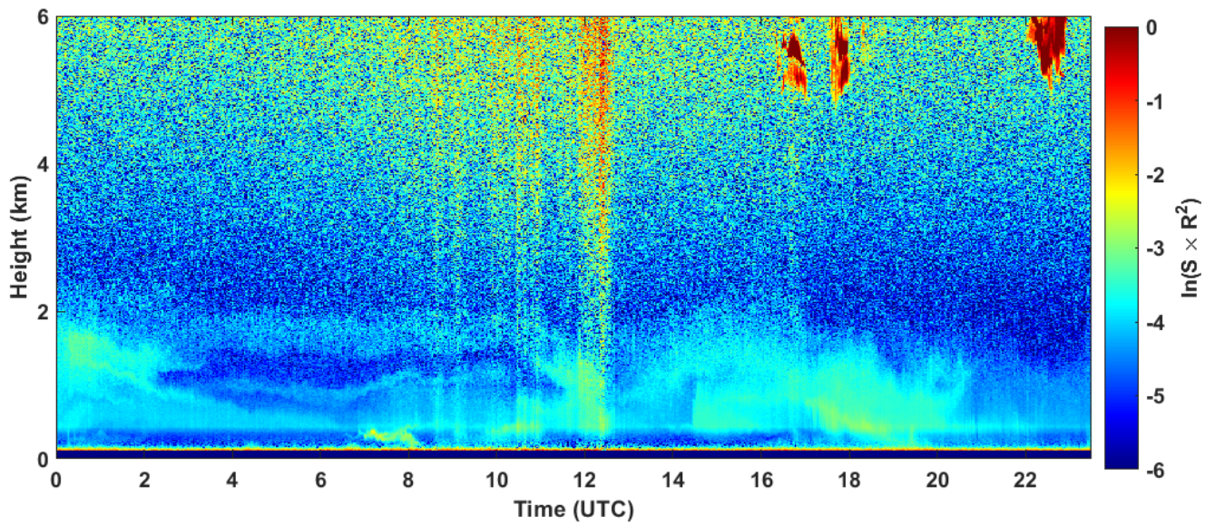
2023-03-26 RCS quick look CHM15k - ILVA LIDAR2 PARCHI
