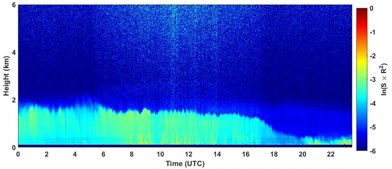
2023-03-18 RCS quick look CHM15k - ILVA LIDAR3 AGGLOMERATO
