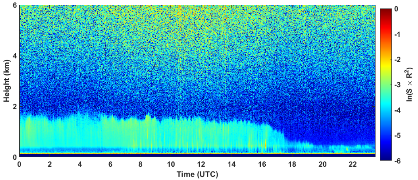
2023-03-18 RCS quick look CHM15k - ILVA LIDAR2 PARCHI
