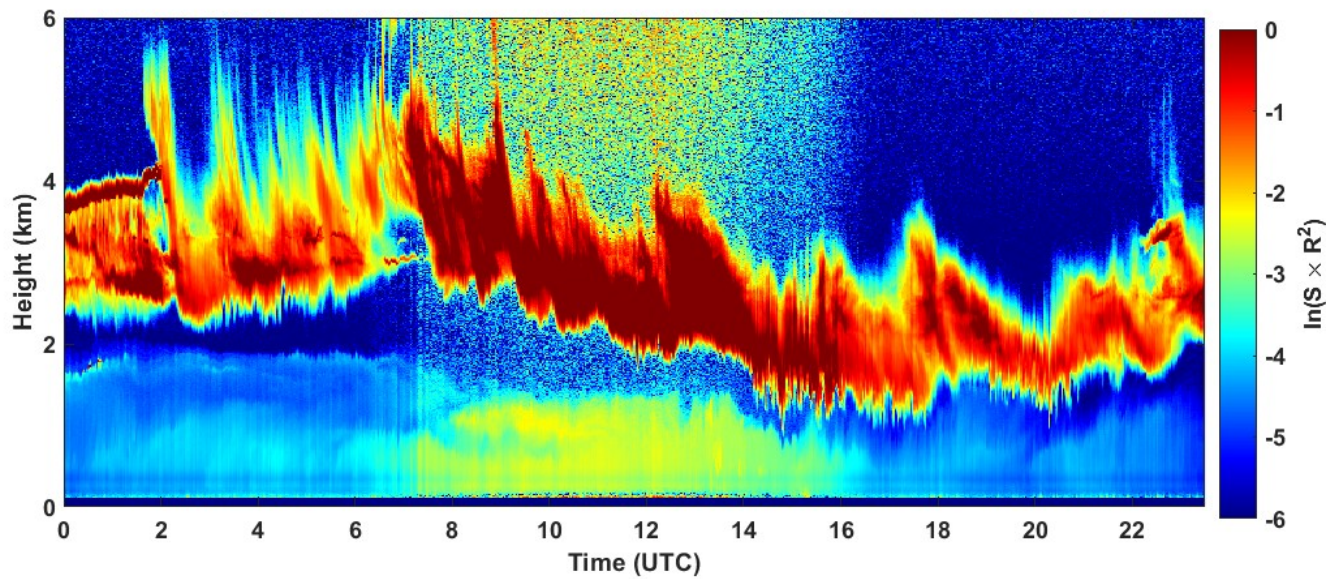
2023-02-10 RCS quick look CHM15k - ILVA LIDAR3 AGGLOMERATO
