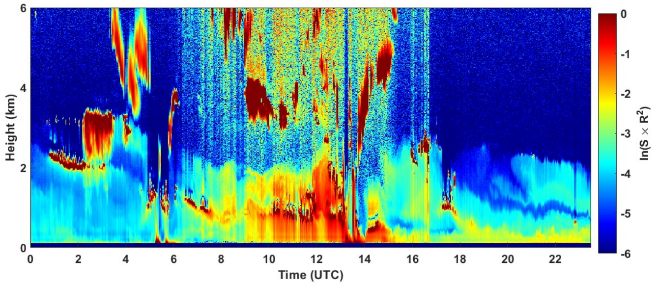
2023-02-28 RCS quick look CHM15k - ILVA LIDAR3 AGGLOMERATO
