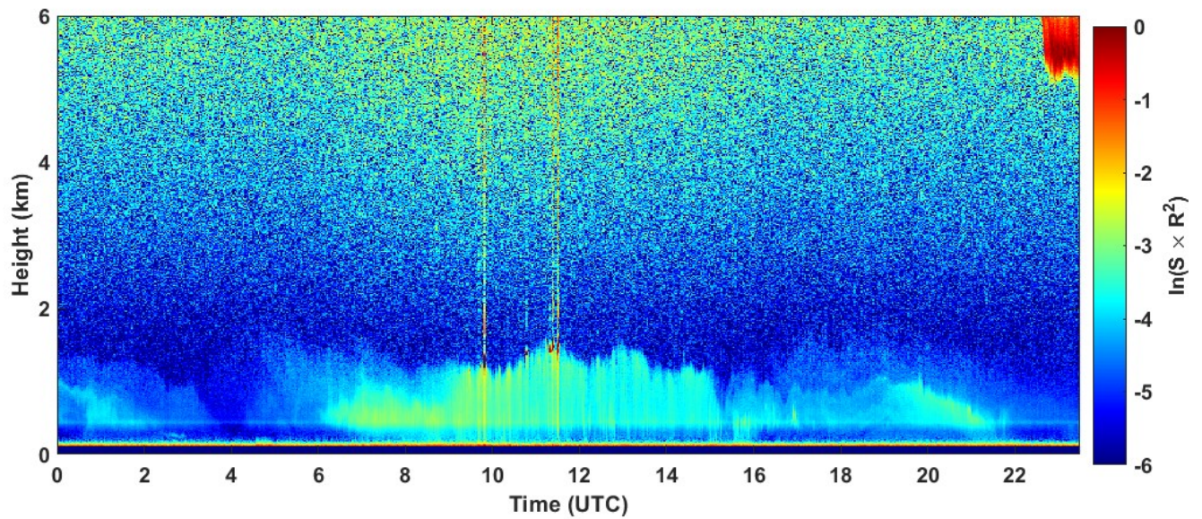
2023-02-04 RCS quick look CHM15k - ILVA LIDAR2 PARCHI
