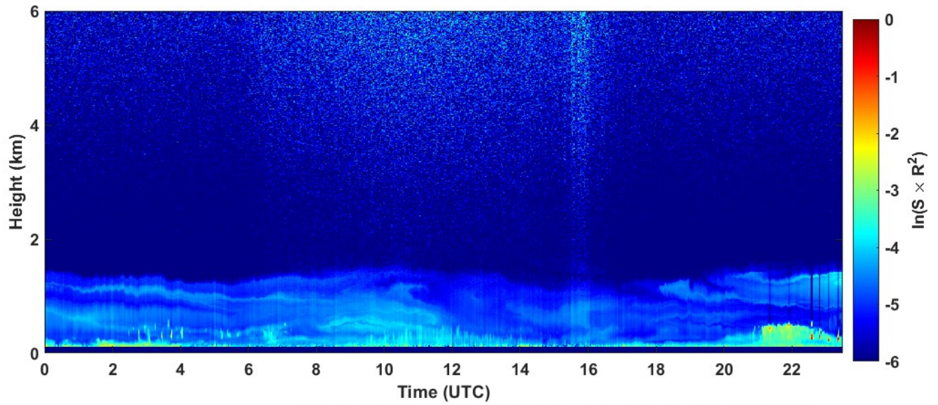
2023-02-22 RCS quick look CHM15k - ILVA LIDAR3 AGGLOMERATO
