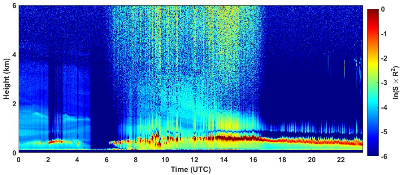
2023-02-24 RCS quick look CHM15k - ILVA LIDAR3 AGGLOMERATO
