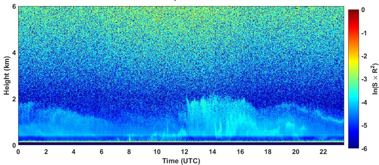
2023-02-02 RCS quick look CHM15k - ILVA LIDAR2 PARCHI
