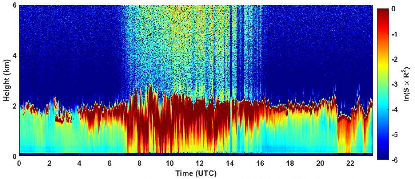
2023-02-06 RCS quick look CHM15k - ILVA LIDAR3 AGGLOMERATO
