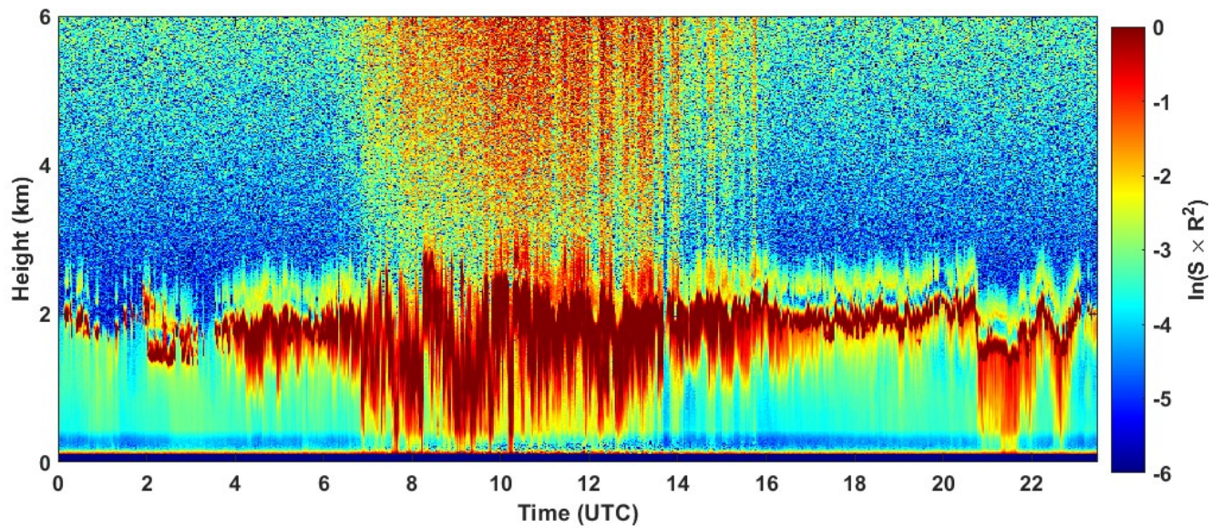
2023-02-06 RCS quick look CHM15k - ILVA LIDAR2 PARCHI
