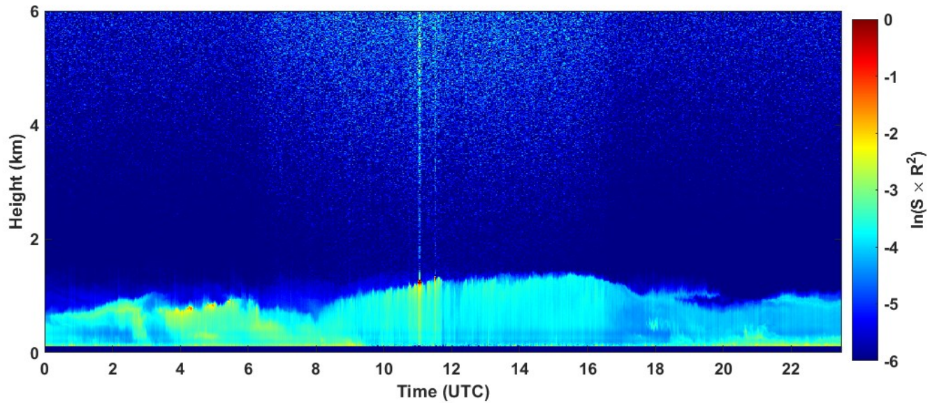
2023-02-16 RCS quick look CHM15k - ILVA LIDAR3 AGGLOMERATO
