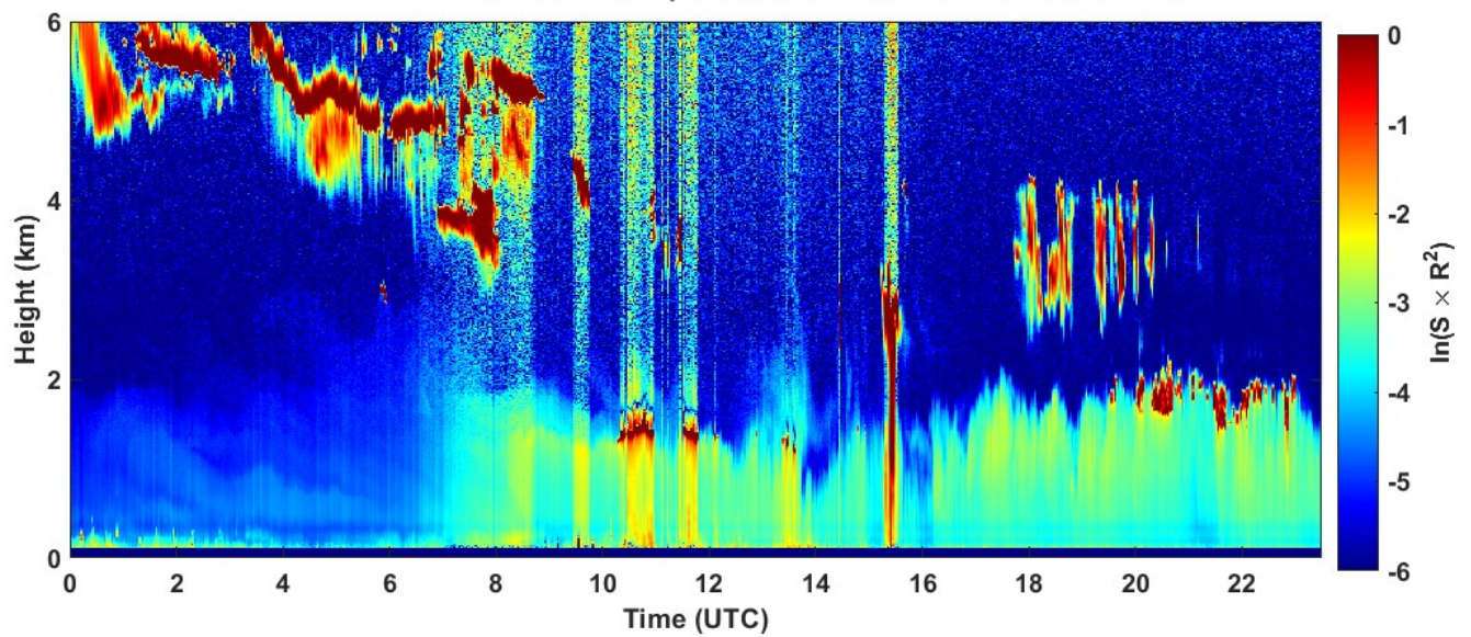
2023-02-04 RCS quick look CHM15k - ILVA LIDAR3 AGGLOMERATO
