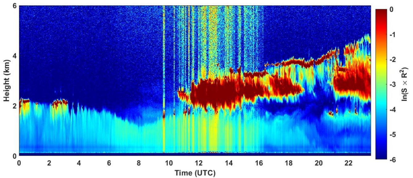
2023-02-08 RCS quick look CHM15k - ILVA LIDAR3 AGGLOMERATO
