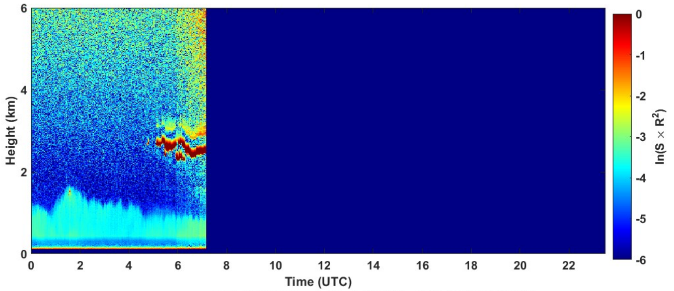
2023-02-28 RCS quick look CHM15k - ILVA LIDAR2 PARCHI
