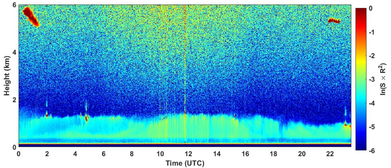
2023-02-12 RCS quick look CHM15k - ILVA LIDAR2 PARCHI
