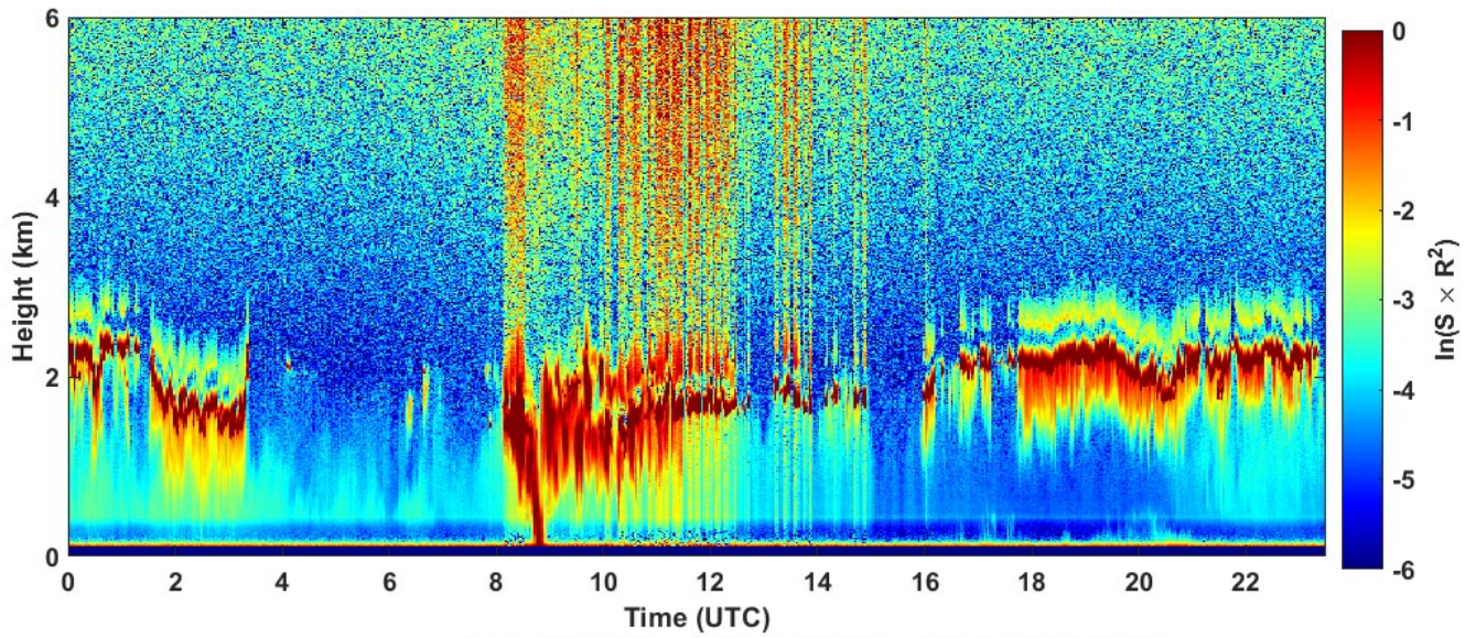
2023-02-08 RCS quick look CHM15k - ILVA LIDAR2 PARCHI
