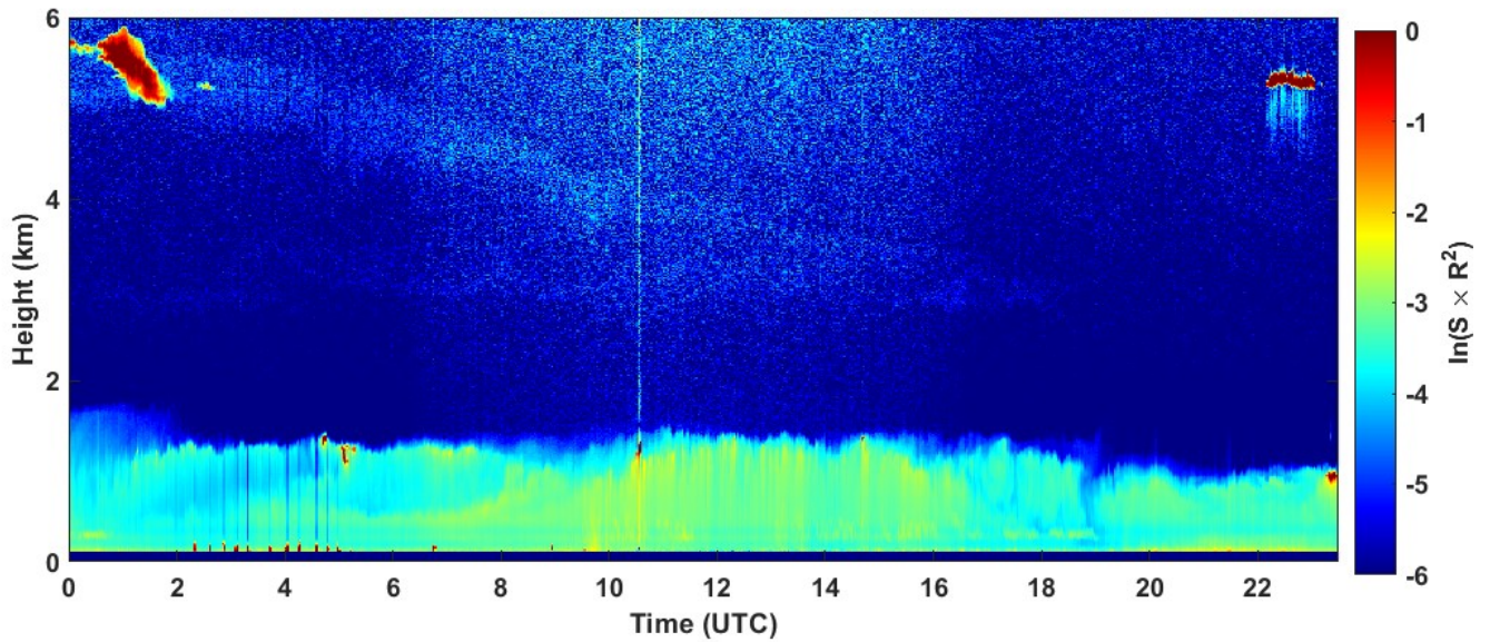
2023-02-12 RCS quick look CHM15k - ILVA LIDAR3 AGGLOMERATO
