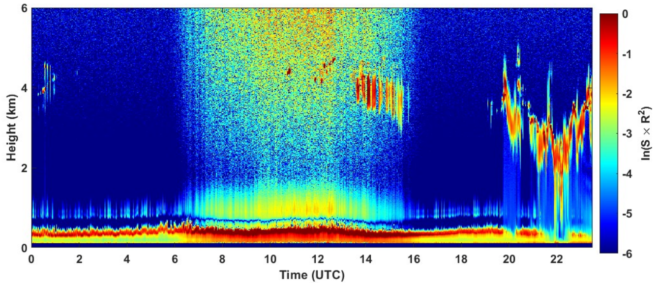
2023-02-26 RCS quick look CHM15k - ILVA LIDAR3 AGGLOMERATO
