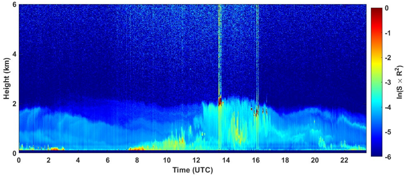
2023-02-02 RCS quick look CHM15k - ILVA LIDAR3 AGGLOMERATO
