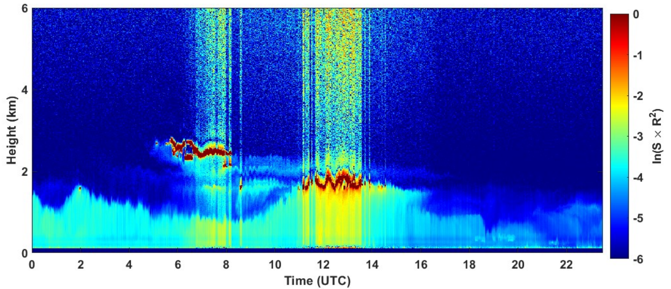
2023-02-14 RCS quick look CHM15k - ILVA LIDAR3 AGGLOMERATO
