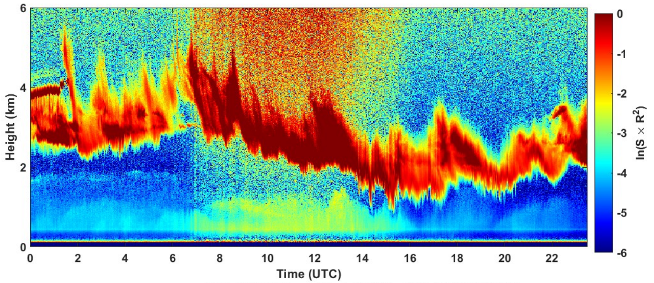
2023-02-10 RCS quick look CHM15k - ILVA LIDAR2 PARCHI
