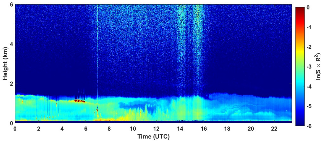
2023-02-18 RCS quick look CHM15k - ILVA LIDAR3 AGGLOMERATO
