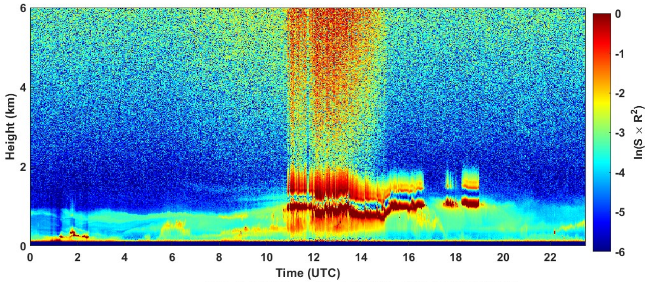
2023-01-04 RCS quick look CHM15k - ILVA LIDAR2 PARCHI
