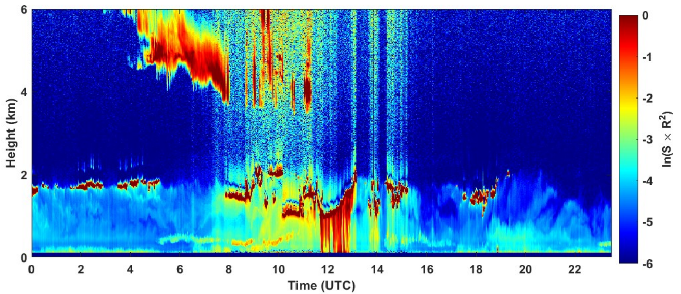
2023-01-12 RCS quick look CHM15k - ILVA LIDAR3 AGGLOMERATO
