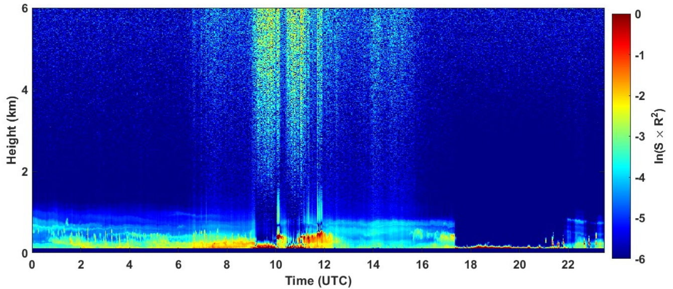
2023-01-02 RCS quick look CHM15k - ILVA LIDAR3 AGGLOMERATO
