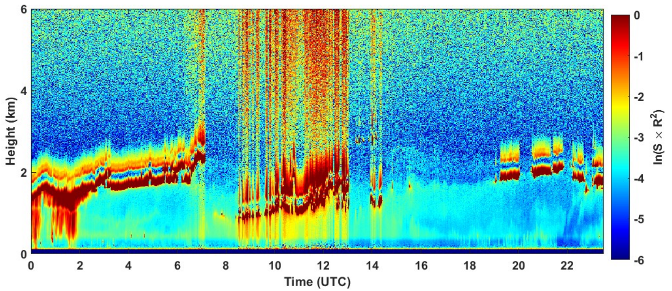
2023-01-28 RCS quick look CHM15k - ILVA LIDAR2 PARCHI
