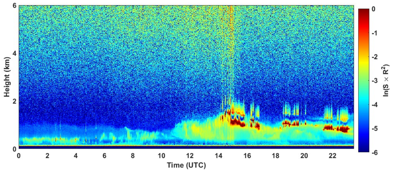
2023-01-08 RCS quick look CHM15k - ILVA LIDAR2 PARCHI
