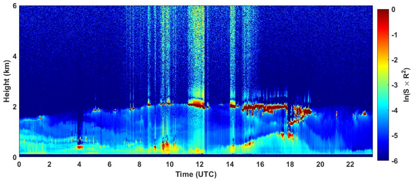
2023-01-08 RCS quick look CHM15k - ILVA LIDAR3 AGGLOMERATO
