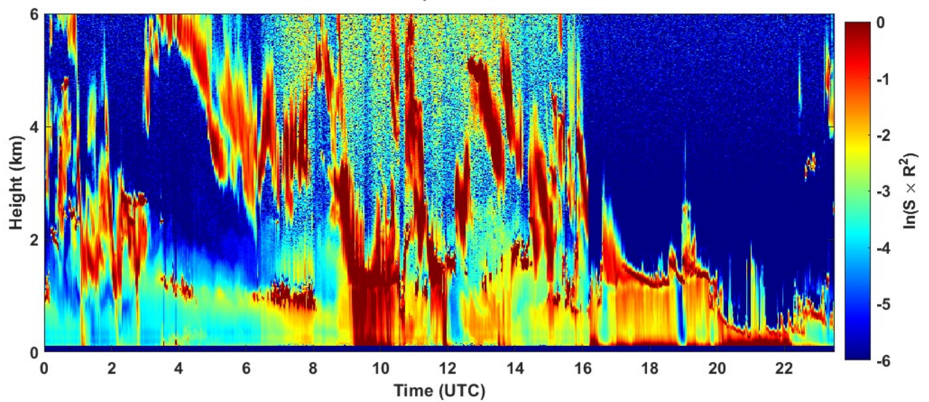
2023-01-22 RCS quick look CHM15k - ILVA LIDAR3 AGGLOMERATO
