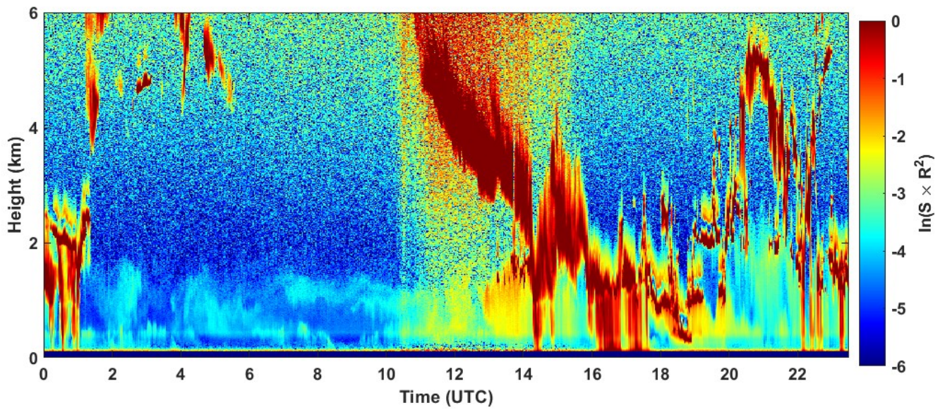
2023-01-20 RCS quick look CHM15k - ILVA LIDAR2 PARCHI
