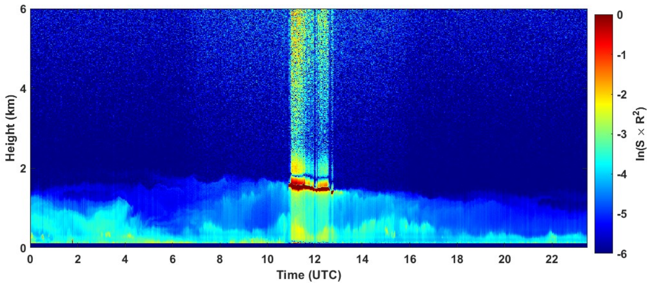
2023-01-06 RCS quick look CHM15k - ILVA LIDAR3 AGGLOMERATO
