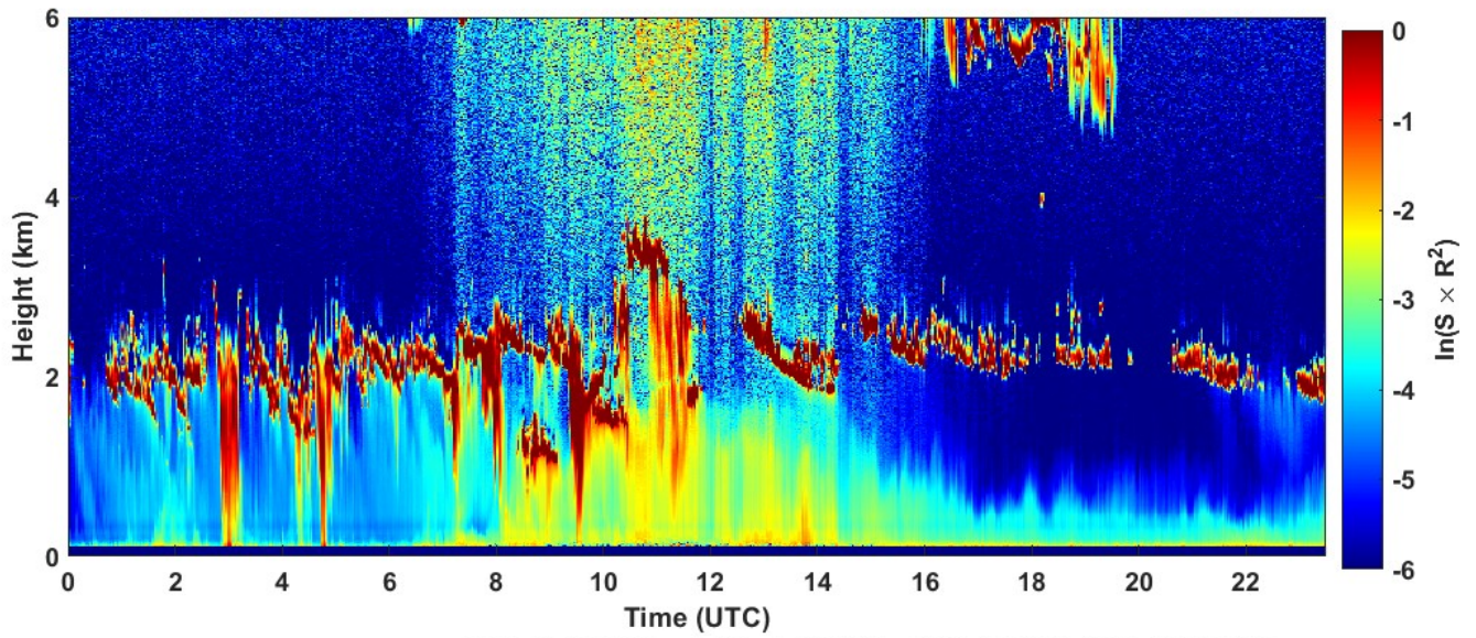
2023-01-18 RCS quick look CHM15k - ILVA LIDAR3 AGGLOMERATO
