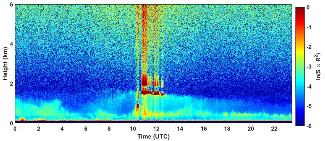
2023-01-06 RCS quick look CHM15k - ILVA LIDAR2 PARCHI
