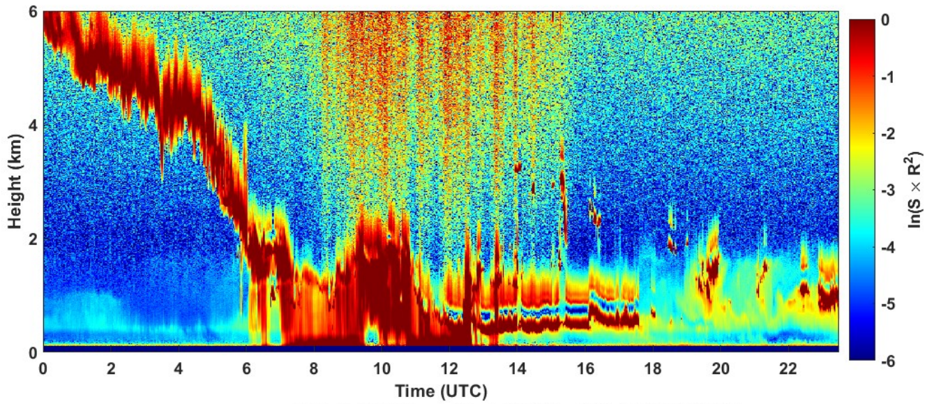
2023-01-26 RCS quick look CHM15k - ILVA LIDAR2 PARCHI
