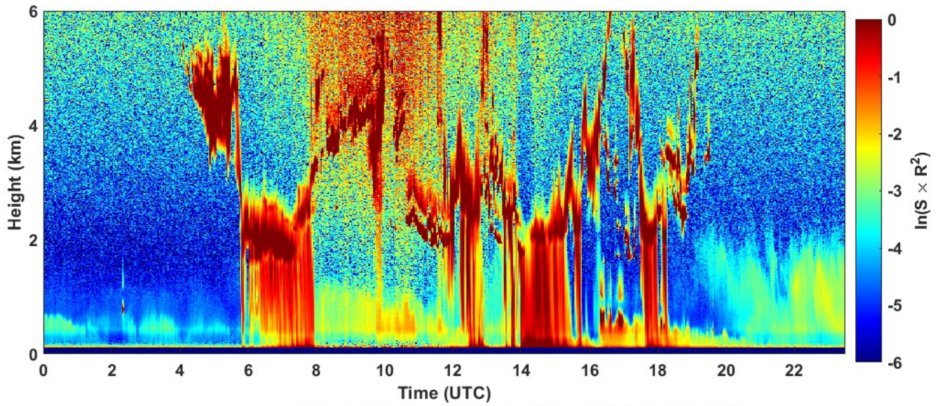
2023-01-10 RCS quick look CHM15k - ILVA LIDAR2 PARCHI
