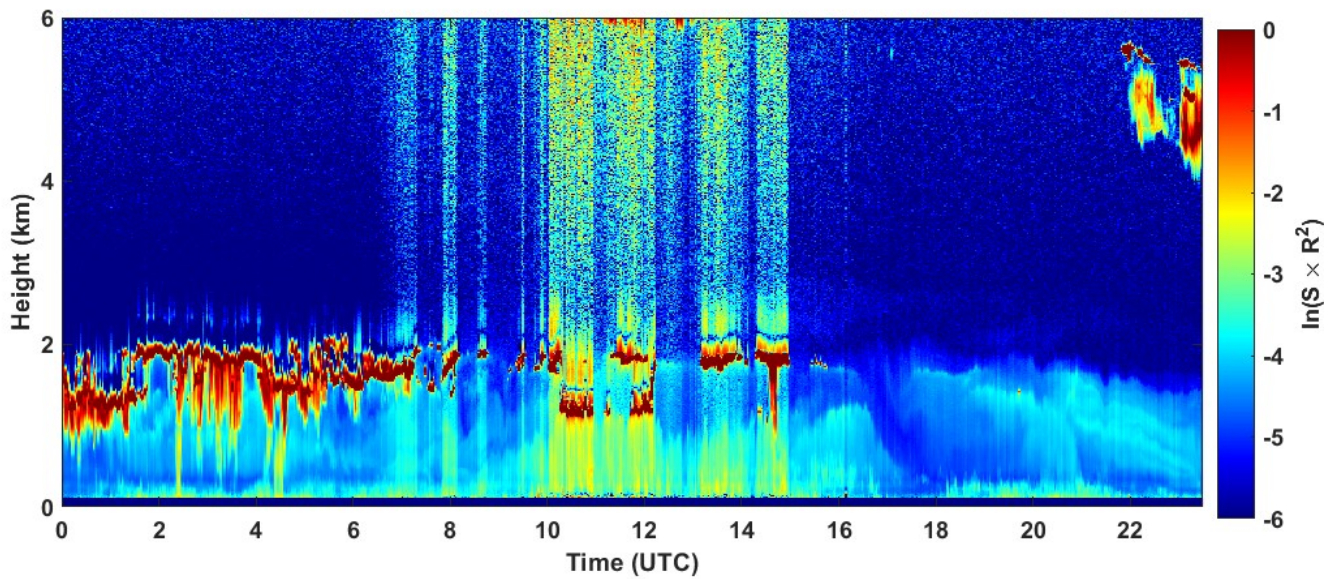
2023-01-30 RCS quick look CHM15k - ILVA LIDAR3 AGGLOMERATO
