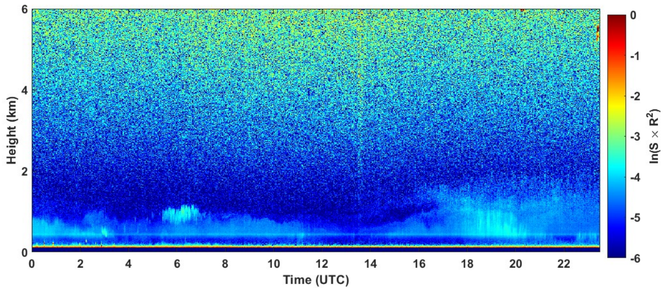
2023-01-16 RCS quick look CHM15k - ILVA LIDAR2 PARCHI
