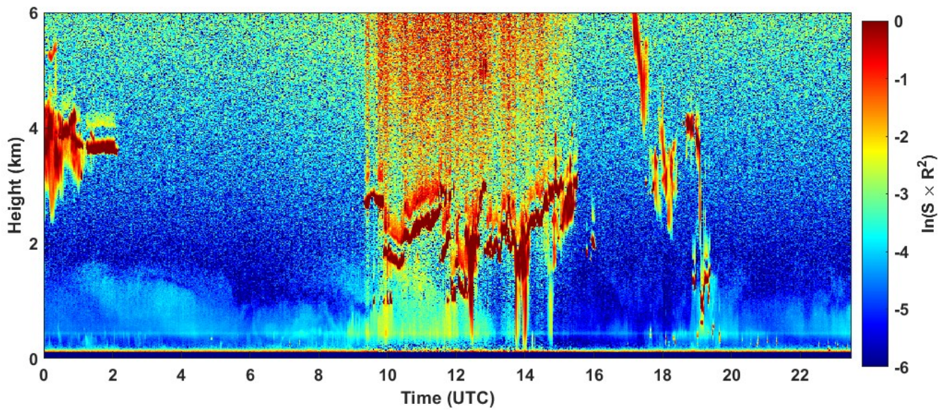
2023-01-14 RCS quick look CHM15k - ILVA LIDAR2 PARCHI
