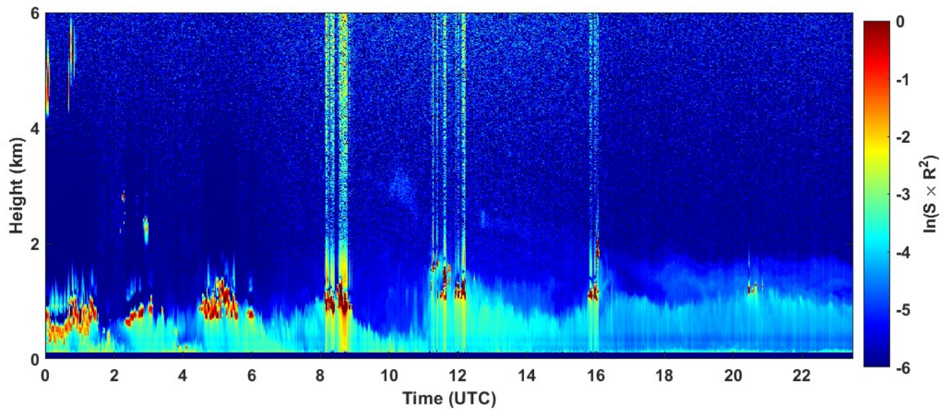
2023-01-24 RCS quick look CHM15k - ILVA LIDAR3 AGGLOMERATO
