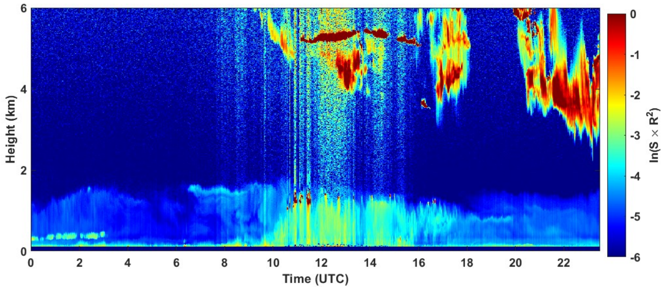
2023-01-14 RCS quick look CHM15k - ILVA LIDAR3 AGGLOMERATO
