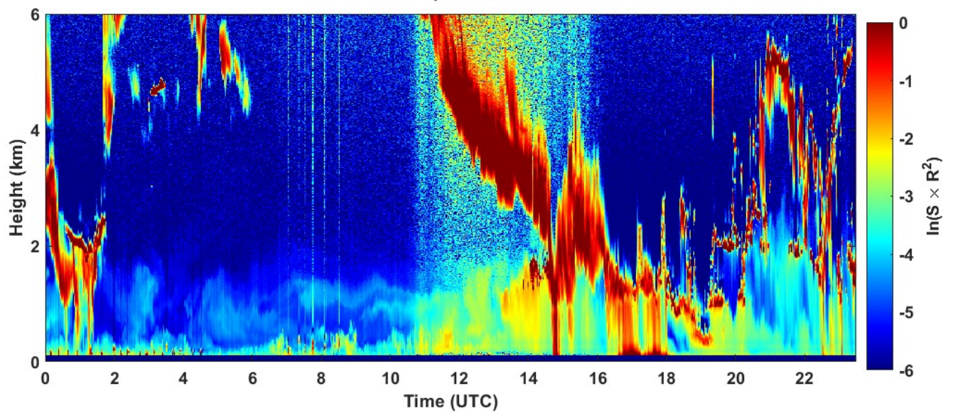
2023-01-20 RCS quick look CHM15k - ILVA LIDAR3 AGGLOMERATO
