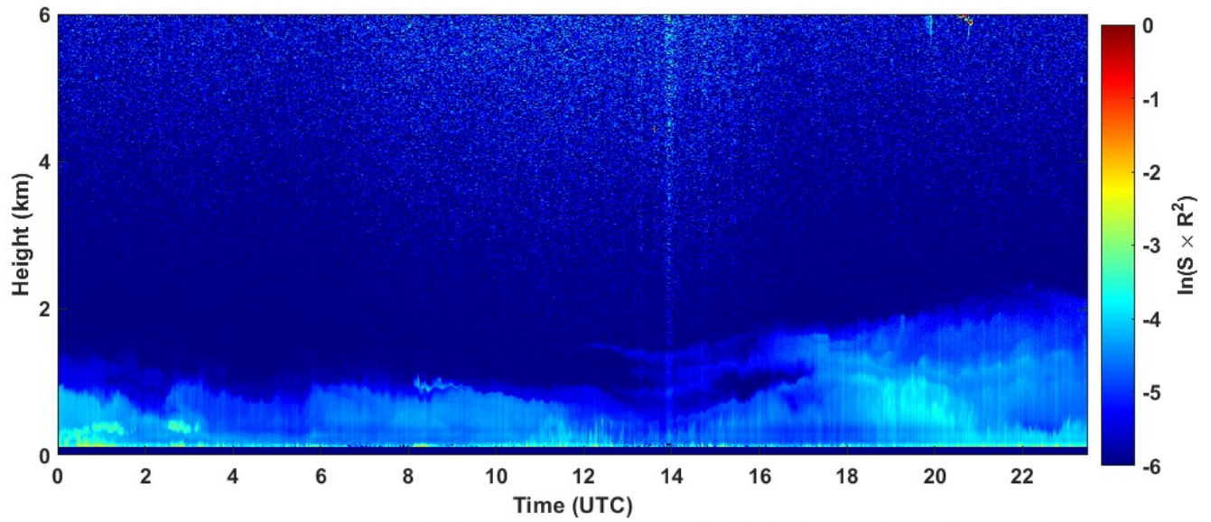
2023-01-16 RCS quick look CHM15k - ILVA LIDAR3 AGGLOMERATO
