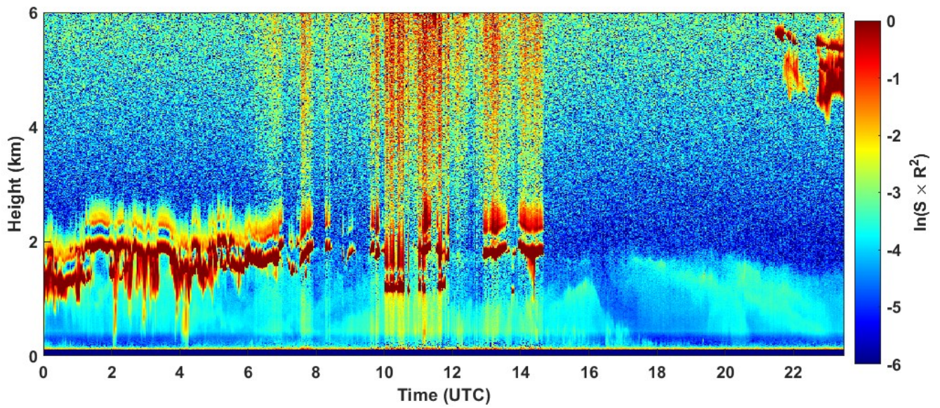
2023-01-30 RCS quick look CHM15k - ILVA LIDAR2 PARCHI
