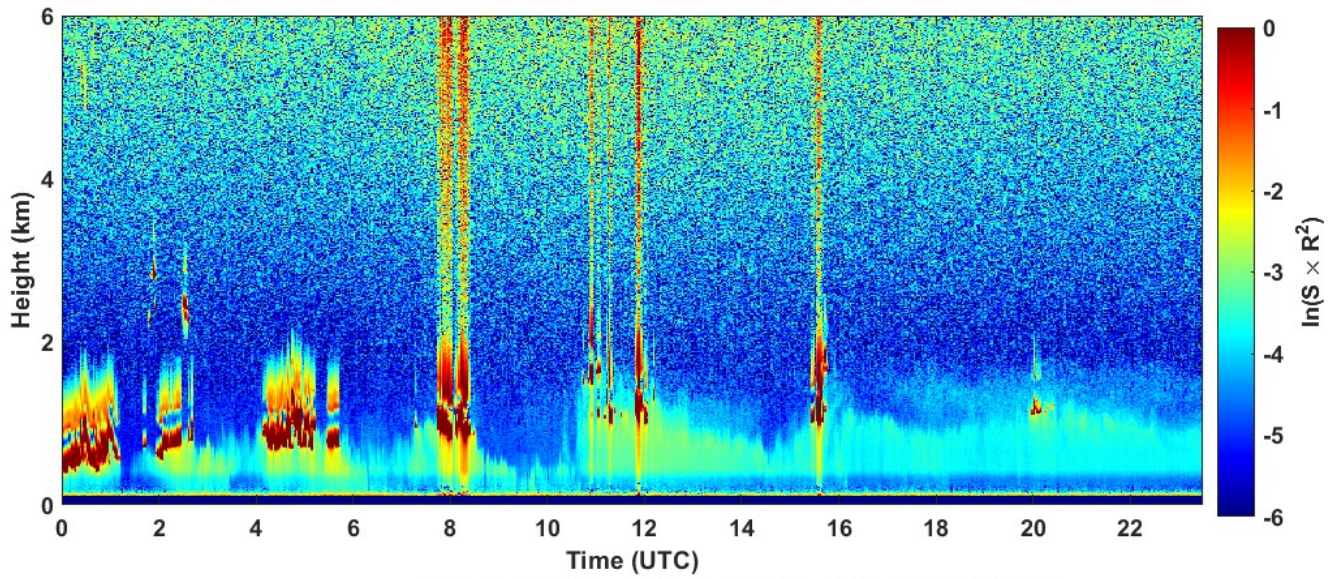
2023-01-24 RCS quick look CHM15k - ILVA LIDAR2 PARCHI
