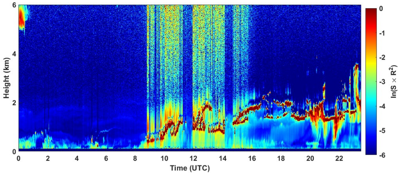
2023-01-28 RCS quick look CHM15k - ILVA LIDAR3 AGGLOMERATO
