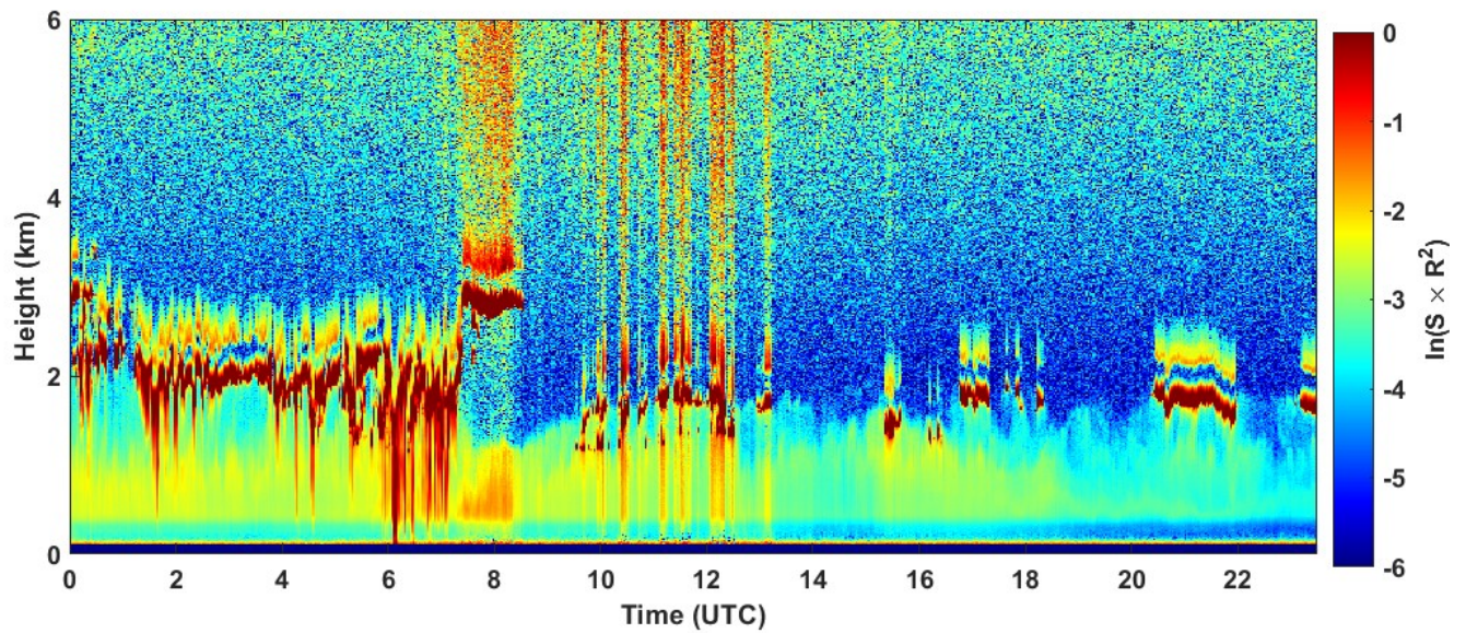
2023-01-12 RCS quick look CHM15k - ILVA LIDAR2 PARCHI
