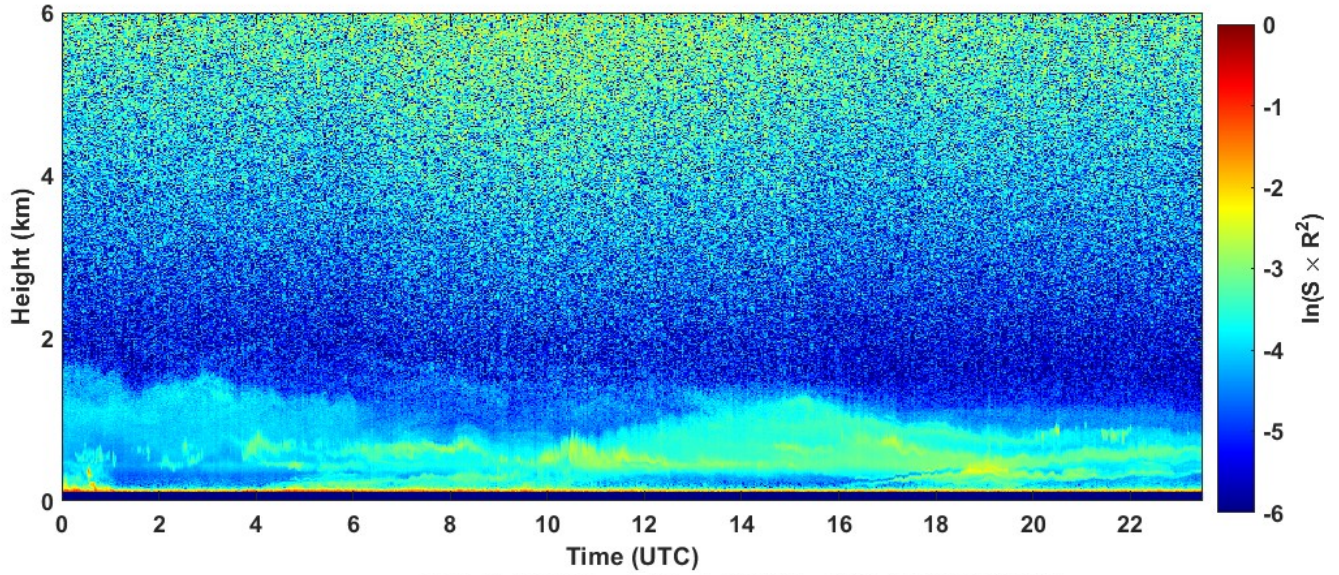
2023-01-02 RCS quick look CHM15k - ILVA LIDAR2 PARCHI
