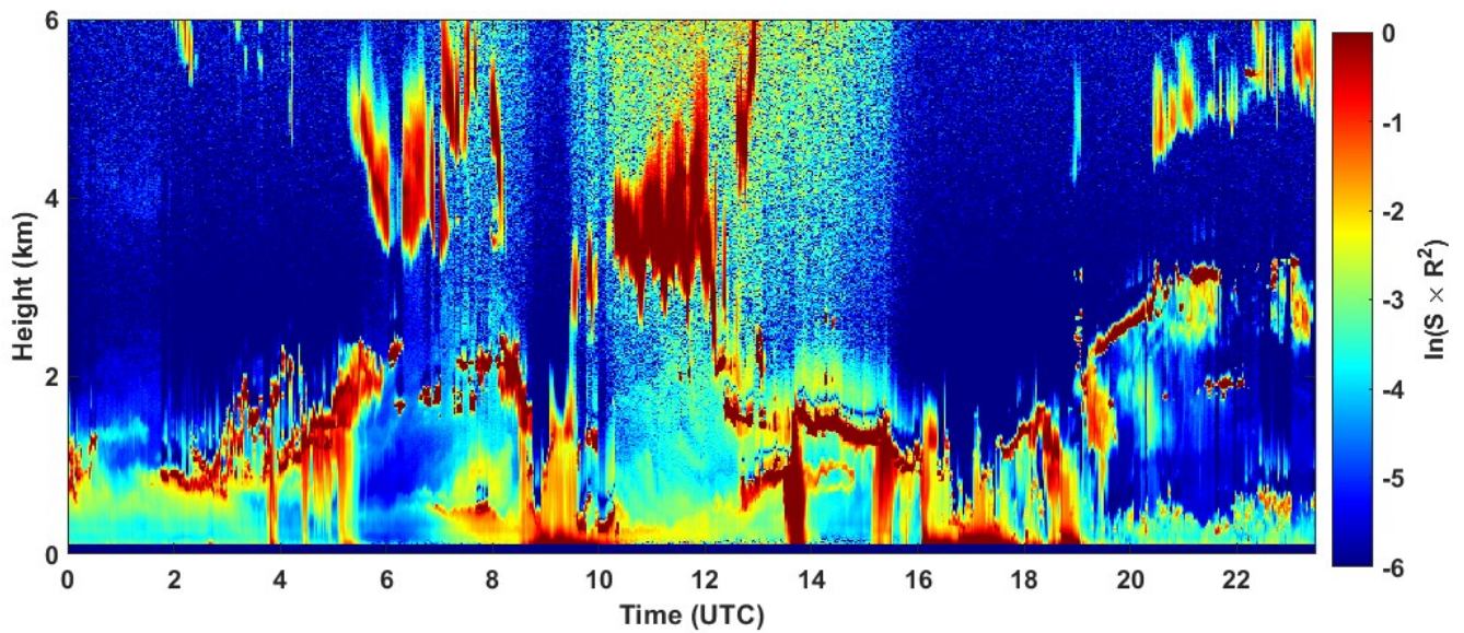
2023-01-26 RCS quick look CHM15k - ILVA LIDAR3 AGGLOMERATO
