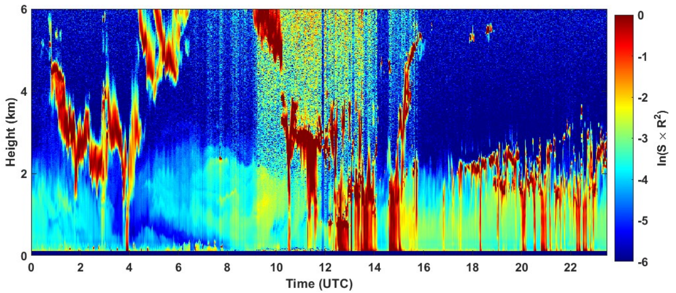
2023-01-10 RCS quick look CHM15k - ILVA LIDAR3 AGGLOMERATO
