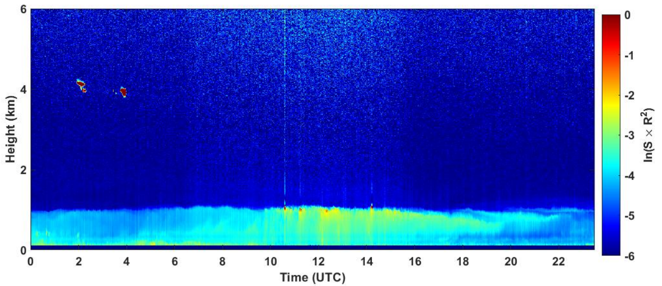
2022-12-20 RCS quick look CHM15k - ILVA LIDAR3 AGGLOMERATO
