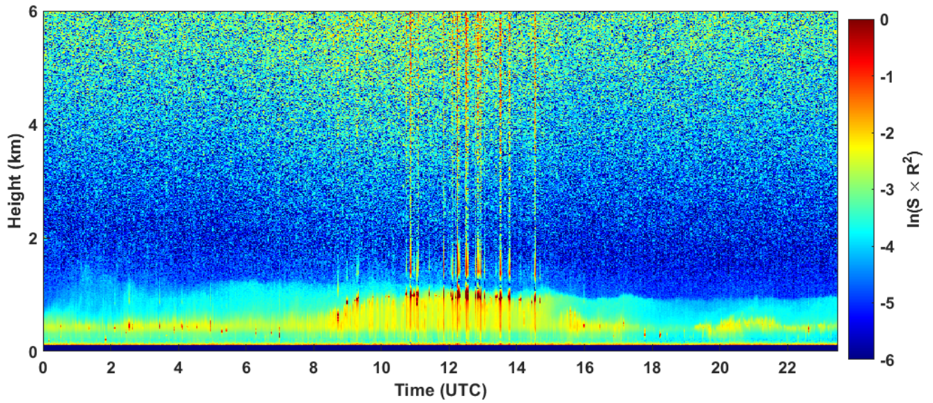
2022-12-20 RCS quick look CHM15k - ILVA LIDAR2 PARCHI
