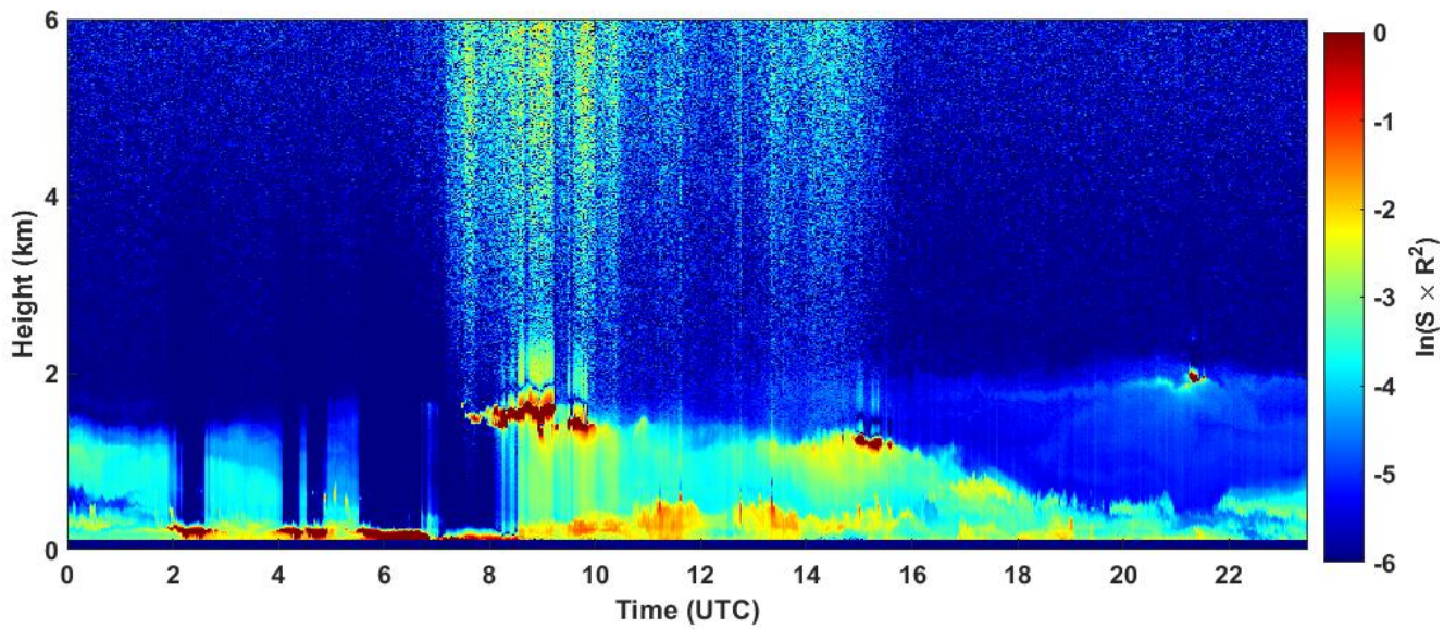
2022-12-24 RCS quick look CHM15k - ILVA LIDAR3 AGGLOMERATO
