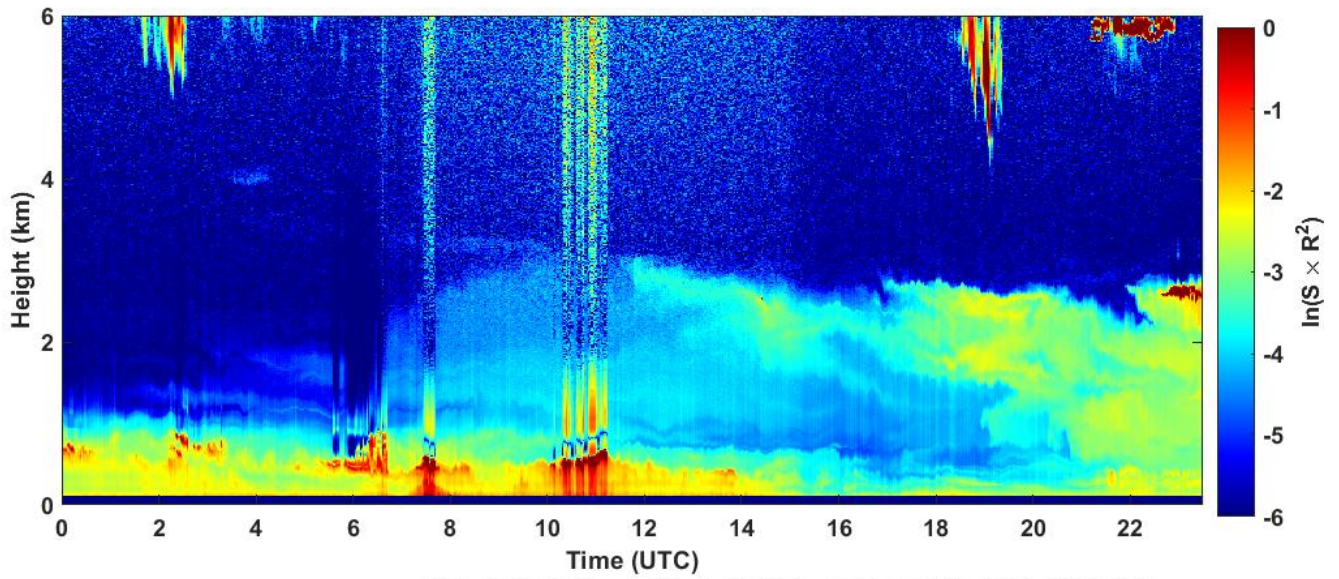
2022-12-08 RCS quick look CHM15k - ILVA LIDAR3 AGGLOMERATO
