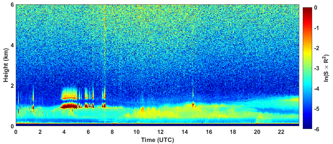
2022-12-22 RCS quick look CHM15k - ILVA LIDAR2 PARCHI
