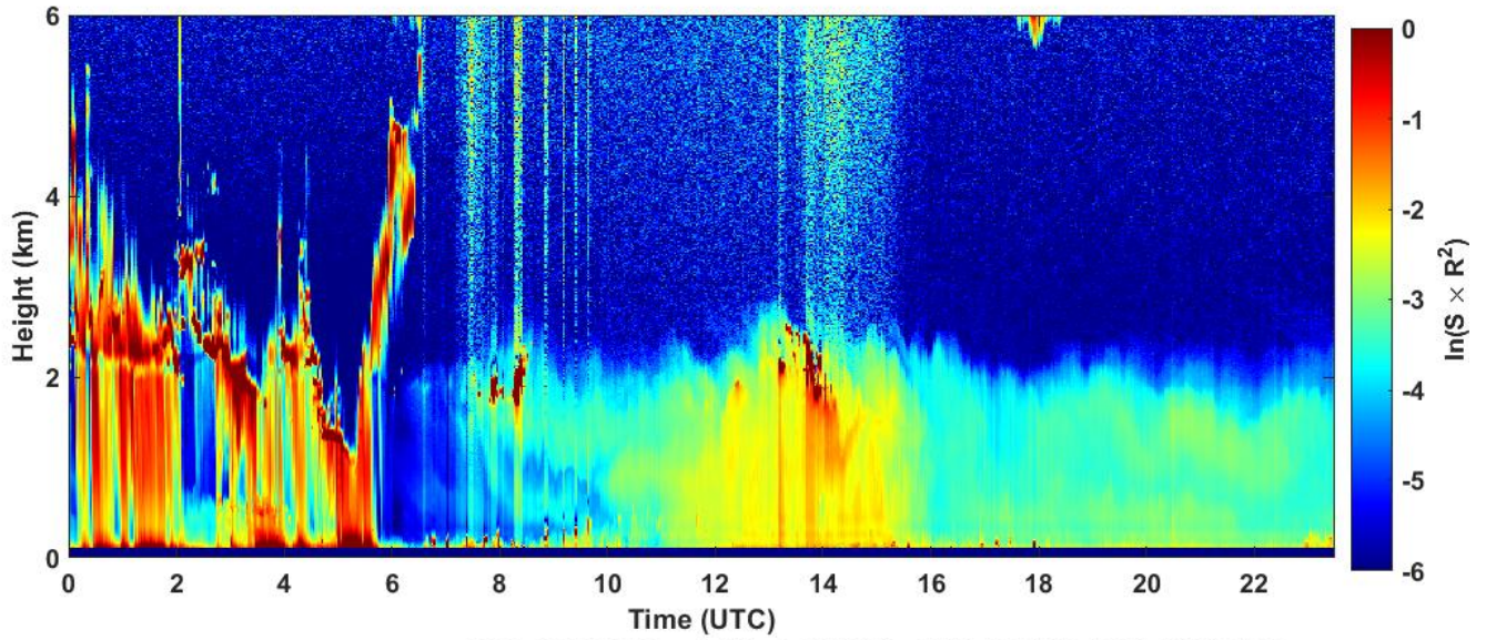
2022-12-12 RCS quick look CHM15k - ILVA LIDAR3 AGGLOMERATO
