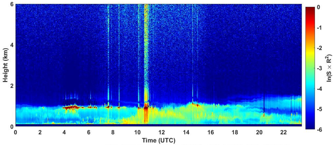
2022-12-22 RCS quick look CHM15k - ILVA LIDAR3 AGGLOMERATO
