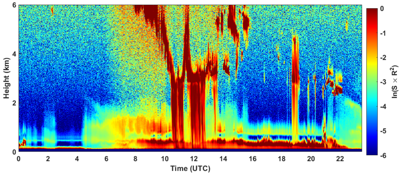
2022-12-10 RCS quick look CHM15k - ILVA LIDAR2 PARCHI
