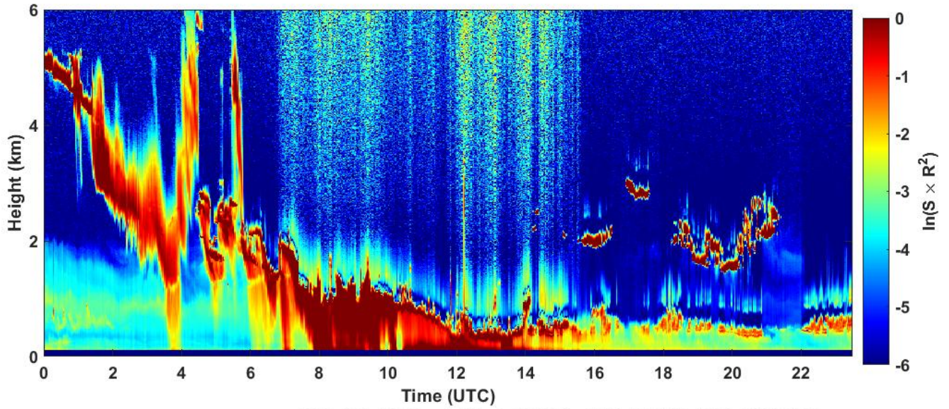
2022-12-14 RCS quick look CHM15k - ILVA LIDAR3 AGGLOMERATO
