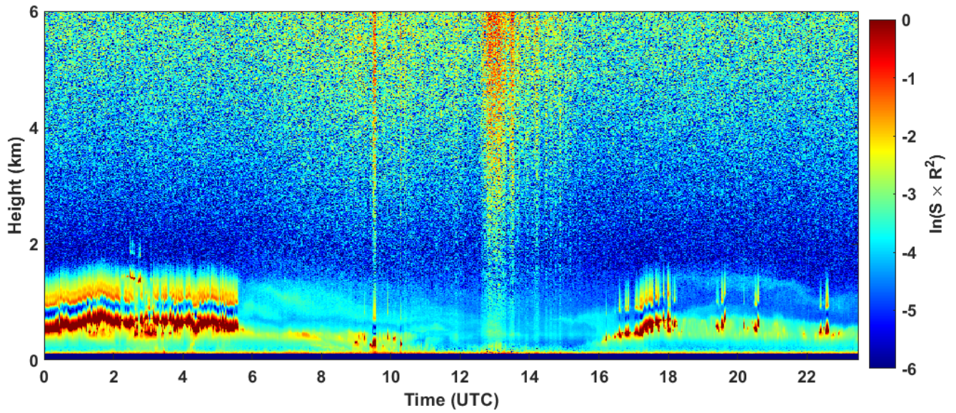
2022-12-30 RCS quick look CHM15k - ILVA LIDAR2 PARCHI
