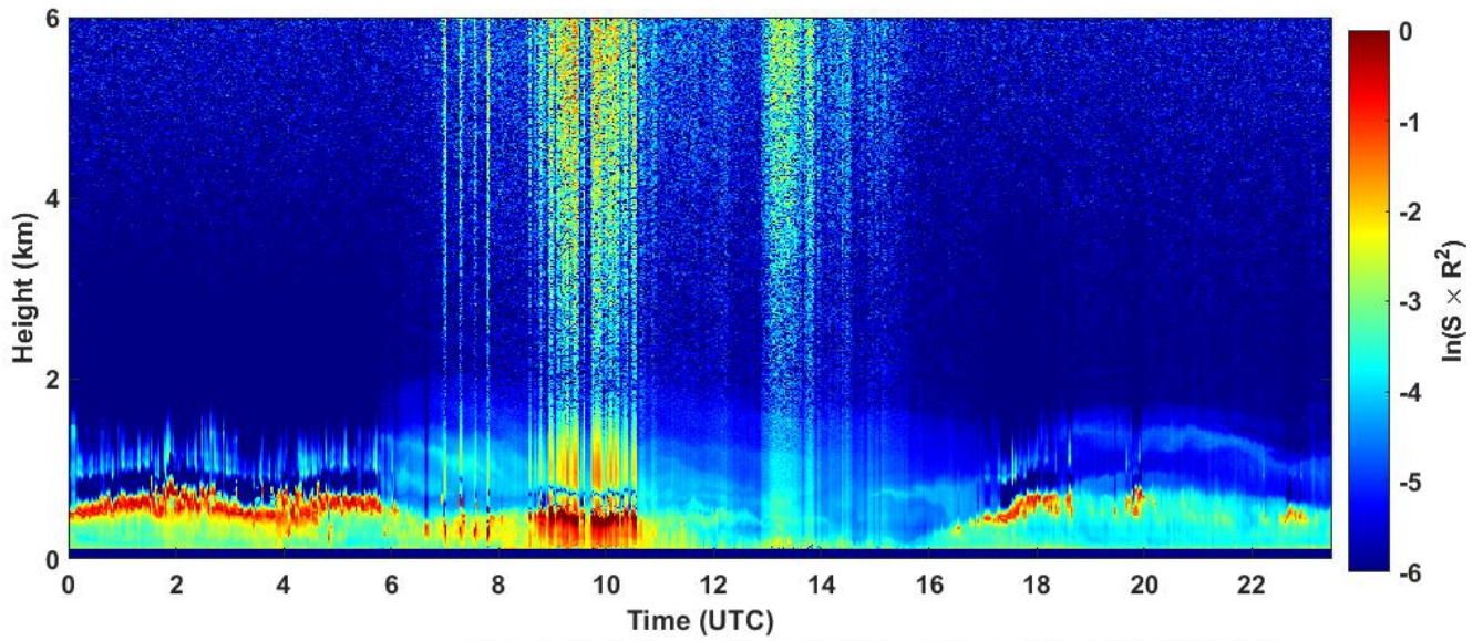
2022-12-30 RCS quick look CHM15k - ILVA LIDAR3 AGGLOMERATO
