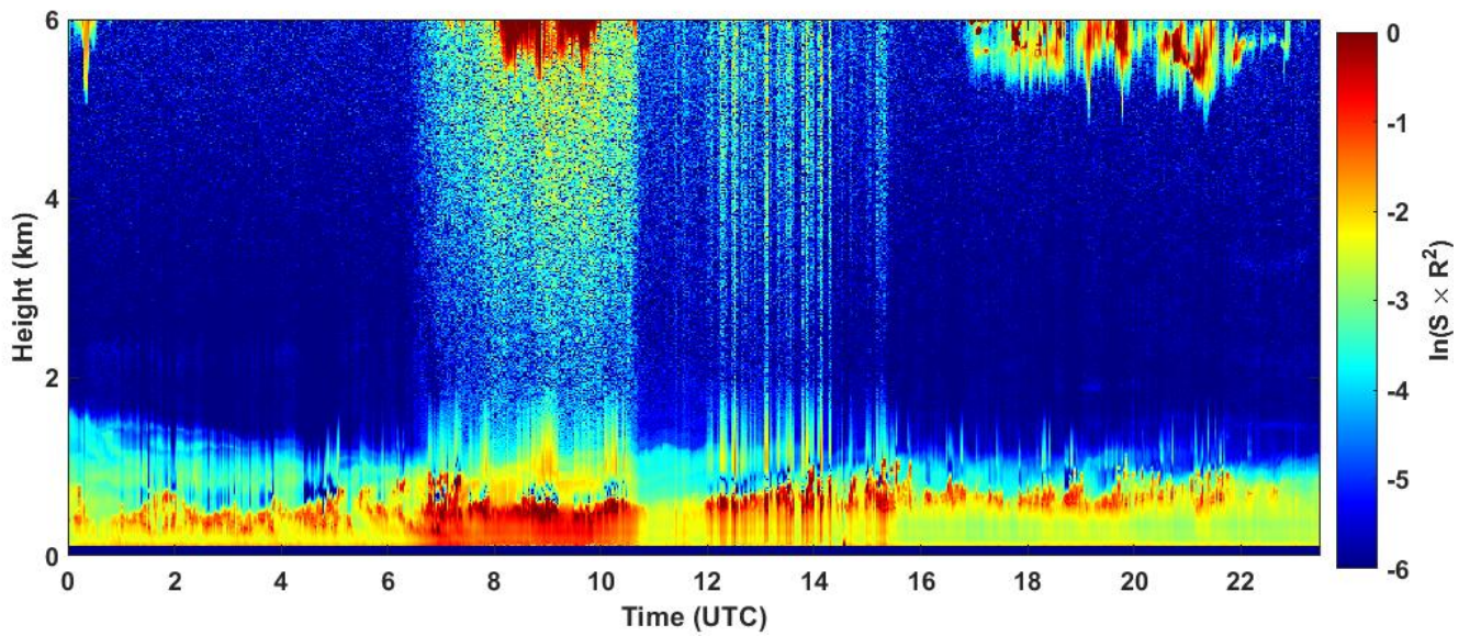
2022-12-06 RCS quick look CHM15k - ILVA LIDAR3 AGGLOMERATO
