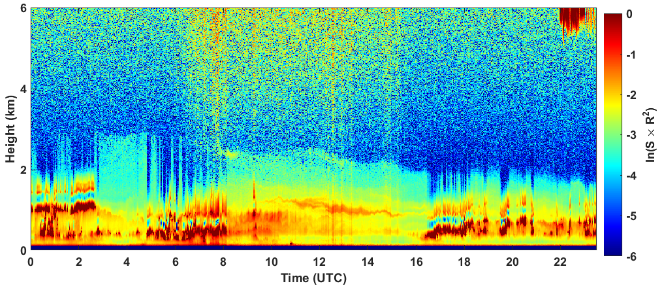
2022-12-06 RCS quick look CHM15k - ILVA LIDAR2 PARCHI
