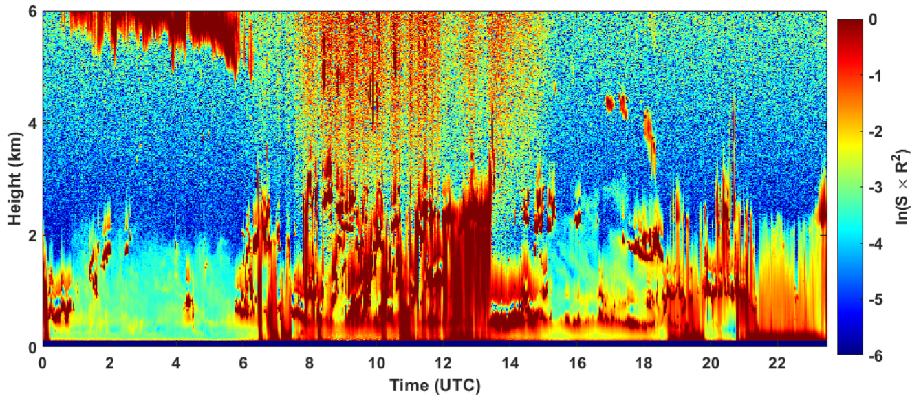
2022-12-04 RCS quick look CHM15k - ILVA LIDAR2 PARCHI
