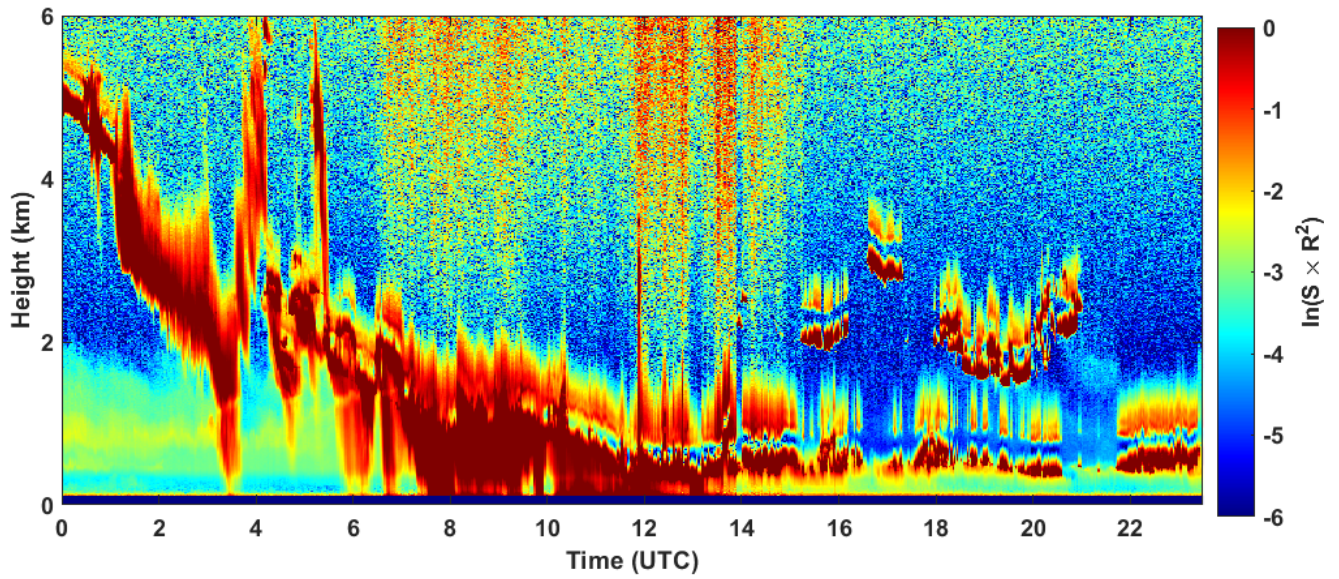
2022-12-14 RCS quick look CHM15k - ILVA LIDAR2 PARCHI
