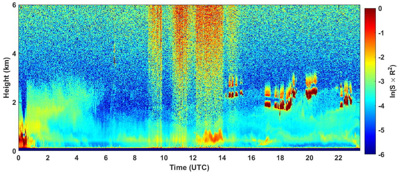
2022-12-18 RCS quick look CHM15k - ILVA LIDAR2 PARCHI
