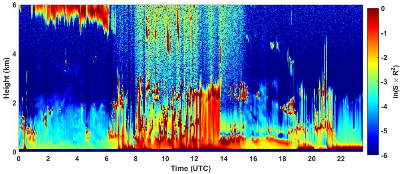
2022-12-04 RCS quick look CHM15k - ILVA LIDAR3 AGGLOMERATO
