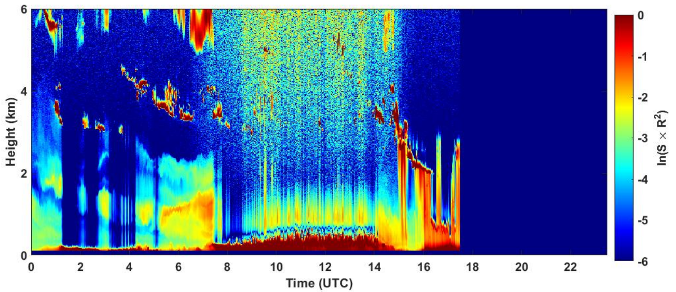
2022-12-10 RCS quick look CHM15k - ILVA LIDAR3 AGGLOMERATO
