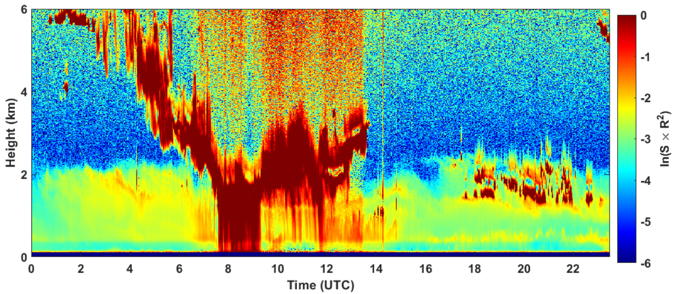
2022-12-12 RCS quick look CHM15k - ILVA LIDAR2 PARCHI
