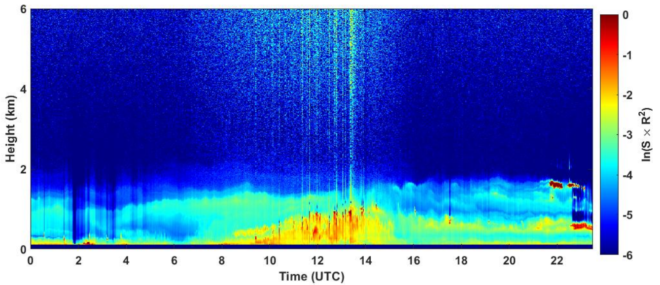
2022-12-28 RCS quick look CHM15k - ILVA LIDAR3 AGGLOMERATO
