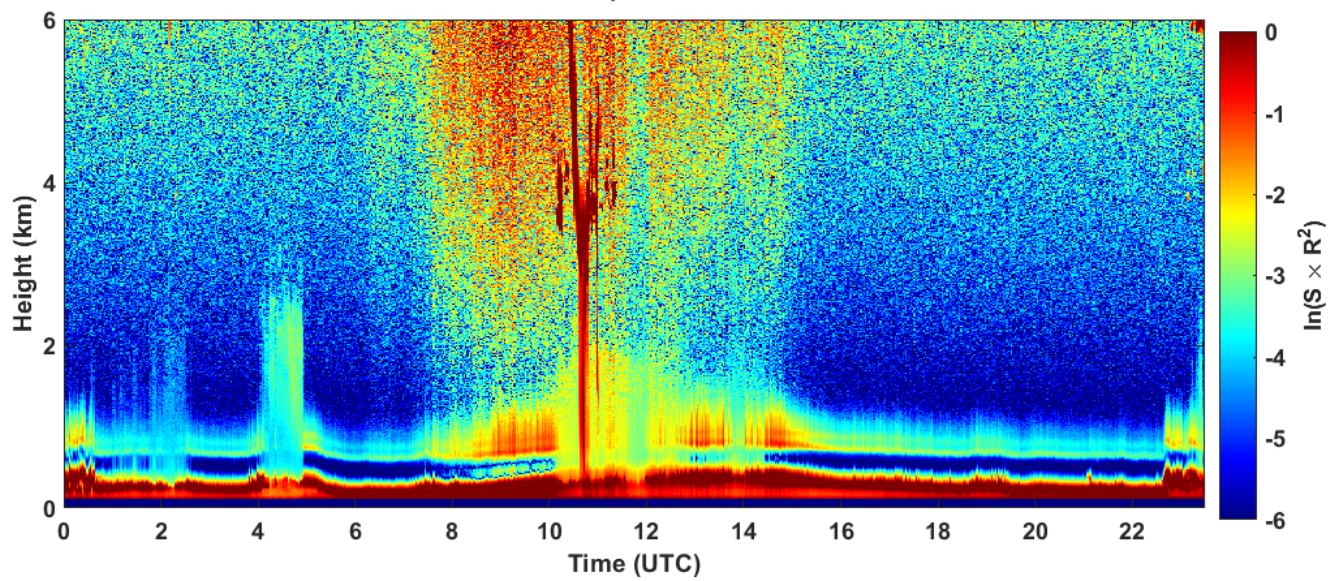
2022-12-16 RCS quick look CHM15k - ILVA LIDAR2 PARCHI
