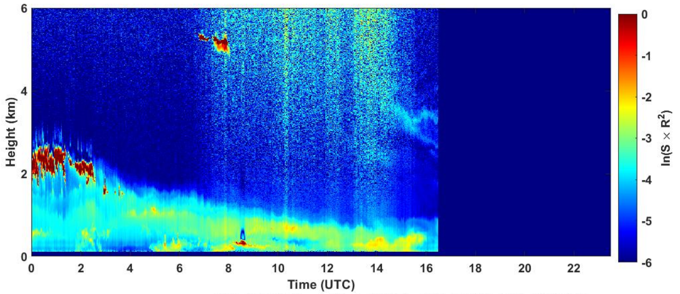
2022-12-16 RCS quick look CHM15k - ILVA LIDAR3 AGGLOMERATO
