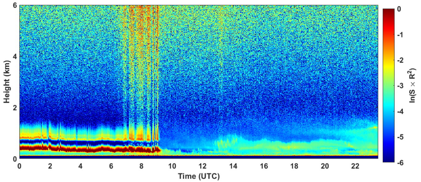
2022-12-28 RCS quick look CHM15k - ILVA LIDAR2 PARCHI
