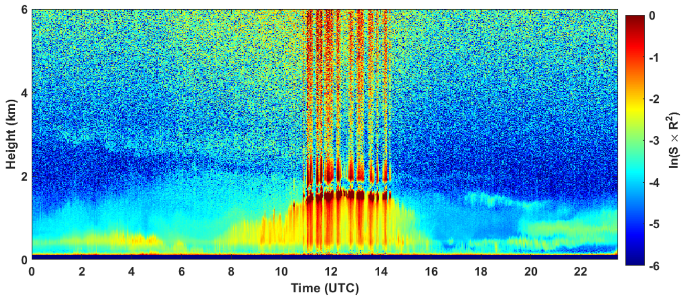
2022-10-20 RCS quick look CHM15k - ILVA LIDAR2 PARCHI
