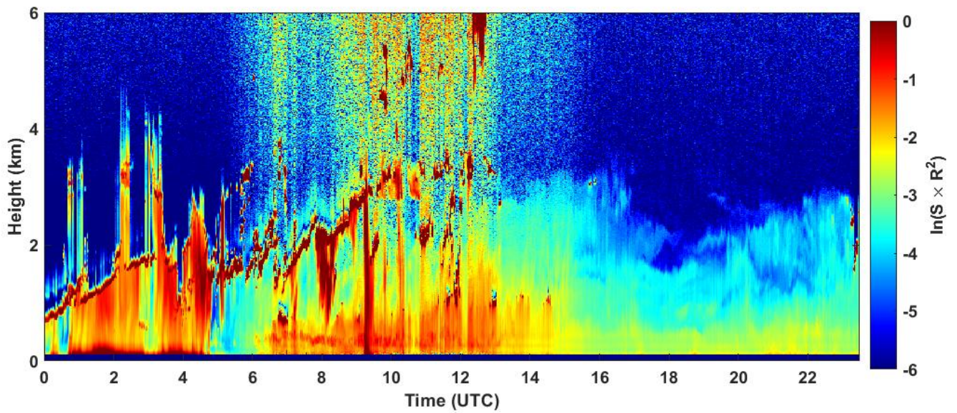
2022-10-14 RCS quick look CHM15k - ILVA LIDAR3 AGGLOMERATO
