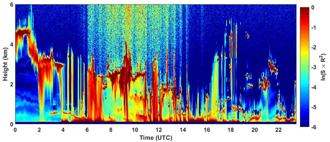
2022-10-10 RCS quick look CHM15k - ILVA LIDAR3 AGGLOMERATO
