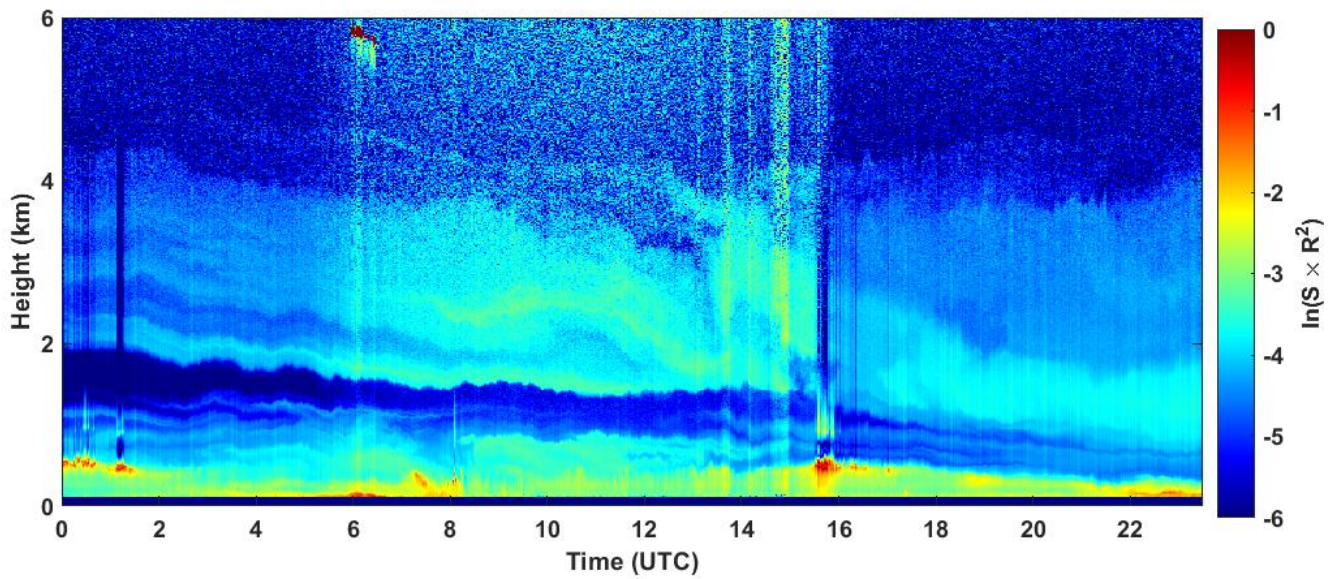
2022-10-22 RCS quick look CHM15k - ILVA LIDAR3 AGGLOMERATO
