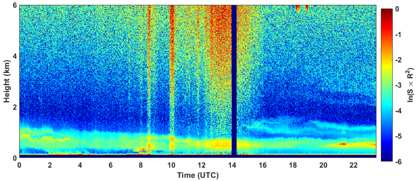
2022-10-22 RCS quick look CHM15k - ILVA LIDAR2 PARCHI
