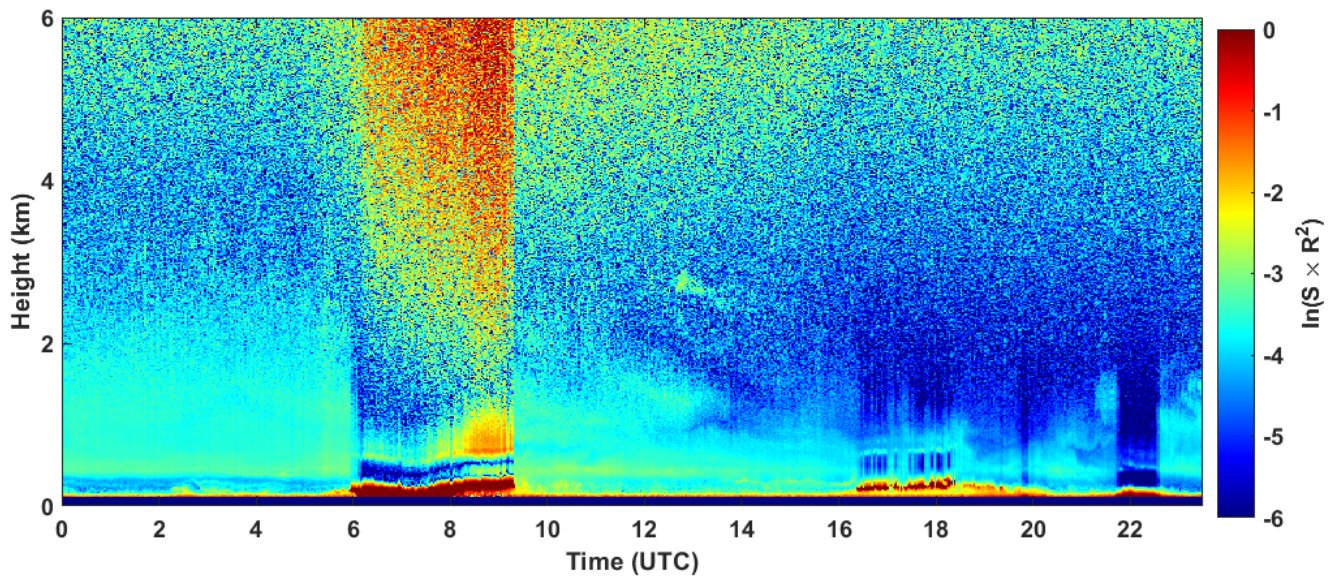
2022-10-24 RCS quick look CHM15k - ILVA LIDAR2 PARCHI
