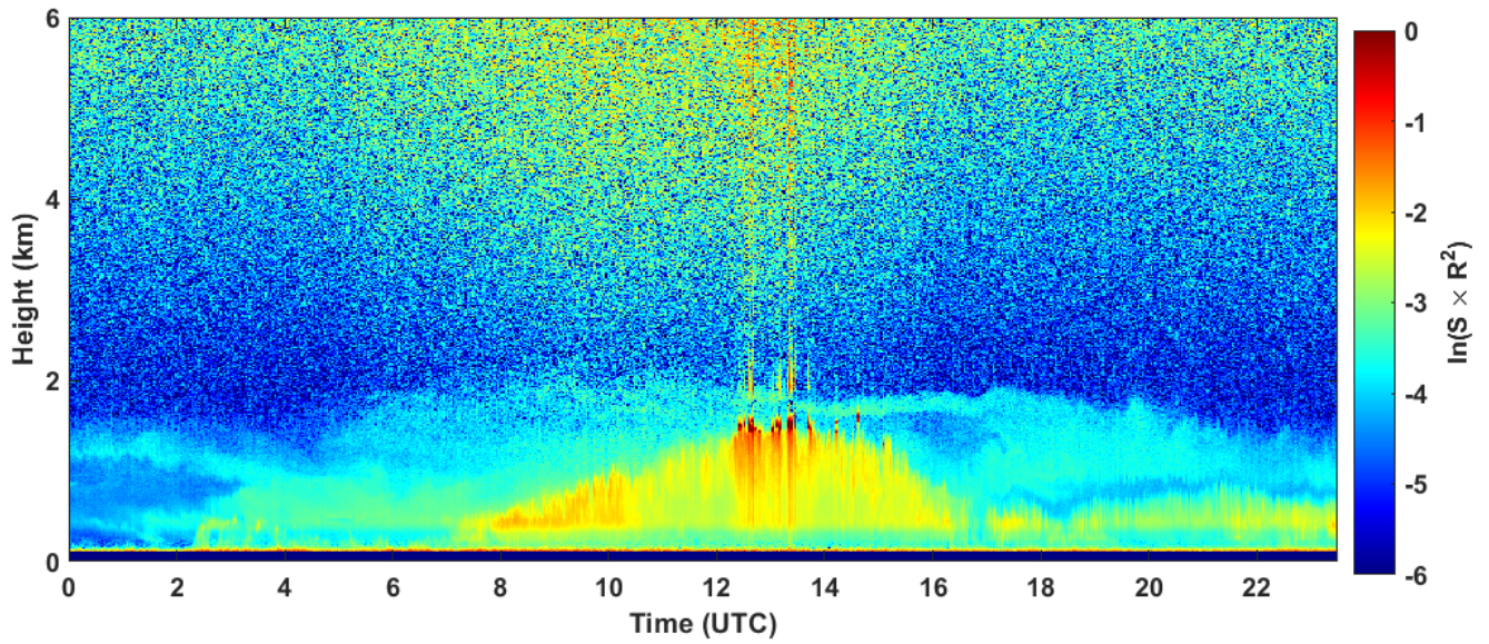
2022-10-18 RCS quick look CHM15k - ILVA LIDAR2 PARCHI
