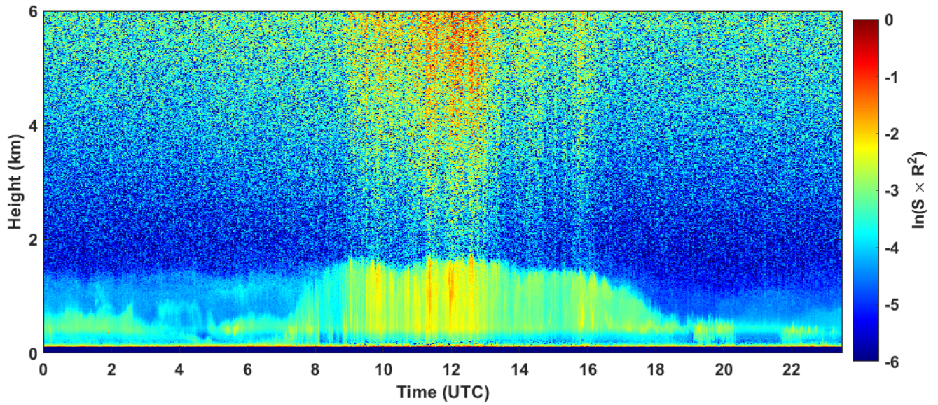
2022-10-06 RCS quick look CHM15k - ILVA LIDAR2 PARCHI
