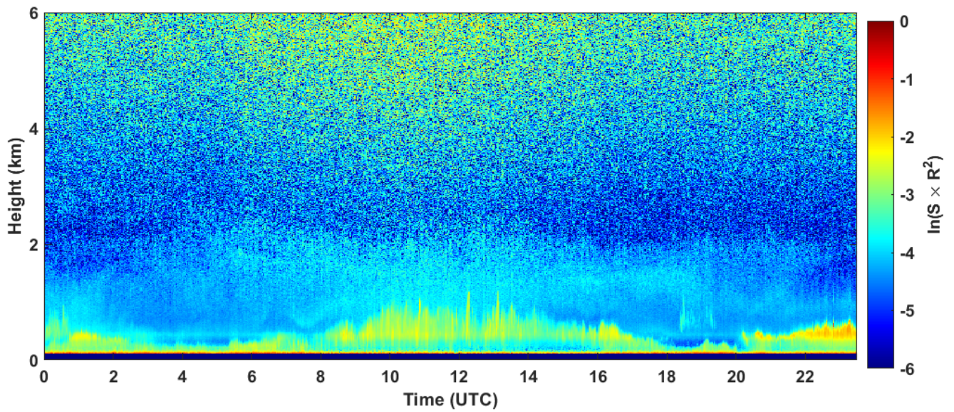
2022-10-28 RCS quick look CHM15k - ILVA LIDAR2 PARCHI
