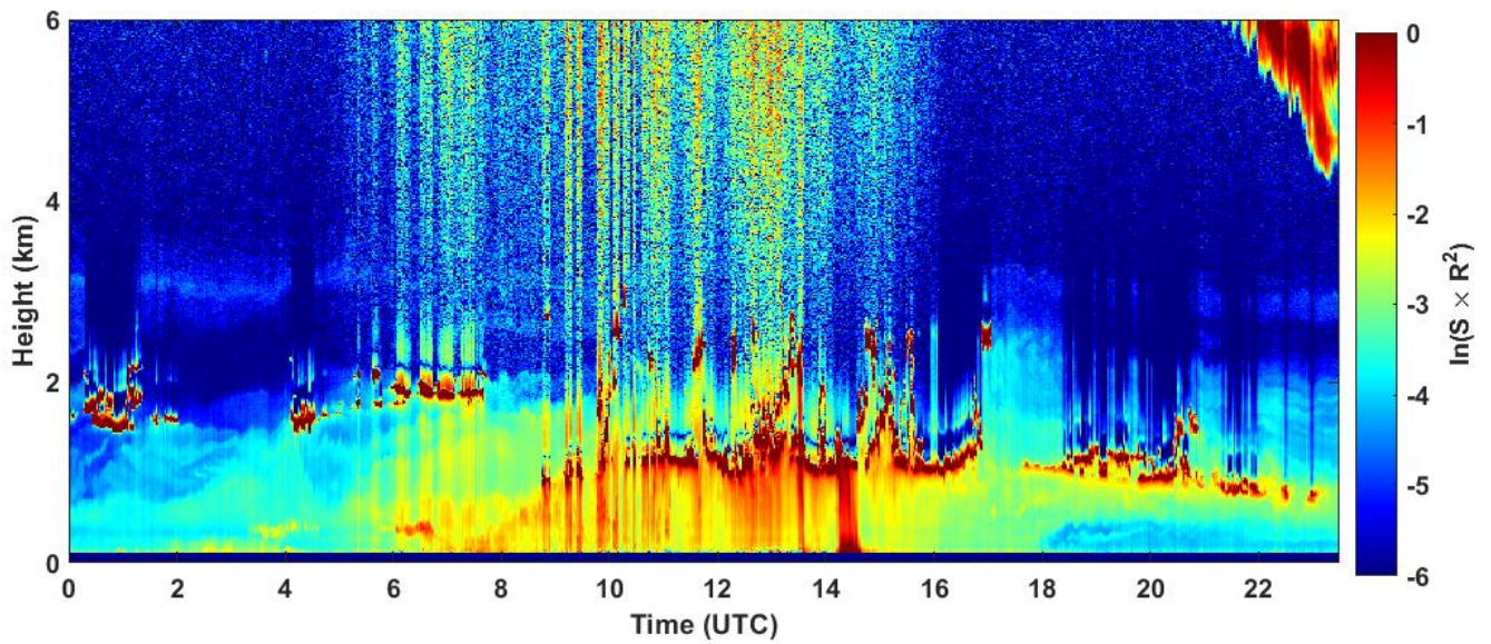
2022-10-12 RCS quick look CHM15k - ILVA LIDAR3 AGGLOMERATO
