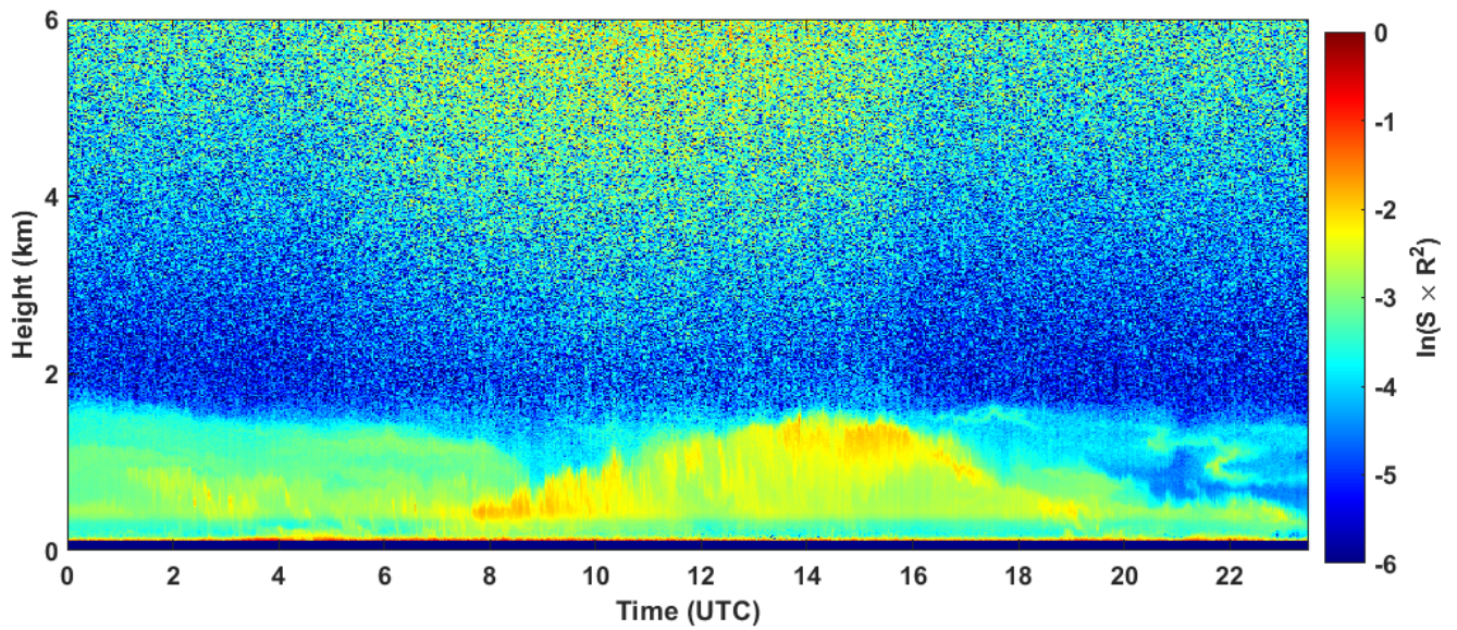
2022-10-16 RCS quick look CHM15k - ILVA LIDAR2 PARCHI
