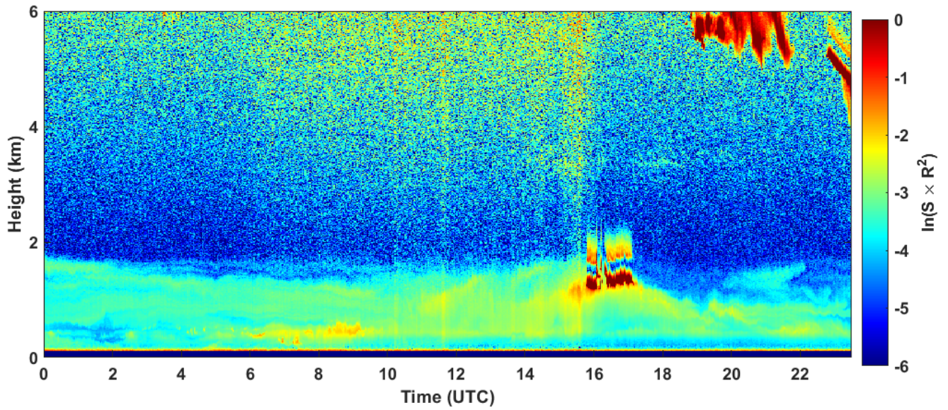
2022-10-10 RCS quick look CHM15k - ILVA LIDAR2 PARCHI
