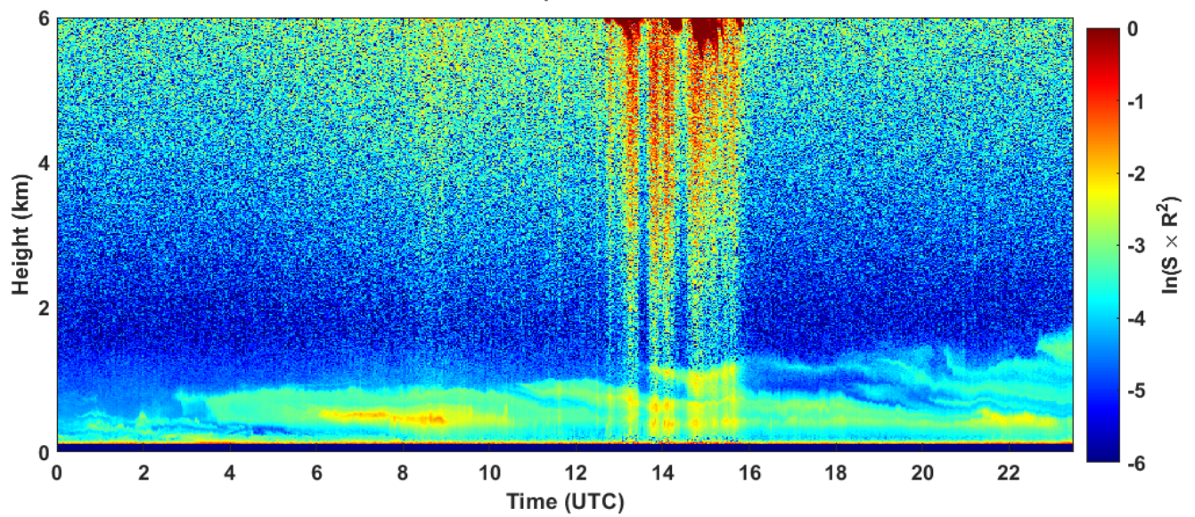
2022-10-08 RCS quick look CHM15k - ILVA LIDAR2 PARCHI
