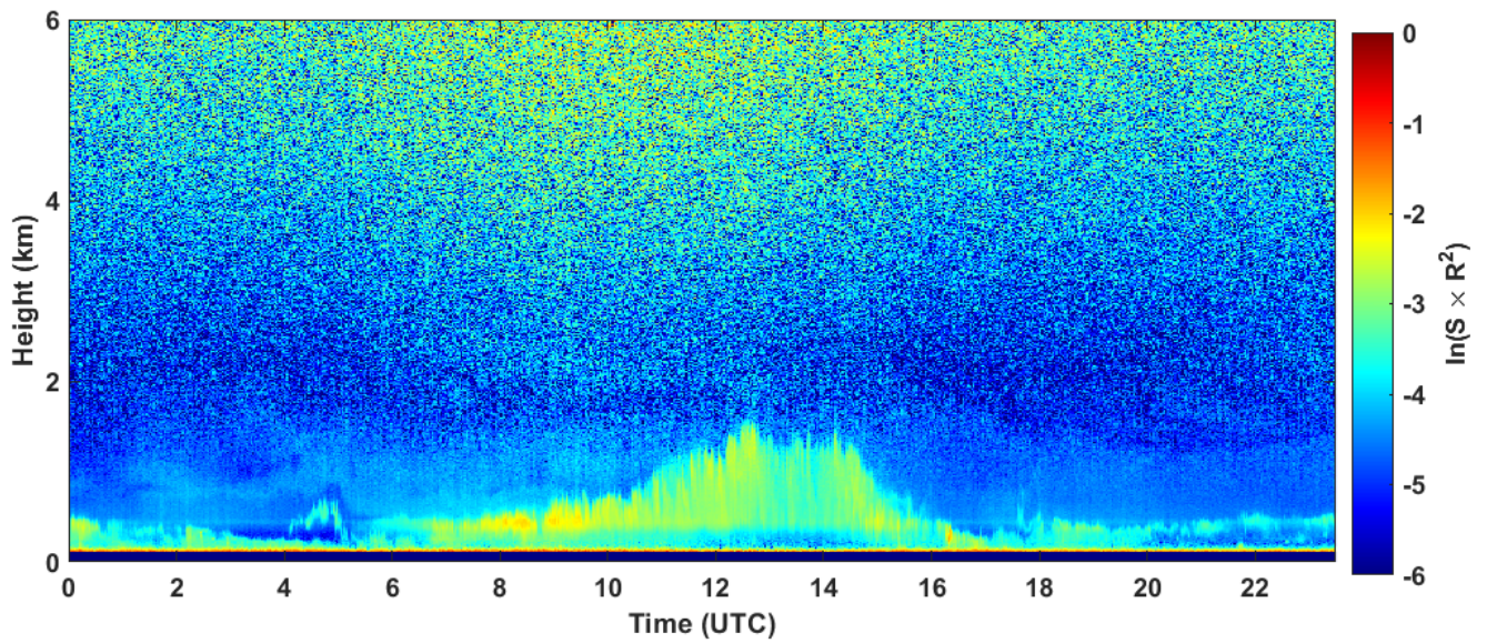
2022-10-30 RCS quick look CHM15k - ILVA LIDAR2 PARCHI
