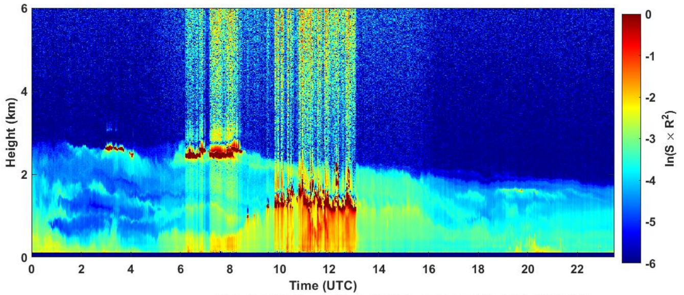
2022-10-16 RCS quick look CHM15k - ILVA LIDAR3 AGGLOMERATO
