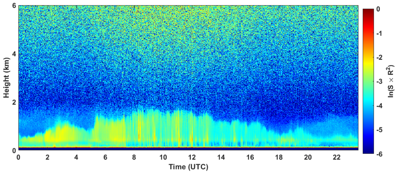
2022-10-04 RCS quick look CHM15k - ILVA LIDAR2 PARCHI
