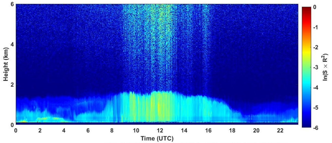
2022-10-06 RCS quick look CHM15k - ILVA LIDAR3 AGGLOMERATO
