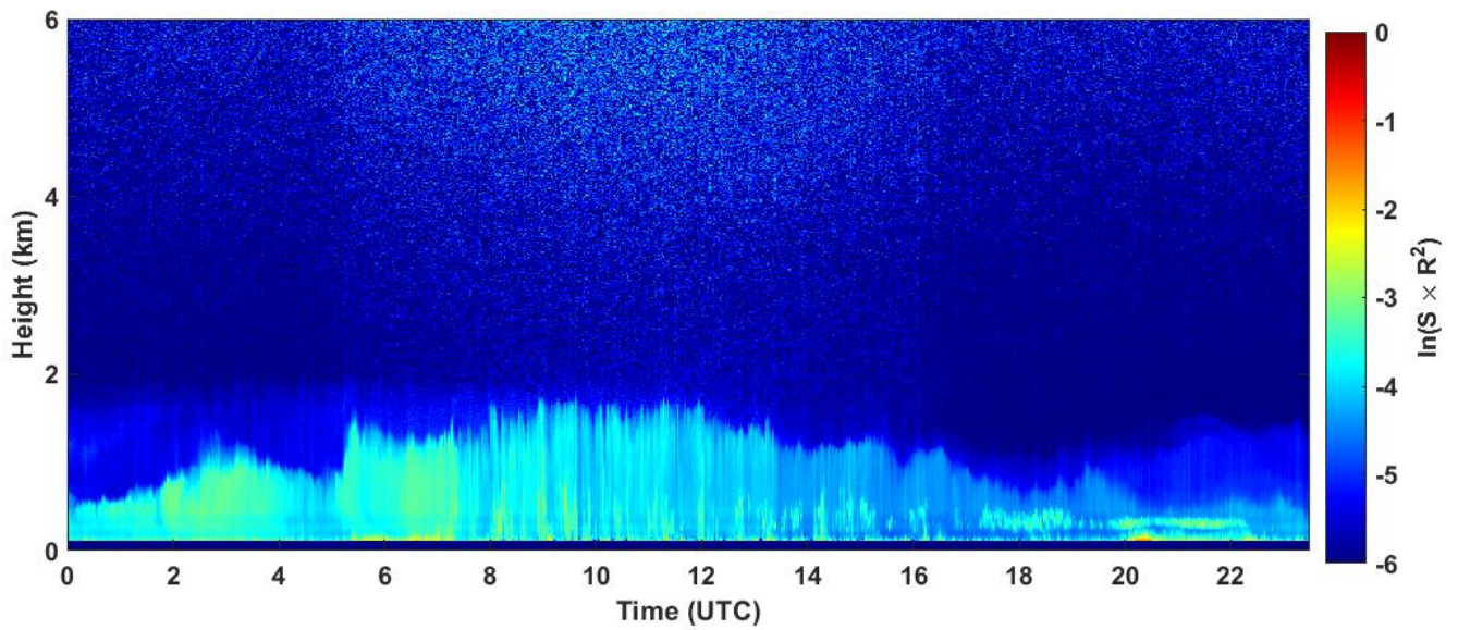
2022-10-04 RCS quick look CHM15k - ILVA LIDAR3 AGGLOMERATO
