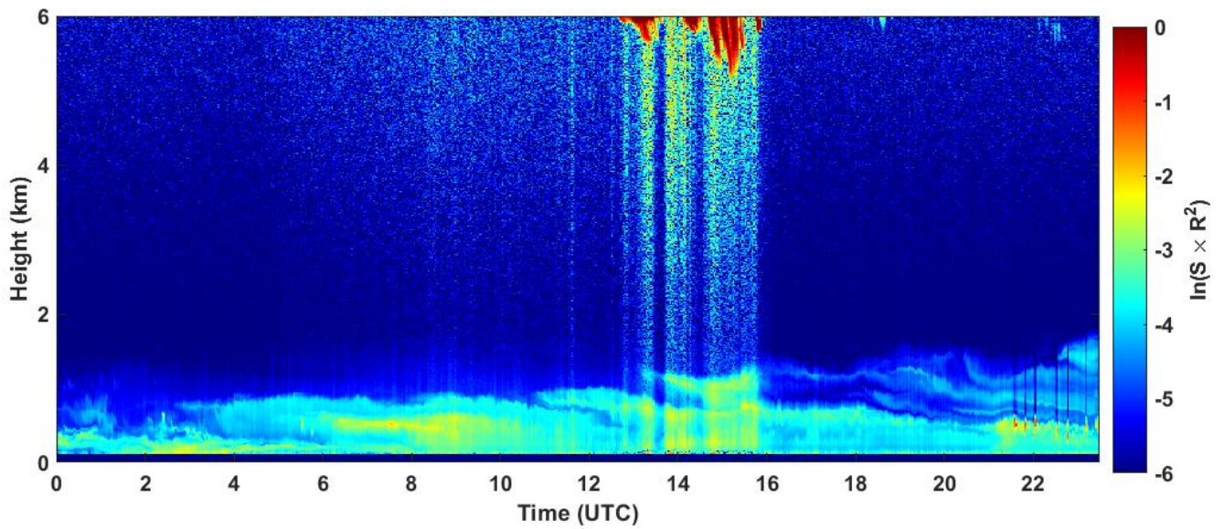
2022-10-08 RCS quick look CHM15k - ILVA LIDAR3 AGGLOMERATO
