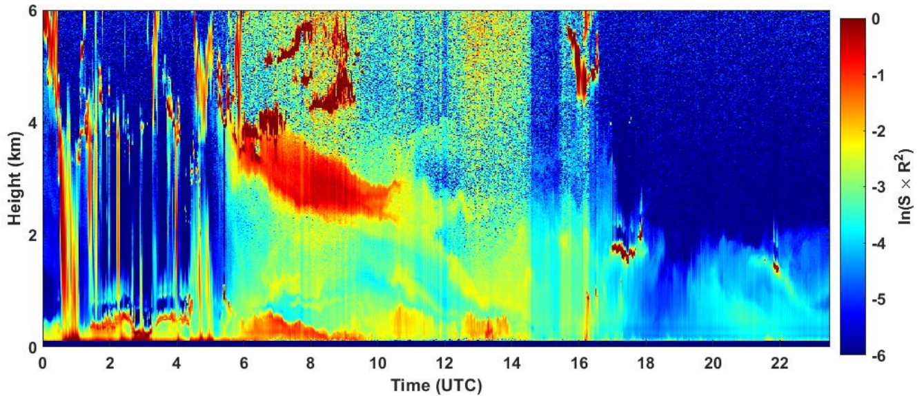
2022-10-02 RCS quick look CHM15k - ILVA LIDAR3 AGGLOMERATO
