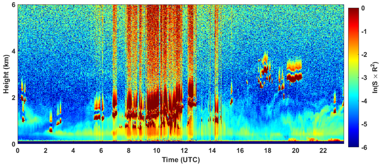
2022-10-12 RCS quick look CHM15k - ILVA LIDAR2 PARCHI
