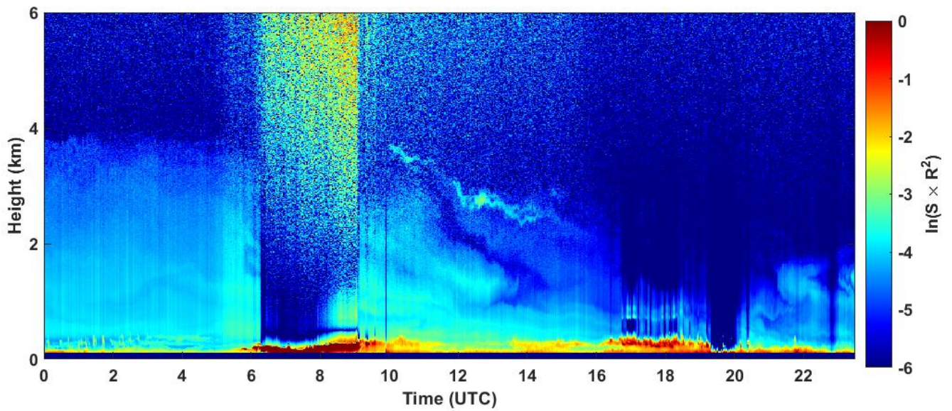
2022-10-24 RCS quick look CHM15k - ILVA LIDAR3 AGGLOMERATO
