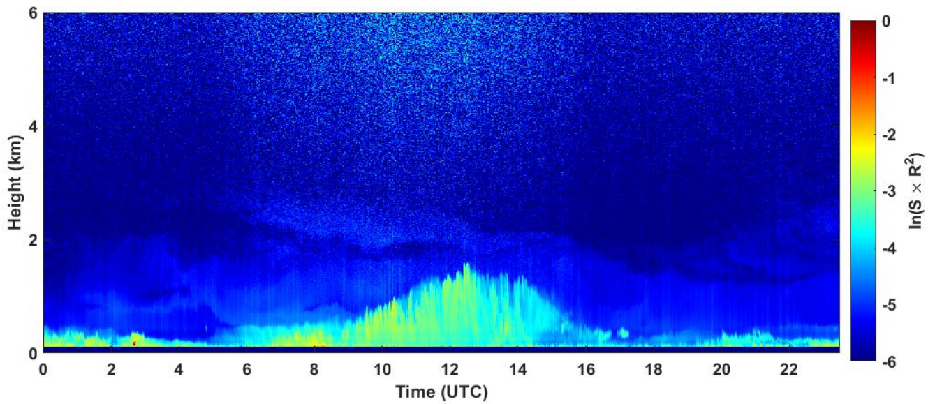
2022-10-30 RCS quick look CHM15k - ILVA LIDAR3 AGGLOMERATO
