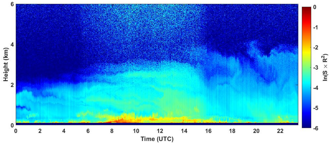
2022-10-26 RCS quick look CHM15k - ILVA LIDAR3 AGGLOMERATO
