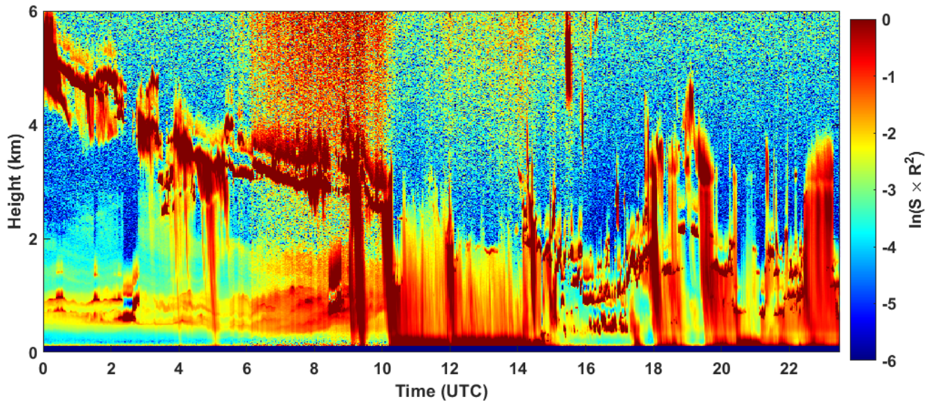
2022-10-14 RCS quick look CHM15k - ILVA LIDAR2 PARCHI
