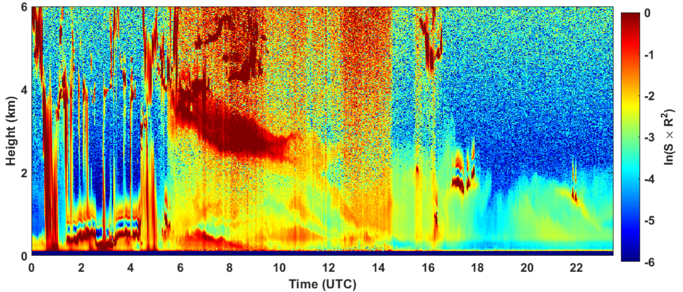
2022-10-02 RCS quick look CHM15k - ILVA LIDAR2 PARCHI
