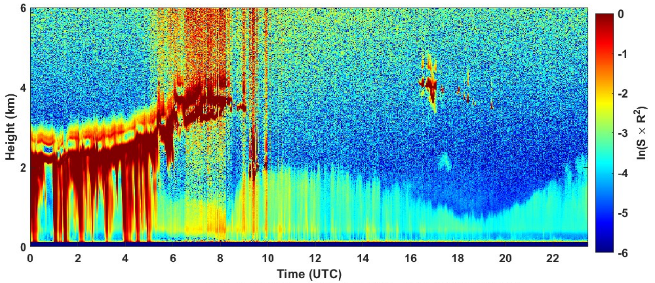
2022-09-22 RCS quick look CHM15k - ILVA LIDAR2 PARCHI
