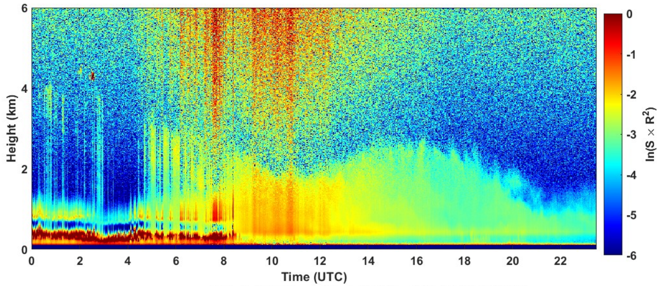
2022-09-10 RCS quick look CHM15k - ILVA LIDAR2 PARCHI
