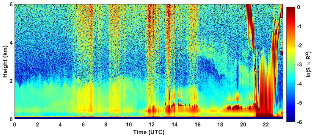
2022-09-30 RCS quick look CHM15k - ILVA LIDAR2 PARCHI
