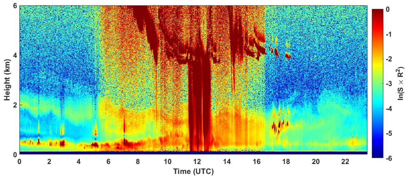
2022-09-04 RCS quick look CHM15k - ILVA LIDAR2 PARCHI
