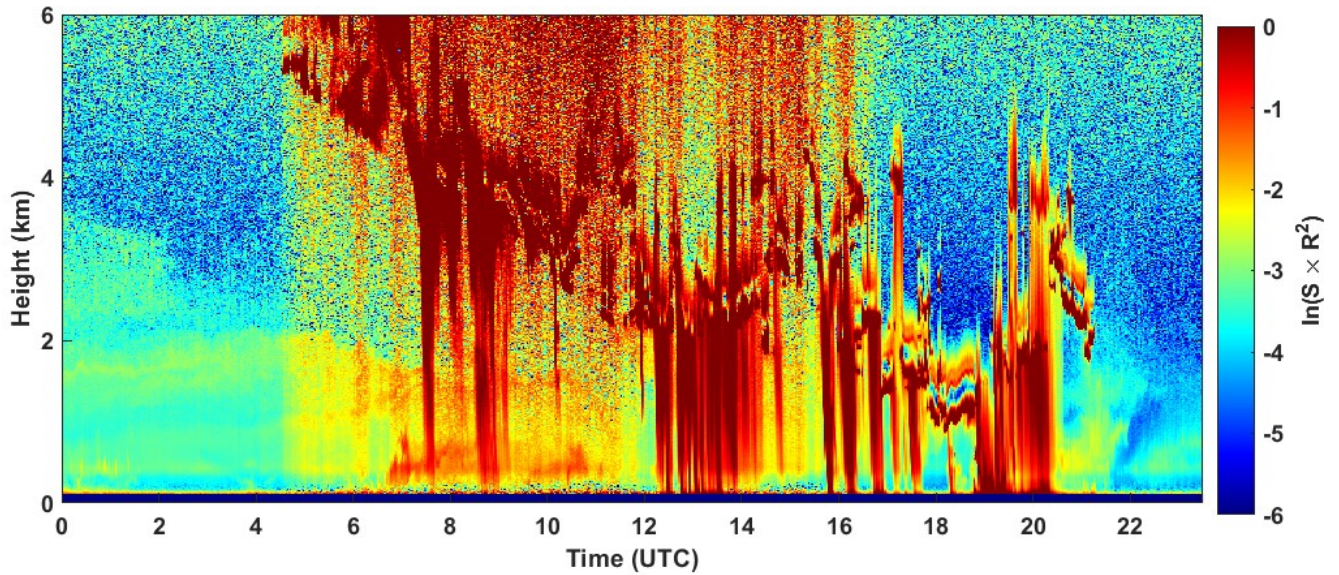
2022-09-02 RCS quick look CHM15k - ILVA LIDAR2 PARCHI
