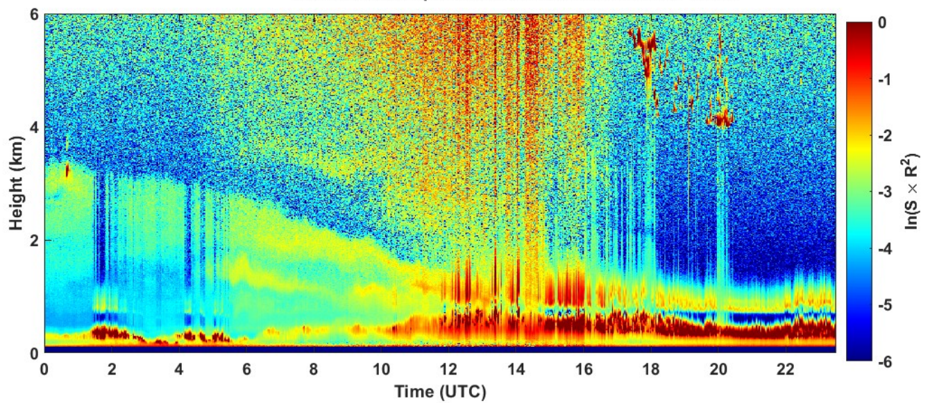
2022-09-08 RCS quick look CHM15k - ILVA LIDAR2 PARCHI
