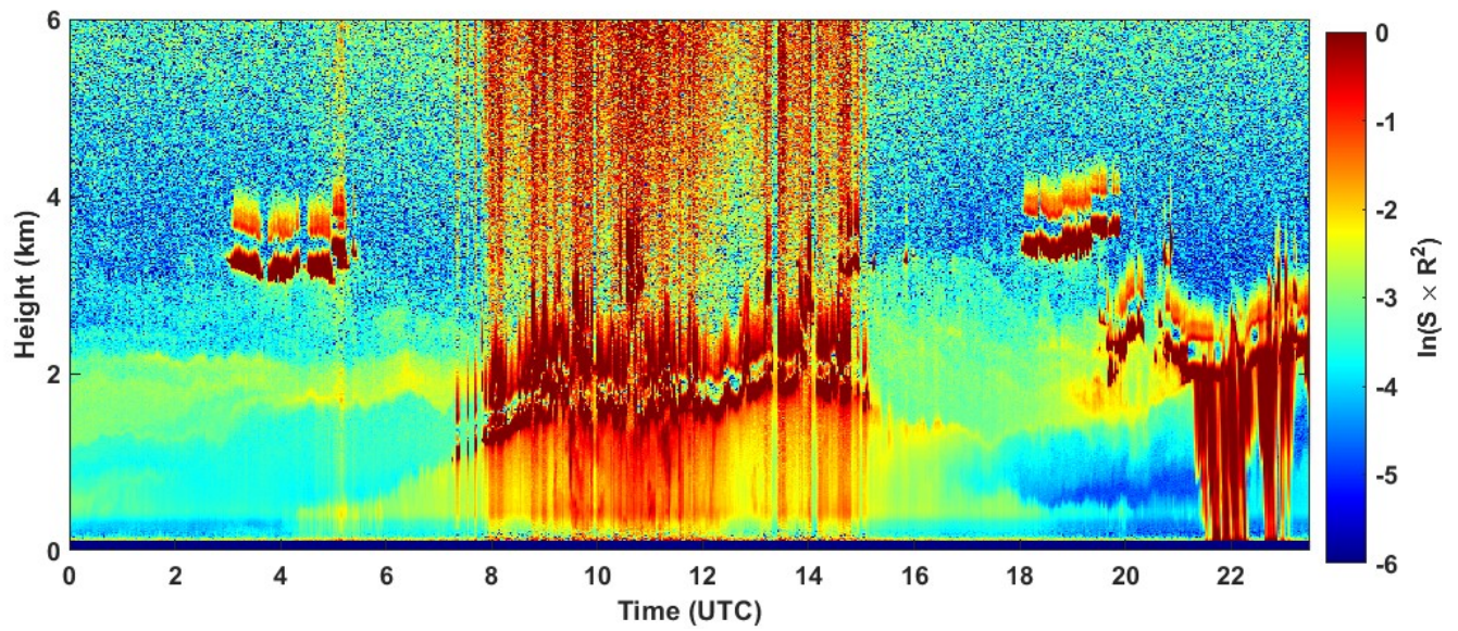
2022-09-20 RCS quick look CHM15k - ILVA LIDAR2 PARCHI
