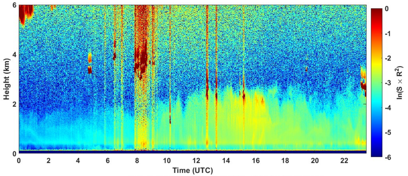
2022-09-28 RCS quick look CHM15k - ILVA LIDAR2 PARCHI
