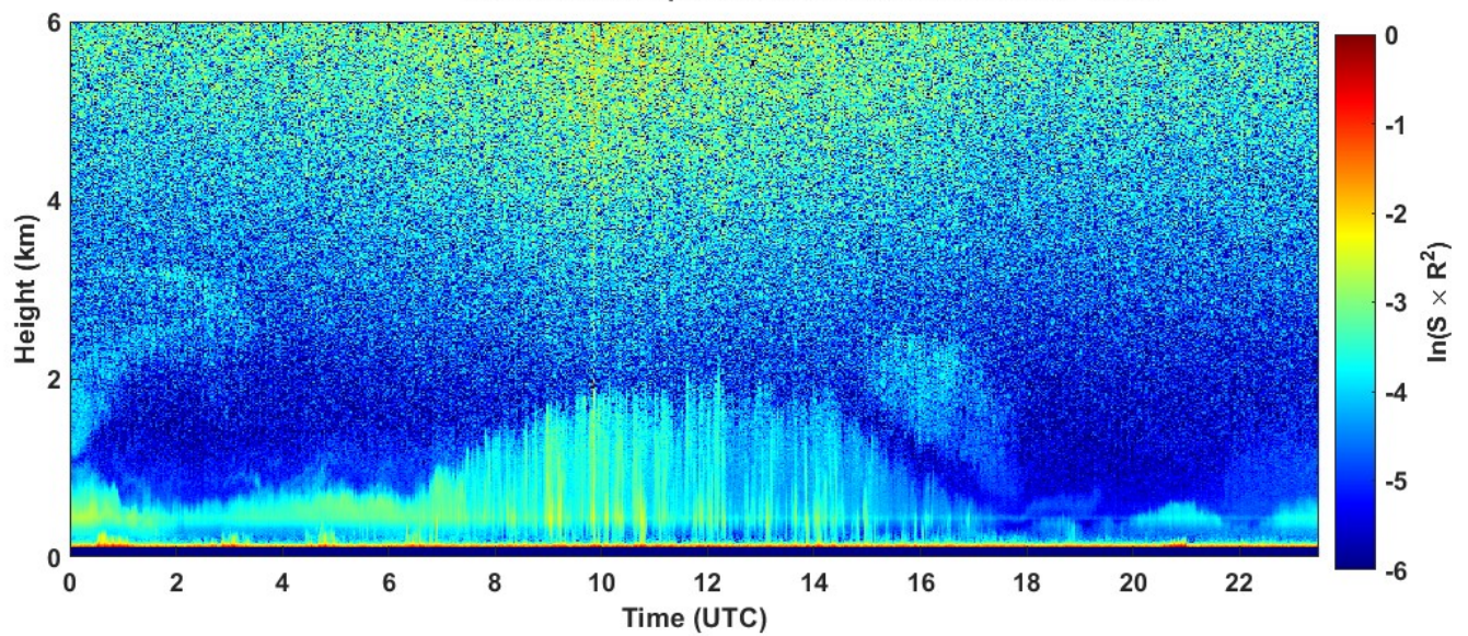
2022-09-12 RCS quick look CHM15k - ILVA LIDAR2 PARCHI
