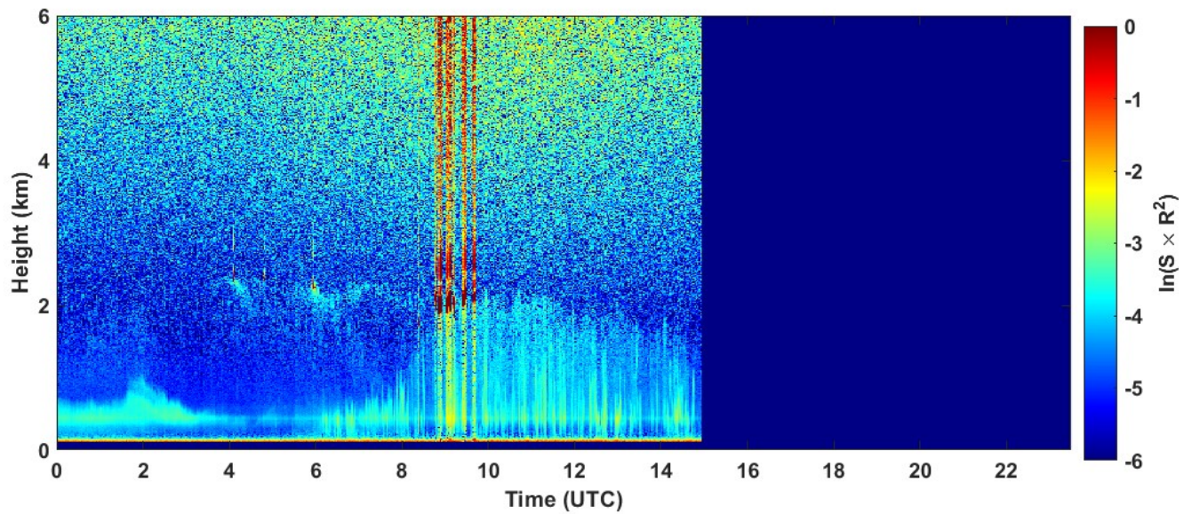
2022-09-14 RCS quick look CHM15k - ILVA LIDAR2 PARCHI
