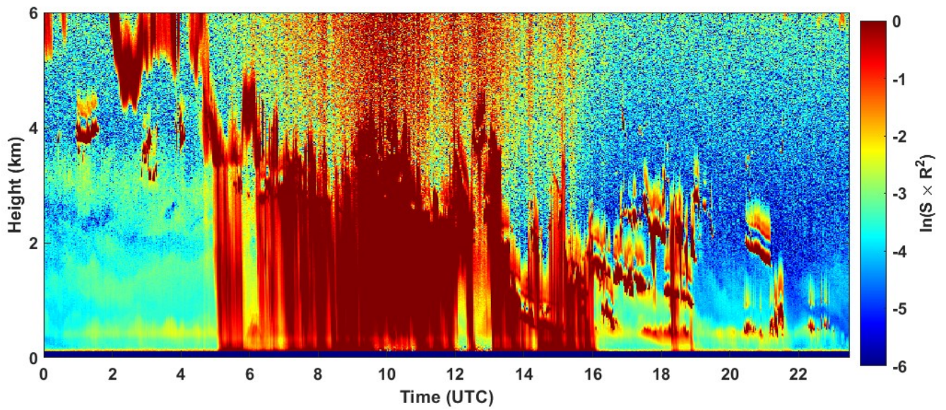
2022-09-26 RCS quick look CHM15k - ILVA LIDAR2 PARCHI
