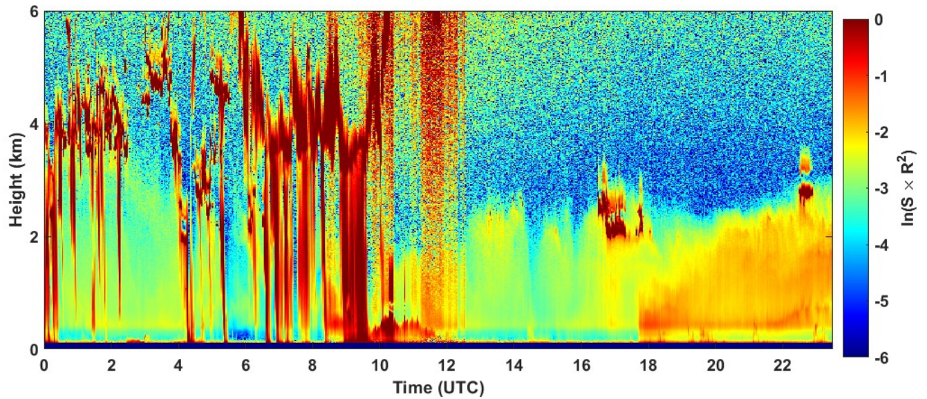
2022-09-18 RCS quick look CHM15k - ILVA LIDAR2 PARCHI
