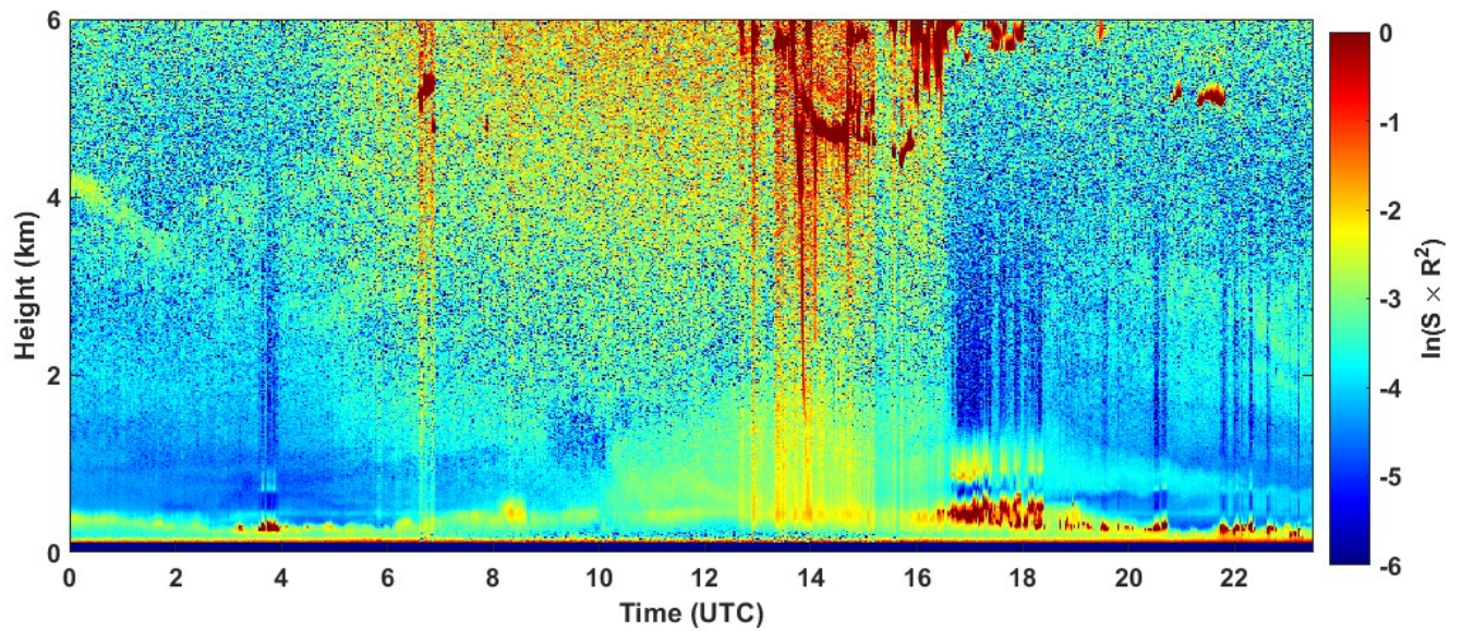
2022-09-16 RCS quick look CHM15k - ILVA LIDAR2 PARCHI
