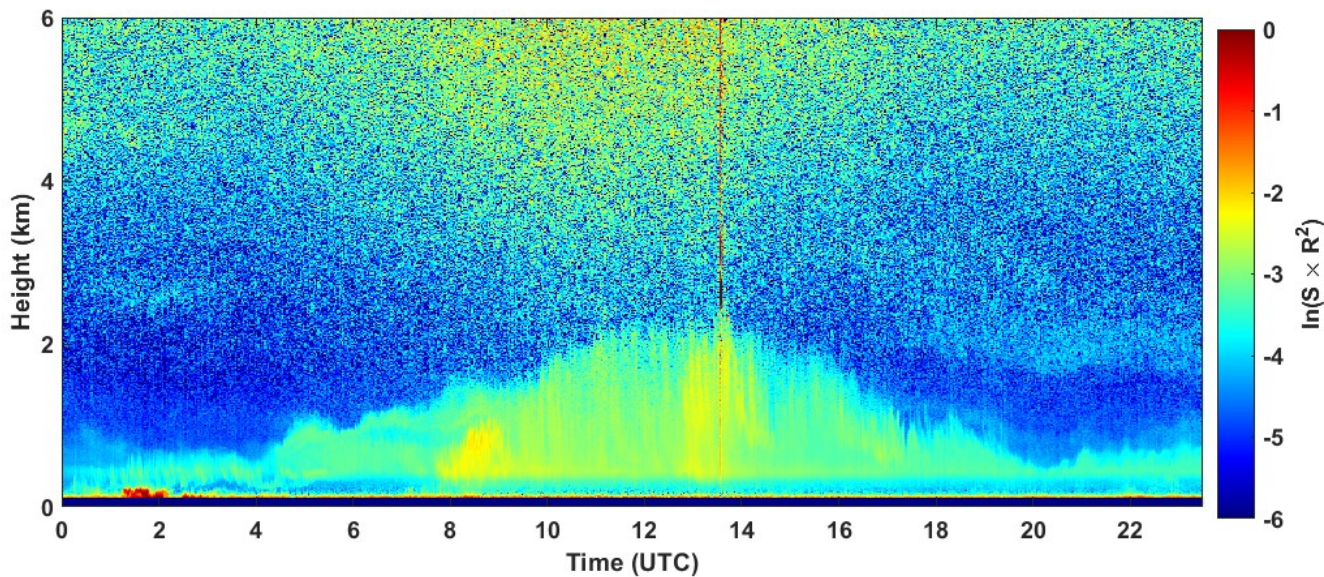
2022-09-06 RCS quick look CHM15k - ILVA LIDAR2 PARCHI
