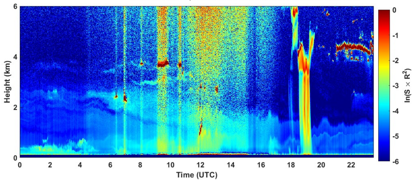
2022-08-28 RCS quick look CHM15k - ILVA LIDAR3 AGGLOMERATO
