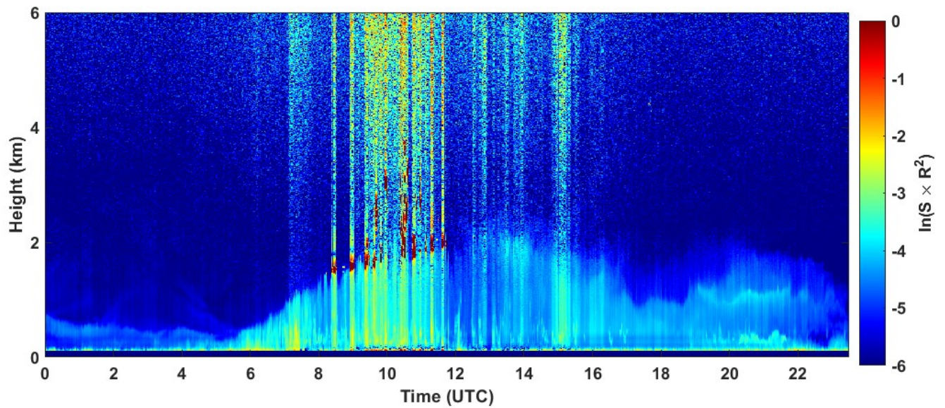
2022-08-22 RCS quick look CHM15k - ILVA LIDAR3 AGGLOMERATO
