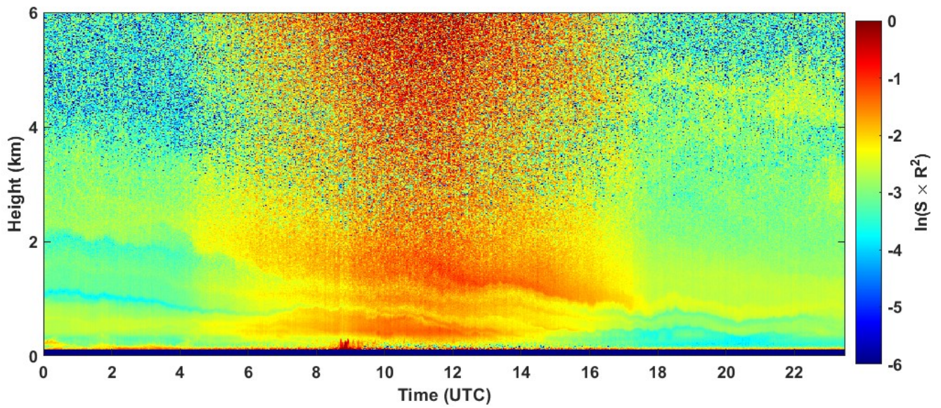
2022-08-18 RCS quick look CHM15k - ILVA LIDAR2 PARCHI
