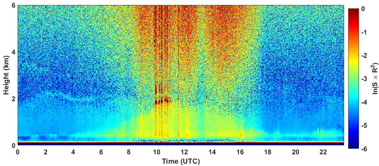
2022-08-10 RCS quick look CHM15k - ILVA LIDAR2 PARCHI
