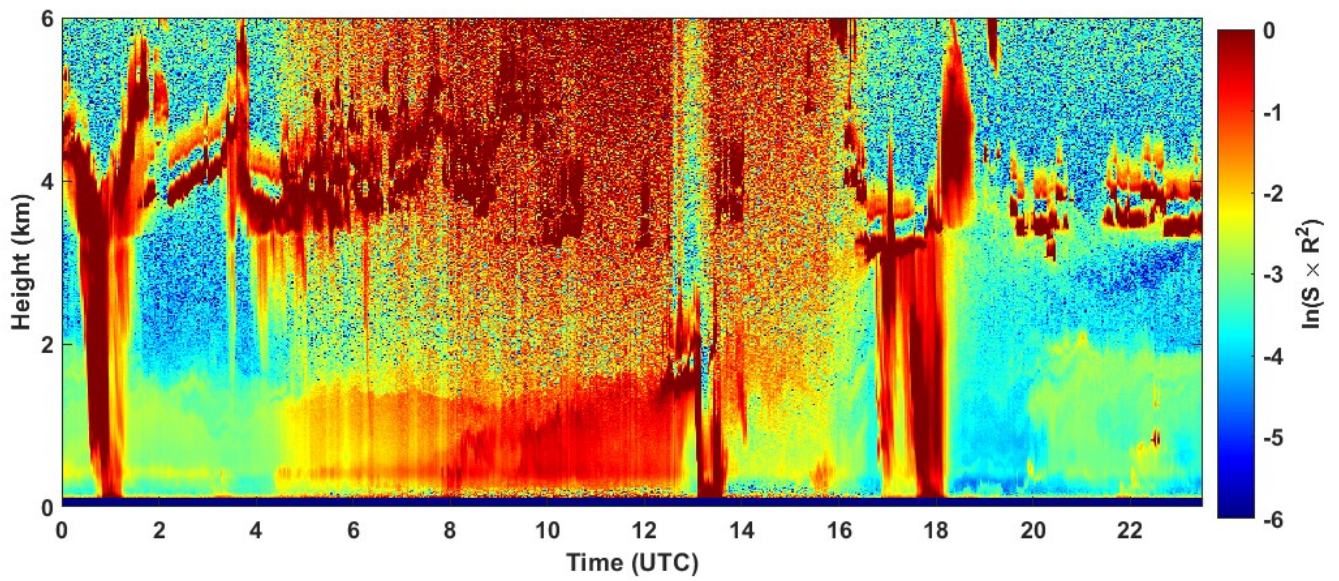
2022-08-12 RCS quick look CHM15k - ILVA LIDAR2 PARCHI
