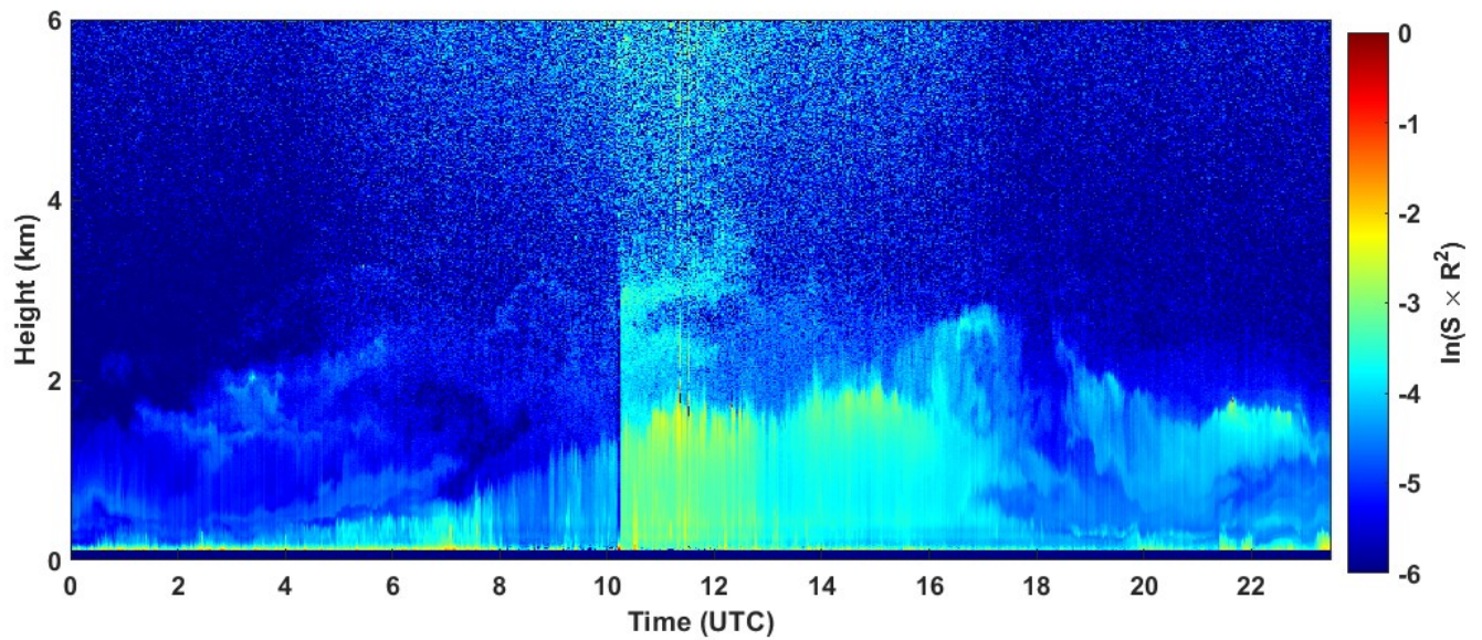
2022-08-30 RCS quick look CHM15k - ILVA LIDAR3 AGGLOMERATO
