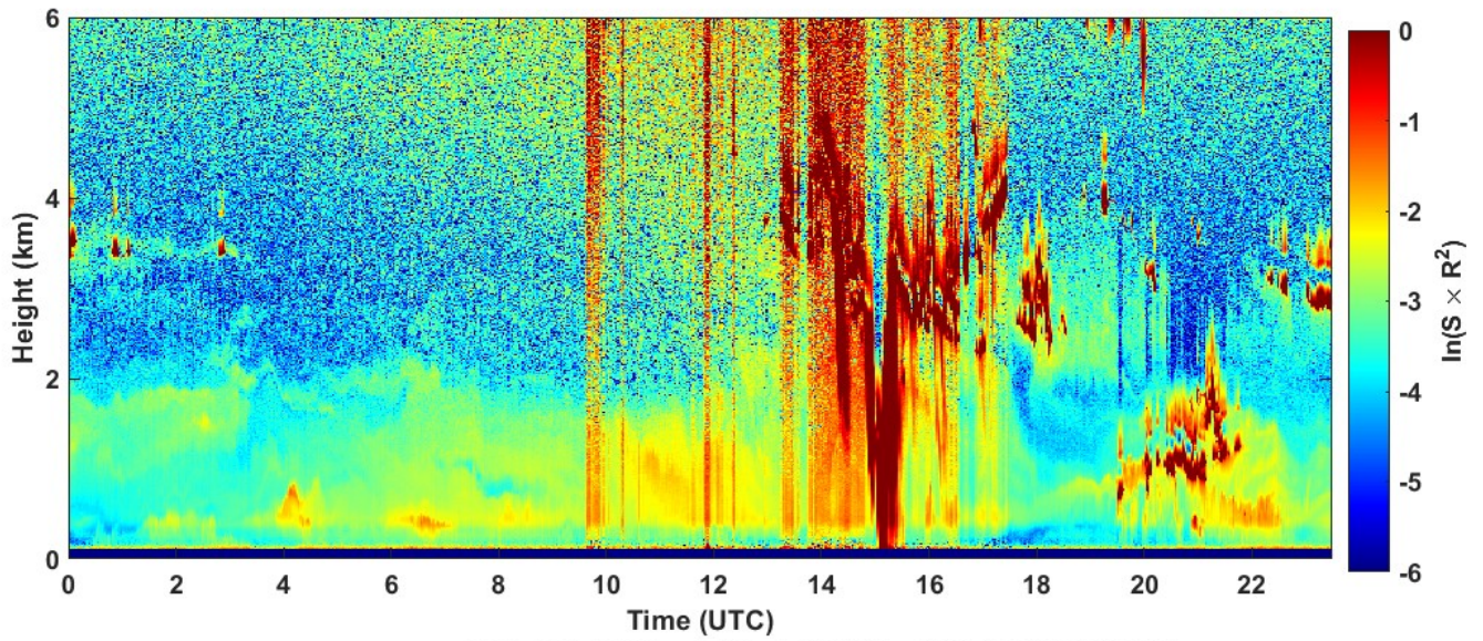
2022-08-14 RCS quick look CHM15k - ILVA LIDAR2 PARCHI
