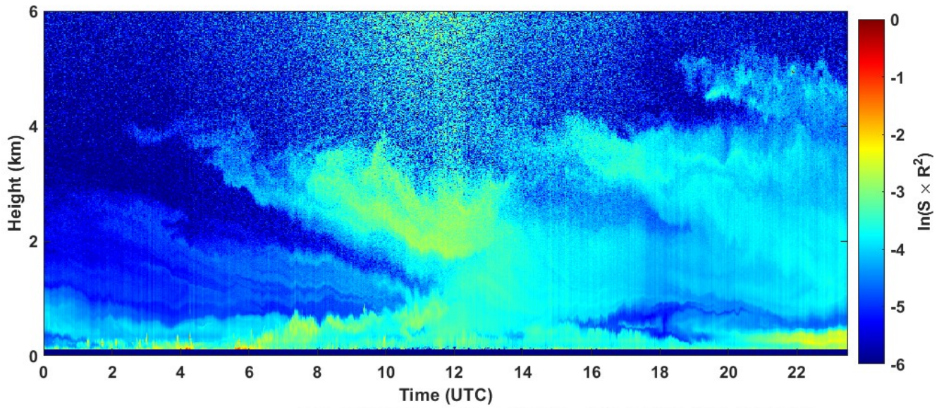
2022-08-16 RCS quick look CHM15k - ILVA LIDAR3 AGGLOMERATO
