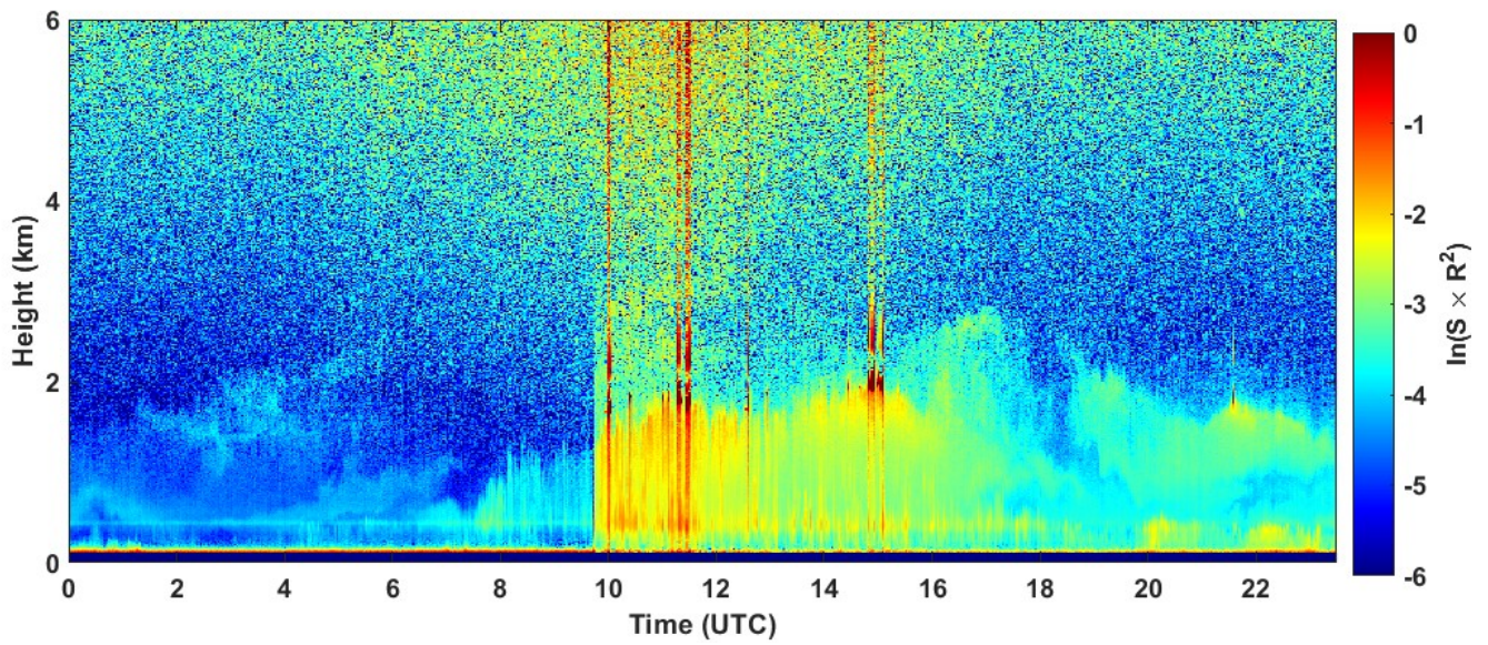
2022-08-30 RCS quick look CHM15k - ILVA LIDAR2 PARCHI
