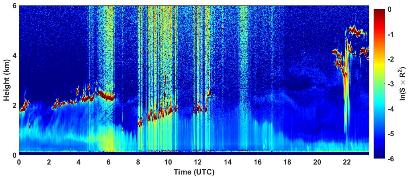
2022-08-24 RCS quick look CHM15k - ILVA LIDAR3 AGGLOMERATO
