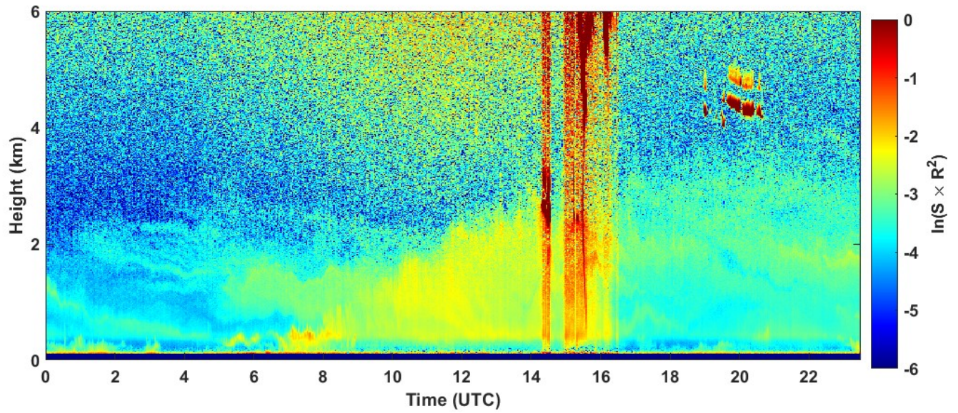
2022-08-31 RCS quick look CHM15k - ILVA LIDAR2 PARCHI
