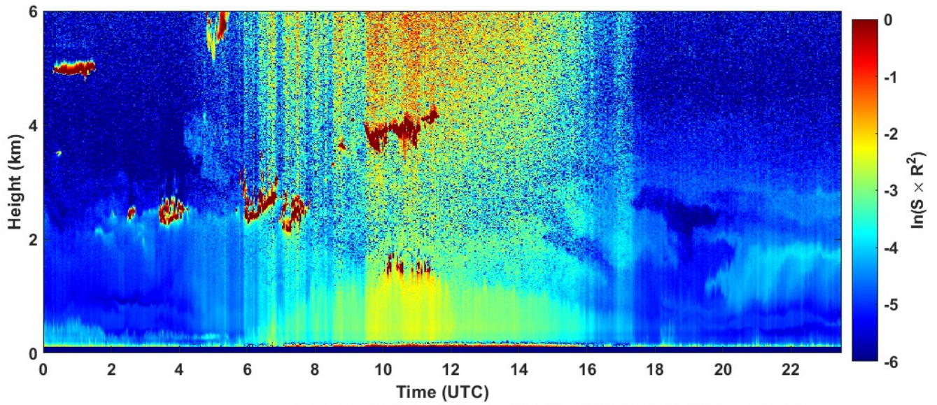
2022-08-26 RCS quick look CHM15k - ILVA LIDAR3 AGGLOMERATO
