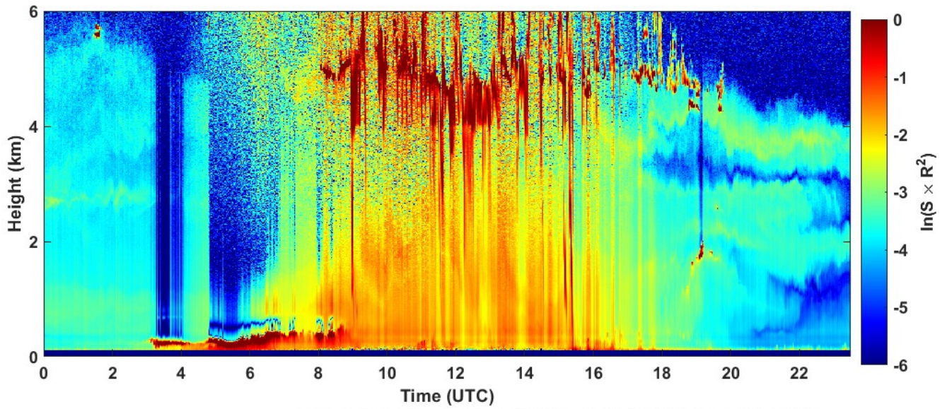
2022-08-20 RCS quick look CHM15k - ILVA LIDAR3 AGGLOMERATO
