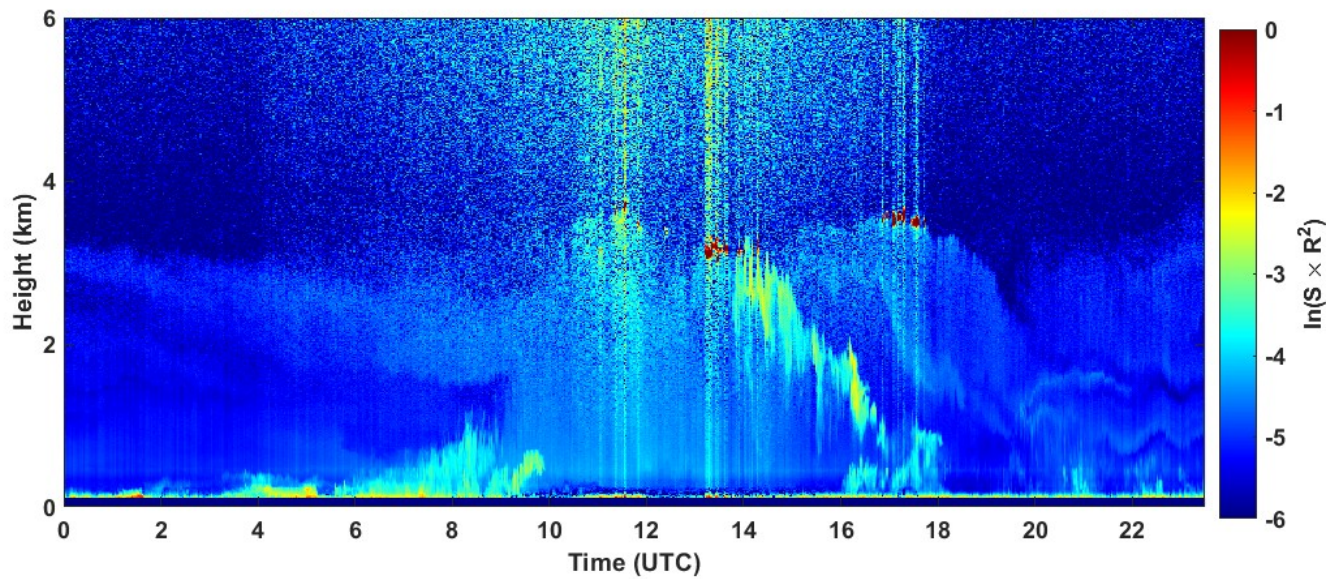
2022-08-06 RCS quick look CHM15k - ILVA LIDAR3 AGGLOMERATO
