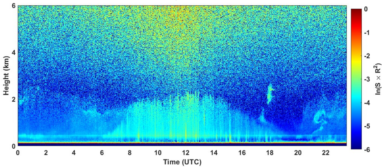
2022-08-02 RCS quick look CHM15k - ILVA LIDAR2 PARCHI
