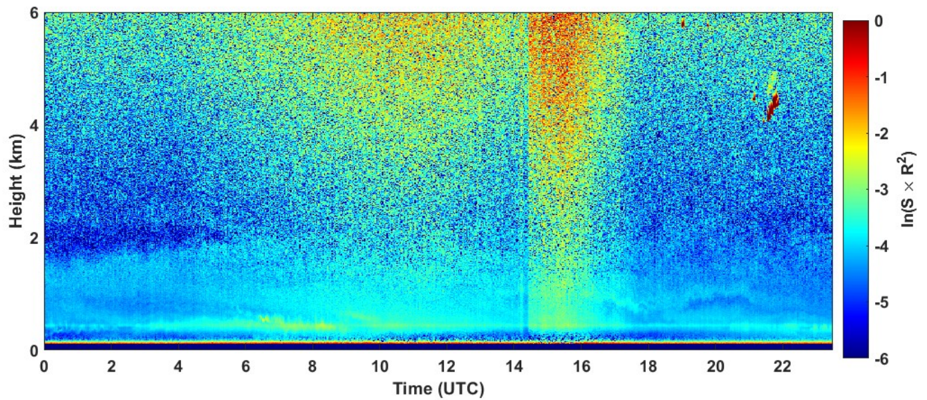
2022-08-28 RCS quick look CHM15k - ILVA LIDAR2 PARCHI
