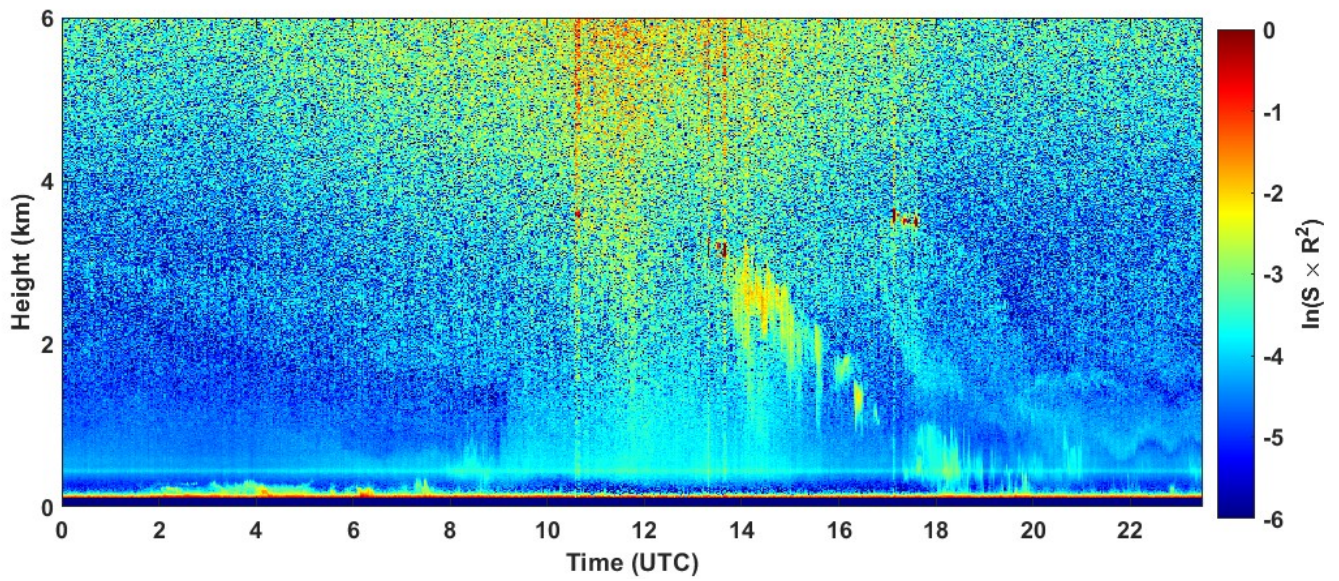
2022-08-06 RCS quick look CHM15k - ILVA LIDAR2 PARCHI
