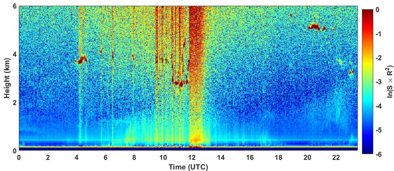
2022-08-08 RCS quick look CHM15k - ILVA LIDAR2 PARCHI
