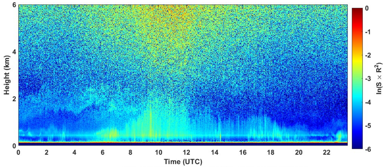
2022-08-04 RCS quick look CHM15k - ILVA LIDAR2 PARCHI
