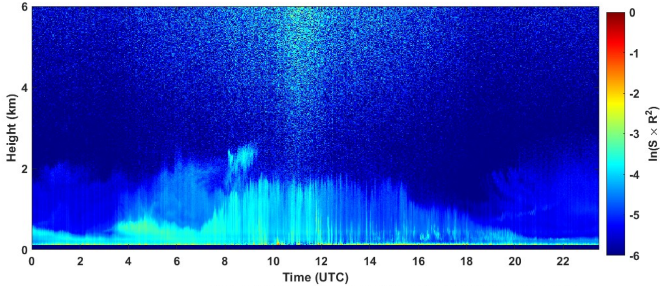
2022-08-02 RCS quick look CHM15k - ILVA LIDAR3 AGGLOMERATO
