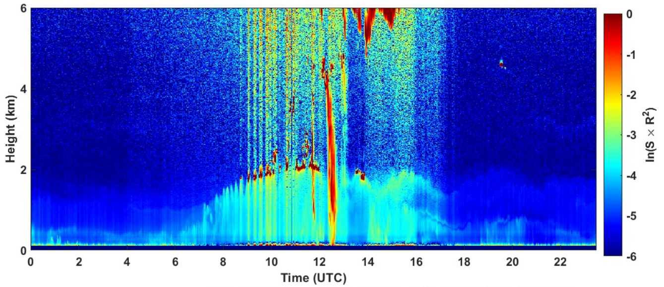
2022-08-10 RCS quick look CHM15k - ILVA LIDAR3 AGGLOMERATO
