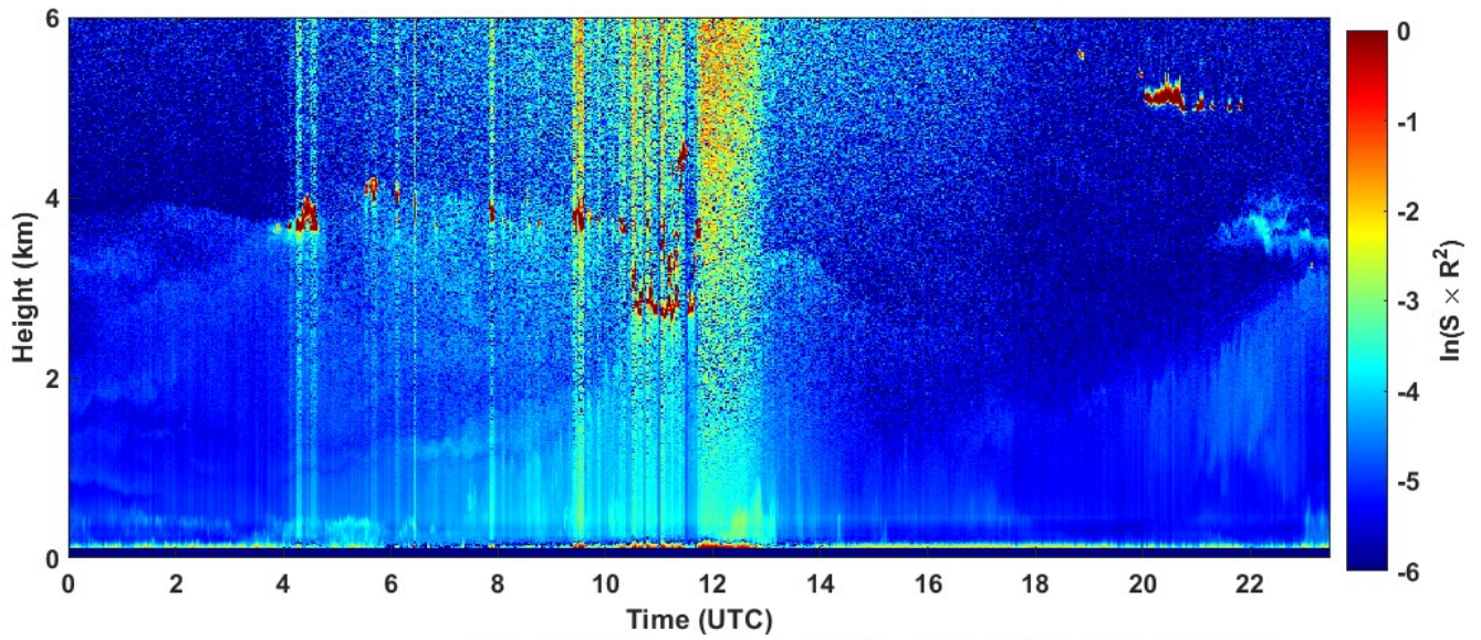
2022-08-08 RCS quick look CHM15k - ILVA LIDAR3 AGGLOMERATO
