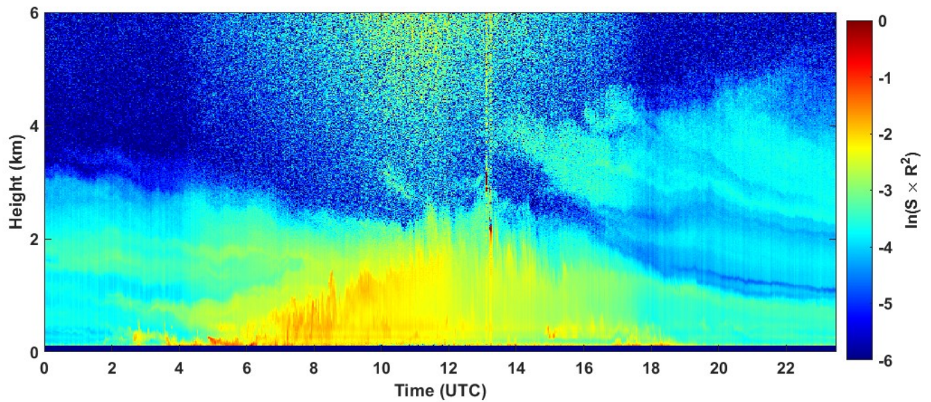
2022-08-18 RCS quick look CHM15k - ILVA LIDAR3 AGGLOMERATO
