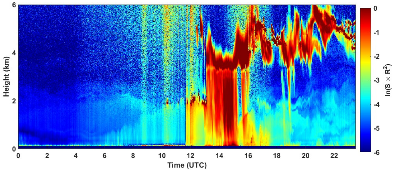
2022-08-12 RCS quick look CHM15k - ILVA LIDAR3 AGGLOMERATO
