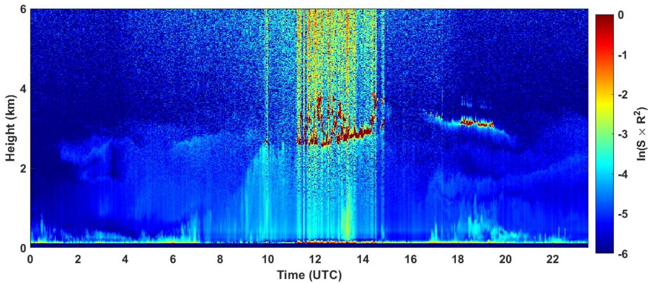
2022-08-04 RCS quick look CHM15k - ILVA LIDAR3 AGGLOMERATO
