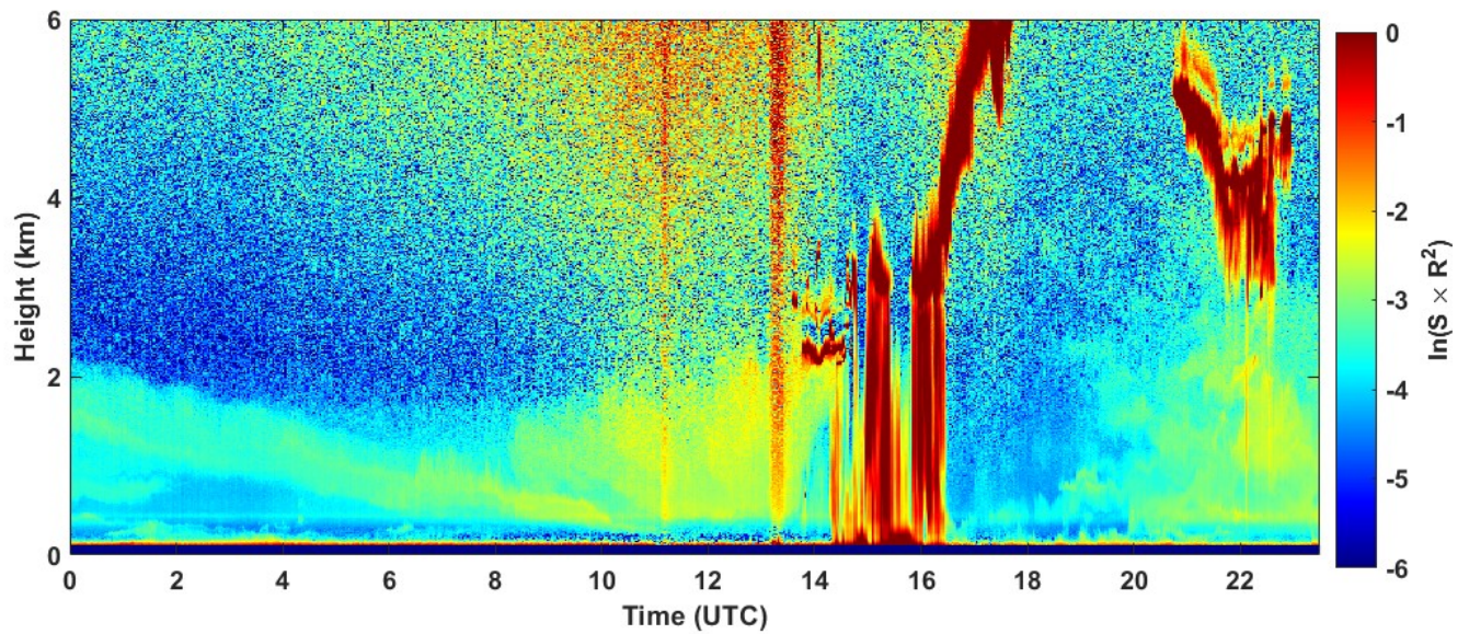
2022-05-18 RCS quick look CHM15k - ILVA LIDAR2 PARCHI
