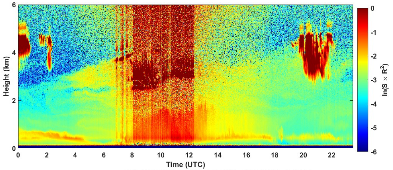
2022-05-10 RCS quick look CHM15k - ILVA LIDAR2 PARCHI
