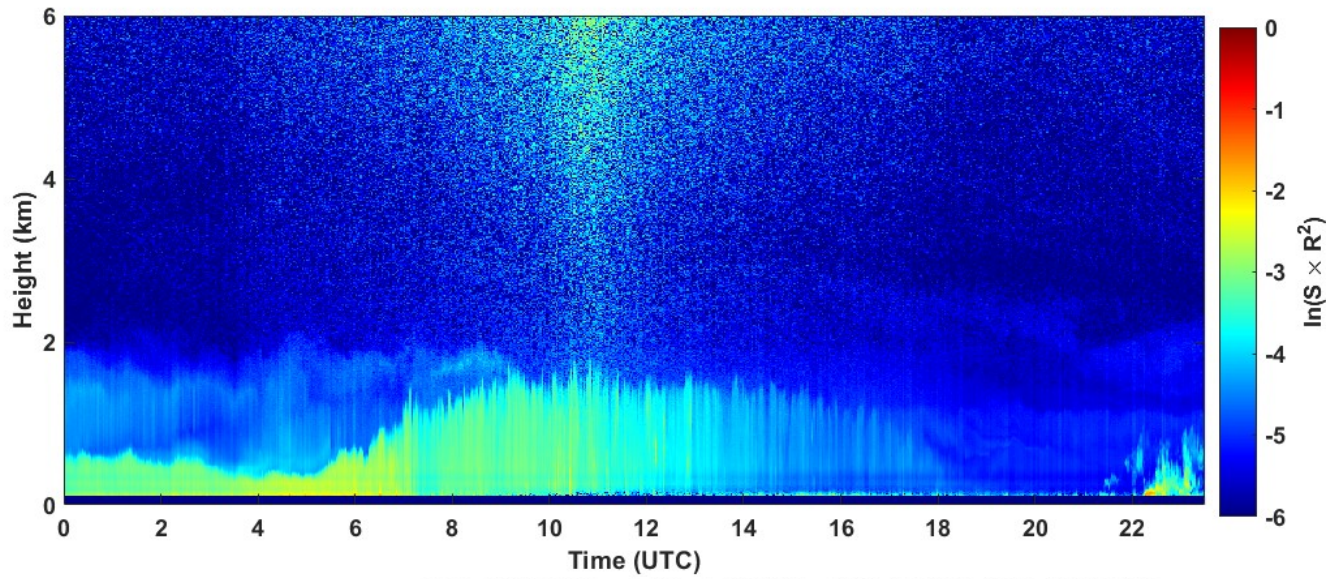
2022-05-20 RCS quick look CHM15k - ILVA LIDAR3 AGGLOMERATO
