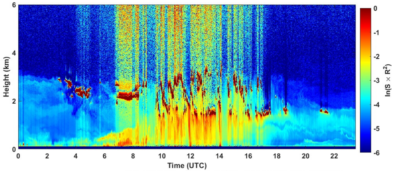
2022-05-04 RCS quick look CHM15k - ILVA LIDAR3 AGGLOMERATO
