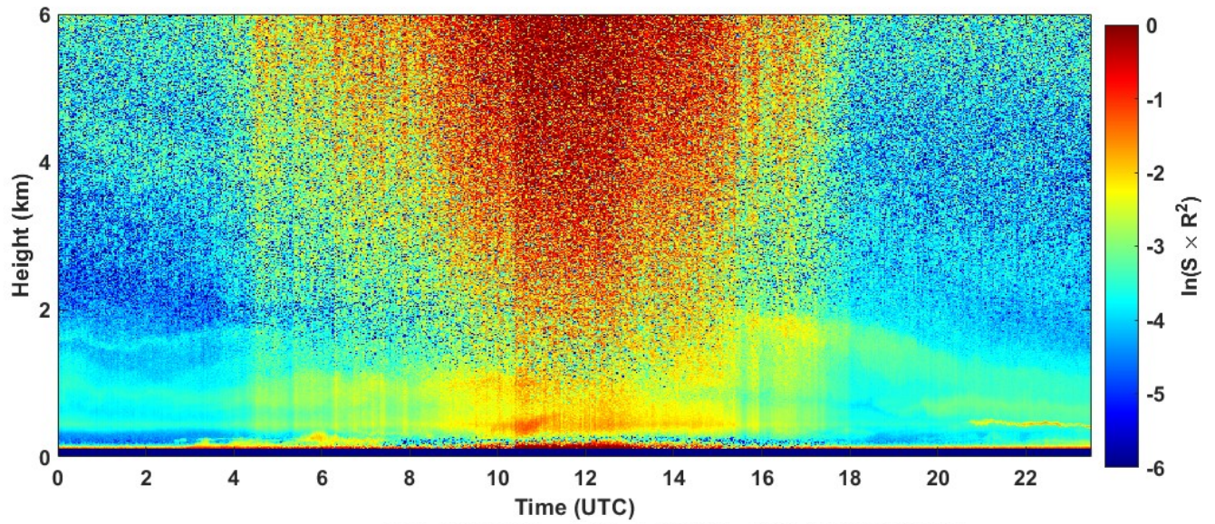
2022-05-24 RCS quick look CHM15k - ILVA LIDAR2 PARCHI
