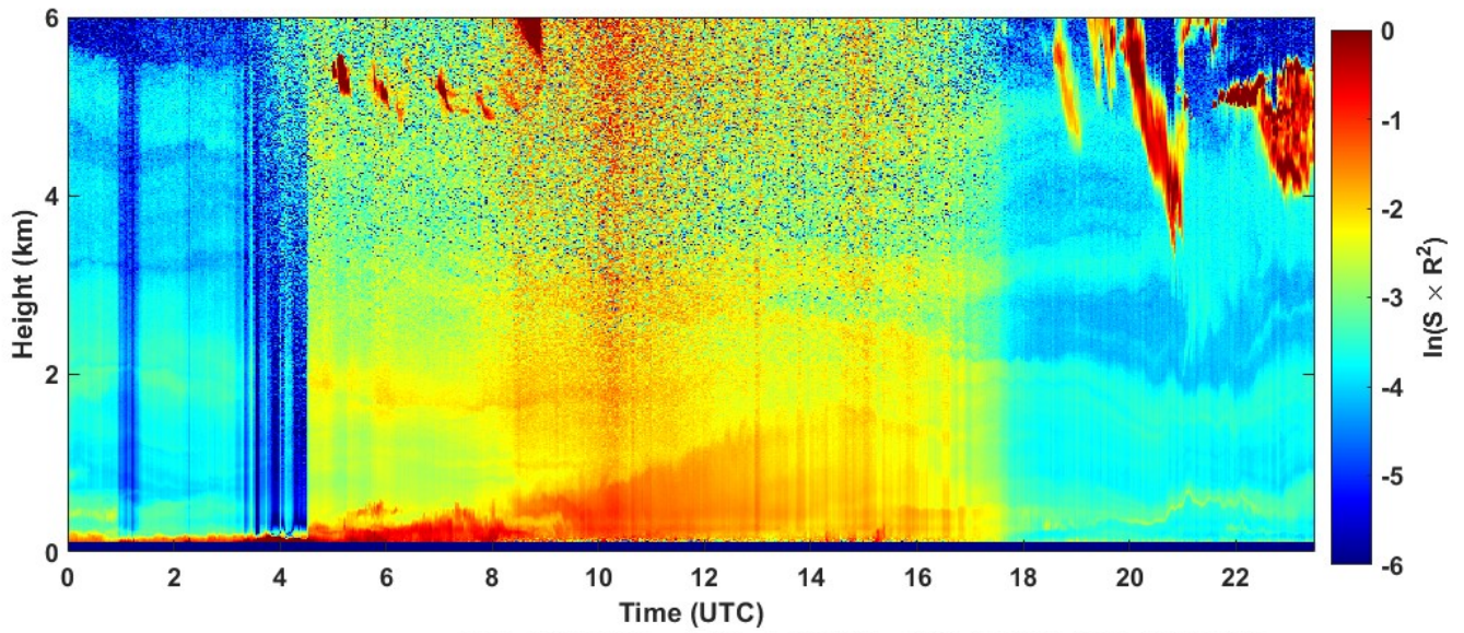
2022-05-28 RCS quick look CHM15k - ILVA LIDAR3 AGGLOMERATO
