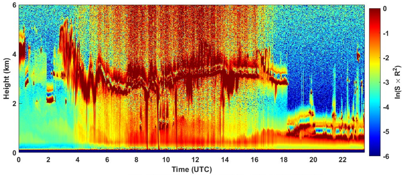
2022-05-08 RCS quick look CHM15k - ILVA LIDAR2 PARCHI
