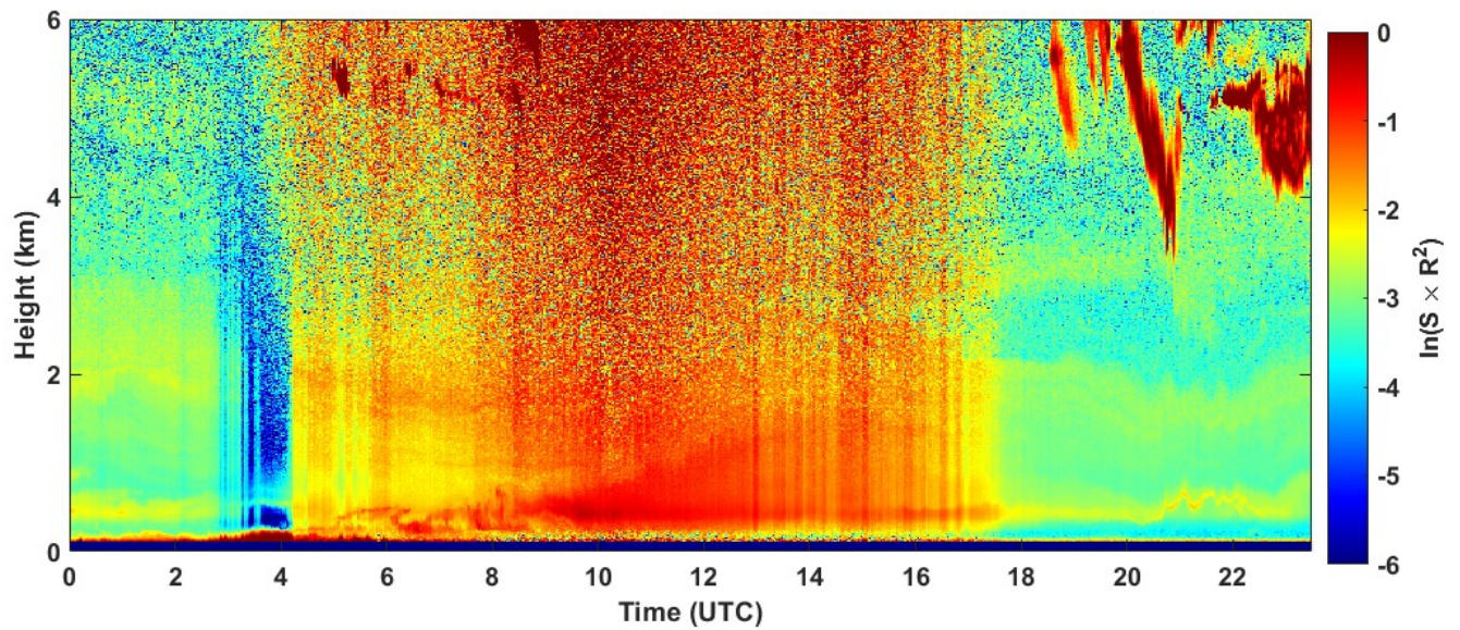
2022-05-28 RCS quick look CHM15k - ILVA LIDAR2 PARCHI
