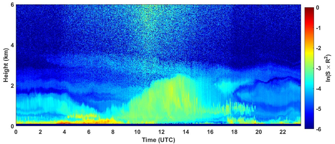
2022-05-14 RCS quick look CHM15k - ILVA LIDAR3 AGGLOMERATO
