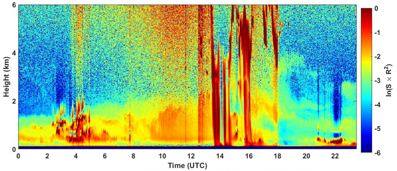
2022-05-30 RCS quick look CHM15k - ILVA LIDAR2 PARCHI
