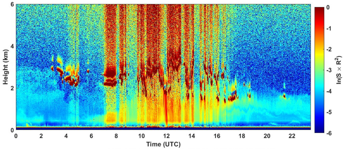
2022-05-04 RCS quick look CHM15k - ILVA LIDAR2 PARCHI
