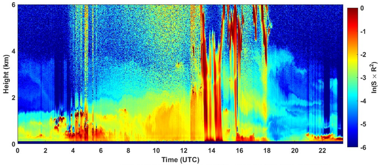
2022-05-30 RCS quick look CHM15k - ILVA LIDAR3 AGGLOMERATO
