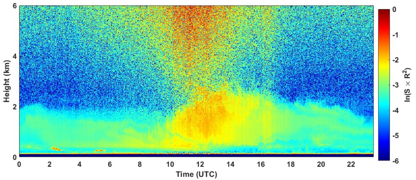
2022-05-12 RCS quick look CHM15k - ILVA LIDAR2 PARCHI
