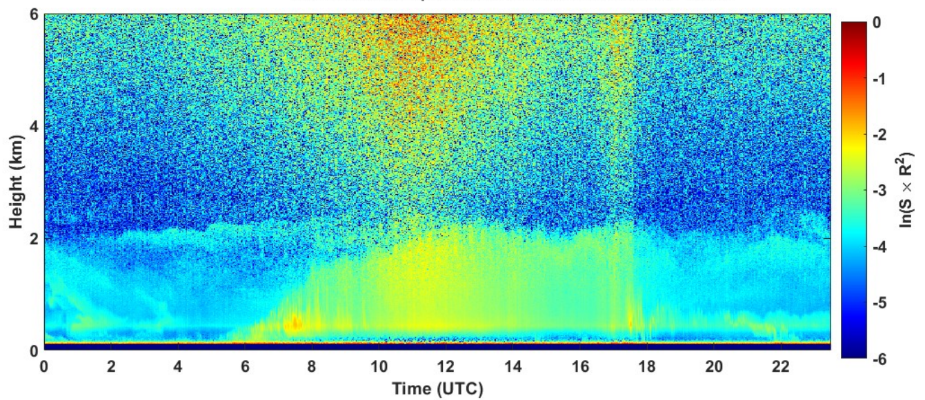
2022-05-14 RCS quick look CHM15k - ILVA LIDAR2 PARCHI
