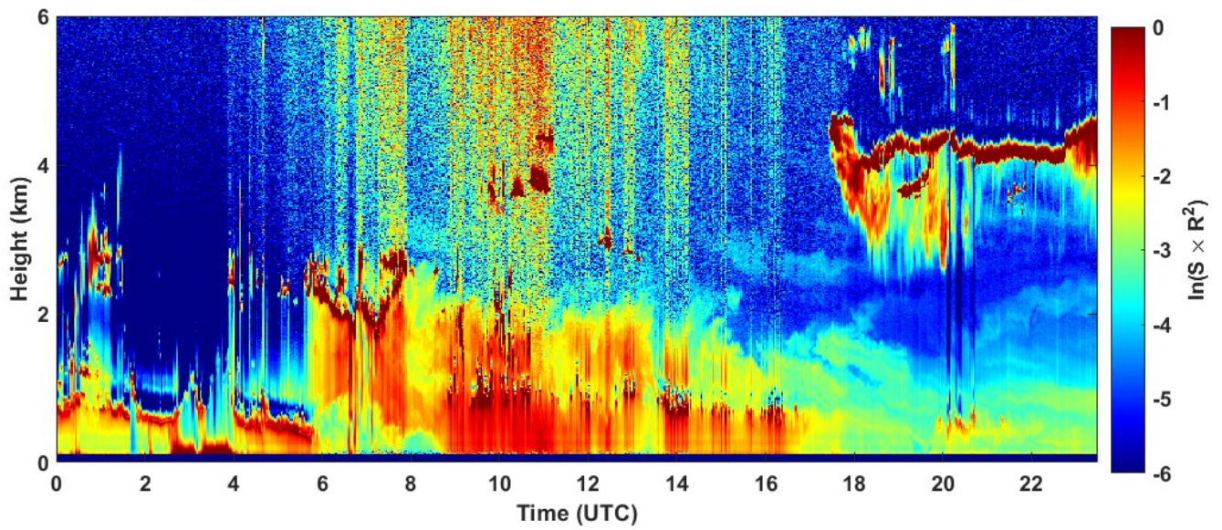
2022-05-08 RCS quick look CHM15k - ILVA LIDAR3 AGGLOMERATO
