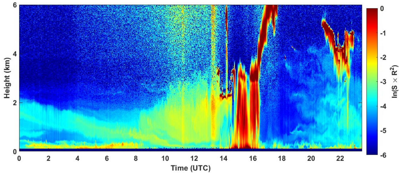
2022-05-18 RCS quick look CHM15k - ILVA LIDAR3 AGGLOMERATO
