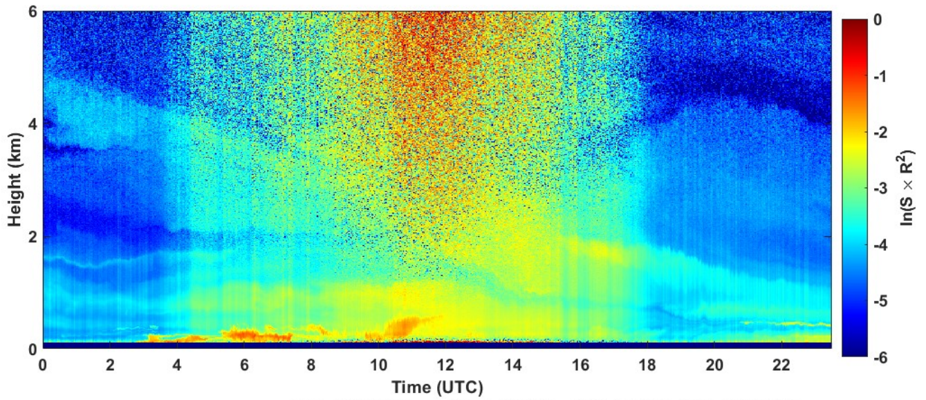
2022-05-24 RCS quick look CHM15k - ILVA LIDAR3 AGGLOMERATO
