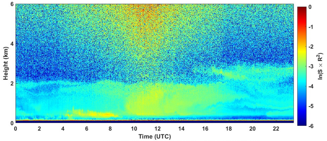
2022-05-16 RCS quick look CHM15k - ILVA LIDAR2 PARCHI
