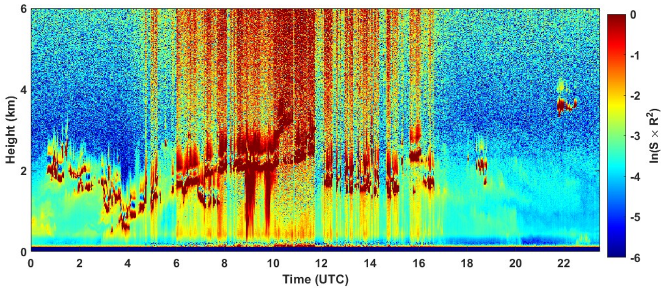
2022-05-02 RCS quick look CHM15k - ILVA LIDAR2 PARCHI
