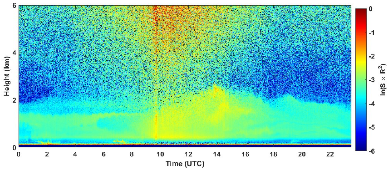
2022-05-22 RCS quick look CHM15k - ILVA LIDAR2 PARCHI
