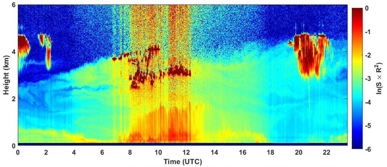
2022-05-10 RCS quick look CHM15k - ILVA LIDAR3 AGGLOMERATO
