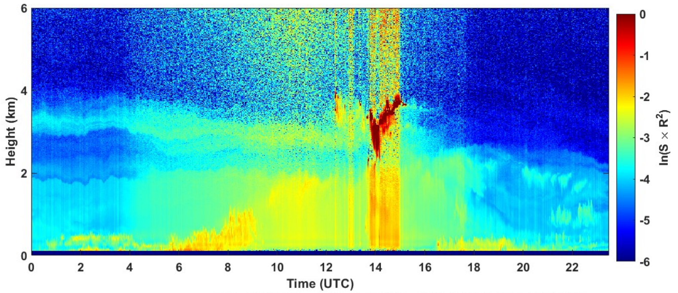
2022-05-12 RCS quick look CHM15k - ILVA LIDAR3 AGGLOMERATO
