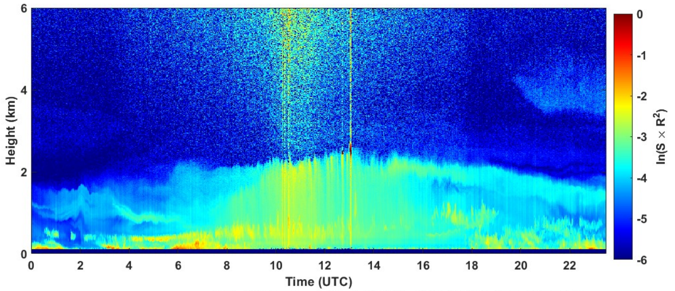
2022-05-22 RCS quick look CHM15k - ILVA LIDAR3 AGGLOMERATO
