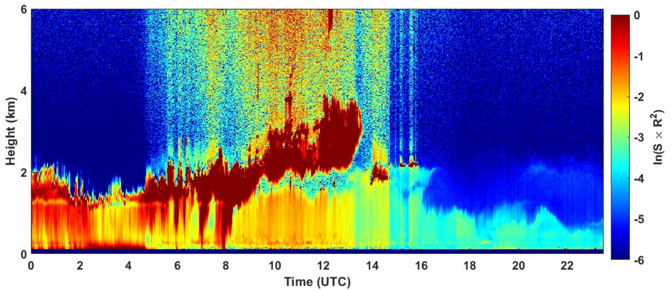
2022-04-18 RCS quick look CHM15k - ILVA LIDAR3 AGGLOMERATO
