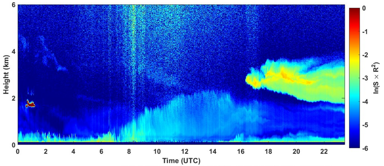
2022-04-24 RCS quick look CHM15k - ILVA LIDAR3 AGGLOMERATO
