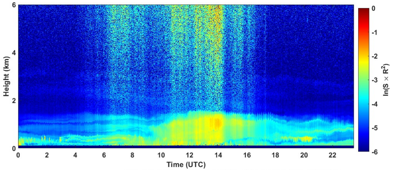
2022-04-14 RCS quick look CHM15k - ILVA LIDAR3 AGGLOMERATO
