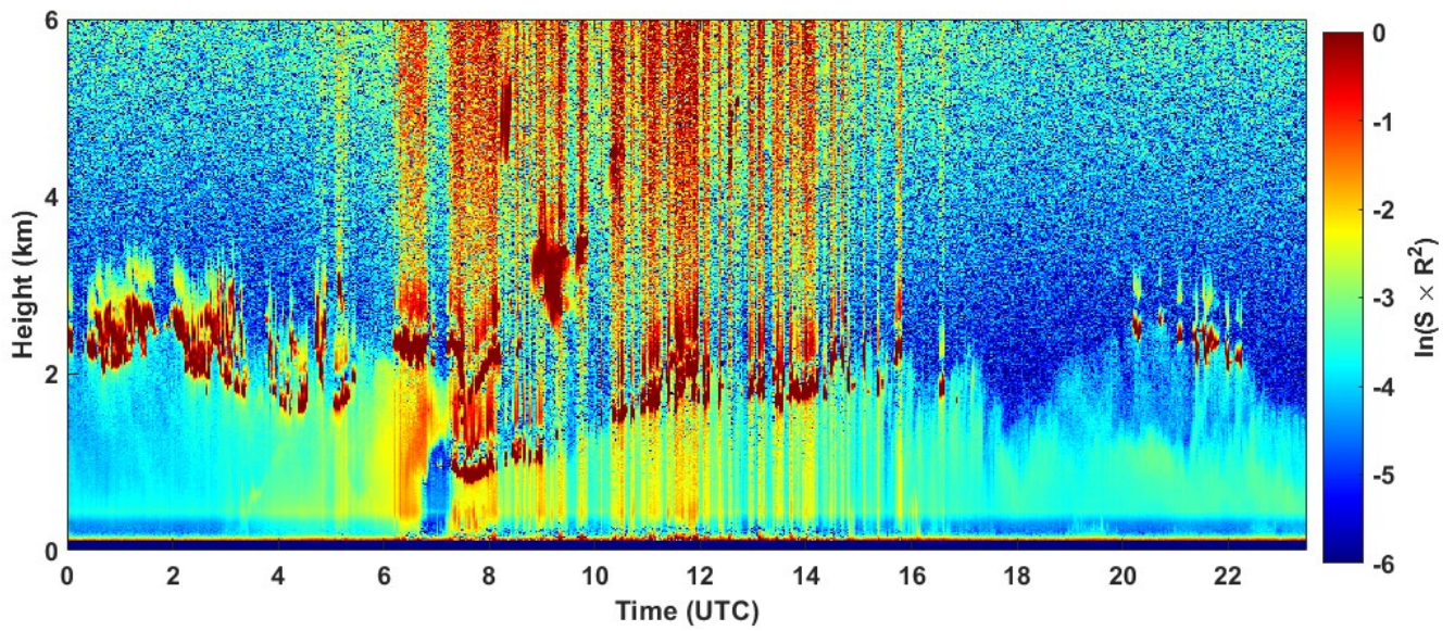
2022-04-10 RCS quick look CHM15k - ILVA LIDAR2 PARCHI
