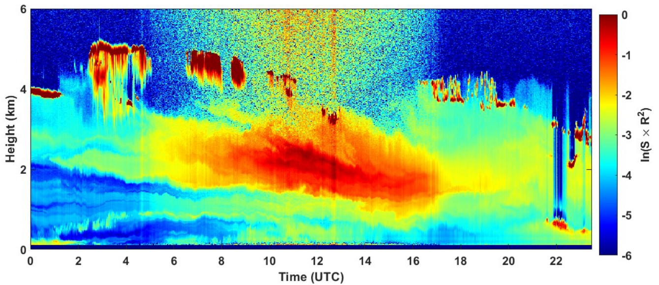
2022-04-06 RCS quick look CHM15k - ILVA LIDAR3 AGGLOMERATO
