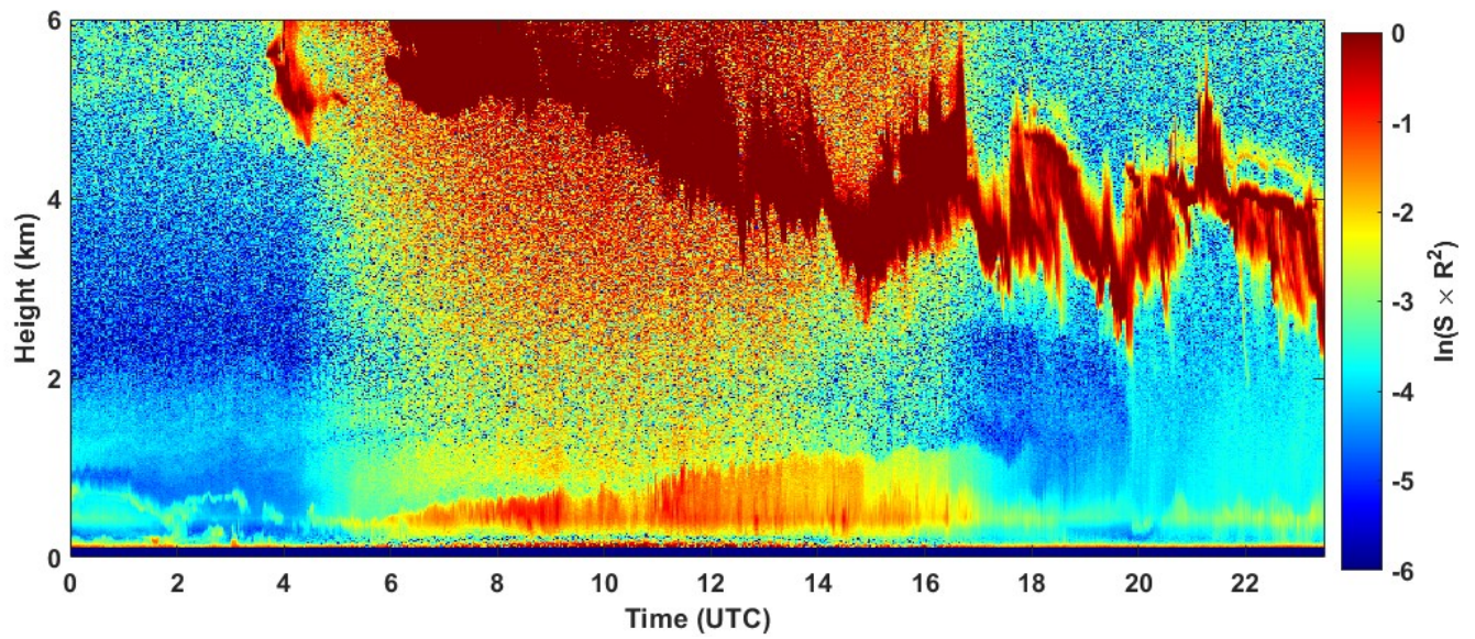
2022-04-16 RCS quick look CHM15k - ILVA LIDAR2 PARCHI
