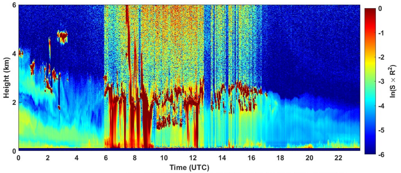
2022-04-08 RCS quick look CHM15k - ILVA LIDAR3 AGGLOMERATO
