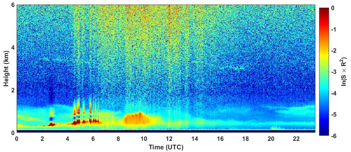
2022-04-14 RCS quick look CHM15k - ILVA LIDAR2 PARCHI
