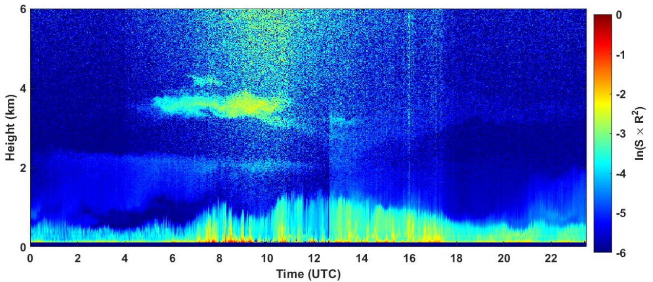
2022-04-28 RCS quick look CHM15k - ILVA LIDAR3 AGGLOMERATO
