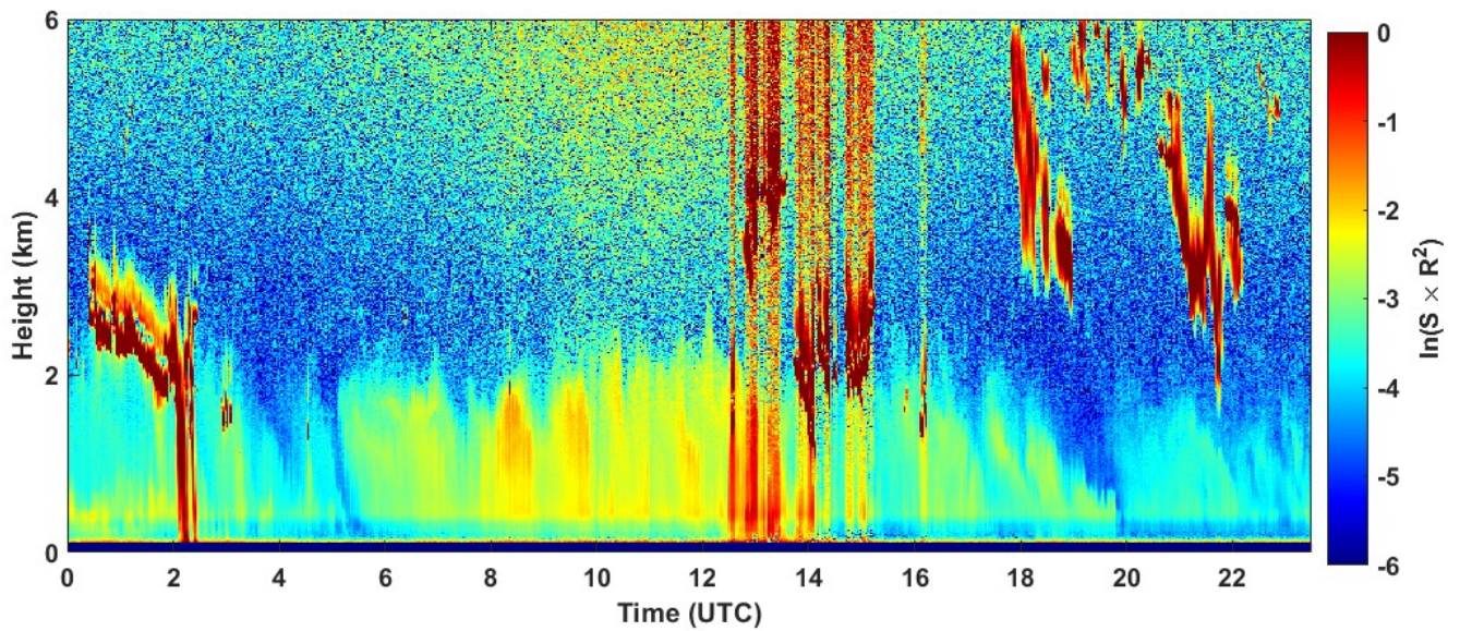
2022-04-02 RCS quick look CHM15k - ILVA LIDAR2 PARCHI
