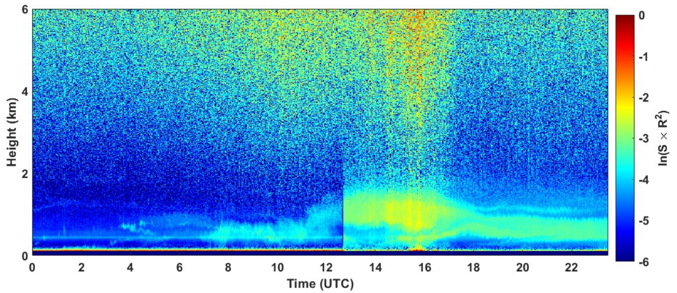
2022-04-12 RCS quick look CHM15k - ILVA LIDAR2 PARCHI
