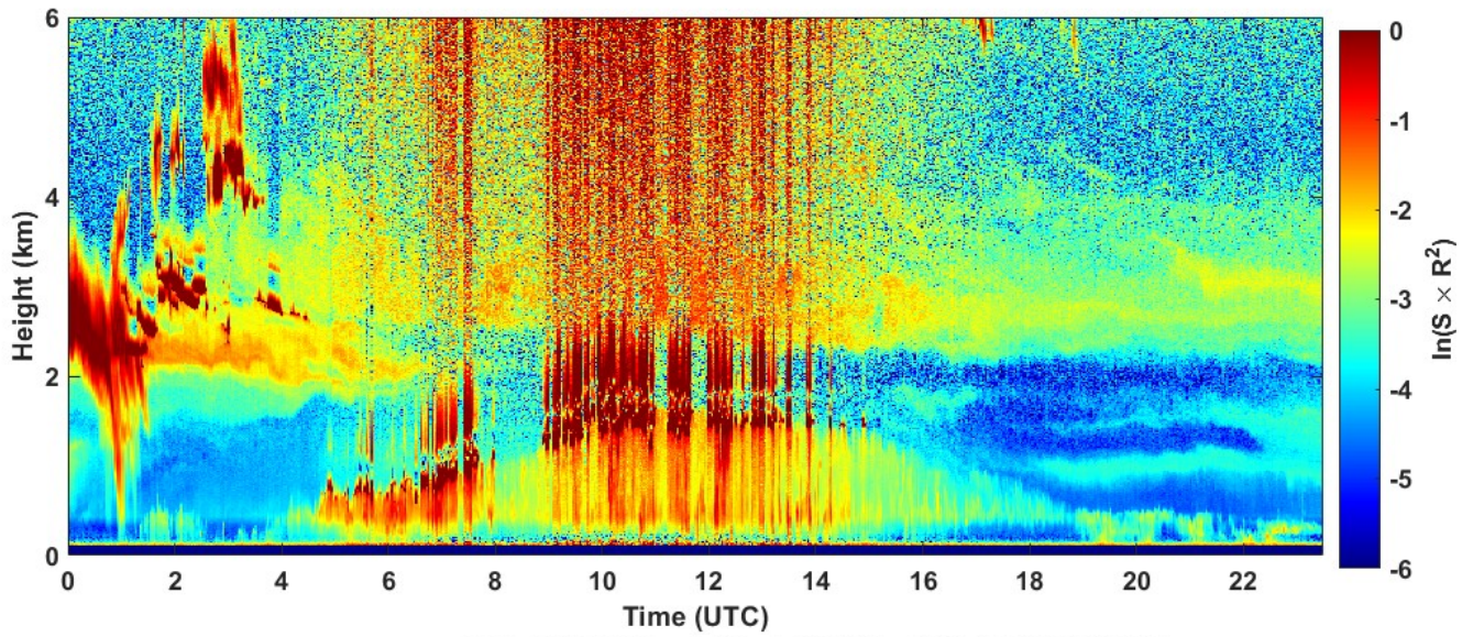
2022-04-06 RCS quick look CHM15k - ILVA LIDAR2 PARCHI
