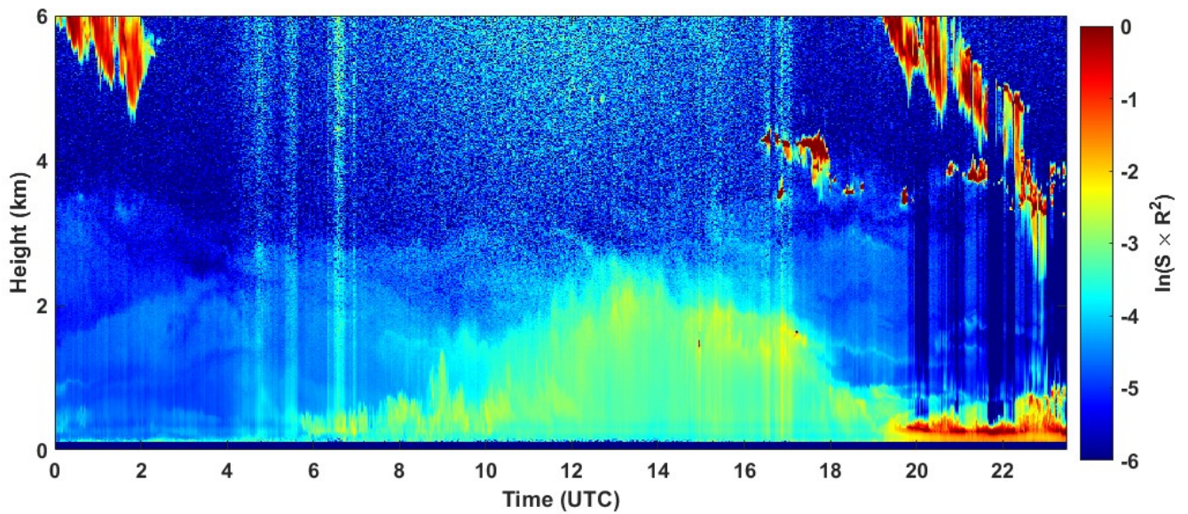
2022-04-20 RCS quick look CHM15k - ILVA LIDAR3 AGGLOMERATO
