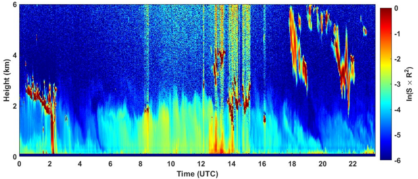
2022-04-02 RCS quick look CHM15k - ILVA LIDAR3 AGGLOMERATO
