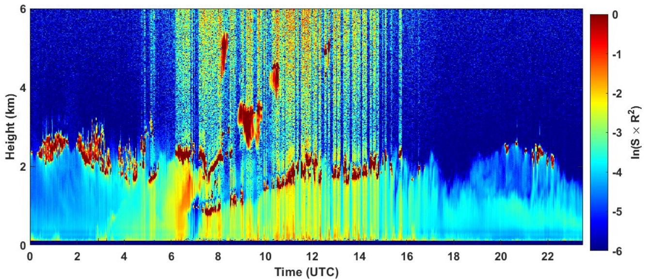
2022-04-10 RCS quick look CHM15k - ILVA LIDAR3 AGGLOMERATO
