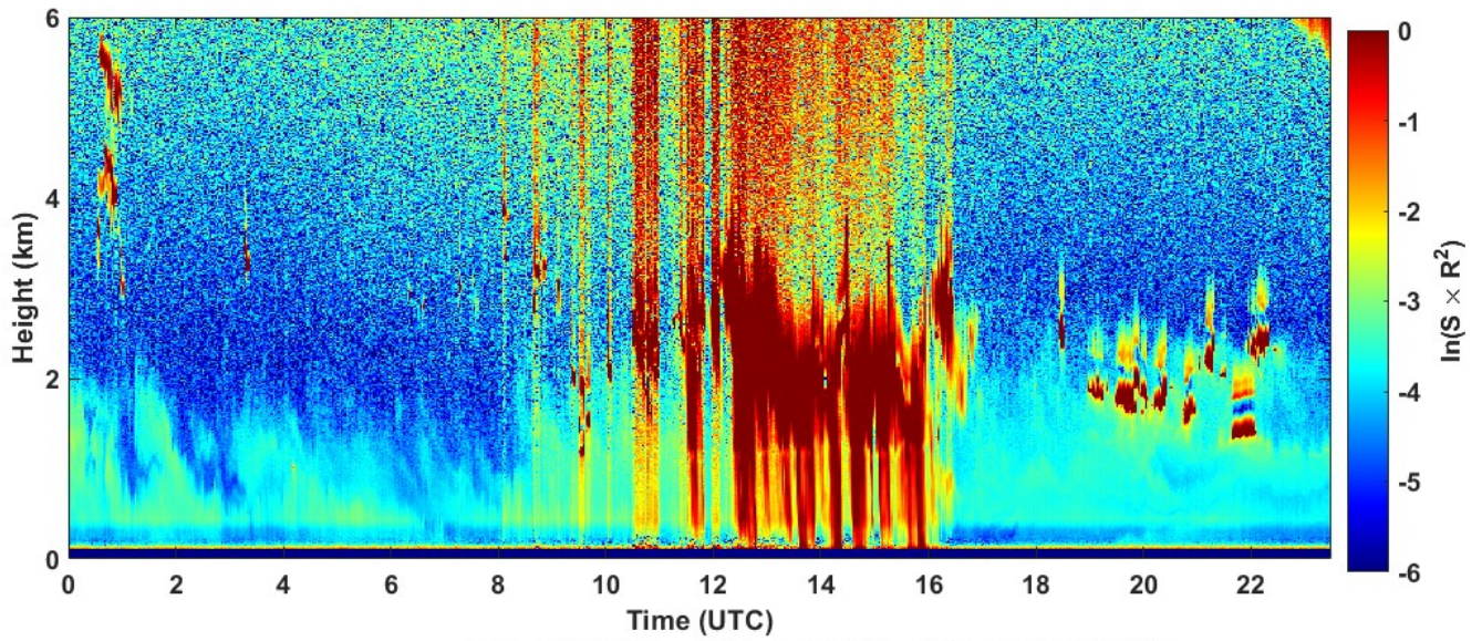
2022-04-04 RCS quick look CHM15k - ILVA LIDAR2 PARCHI
