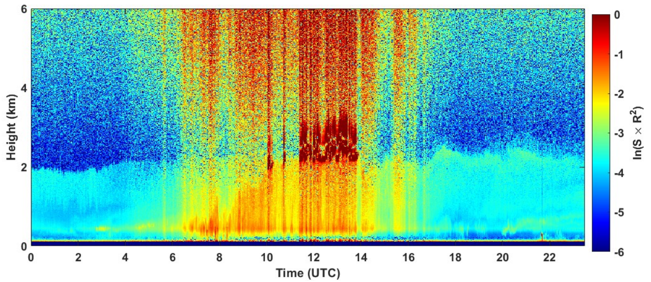
2022-04-30 RCS quick look CHM15k - ILVA LIDAR2 PARCHI
