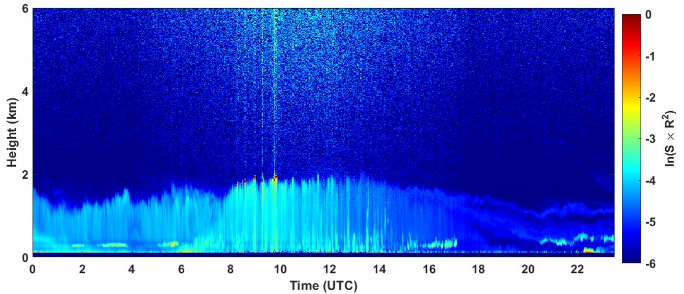
2022-04-12 RCS quick look CHM15k - ILVA LIDAR3 AGGLOMERATO
