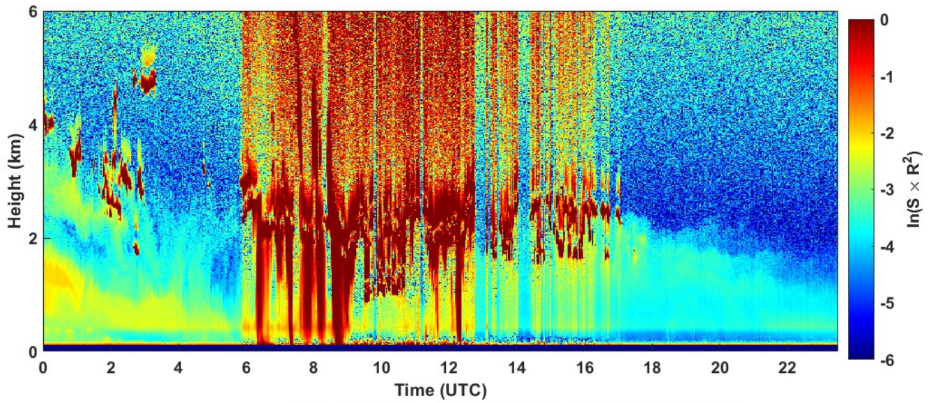
2022-04-08 RCS quick look CHM15k - ILVA LIDAR2 PARCHI
