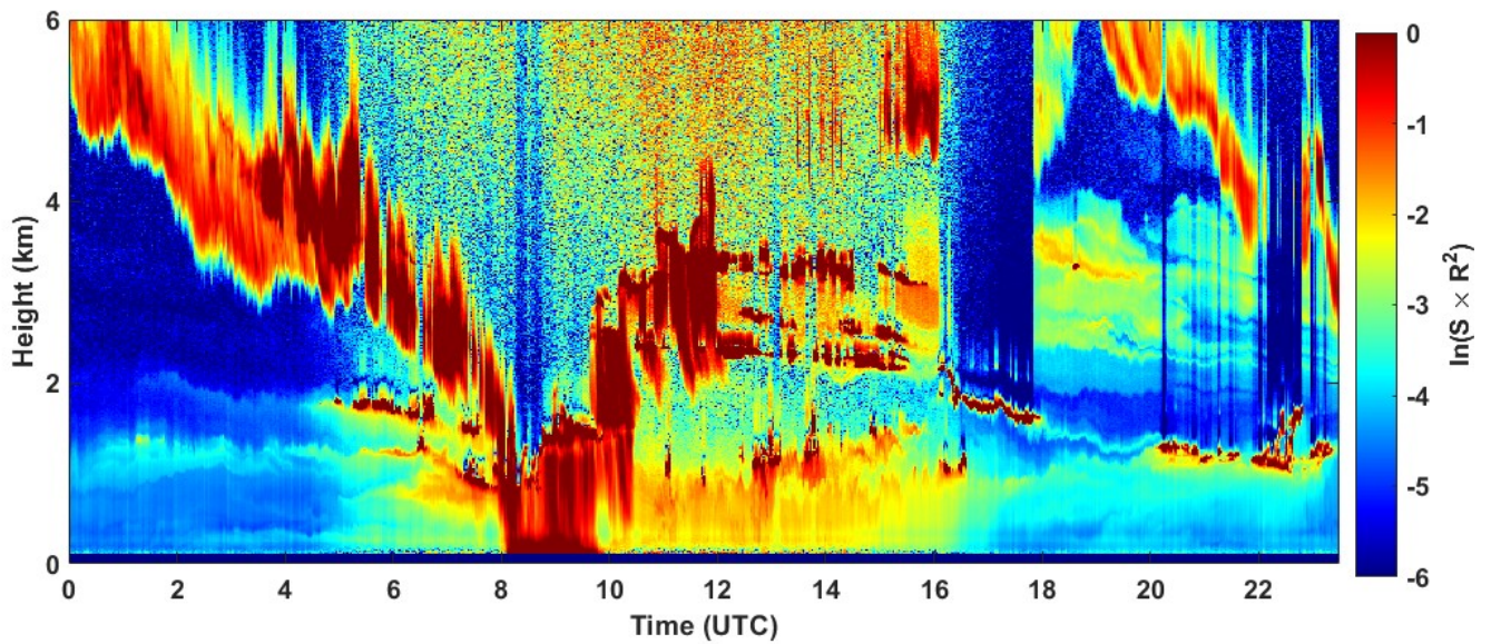
2022-04-04 RCS quick look CHM15k - ILVA LIDAR3 AGGLOMERATO
