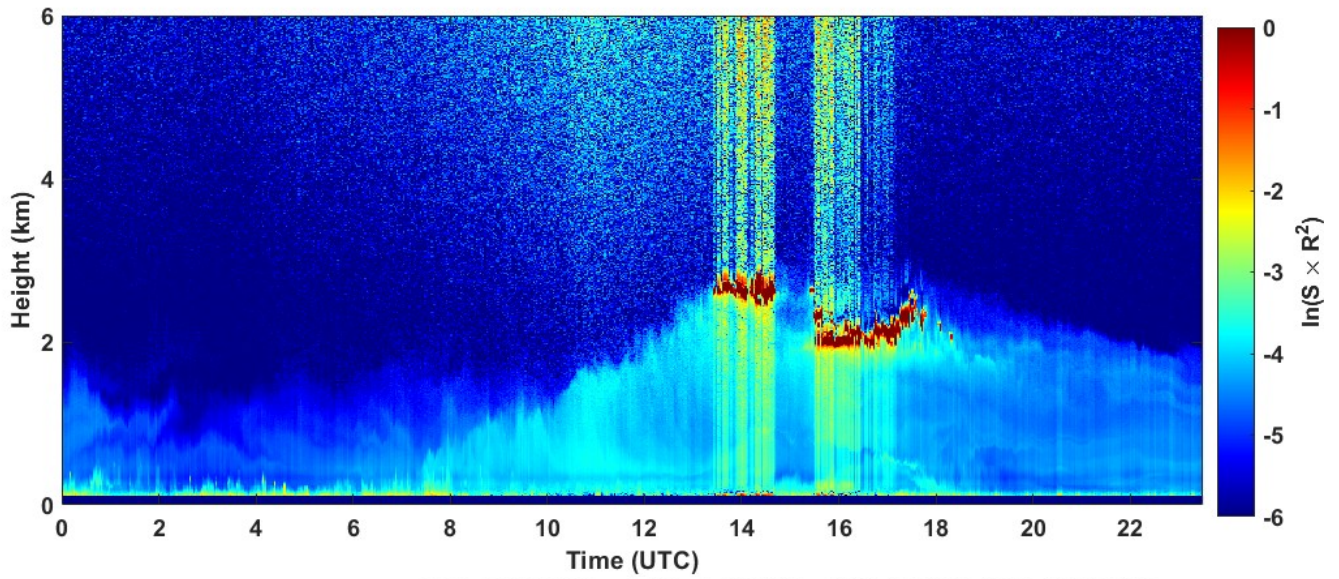
2022-04-26 RCS quick look CHM15k - ILVA LIDAR3 AGGLOMERATO
