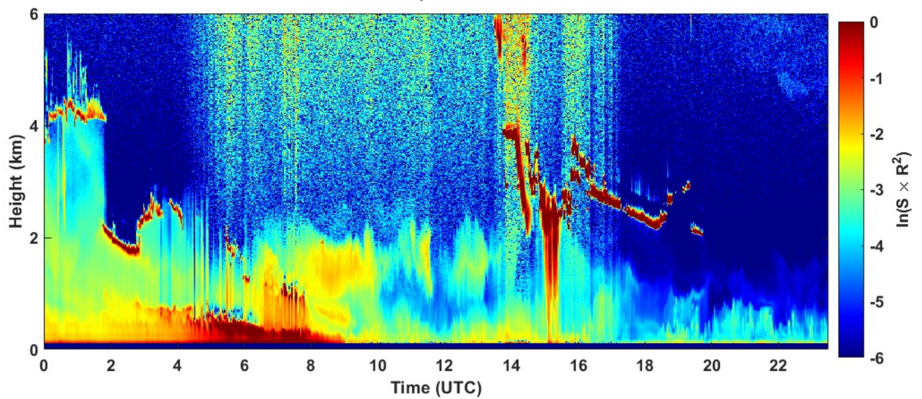
2022-04-22 RCS quick look CHM15k - ILVA LIDAR3 AGGLOMERATO
