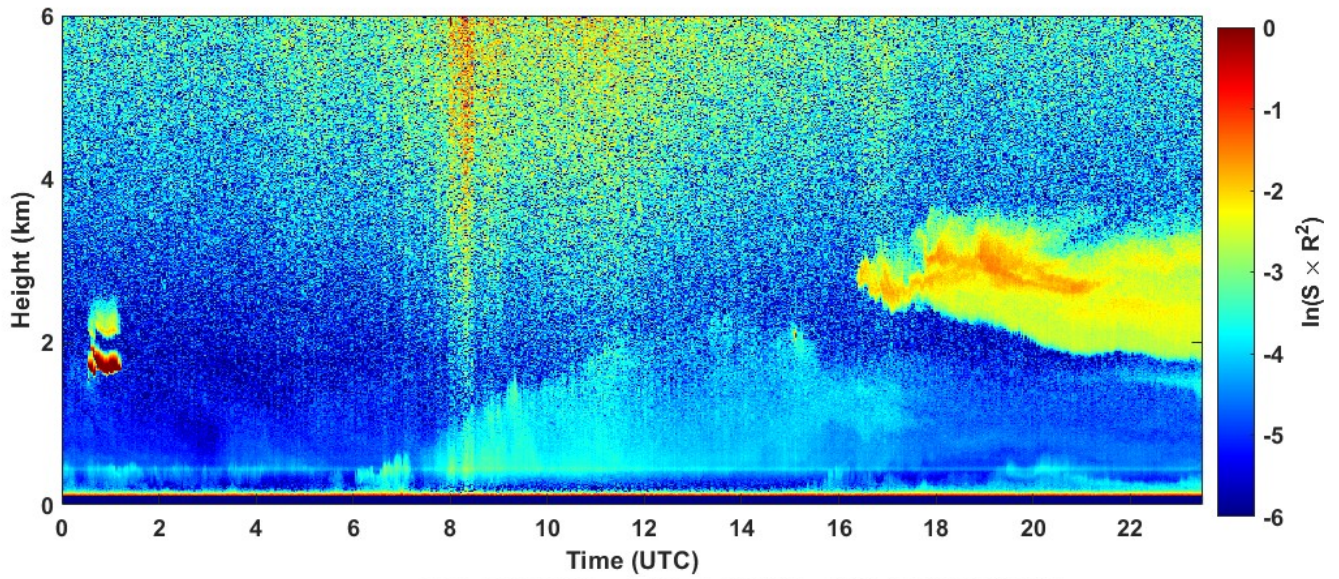
2022-04-24 RCS quick look CHM15k - ILVA LIDAR2 PARCHI
