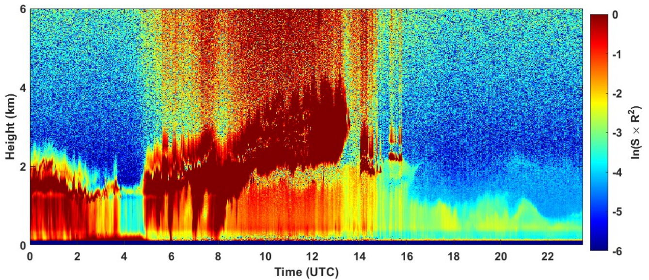
2022-04-18 RCS quick look CHM15k - ILVA LIDAR2 PARCHI
