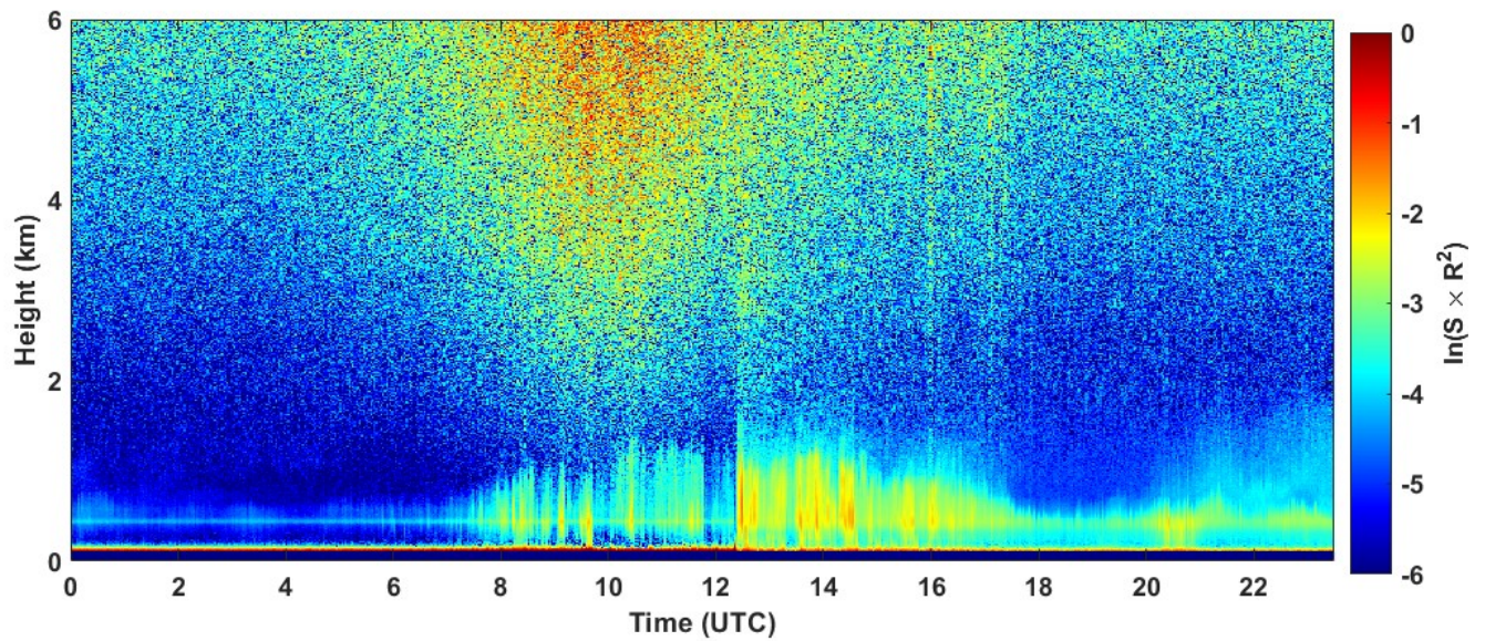
2022-04-28 RCS quick look CHM15k - ILVA LIDAR2 PARCHI
