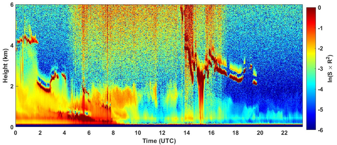
2022-04-22 RCS quick look CHM15k - ILVA LIDAR2 PARCHI
