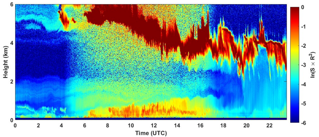
2022-04-16 RCS quick look CHM15k - ILVA LIDAR3 AGGLOMERATO
