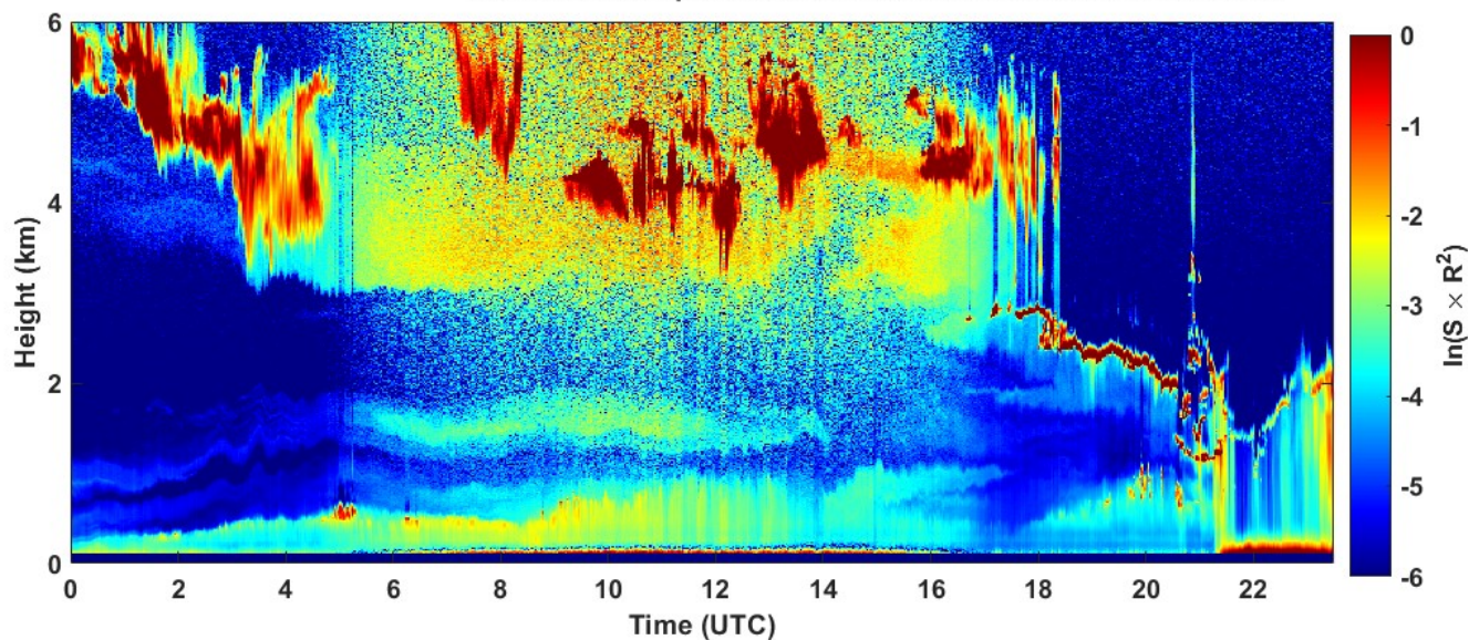
2022-03-28 RCS quick look CHM15k - ILVA LIDAR3 AGGLOMERATO
