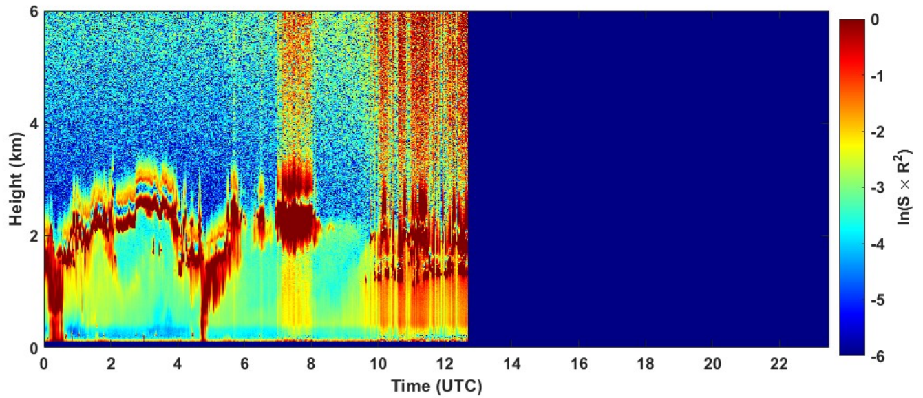
2022-03-02 RCS quick look CHM15k - ILVA LIDAR2 PARCHI
