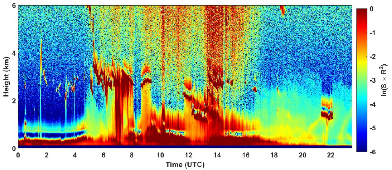
2022-03-31 RCS quick look CHM15k - ILVA LIDAR2 PARCHI
