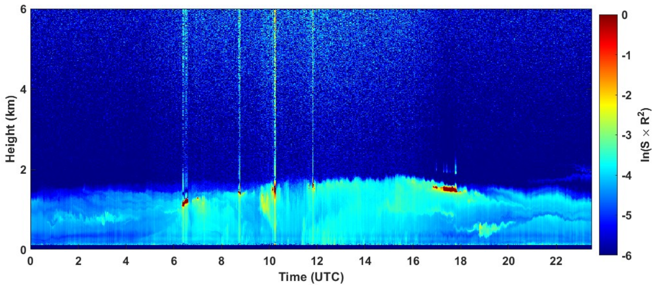
2022-03-14 RCS quick look CHM15k - ILVA LIDAR3 AGGLOMERATO
