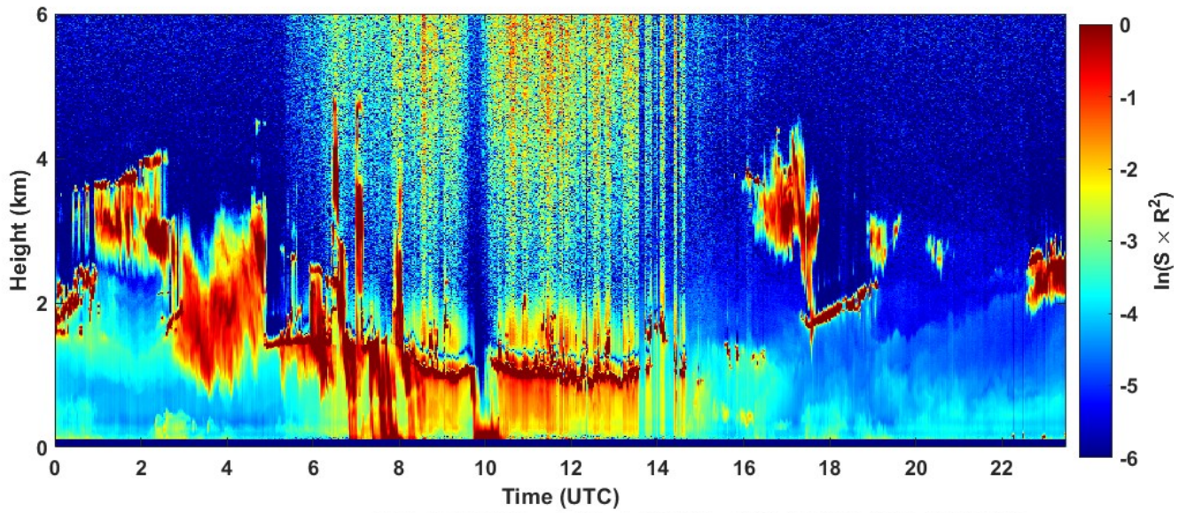
2022-03-08 RCS quick look CHM15k - ILVA LIDAR3 AGGLOMERATO
