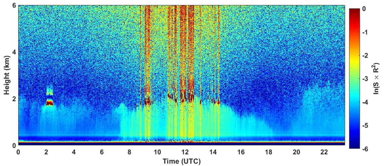
2022-03-25 RCS quick look CHM15k - ILVA LIDAR2 PARCHI
