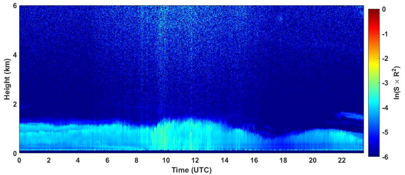
2022-03-16 RCS quick look CHM15k - ILVA LIDAR3 AGGLOMERATO
