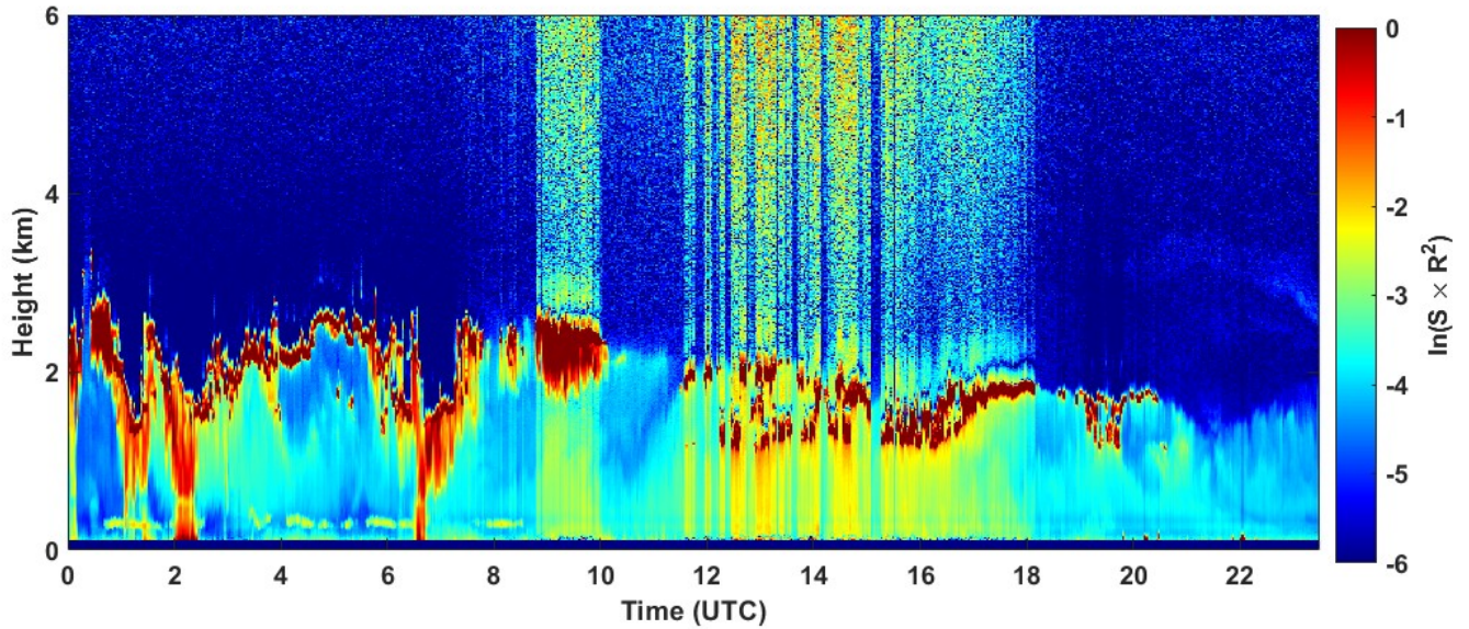
2022-03-02 RCS quick look CHM15k - ILVA LIDAR3 AGGLOMERATO
