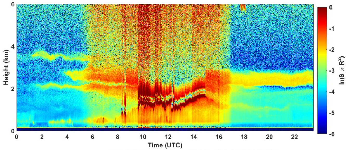
2022-03-18 RCS quick look CHM15k - ILVA LIDAR2 PARCHI
