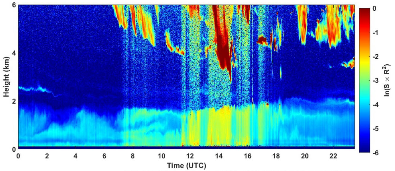
2022-03-04 RCS quick look CHM15k - ILVA LIDAR3 AGGLOMERATO
