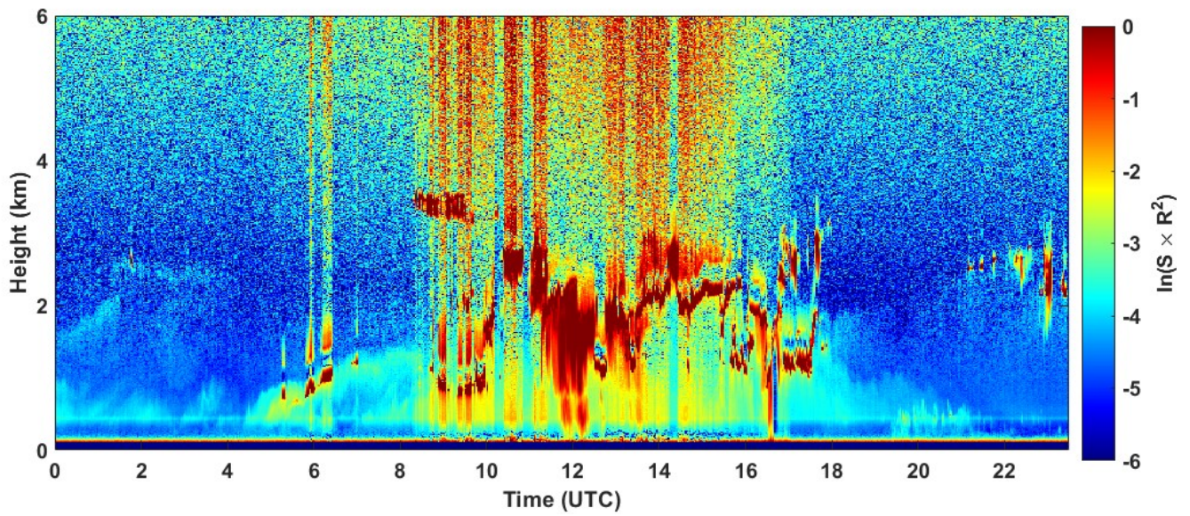
2022-03-20 RCS quick look CHM15k - ILVA LIDAR2 PARCHI
