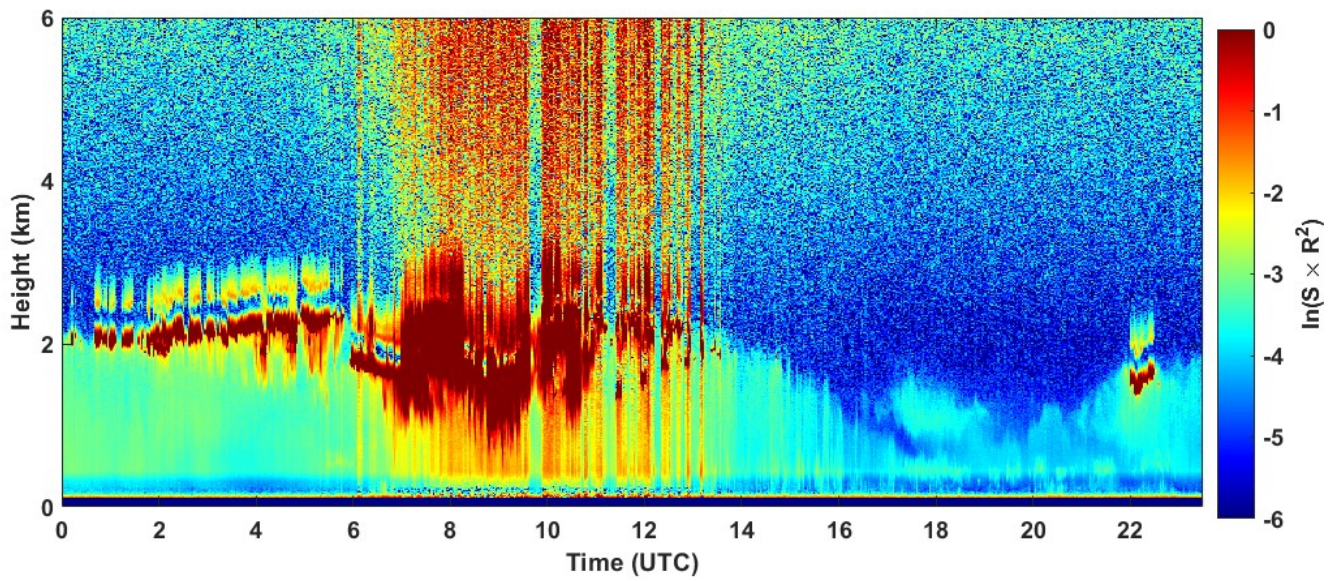
2022-03-11 RCS quick look CHM15k - ILVA LIDAR2 PARCHI
