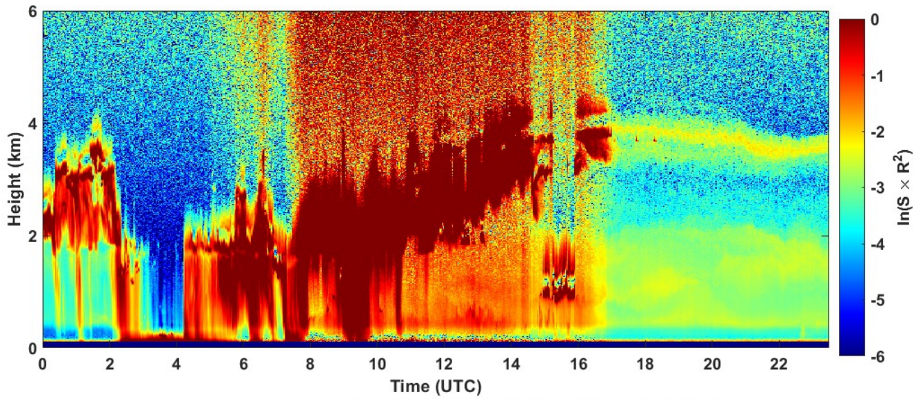
2022-03-29 RCS quick look CHM15k - ILVA LIDAR2 PARCHI
