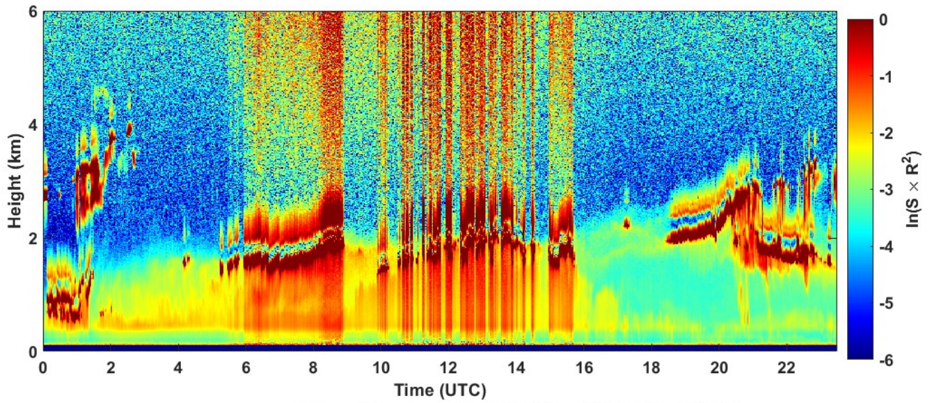
2022-03-07 RCS quick look CHM15k - ILVA LIDAR2 PARCHI
