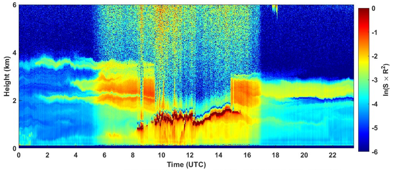
2022-03-18 RCS quick look CHM15k - ILVA LIDAR3 AGGLOMERATO
