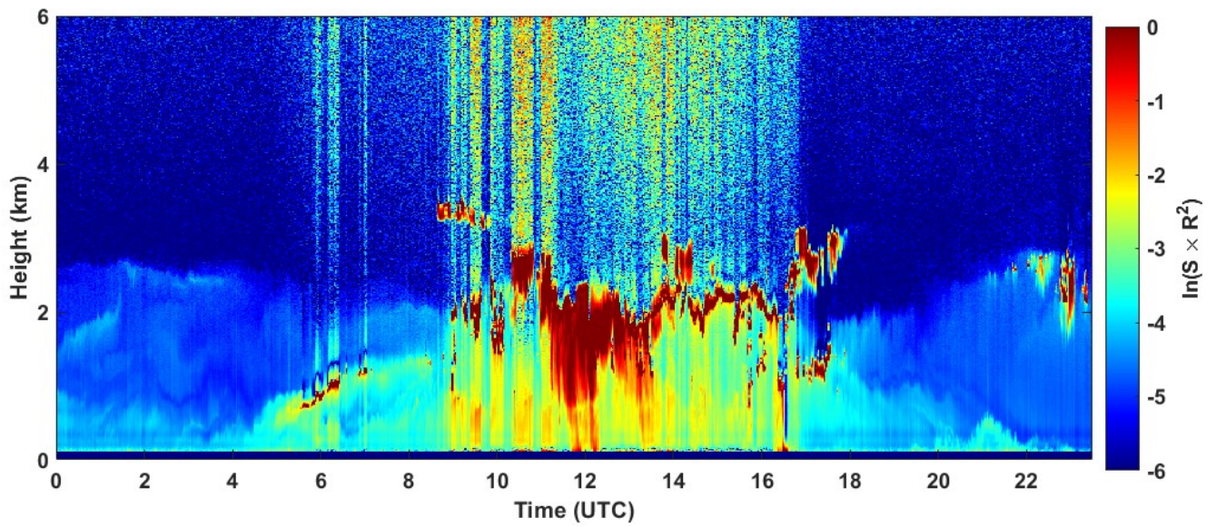
2022-03-20 RCS quick look CHM15k - ILVA LIDAR3 AGGLOMERATO
