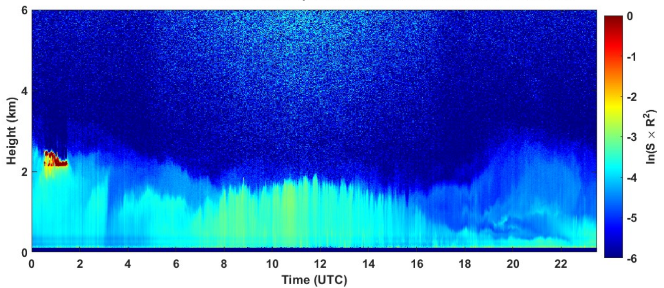
2022-03-22 RCS quick look CHM15k - ILVA LIDAR3 AGGLOMERATO
