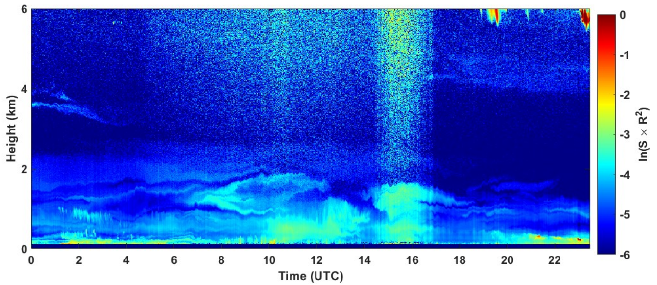
2022-03-26 RCS quick look CHM15k - ILVA LIDAR3 AGGLOMERATO
