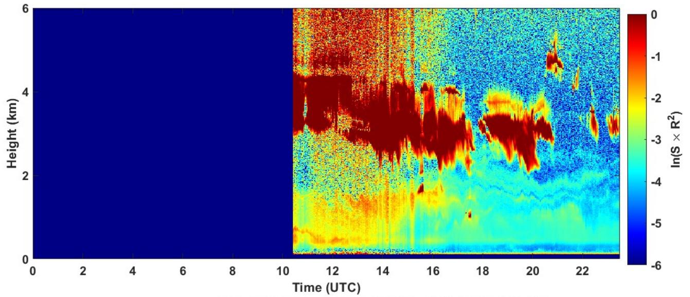
2022-03-05 RCS quick look CHM15k - ILVA LIDAR2 PARCHI
