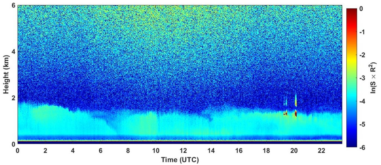
2022-03-13 RCS quick look CHM15k - ILVA LIDAR2 PARCHI
