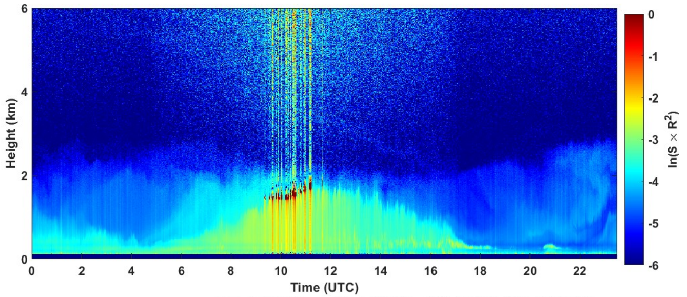
2022-03-24 RCS quick look CHM15k - ILVA LIDAR3 AGGLOMERATO
