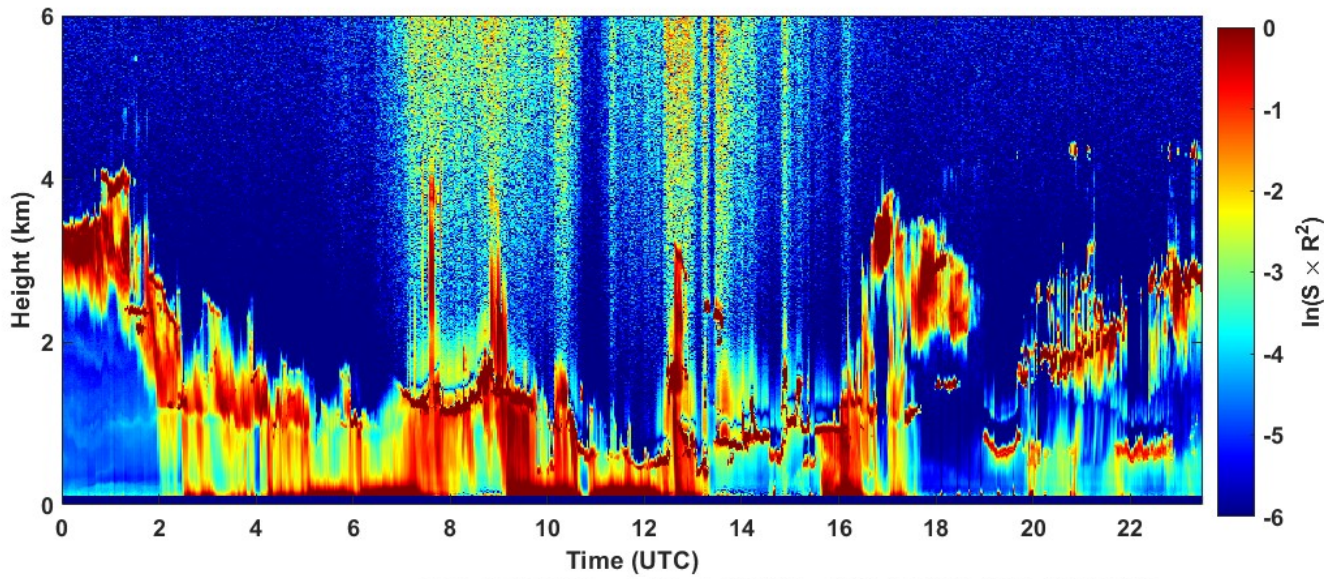
2022-03-06 RCS quick look CHM15k - ILVA LIDAR3 AGGLOMERATO
