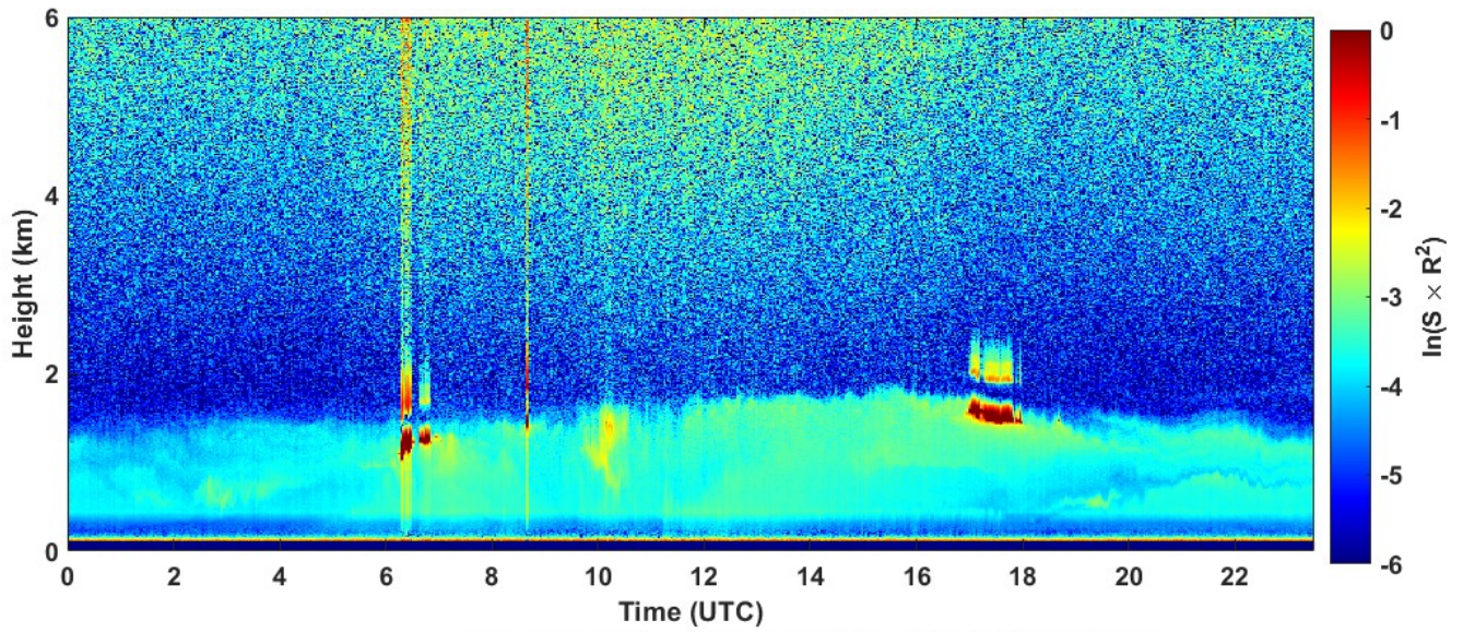
2022-03-15 RCS quick look CHM15k - ILVA LIDAR2 PARCHI
