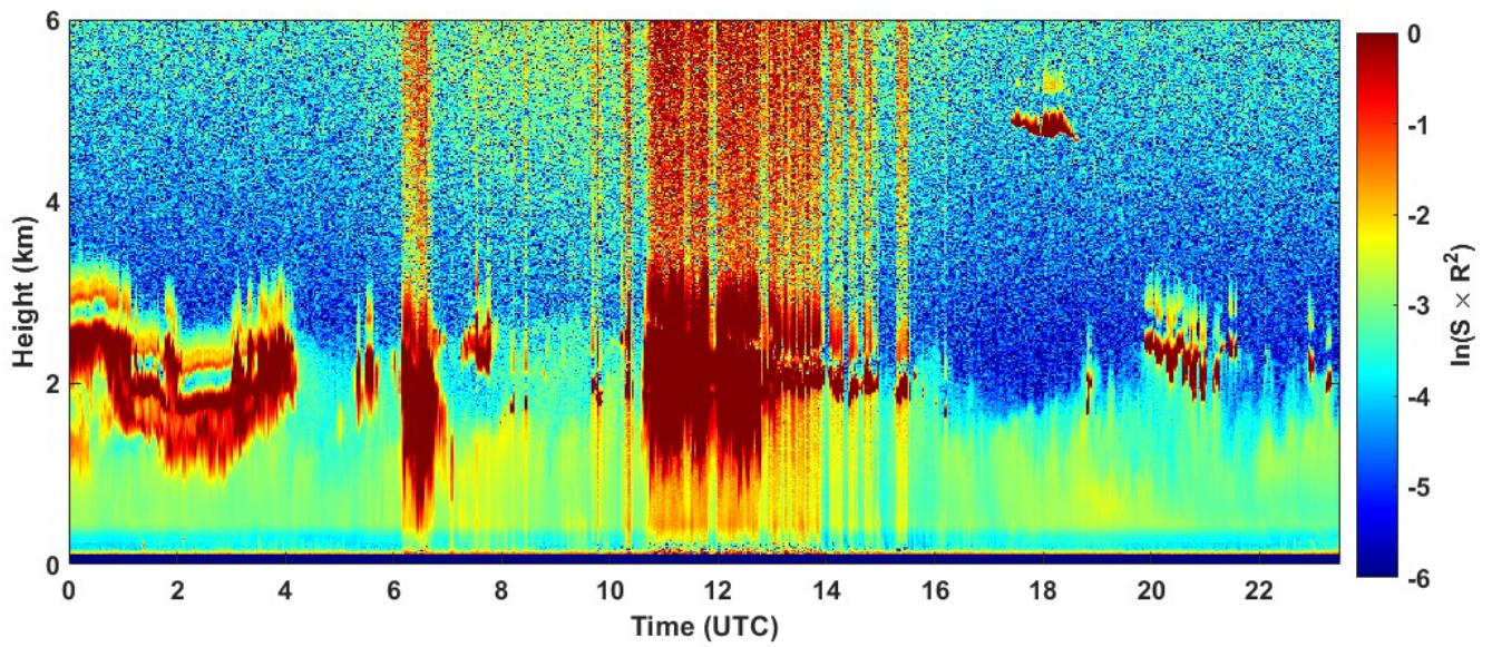
2022-03-09 RCS quick look CHM15k - ILVA LIDAR2 PARCHI
