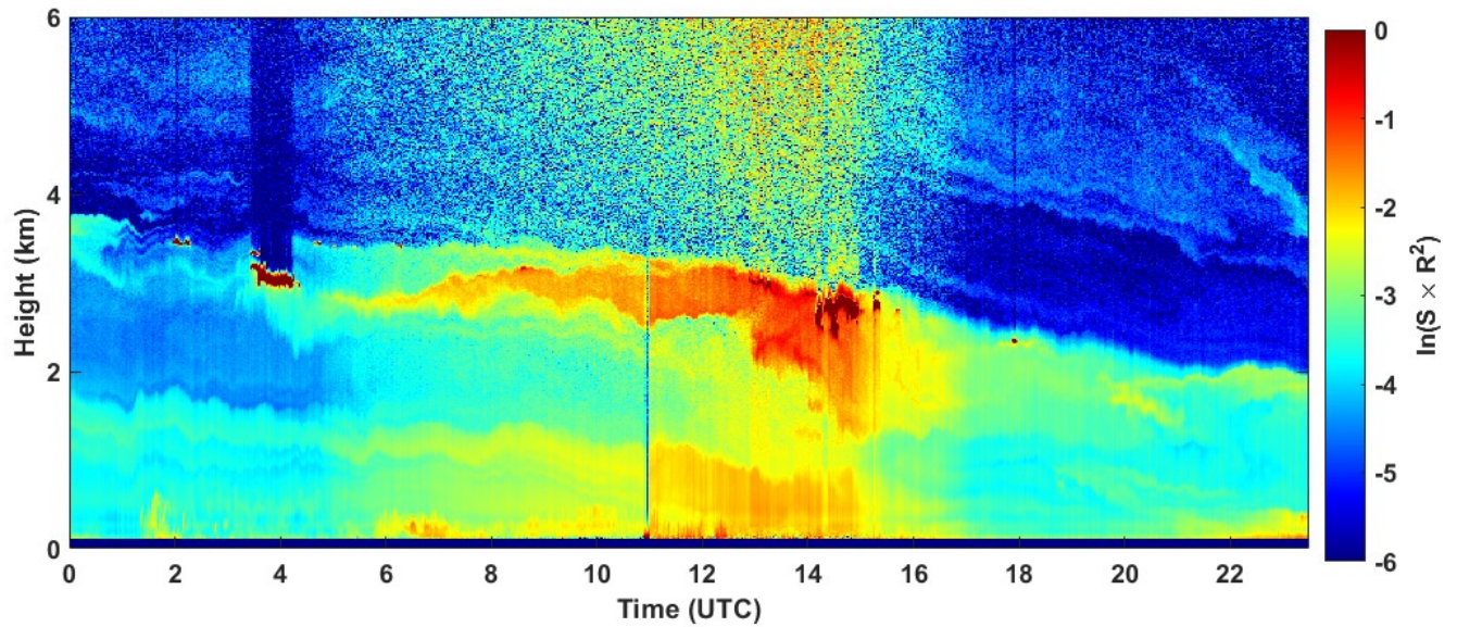
2022-03-30 RCS quick look CHM15k - ILVA LIDAR3 AGGLOMERATO
