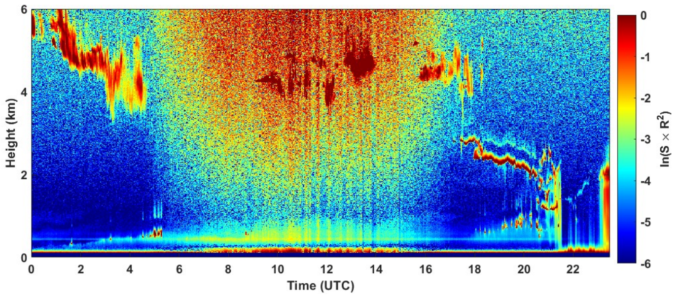
2022-03-27 RCS quick look CHM15k - ILVA LIDAR2 PARCHI
