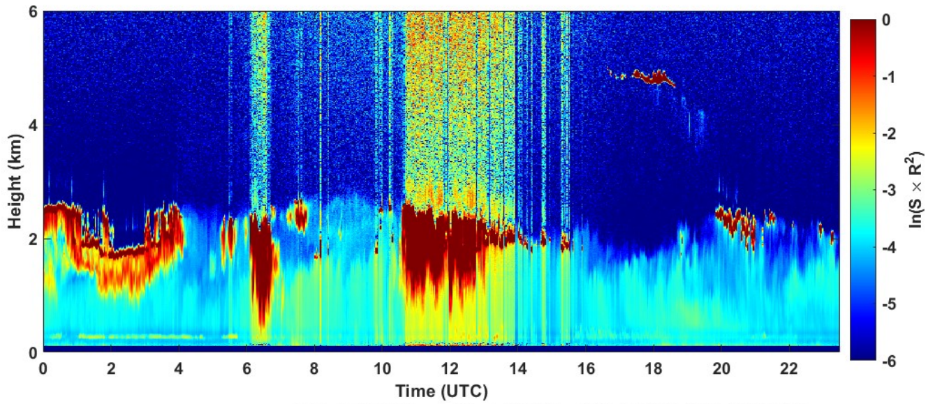
2022-03-10 RCS quick look CHM15k - ILVA LIDAR3 AGGLOMERATO
