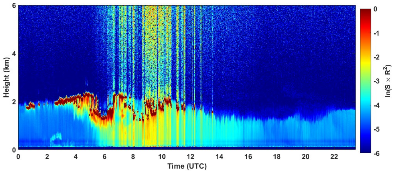
2022-03-12 RCS quick look CHM15k - ILVA LIDAR3 AGGLOMERATO
