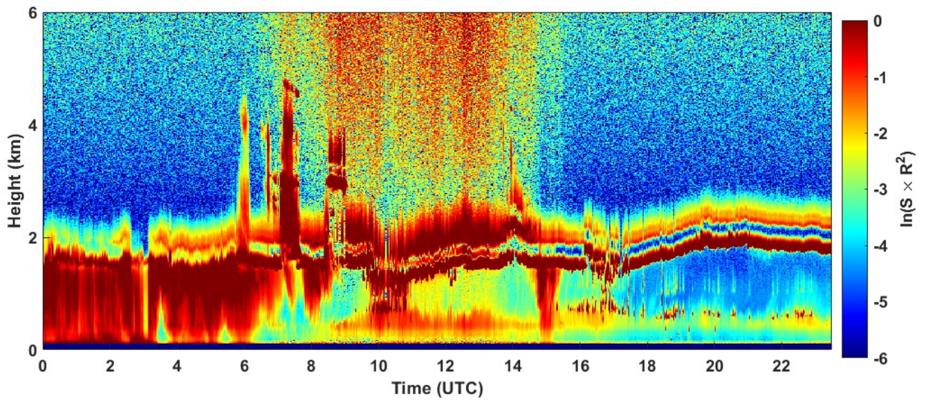
2022-01-08 RCS quick look CHM15k - ILVA LIDAR2 PARCHI
