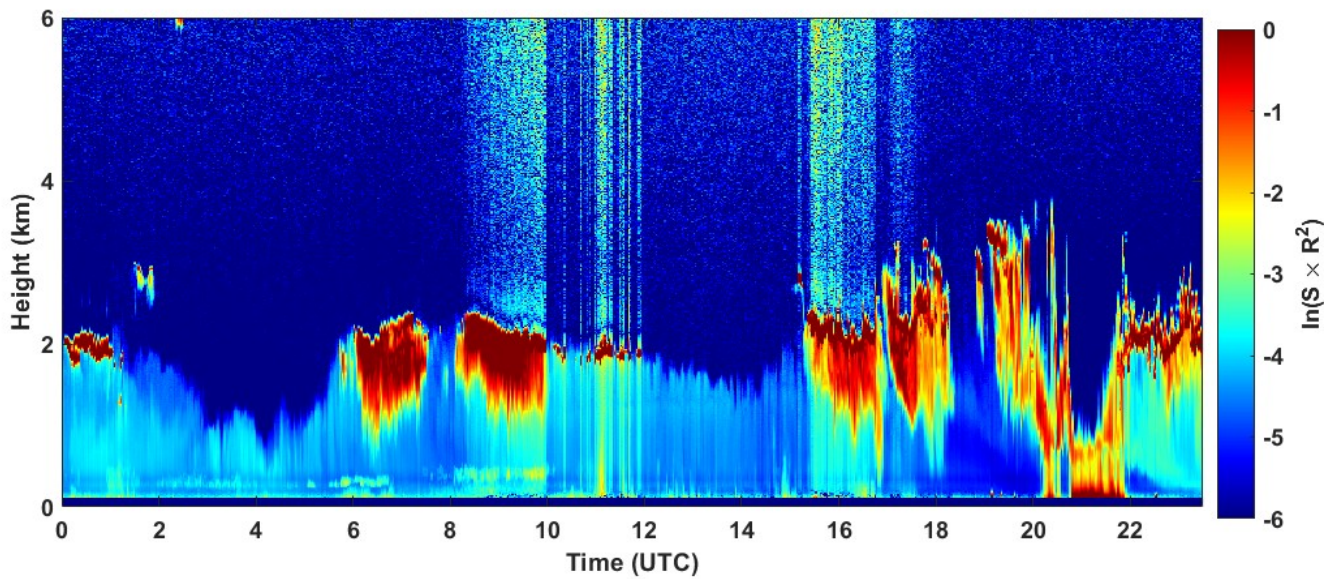
2022-01-22 RCS quick look CHM15k - ILVA LIDAR3 AGGLOMERATO
