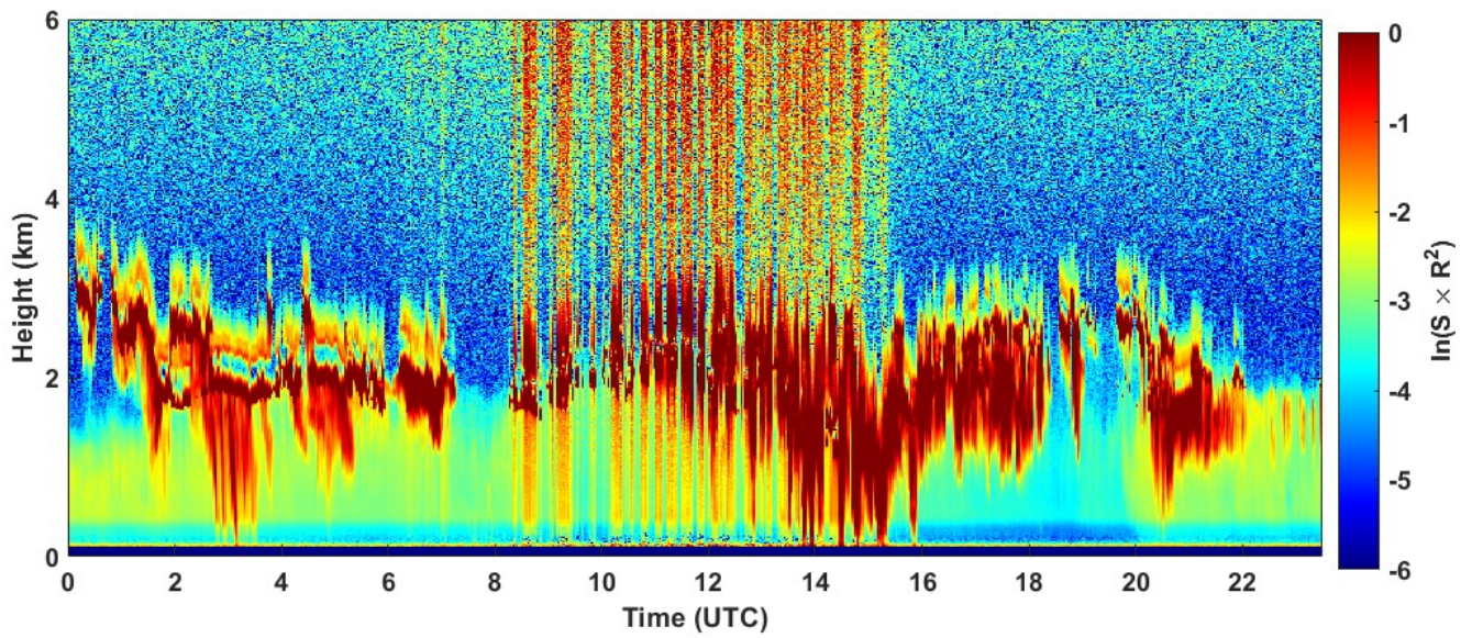
2022-01-24 RCS quick look CHM15k - ILVA LIDAR2 PARCHI
