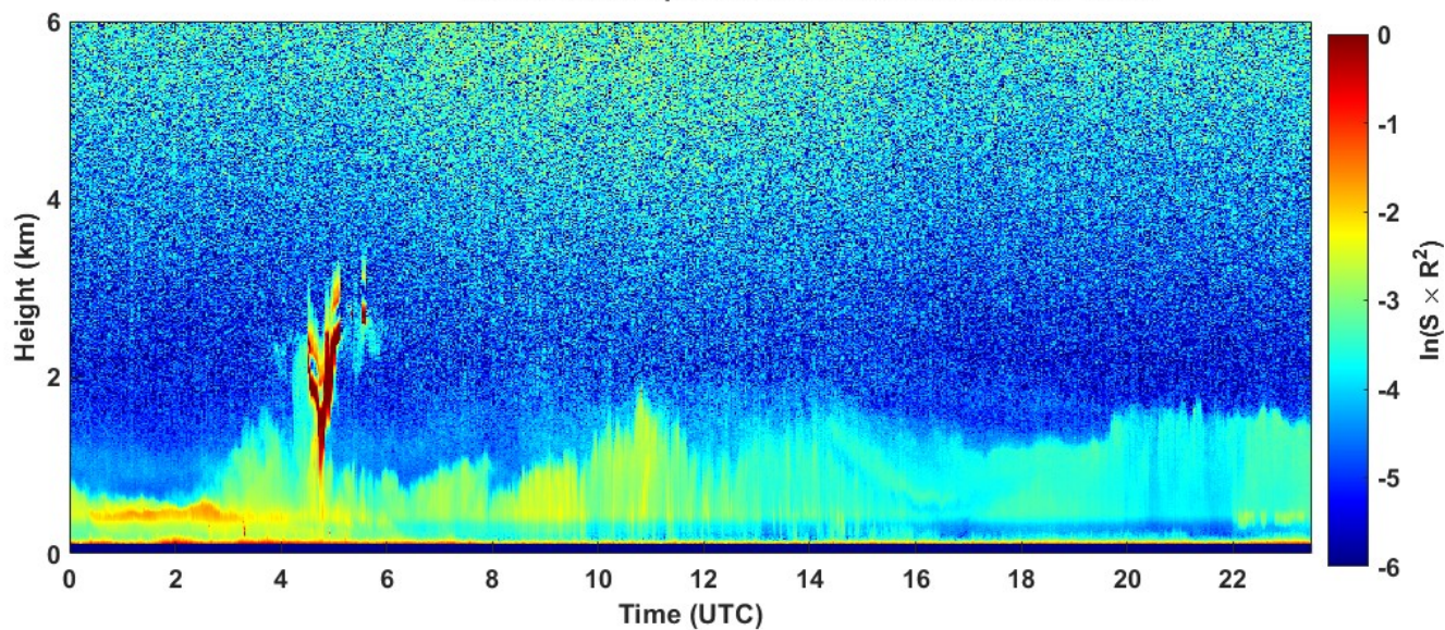
2022-01-18 RCS quick look CHM15k - ILVA LIDAR2 PARCHI
