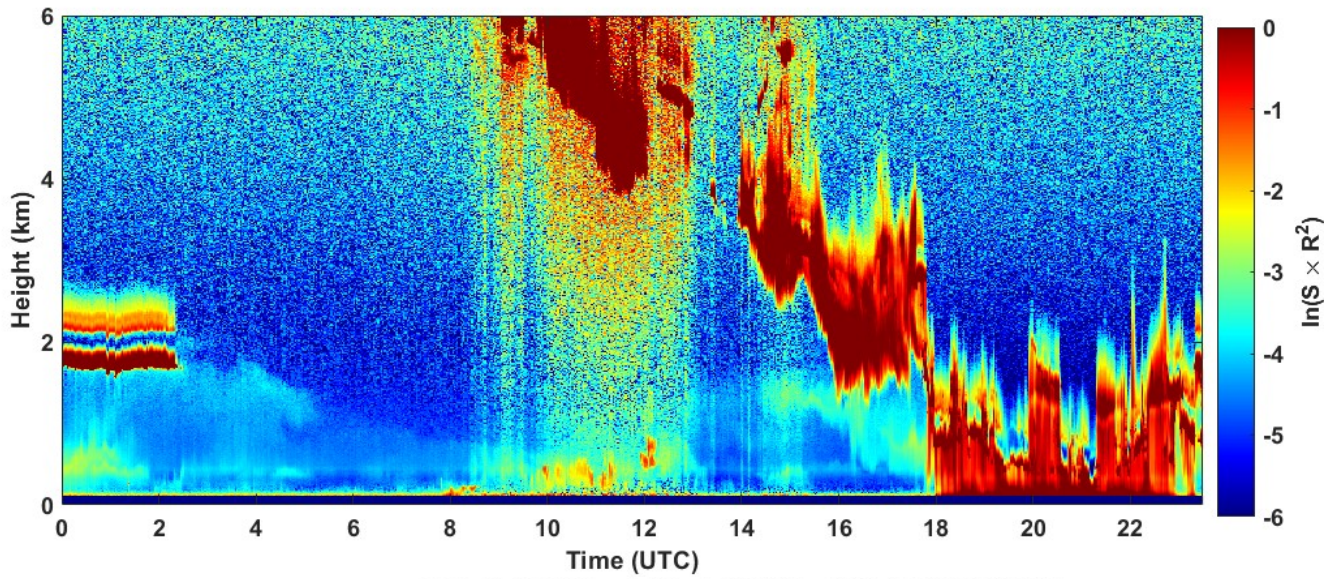
2022-01-10 RCS quick look CHM15k - ILVA LIDAR2 PARCHI
