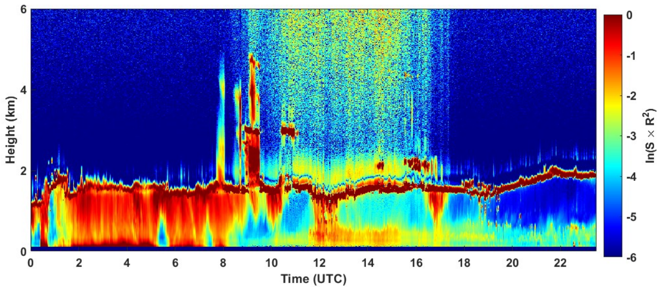
2022-01-08 RCS quick look CHM15k - ILVA LIDAR3 AGGLOMERATO
