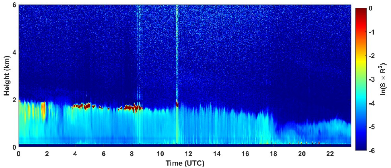
2022-01-26 RCS quick look CHM15k - ILVA LIDAR3 AGGLOMERATO
