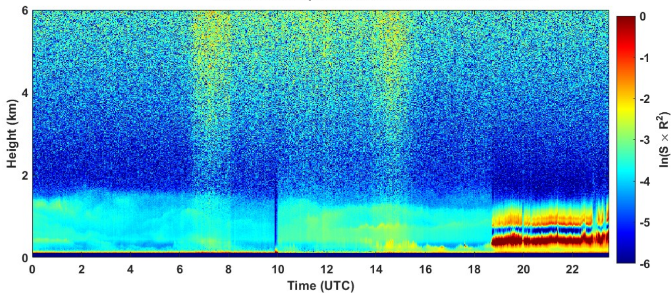
2022-01-04 RCS quick look CHM15k - ILVA LIDAR2 PARCHI
