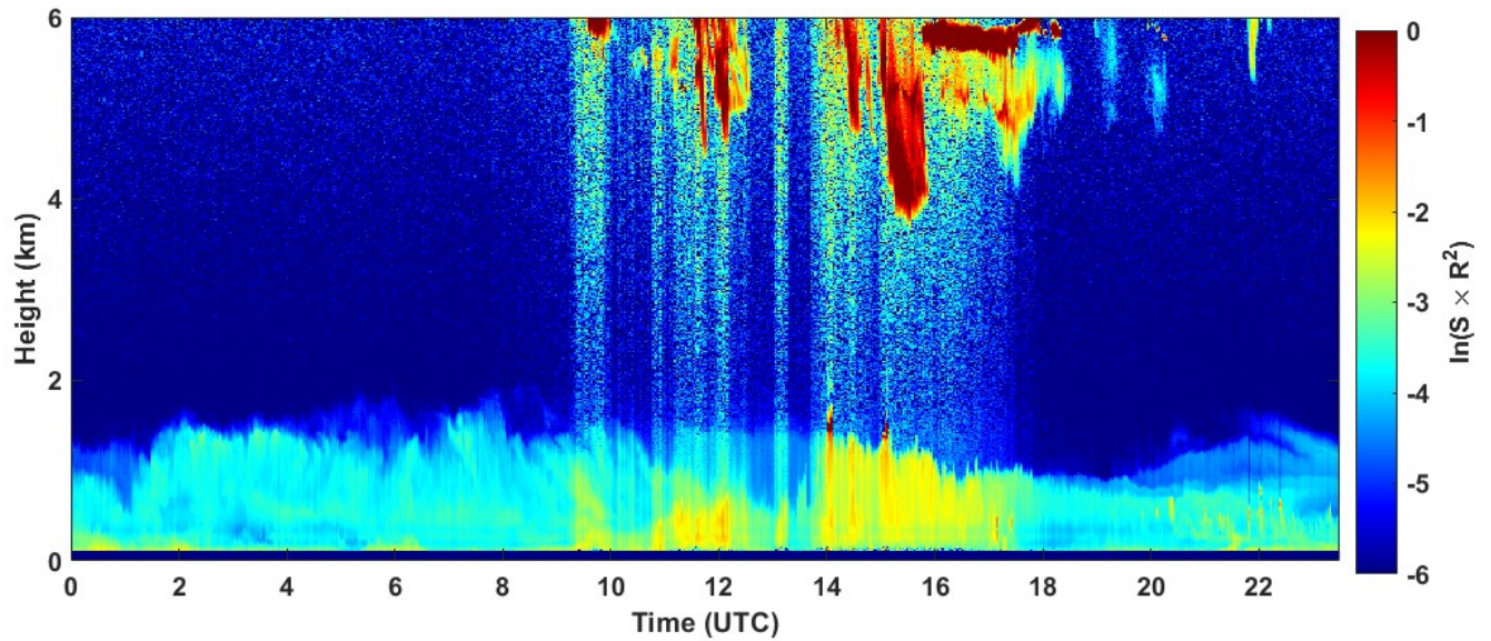
2022-01-28 RCS quick look CHM15k - ILVA LIDAR3 AGGLOMERATO
