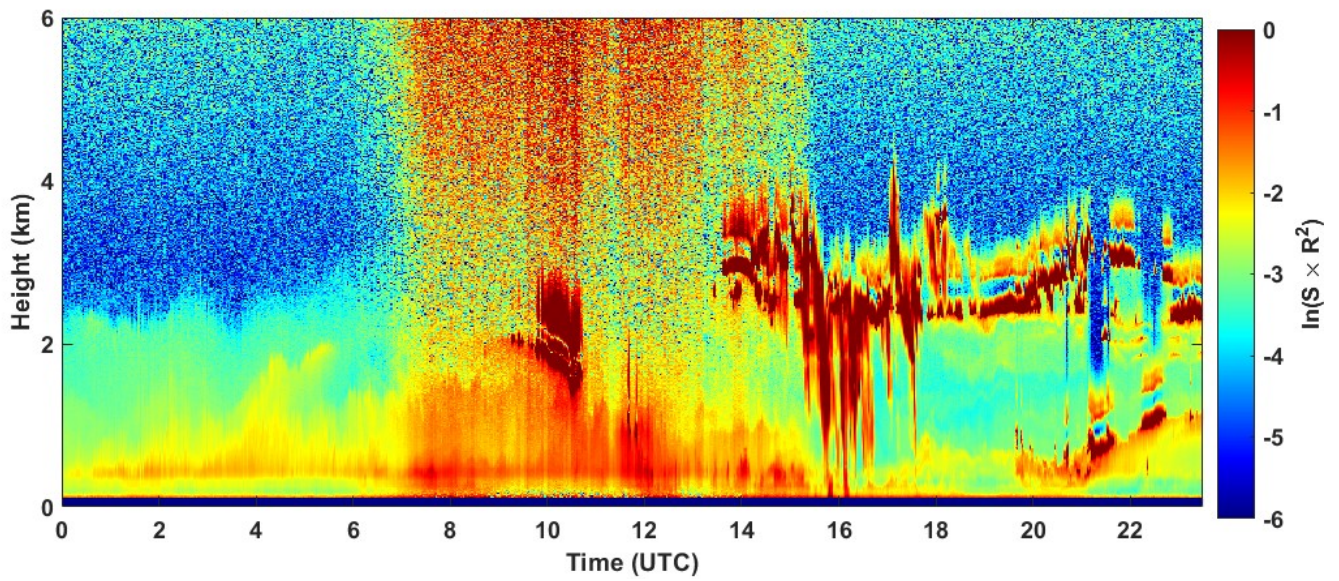
2022-01-06 RCS quick look CHM15k - ILVA LIDAR2 PARCHI
