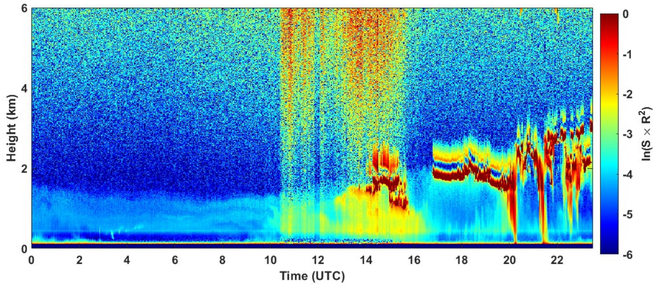
2022-01-31 RCS quick look CHM15k - ILVA LIDAR2 PARCHI
