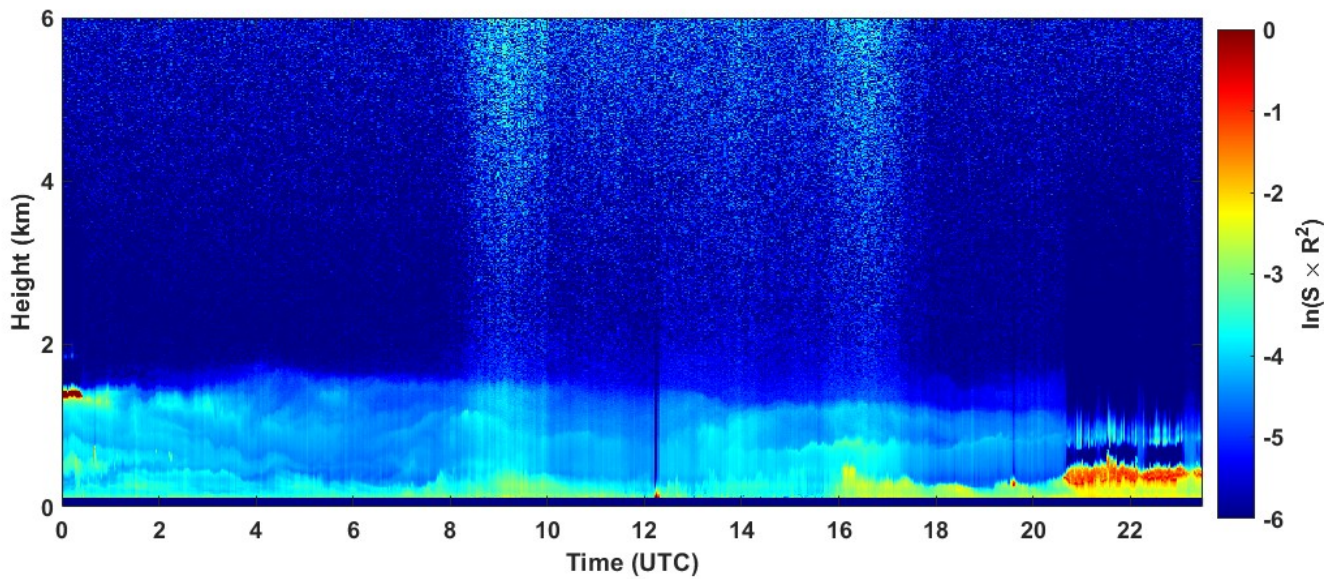
2022-01-04 RCS quick look CHM15k - ILVA LIDAR3 AGGLOMERATO
