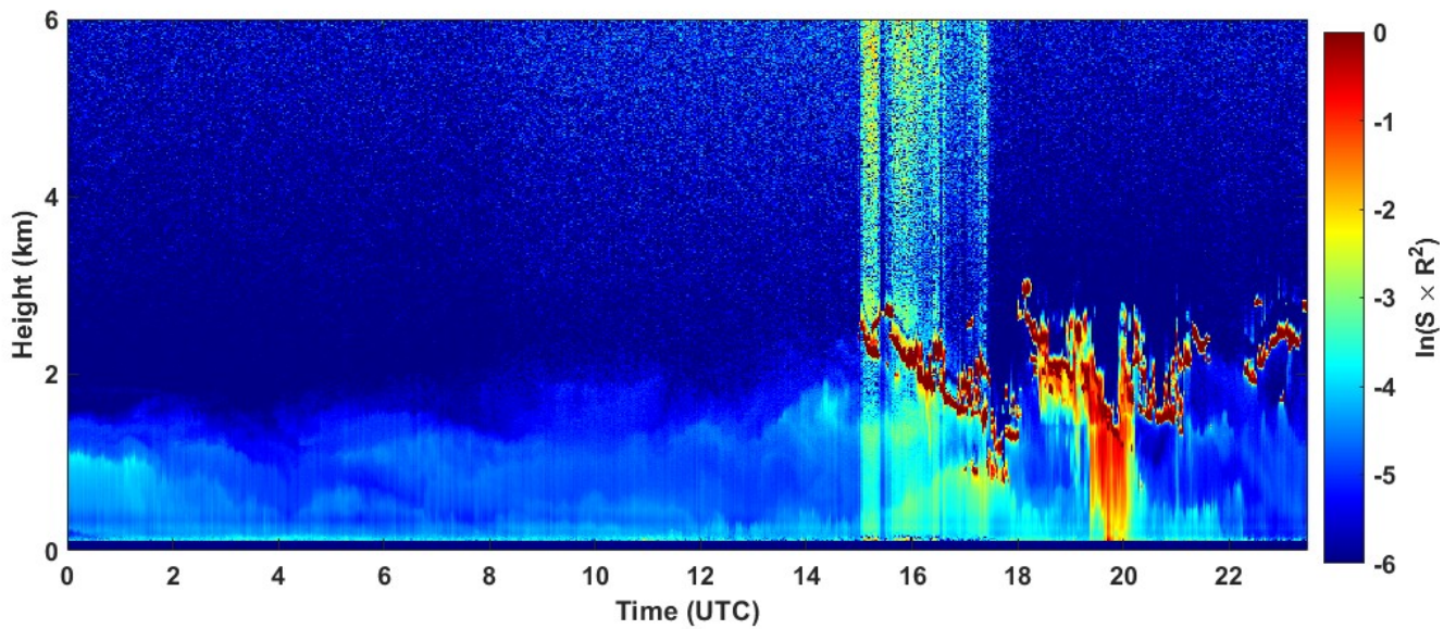
2022-01-20 RCS quick look CHM15k - ILVA LIDAR3 AGGLOMERATO
