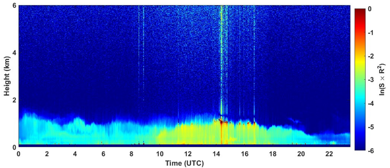
2022-01-14 RCS quick look CHM15k - ILVA LIDAR3 AGGLOMERATO
