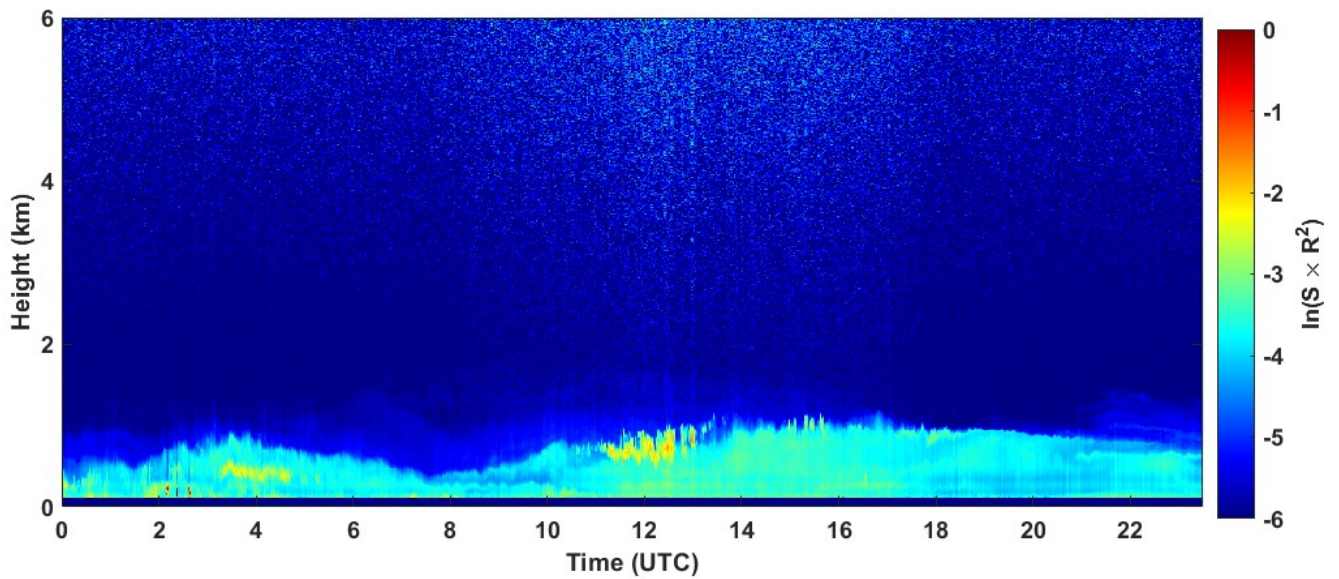
2022-01-16 RCS quick look CHM15k - ILVA LIDAR3 AGGLOMERATO
