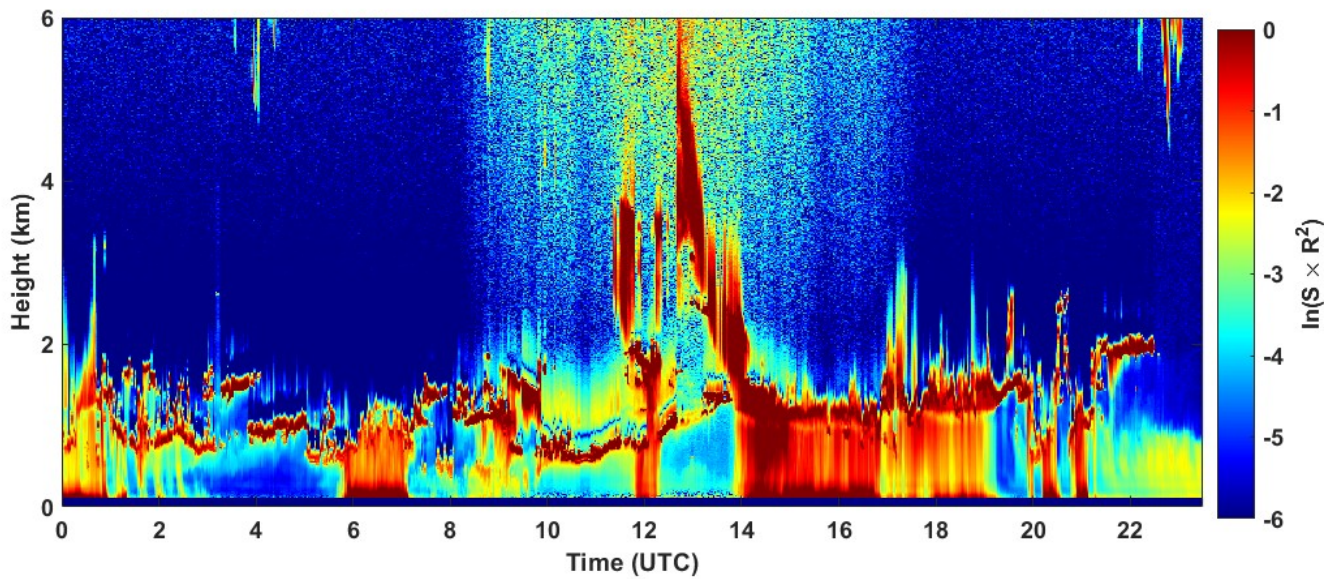
2022-01-10 RCS quick look CHM15k - ILVA LIDAR3 AGGLOMERATO
