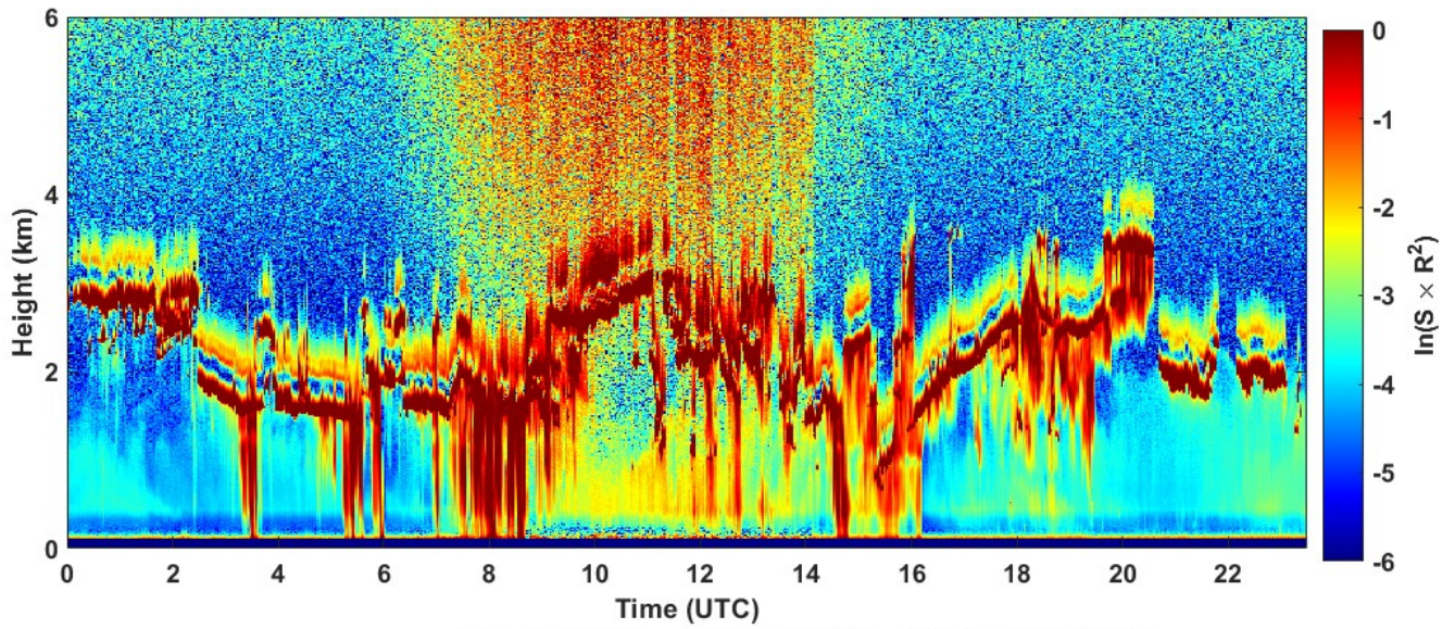
2022-01-22 RCS quick look CHM15k - ILVA LIDAR2 PARCHI
