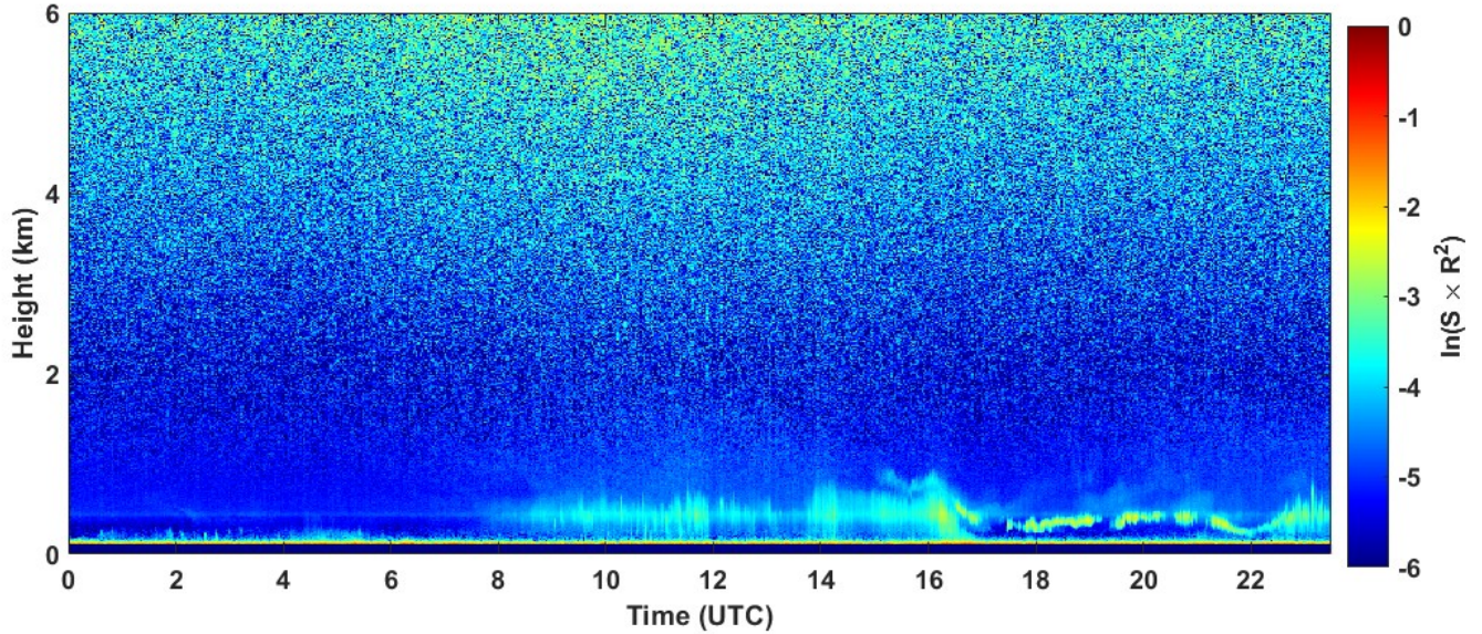
2022-01-02 RCS quick look CHM15k - ILVA LIDAR2 PARCHI
