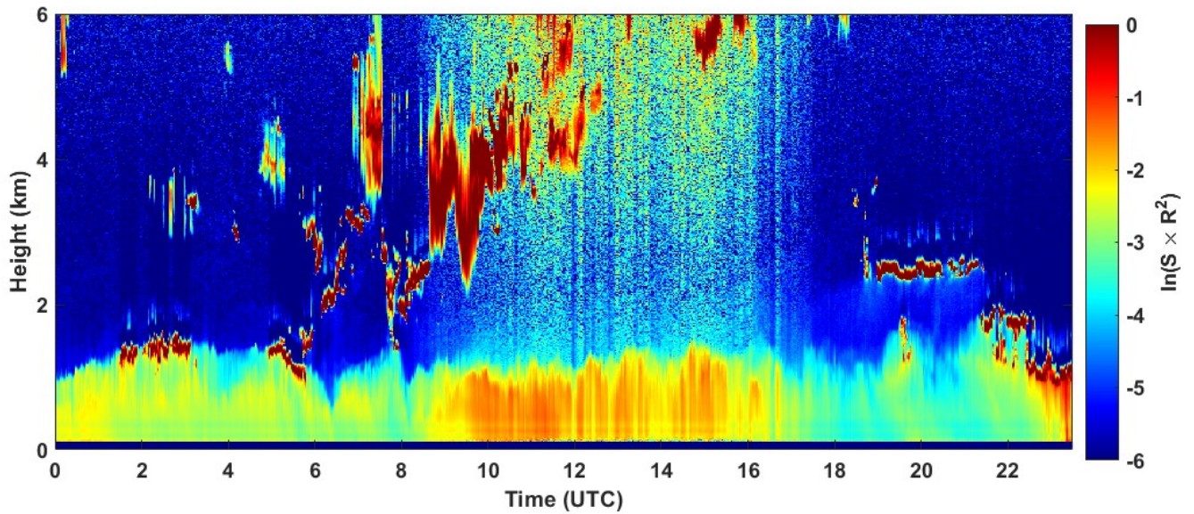
2022-01-12 RCS quick look CHM15k - ILVA LIDAR3 AGGLOMERATO
