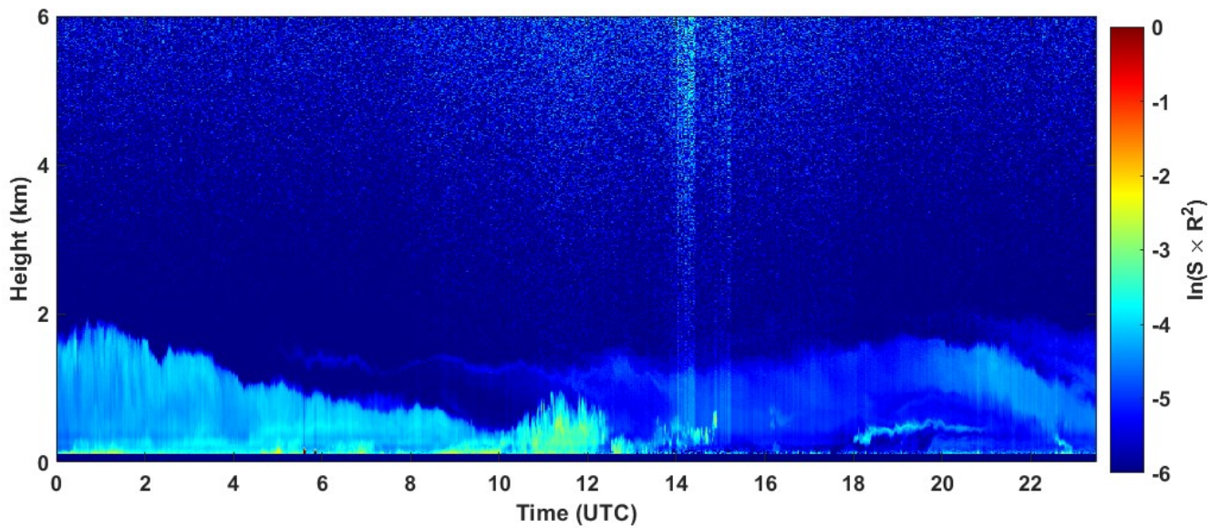
2022-01-30 RCS quick look CHM15k - ILVA LIDAR3 AGGLOMERATO
