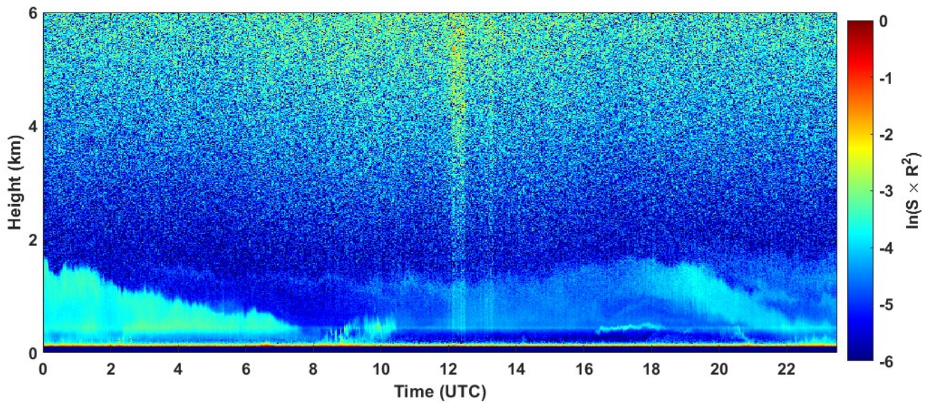
2022-01-30 RCS quick look CHM15k - ILVA LIDAR2 PARCHI
