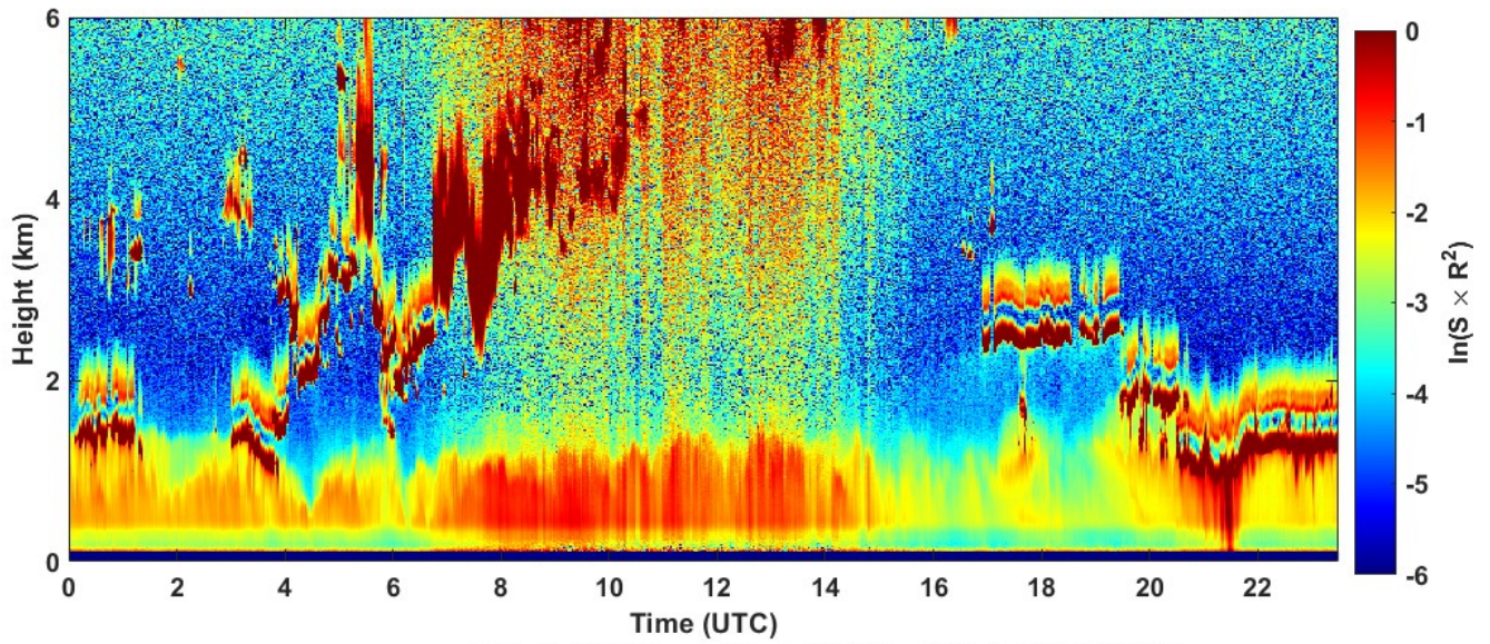
2022-01-12 RCS quick look CHM15k - ILVA LIDAR2 PARCHI
