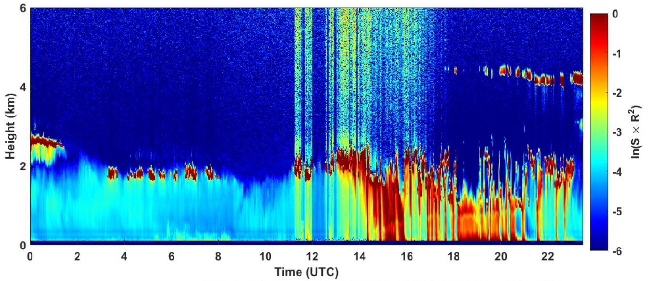
2022-01-24 RCS quick look CHM15k - ILVA LIDAR3 AGGLOMERATO
