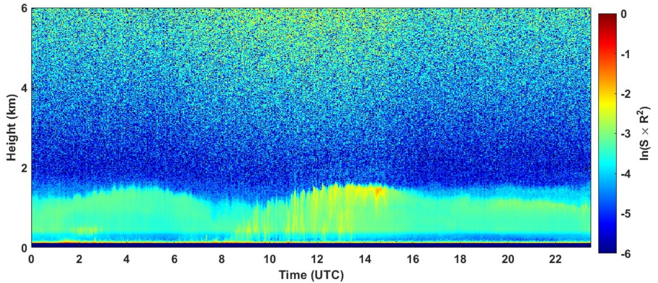
2022-01-20 RCS quick look CHM15k - ILVA LIDAR2 PARCHI
