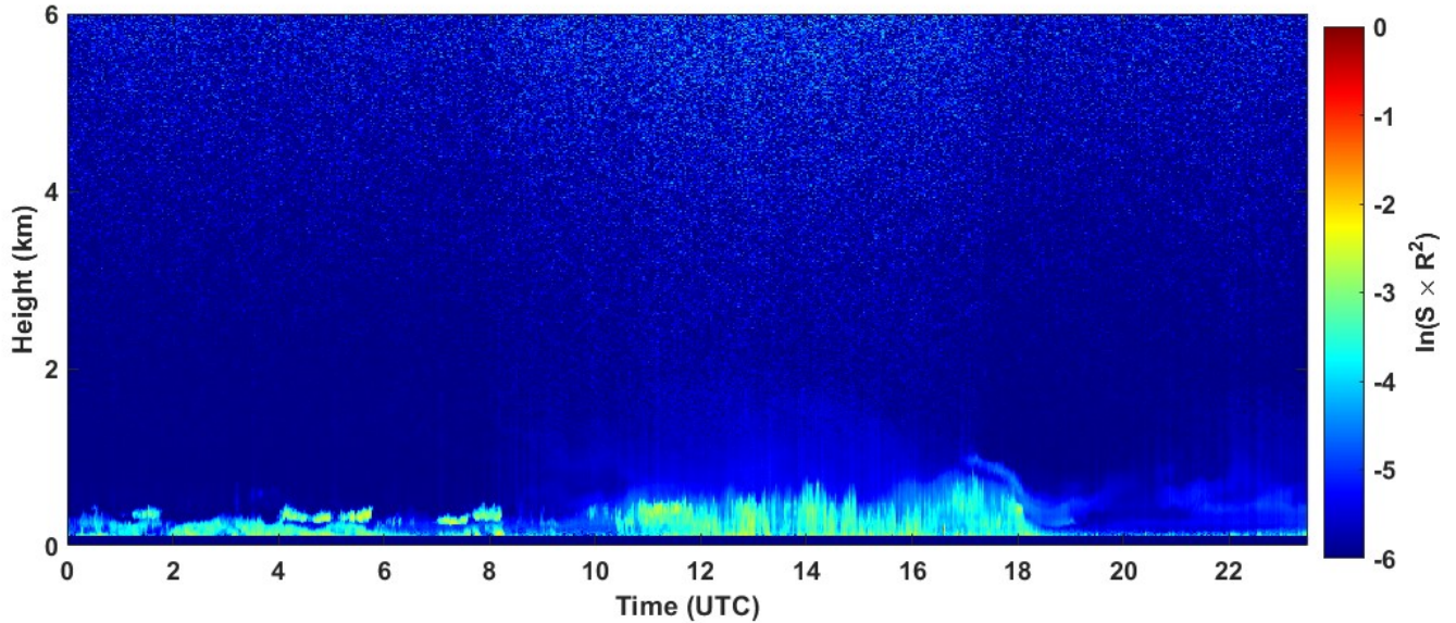
2022-01-02 RCS quick look CHM15k - ILVA LIDAR3 AGGLOMERATO
