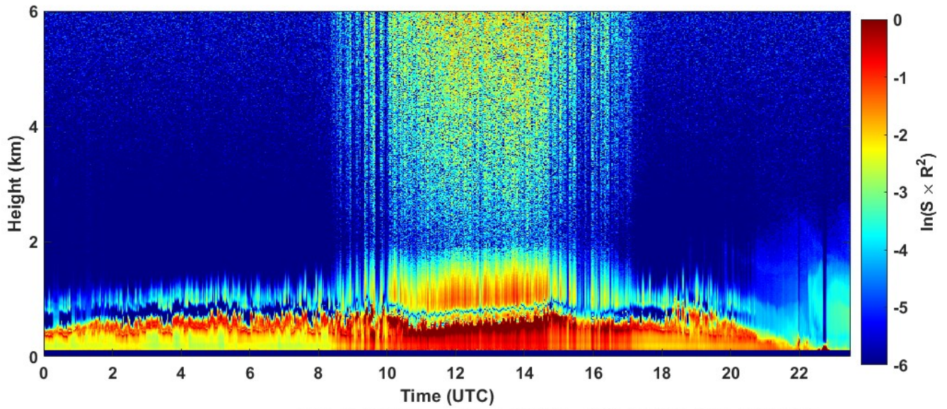
2022-01-06 RCS quick look CHM15k - ILVA LIDAR3 AGGLOMERATO
