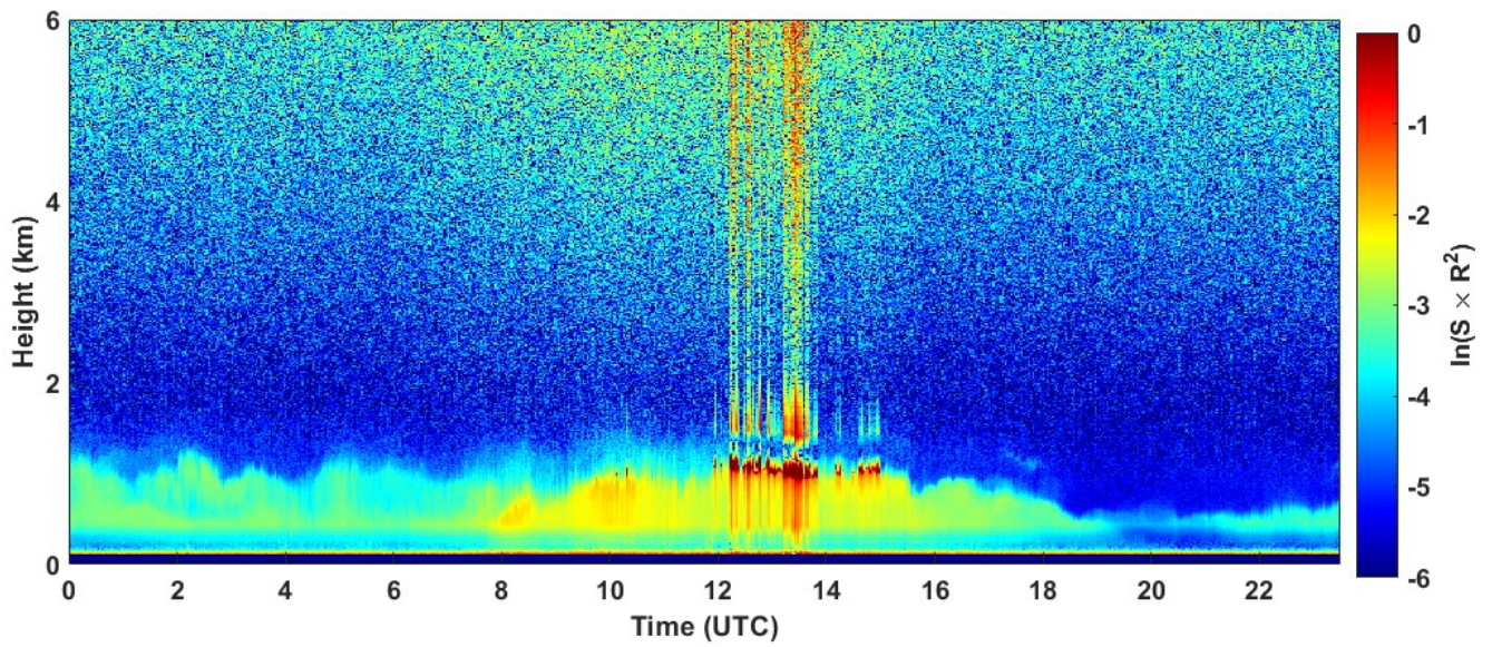
2022-01-14 RCS quick look CHM15k - ILVA LIDAR2 PARCHI
