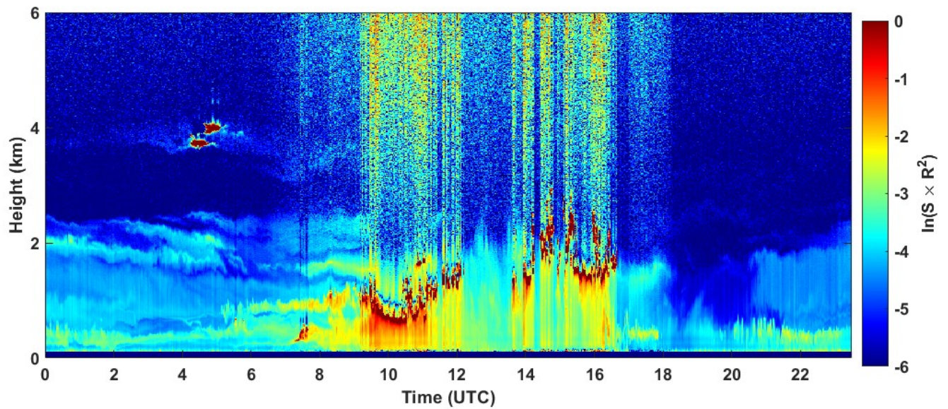
2021-09-30 RCS quick look CHM15k - ILVA LIDAR3 AGGLOMERATO
