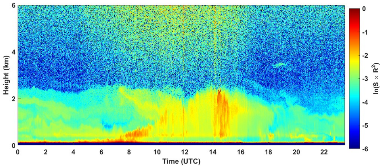
2021-09-14 RCS quick look CHM15k - ILVA LIDAR2 PARCHI
