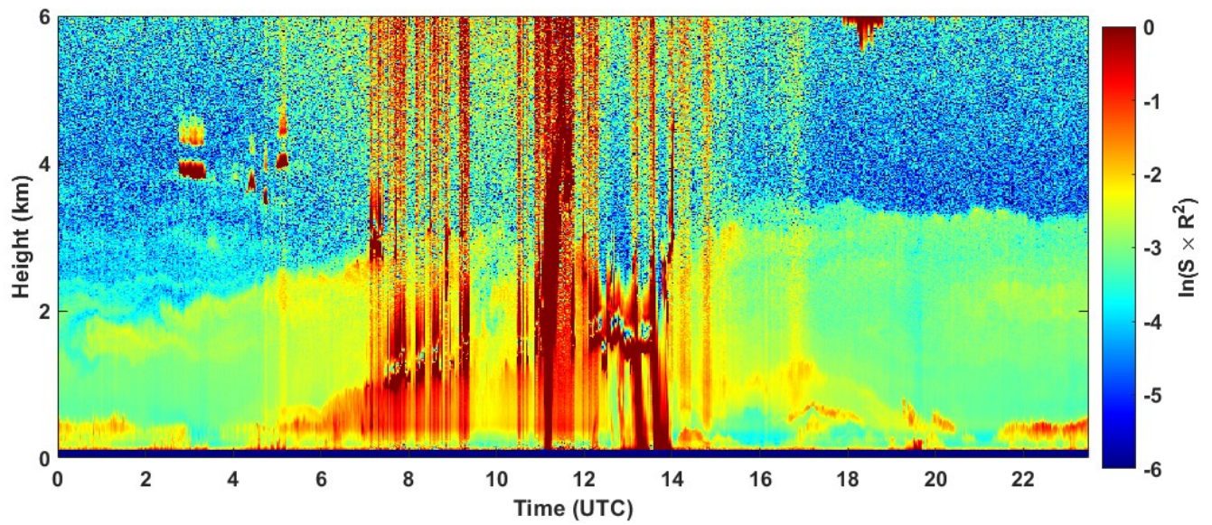
2021-09-06 RCS quick look CHM15k - ILVA LIDAR2 PARCHI
