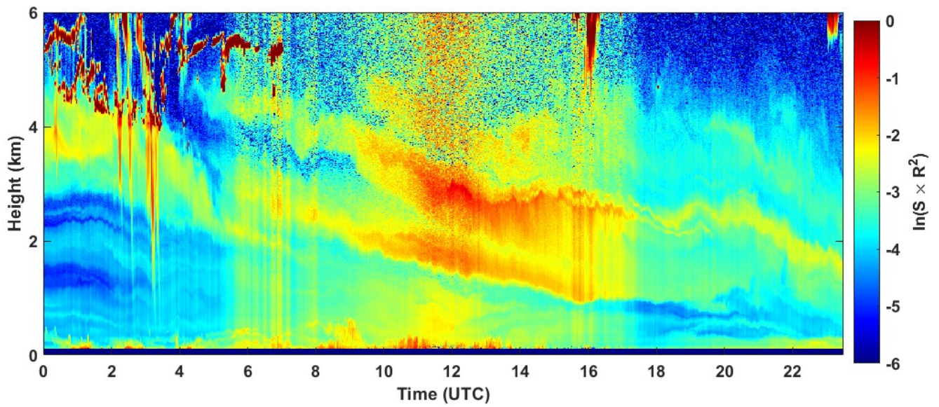
2021-09-16 RCS quick look CHM15k - ILVA LIDAR3 AGGLOMERATO
