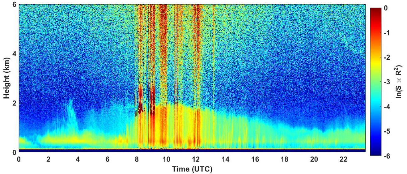
2021-09-02 RCS quick look CHM15k - ILVA LIDAR2 PARCHI
