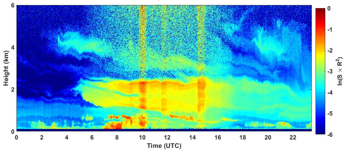
2021-09-26 RCS quick look CHM15k - ILVA LIDAR3 AGGLOMERATO
