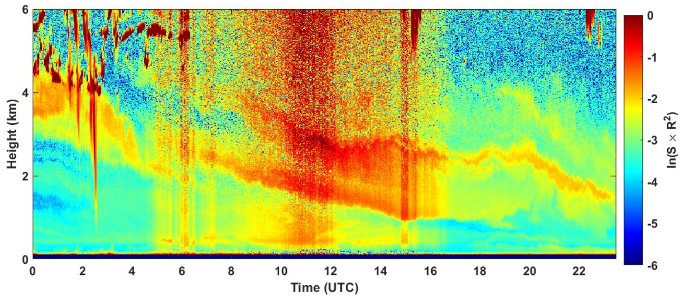
2021-09-16 RCS quick look CHM15k - ILVA LIDAR2 PARCHI
