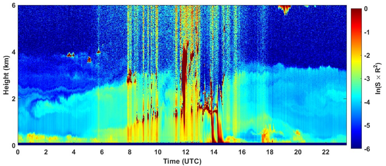
2021-09-06 RCS quick look CHM15k - ILVA LIDAR3 AGGLOMERATO
