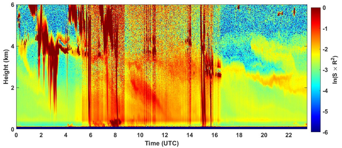
2021-09-18 RCS quick look CHM15k - ILVA LIDAR2 PARCHI
