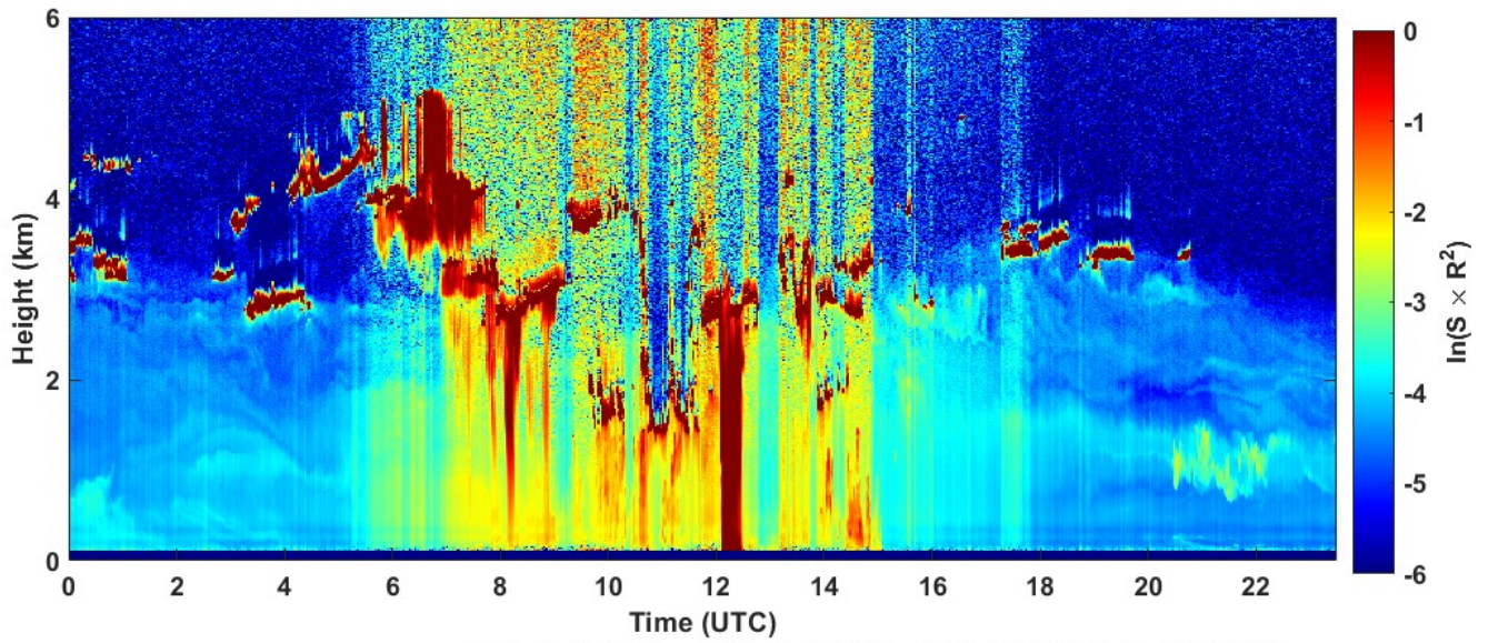
2021-09-10 RCS quick look CHM15k - ILVA LIDAR3 AGGLOMERATO
