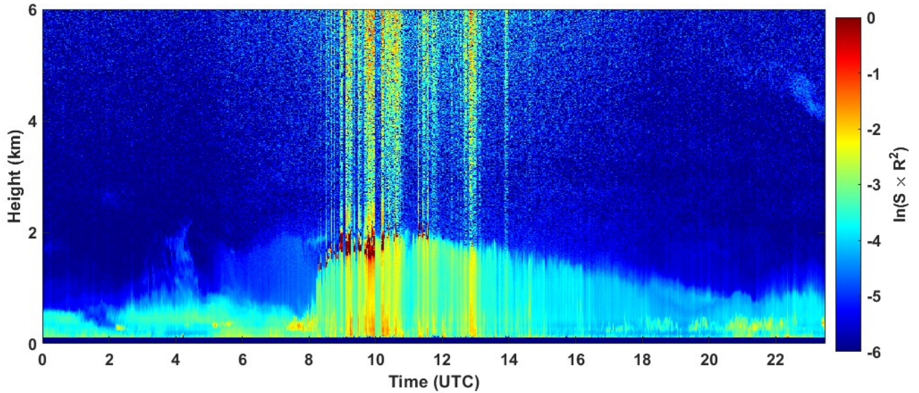
2021-09-02 RCS quick look CHM15k - ILVA LIDAR3 AGGLOMERATO
