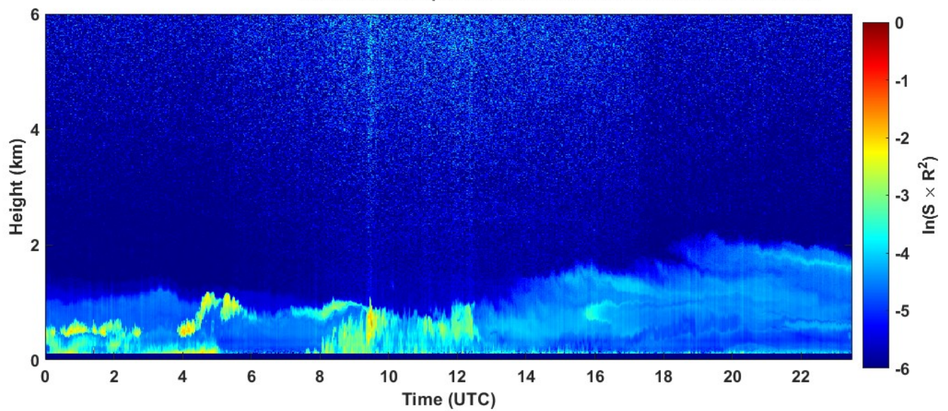
2021-09-24 RCS quick look CHM15k - ILVA LIDAR3 AGGLOMERATO
