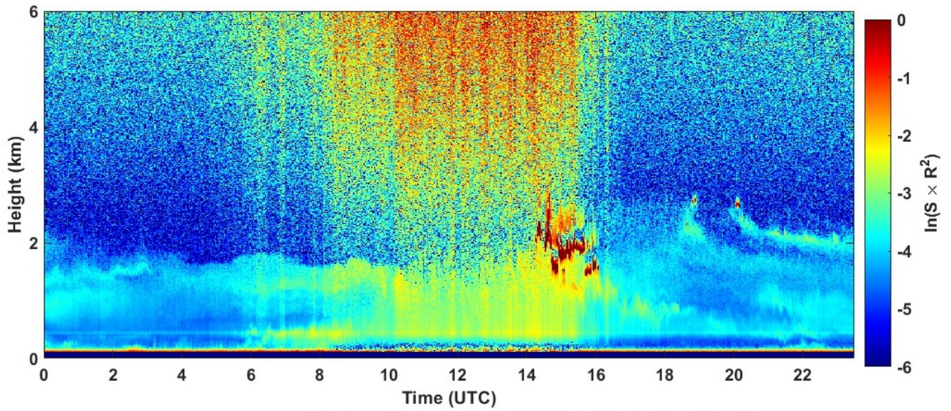
2021-09-30 RCS quick look CHM15k - ILVA LIDAR2 PARCHI
