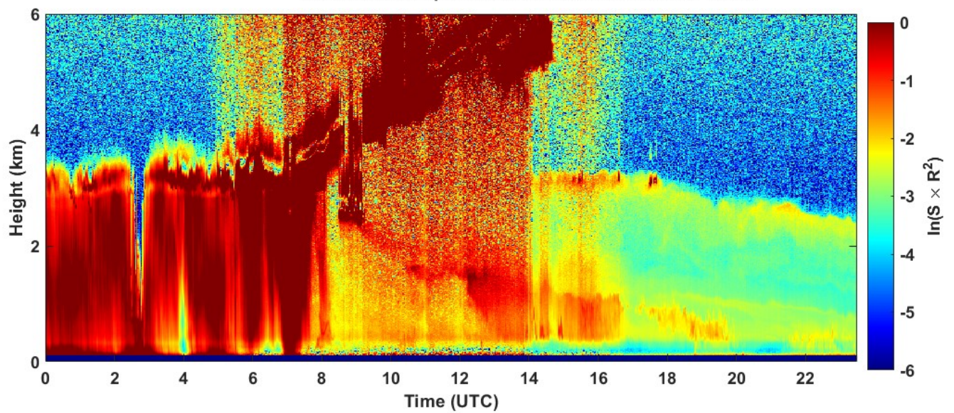
2021-09-12 RCS quick look CHM15k - ILVA LIDAR2 PARCHI
