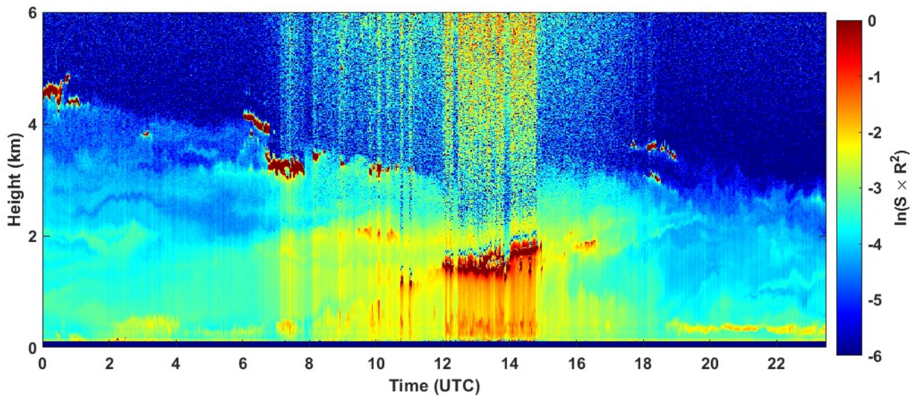
2021-09-28 RCS quick look CHM15k - ILVA LIDAR3 AGGLOMERATO
