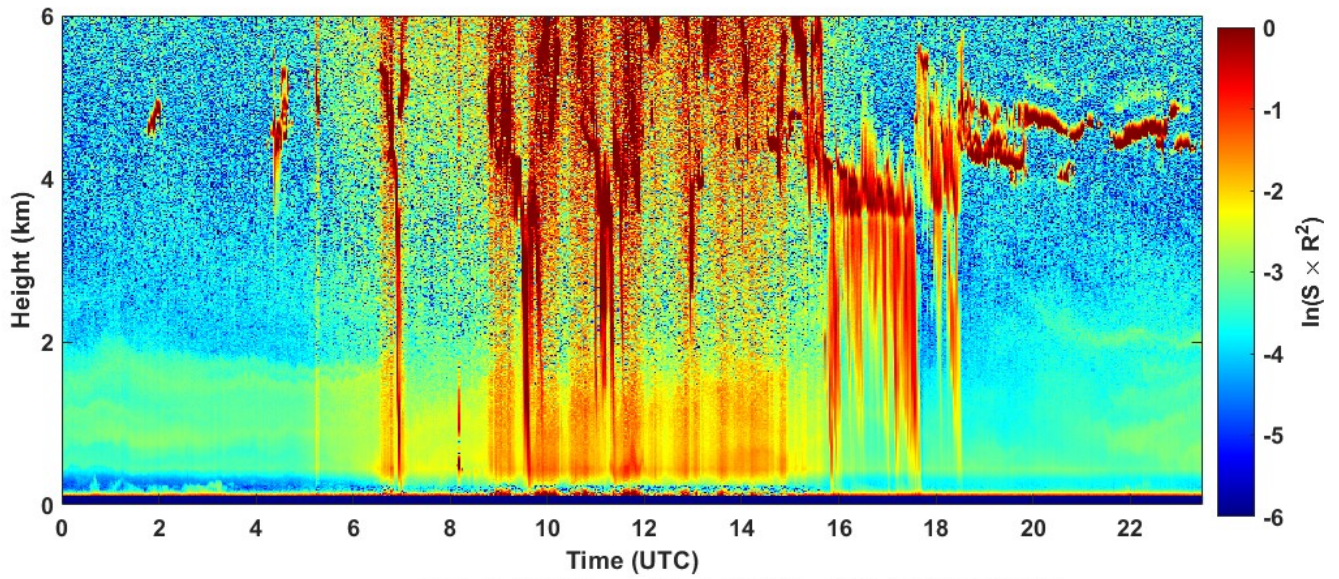
2021-09-28 RCS quick look CHM15k - ILVA LIDAR2 PARCHI
