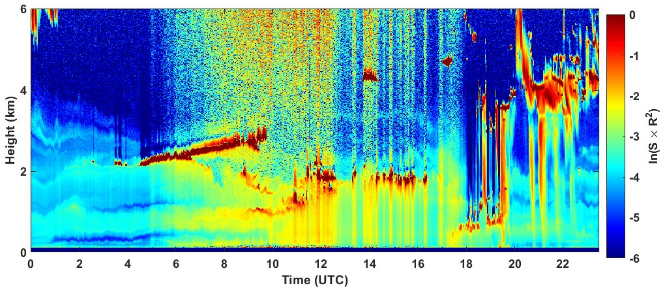
2021-09-04 RCS quick look CHM15k - ILVA LIDAR3 AGGLOMERATO
