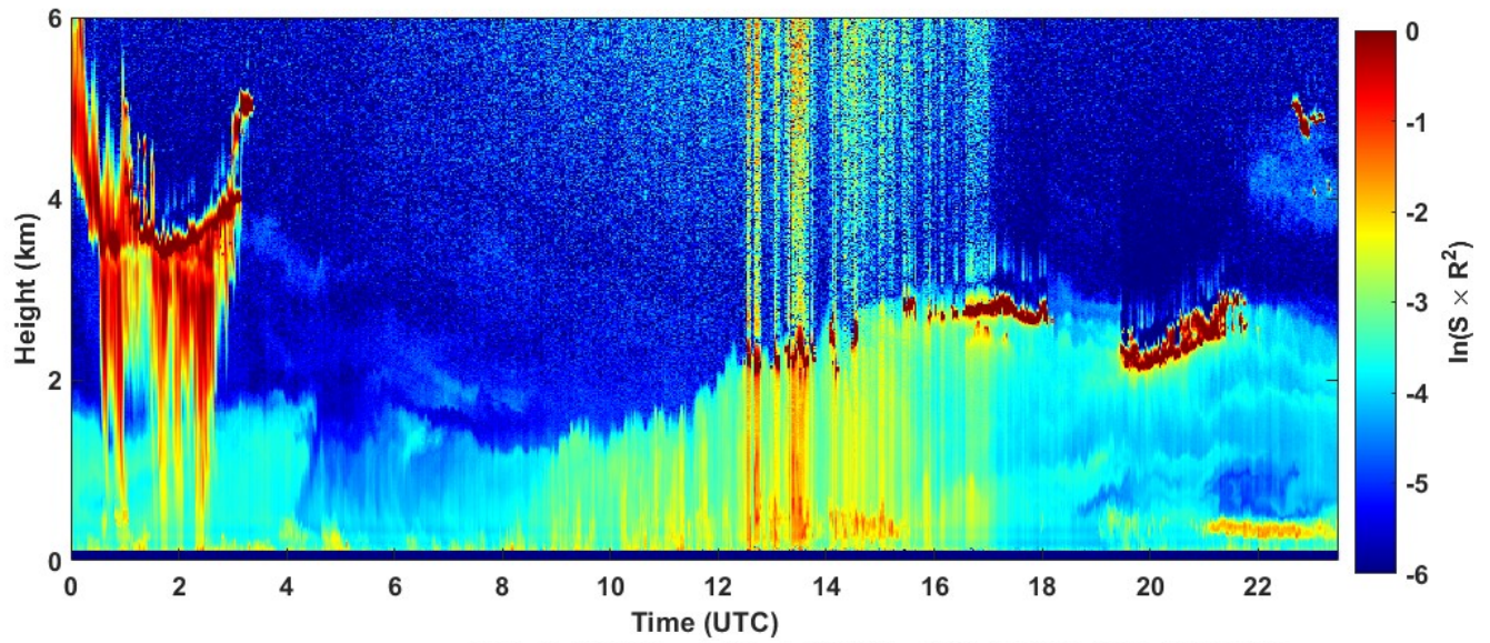
2021-09-22 RCS quick look CHM15k - ILVA LIDAR3 AGGLOMERATO
