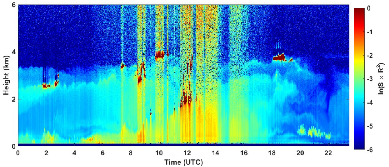
2021-09-08 RCS quick look CHM15k - ILVA LIDAR3 AGGLOMERATO
