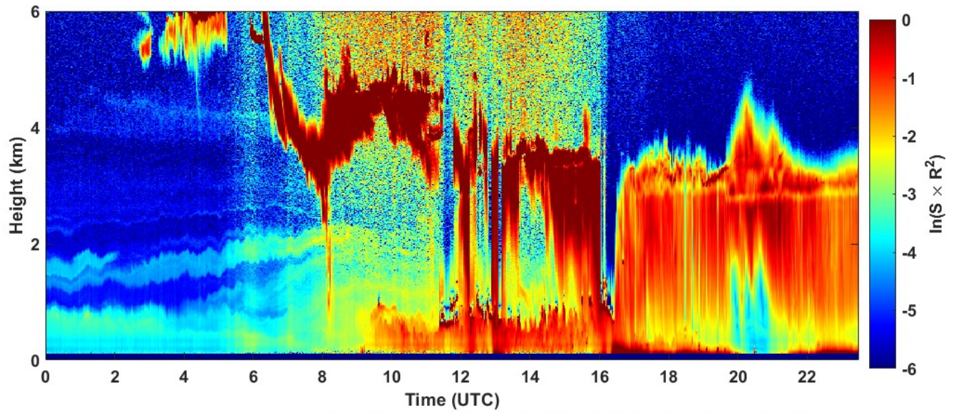
2021-09-12 RCS quick look CHM15k - ILVA LIDAR3 AGGLOMERATO
