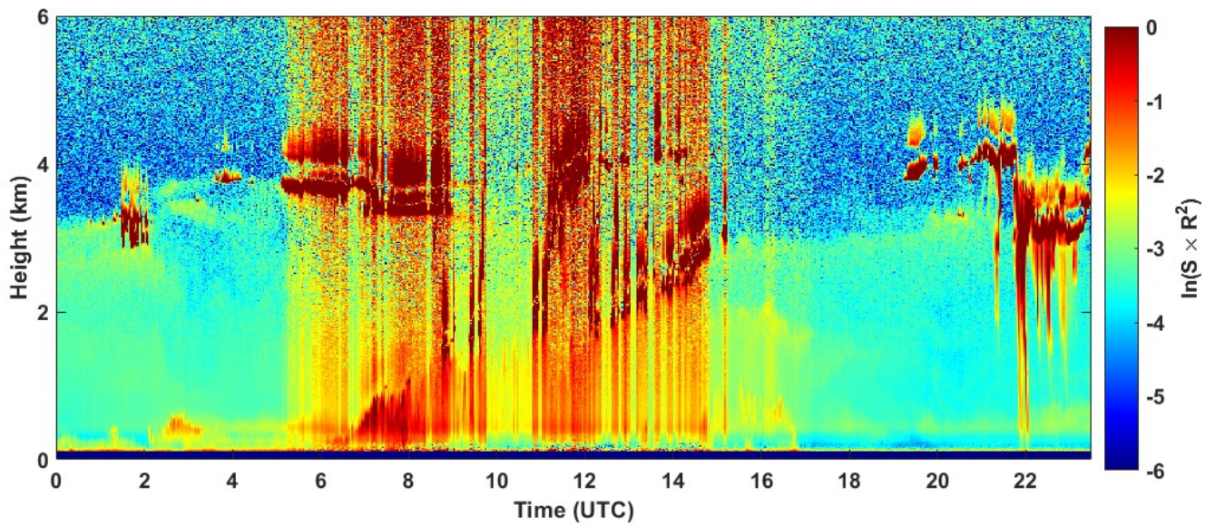
2021-09-08 RCS quick look CHM15k - ILVA LIDAR2 PARCHI
