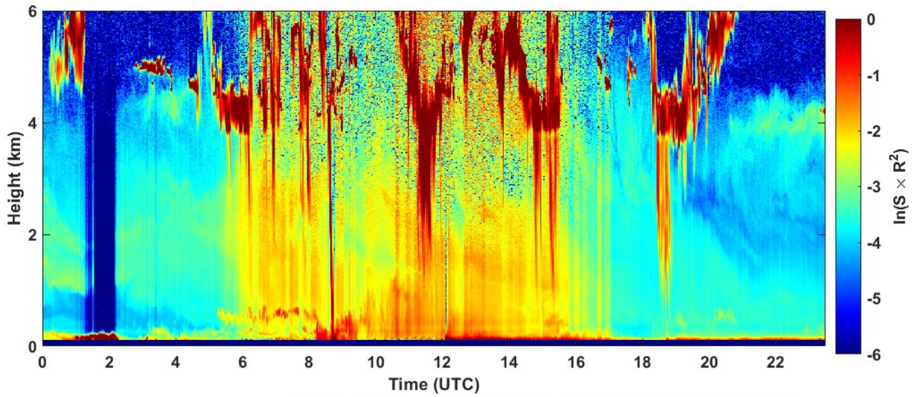
2021-09-18 RCS quick look CHM15k - ILVA LIDAR3 AGGLOMERATO
