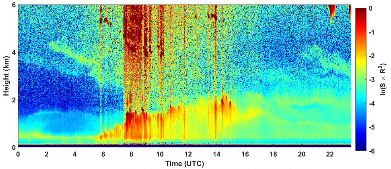
2021-09-04 RCS quick look CHM15k - ILVA LIDAR2 PARCHI
