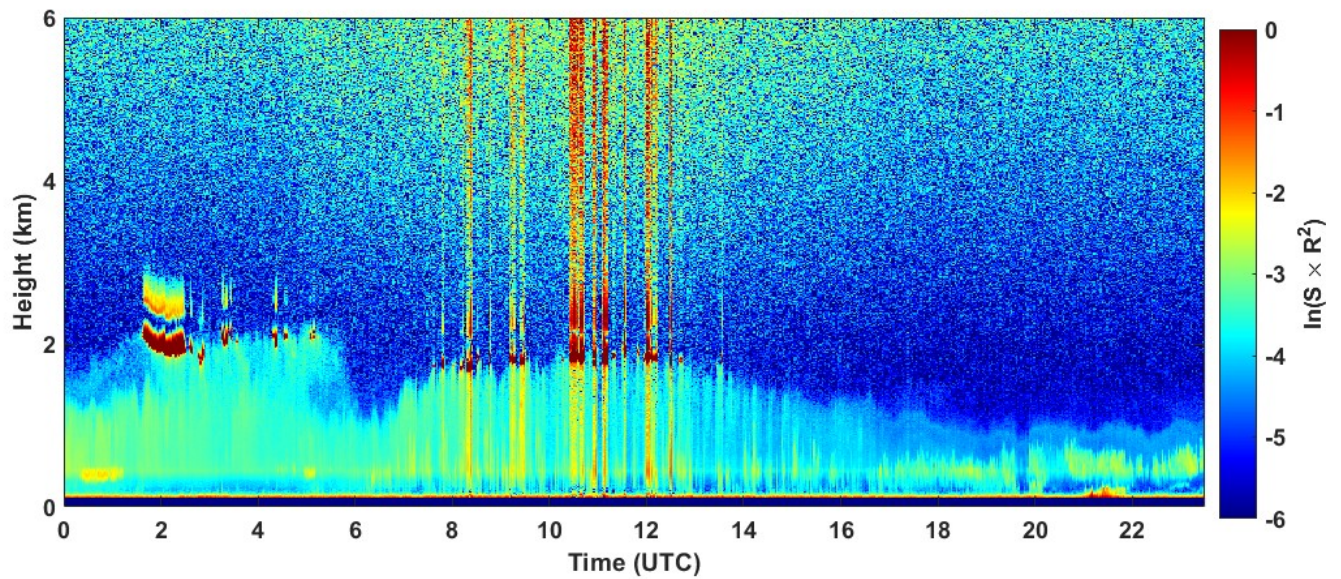
2021-09-24 RCS quick look CHM15k - ILVA LIDAR2 PARCHI
