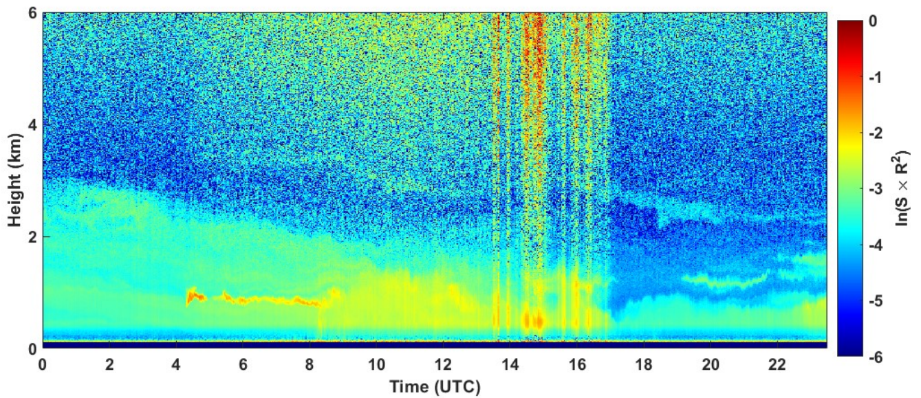
2021-09-10 RCS quick look CHM15k - ILVA LIDAR2 PARCHI
