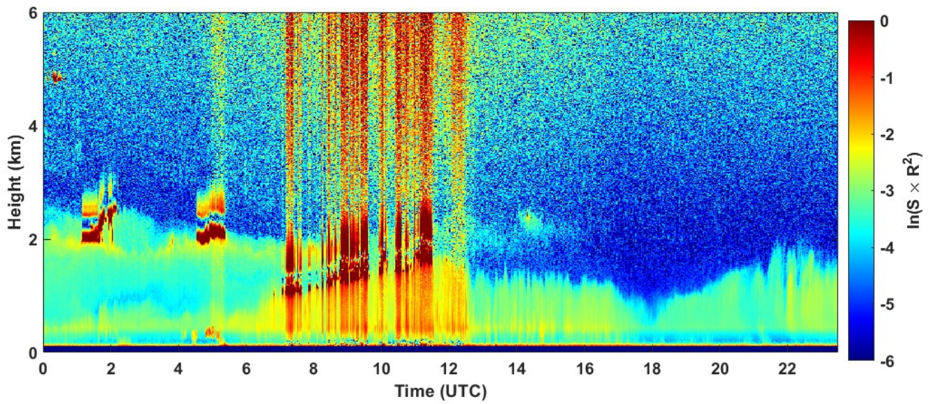
2021-09-22 RCS quick look CHM15k - ILVA LIDAR2 PARCHI
