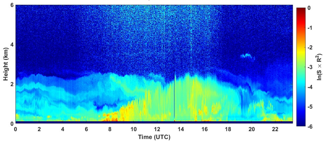
2021-09-14 RCS quick look CHM15k - ILVA LIDAR3 AGGLOMERATO
