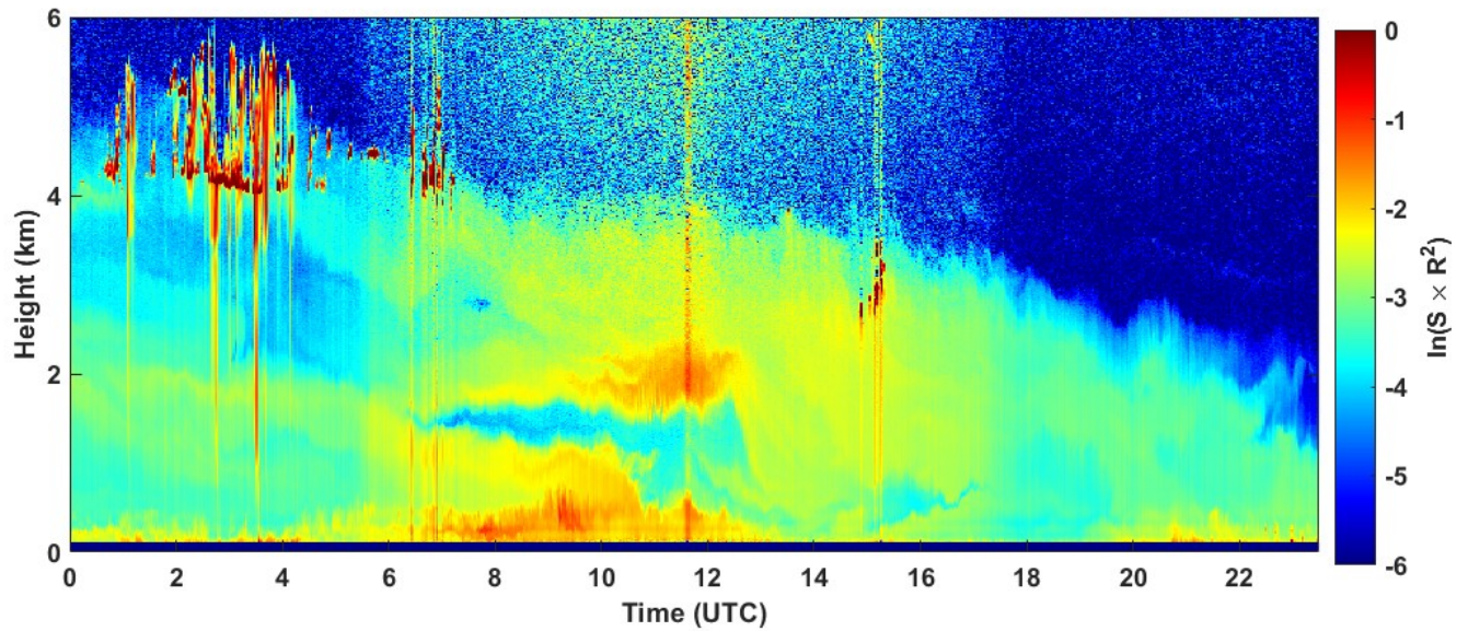
2021-09-20 RCS quick look CHM15k - ILVA LIDAR3 AGGLOMERATO
