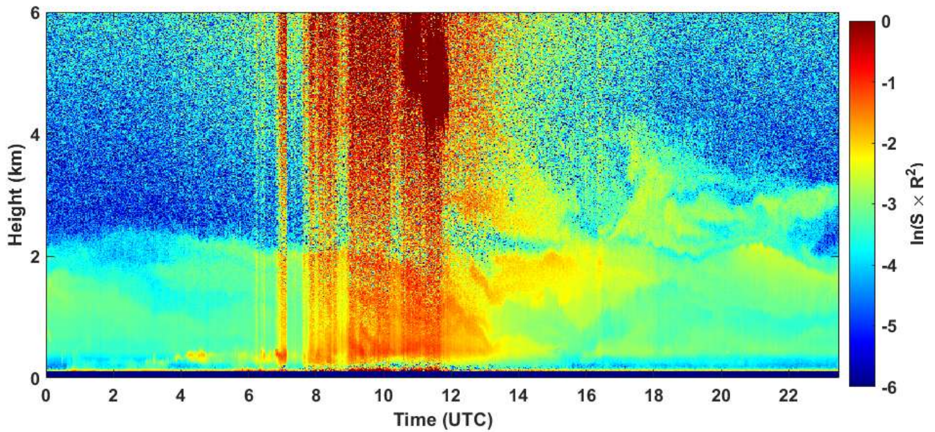
2021-05-28 RCS quick look CHM15k - ILVA LIDAR2 PARCHI
