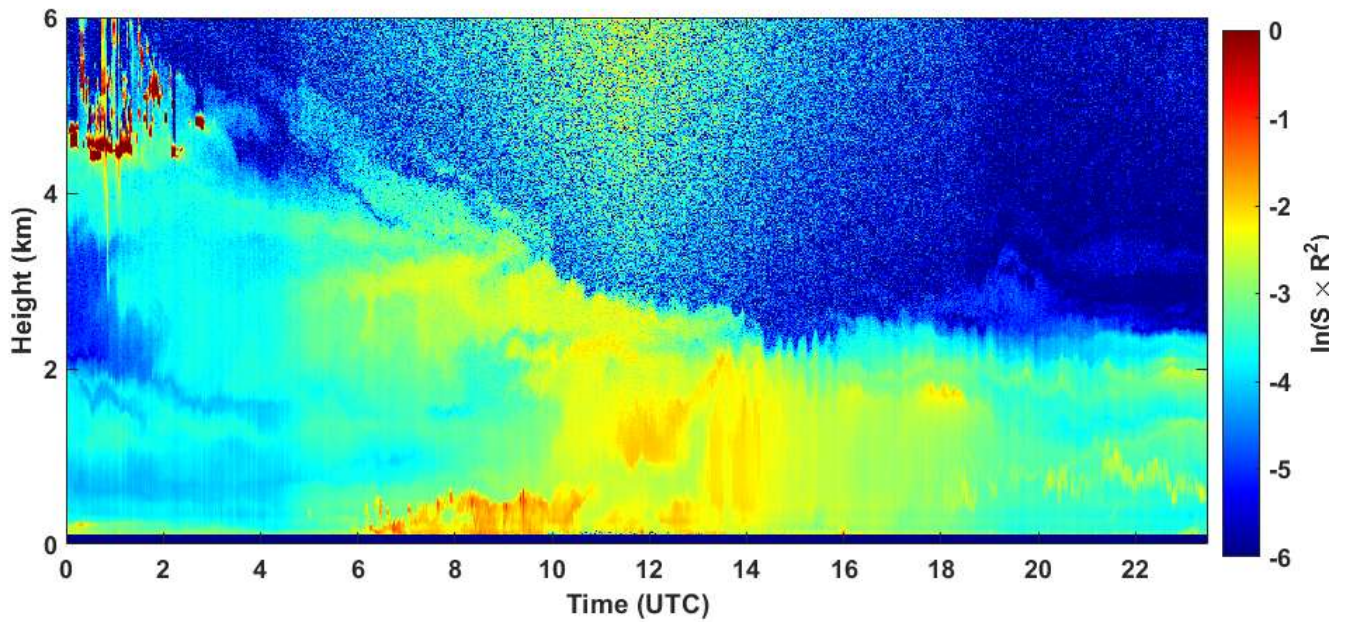
2021-05-26 RCS quick look CHM15k - ILVA LIDAR3 AGGLOMERATO
