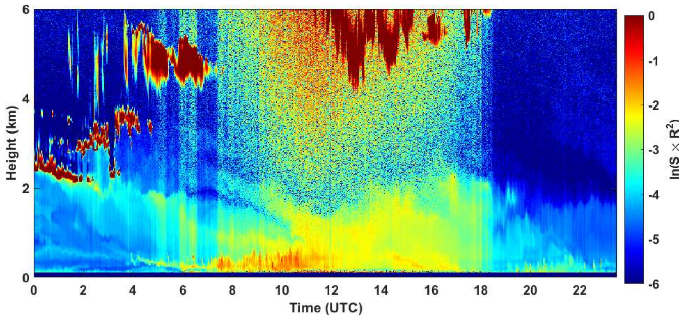
2021-05-06 RCS quick look CHM15k - ILVA LIDAR3 AGGLOMERATO
