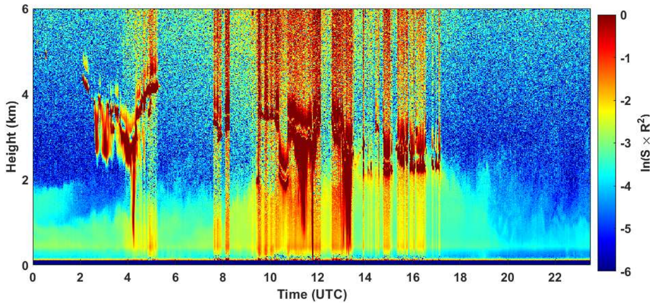
2021-05-14 RCS quick look CHM15k - ILVA LIDAR2 PARCHI
