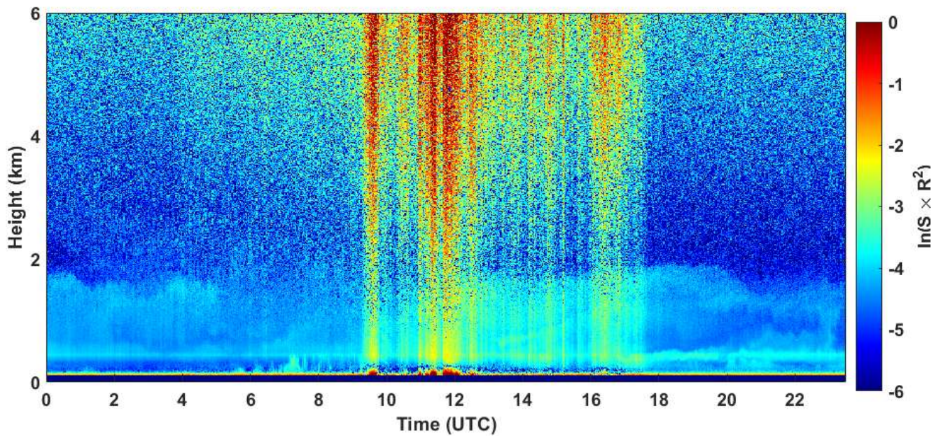
2021-05-06 RCS quick look CHM15k - ILVA LIDAR2 PARCHI
