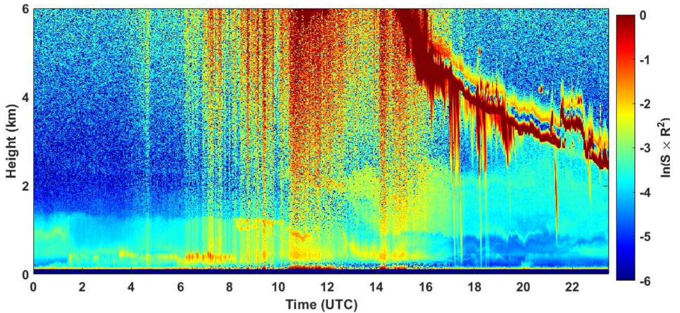
2021-05-04 RCS quick look CHM15k - ILVA LIDAR2 PARCHI
