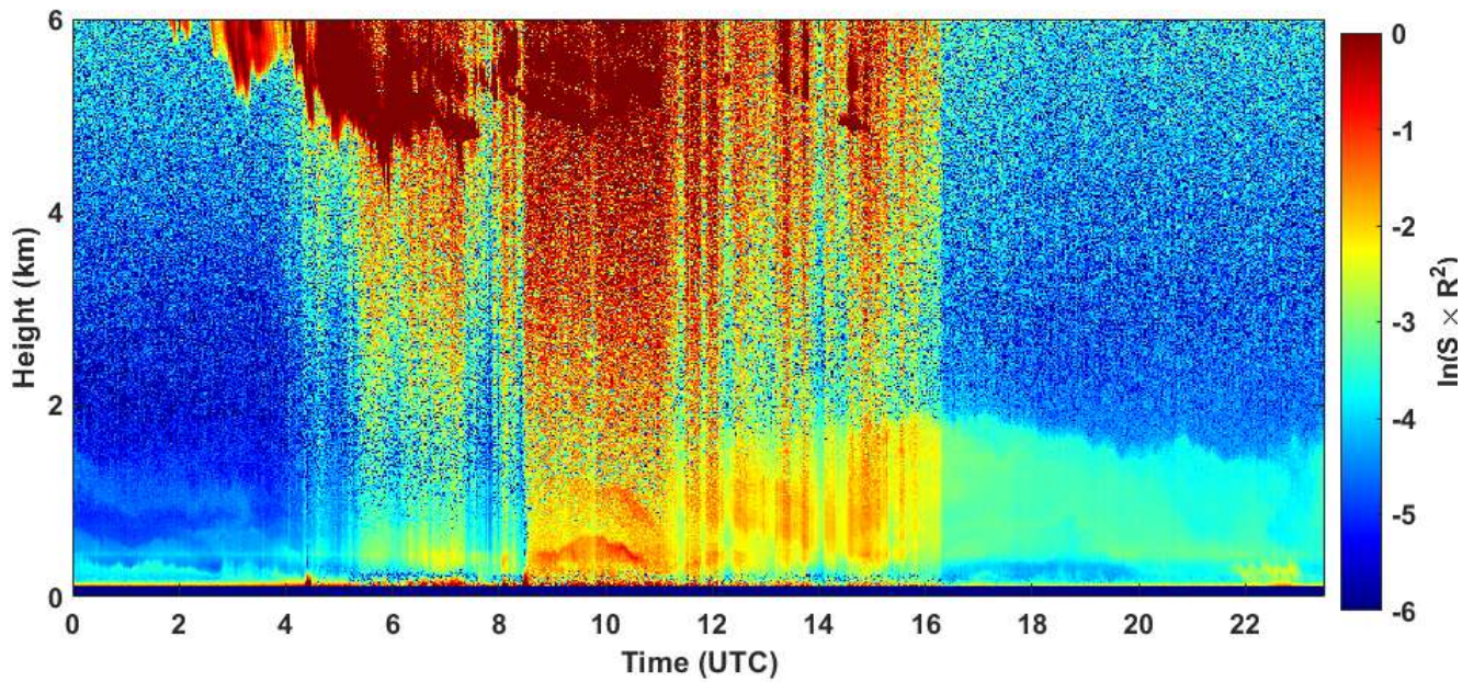
2021-05-08 RCS quick look CHM15k - ILVA LIDAR2 PARCHI
