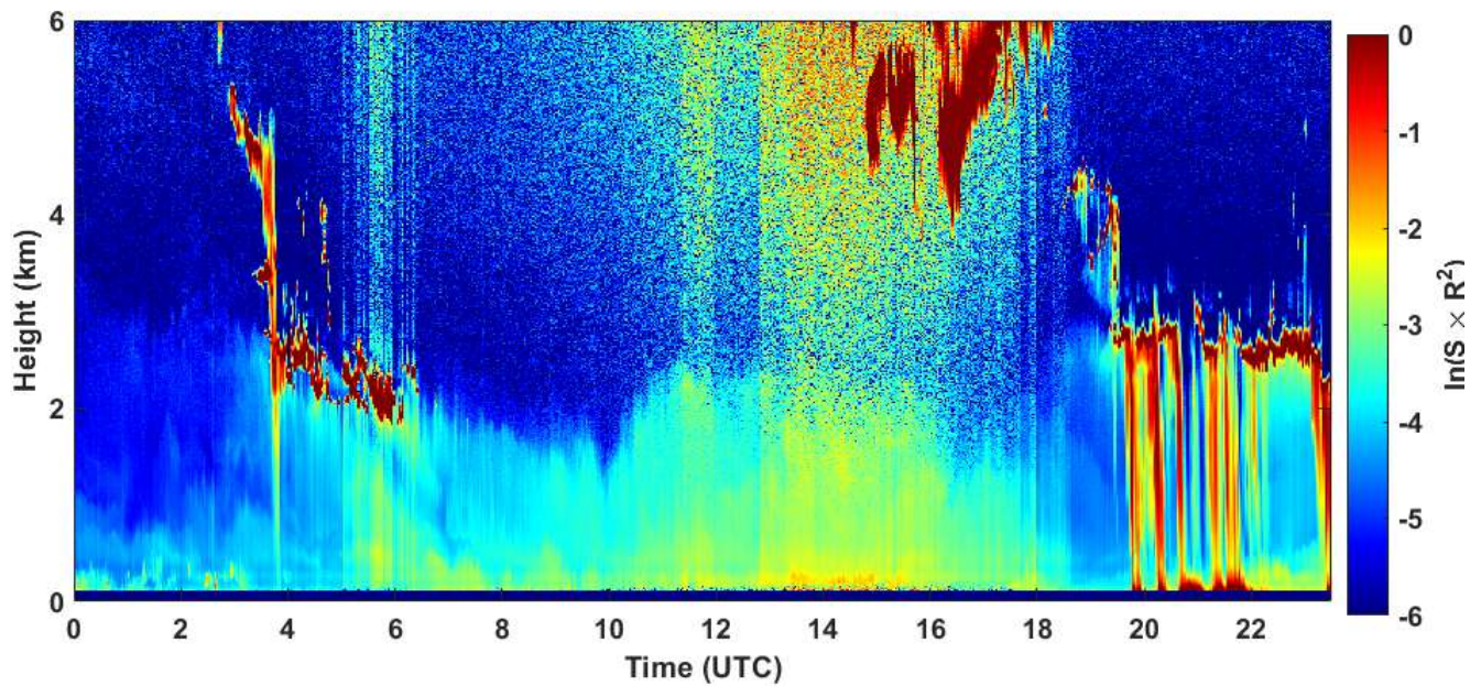
2021-05-14 RCS quick look CHM15k - ILVA LIDAR3 AGGLOMERATO
