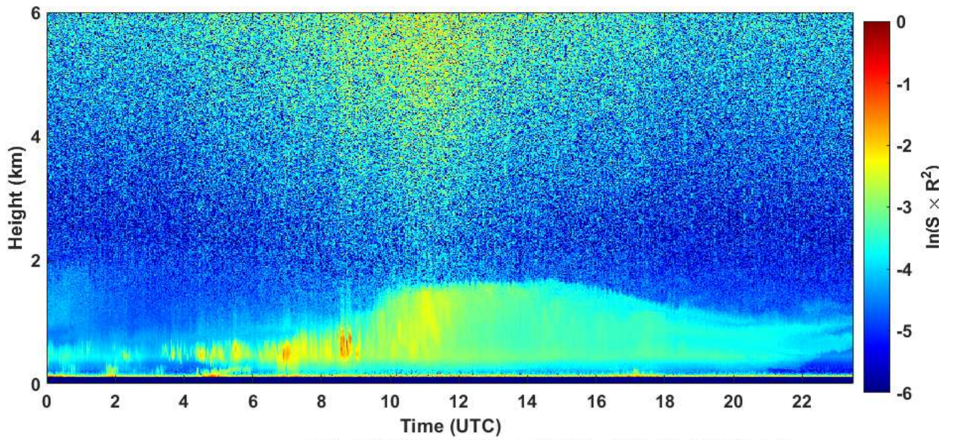
2021-05-10 RCS quick look CHM15k - ILVA LIDAR2 PARCHI
