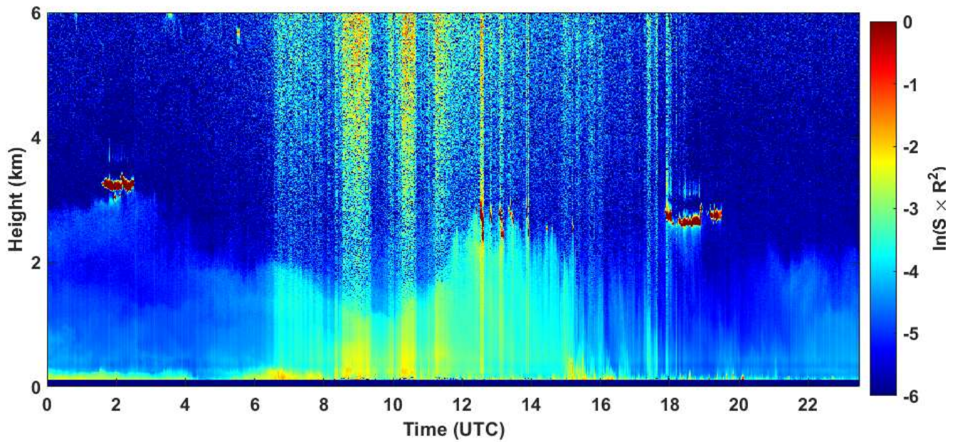
2021-05-18 RCS quick look CHM15k - ILVA LIDAR3 AGGLOMERATO
