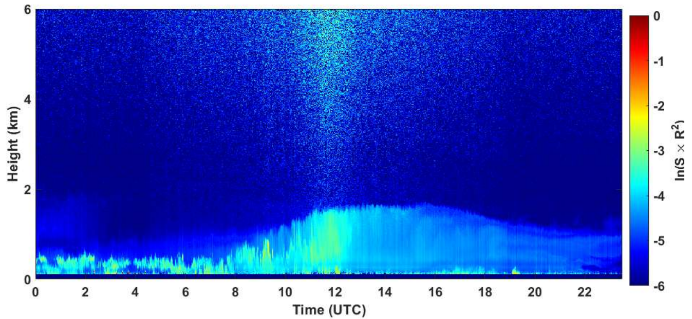
2021-05-10 RCS quick look CHM15k - ILVA LIDAR3 AGGLOMERATO
