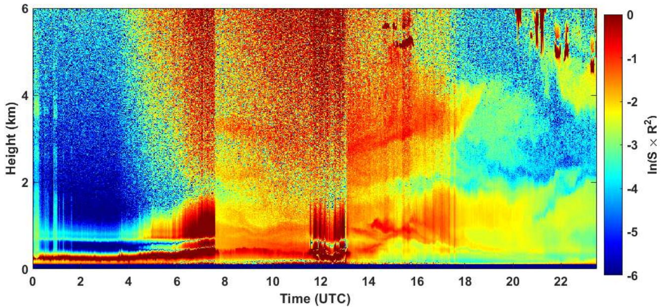
2021-05-24 RCS quick look CHM15k - ILVA LIDAR2 PARCHI
