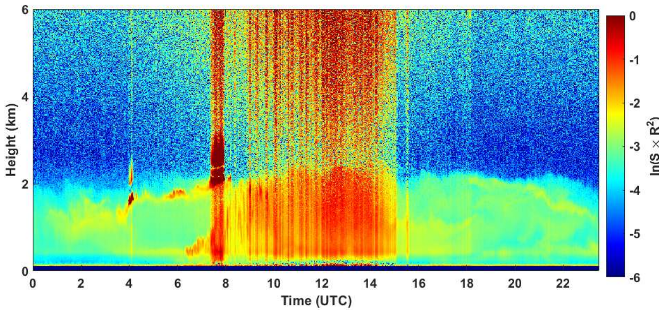
2021-05-18 RCS quick look CHM15k - ILVA LIDAR2 PARCHI
