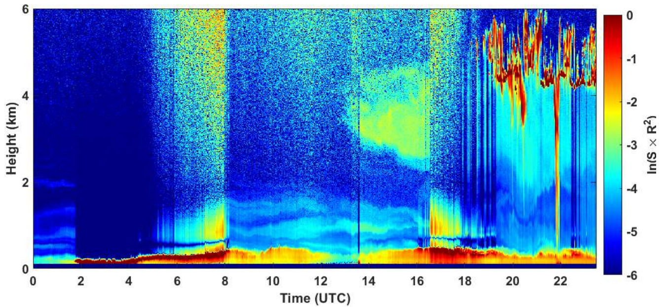
2021-05-12 RCS quick look CHM15k - ILVA LIDAR3 AGGLOMERATO
