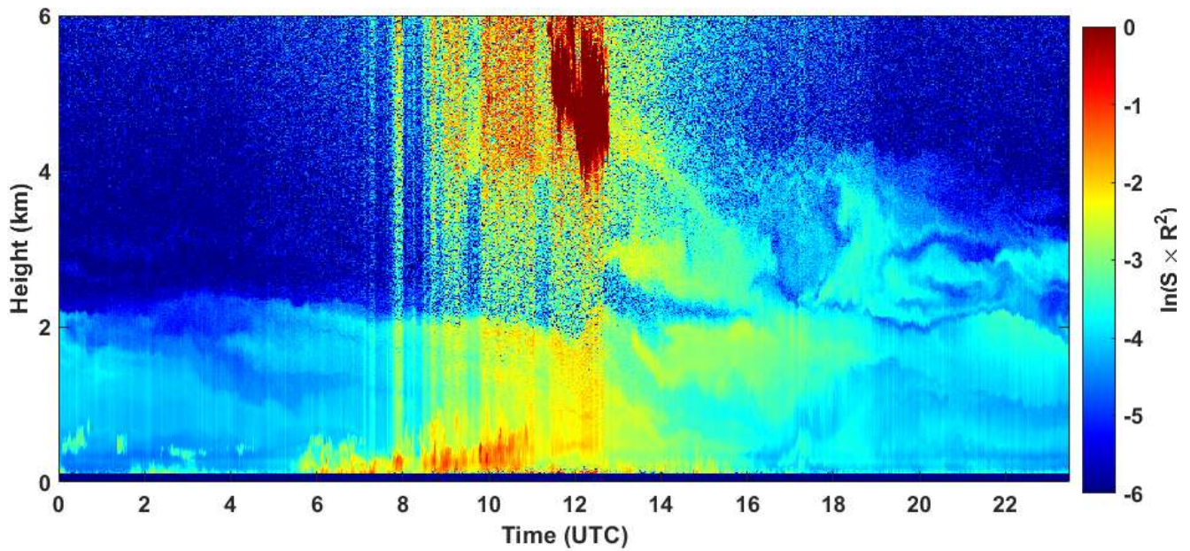
2021-05-28 RCS quick look CHM15k - ILVA LIDAR3 AGGLOMERATO
