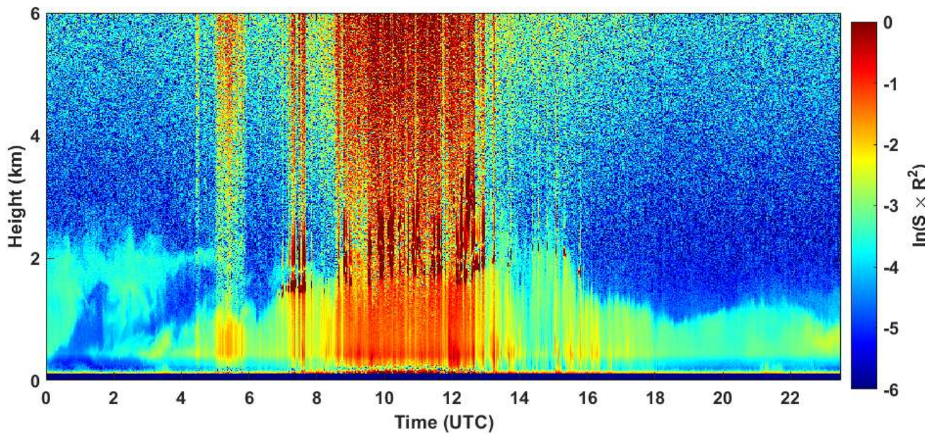
2021-05-20 RCS quick look CHM15k - ILVA LIDAR2 PARCHI
