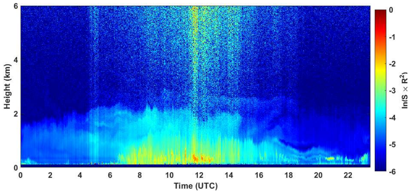
2021-05-08 RCS quick look CHM15k - ILVA LIDAR3 AGGLOMERATO
