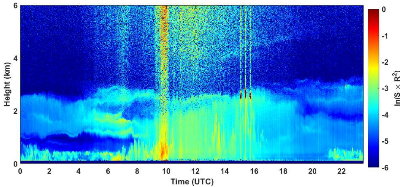
2021-05-30 RCS quick look CHM15k - ILVA LIDAR3 AGGLOMERATO
