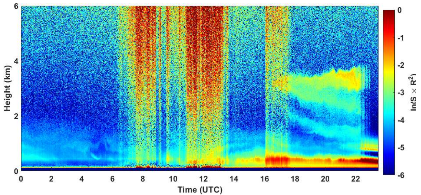
2021-05-22 RCS quick look CHM15k - ILVA LIDAR2 PARCHI
