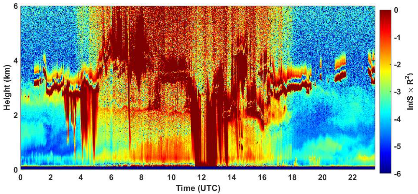
2021-05-30 RCS quick look CHM15k - ILVA LIDAR2 PARCHI
