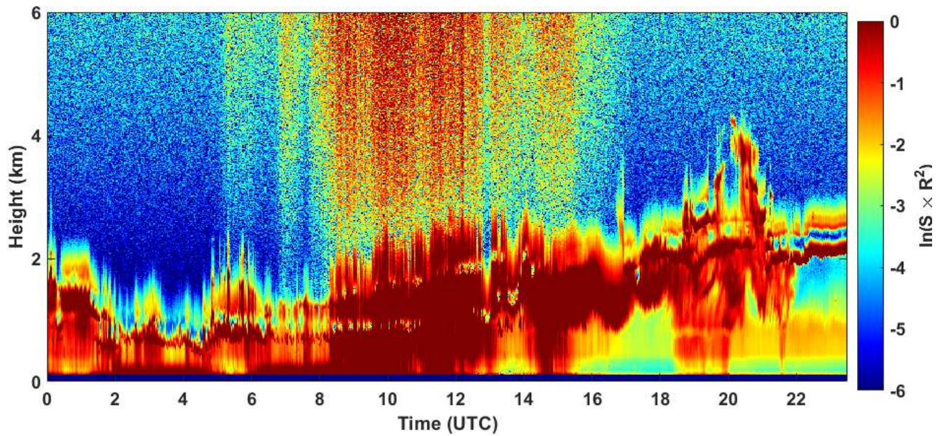
2021-03-22 RCS quick look CHM15k - ILVA LIDAR2 PARCHI
