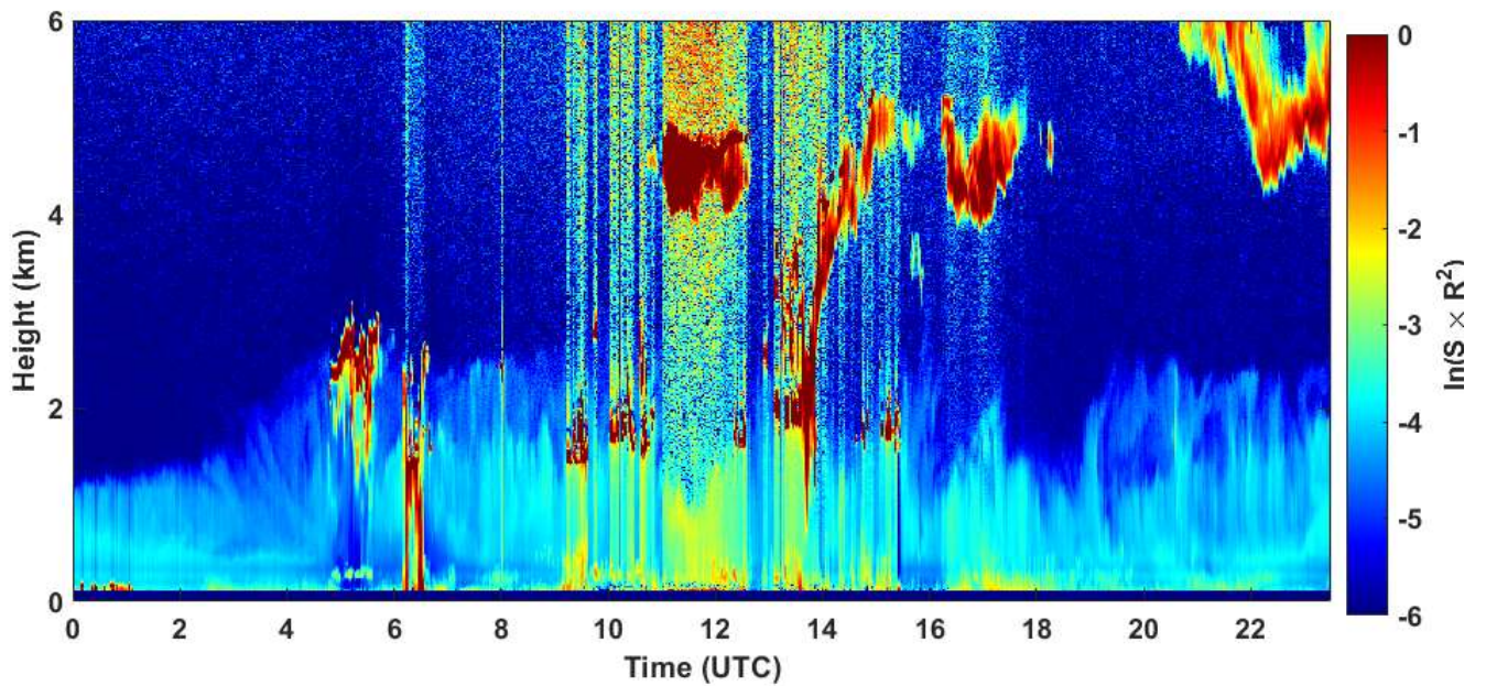
2021-03-16 RCS quick look CHM15k - ILVA LIDAR3 AGGLOMERATO
