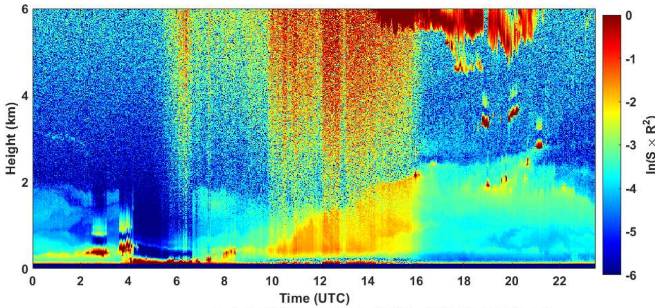
2021-03-06 RCS quick look CHM15k - ILVA LIDAR2 PARCHI
