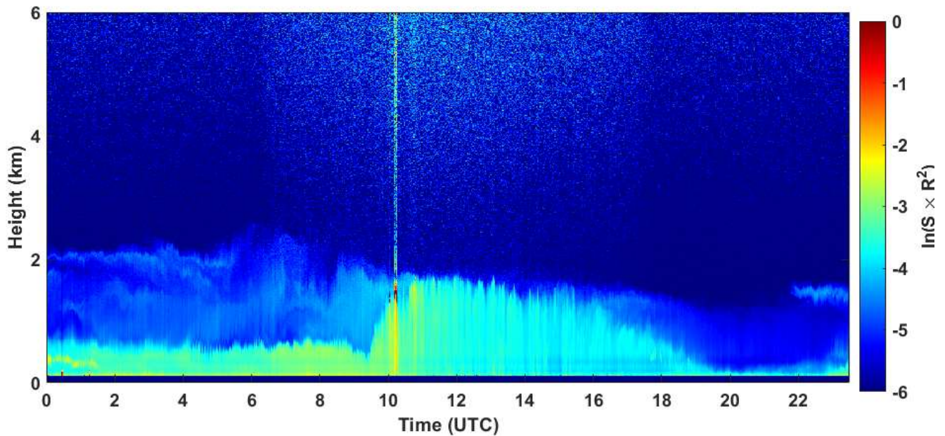
2021-03-02 RCS quick look CHM15k - ILVA LIDAR3 AGGLOMERATO
