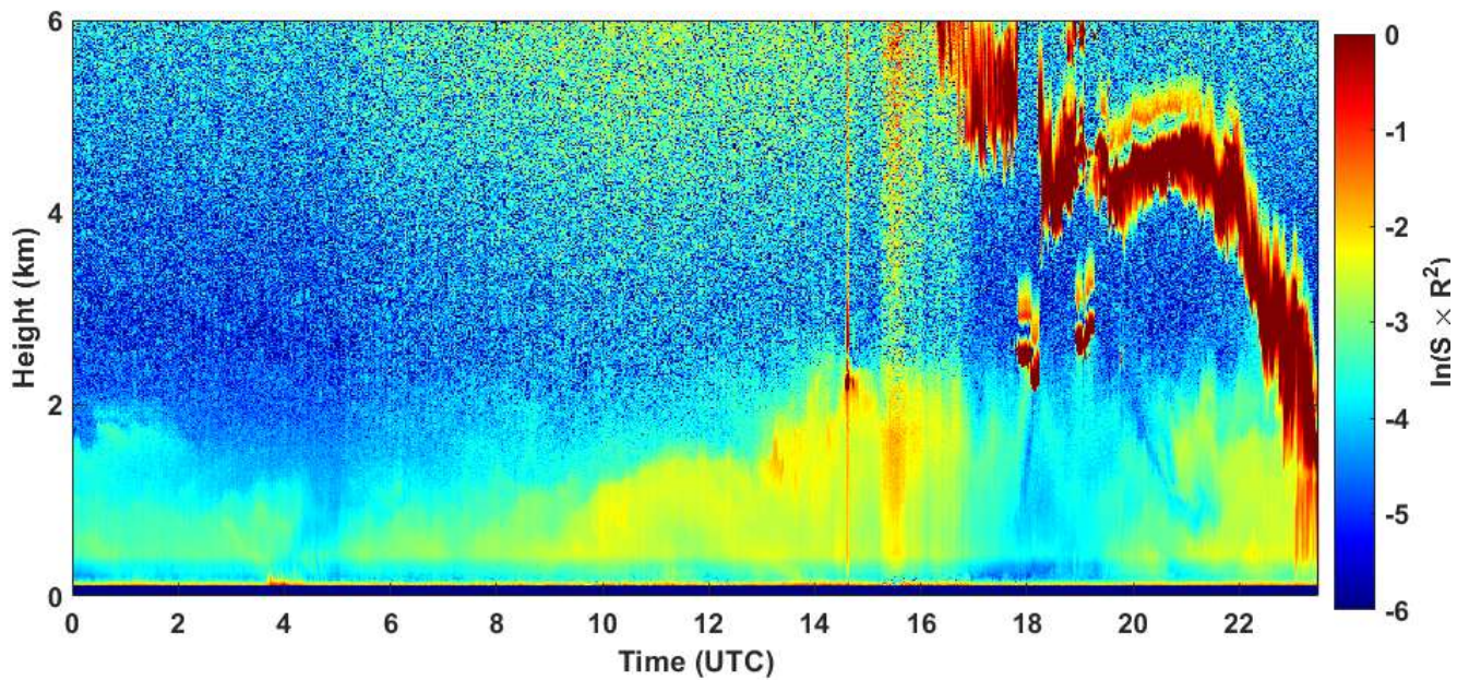
2021-03-14 RCS quick look CHM15k - ILVA LIDAR2 PARCHI
