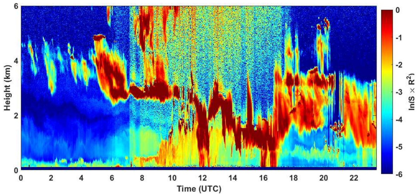
2021-03-18 RCS quick look CHM15k - ILVA LIDAR3 AGGLOMERATO
