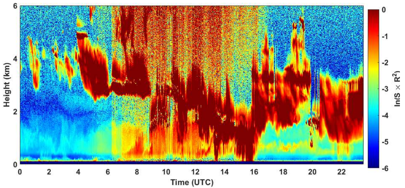
2021-03-18 RCS quick look CHM15k - ILVA LIDAR2 PARCHI
