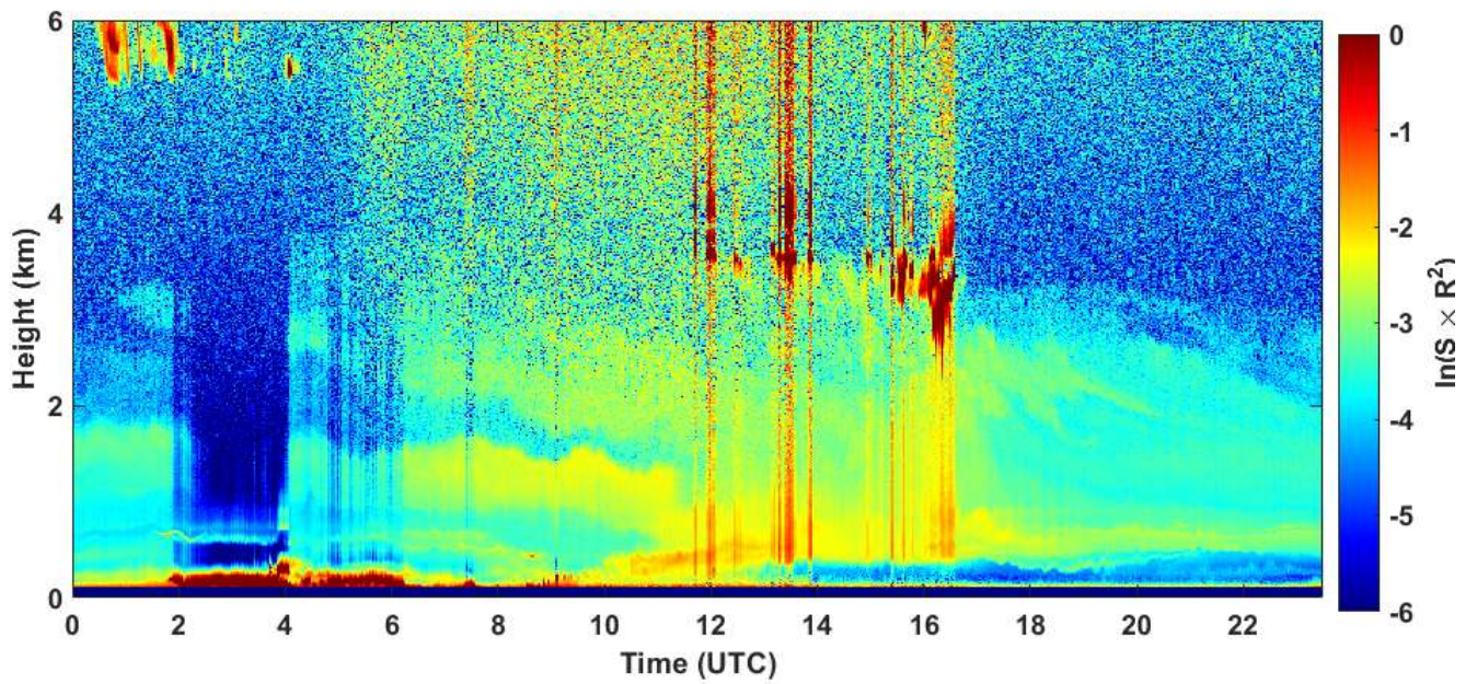
2021-03-28 RCS quick look CHM15k - ILVA LIDAR2 PARCHI
