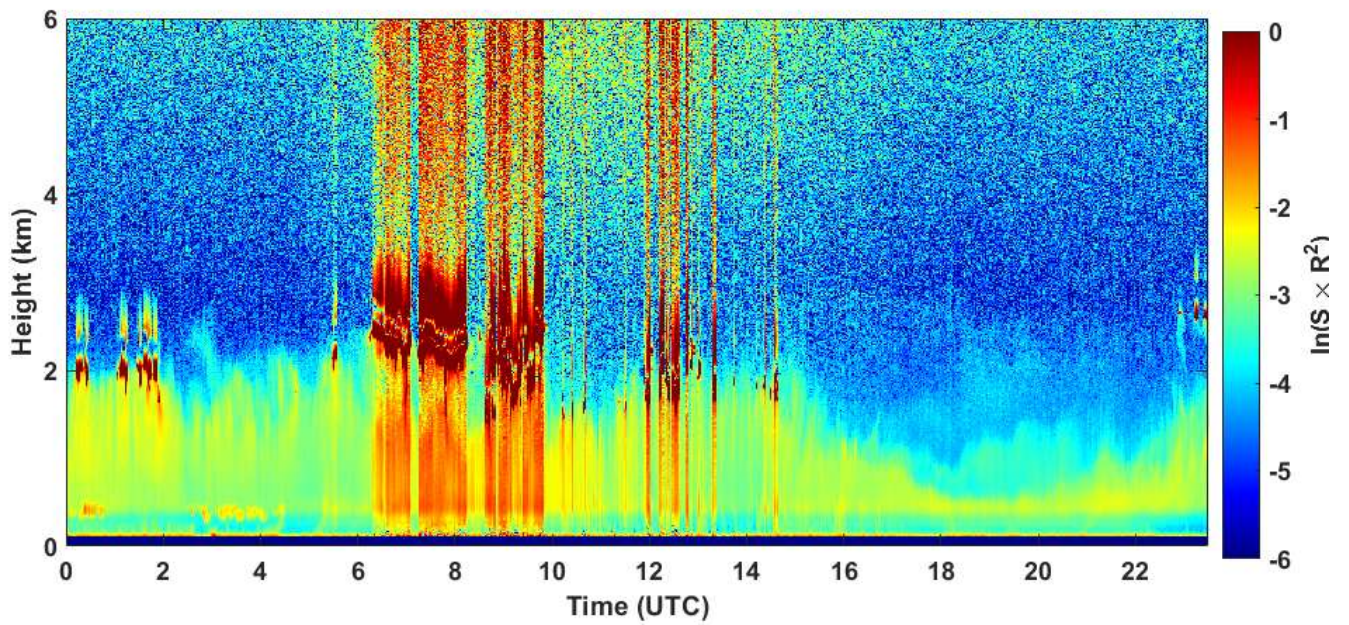
2021-03-24 RCS quick look CHM15k - ILVA LIDAR2 PARCHI
