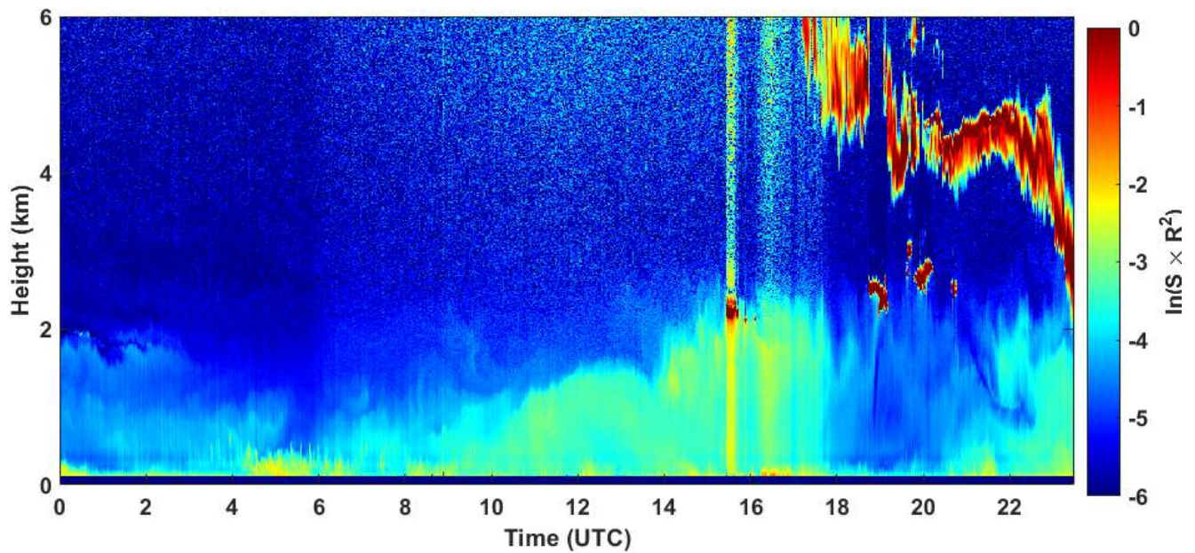
2021-03-14 RCS quick look CHM15k - ILVA LIDAR3 AGGLOMERATO
