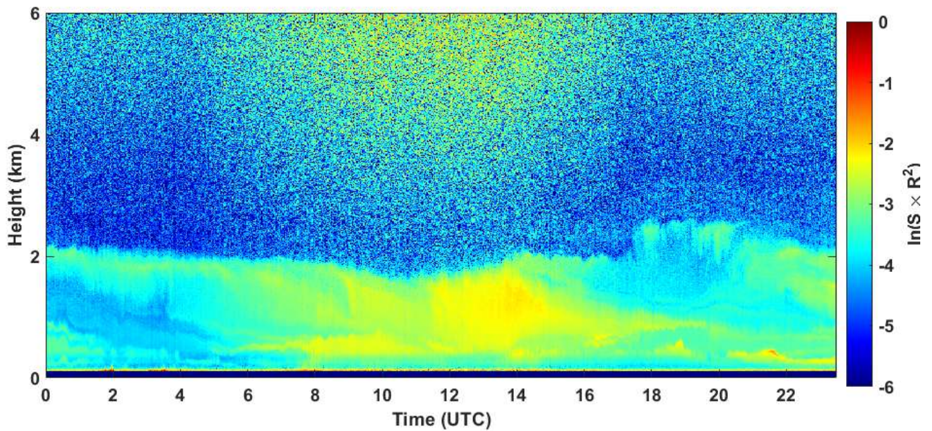
2021-03-26 RCS quick look CHM15k - ILVA LIDAR2 PARCHI
