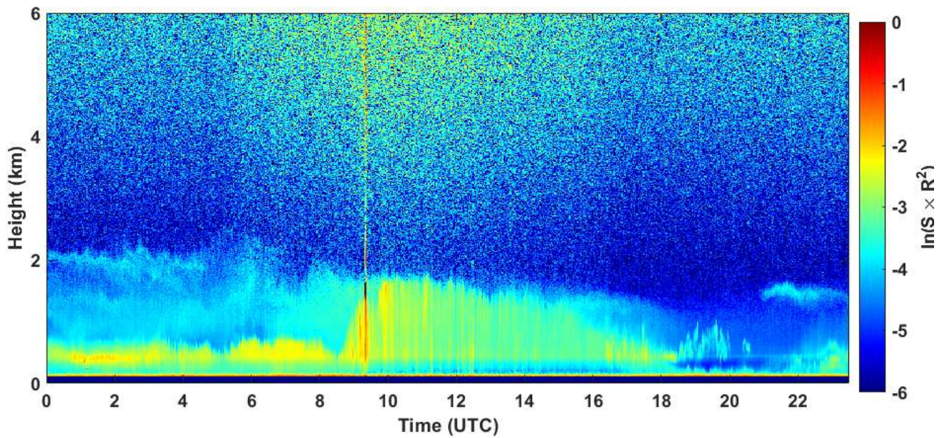
2021-03-02 RCS quick look CHM15k - ILVA LIDAR2 PARCHI
