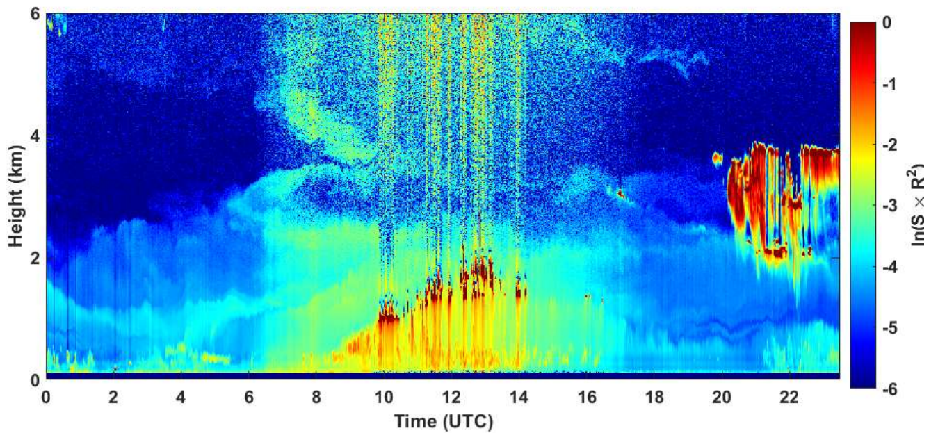
2021-03-06 RCS quick look CHM15k - ILVA LIDAR3 AGGLOMERATO
