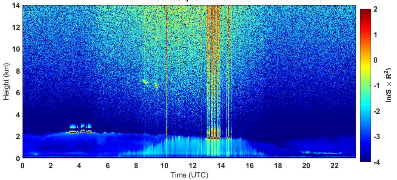
2021-03-31 RCS quick look CHM15k - ILVA LIDAR2 PARCHI
