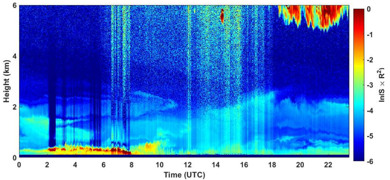
2021-03-28 RCS quick look CHM15k - ILVA LIDAR3 AGGLOMERATO
