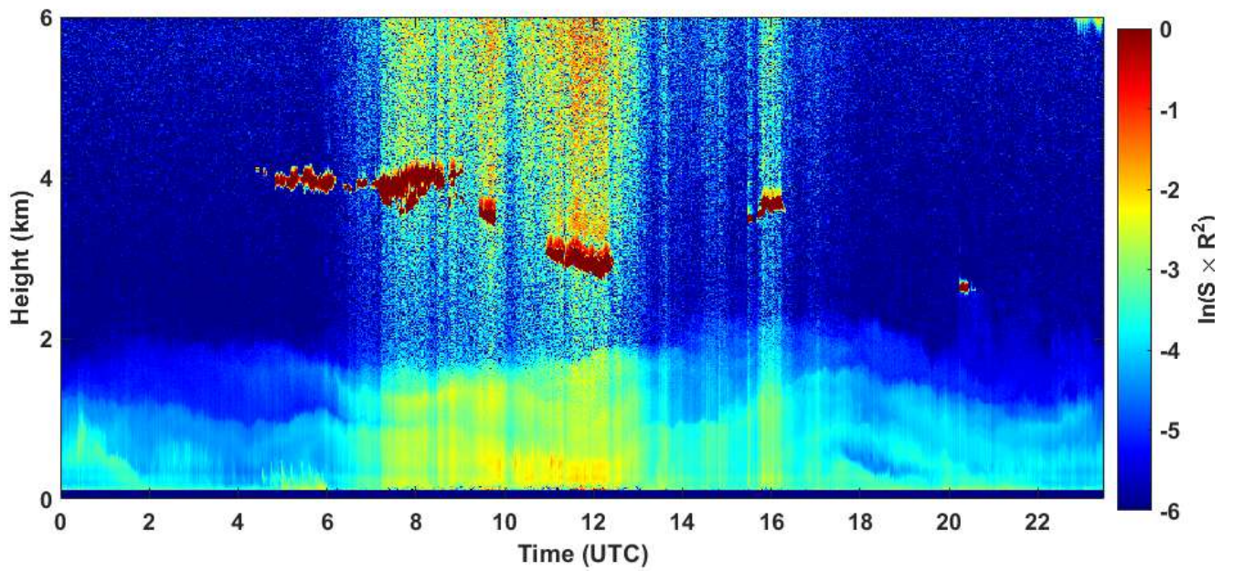
2021-03-12 RCS quick look CHM15k - ILVA LIDAR3 AGGLOMERATO
