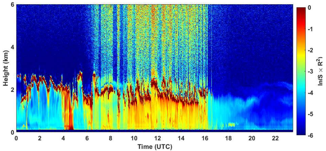
2021-03-26 RCS quick look CHM15k - ILVA LIDAR3 AGGLOMERATO
