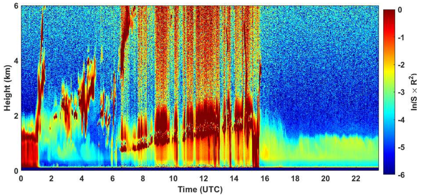
2021-03-16 RCS quick look CHM15k - ILVA LIDAR2 PARCHI
