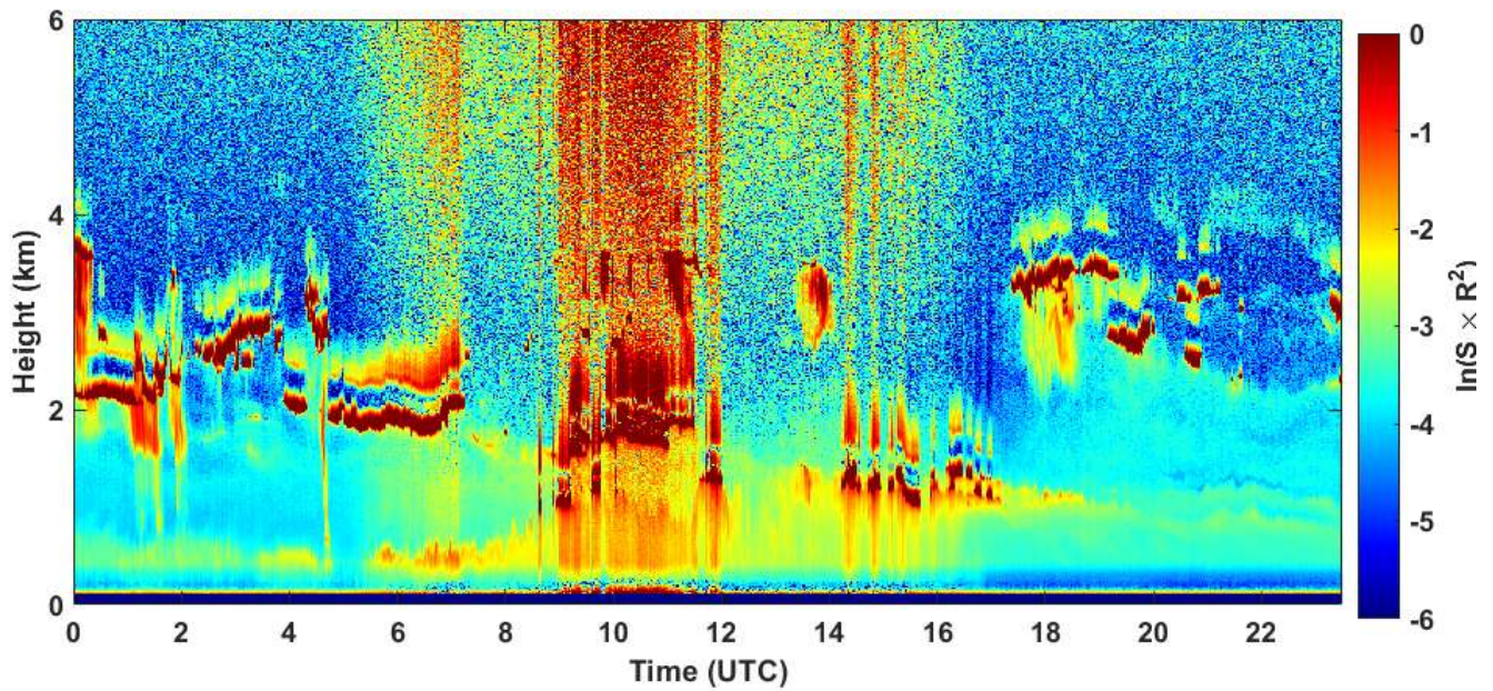
2021-03-08 RCS quick look CHM15k - ILVA LIDAR2 PARCHI
