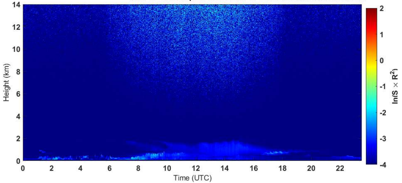
2021-03-26 RCS quick look CHM15k - ILVA LIDAR3 AGGLOMERATO
