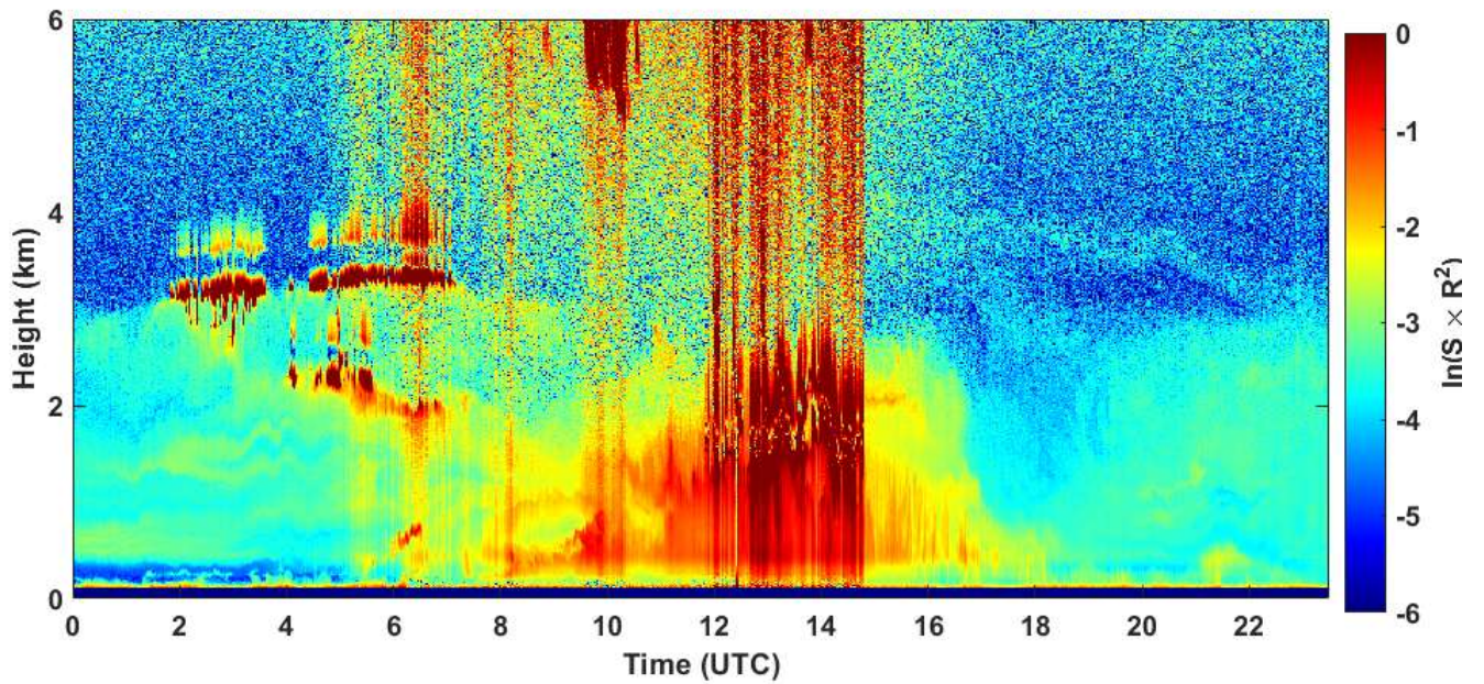
2021-03-30 RCS quick look CHM15k - ILVA LIDAR2 PARCHI
