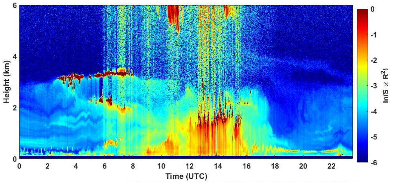
2021-03-30 RCS quick look CHM15k - ILVA LIDAR3 AGGLOMERATO
