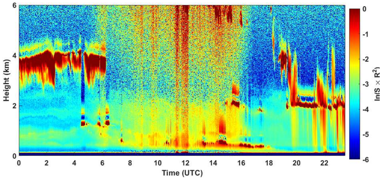
2021-03-10 RCS quick look CHM15k - ILVA LIDAR2 PARCHI
