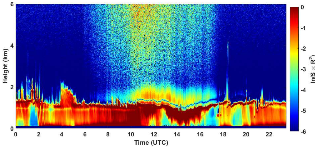
2021-03-20 RCS quick look CHM15k - ILVA LIDAR3 AGGLOMERATO
