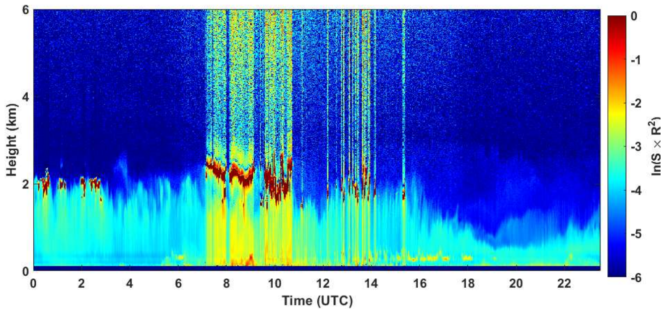
2021-03-24 RCS quick look CHM15k - ILVA LIDAR3 AGGLOMERATO
