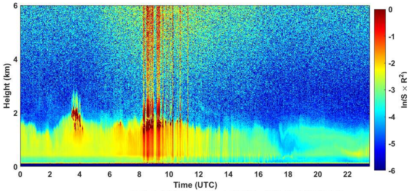
2021-03-12 RCS quick look CHM15k - ILVA LIDAR2 PARCHI
