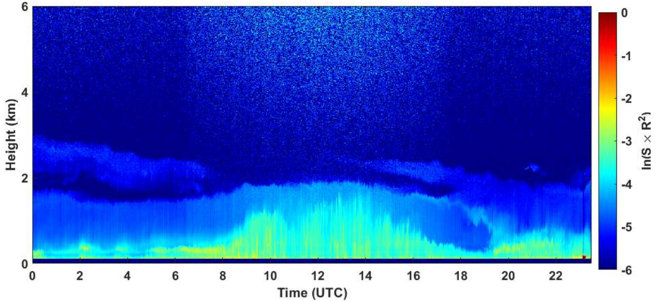
2021-03-02 RCS quick look CHM15k - ILVA LIDAR3 AGGLOMERATO
