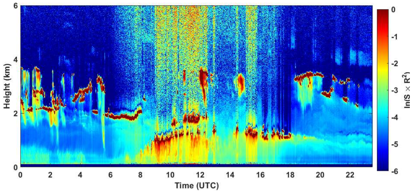
2021-03-08 RCS quick look CHM15k - ILVA LIDAR3 AGGLOMERATO
