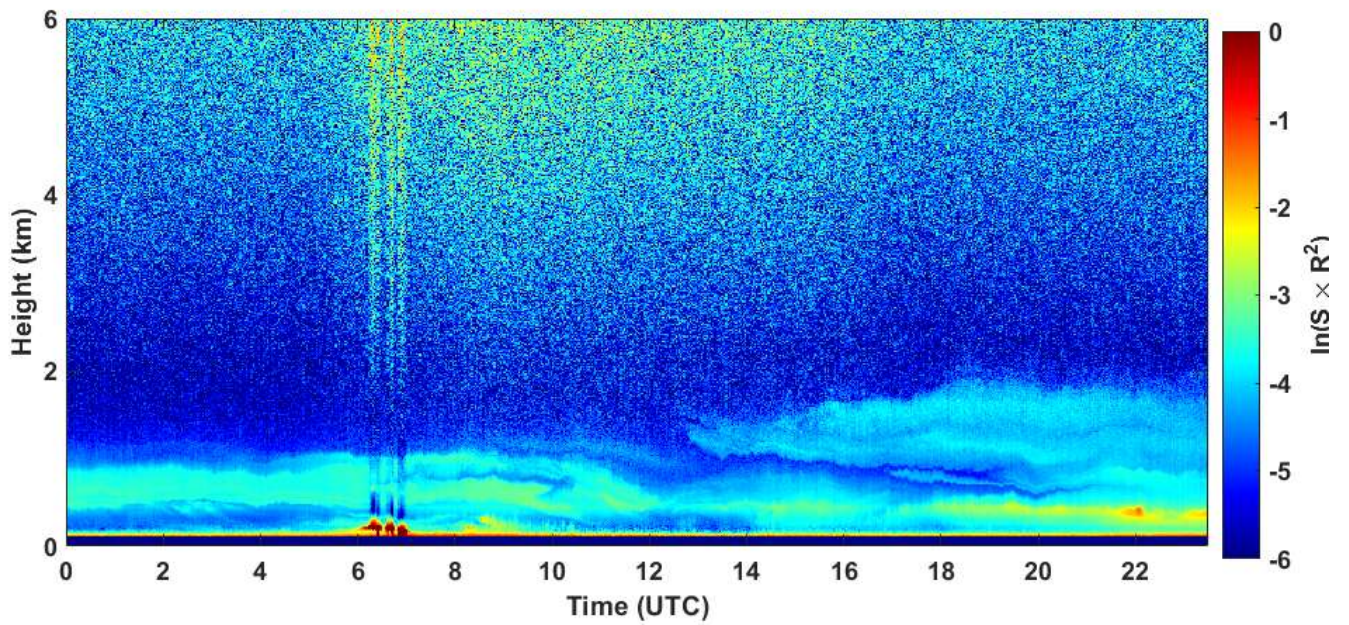
2021-03-04 RCS quick look CHM15k - ILVA LIDAR2 PARCHI
