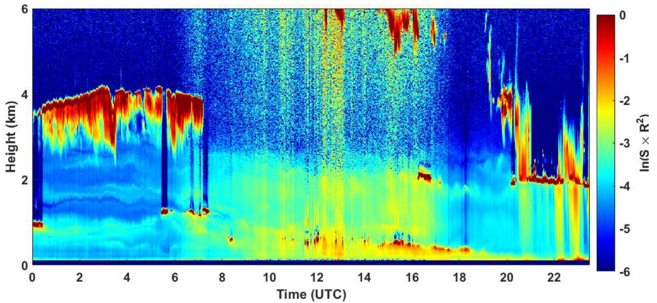
2021-03-10 RCS quick look CHM15k - ILVA LIDAR3 AGGLOMERATO
