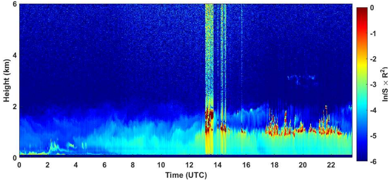
2021-01-02 RCS quick look CHM15k - ILVA LIDAR3 AGGLOMERATO
