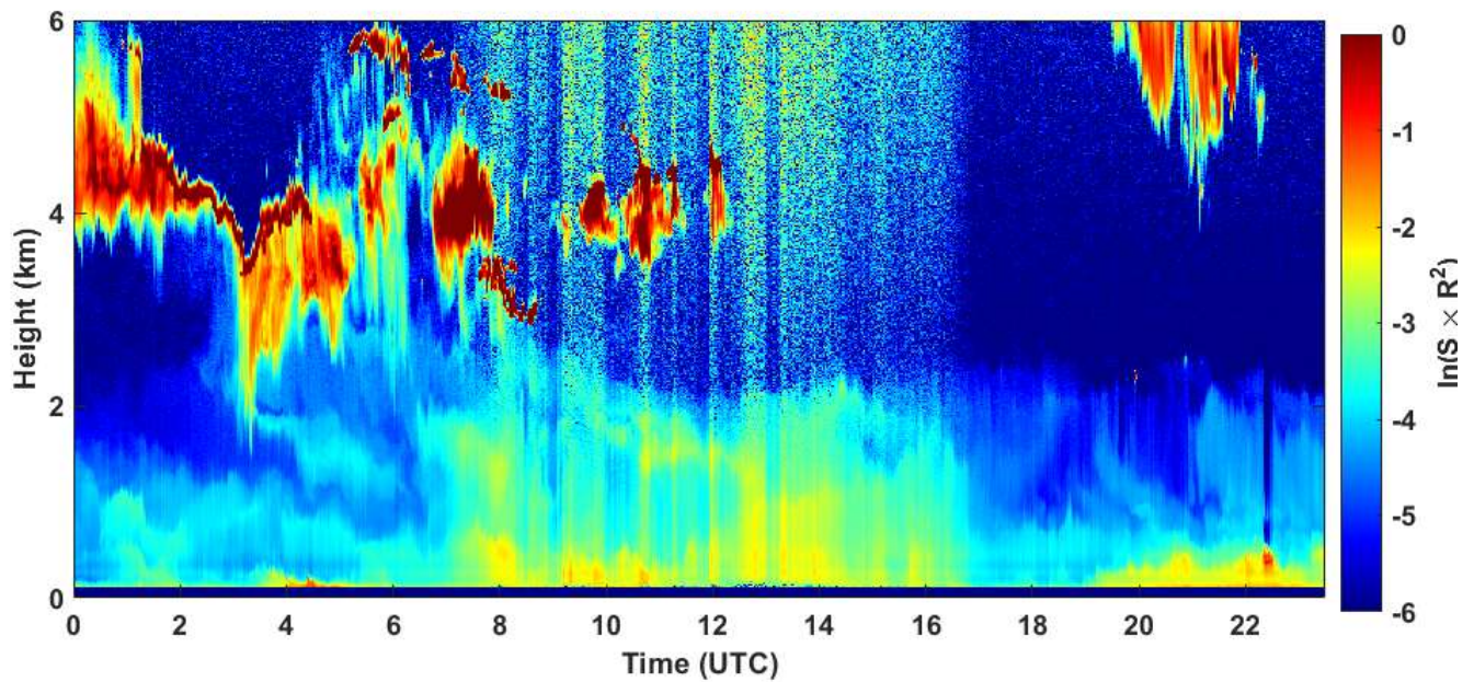
2021-01-22 RCS quick look CHM15k - ILVA LIDAR3 AGGLOMERATO
