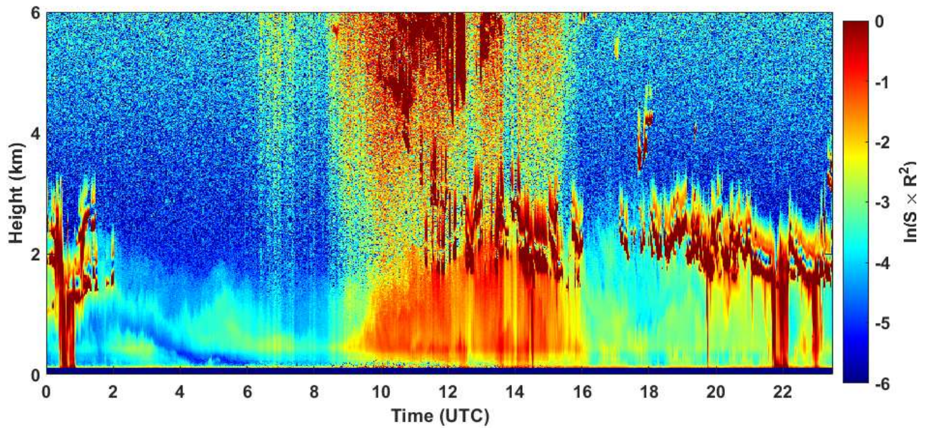
2021-01-26 RCS quick look CHM15k - ILVA LIDAR2 PARCHI
