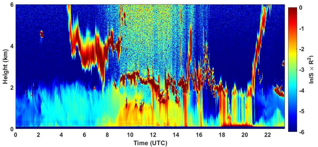
2021-01-24 RCS quick look CHM15k - ILVA LIDAR3 AGGLOMERATO
