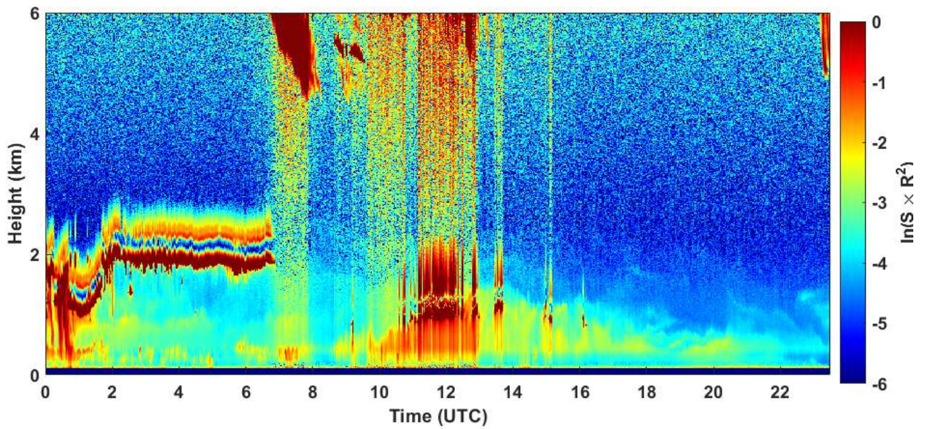
2021-01-12 RCS quick look CHM15k - ILVA LIDAR2 PARCHI
