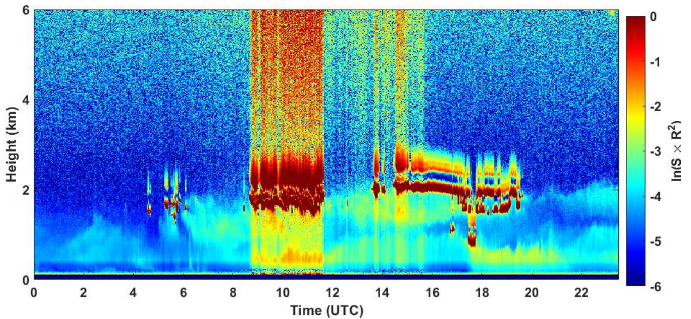
2021-01-20 RCS quick look CHM15k - ILVA LIDAR2 PARCHI
