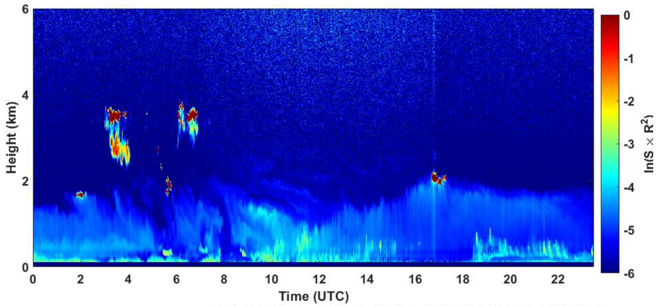
2021-01-20 RCS quick look CHM15k - ILVA LIDAR3 AGGLOMERATO
