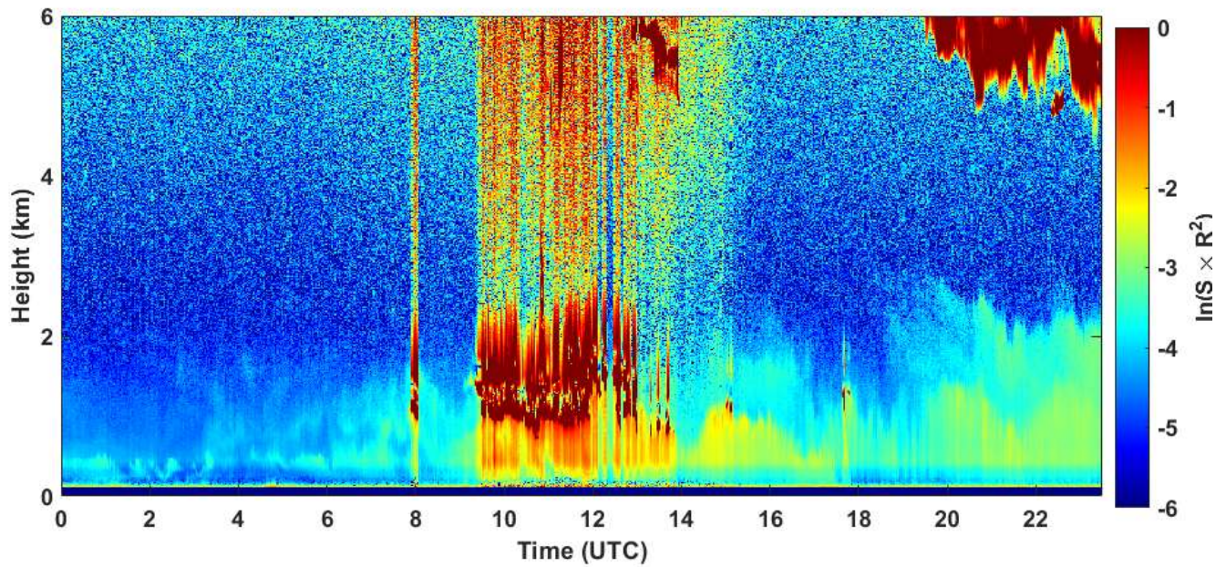
2021-01-06 RCS quick look CHM15k - ILVA LIDAR2 PARCHI
