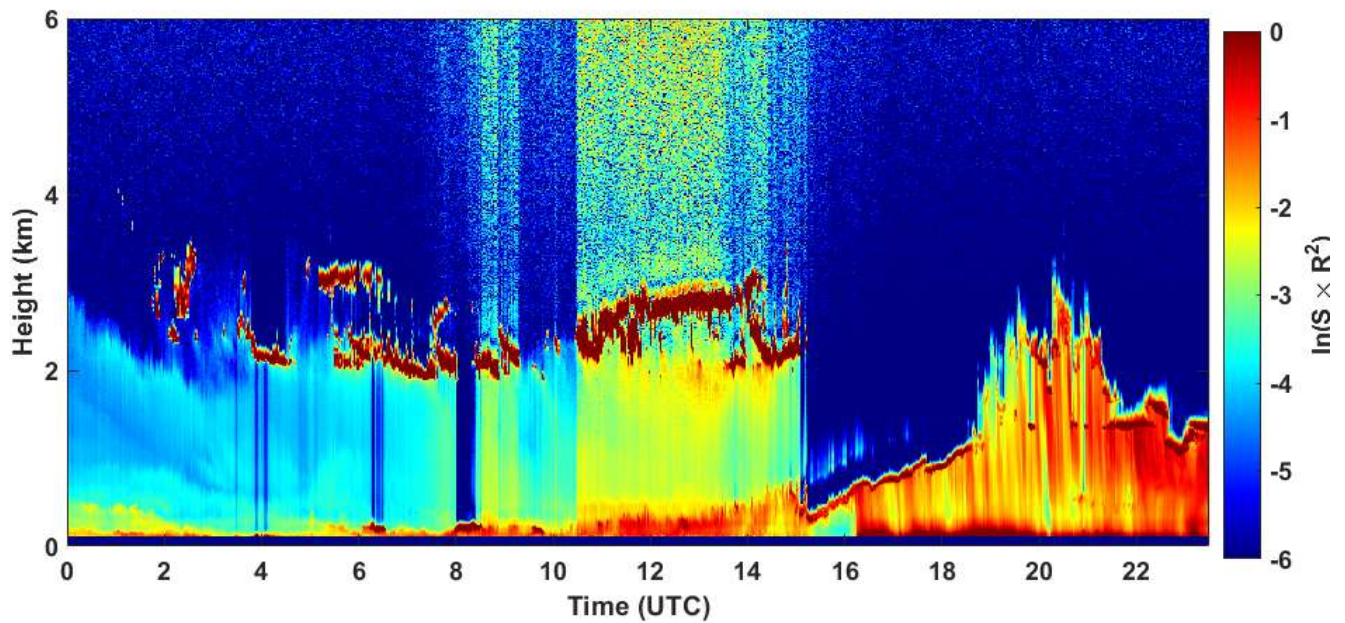
2021-01-08 RCS quick look CHM15k - ILVA LIDAR3 AGGLOMERATO
