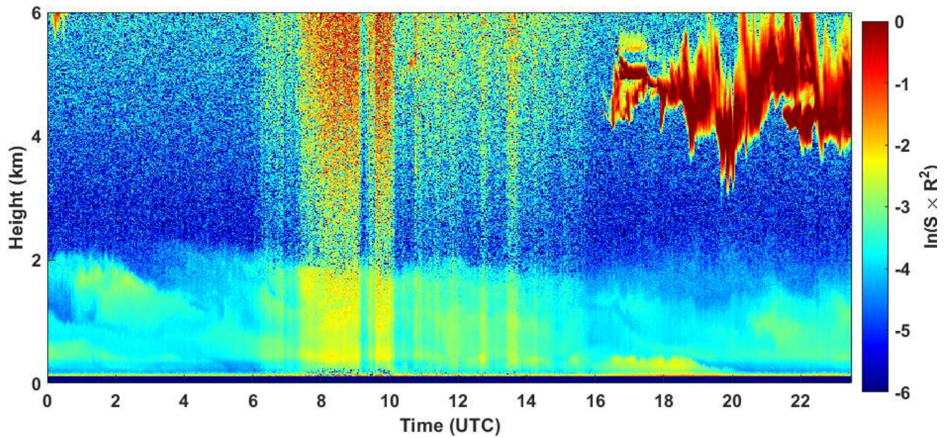
2021-01-22 RCS quick look CHM15k - ILVA LIDAR2 PARCHI
