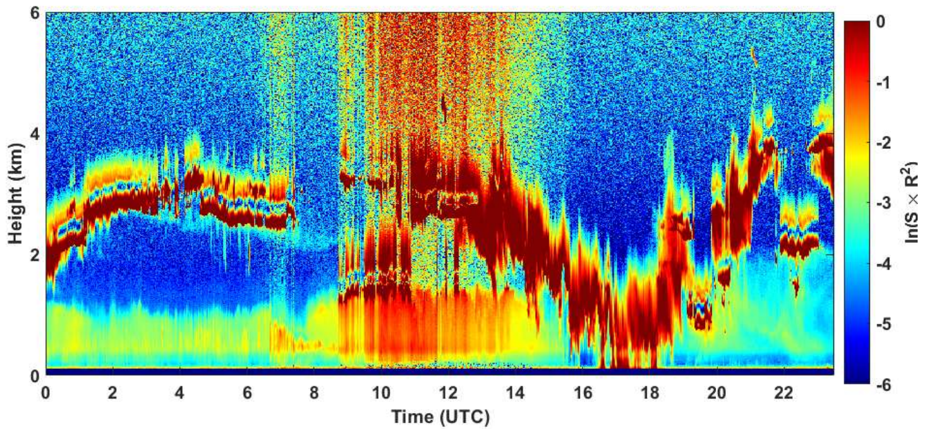
2021-01-16 RCS quick look CHM15k - ILVA LIDAR2 PARCHI
