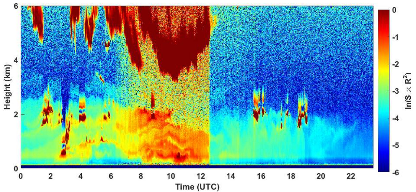
2021-01-04 RCS quick look CHM15k - ILVA LIDAR2 PARCHI
