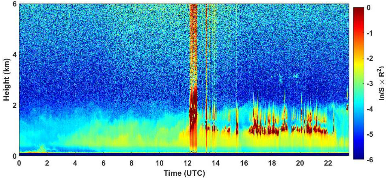
2021-01-02 RCS quick look CHM15k - ILVA LIDAR2 PARCHI
