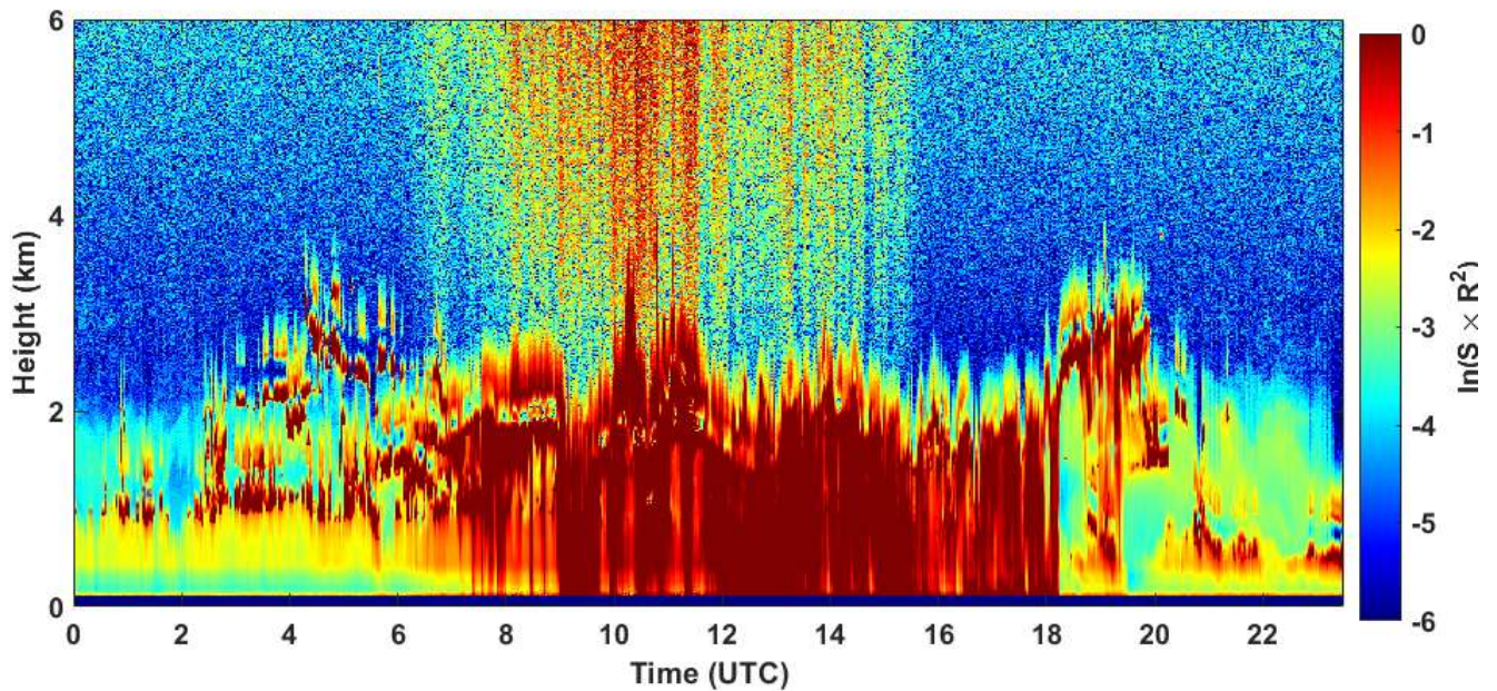
2021-01-02 RCS quick look CHM15k - ILVA LIDAR2 PARCHI
