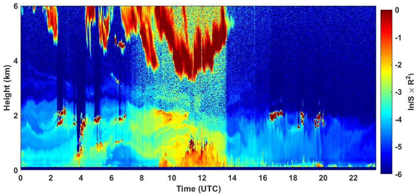
2021-01-04 RCS quick look CHM15k - ILVA LIDAR3 AGGLOMERATO
