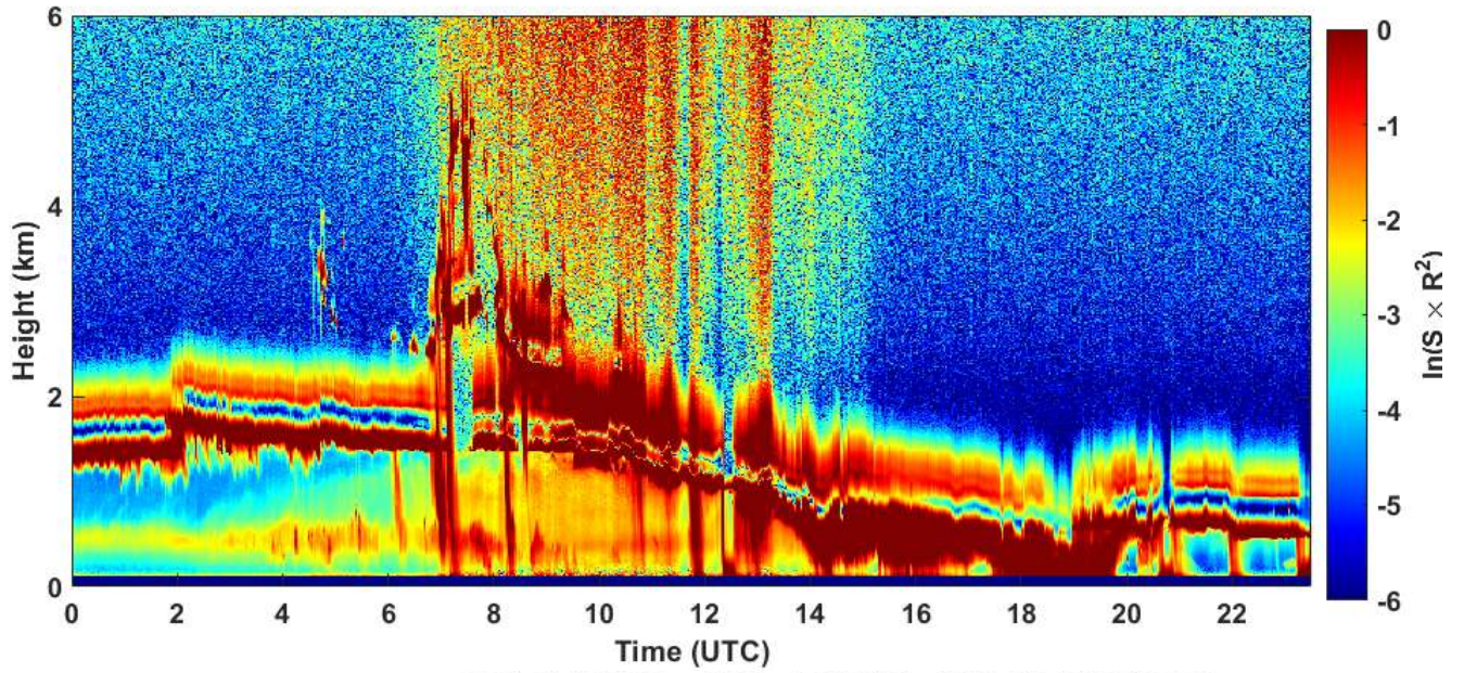
2021-01-10 RCS quick look CHM15k - ILVA LIDAR2 PARCHI
