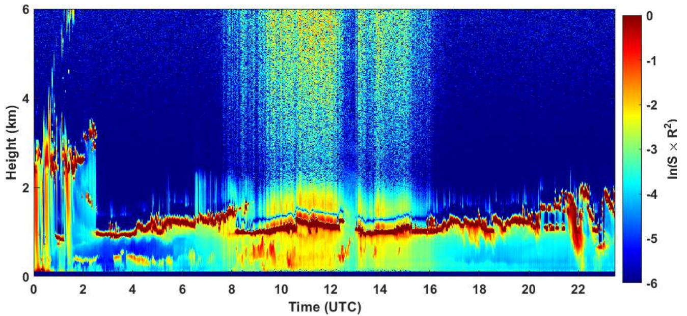
2021-01-12 RCS quick look CHM15k - ILVA LIDAR3 AGGLOMERATO
