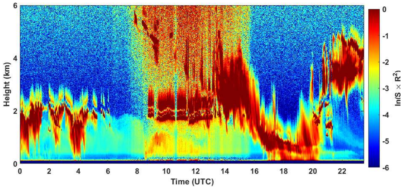
2021-01-18 RCS quick look CHM15k - ILVA LIDAR2 PARCHI
