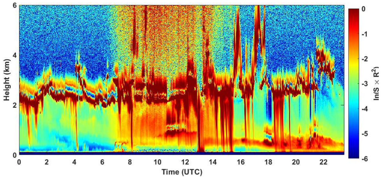
2021-01-08 RCS quick look CHM15k - ILVA LIDAR2 PARCHI
