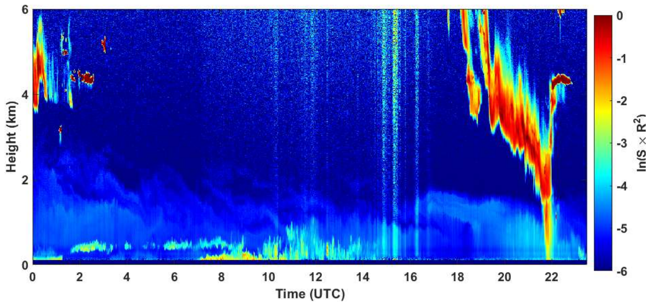
2021-01-28 RCS quick look CHM15k - ILVA LIDAR3 AGGLOMERATO
