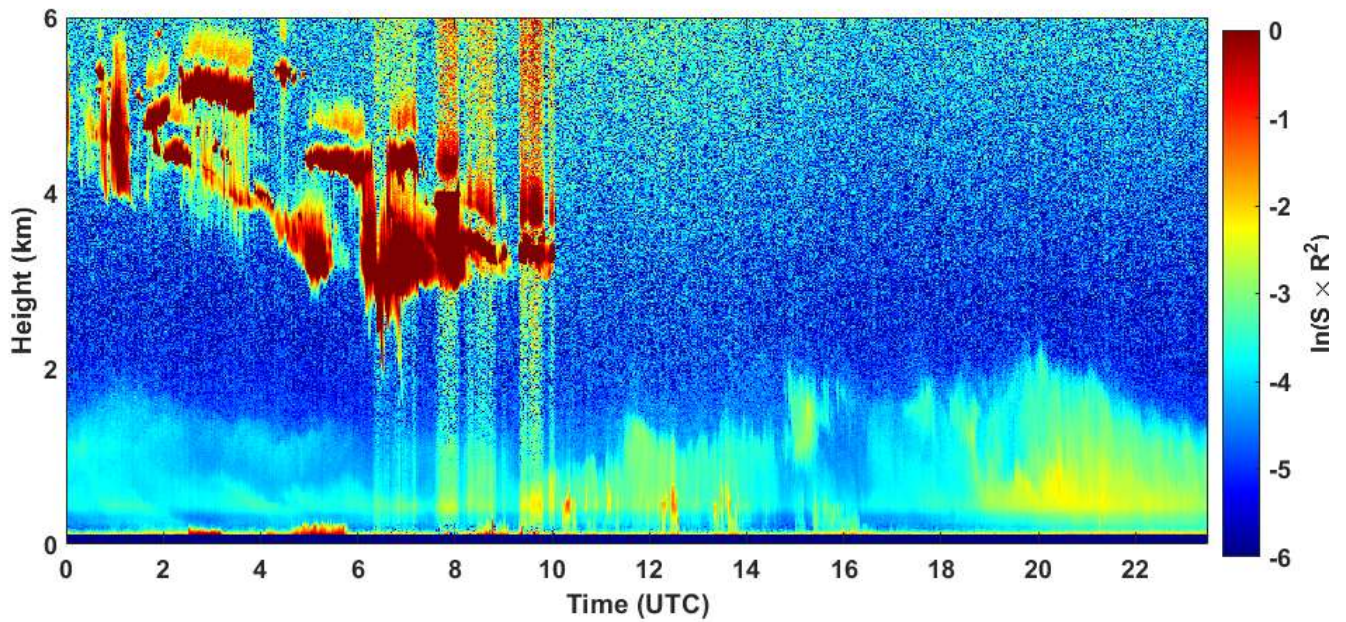
2021-01-14 RCS quick look CHM15k - ILVA LIDAR2 PARCHI
