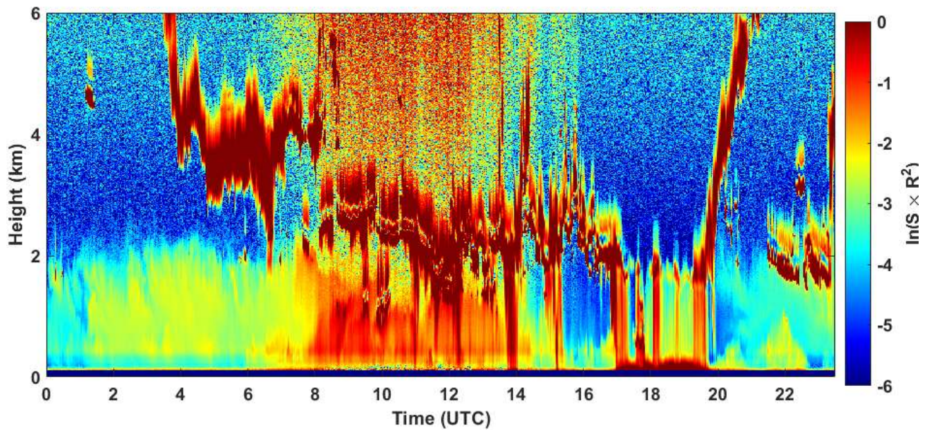
2021-01-24 RCS quick look CHM15k - ILVA LIDAR2 PARCHI
