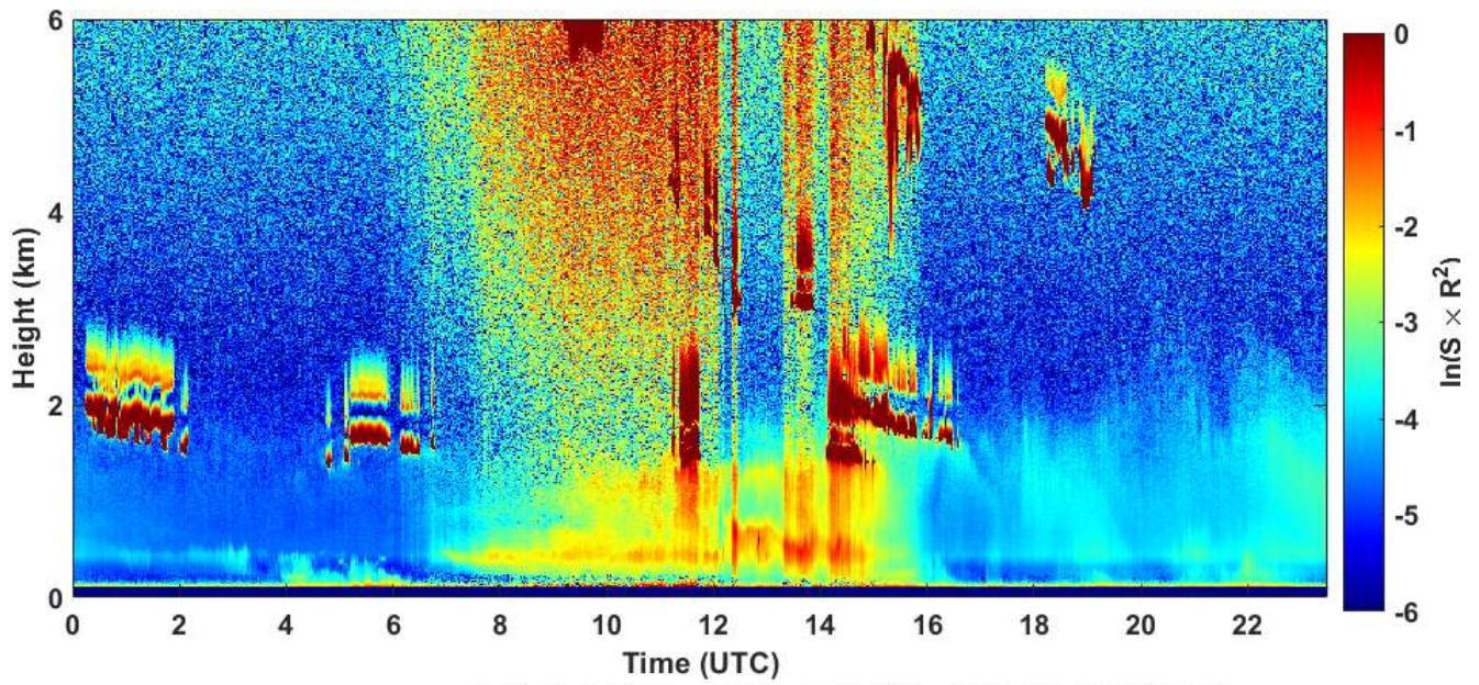
2021-01-30 RCS quick look CHM15k - ILVA LIDAR2 PARCHI
