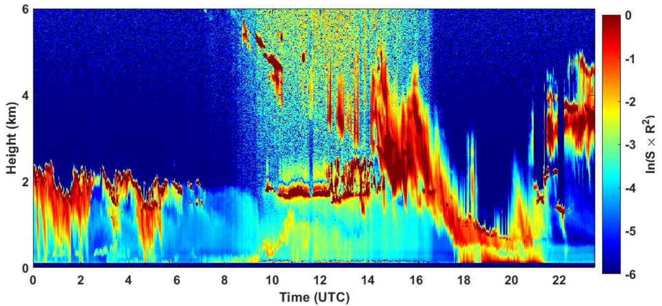
2021-01-18 RCS quick look CHM15k - ILVA LIDAR3 AGGLOMERATO
