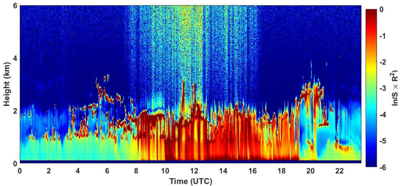
2021-01-02 RCS quick look CHM15k - ILVA LIDAR3 AGGLOMERATO
