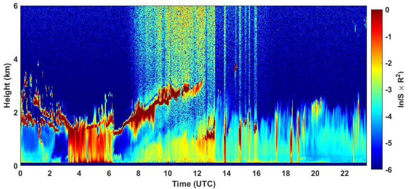
2021-01-26 RCS quick look CHM15k - ILVA LIDAR3 AGGLOMERATO
