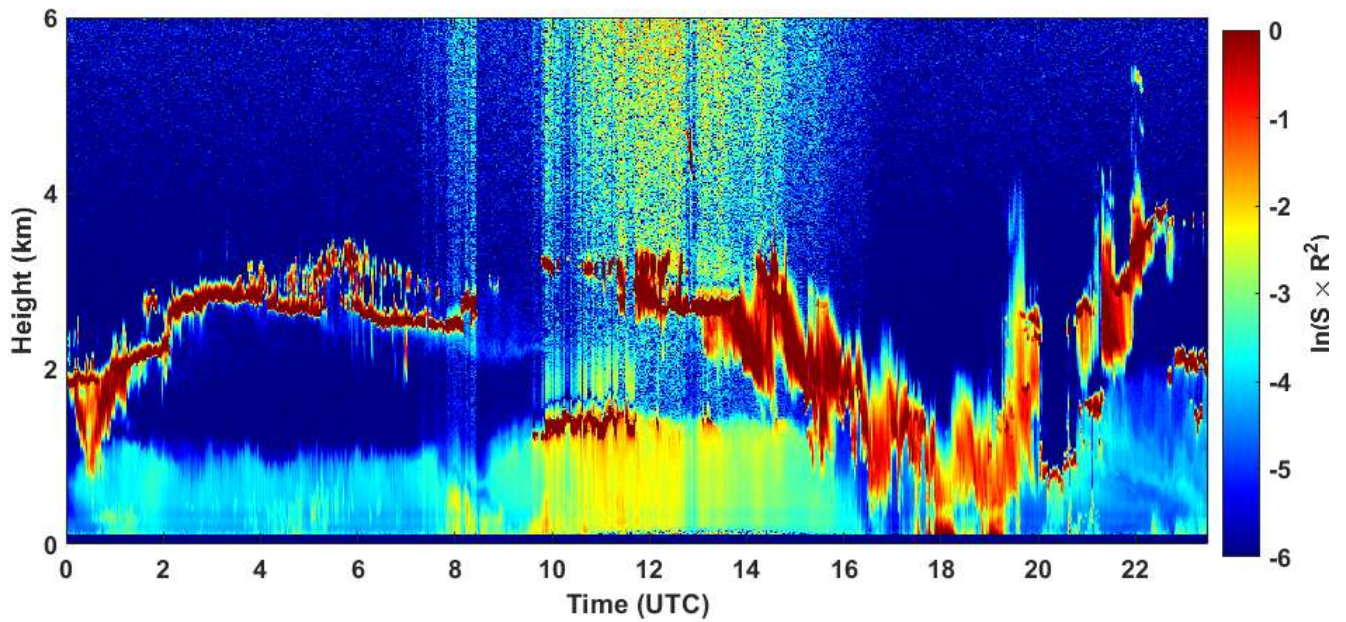
2021-01-16 RCS quick look CHM15k - ILVA LIDAR3 AGGLOMERATO
