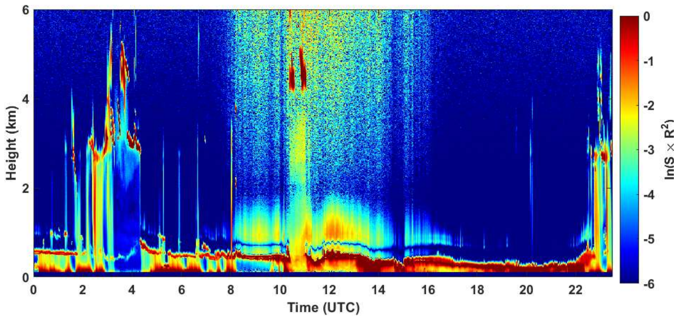
2021-01-10 RCS quick look CHM15k - ILVA LIDAR3 AGGLOMERATO
