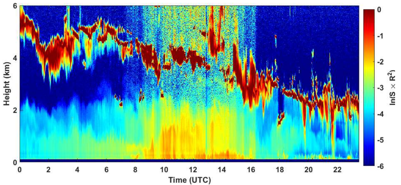
2021-01-06 RCS quick look CHM15k - ILVA LIDAR3 AGGLOMERATO
