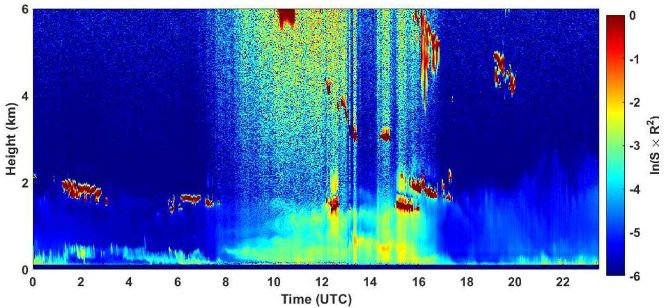
2021-01-30 RCS quick look CHM15k - ILVA LIDAR3 AGGLOMERATO
