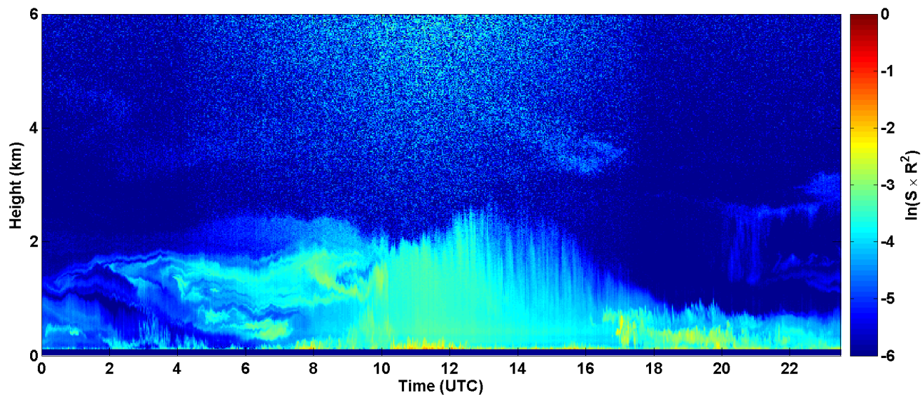
2017-08-25 RCS quick look CHM15k - ILVA LIDAR3 AGGLOMERATO
