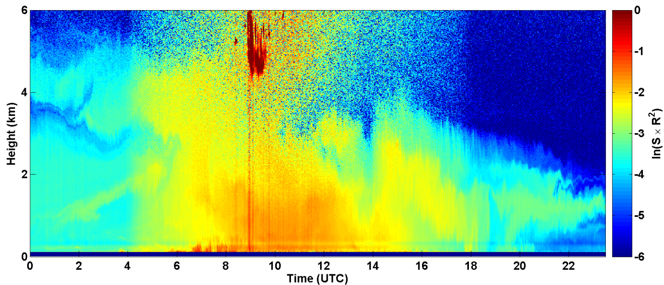
2017-08-12 RCS quick look CHM15k - ILVA LIDAR2 PARCHI
