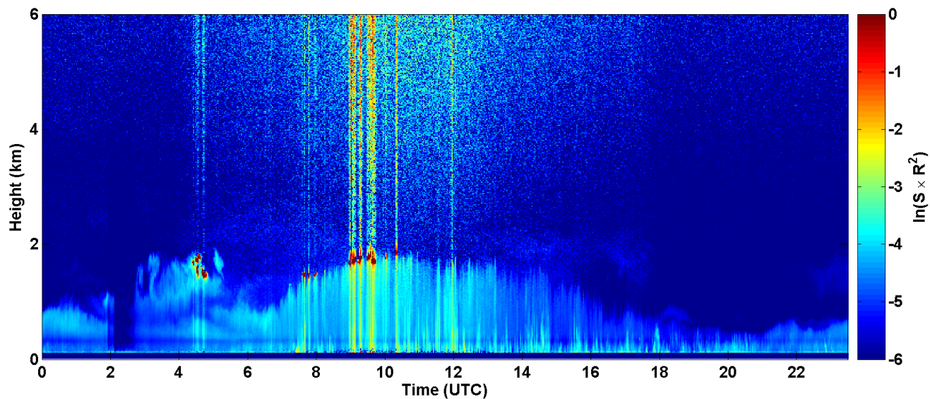
2017-08-15 RCS quick look CHM15k - ILVA LIDAR2 PARCHI
