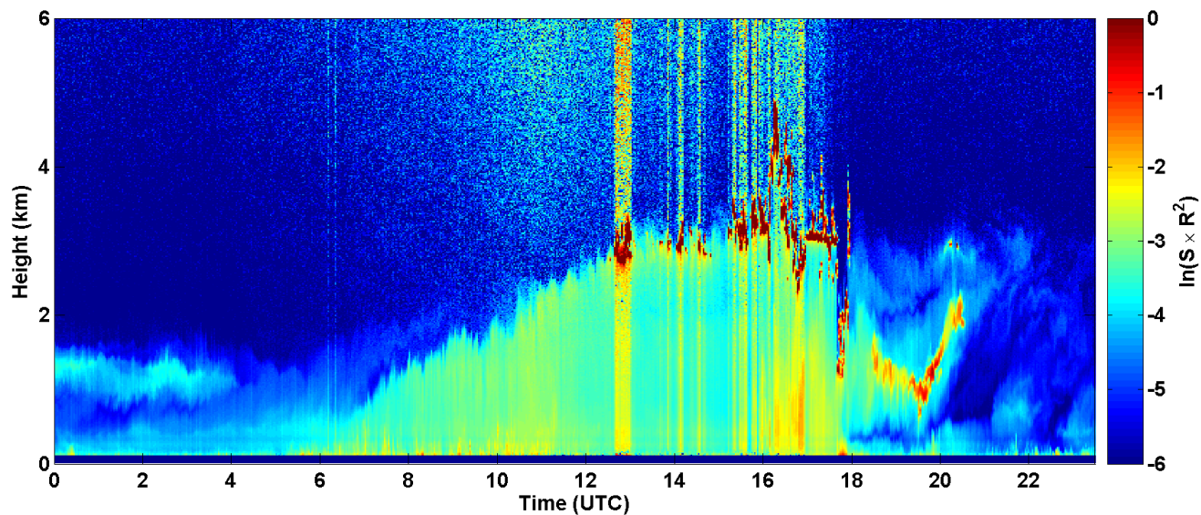
2017-08-13 RCS quick look CHM15k - ILVA LIDAR3 AGGLOMERATO
