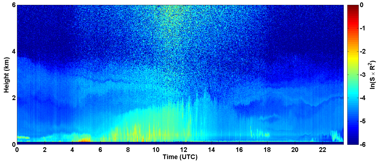
2017-08-02 RCS quick look CHM15k - ILVA LIDAR3 AGGLOMERATO
