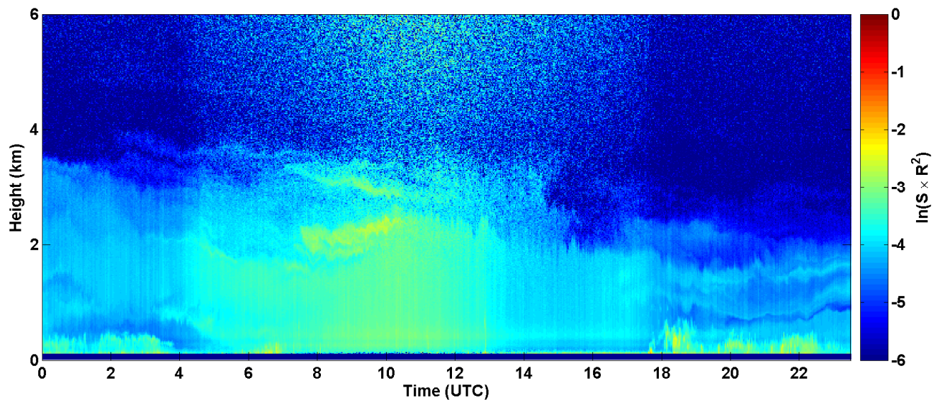
2017-08-19 RCS quick look CHM15k - ILVA LIDAR3 AGGLOMERATO
