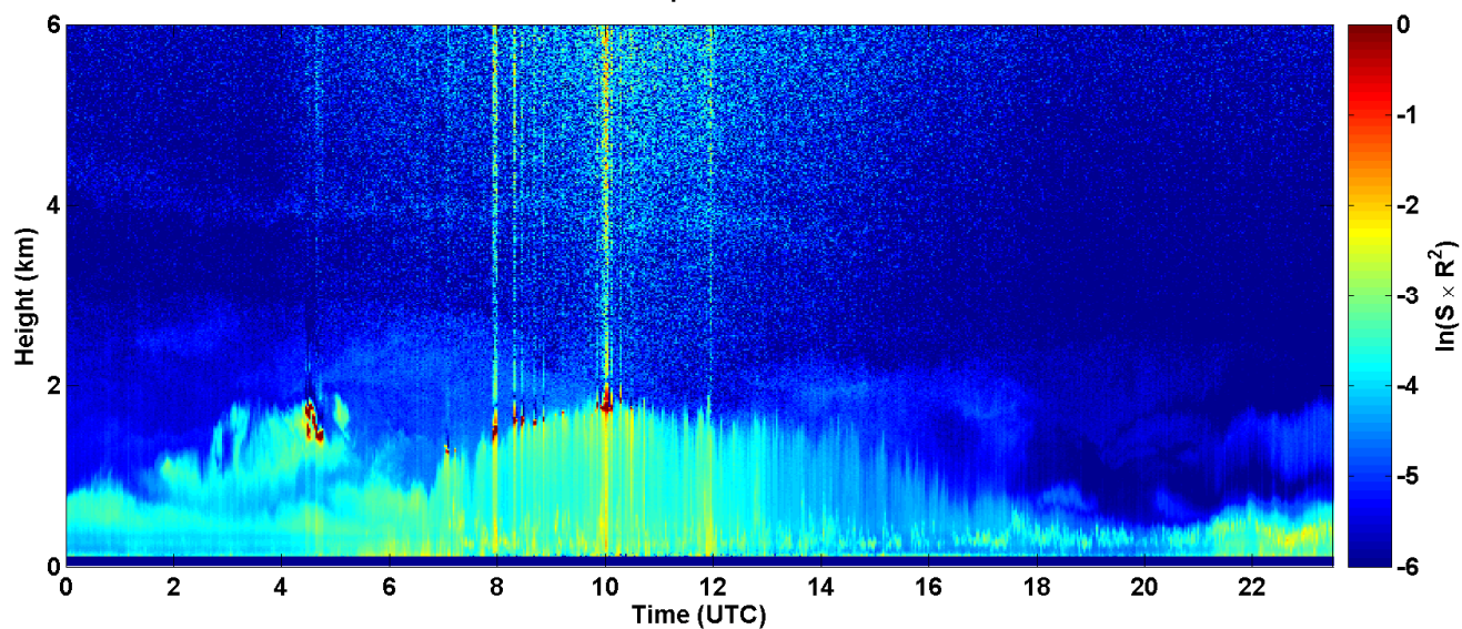
2017-08-14 RCS quick look CHM15k - ILVA LIDAR3 AGGLOMERATO
