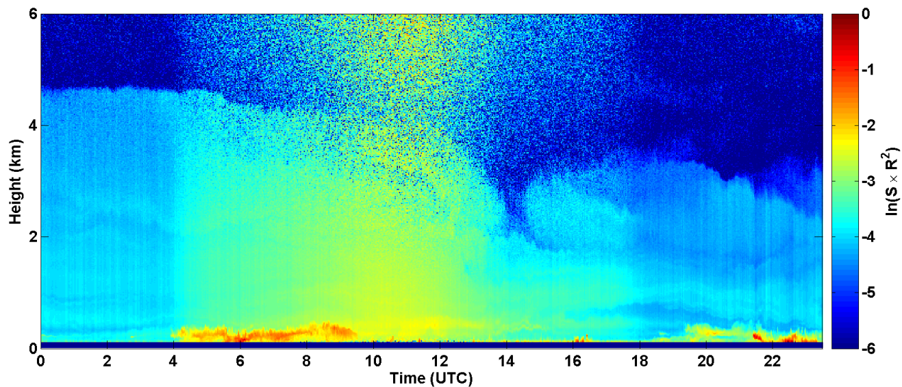
2017-08-07 RCS quick look CHM15k - ILVA LIDAR3 AGGLOMERATO
