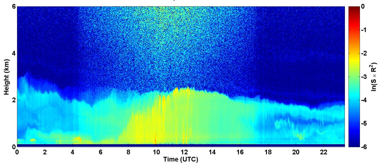
2017-08-30 RCS quick look CHM15k - ILVA LIDAR3 AGGLOMERATO
