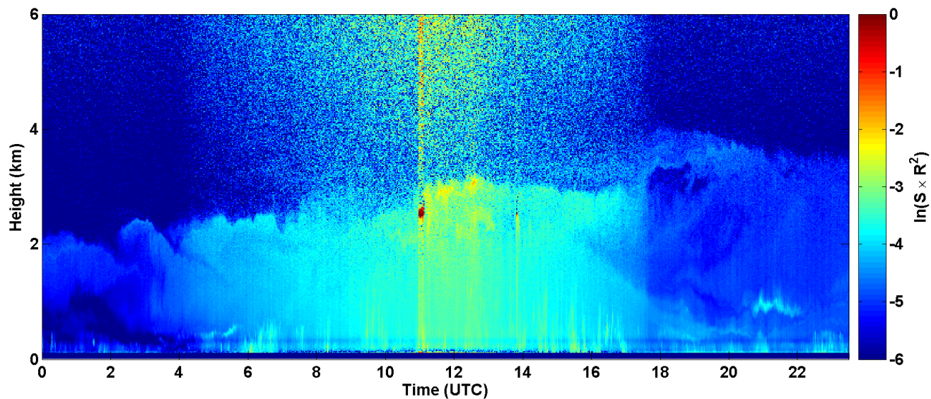
2017-08-18 RCS quick look CHM15k - ILVA LIDAR2 PARCHI
