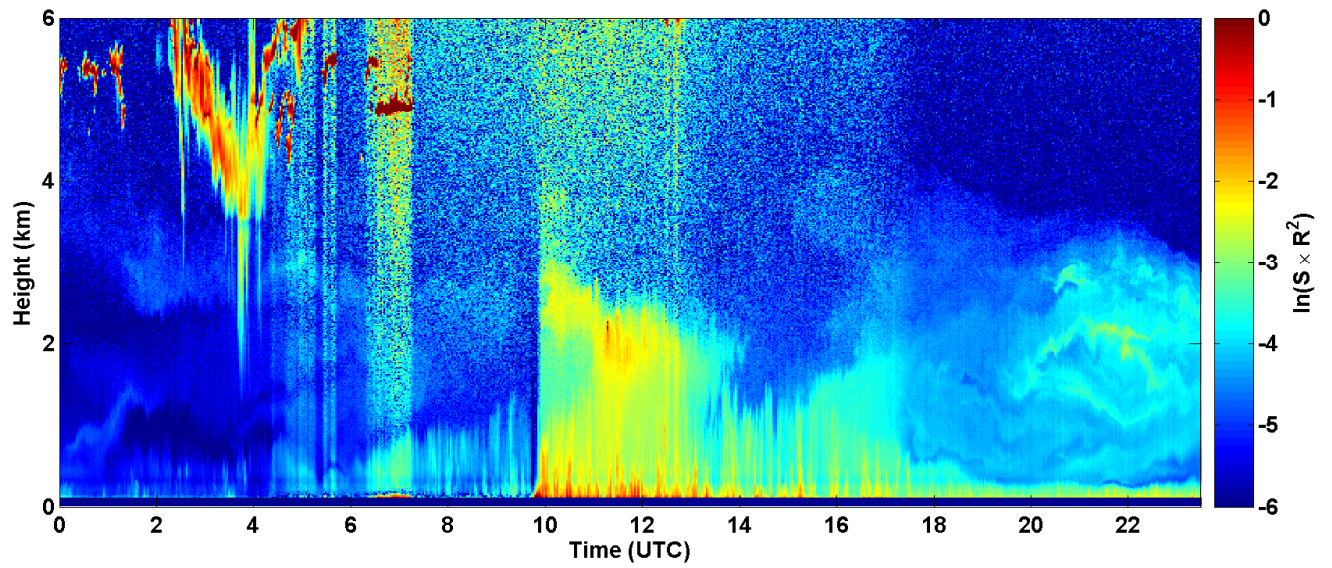
2017-08-30 RCS quick look CHM15k - ILVA LIDAR2 PARCHI
