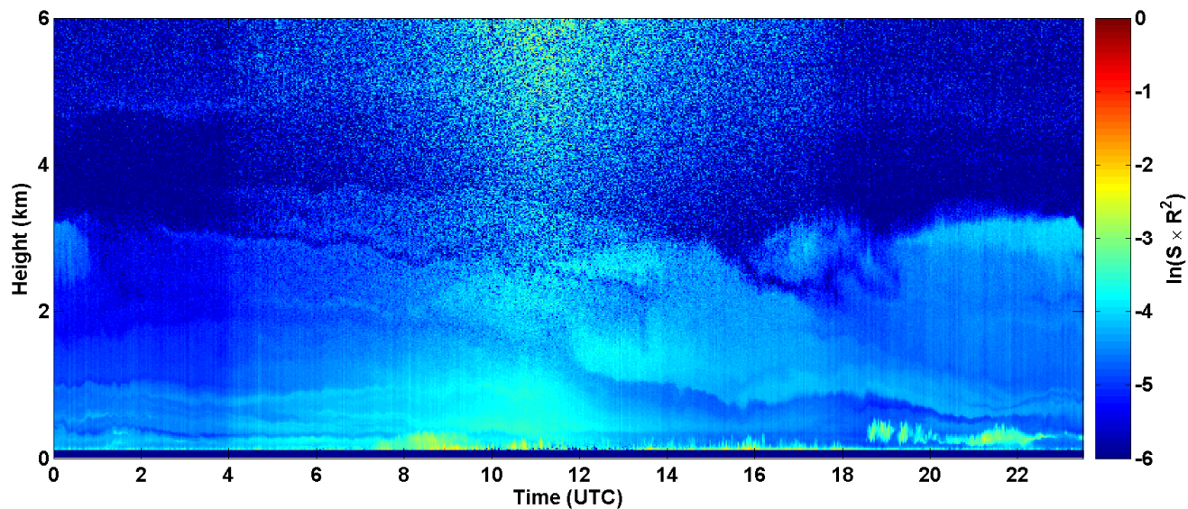
2017-08-10 RCS quick look CHM15k - ILVA LIDAR3 AGGLOMERATO
