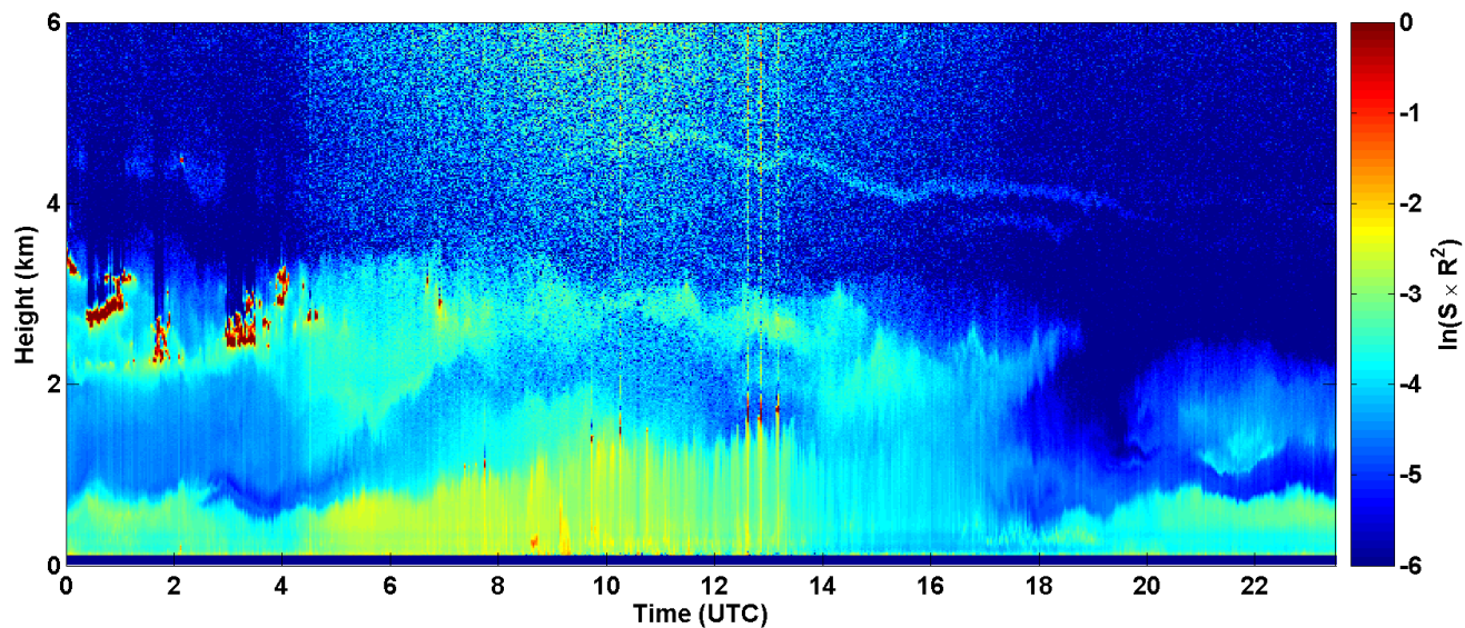
2017-08-22 RCS quick look CHM15k - ILVA LIDAR3 AGGLOMERATO
