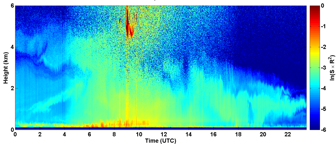
2017-08-11 RCS quick look CHM15k - ILVA LIDAR3 AGGLOMERATO
