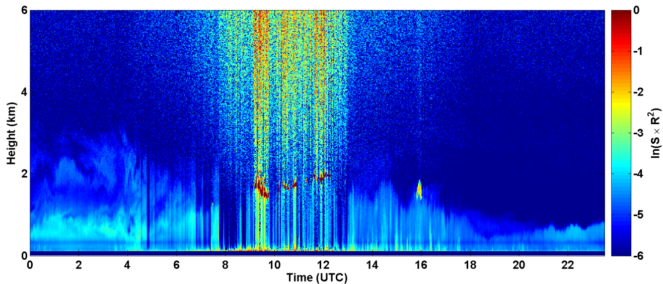
2017-08-13 RCS quick look CHM15k - ILVA LIDAR2 PARCHI
