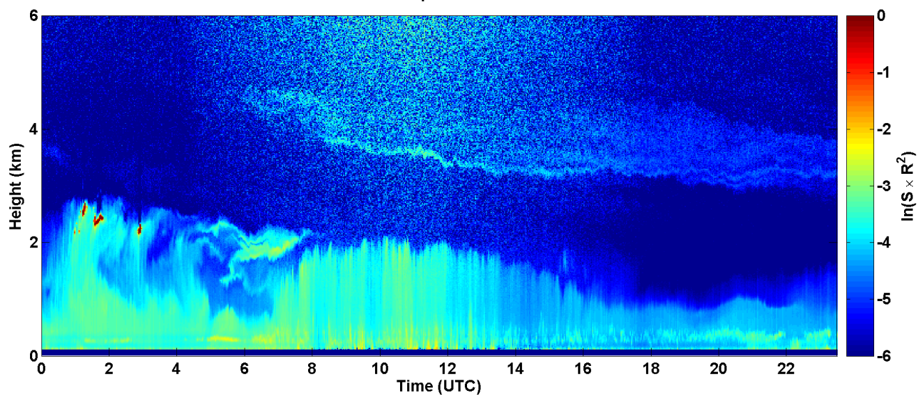
2017-08-23 RCS quick look CHM15k - ILVA LIDAR3 AGGLOMERATO
