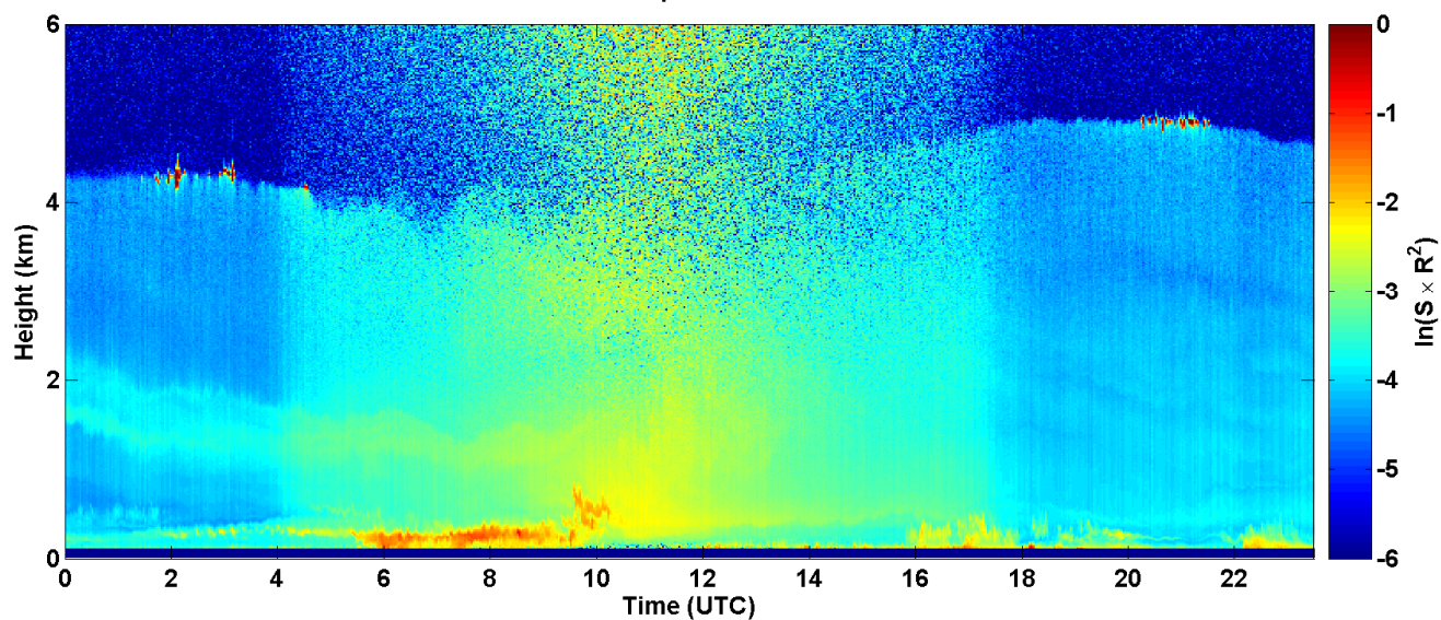
2017-08-05 RCS quick look CHM15k - ILVA LIDAR3 AGGLOMERATO
