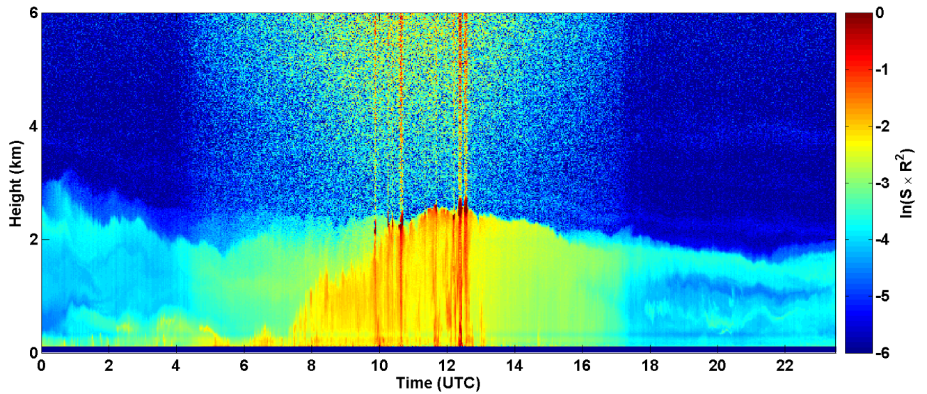
2017-08-31 RCS quick look CHM15k - ILVA LIDAR2 PARCHI
