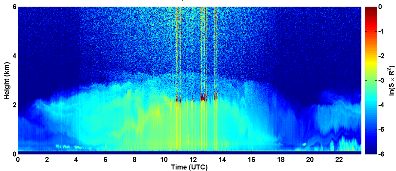
2017-08-17 RCS quick look CHM15k - ILVA LIDAR3 AGGLOMERATO
