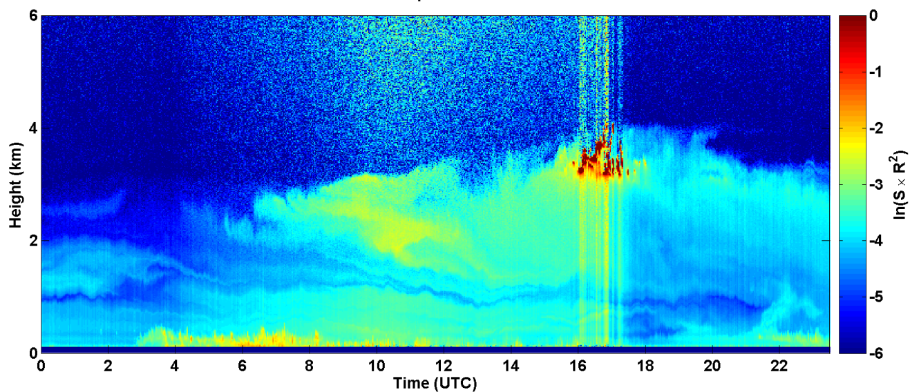
2017-08-20 RCS quick look CHM15k - ILVA LIDAR3 AGGLOMERATO
