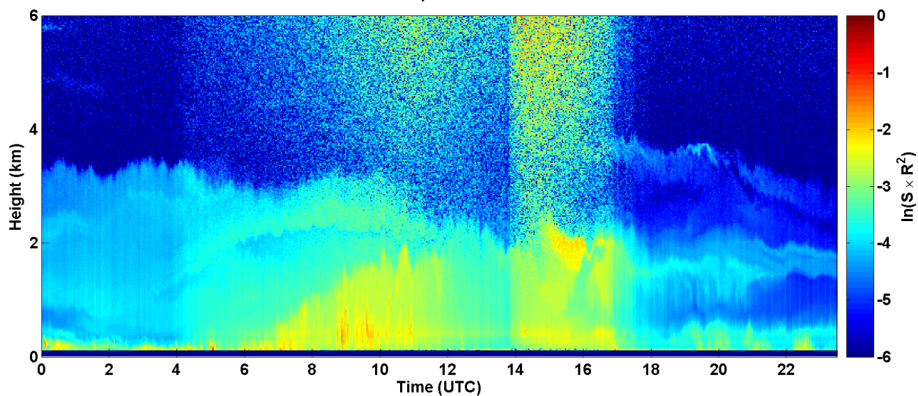
2017-08-08 RCS quick look CHM15k - ILVA LIDAR3 AGGLOMERATO
