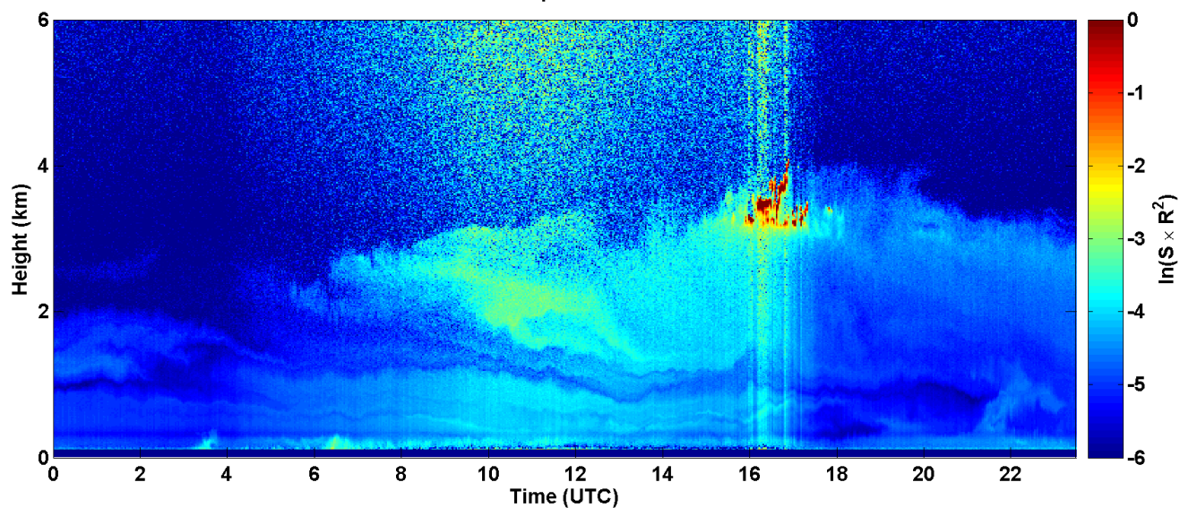
2017-08-19 RCS quick look CHM15k - ILVA LIDAR2 PARCHI
