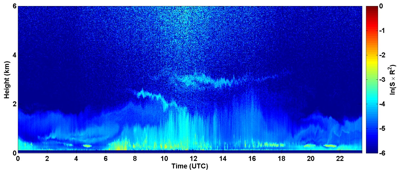
2017-08-16 RCS quick look CHM15k - ILVA LIDAR3 AGGLOMERATO
