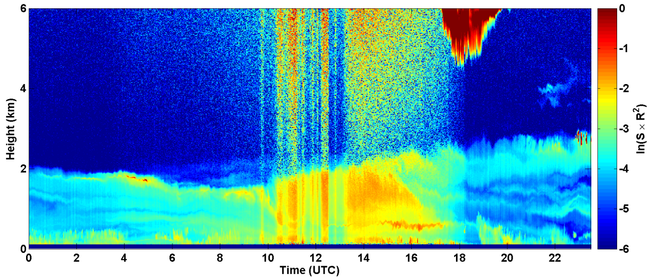
2017-06-10 RCS quick look CHM15k - ILVA LIDAR3 AGGLOMERATO
