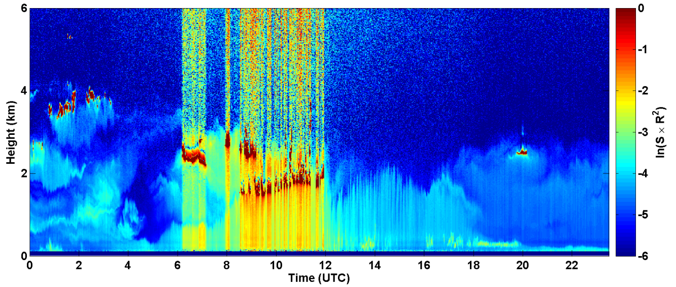
2017-06-12 RCS quick look CHM15k - ILVA LIDAR3 AGGLOMERATO
