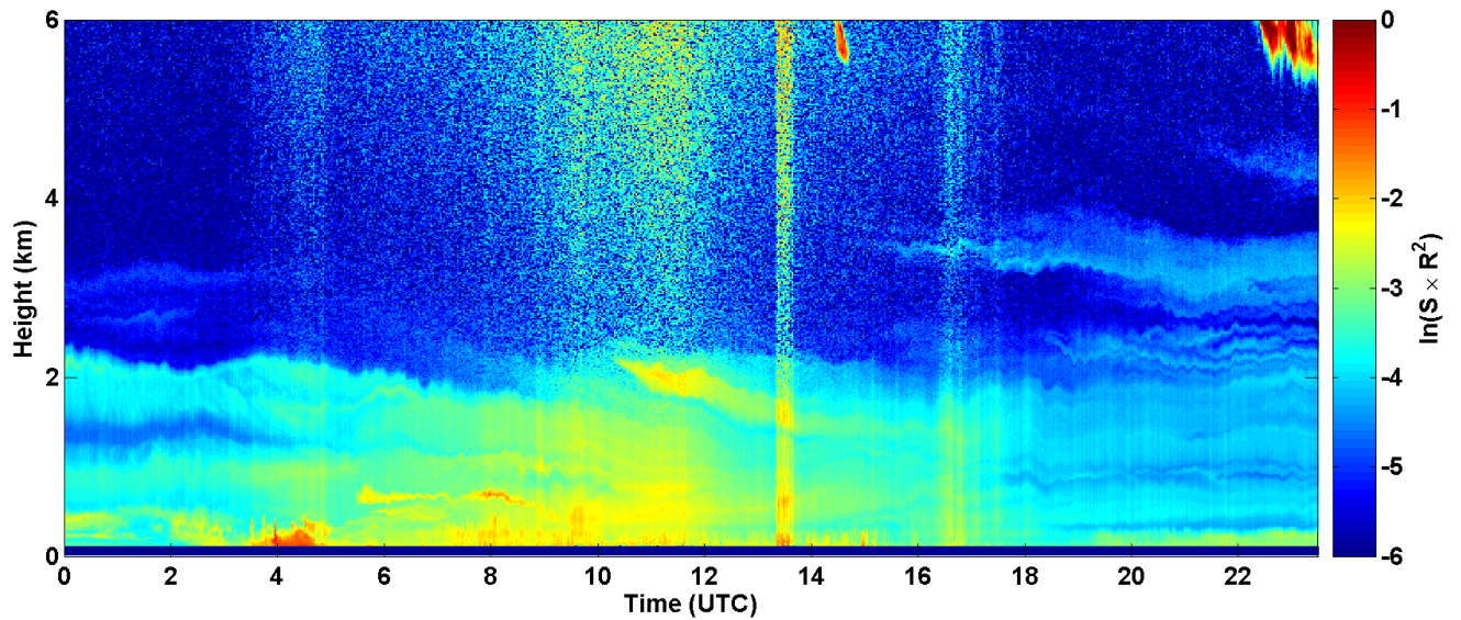
2017-06-06 RCS quick look CHM15k - ILVA LIDAR3 AGGLOMERATO
