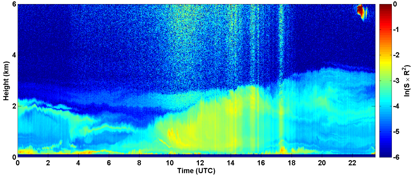
2017-06-02 RCS quick look CHM15k - ILVA LIDAR3 AGGLOMERATO
