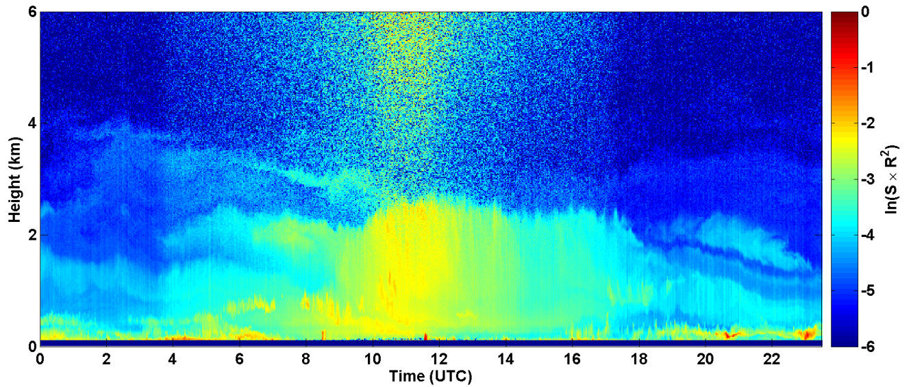
2017-06-24 RCS quick look CHM15k - ILVA LIDAR3 AGGLOMERATO
