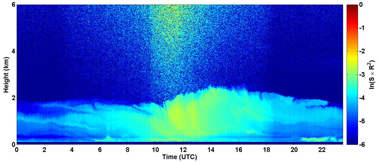
2017-06-14 RCS quick look CHM15k - ILVA LIDAR2 PARCHI
