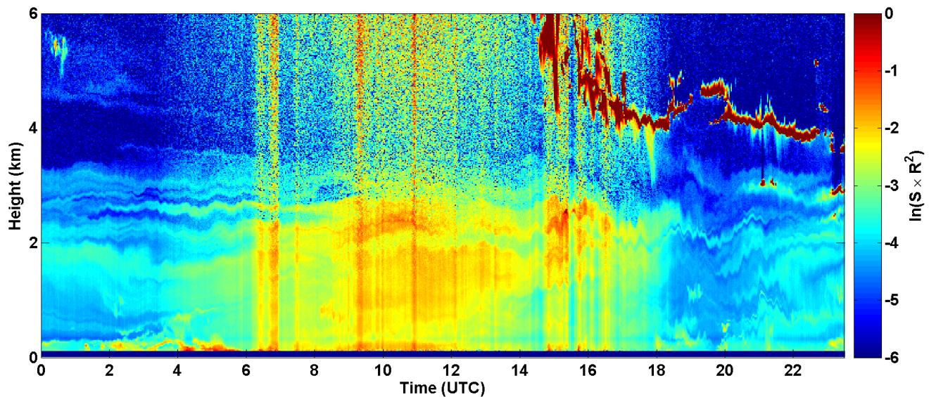
2017-06-02 RCS quick look CHM15k - ILVA LIDAR2 PARCHI
