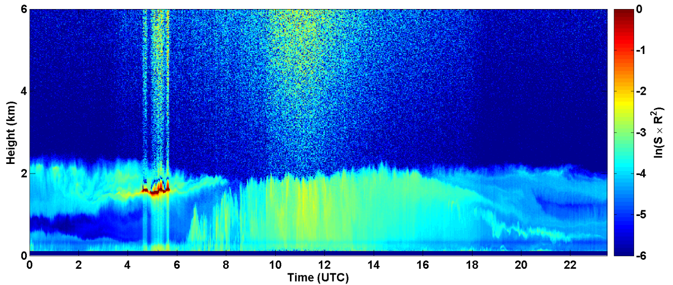
2017-06-10 RCS quick look CHM15k - ILVA LIDAR2 PARCHI
