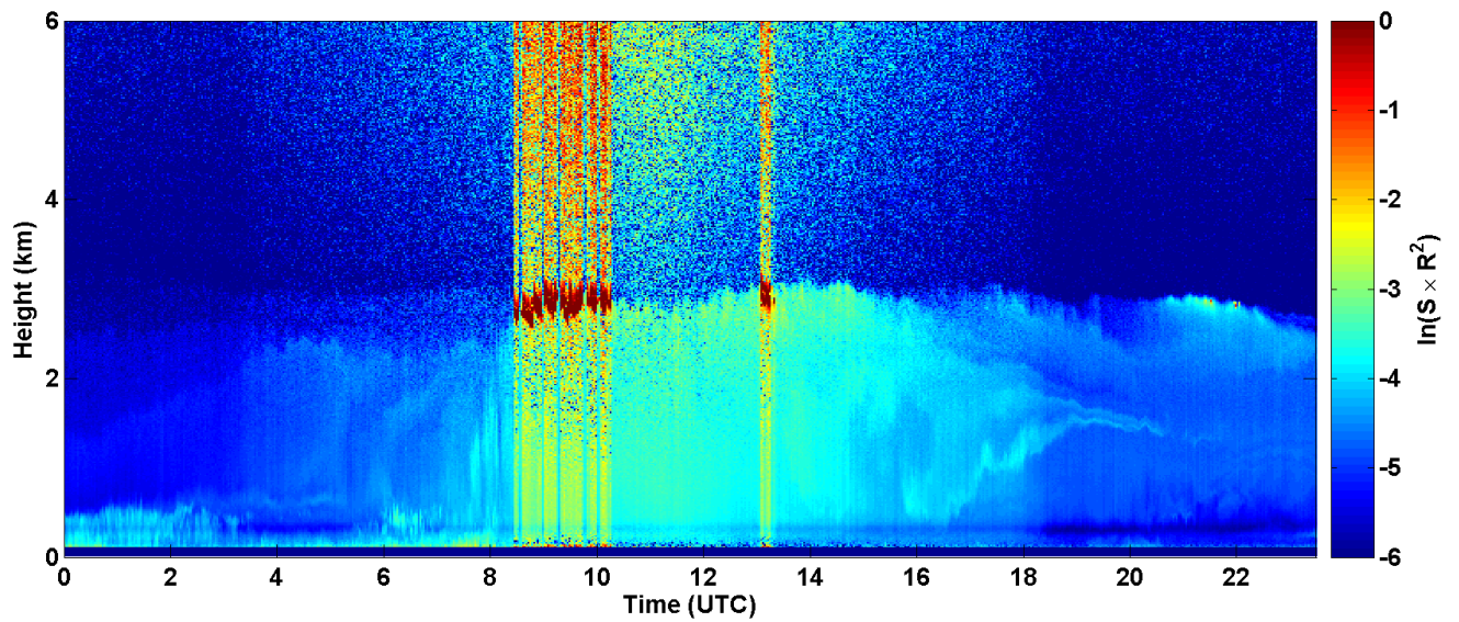
2017-06-20 RCS quick look CHM15k - ILVA LIDAR2 PARCHI
