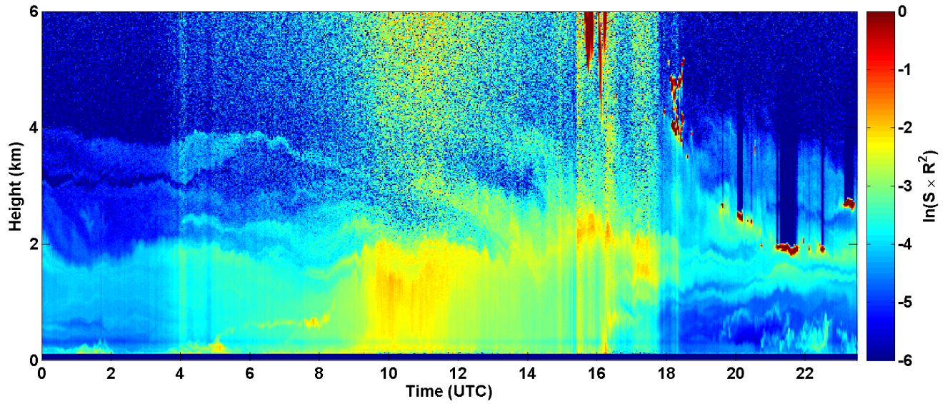
2017-06-16 RCS quick look CHM15k - ILVA LIDAR2 PARCHI
