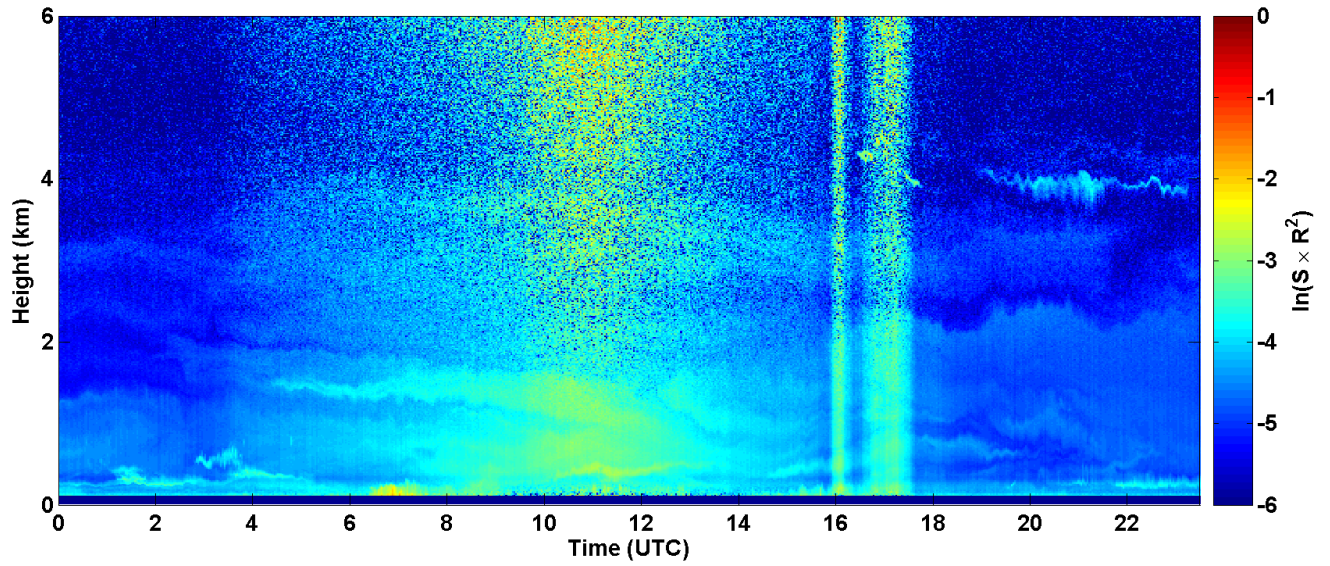
2017-06-26 RCS quick look CHM15k - ILVA LIDAR2 PARCHI
