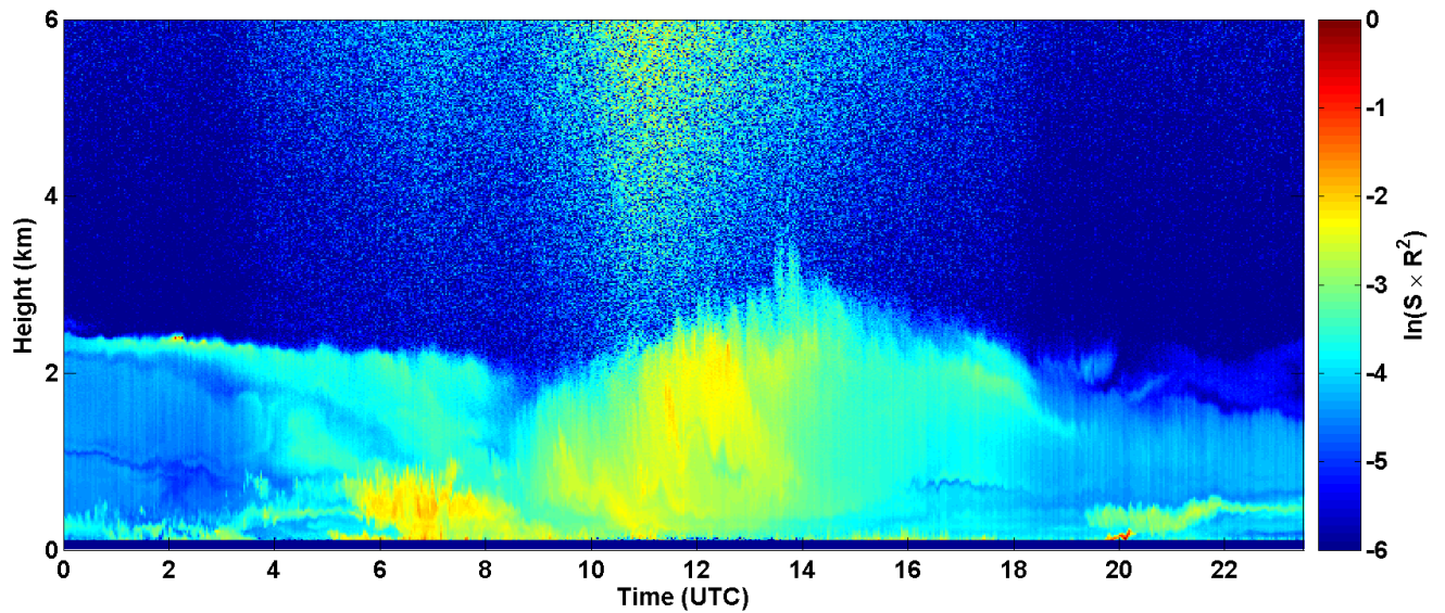
2017-06-22 RCS quick look CHM15k - ILVA LIDAR3 AGGLOMERATO
