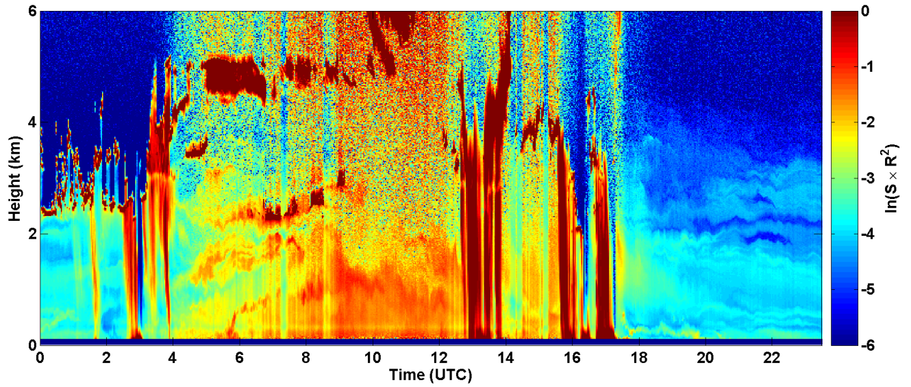
2017-06-04 RCS quick look CHM15k - ILVA LIDAR2 PARCHI
