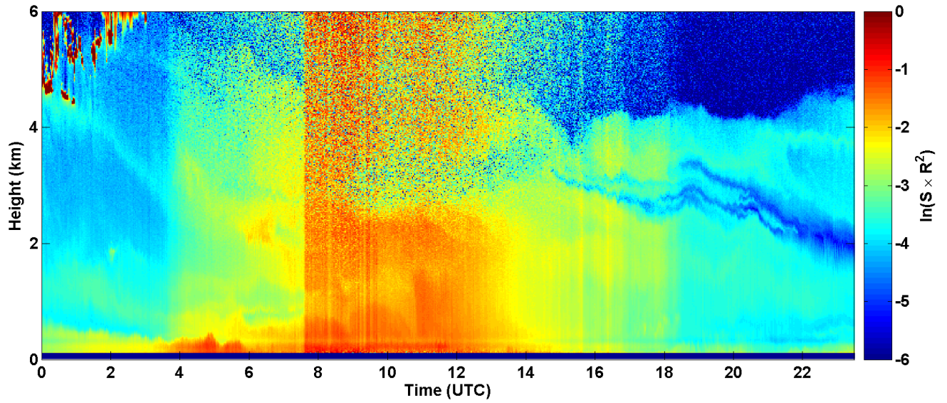
2017-06-30 RCS quick look CHM15k - ILVA LIDAR2 PARCHI
