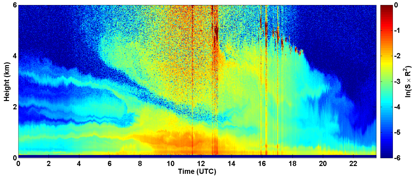
2017-06-28 RCS quick look CHM15k - ILVA LIDAR2 PARCHI
