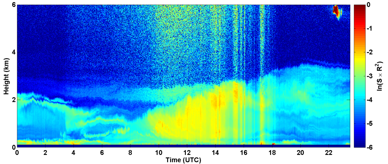
2017-06-02 RCS quick look CHM15k - ILVA LIDAR2 PARCHI
