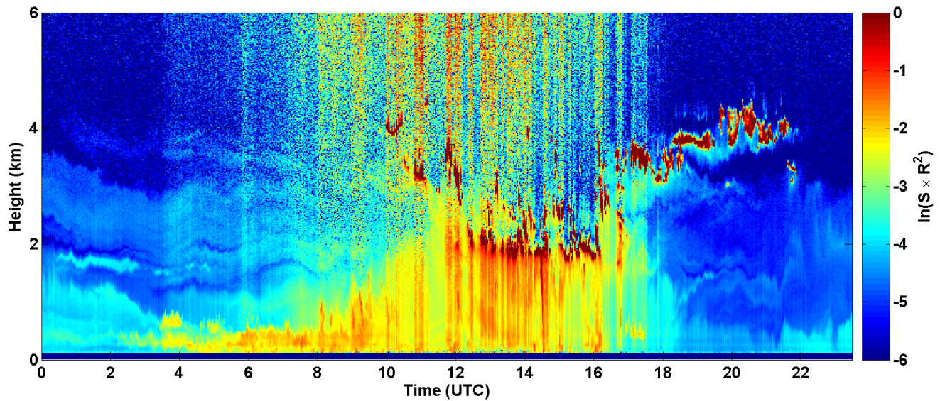
2017-06-18 RCS quick look CHM15k - ILVA LIDAR3 AGGLOMERATO
