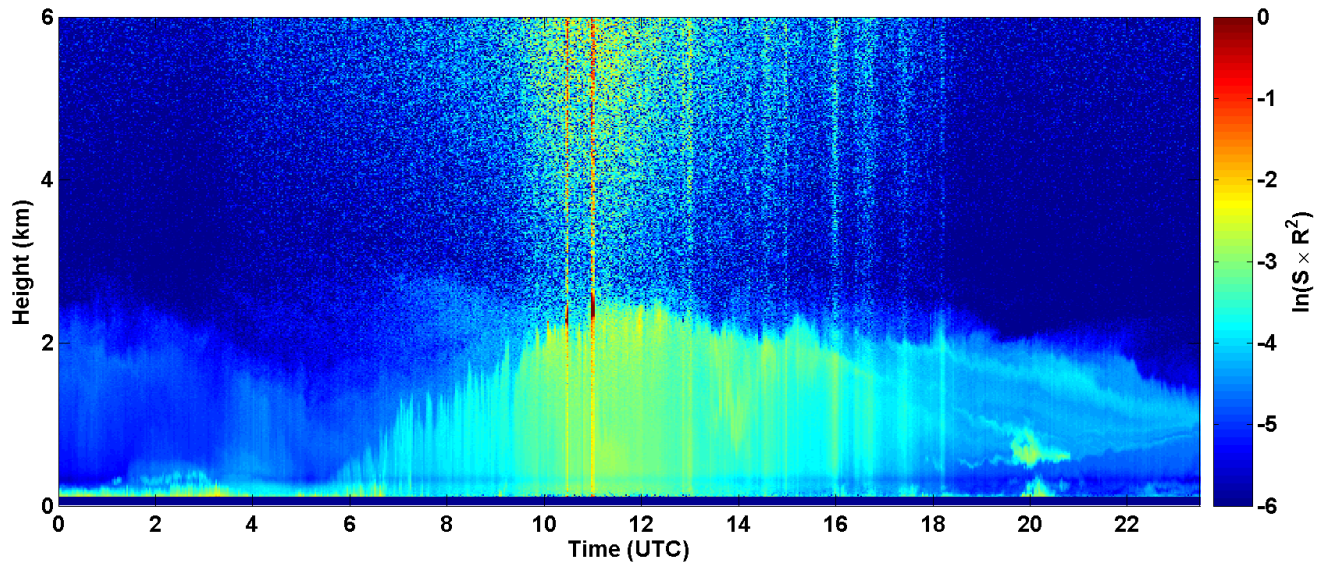
2017-06-12 RCS quick look CHM15k - ILVA LIDAR2 PARCHI
