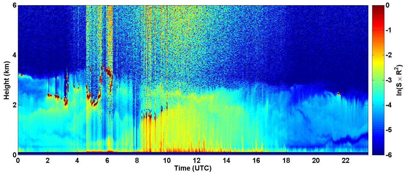
2017-06-08 RCS quick look CHM15k - ILVA LIDAR2 PARCHI
