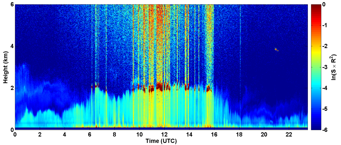
2017-06-18 RCS quick look CHM15k - ILVA LIDAR2 PARCHI
