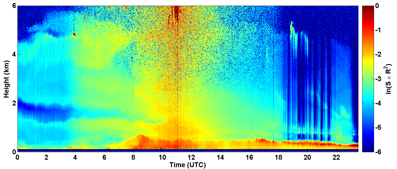
2017-06-30 RCS quick look CHM15k - ILVA LIDAR3 AGGLOMERATO
