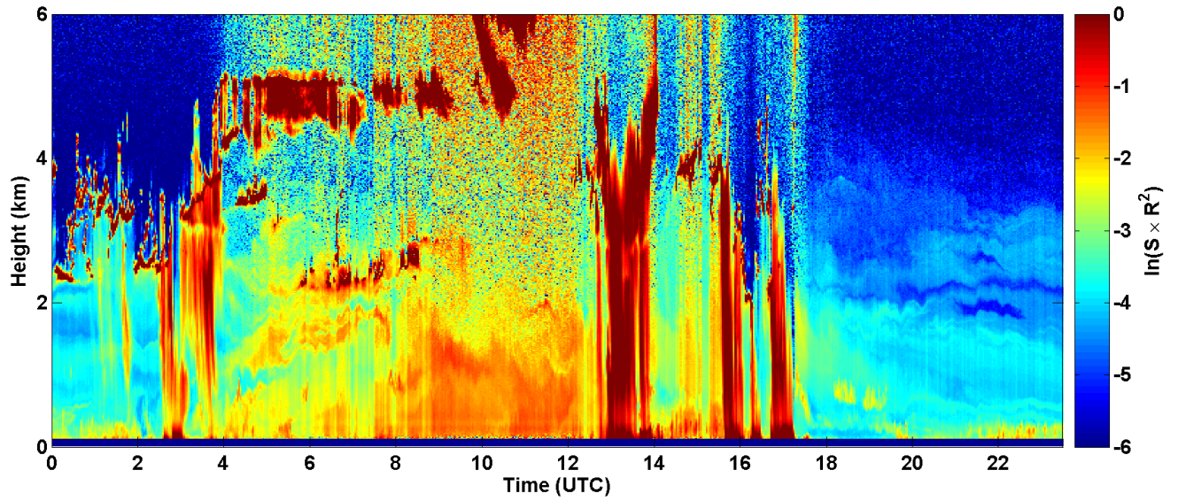
2017-06-04 RCS quick look CHM15k - ILVA LIDAR3 AGGLOMERATO
