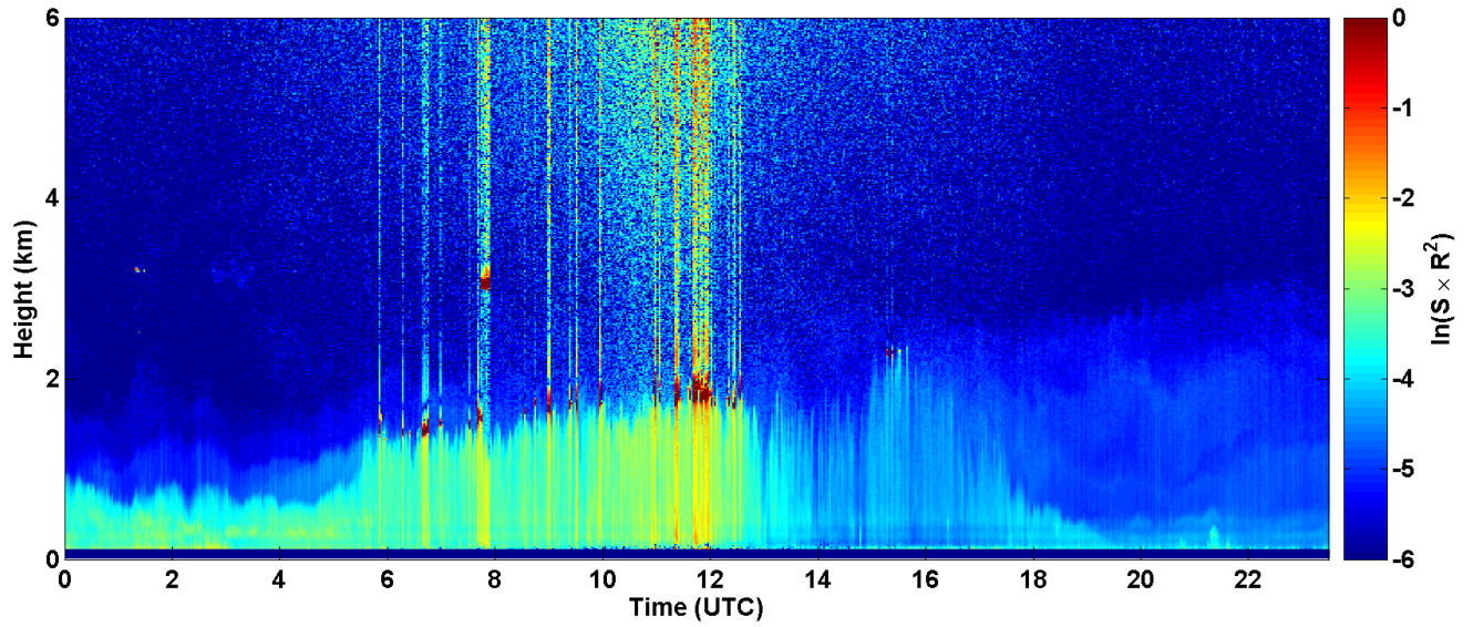
2017-06-20 RCS quick look CHM15k - ILVA LIDAR3 AGGLOMERATO
