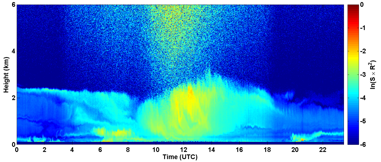
2017-06-22 RCS quick look CHM15k - ILVA LIDAR2 PARCHI
