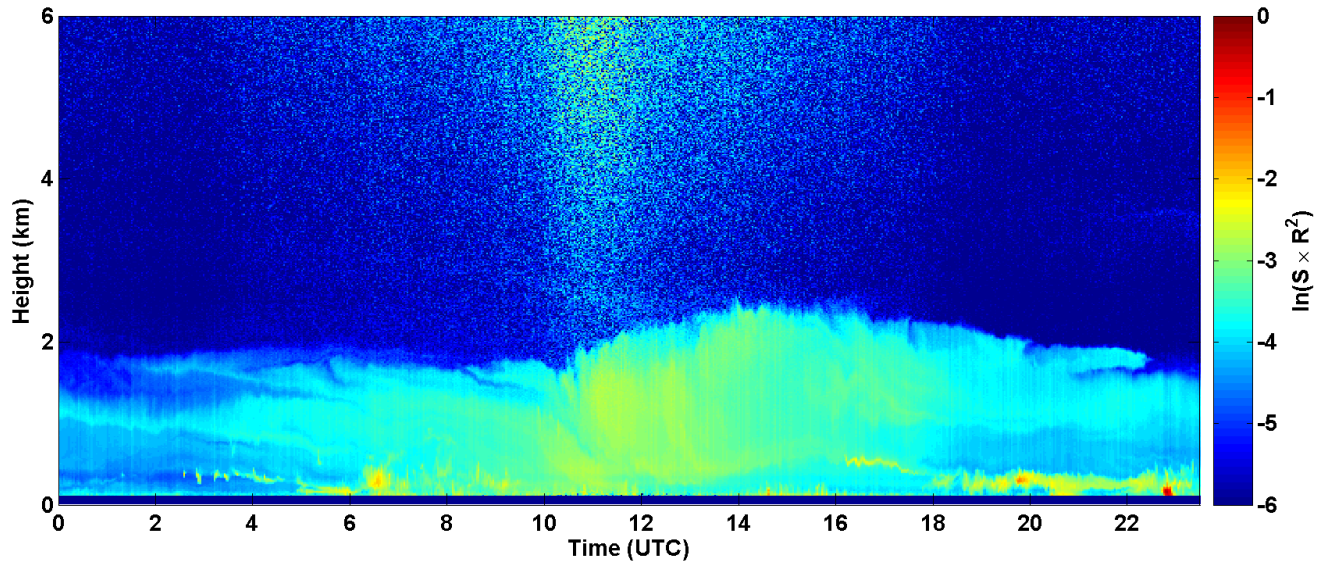
2017-06-14 RCS quick look CHM15k - ILVA LIDAR3 AGGLOMERATO
