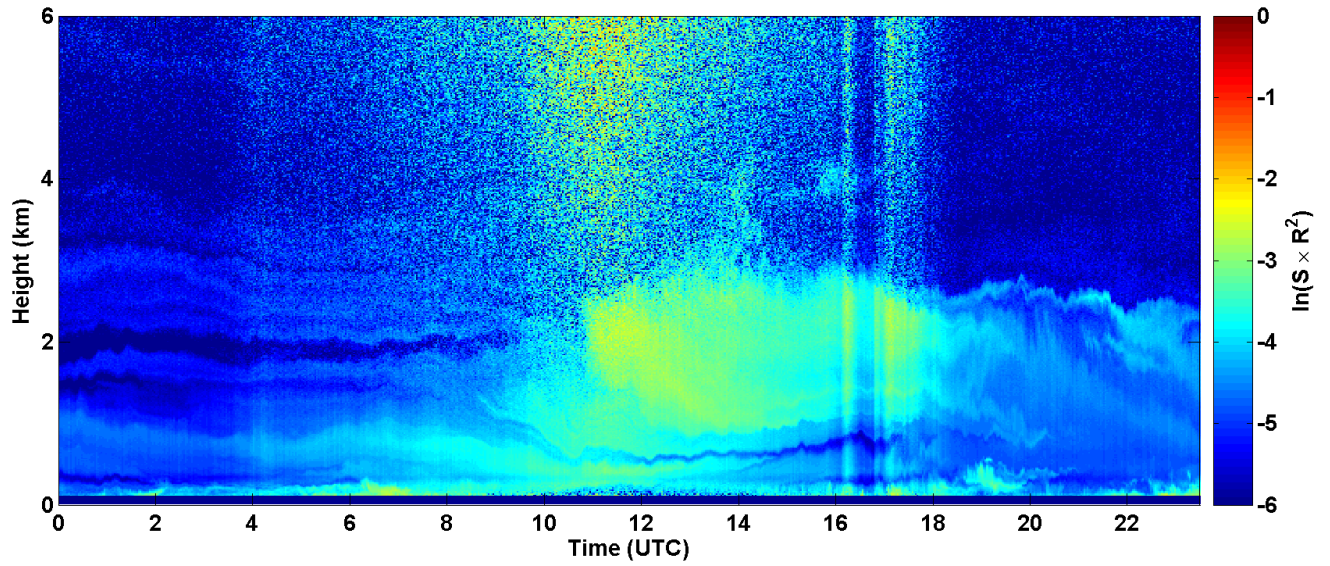
2017-06-24 RCS quick look CHM15k - ILVA LIDAR2 PARCHI
