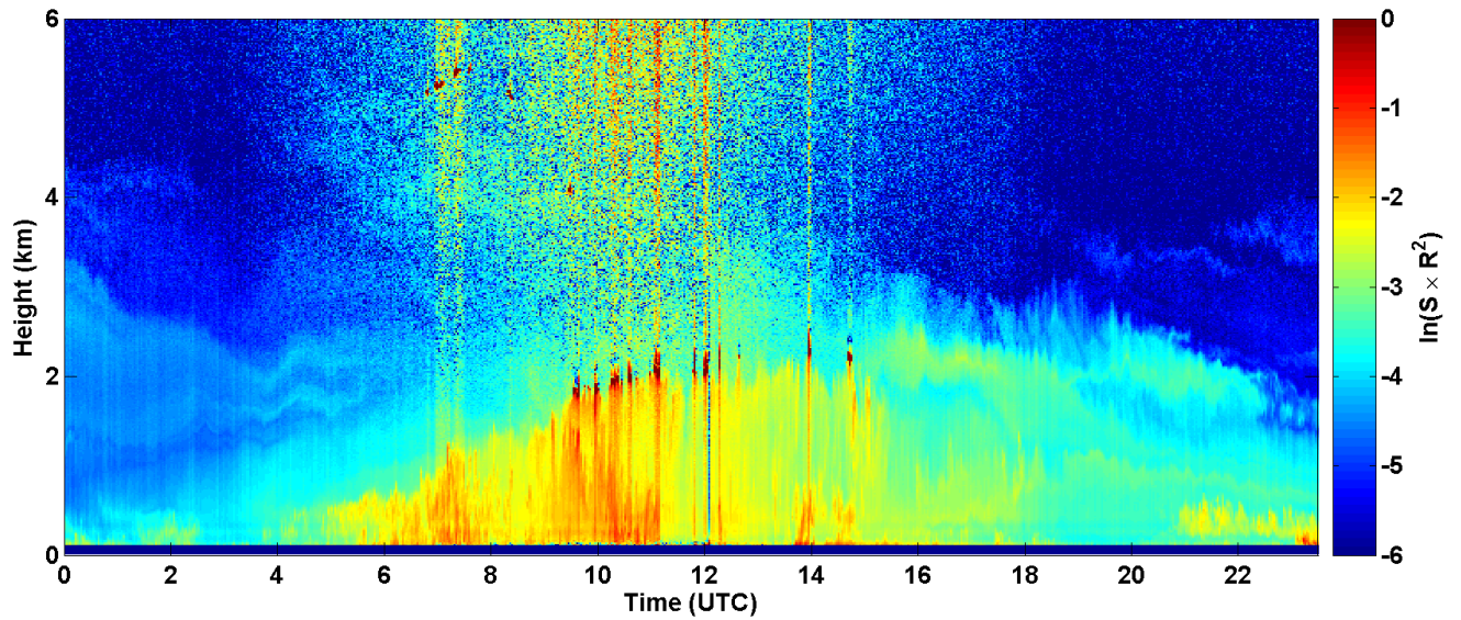
2017-06-26 RCS quick look CHM15k - ILVA LIDAR3 AGGLOMERATO
