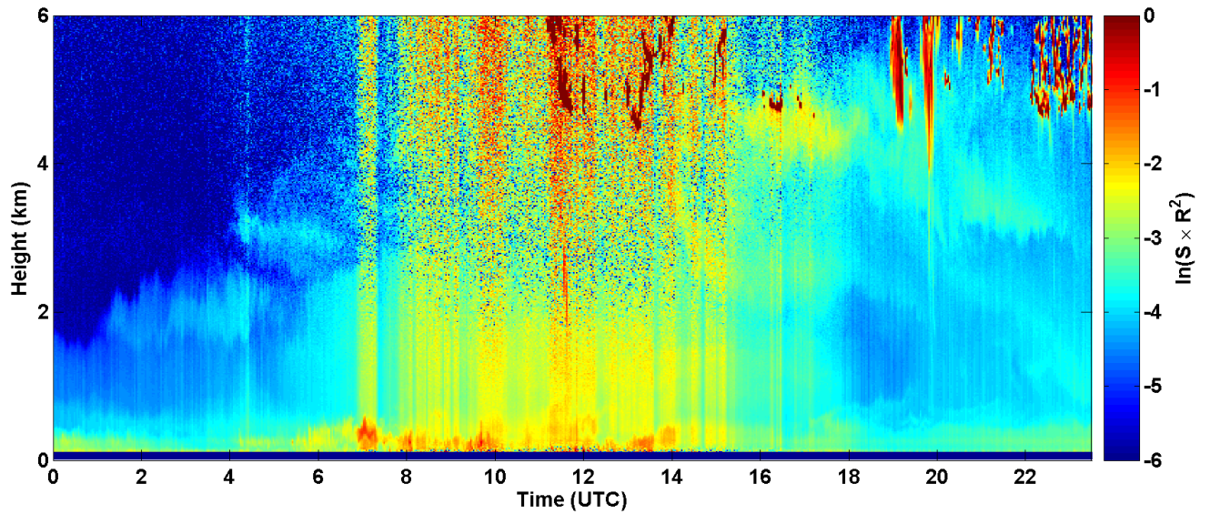
2017-06-28 RCS quick look CHM15k - ILVA LIDAR3 AGGLOMERATO
