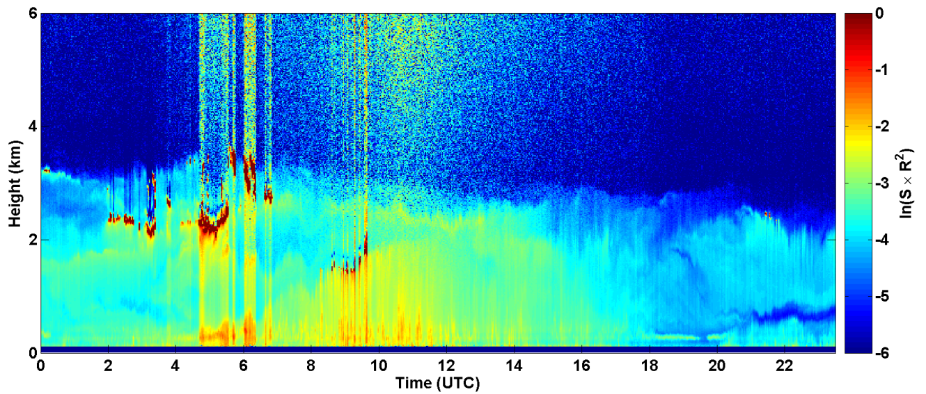
2017-06-08 RCS quick look CHM15k - ILVA LIDAR3 AGGLOMERATO
