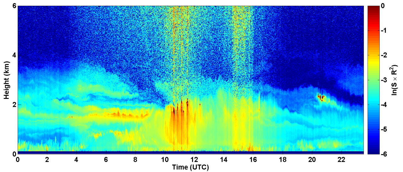
2017-06-16 RCS quick look CHM15k - ILVA LIDAR3 AGGLOMERATO
