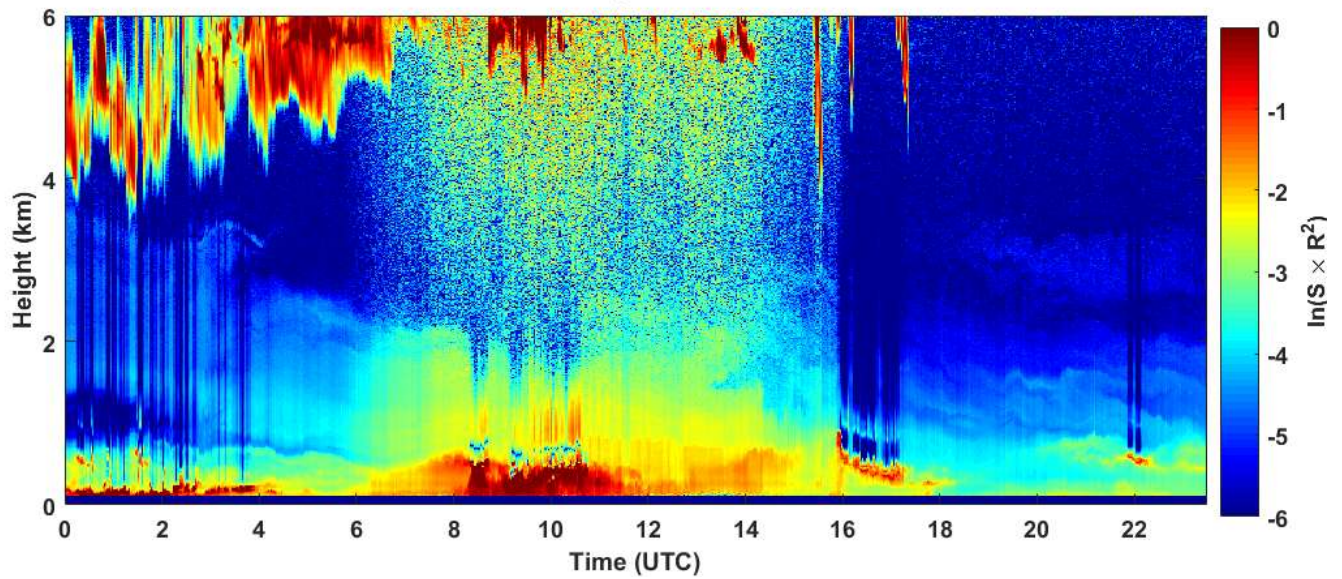
2018-11-04 RCS quick look CHM15k - ILVA LIDAR3 AGGLOMERATO
