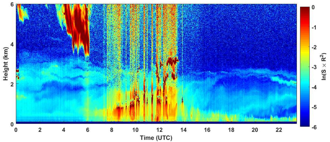
2018-11-09 RCS quick look CHM15k - ILVA LIDAR2 PARCHI
