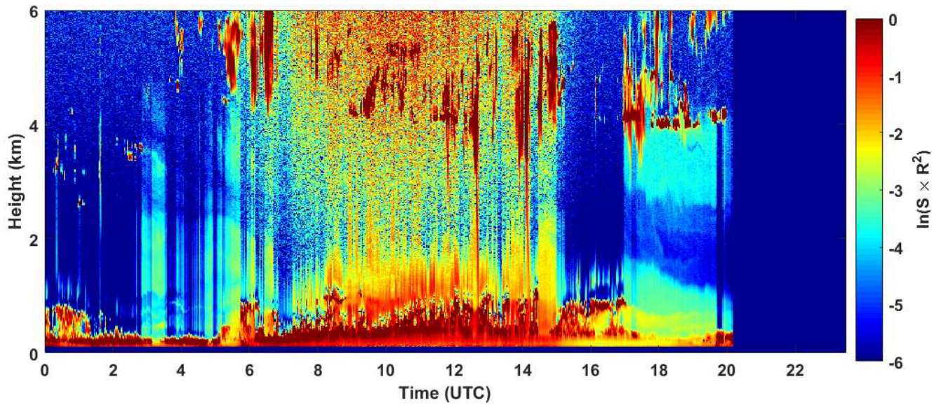
2018-11-02 RCS quick look CHM15k - ILVA LIDAR2 PARCHI
