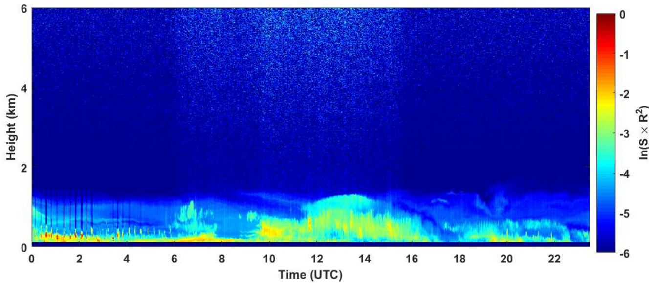
2018-11-14 RCS quick look CHM15k - ILVA LIDAR3 AGGLOMERATO
