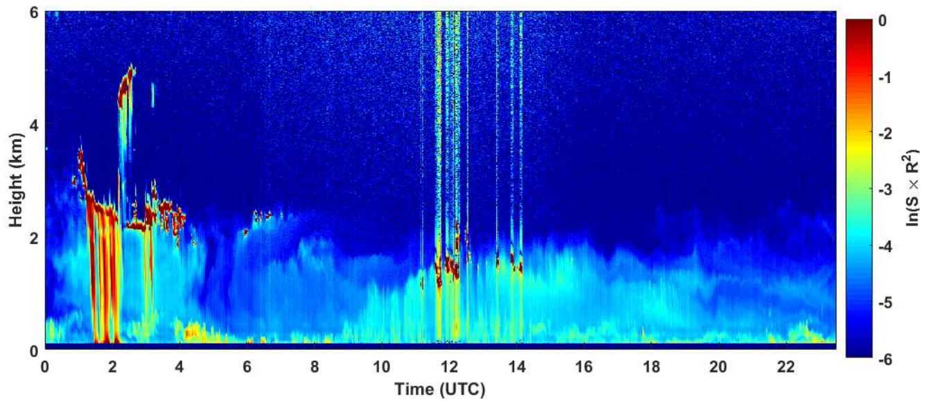
2018-11-22 RCS quick look CHM15k - ILVA LIDAR3 AGGLOMERATO
