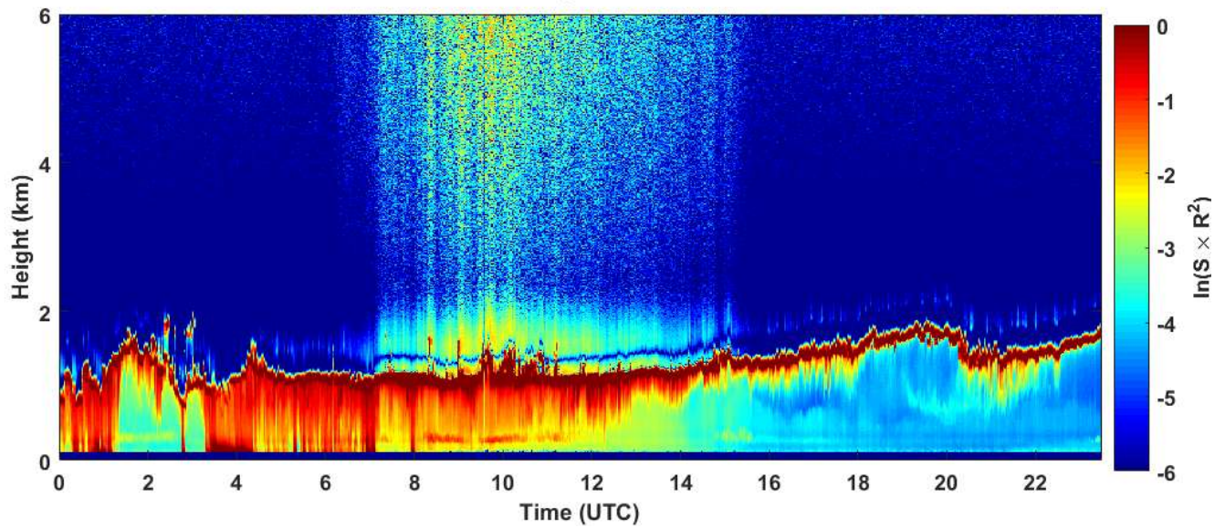
2018-11-30 RCS quick look CHM15k - ILVA LIDAR3 AGGLOMERATO
