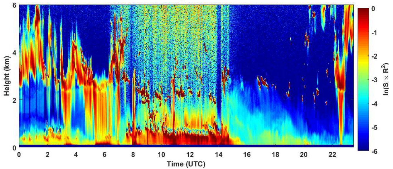
2018-11-26 RCS quick look CHM15k - ILVA LIDAR3 AGGLOMERATO
