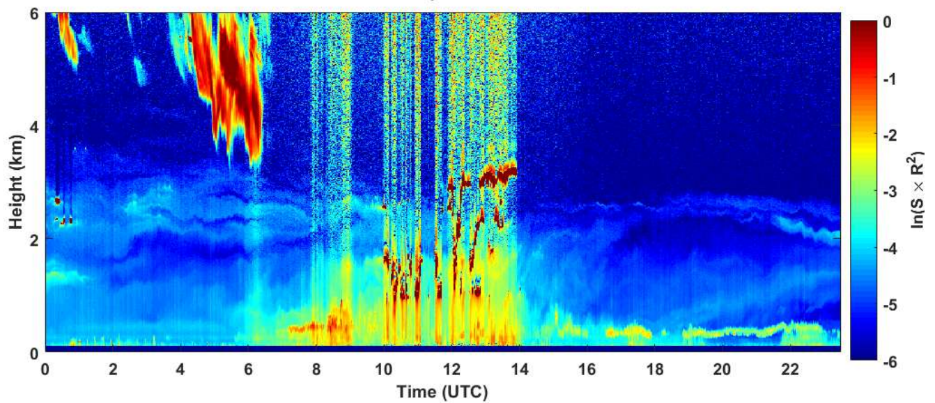
2018-11-08 RCS quick look CHM15k - ILVA LIDAR3 AGGLOMERATO
