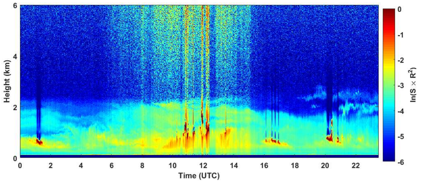
2018-11-11 RCS quick look CHM15k - ILVA LIDAR2 PARCHI
