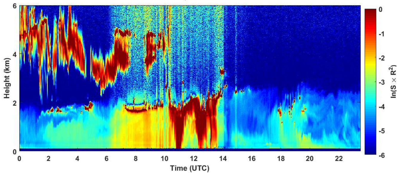
2018-11-16 RCS quick look CHM15k - ILVA LIDAR3 AGGLOMERATO
