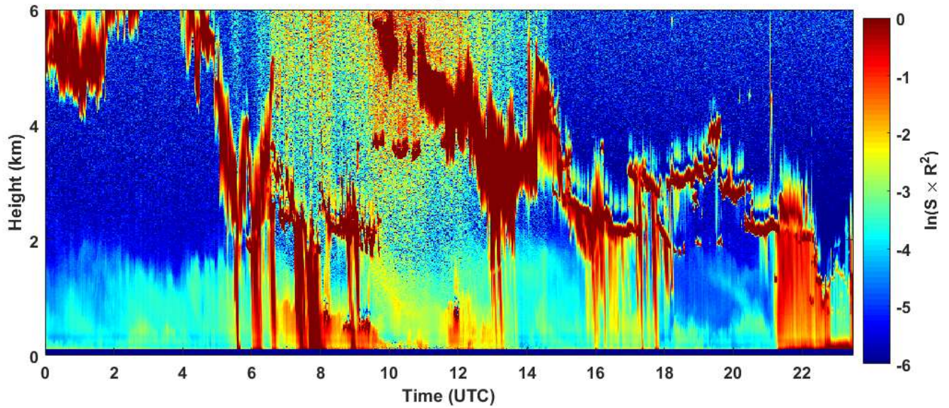
2018-11-27 RCS quick look CHM15k - ILVA LIDAR2 PARCHI
