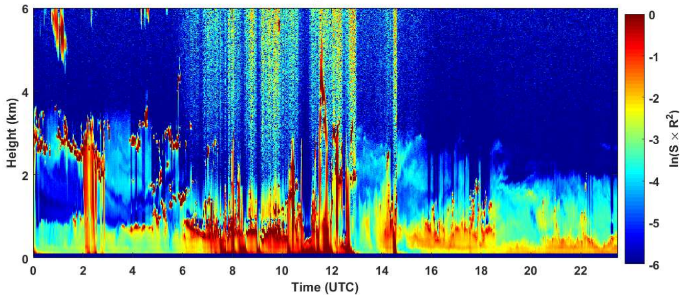
2018-11-06 RCS quick look CHM15k - ILVA LIDAR3 AGGLOMERATO
