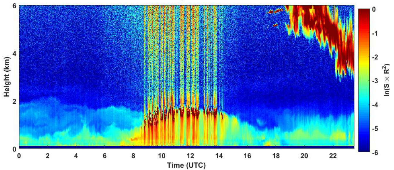
2018-11-15 RCS quick look CHM15k - ILVA LIDAR2 PARCHI
