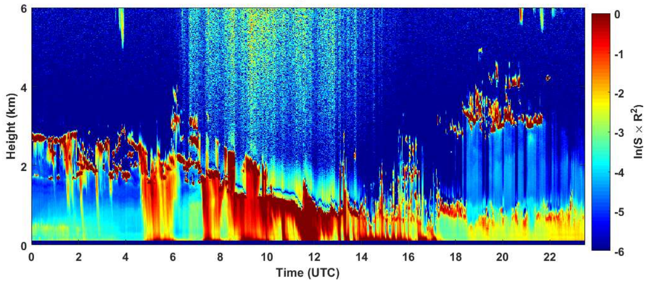
2018-11-20 RCS quick look CHM15k - ILVA LIDAR3 AGGLOMERATO
