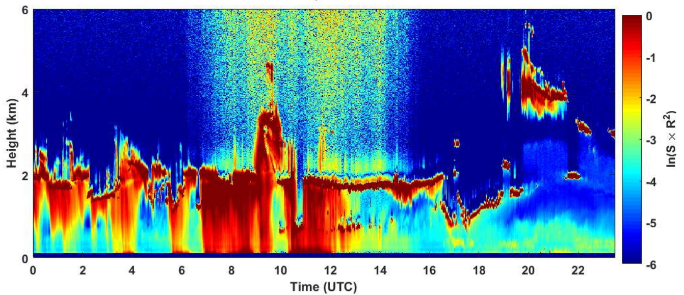
2018-11-18 RCS quick look CHM15k - ILVA LIDAR3 AGGLOMERATO
