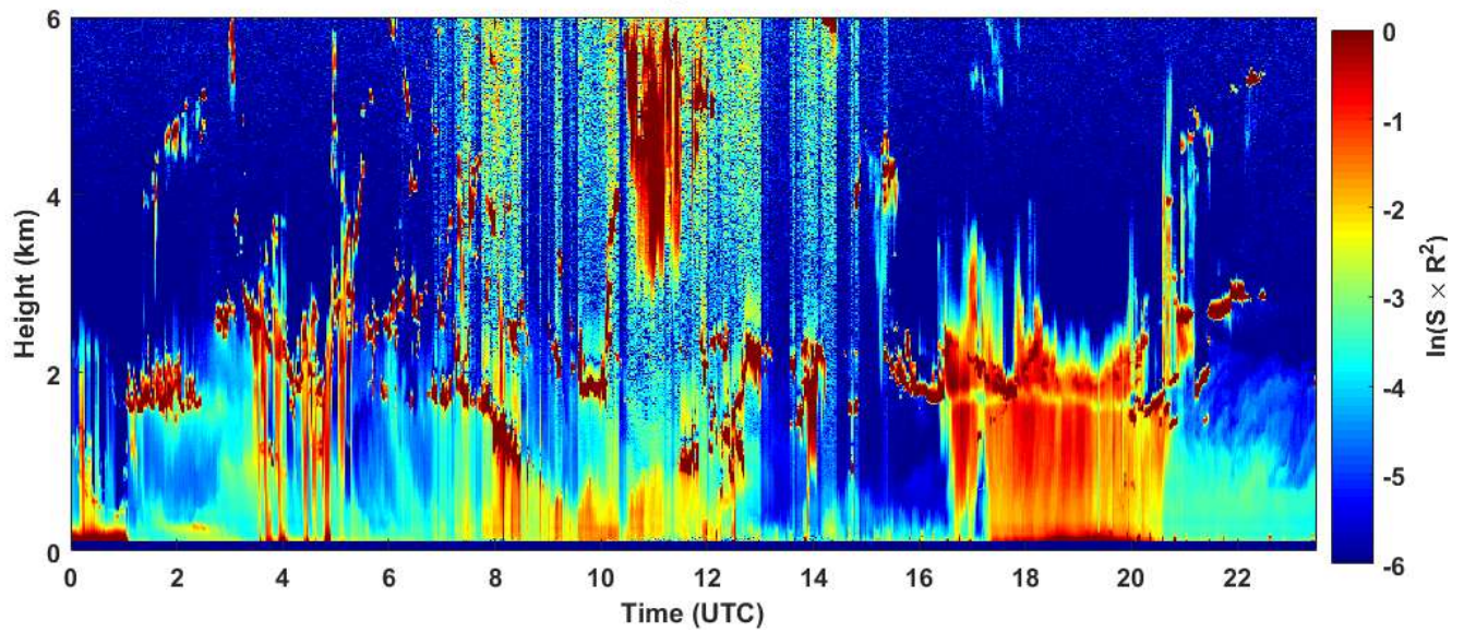
2018-11-28 RCS quick look CHM15k - ILVA LIDAR3 AGGLOMERATO
