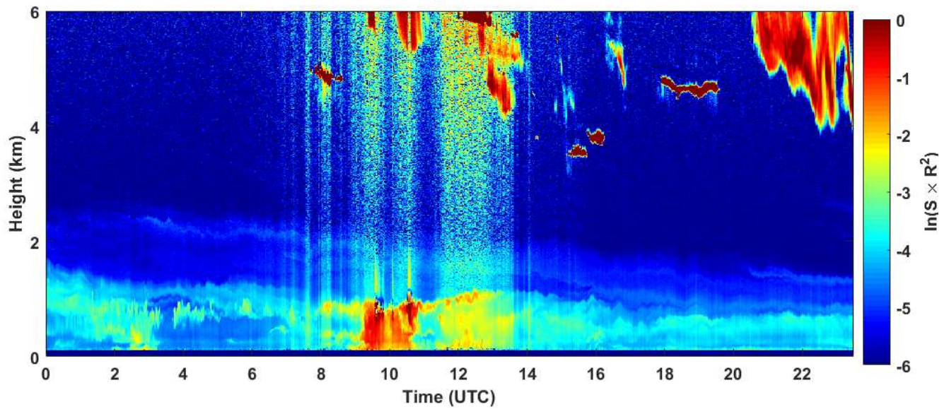
2018-11-24 RCS quick look CHM15k - ILVA LIDAR3 AGGLOMERATO
