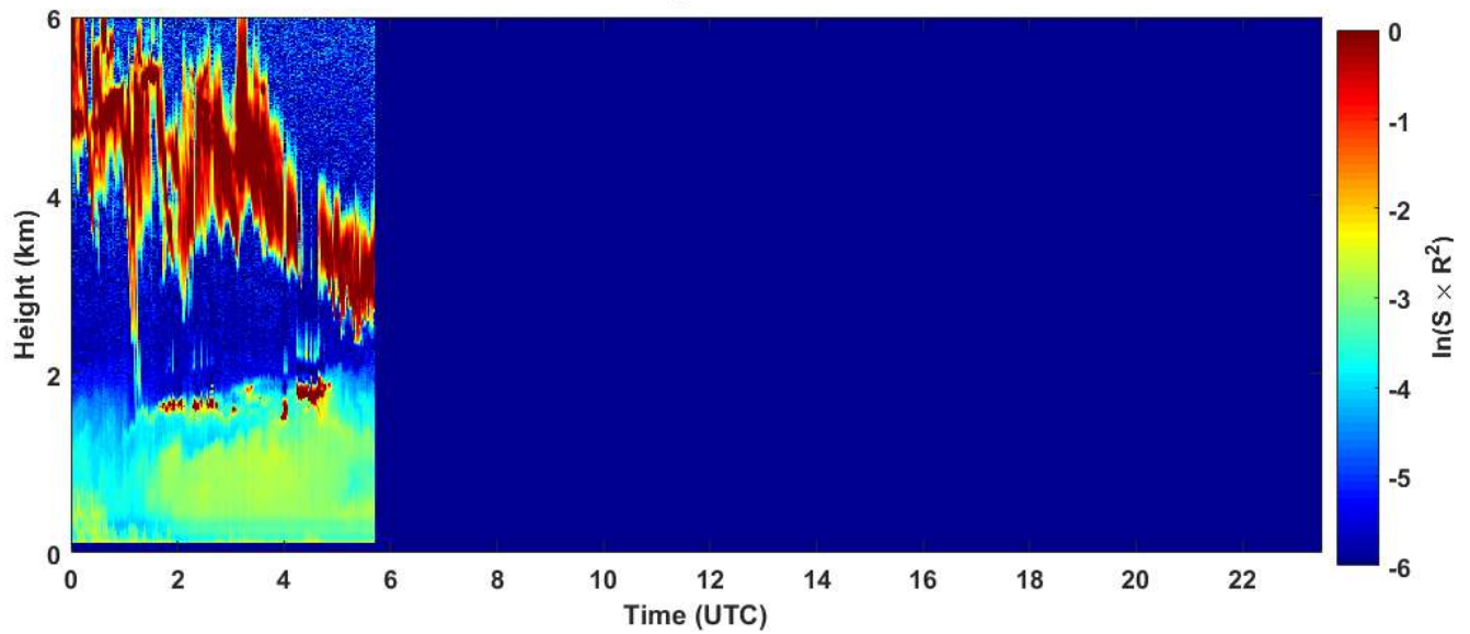
2018-11-23 RCS quick look CHM15k - ILVA LIDAR2 PARCHI
