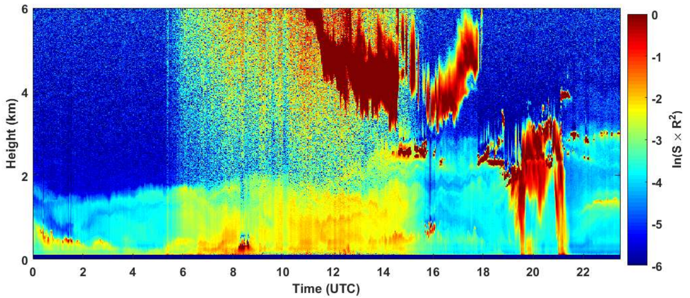
2018-11-07 RCS quick look CHM15k - ILVA LIDAR2 PARCHI
