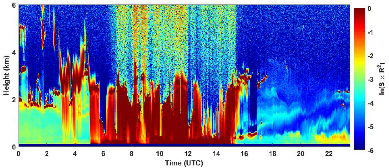
2018-10-22 RCS quick look CHM15k - ILVA LIDAR2 PARCHI
