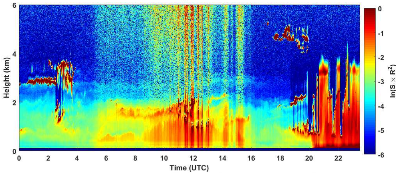
2018-10-16 RCS quick look CHM15k - ILVA LIDAR2 PARCHI
