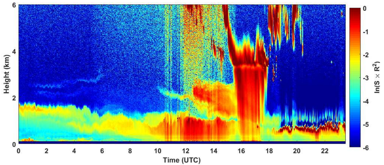
2018-10-31 RCS quick look CHM15k - ILVA LIDAR2 PARCHI
