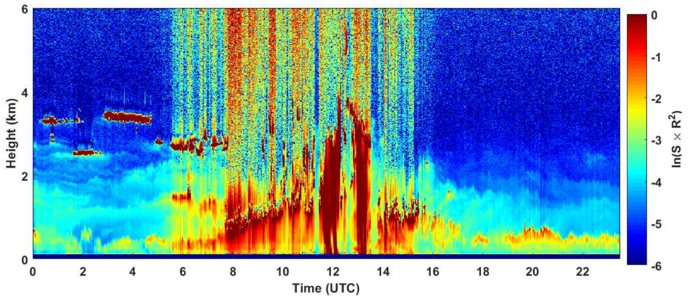
2018-10-08 RCS quick look CHM15k - ILVA LIDAR2 PARCHI
