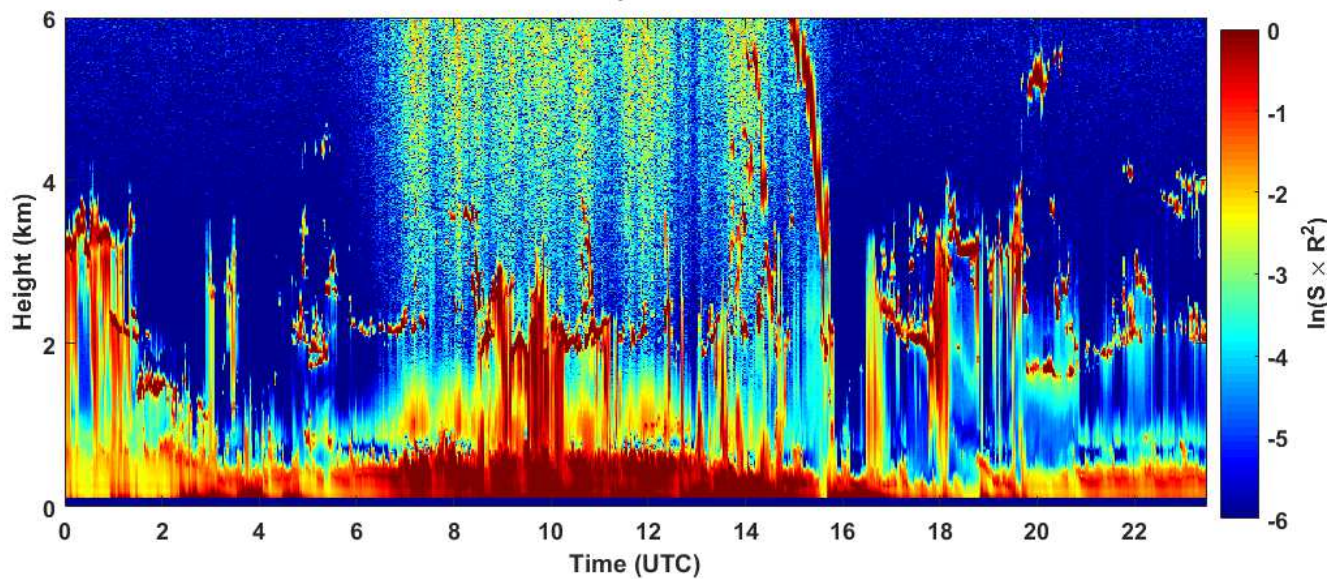
2018-10-28 RCS quick look CHM15k - ILVA LIDAR3 AGGLOMERATO
