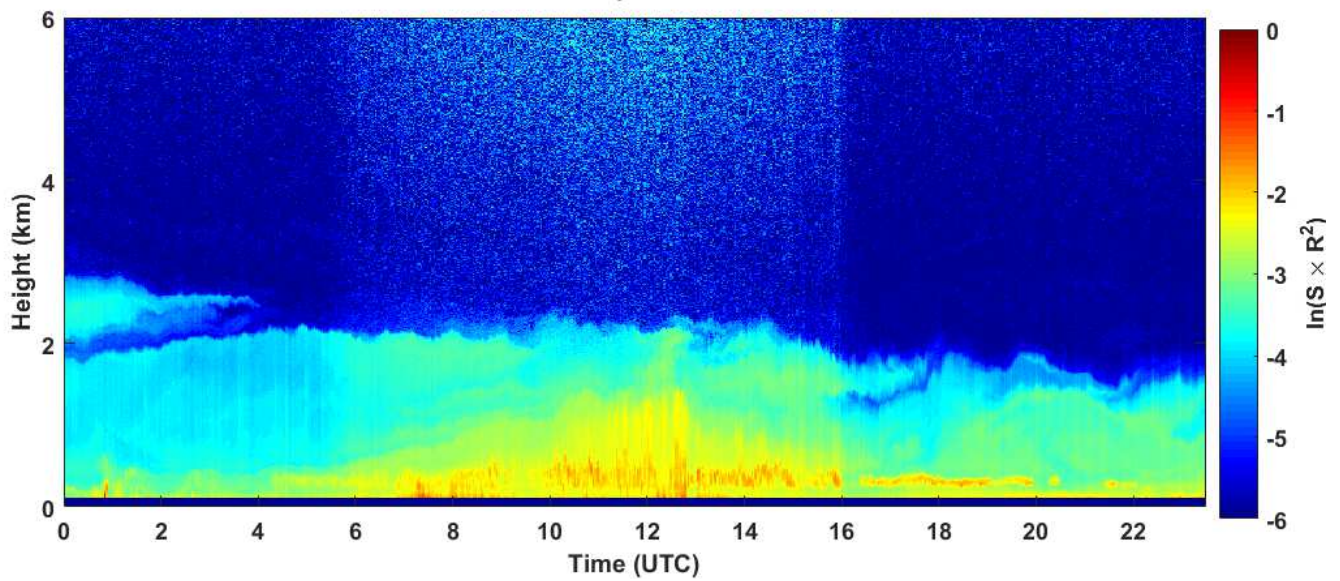
2018-10-20 RCS quick look CHM15k - ILVA LIDAR3 AGGLOMERATO
