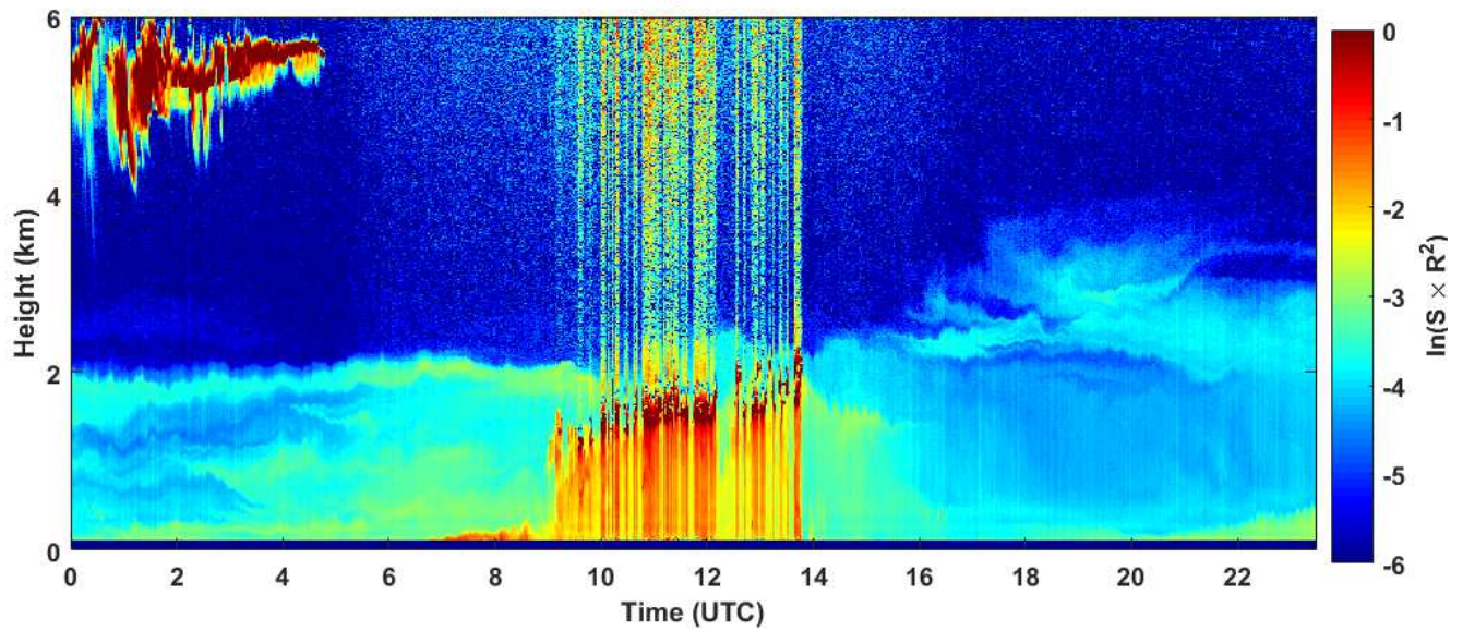
2018-10-12 RCS quick look CHM15k - ILVA LIDAR3 AGGLOMERATO
