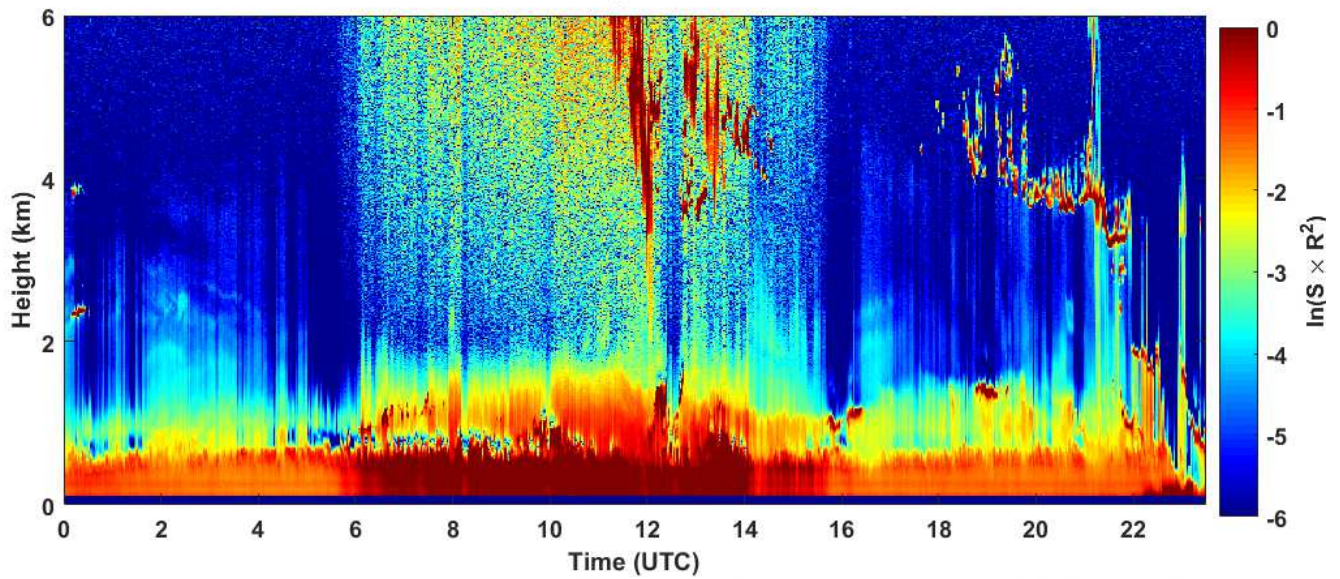
2018-10-30 RCS quick look CHM15k - ILVA LIDAR3 AGGLOMERATO
