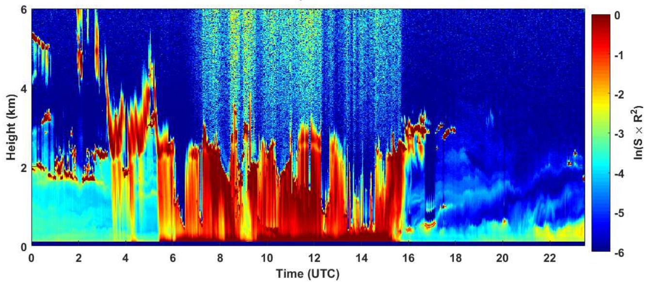
2018-10-22 RCS quick look CHM15k - ILVA LIDAR3 AGGLOMERATO
