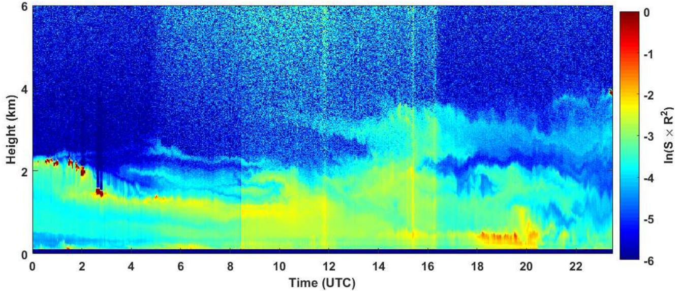
2018-10-02 RCS quick look CHM15k - ILVA LIDAR2 PARCHI
