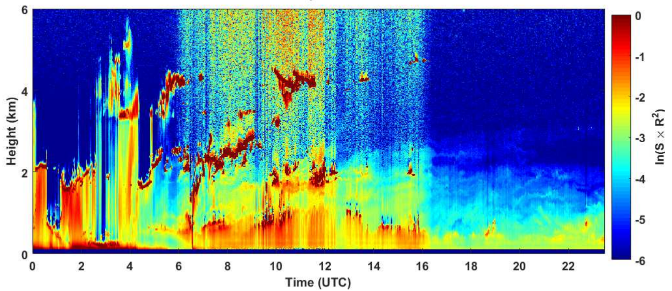
2018-10-16 RCS quick look CHM15k - ILVA LIDAR3 AGGLOMERATO
