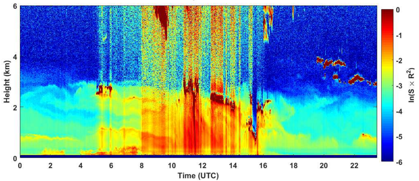
2018-10-14 RCS quick look CHM15k - ILVA LIDAR2 PARCHI
