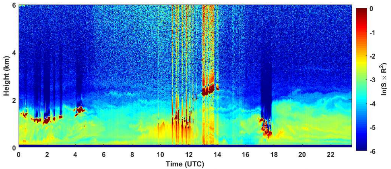
2018-10-18 RCS quick look CHM15k - ILVA LIDAR2 PARCHI
