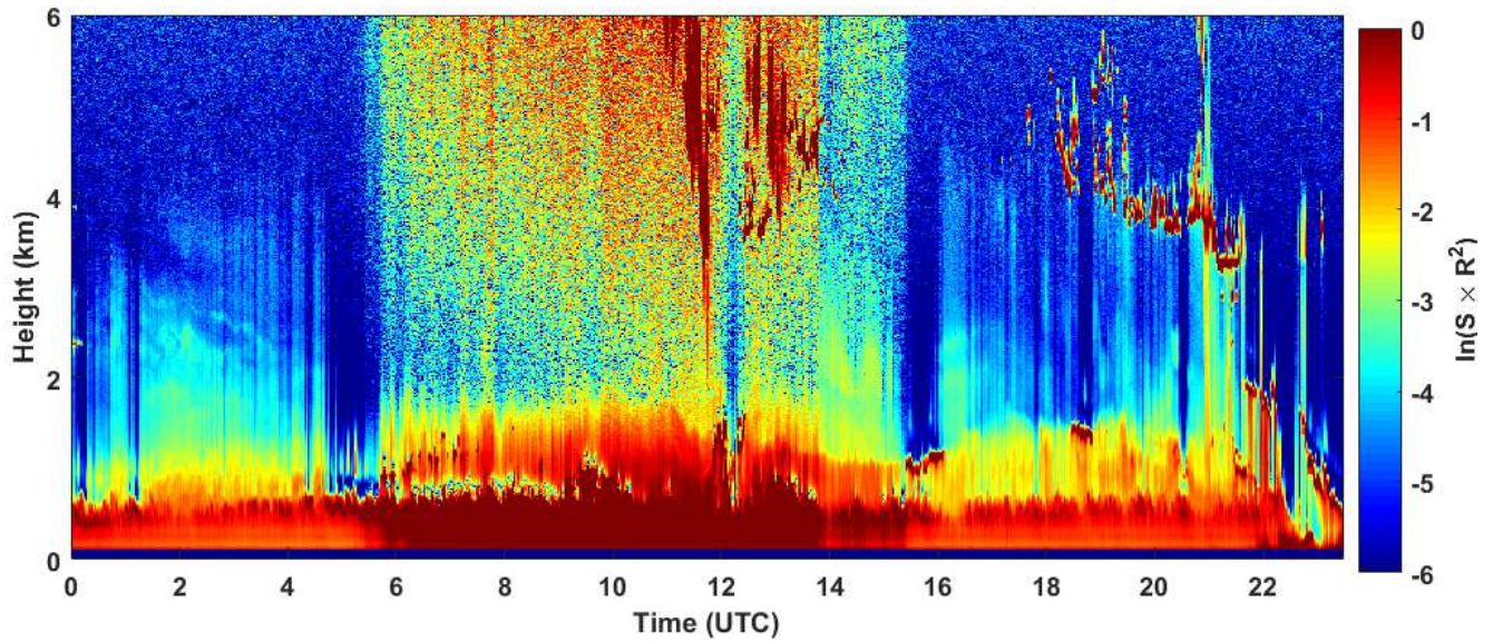
2018-10-30 RCS quick look CHM15k - ILVA LIDAR2 PARCHI
