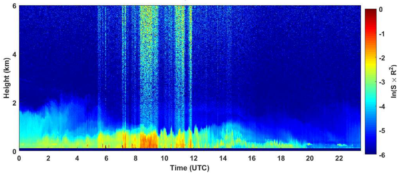
2018-10-24 RCS quick look CHM15k - ILVA LIDAR3 AGGLOMERATO
