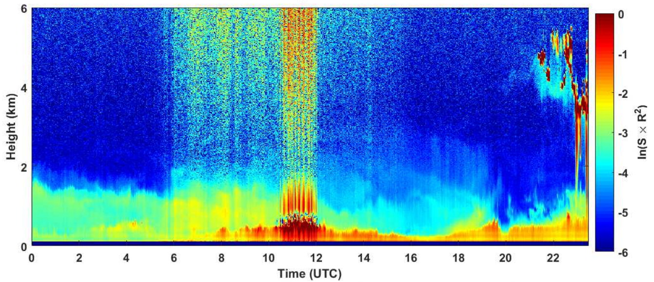
2018-10-28 RCS quick look CHM15k - ILVA LIDAR2 PARCHI
