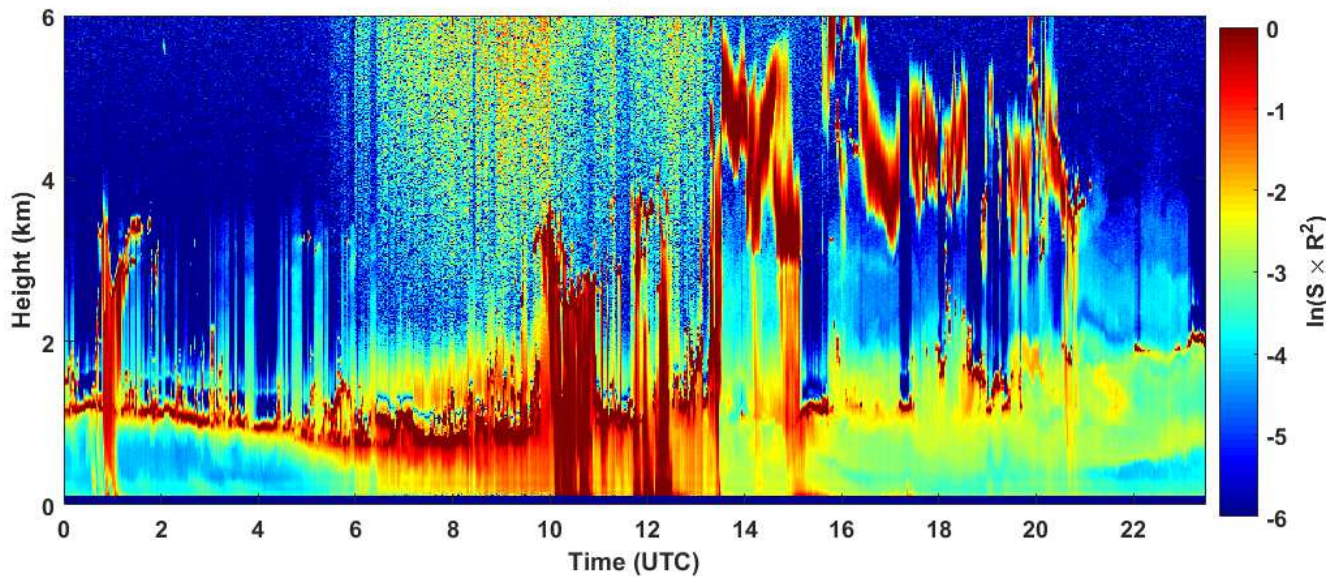
2018-10-04 RCS quick look CHM15k - ILVA LIDAR3 AGGLOMERATO
