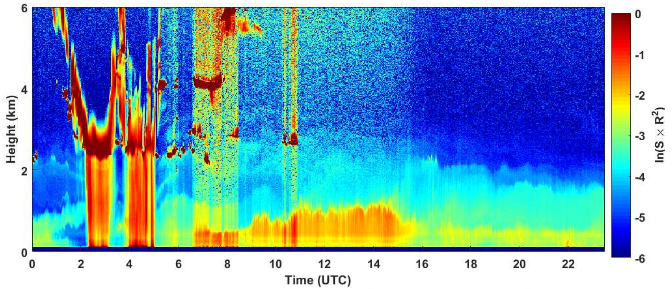
2018-10-24 RCS quick look CHM15k - ILVA LIDAR2 PARCHI
