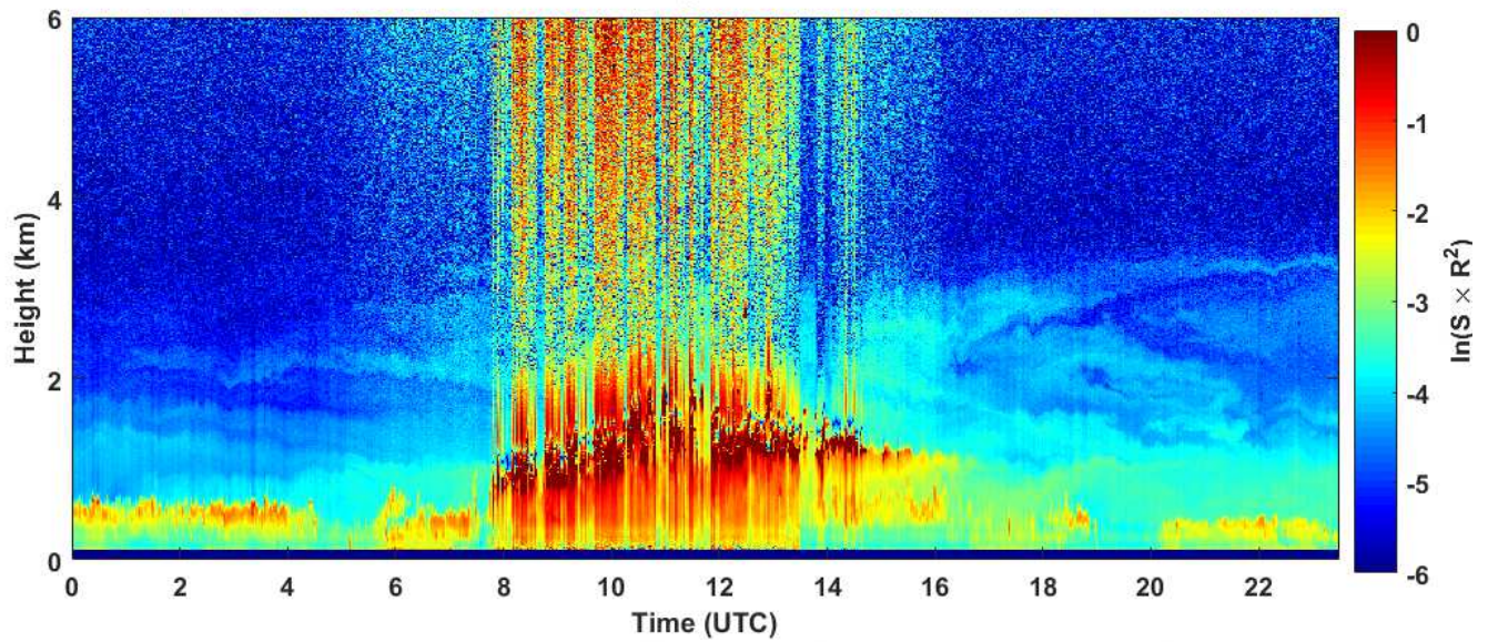
2018-10-10 RCS quick look CHM15k - ILVA LIDAR2 PARCHI
