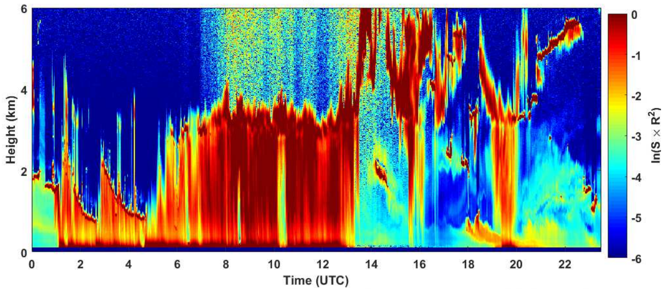
2018-10-06 RCS quick look CHM15k - ILVA LIDAR3 AGGLOMERATO
