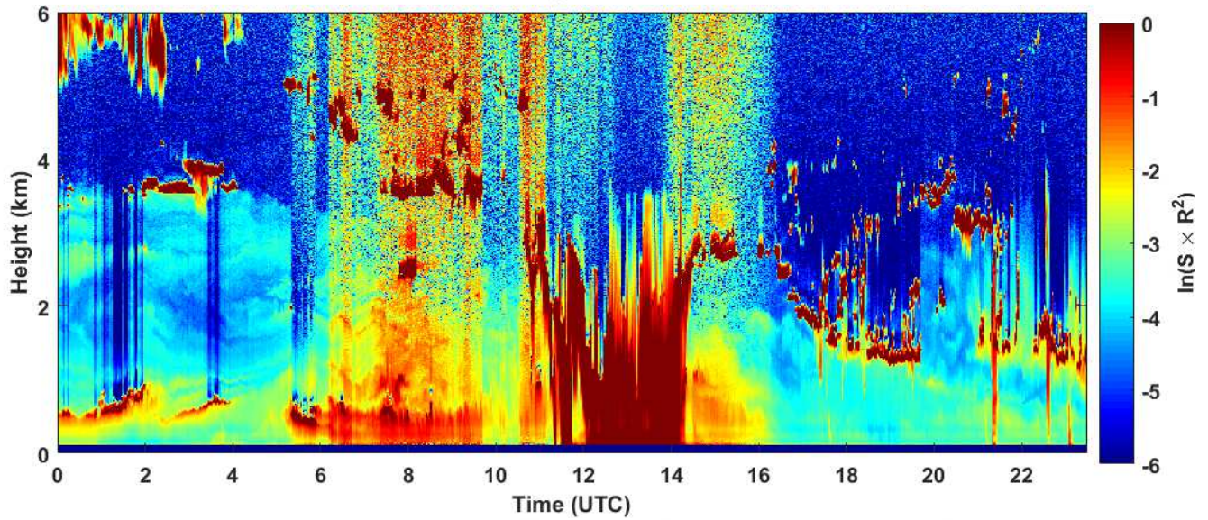
2018-10-04 RCS quick look CHM15k - ILVA LIDAR2 PARCHI
