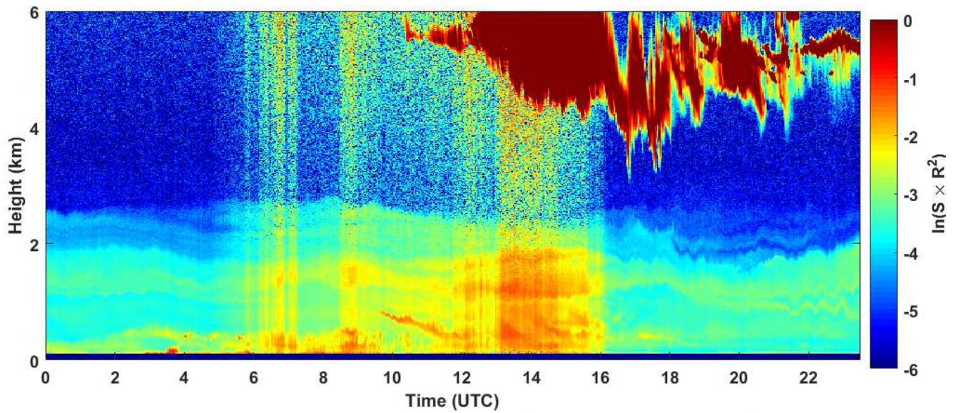
2018-10-12 RCS quick look CHM15k - ILVA LIDAR2 PARCHI
