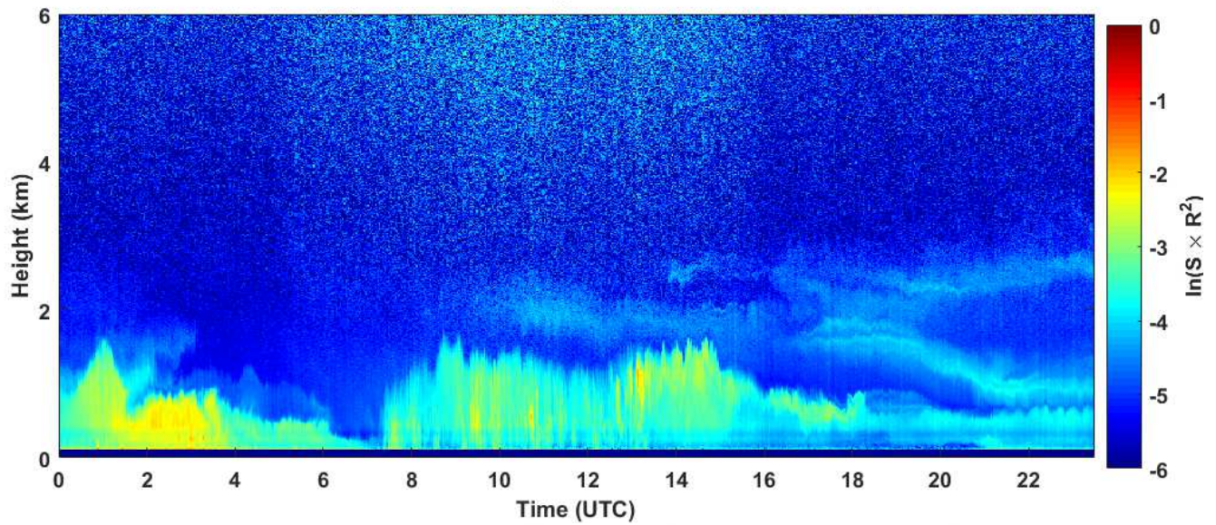
2018-10-26 RCS quick look CHM15k - ILVA LIDAR2 PARCHI
