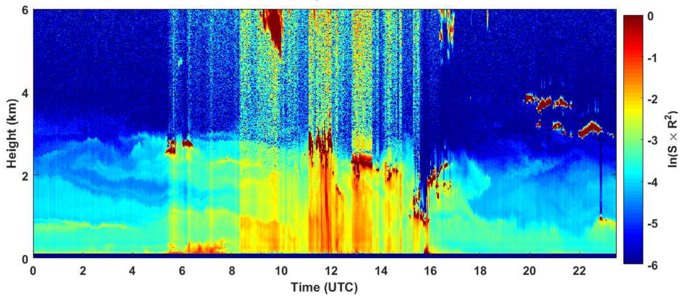
2018-10-14 RCS quick look CHM15k - ILVA LIDAR3 AGGLOMERATO
