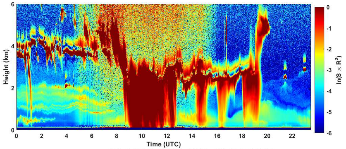
2019-10-08 RCS quick look CHM15k - ILVA LIDAR2 PARCHI
