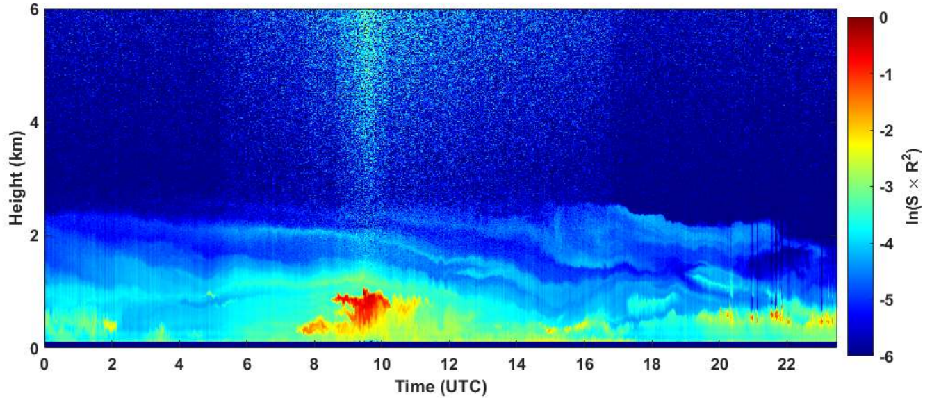
2019-10-02 RCS quick look CHM15k - ILVA LIDAR3 AGGLOMERATO
