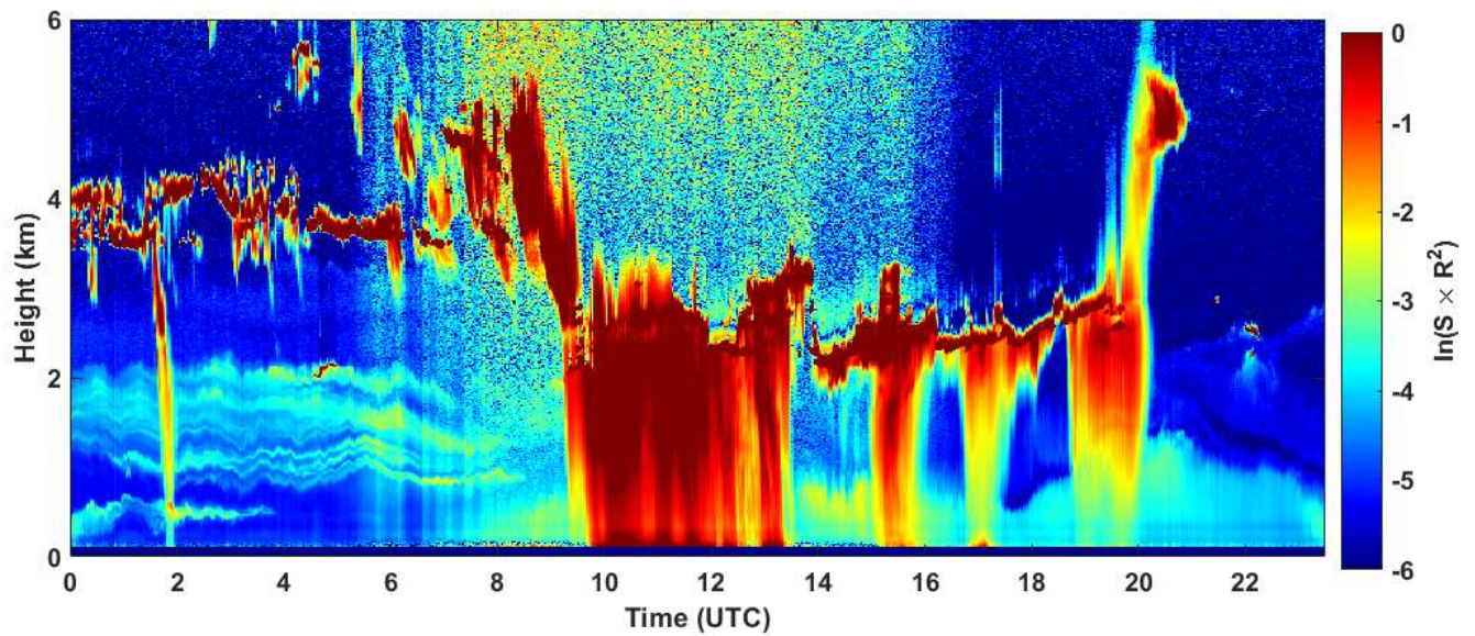
2019-10-08 RCS quick look CHM15k - ILVA LIDAR3 AGGLOMERATO
