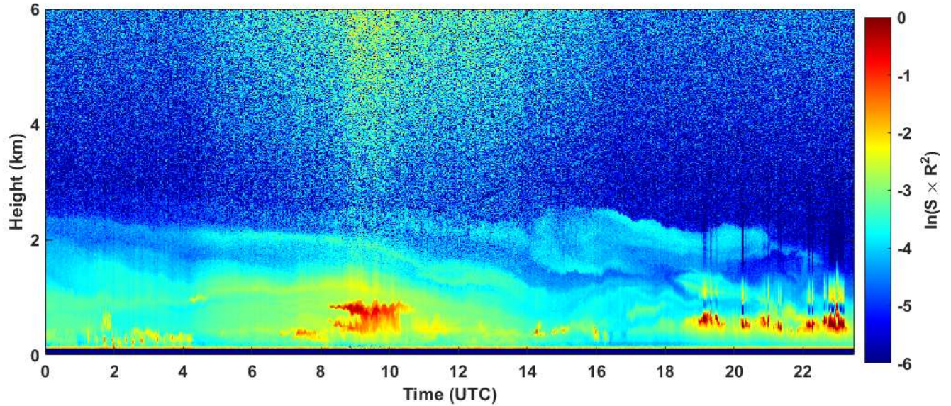
2019-10-02 RCS quick look CHM15k - ILVA LIDAR2 PARCHI
