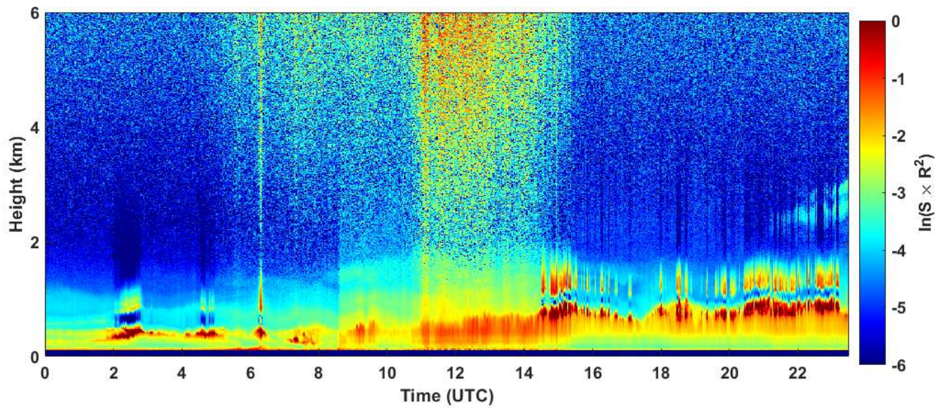
2019-10-24 RCS quick look CHM15k - ILVA LIDAR2 PARCHI
