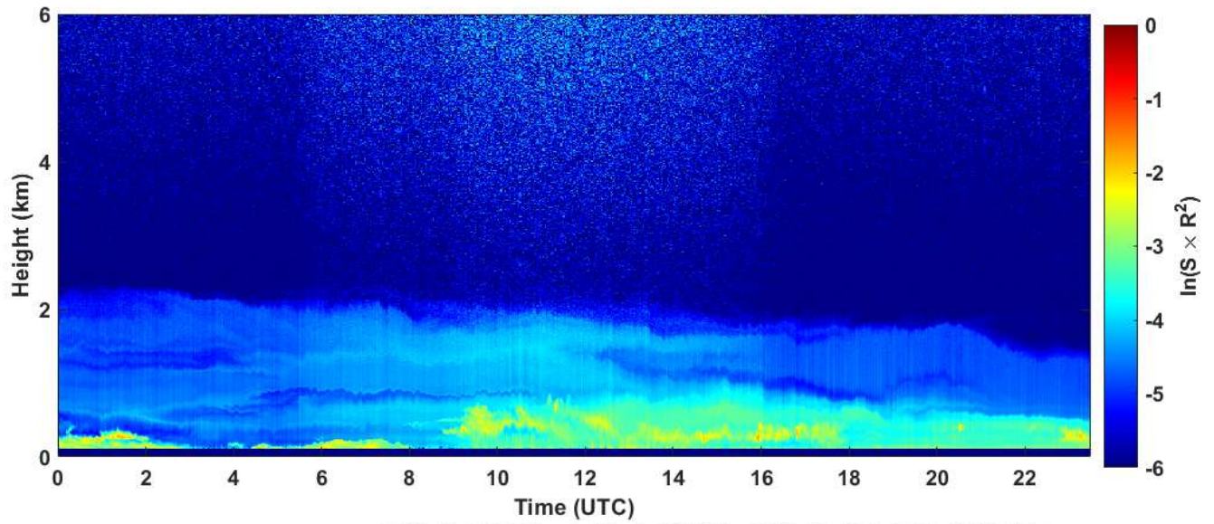
2019-10-24 RCS quick look CHM15k - ILVA LIDAR3 AGGLOMERATO
