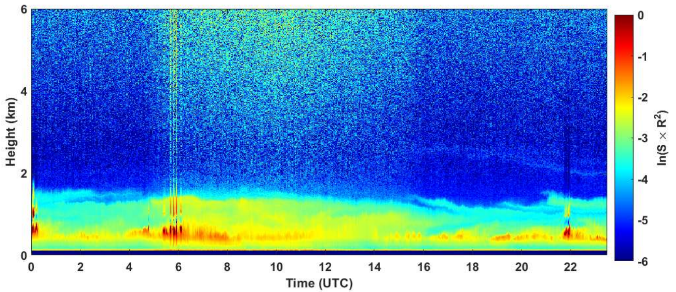
2019-10-20 RCS quick look CHM15k - ILVA LIDAR2 PARCHI
