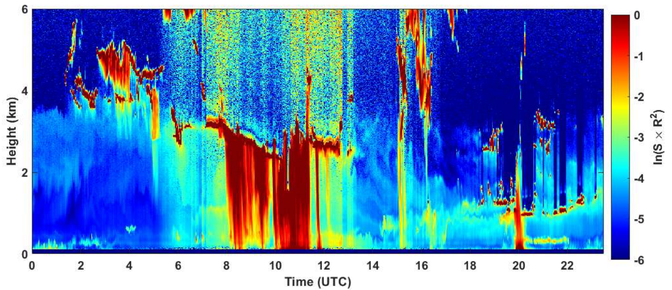
2019-10-04 RCS quick look CHM15k - ILVA LIDAR3 AGGLOMERATO
