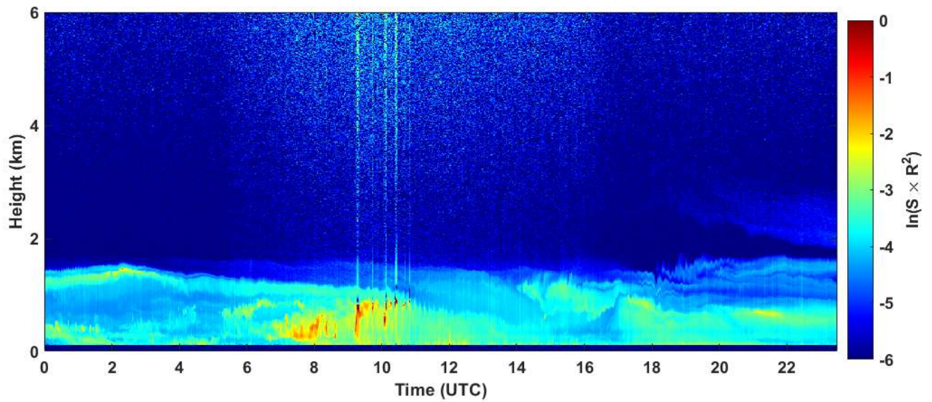
2019-10-14 RCS quick look CHM15k - ILVA LIDAR3 AGGLOMERATO
