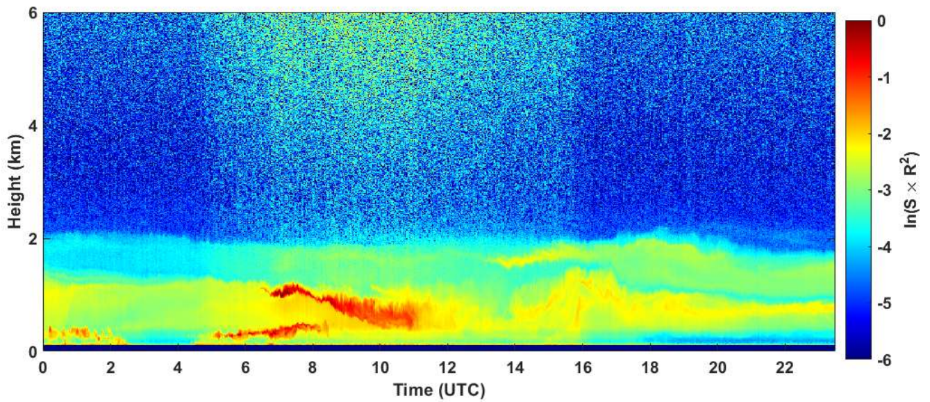
2019-10-12 RCS quick look CHM15k - ILVA LIDAR2 PARCHI
