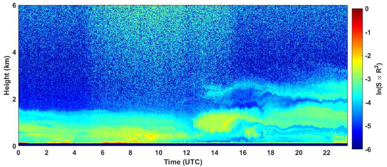
2019-10-28 RCS quick look CHM15k - ILVA LIDAR2 PARCHI
