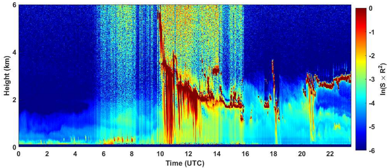
2019-10-06 RCS quick look CHM15k - ILVA LIDAR3 AGGLOMERATO
