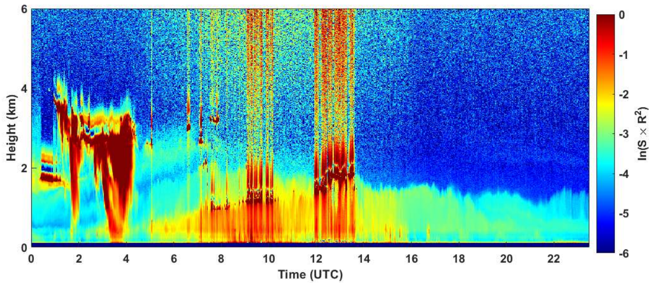
2019-10-04 RCS quick look CHM15k - ILVA LIDAR2 PARCHI
