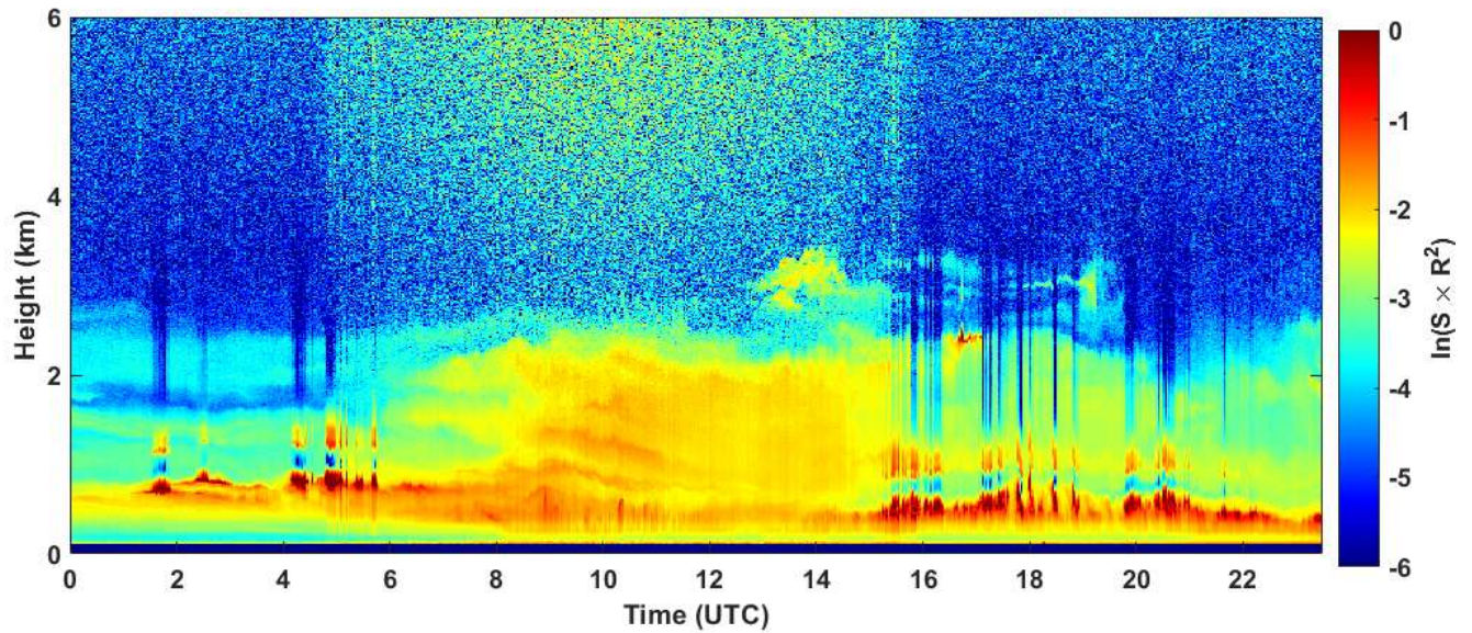
2019-10-16 RCS quick look CHM15k - ILVA LIDAR2 PARCHI
