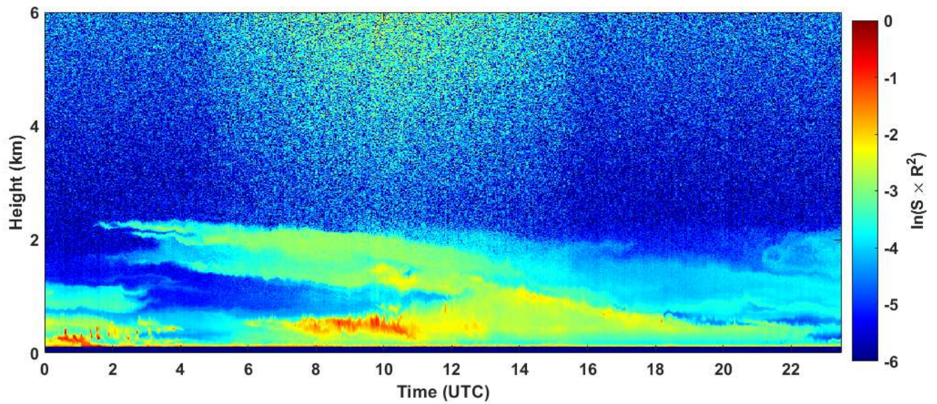
2019-10-22 RCS quick look CHM15k - ILVA LIDAR2 PARCHI
