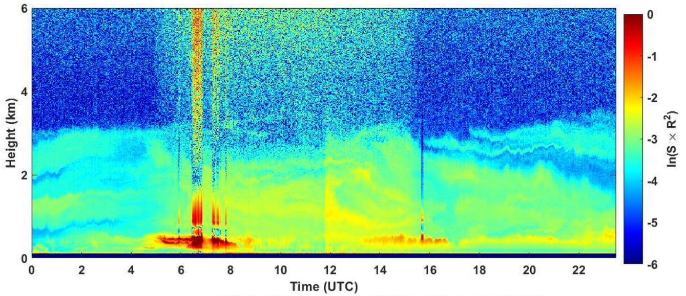
2019-10-30 RCS quick look CHM15k - ILVA LIDAR2 PARCHI
