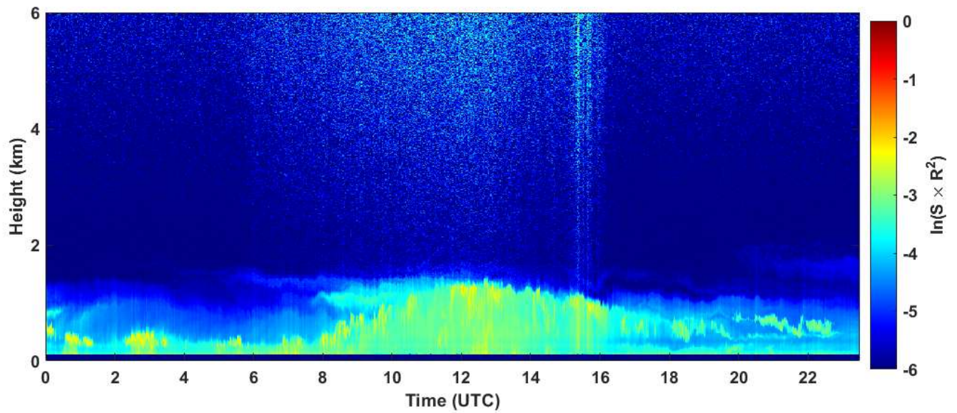
2019-10-26 RCS quick look CHM15k - ILVA LIDAR3 AGGLOMERATO
