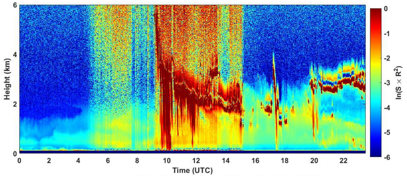
2019-10-06 RCS quick look CHM15k - ILVA LIDAR2 PARCHI
