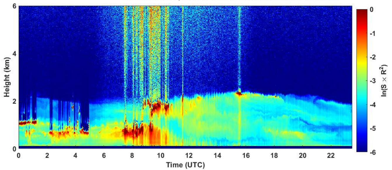
2019-10-18 RCS quick look CHM15k - ILVA LIDAR3 AGGLOMERATO
