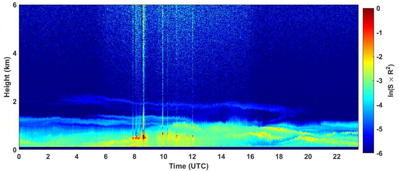
2019-10-22 RCS quick look CHM15k - ILVA LIDAR3 AGGLOMERATO
