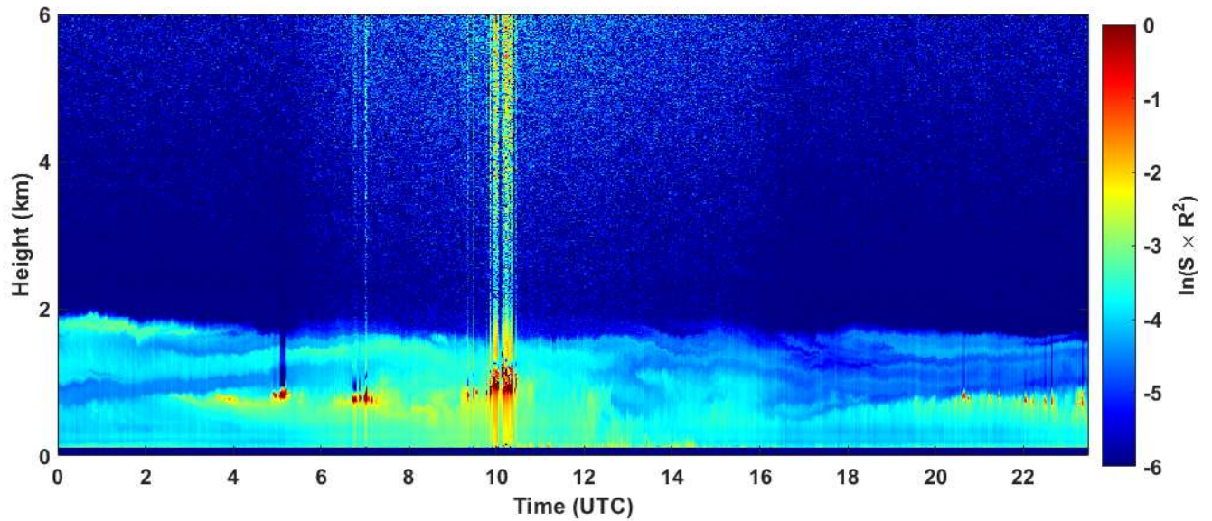
2019-10-20 RCS quick look CHM15k - ILVA LIDAR3 AGGLOMERATO
