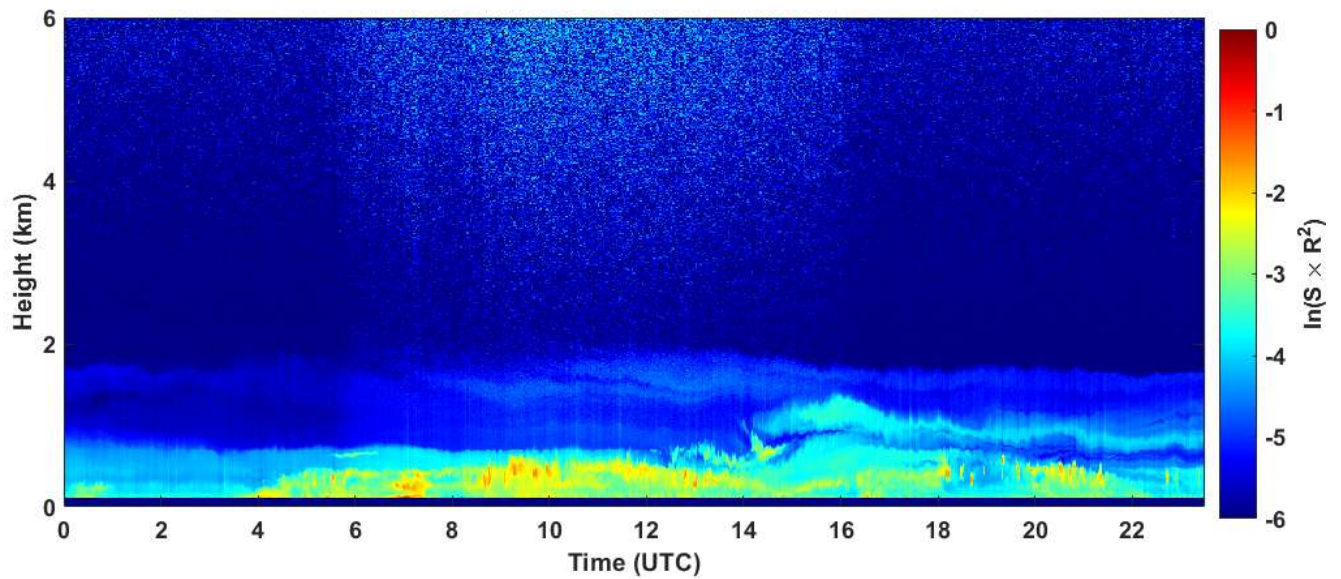
2019-10-28 RCS quick look CHM15k - ILVA LIDAR3 AGGLOMERATO
