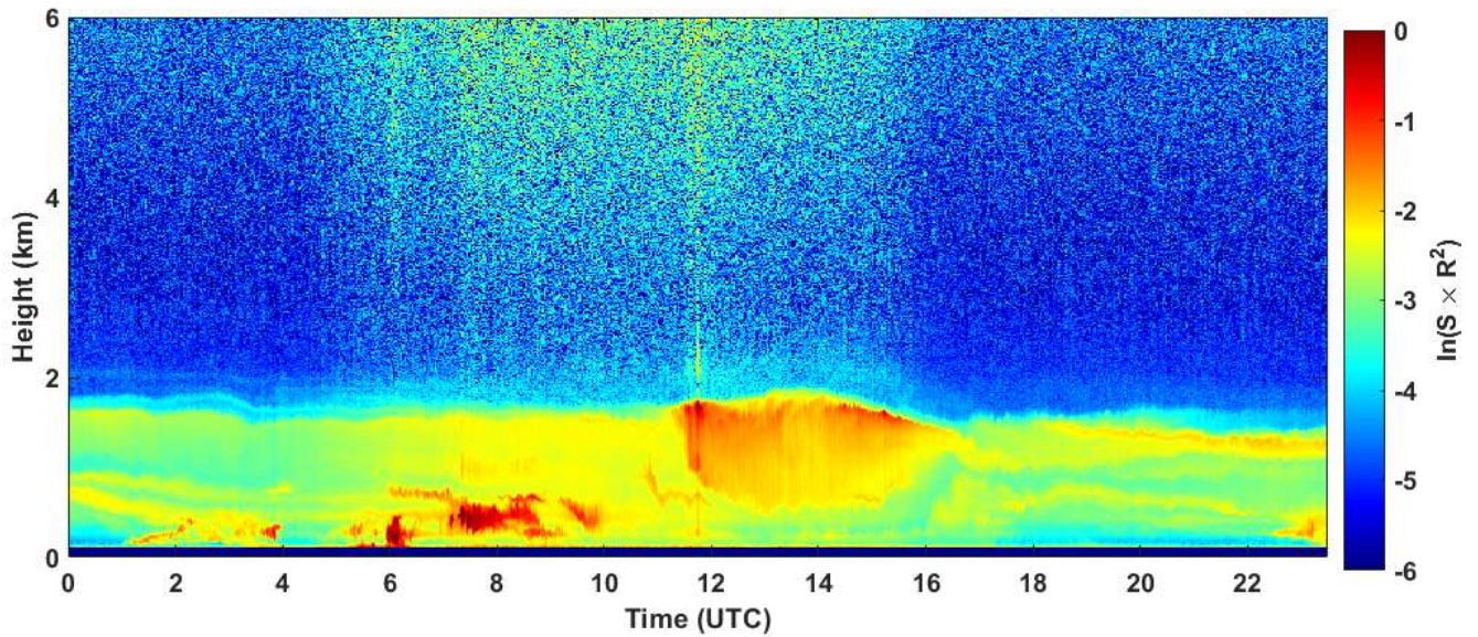
2019-10-14 RCS quick look CHM15k - ILVA LIDAR2 PARCHI
