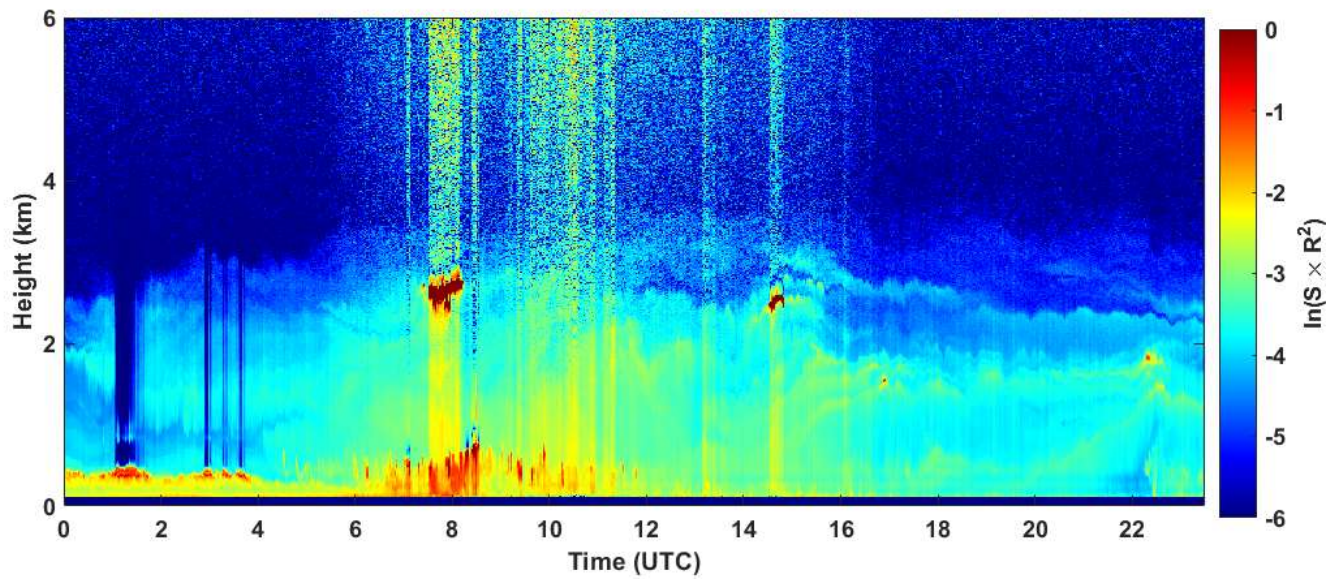
2019-10-16 RCS quick look CHM15k - ILVA LIDAR3 AGGLOMERATO
