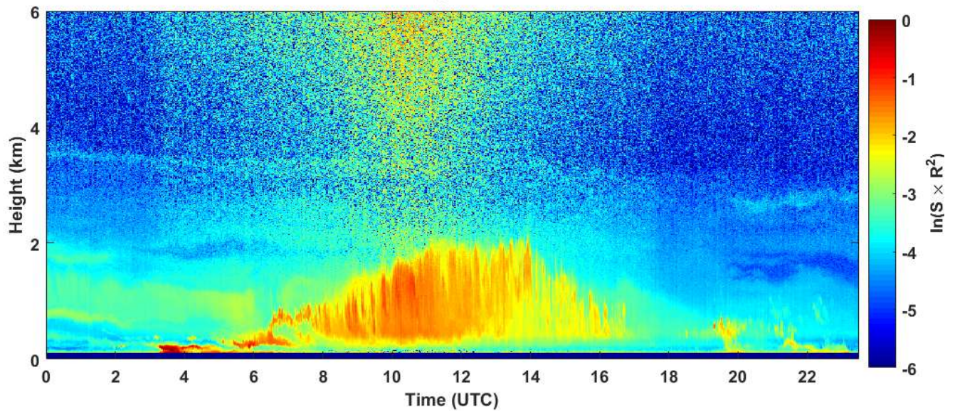
2019-07-22 RCS quick look CHM15k - ILVA LIDAR2 PARCHI
