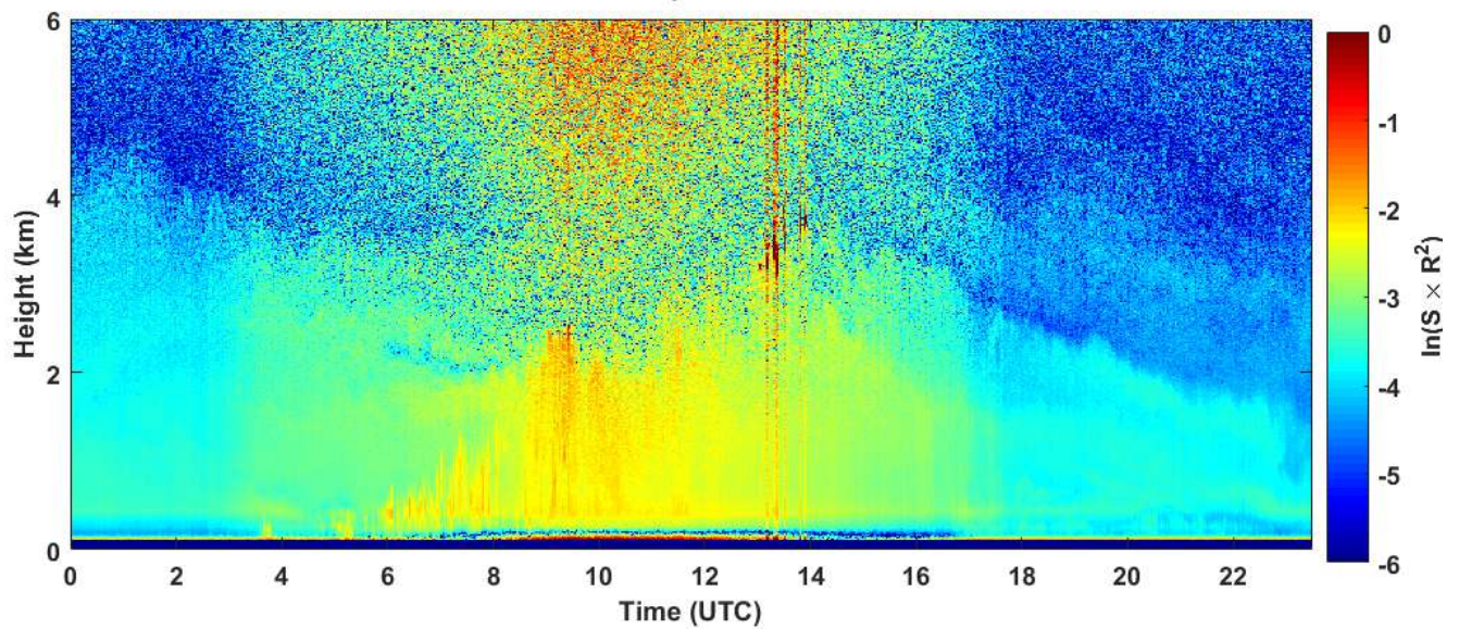
2019-07-08 RCS quick look CHM15k - ILVA LIDAR2 PARCHI
