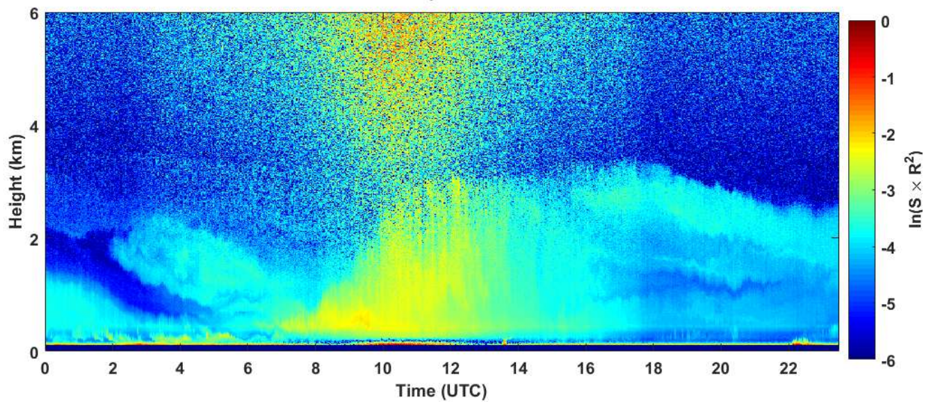
2019-07-06 RCS quick look CHM15k - ILVA LIDAR2 PARCHI
