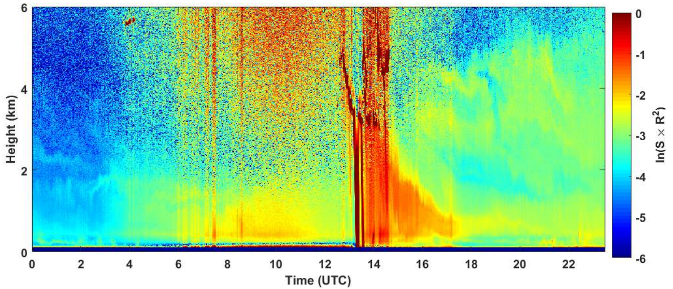
2019-07-10 RCS quick look CHM15k - ILVA LIDAR2 PARCHI
