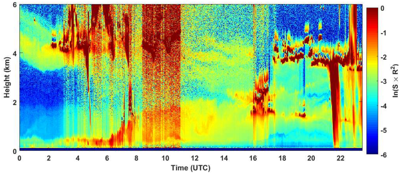
2019-07-16 RCS quick look CHM15k - ILVA LIDAR2 PARCHI
