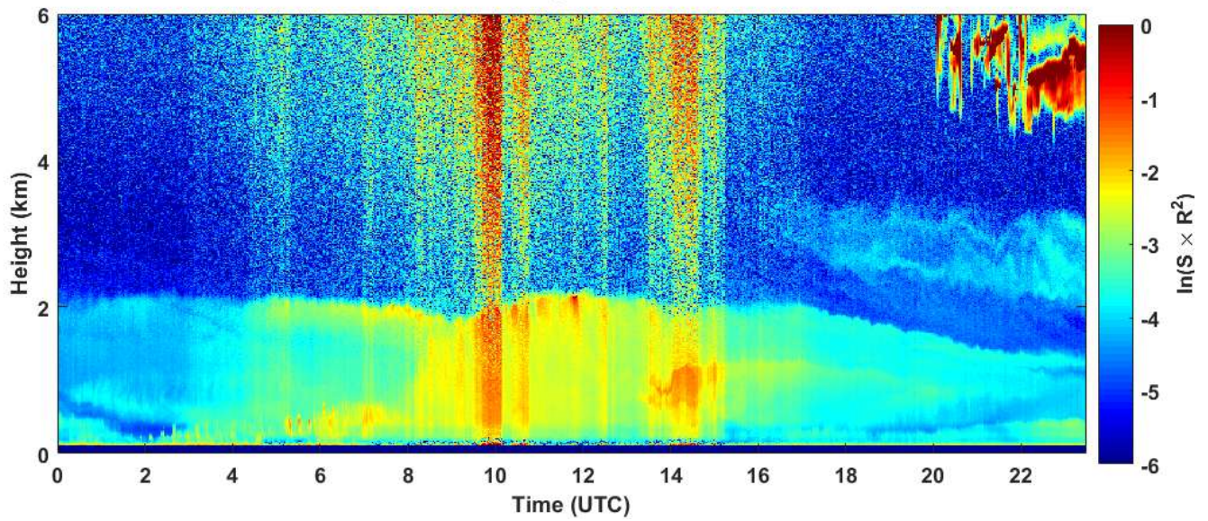
2019-05-08 RCS quick look CHM15k - ILVA LIDAR2 PARCHI
