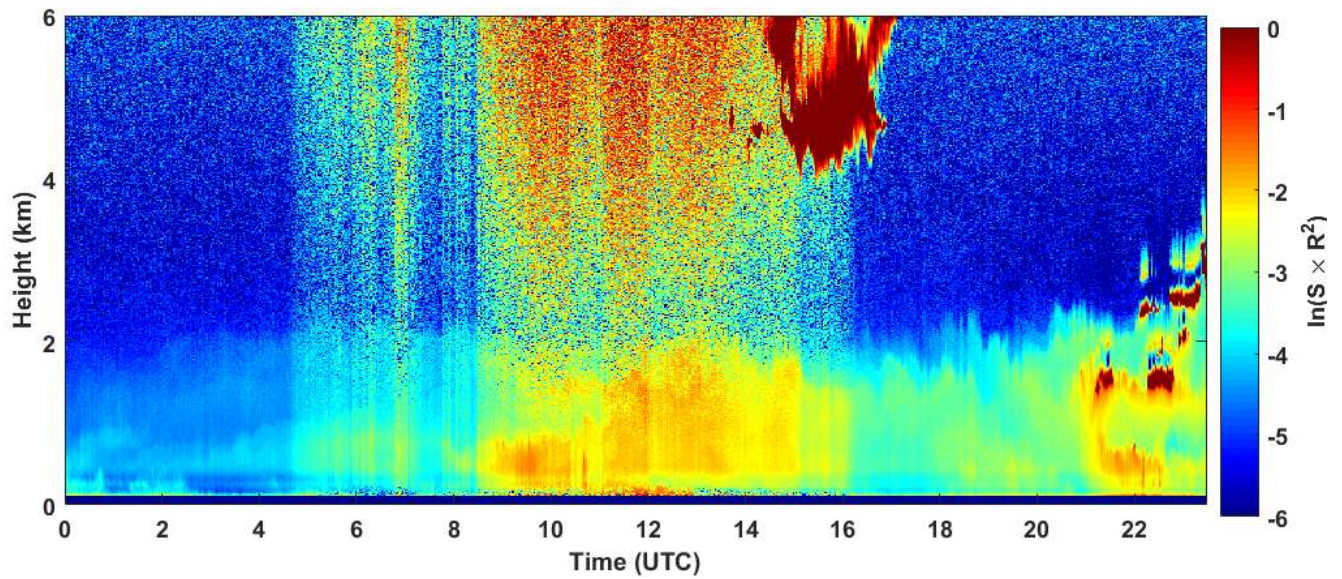
2019-03-12 RCS quick look CHM15k - ILVA LIDAR2 PARCHI
