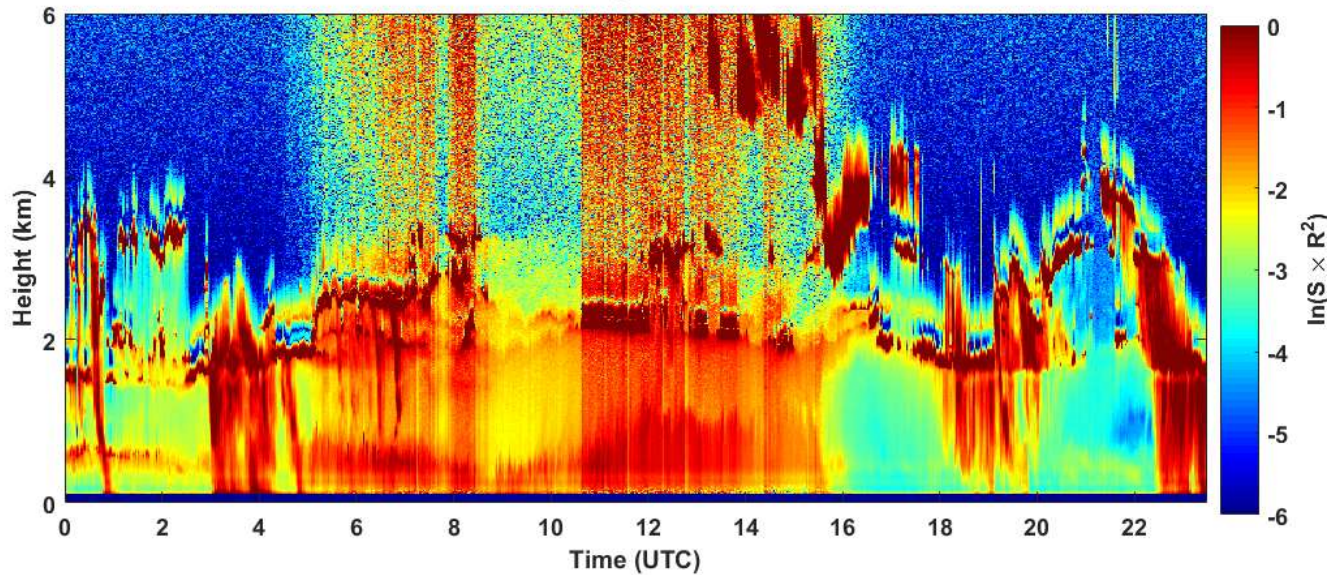
2019-03-28 RCS quick look CHM15k - ILVA LIDAR2 PARCHI
