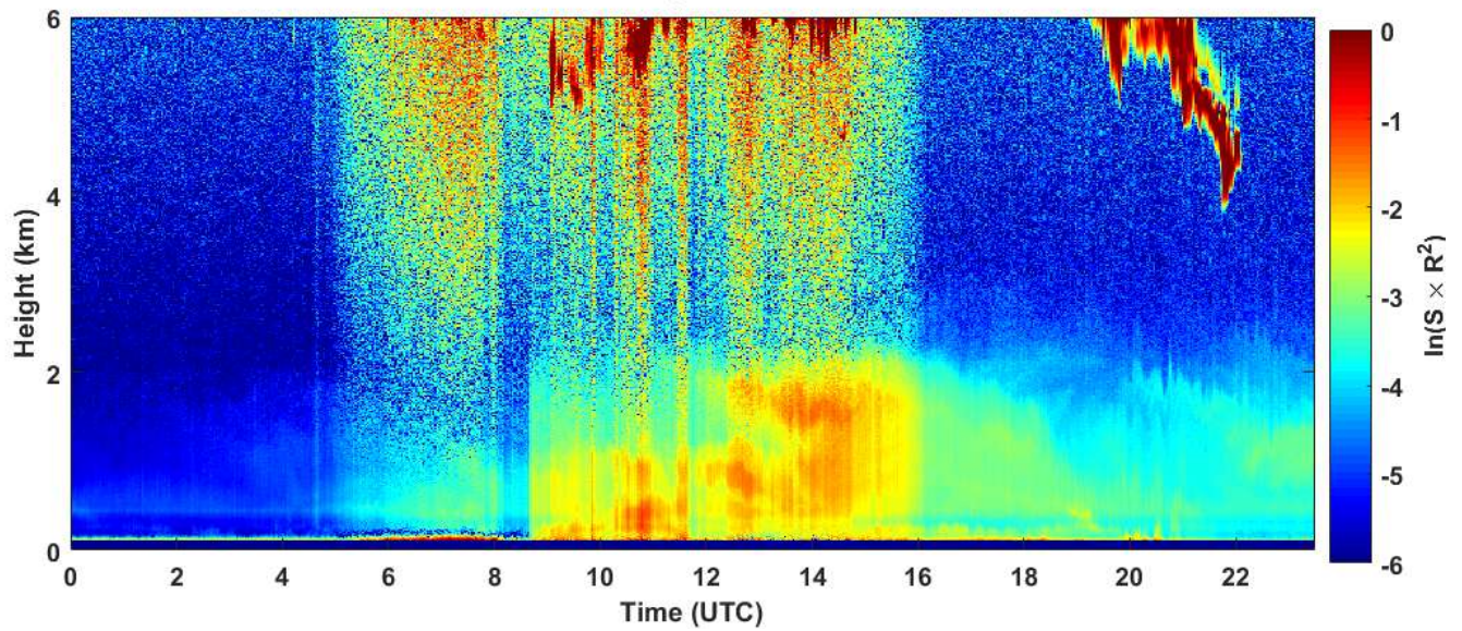
2019-03-06 RCS quick look CHM15k - ILVA LIDAR2 PARCHI
