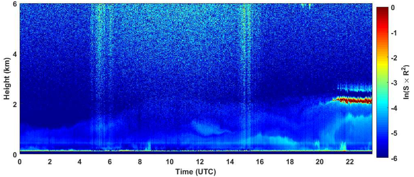
2019-03-02 RCS quick look CHM15k - ILVA LIDAR2 PARCHI
