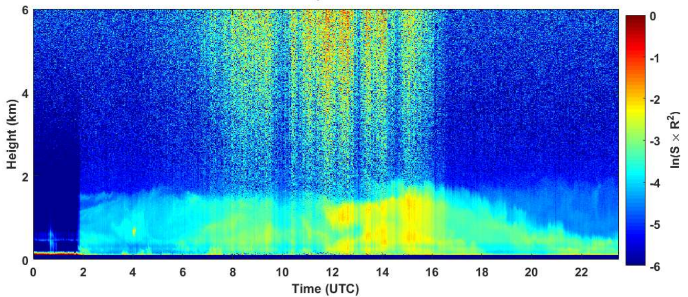
2019-03-10 RCS quick look CHM15k - ILVA LIDAR2 PARCHI
