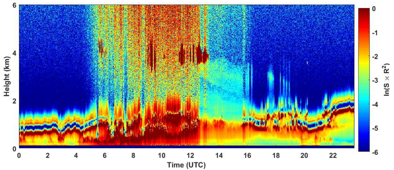
2019-03-20 RCS quick look CHM15k - ILVA LIDAR2 PARCHI
