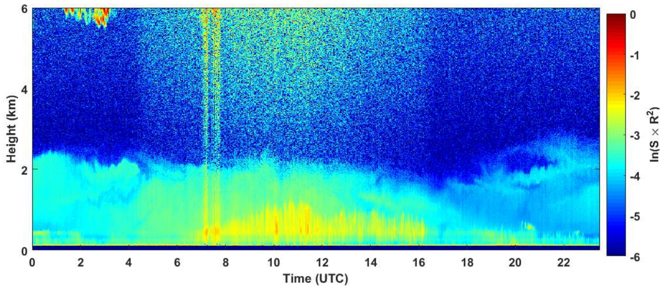
2019-03-24 RCS quick look CHM15k - ILVA LIDAR2 PARCHI
