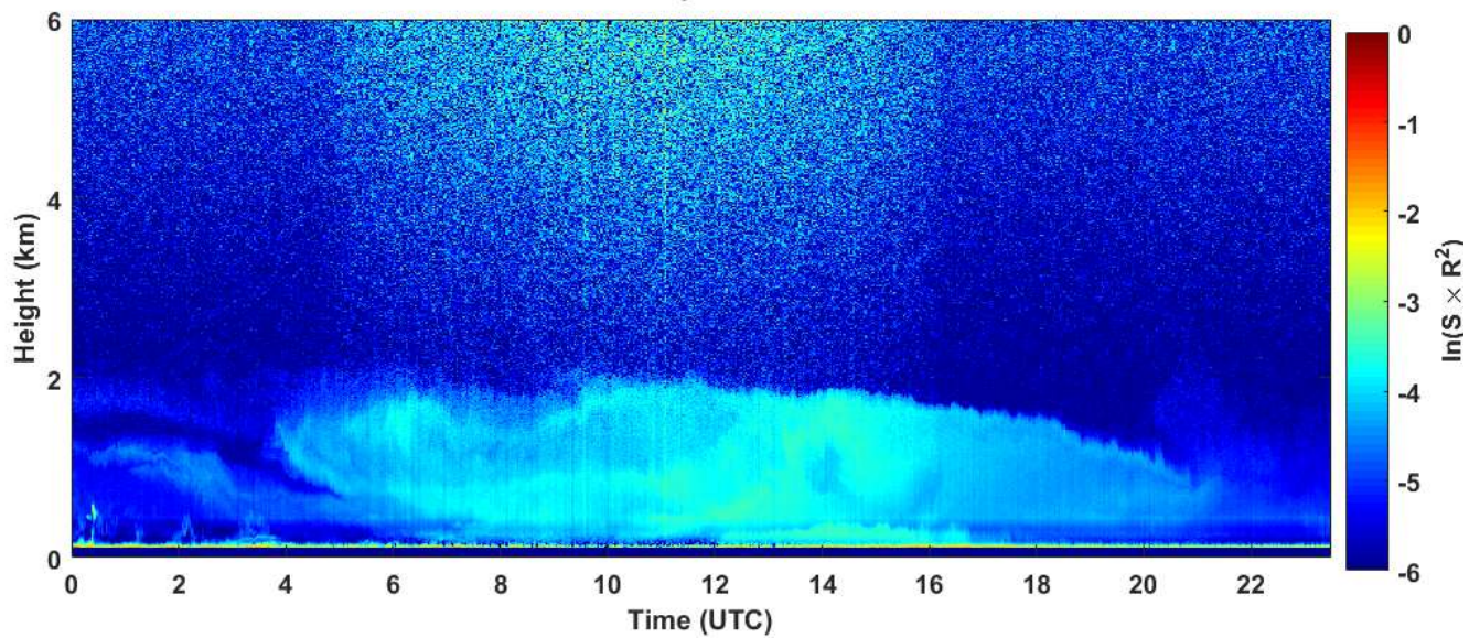
2019-03-04 RCS quick look CHM15k - ILVA LIDAR2 PARCHI
