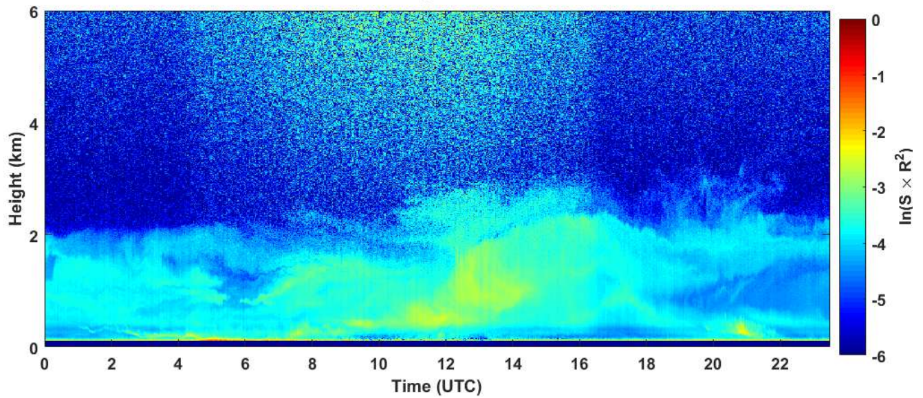
2019-03-26 RCS quick look CHM15k - ILVA LIDAR2 PARCHI
