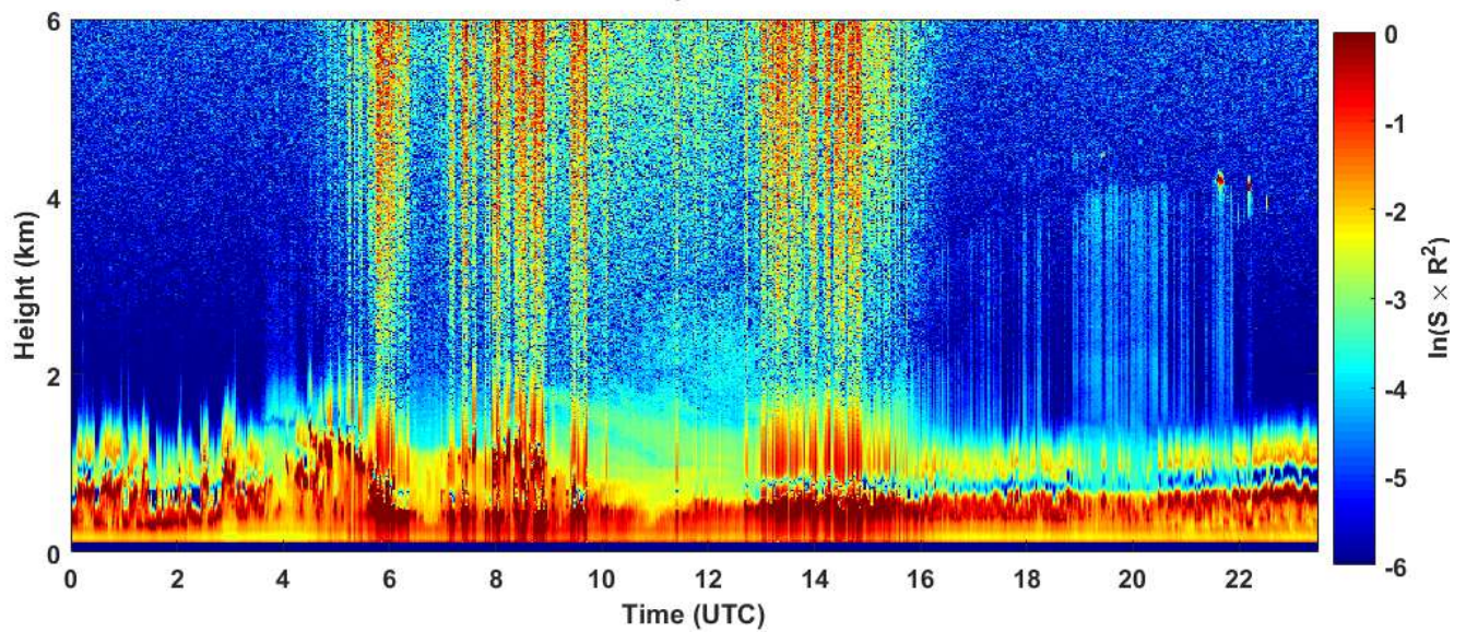
2019-03-18 RCS quick look CHM15k - ILVA LIDAR2 PARCHI
