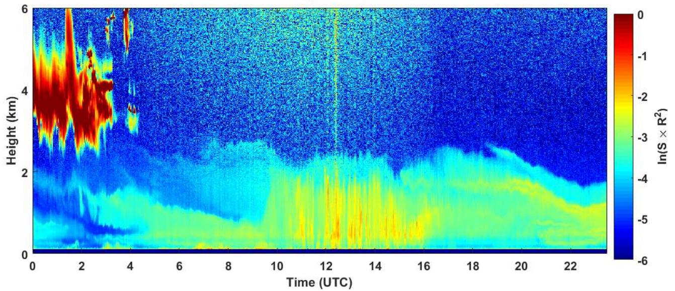
2019-03-16 RCS quick look CHM15k - ILVA LIDAR2 PARCHI
