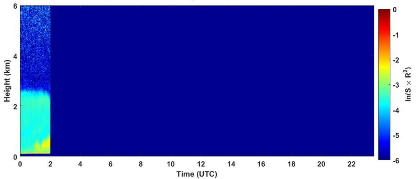
2019-03-22 RCS quick look CHM15k - ILVA LIDAR2 PARCHI
