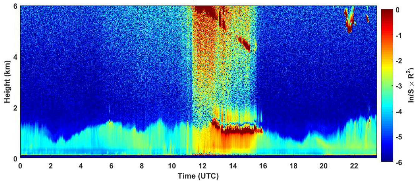
2019-02-14 RCS quick look CHM15k - ILVA LIDAR2 PARCHI
