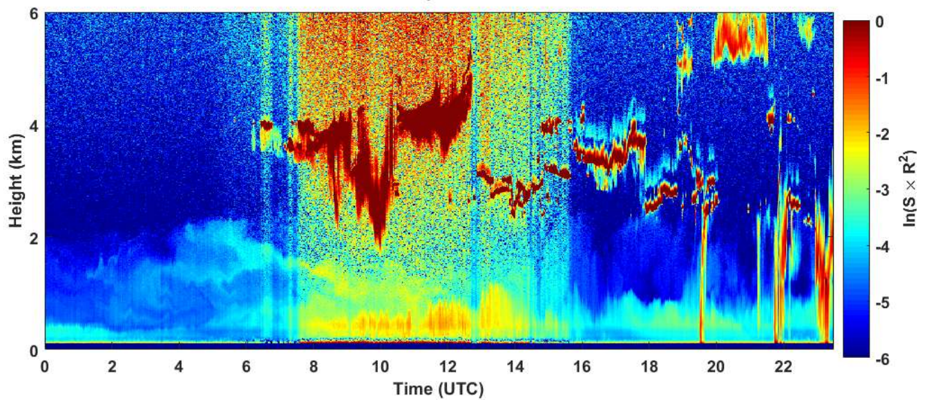
2019-02-22 RCS quick look CHM15k - ILVA LIDAR2 PARCHI
