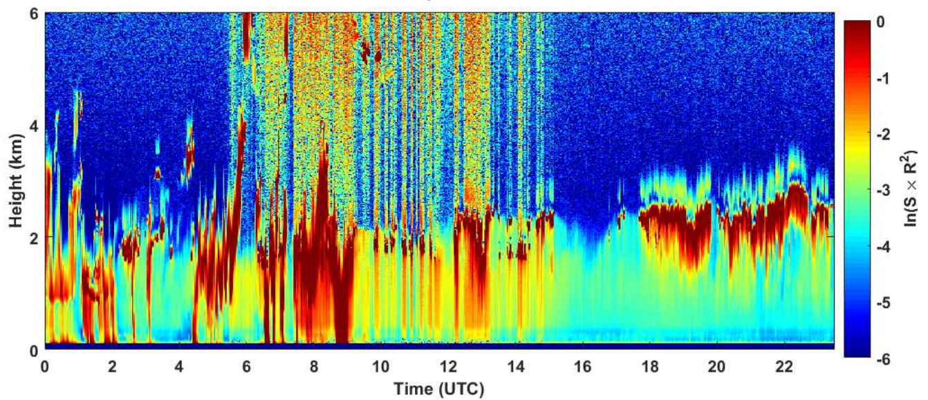
2019-02-12 RCS quick look CHM15k - ILVA LIDAR2 PARCHI
