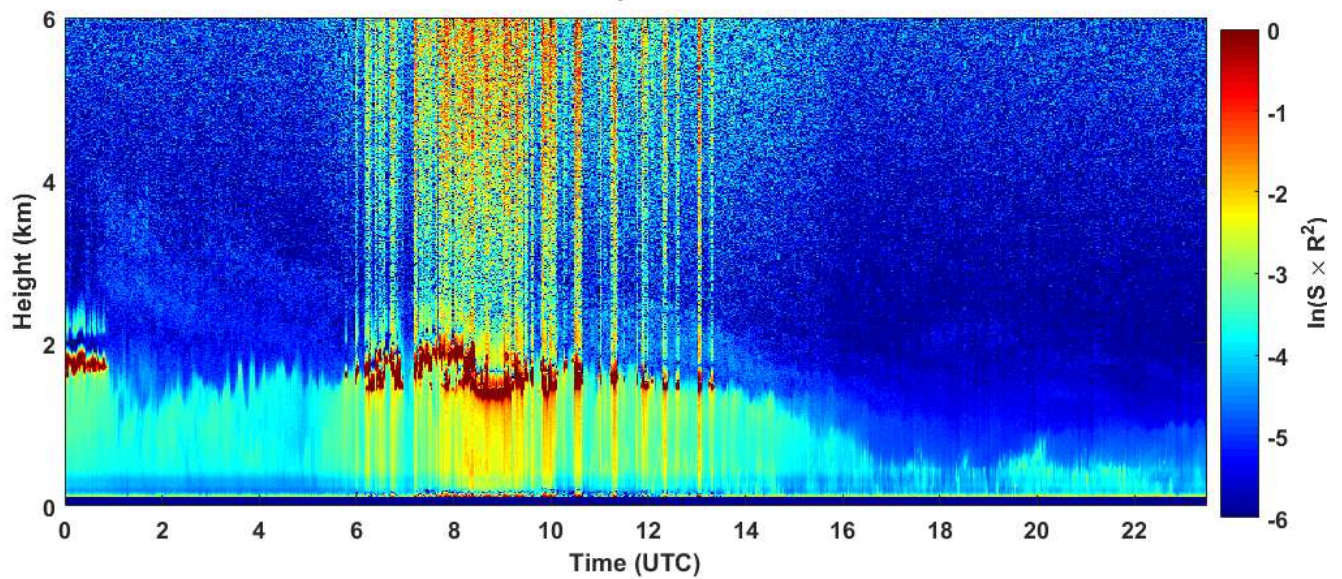
2019-02-16 RCS quick look CHM15k - ILVA LIDAR2 PARCHI
