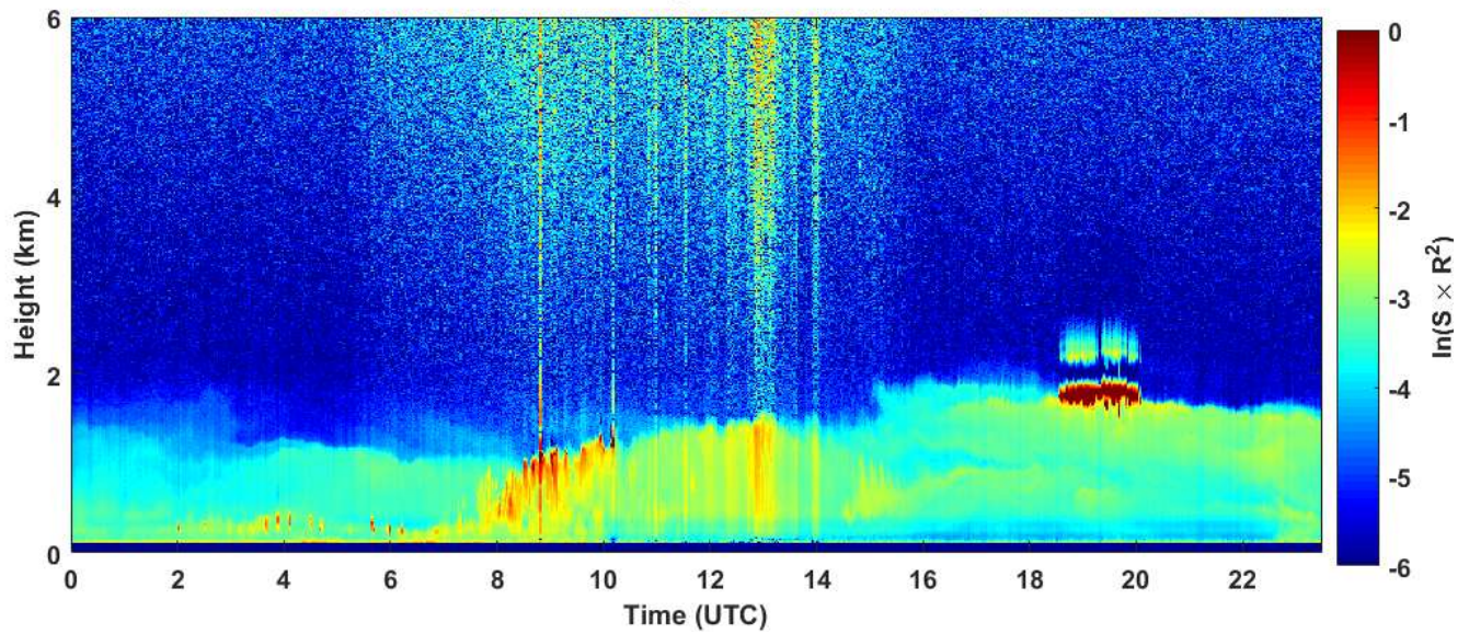
2019-02-10 RCS quick look CHM15k - ILVA LIDAR2 PARCHI
