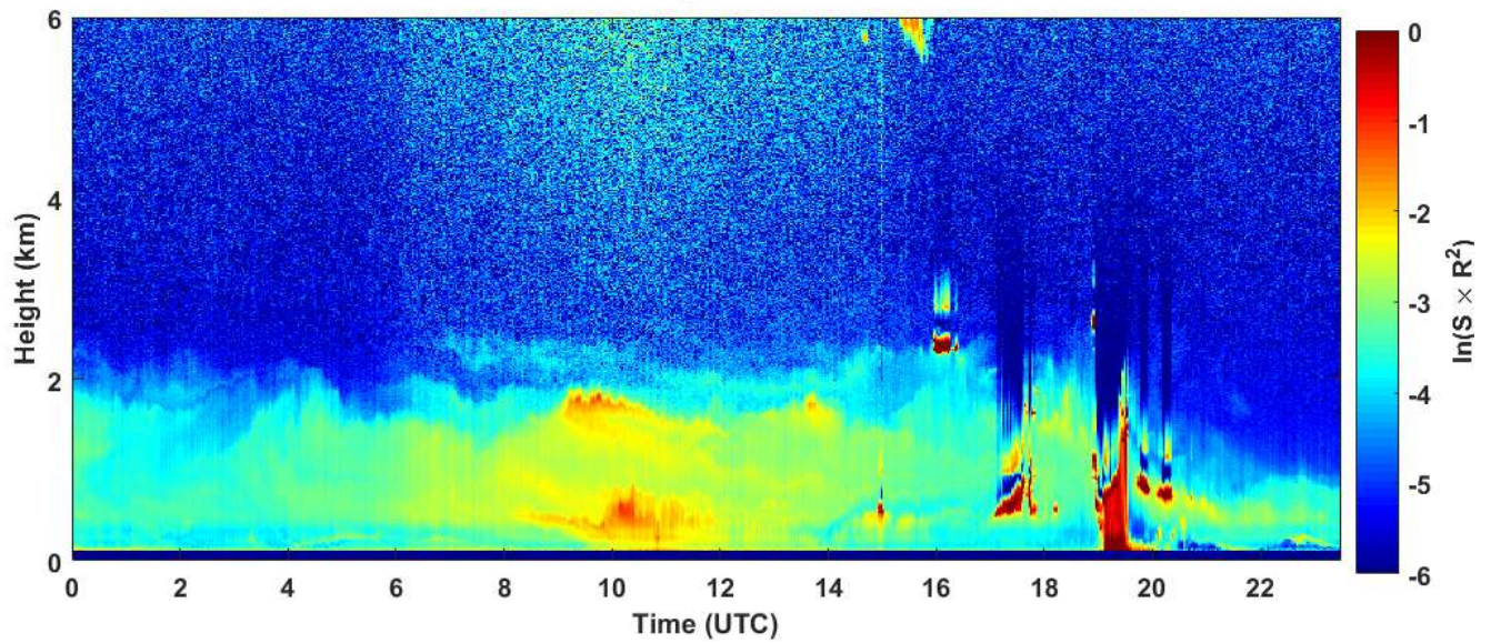
2019-01-20 RCS quick look CHM15k - ILVA LIDAR2 PARCHI
