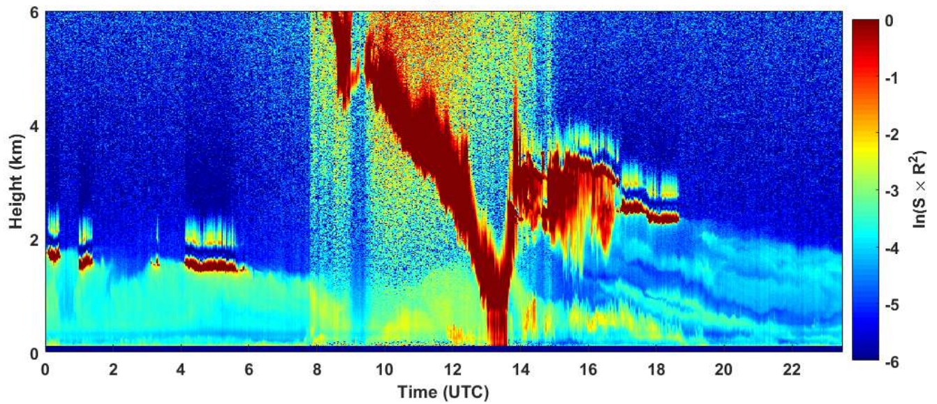
2019-01-14 RCS quick look CHM15k - ILVA LIDAR2 PARCHI
