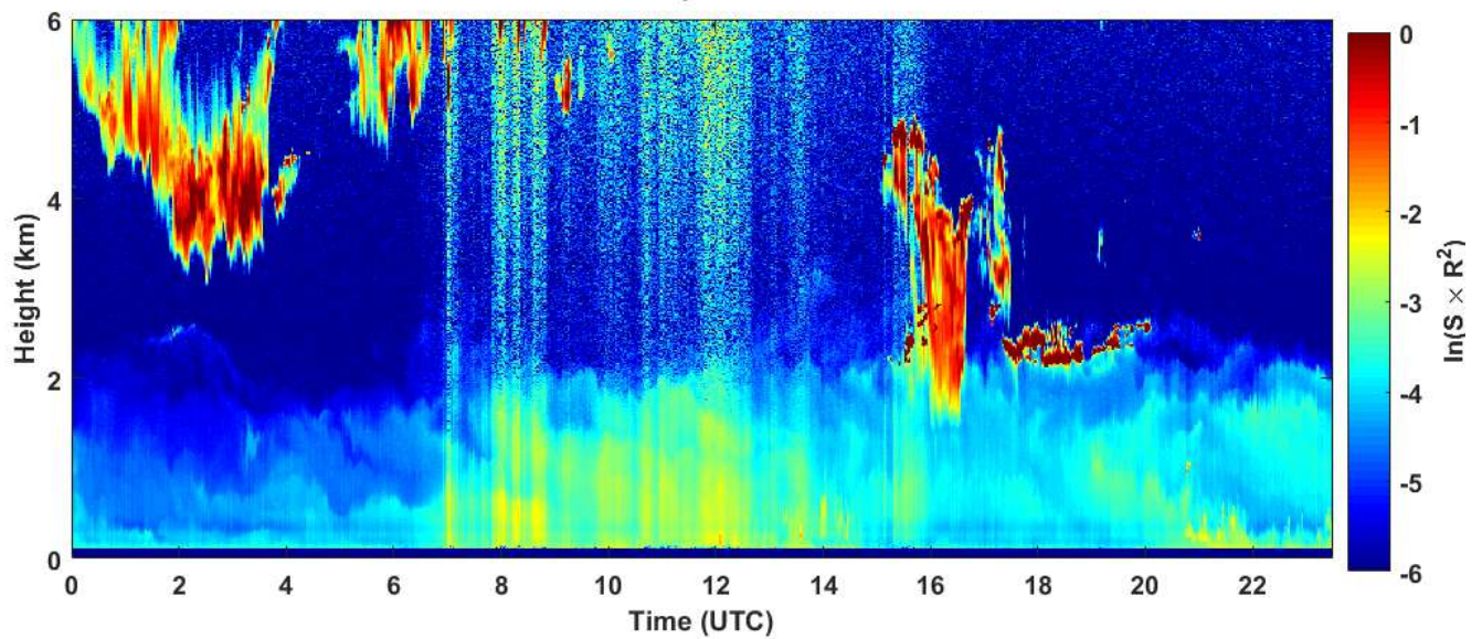
2019-01-18 RCS quick look CHM15k - ILVA LIDAR3 AGGLOMERATO
