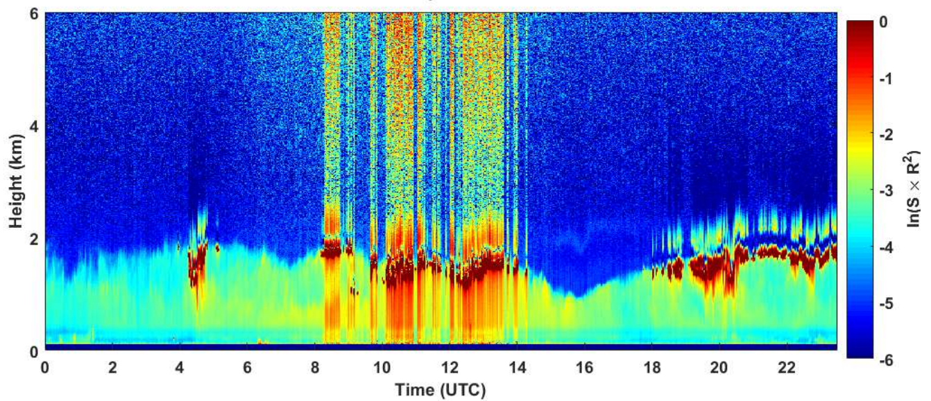
2019-01-12 RCS quick look CHM15k - ILVA LIDAR2 PARCHI
