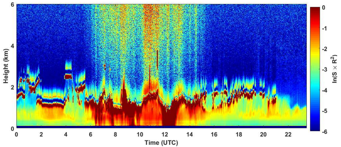
2019-01-27 RCS quick look CHM15k - ILVA LIDAR2 PARCHI
