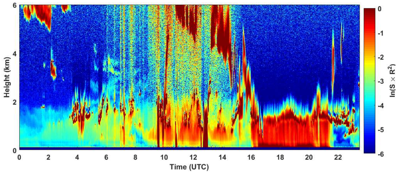
2019-01-25 RCS quick look CHM15k - ILVA LIDAR2 PARCHI
