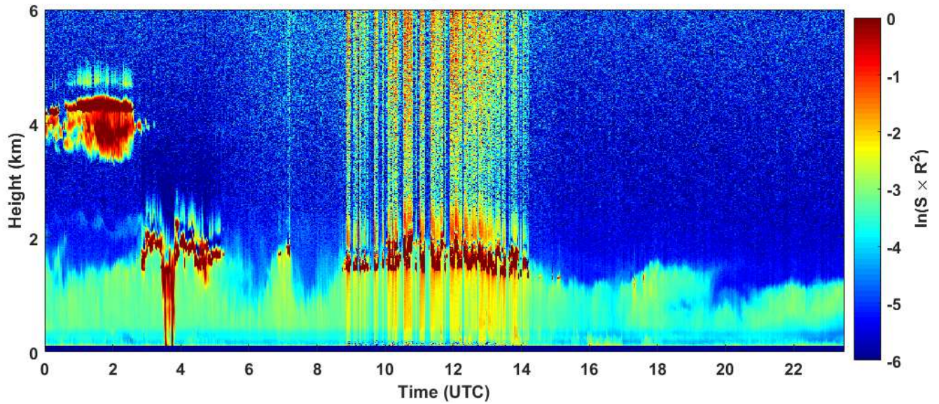
2019-01-02 RCS quick look CHM15k - ILVA LIDAR2 PARCHI
