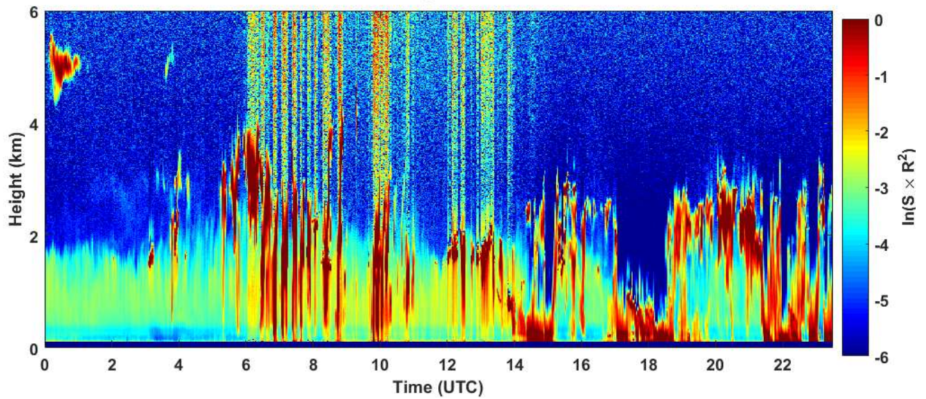
2019-01-04 RCS quick look CHM15k - ILVA LIDAR2 PARCHI
