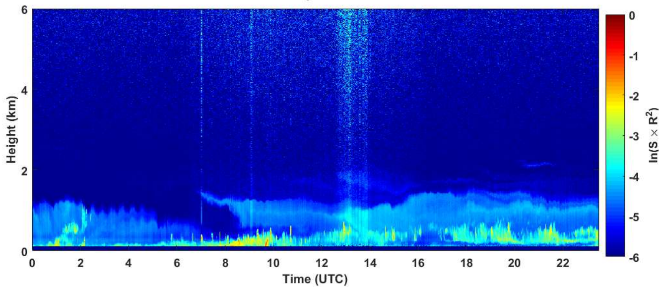
2019-01-16 RCS quick look CHM15k - ILVA LIDAR3 AGGLOMERATO
