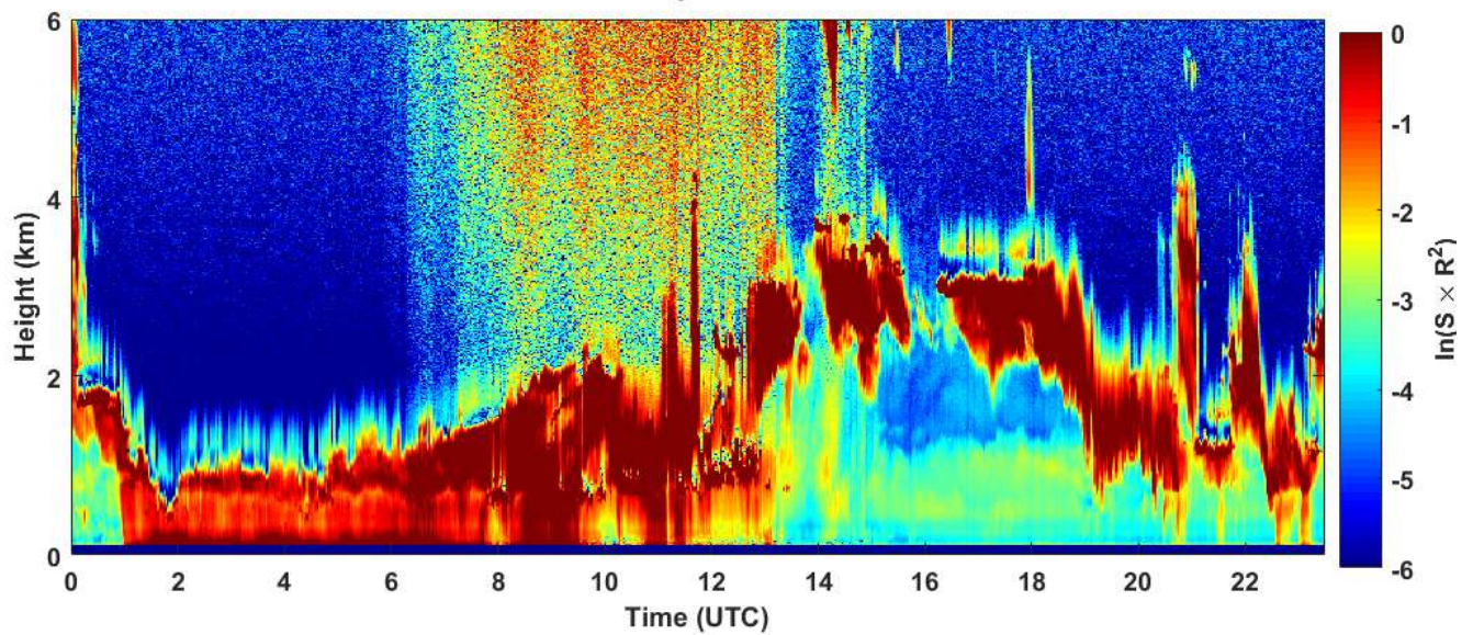
2019-01-10 RCS quick look CHM15k - ILVA LIDAR2 PARCHI
