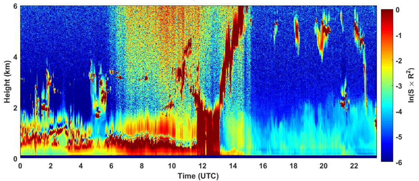
2019-01-22 RCS quick look CHM15k - ILVA LIDAR2 PARCHI
