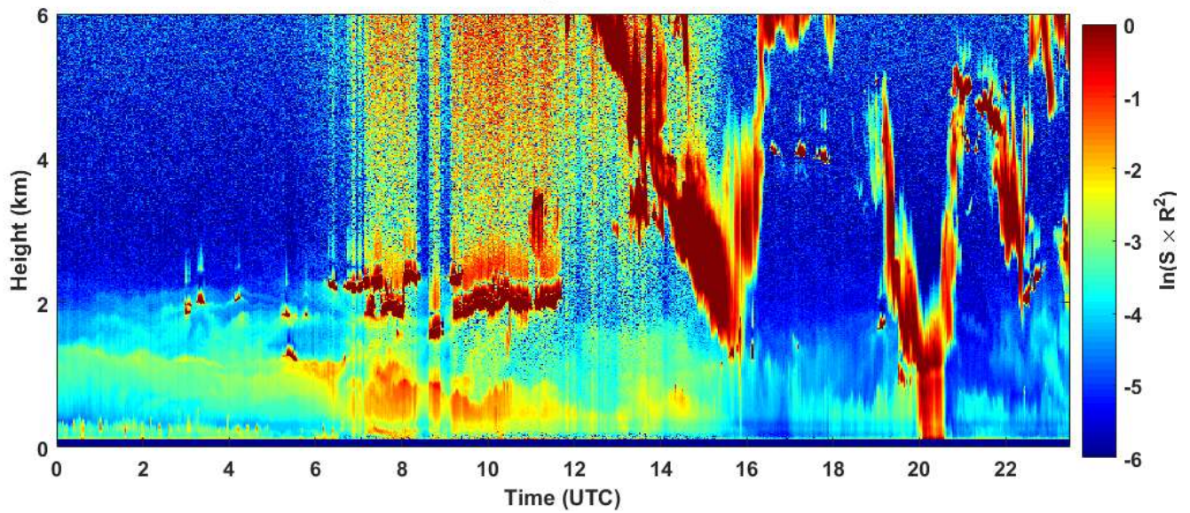
2019-01-31 RCS quick look CHM15k - ILVA LIDAR2 PARCHI
