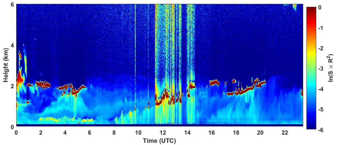
2019-01-12 RCS quick look CHM15k - ILVA LIDAR3 AGGLOMERATO
