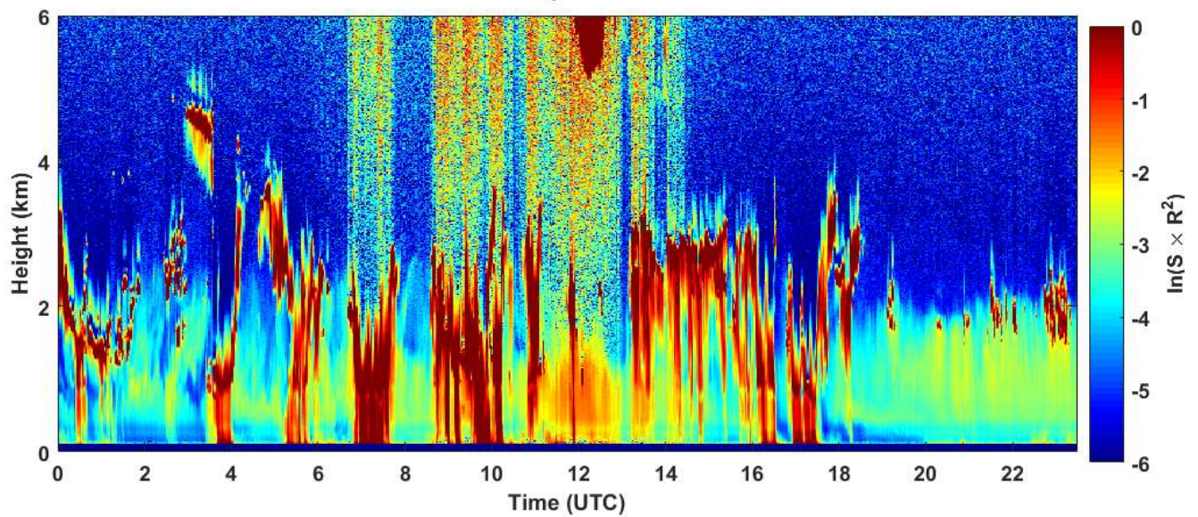
2019-01-06 RCS quick look CHM15k - ILVA LIDAR2 PARCHI
