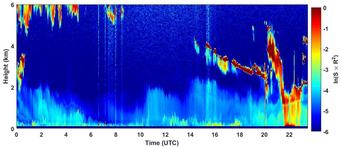
2019-01-31 RCS quick look CHM15k - ILVA LIDAR3 AGGLOMERATO
