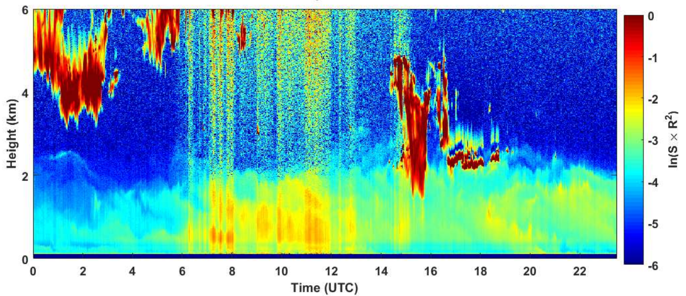
2019-01-18 RCS quick look CHM15k - ILVA LIDAR2 PARCHI
