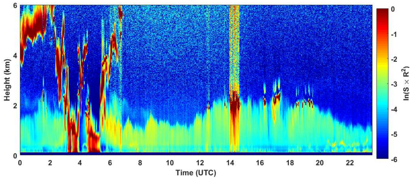
2019-01-16 RCS quick look CHM15k - ILVA LIDAR2 PARCHI
