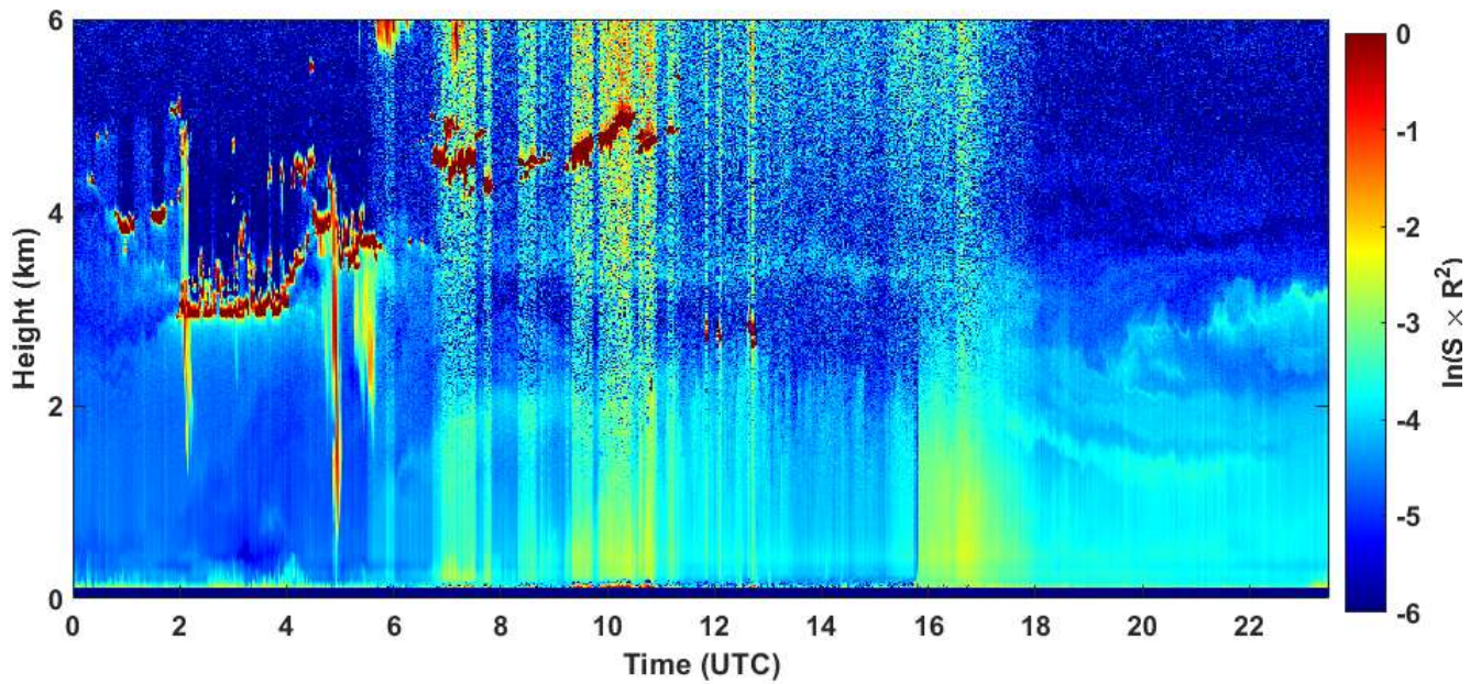
2020-09-16 RCS quick look CHM15k - ILVA LIDAR3 AGGLOMERATO
