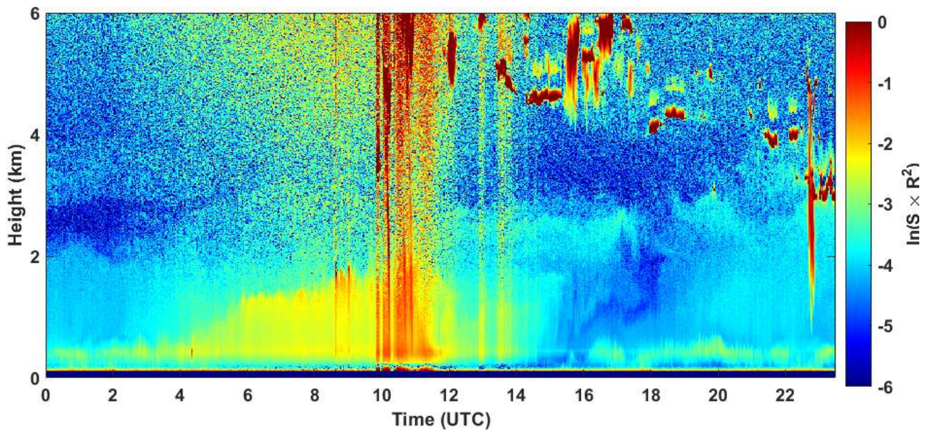
2020-09-14 RCS quick look CHM15k - ILVA LIDAR2 PARCHI
