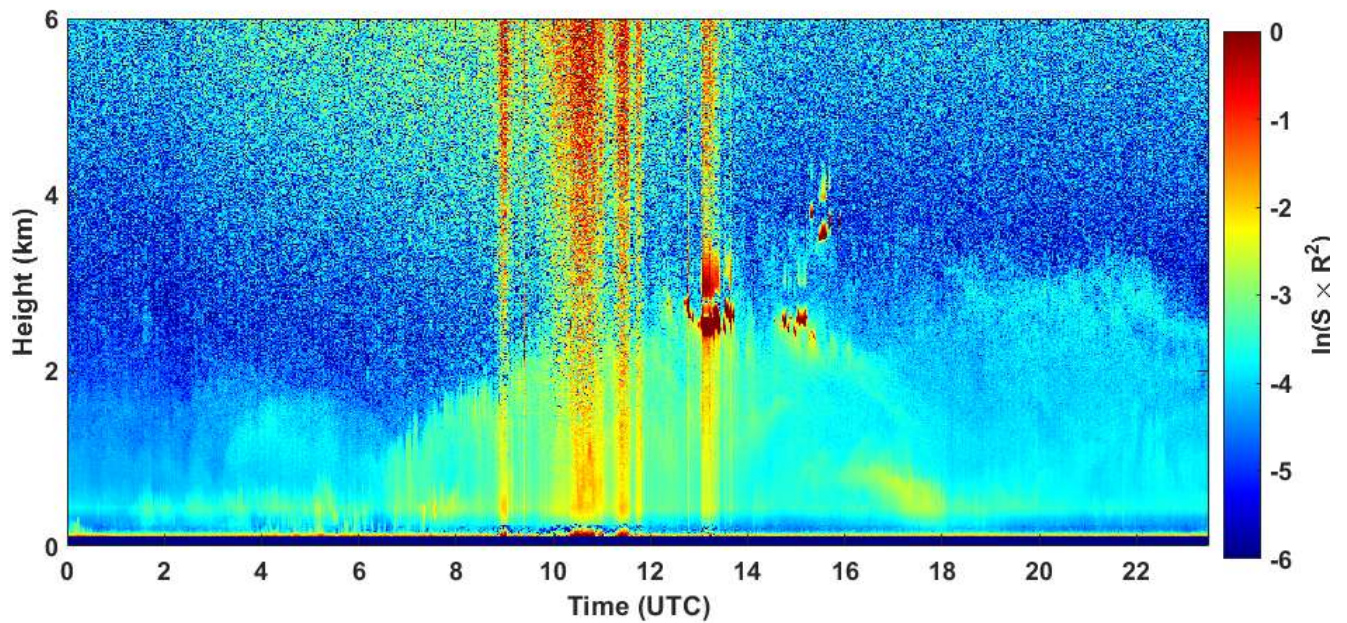
2020-09-24 RCS quick look CHM15k - ILVA LIDAR2 PARCHI
