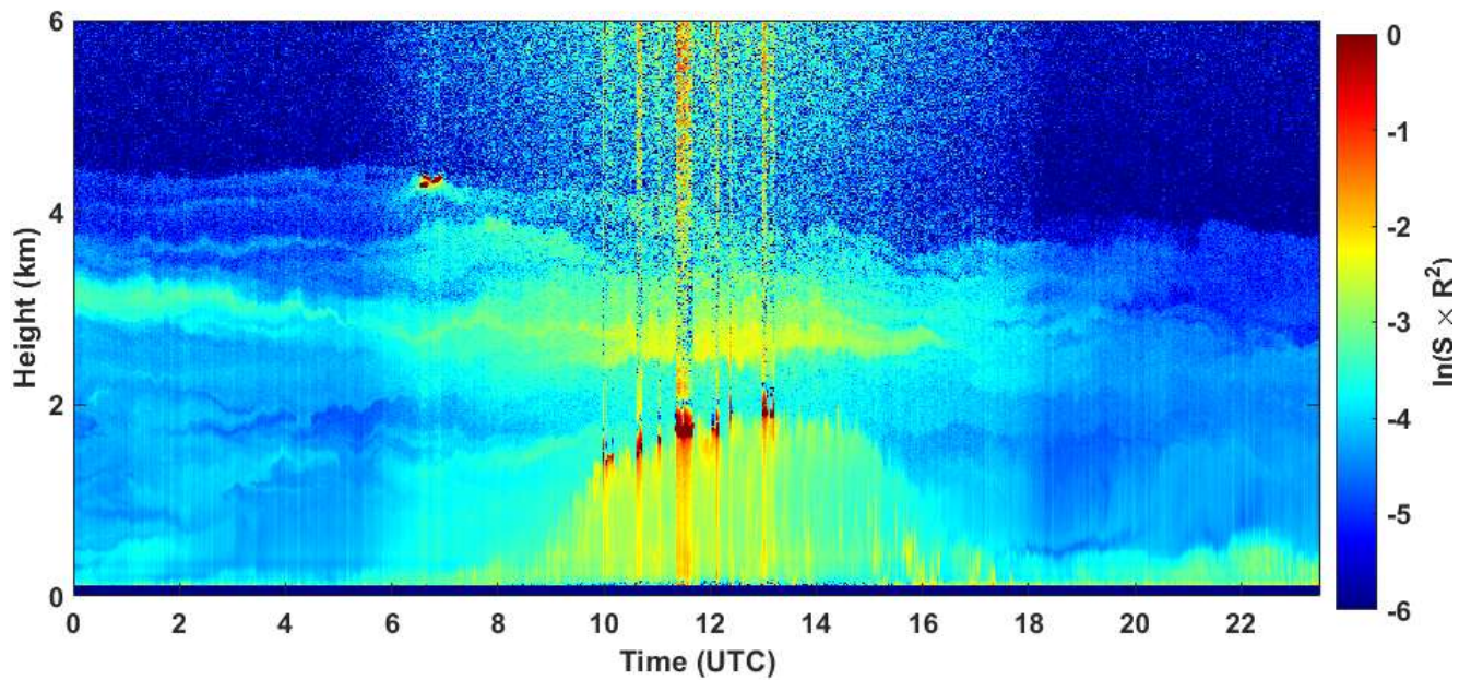
2020-09-08 RCS quick look CHM15k - ILVA LIDAR3 AGGLOMERATO
