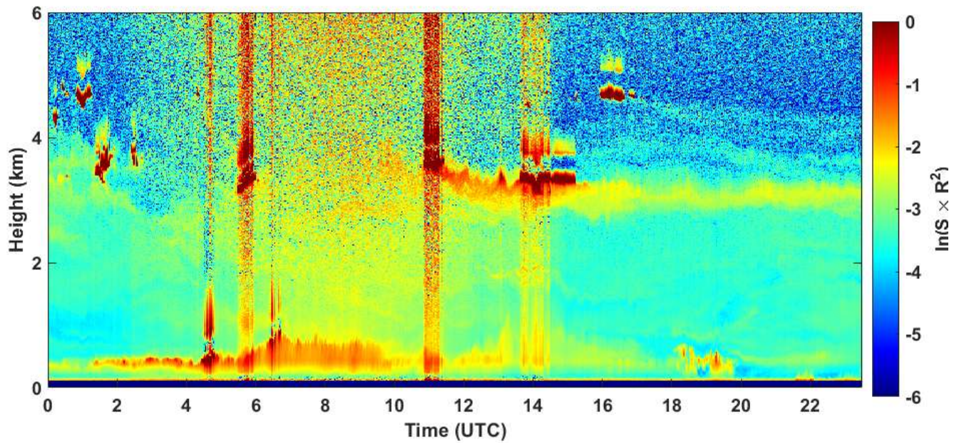
2020-09-08 RCS quick look CHM15k - ILVA LIDAR2 PARCHI
