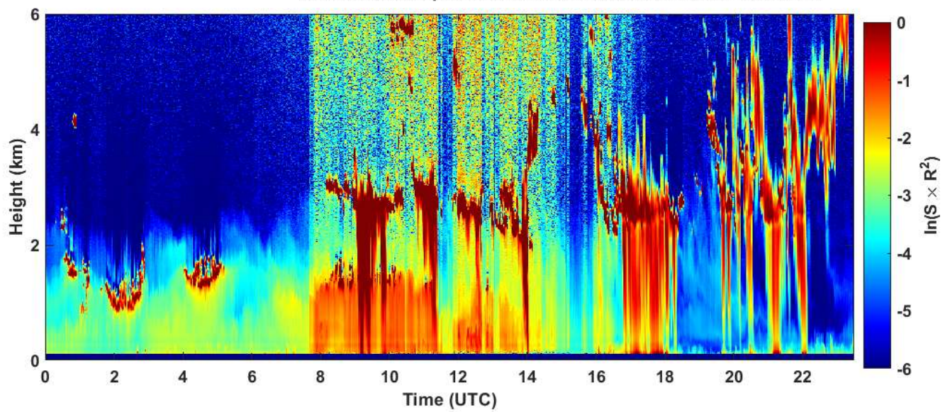
2020-09-28 RCS quick look CHM15k - ILVA LIDAR3 AGGLOMERATO
