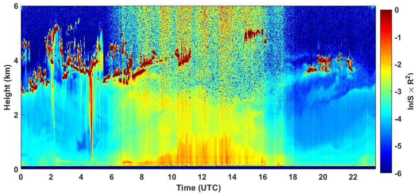
2020-09-18 RCS quick look CHM15k - ILVA LIDAR3 AGGLOMERATO
