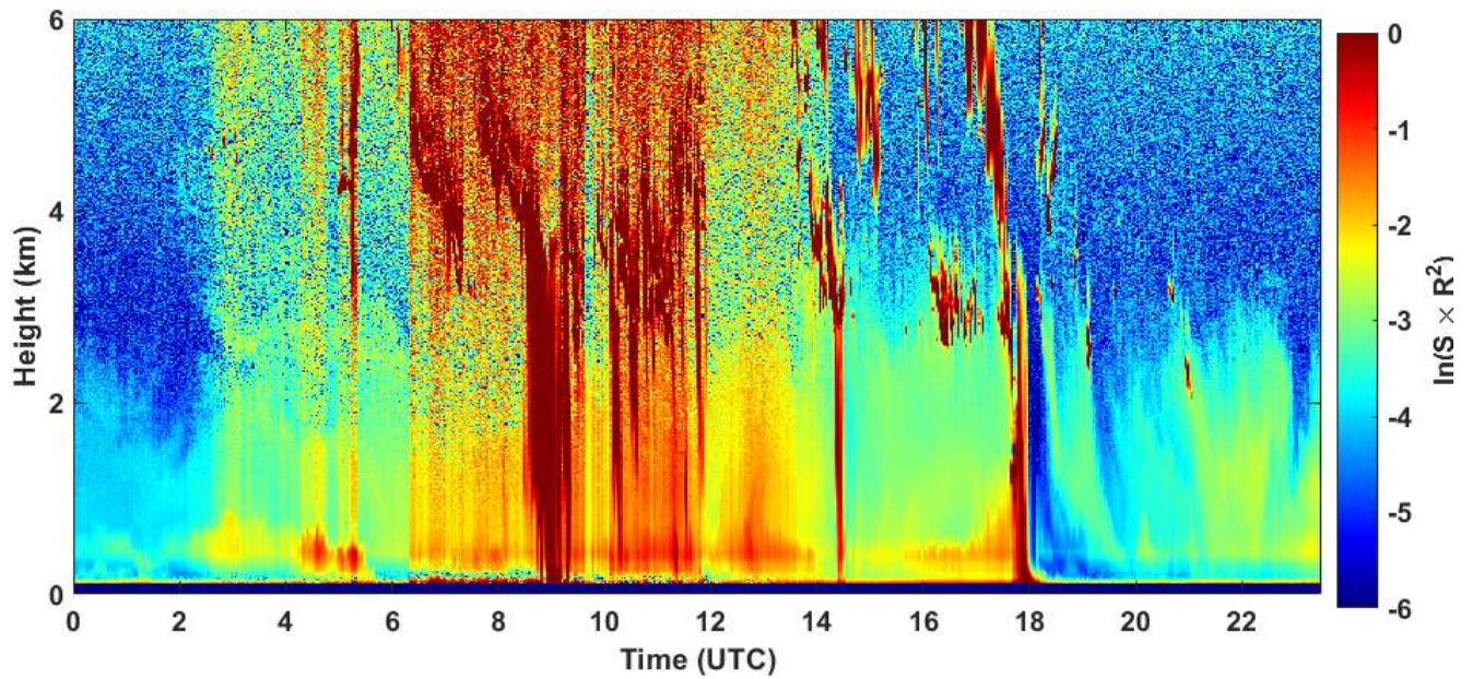
2020-09-26 RCS quick look CHM15k - ILVA LIDAR2 PARCHI
