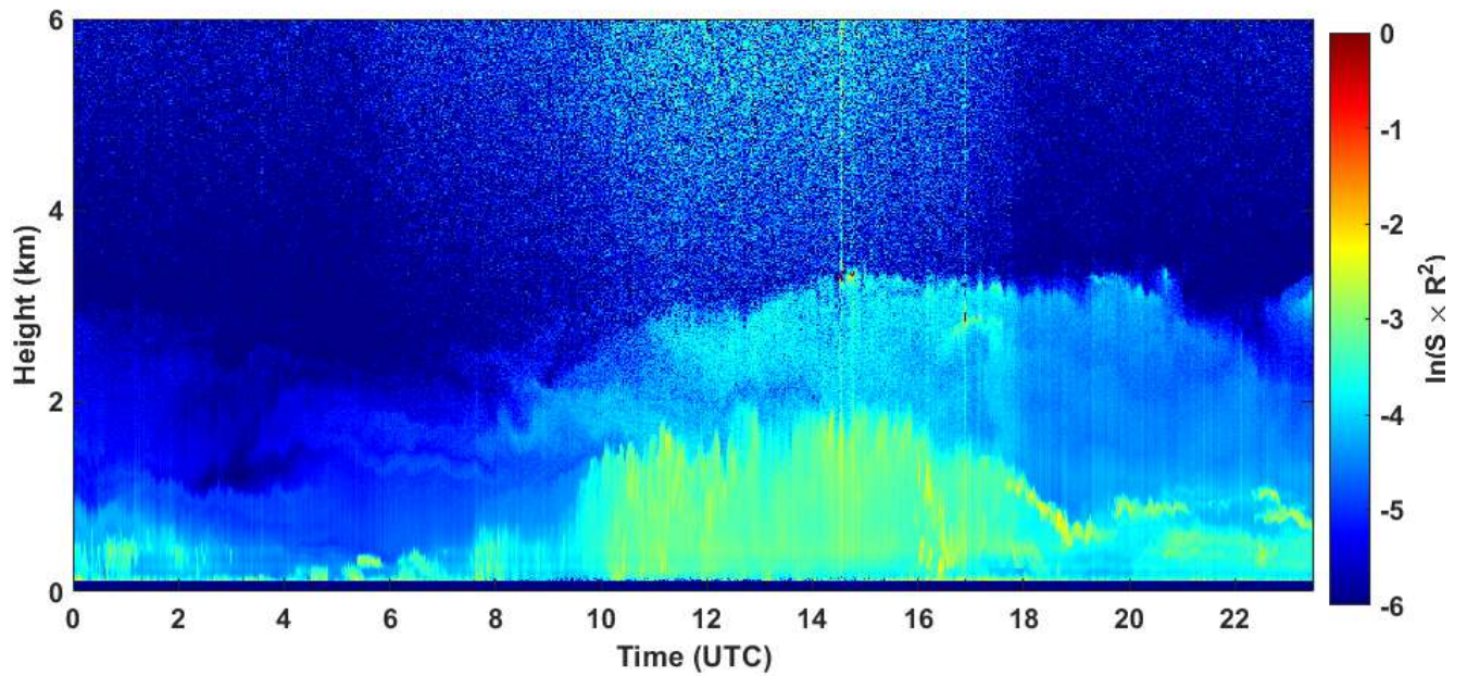
2020-09-12 RCS quick look CHM15k - ILVA LIDAR3 AGGLOMERATO
