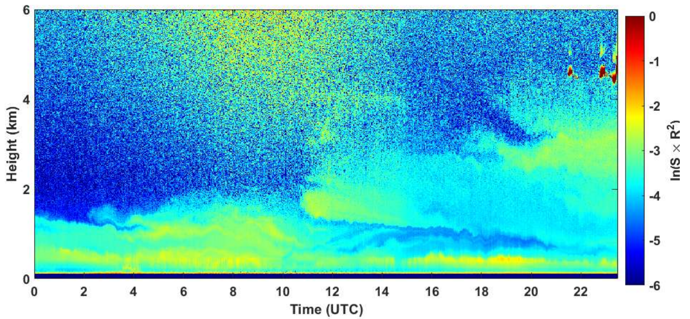
2020-09-06 RCS quick look CHM15k - ILVA LIDAR2 PARCHI
