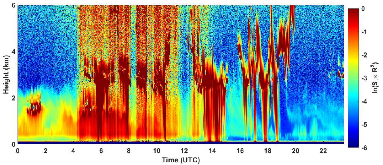
2020-09-28 RCS quick look CHM15k - ILVA LIDAR2 PARCHI
