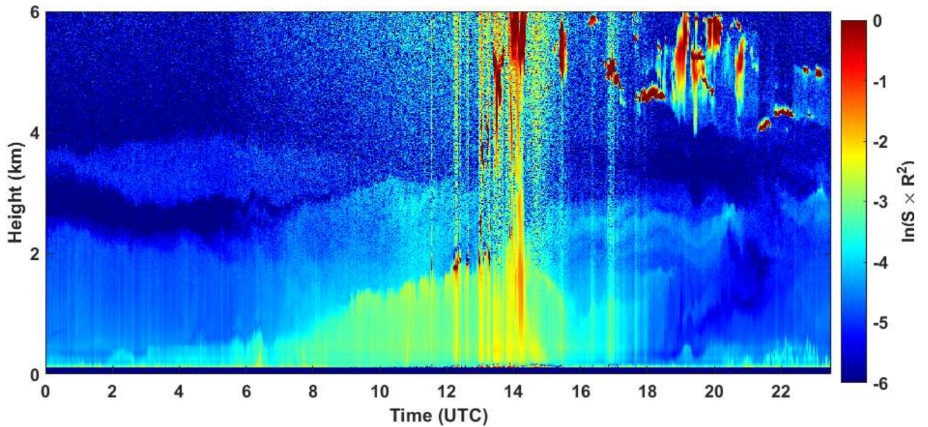
2020-09-14 RCS quick look CHM15k - ILVA LIDAR3 AGGLOMERATO
