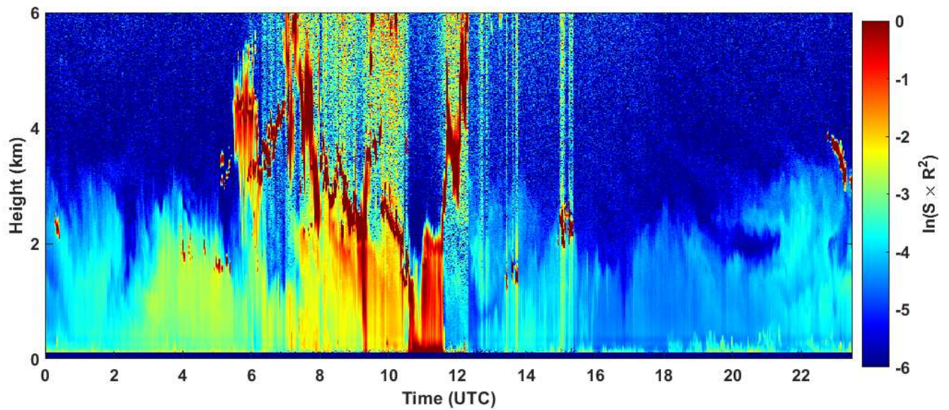
2020-09-26 RCS quick look CHM15k - ILVA LIDAR3 AGGLOMERATO
