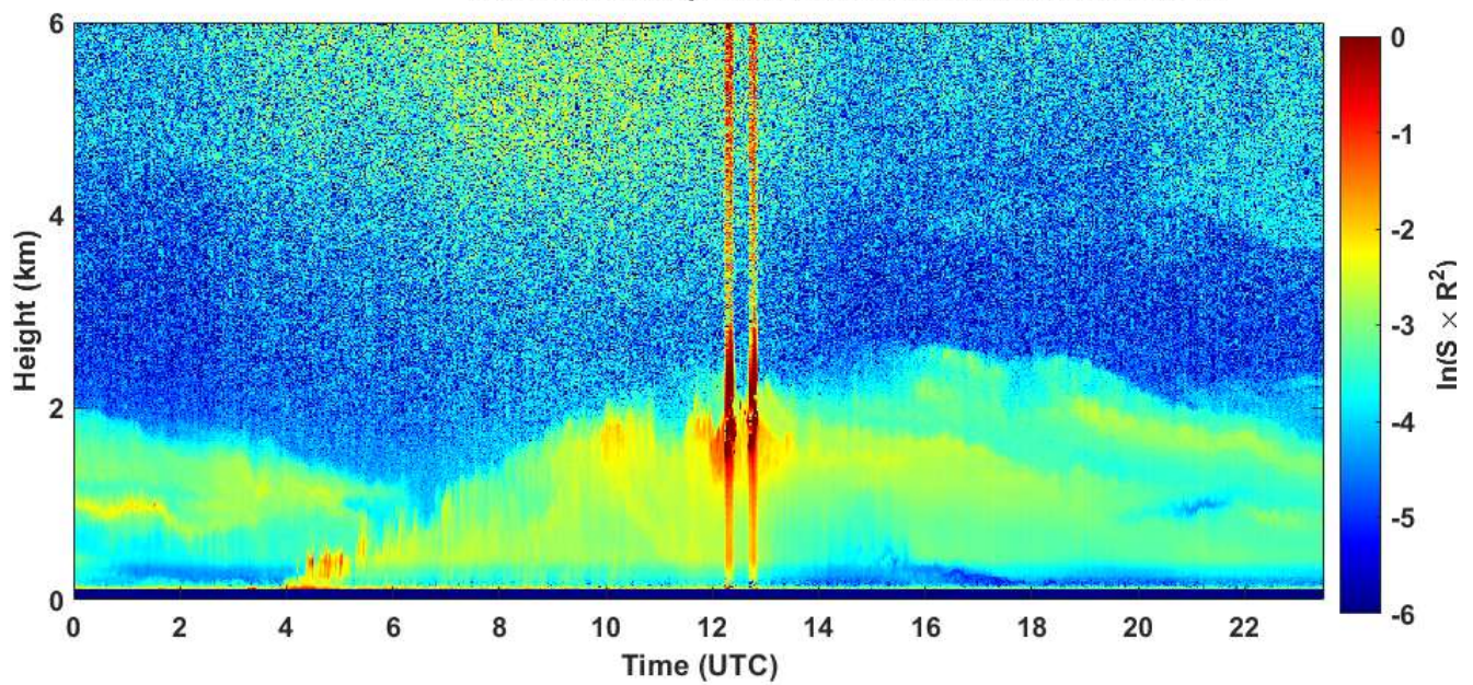
2020-09-30 RCS quick look CHM15k - ILVA LIDAR2 PARCHI
