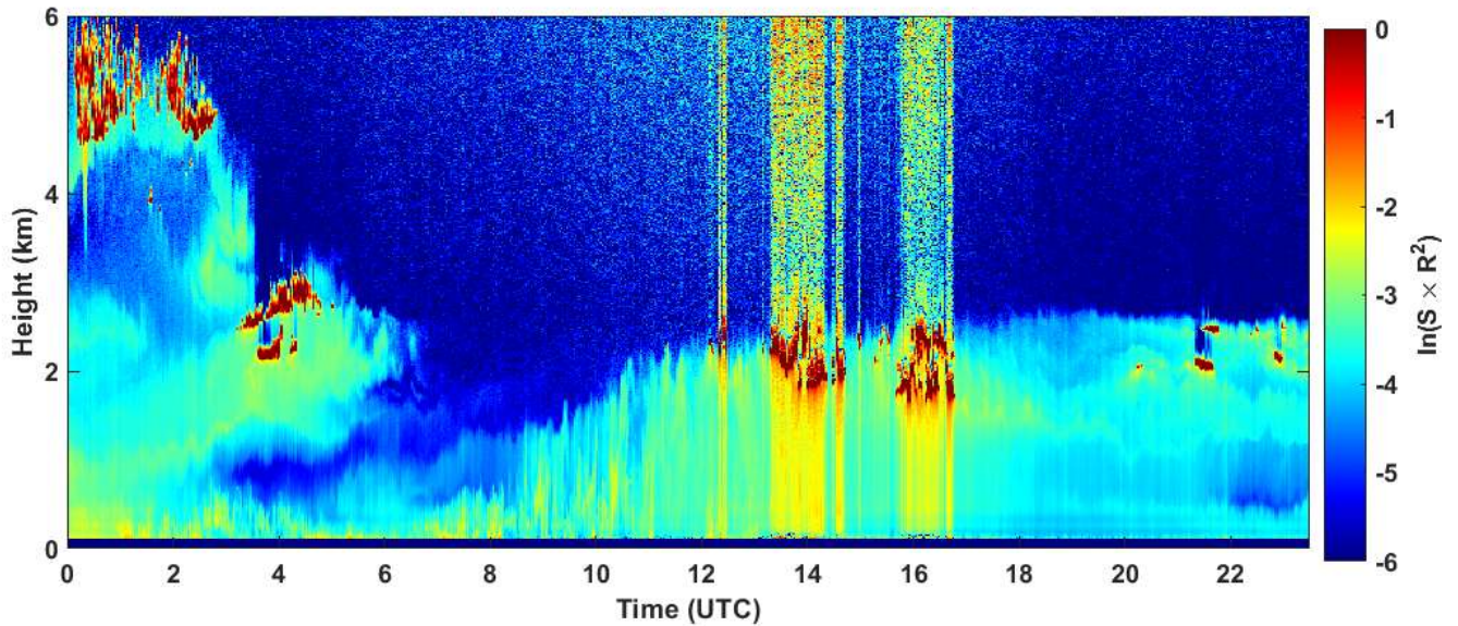
2020-09-02 RCS quick look CHM15k - ILVA LIDAR3 AGGLOMERATO
