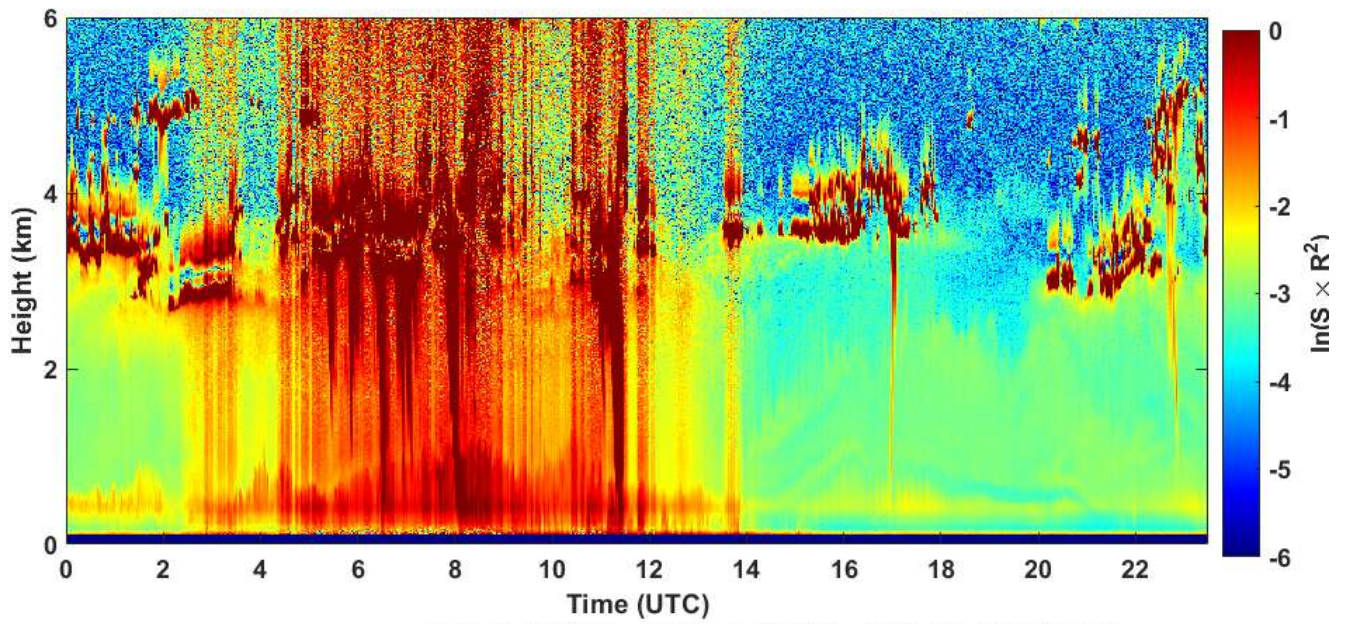
2020-09-18 RCS quick look CHM15k - ILVA LIDAR2 PARCHI
