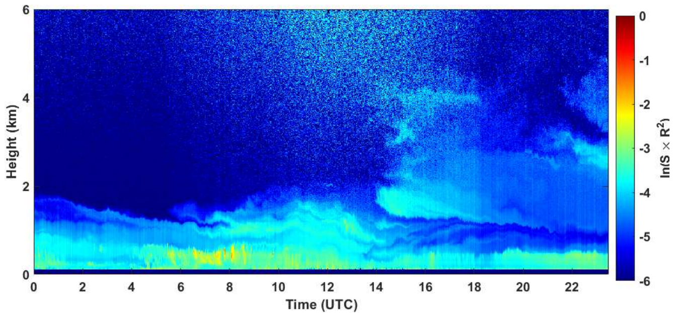
2020-09-06 RCS quick look CHM15k - ILVA LIDAR3 AGGLOMERATO
