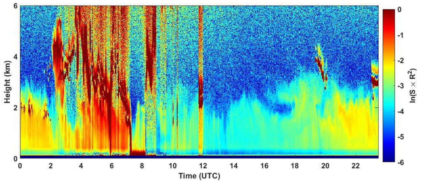
2020-09-26 RCS quick look CHM15k - ILVA LIDAR2 PARCHI
