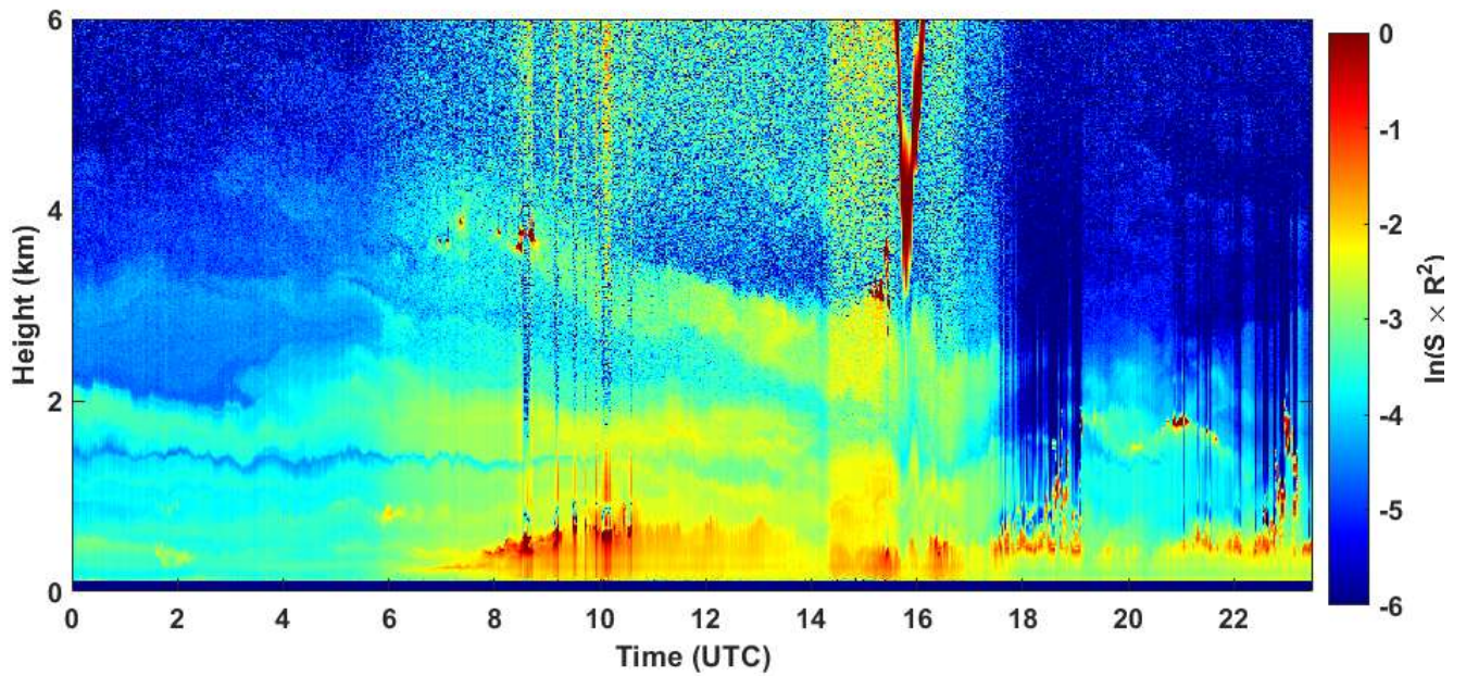
2020-09-22 RCS quick look CHM15k - ILVA LIDAR3 AGGLOMERATO
