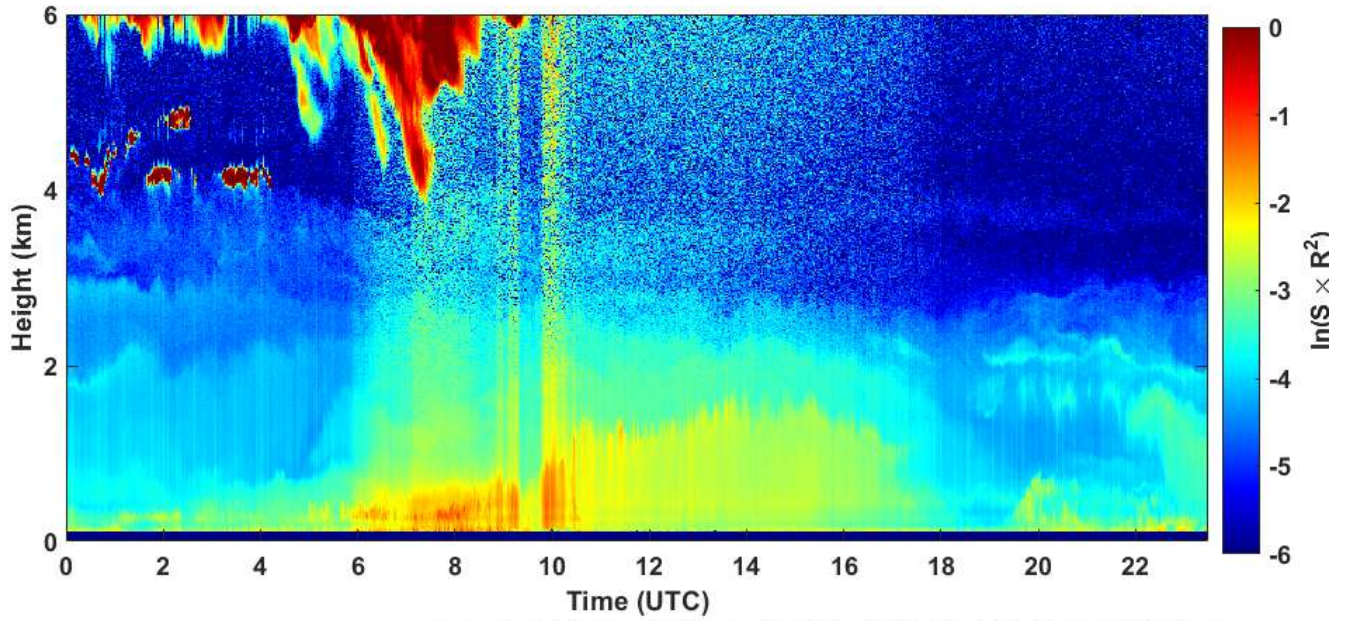
2020-09-20 RCS quick look CHM15k - ILVA LIDAR3 AGGLOMERATO
