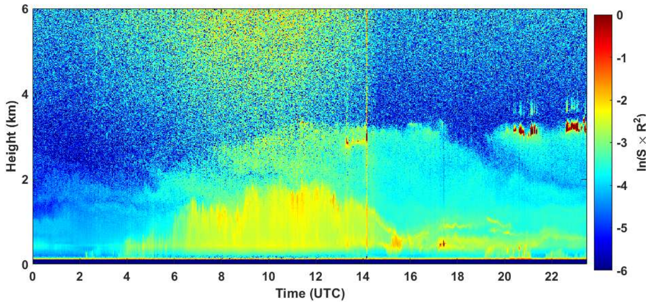
2020-09-12 RCS quick look CHM15k - ILVA LIDAR2 PARCHI
