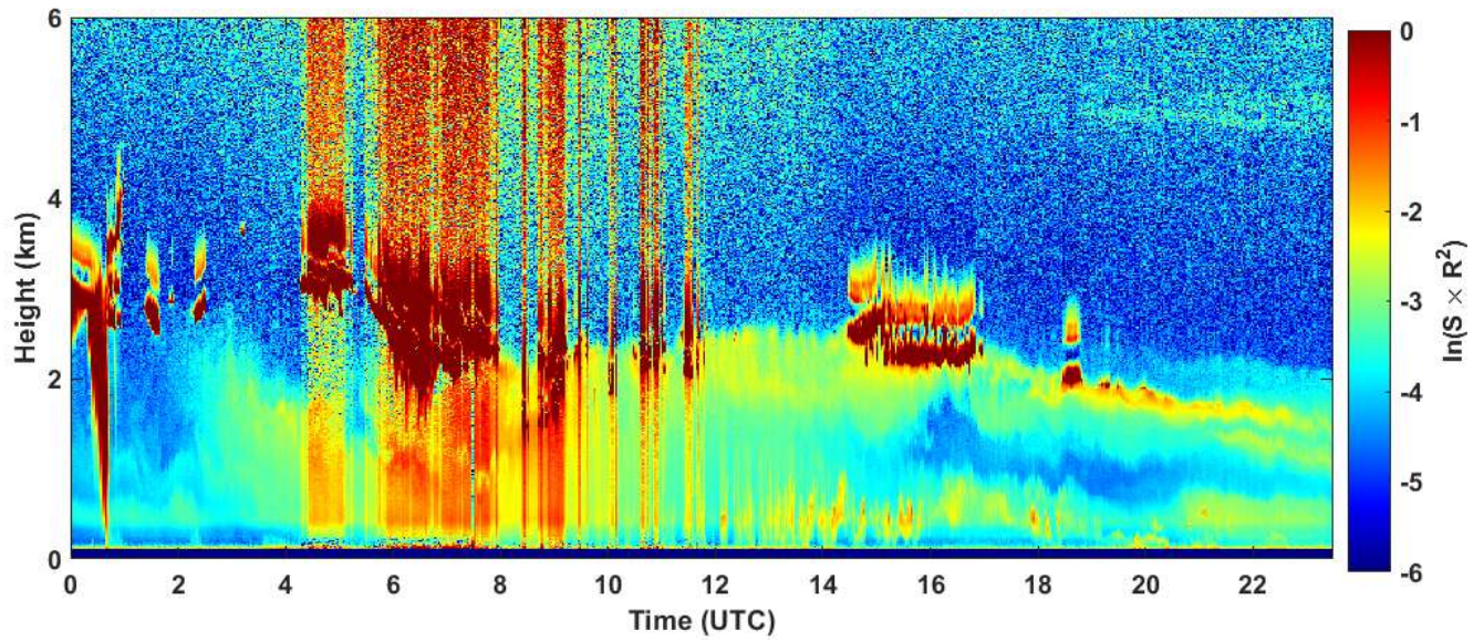
2020-09-29 RCS quick look CHM15k - ILVA LIDAR2 PARCHI
