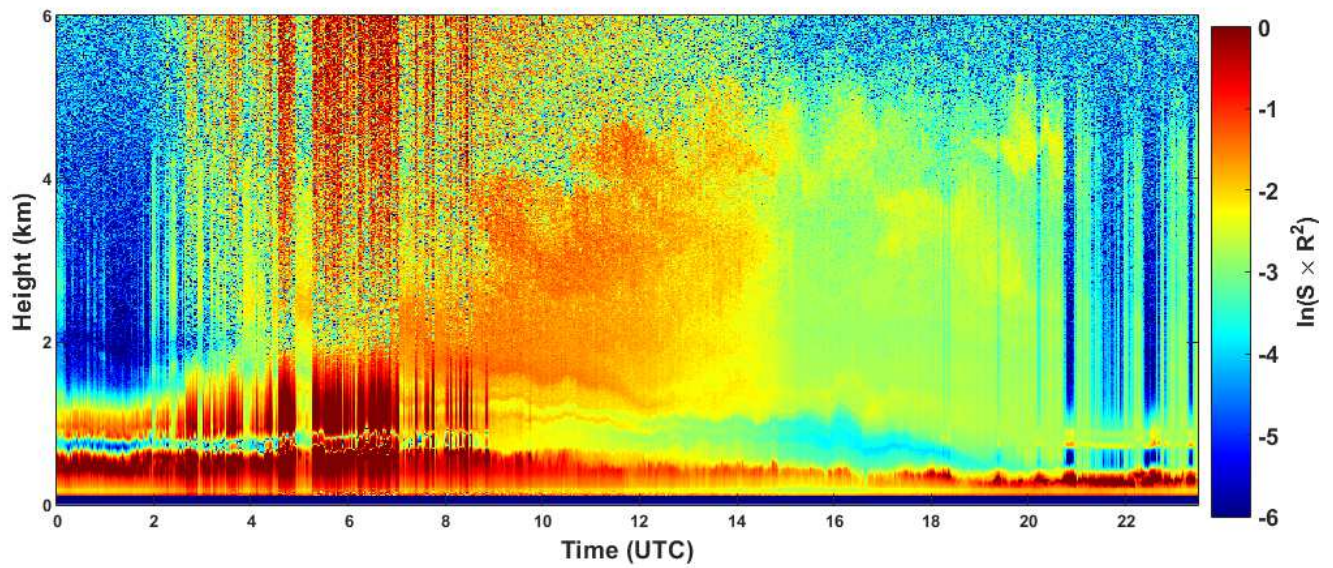
2020-08-30 RCS quick look CHM15k - ILVA LIDAR2 PARCHI
