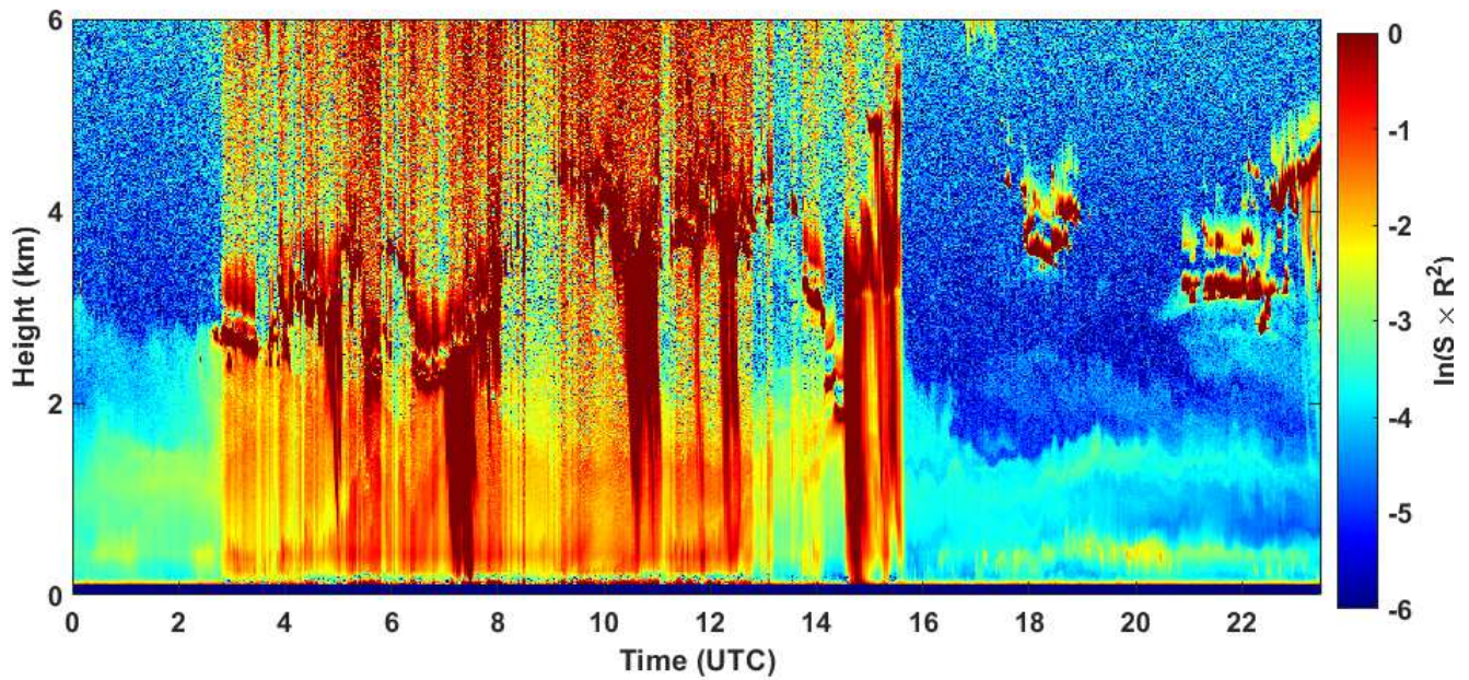
2020-08-06 RCS quick look CHM15k - ILVA LIDAR2 PARCHI
