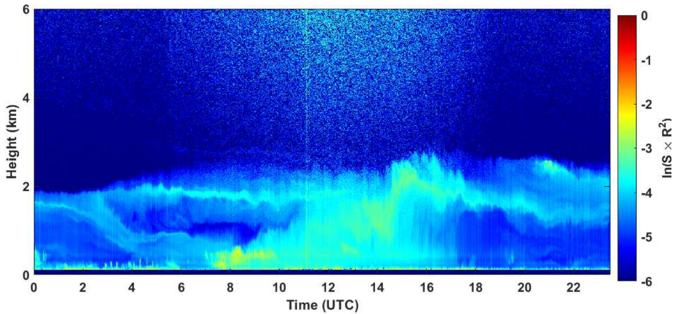
2020-08-28 RCS quick look CHM15k - ILVA LIDAR3 AGGLOMERATO
