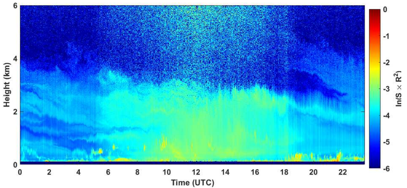
2020-08-14 RCS quick look CHM15k - ILVA LIDAR3 AGGLOMERATO
