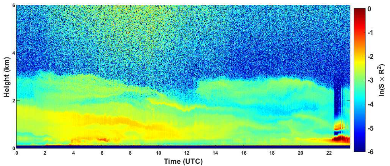
2020-08-28 RCS quick look CHM15k - ILVA LIDAR2 PARCHI
