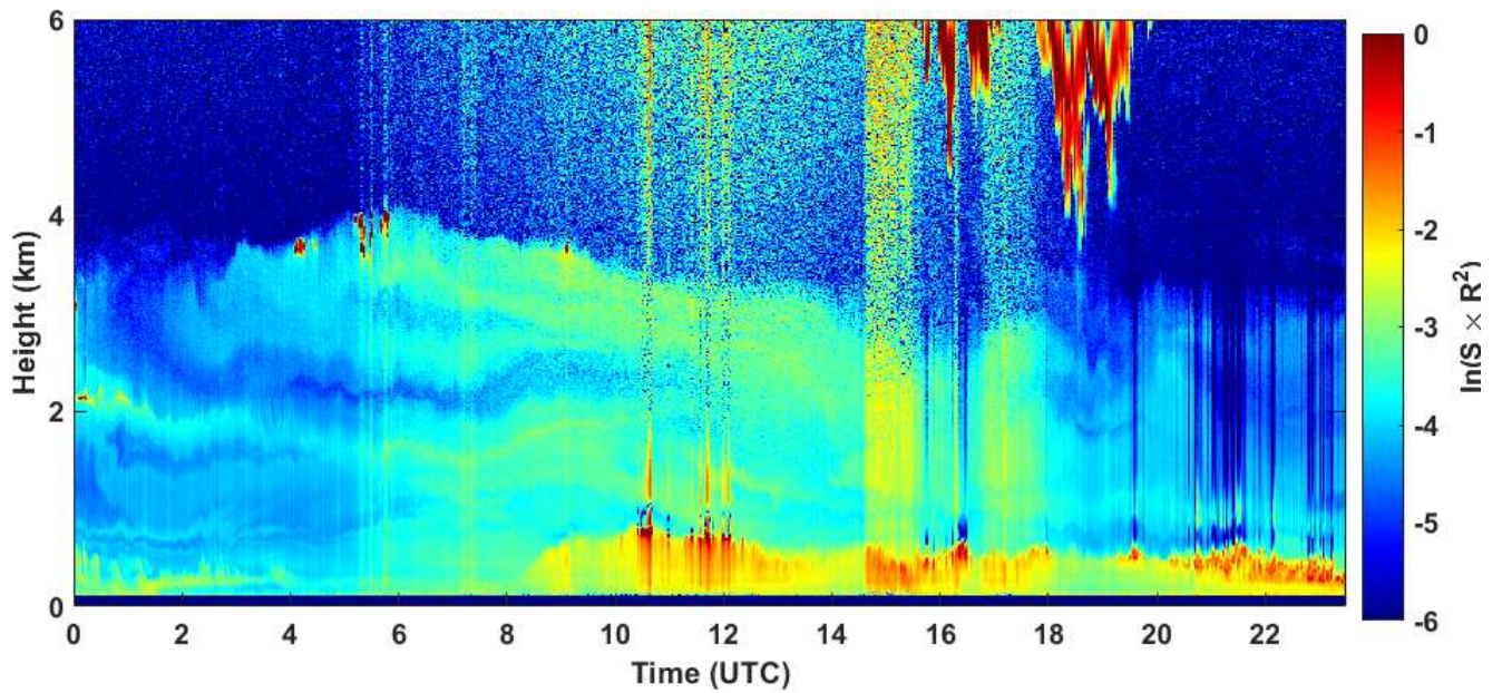
2020-08-18 RCS quick look CHM15k - ILVA LIDAR3 AGGLOMERATO
