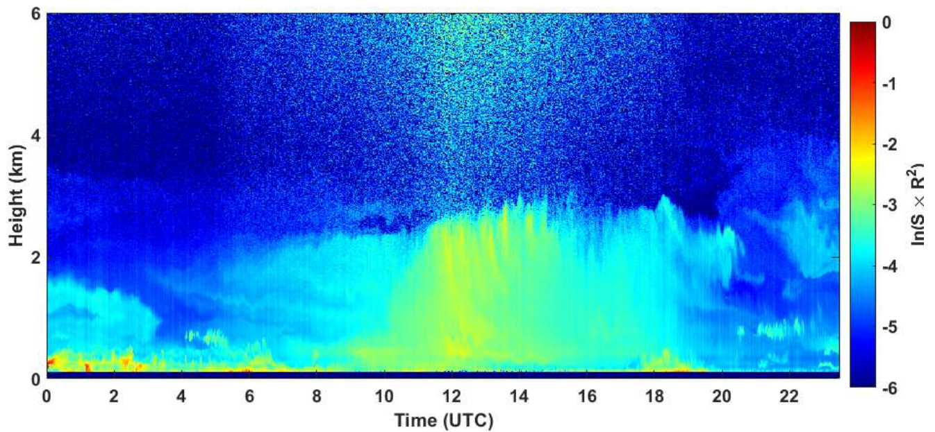
2020-08-12 RCS quick look CHM15k - ILVA LIDAR3 AGGLOMERATO
