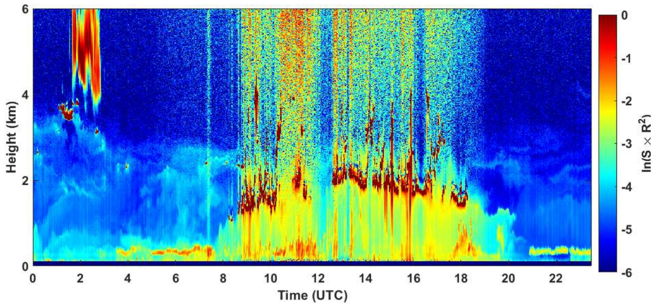
2020-08-08 RCS quick look CHM15k - ILVA LIDAR3 AGGLOMERATO
