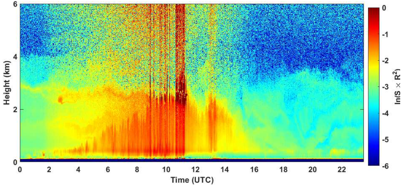
2020-08-02 RCS quick look CHM15k - ILVA LIDAR2 PARCHI
