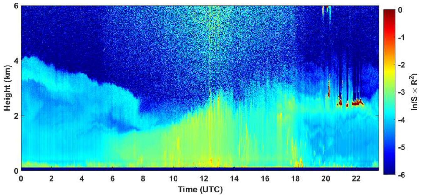
2020-08-16 RCS quick look CHM15k - ILVA LIDAR3 AGGLOMERATO
