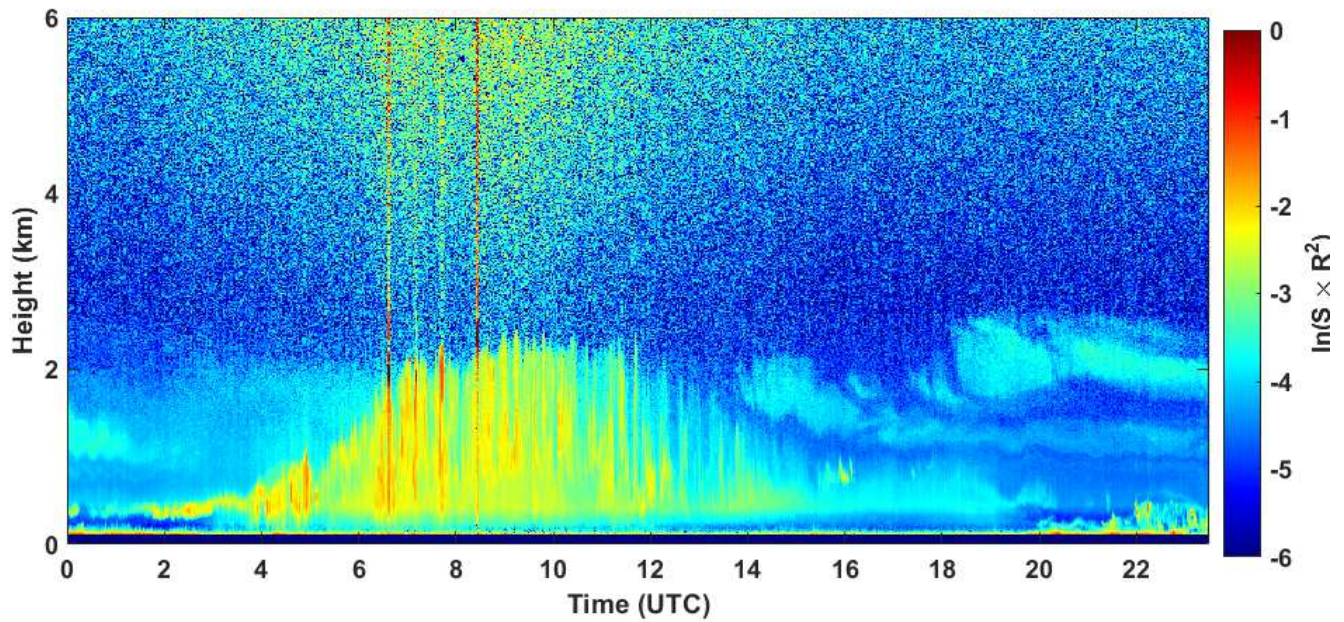
2020-08-22 RCS quick look CHM15k - ILVA LIDAR2 PARCHI
