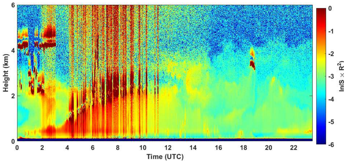
2020-08-08 RCS quick look CHM15k - ILVA LIDAR2 PARCHI
