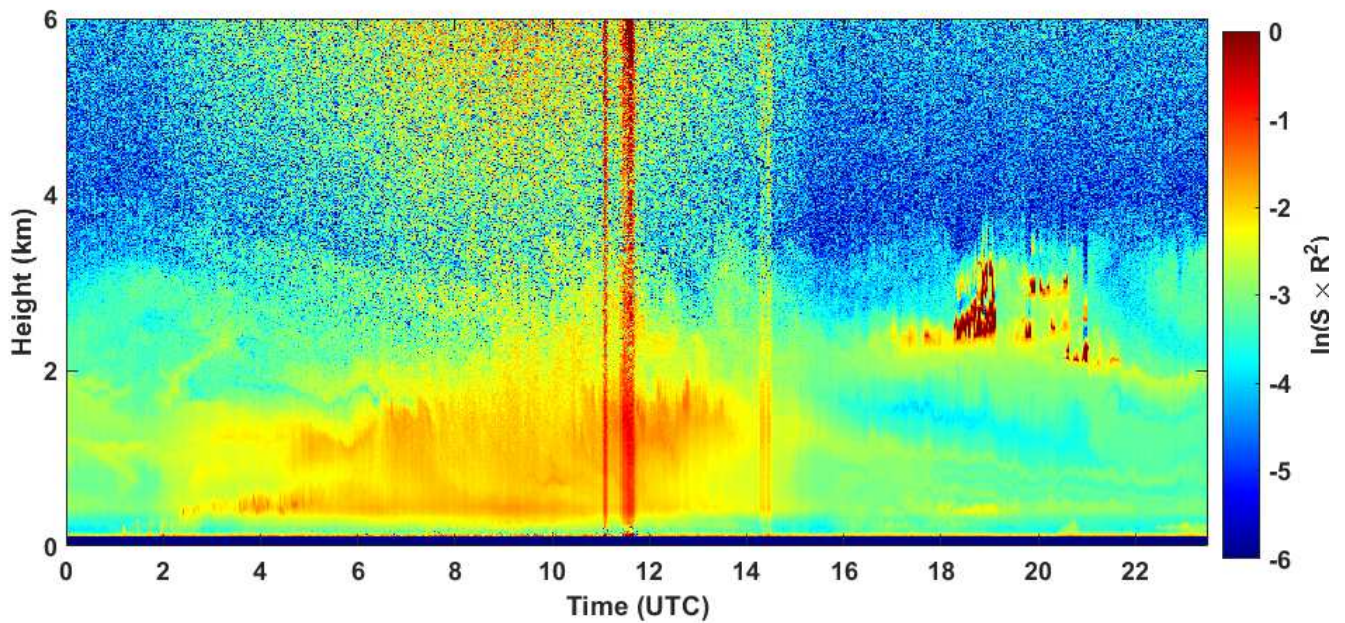
2020-08-16 RCS quick look CHM15k - ILVA LIDAR2 PARCHI
