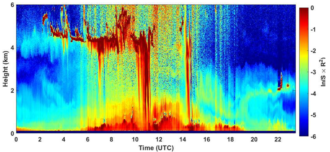
2020-08-04 RCS quick look CHM15k - ILVA LIDAR3 AGGLOMERATO
