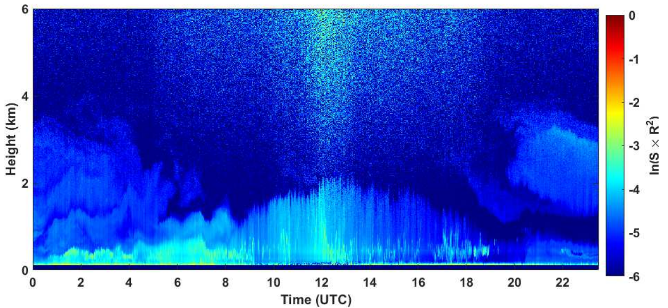
2020-08-02 RCS quick look CHM15k - ILVA LIDAR3 AGGLOMERATO
