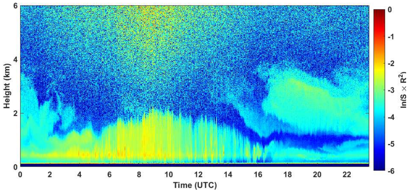
2020-08-02 RCS quick look CHM15k - ILVA LIDAR2 PARCHI
