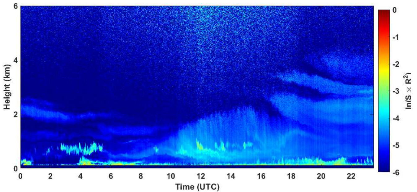
2020-08-22 RCS quick look CHM15k - ILVA LIDAR3 AGGLOMERATO
