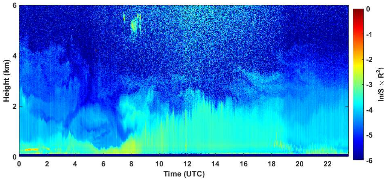
2020-08-10 RCS quick look CHM15k - ILVA LIDAR3 AGGLOMERATO
