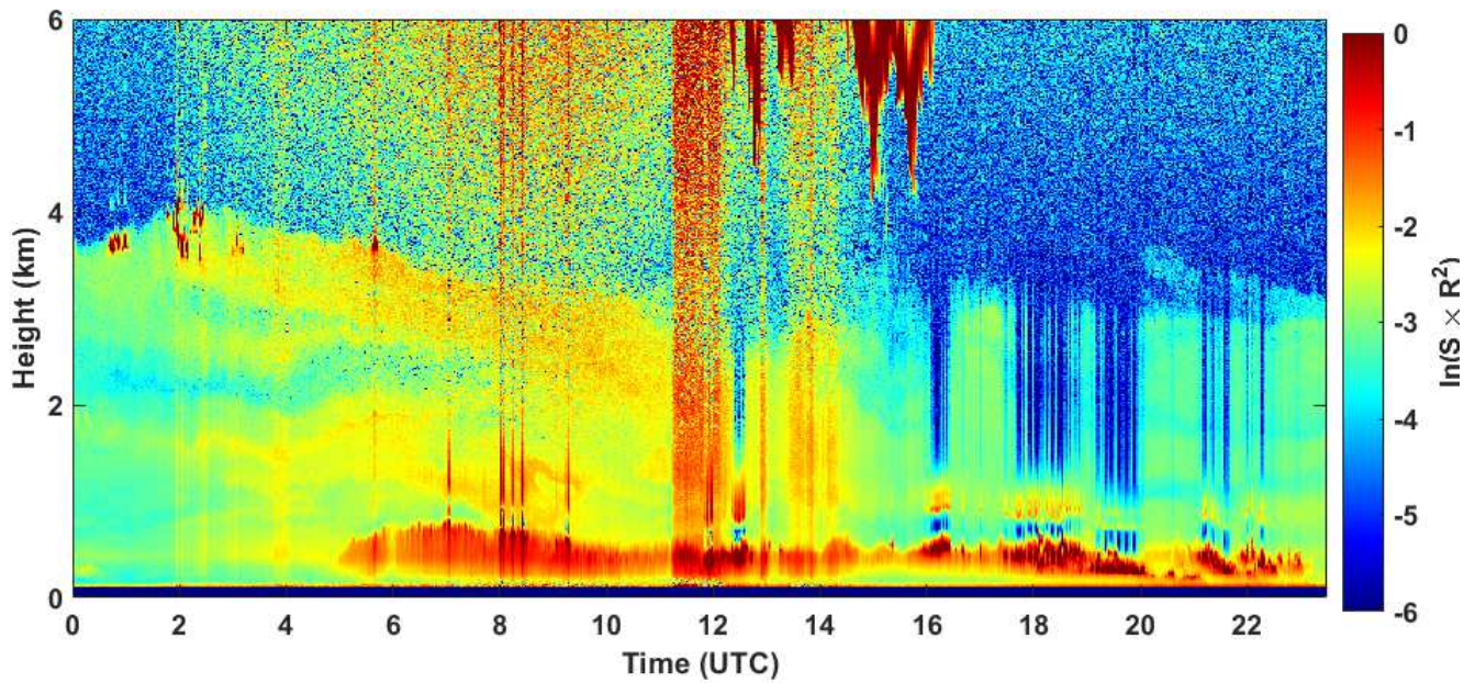
2020-08-18 RCS quick look CHM15k - ILVA LIDAR2 PARCHI
