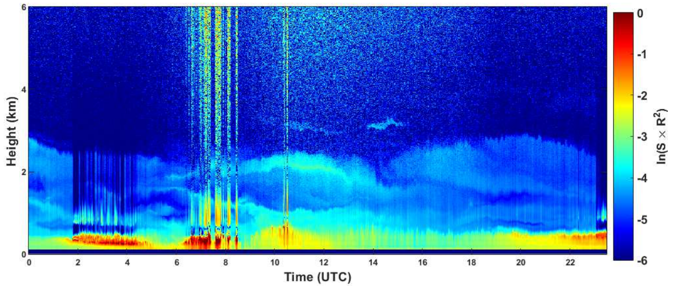
2020-08-30 RCS quick look CHM15k - ILVA LIDAR3 AGGLOMERATO
