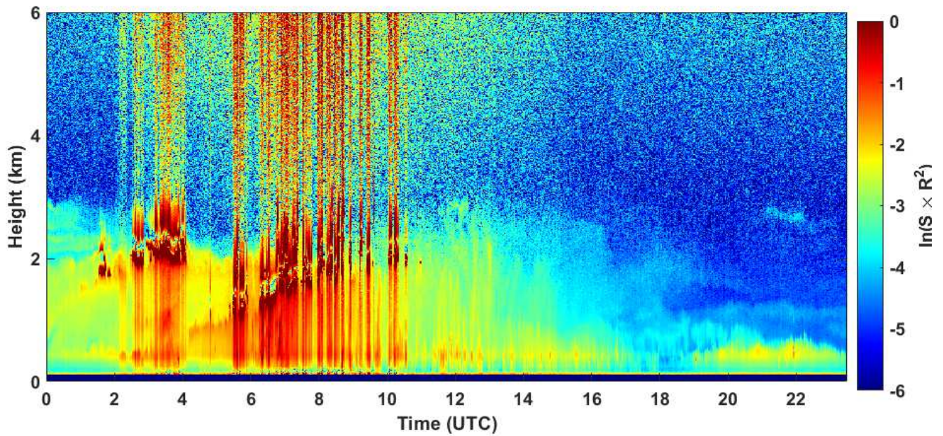
2020-08-26 RCS quick look CHM15k - ILVA LIDAR2 PARCHI
