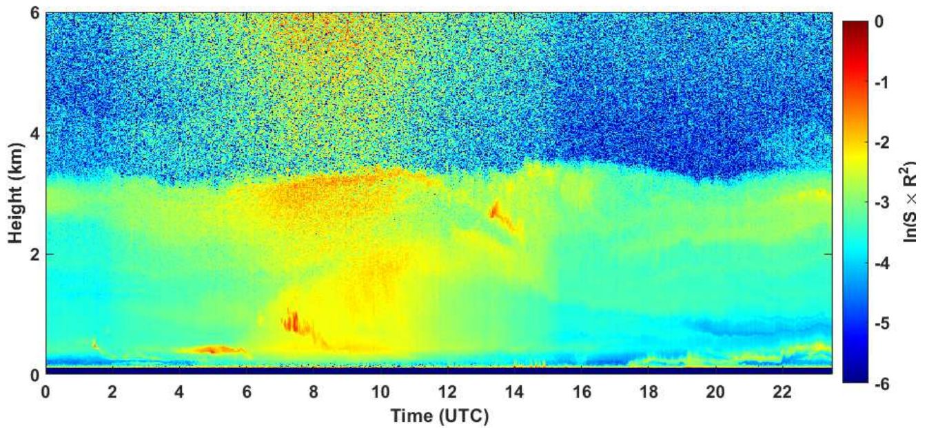
2020-08-24 RCS quick look CHM15k - ILVA LIDAR2 PARCHI
