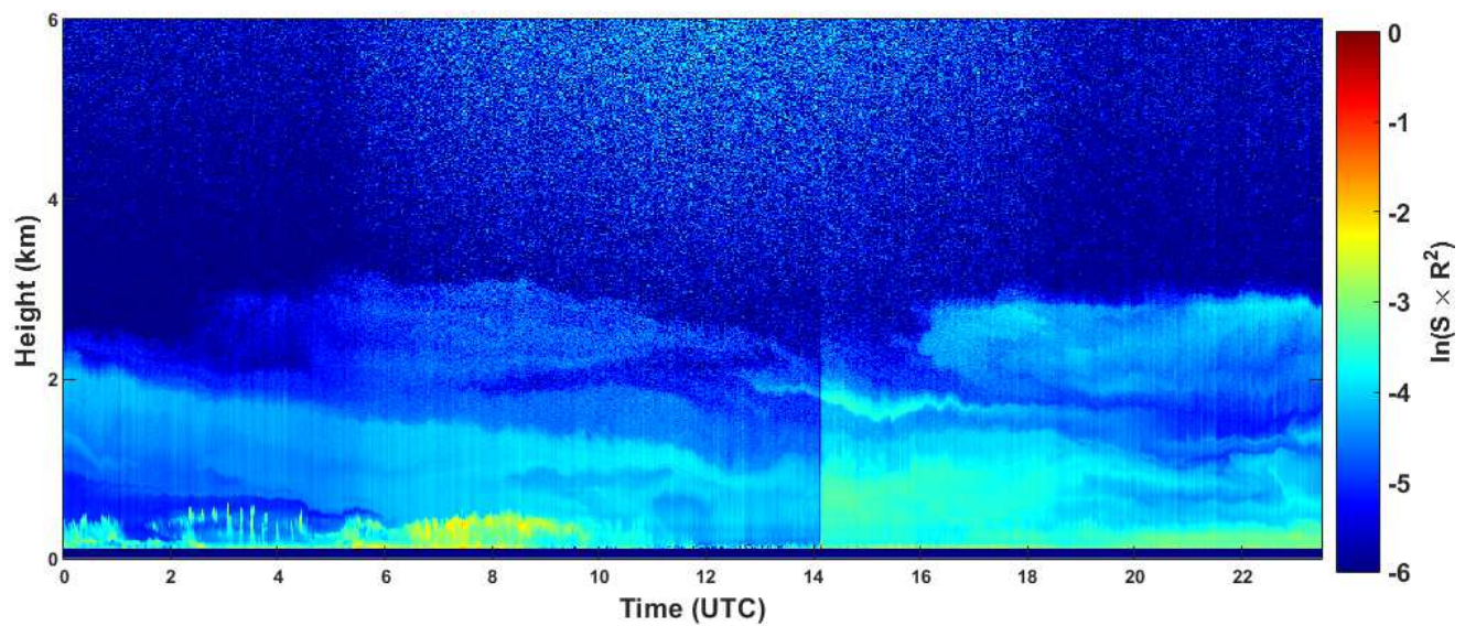
2020-08-28 RCS quick look CHM15k - ILVA LIDAR3 AGGLOMERATO
