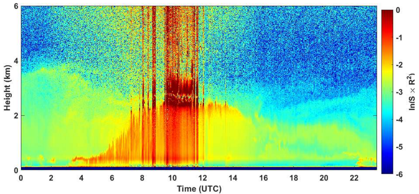
2020-08-10 RCS quick look CHM15k - ILVA LIDAR2 PARCHI
