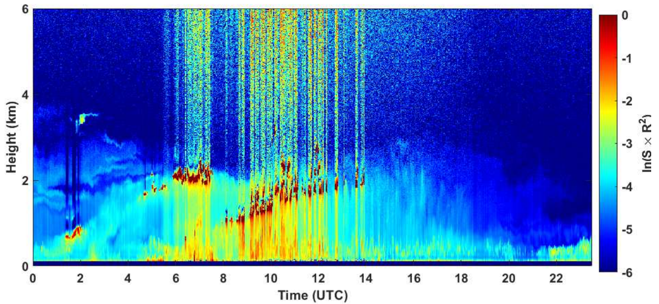
2020-08-26 RCS quick look CHM15k - ILVA LIDAR3 AGGLOMERATO
