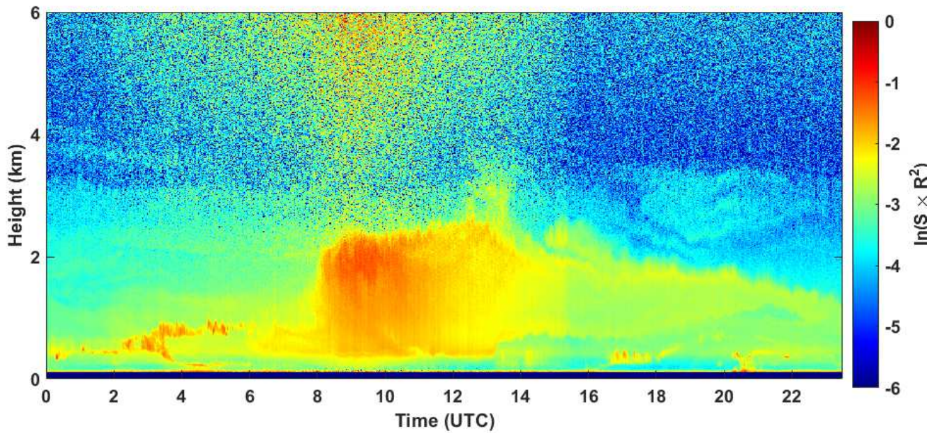
2020-08-12 RCS quick look CHM15k - ILVA LIDAR2 PARCHI
