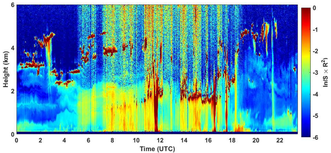
2020-08-06 RCS quick look CHM15k - ILVA LIDAR3 AGGLOMERATO
