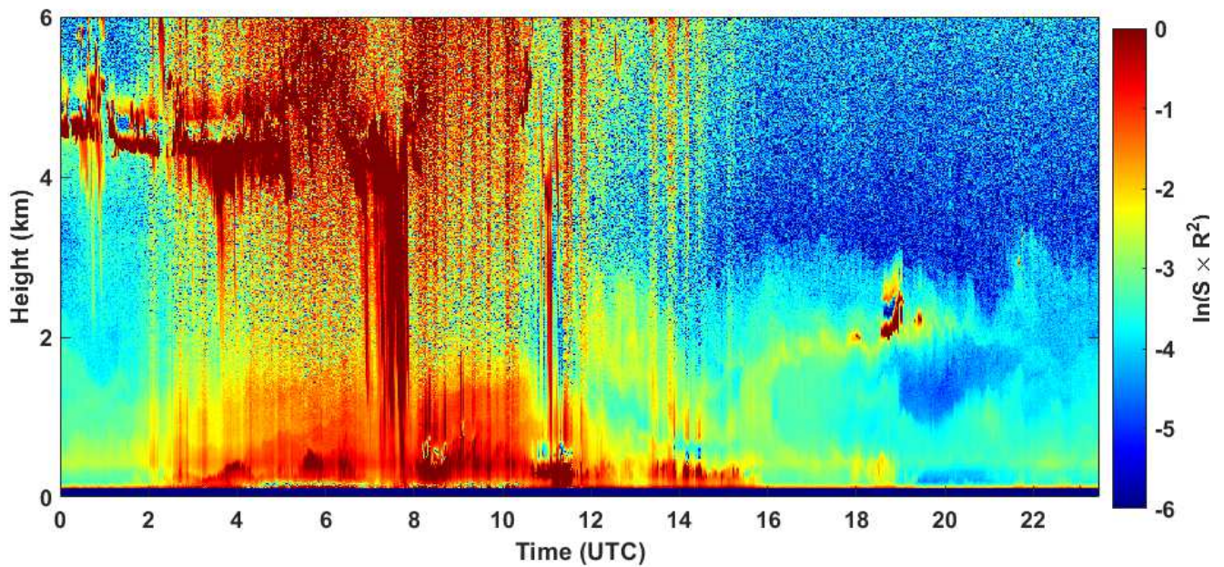
2020-08-04 RCS quick look CHM15k - ILVA LIDAR2 PARCHI
