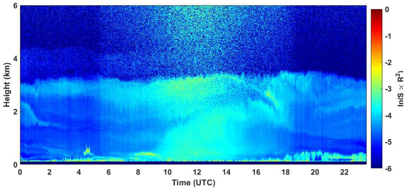
2020-08-24 RCS quick look CHM15k - ILVA LIDAR3 AGGLOMERATO
