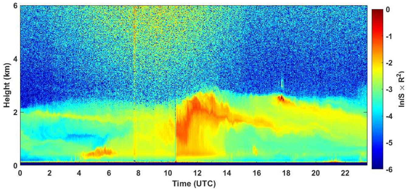
2020-08-28 RCS quick look CHM15k - ILVA LIDAR2 PARCHI
