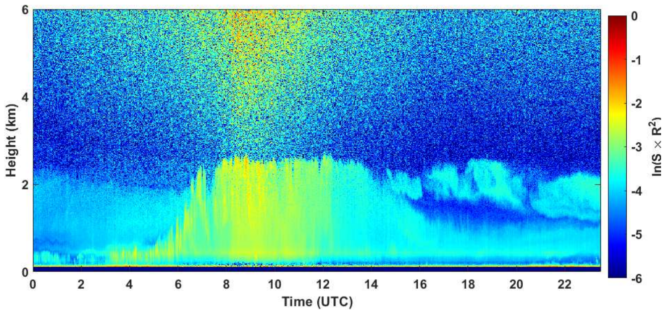
2020-07-28 RCS quick look CHM15k - ILVA LIDAR2 PARCHI
