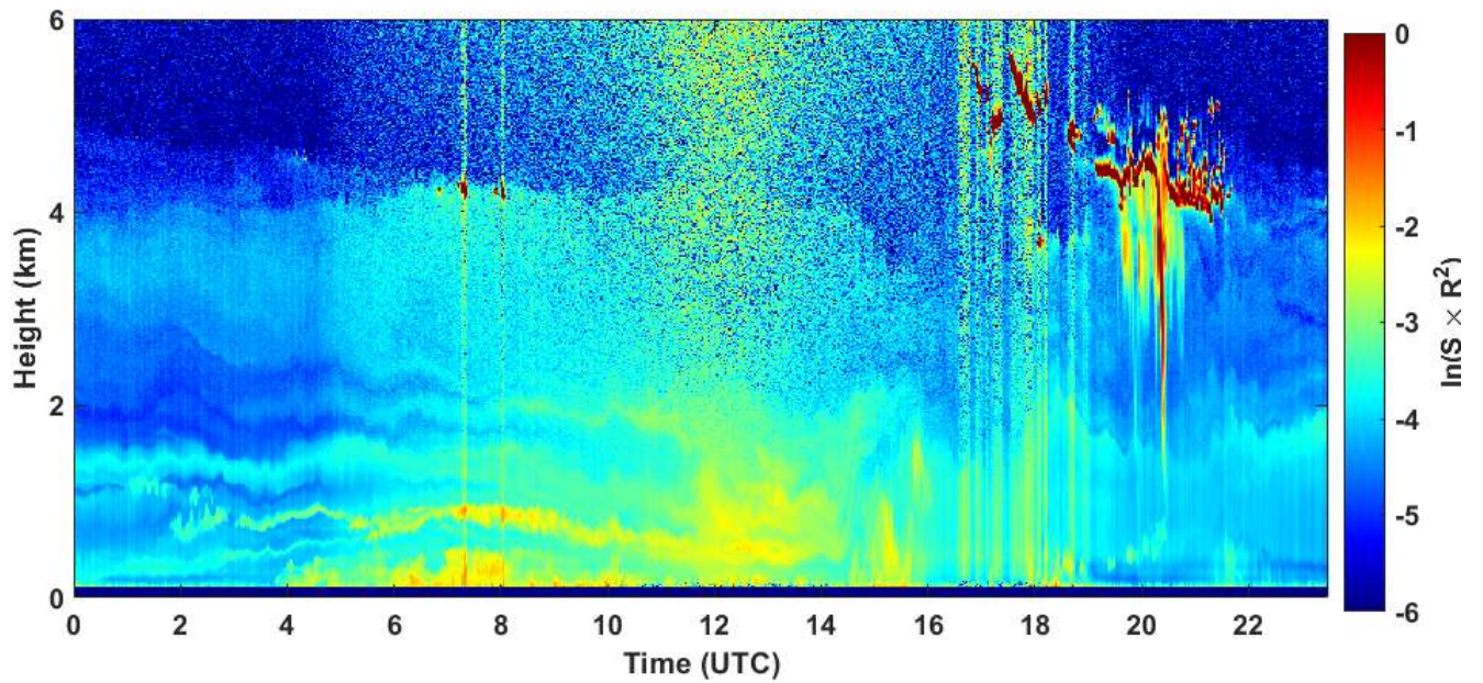
2020-07-04 RCS quick look CHM15k - ILVA LIDAR3 AGGLOMERATO
