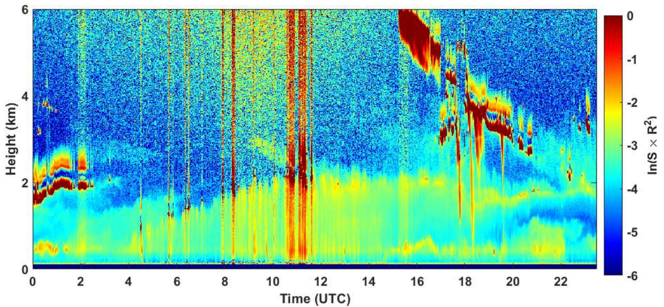
2020-07-18 RCS quick look CHM15k - ILVA LIDAR2 PARCHI
