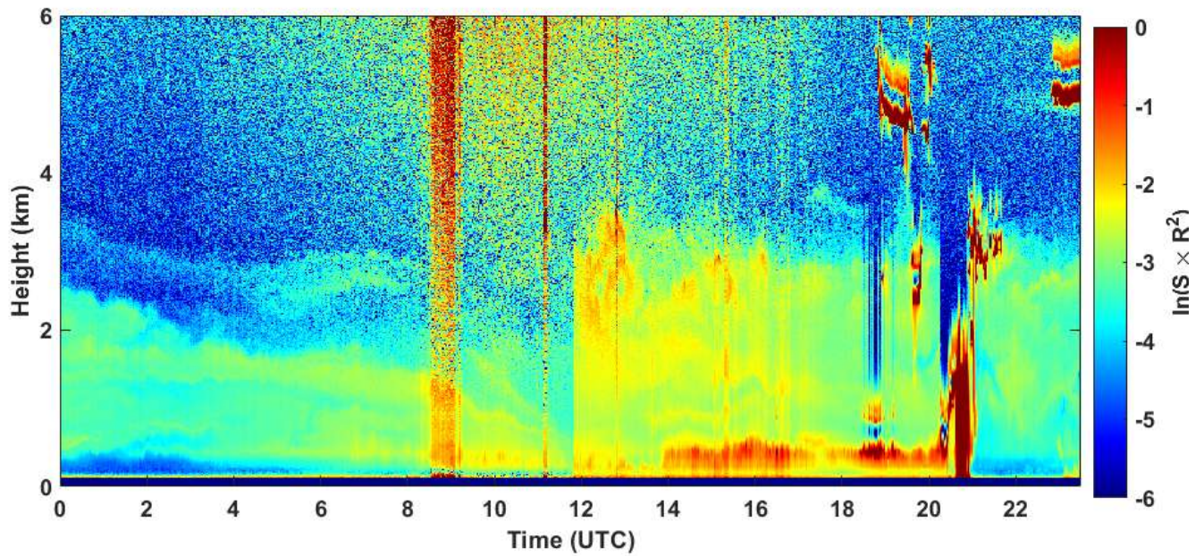
2020-07-16 RCS quick look CHM15k - ILVA LIDAR2 PARCHI
