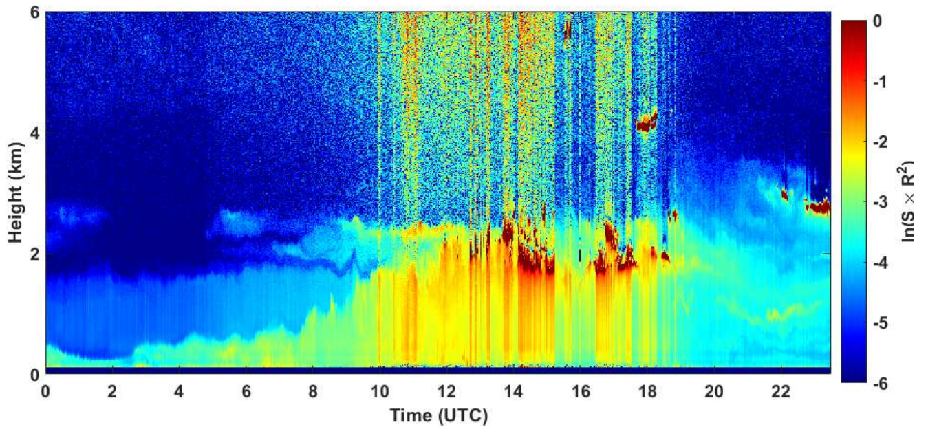
2020-07-14 RCS quick look CHM15k - ILVA LIDAR3 AGGLOMERATO
