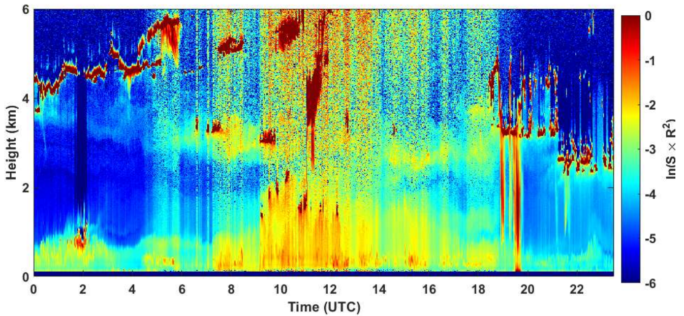
2020-07-06 RCS quick look CHM15k - ILVA LIDAR3 AGGLOMERATO
