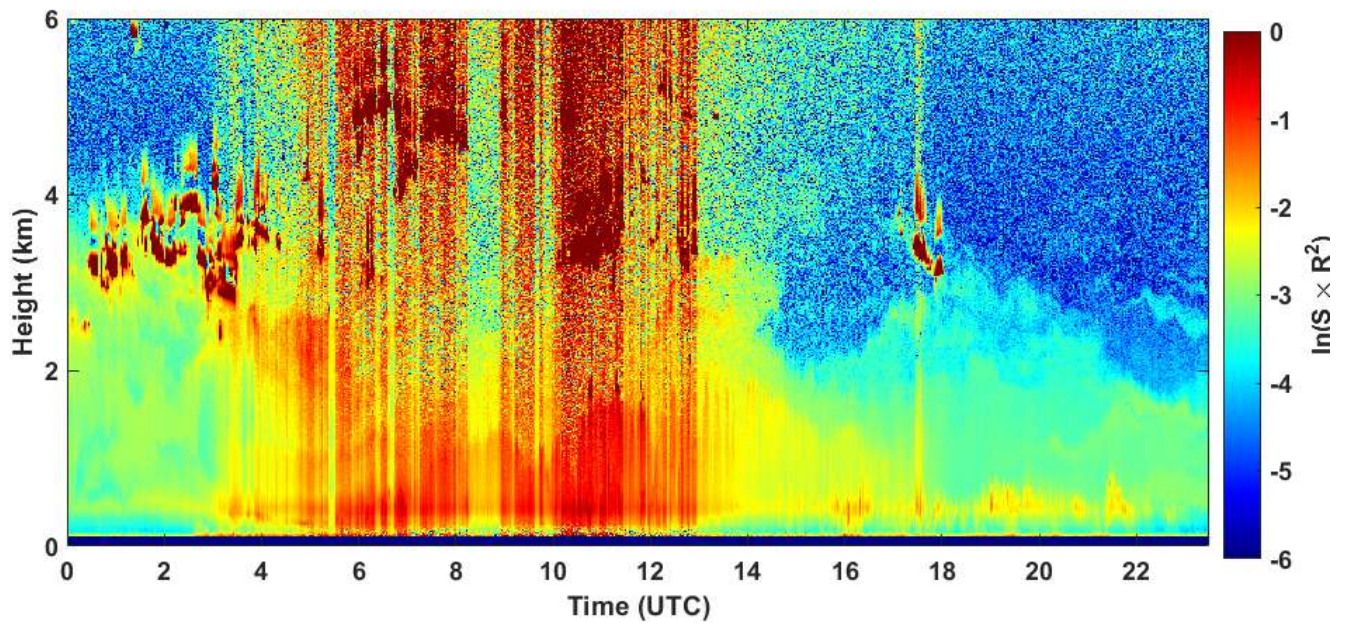
2020-07-06 RCS quick look CHM15k - ILVA LIDAR2 PARCHI
