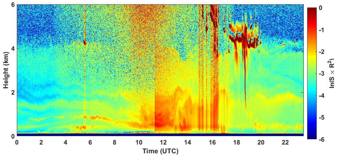
2020-07-04 RCS quick look CHM15k - ILVA LIDAR2 PARCHI
