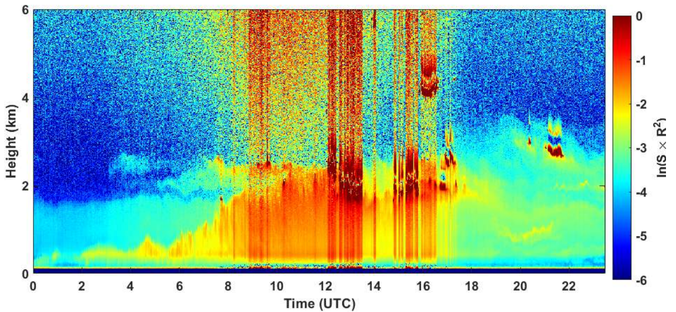
2020-07-14 RCS quick look CHM15k - ILVA LIDAR2 PARCHI
