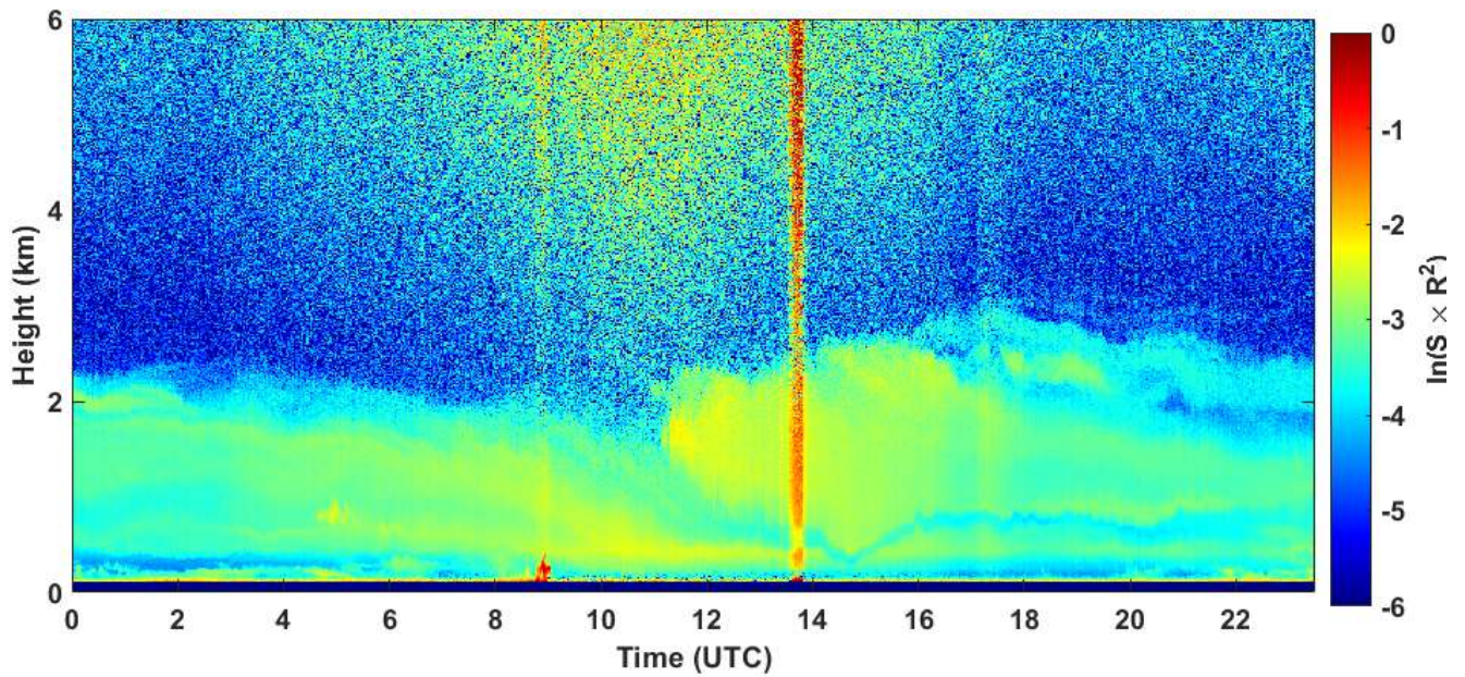
2020-07-12 RCS quick look CHM15k - ILVA LIDAR2 PARCHI
