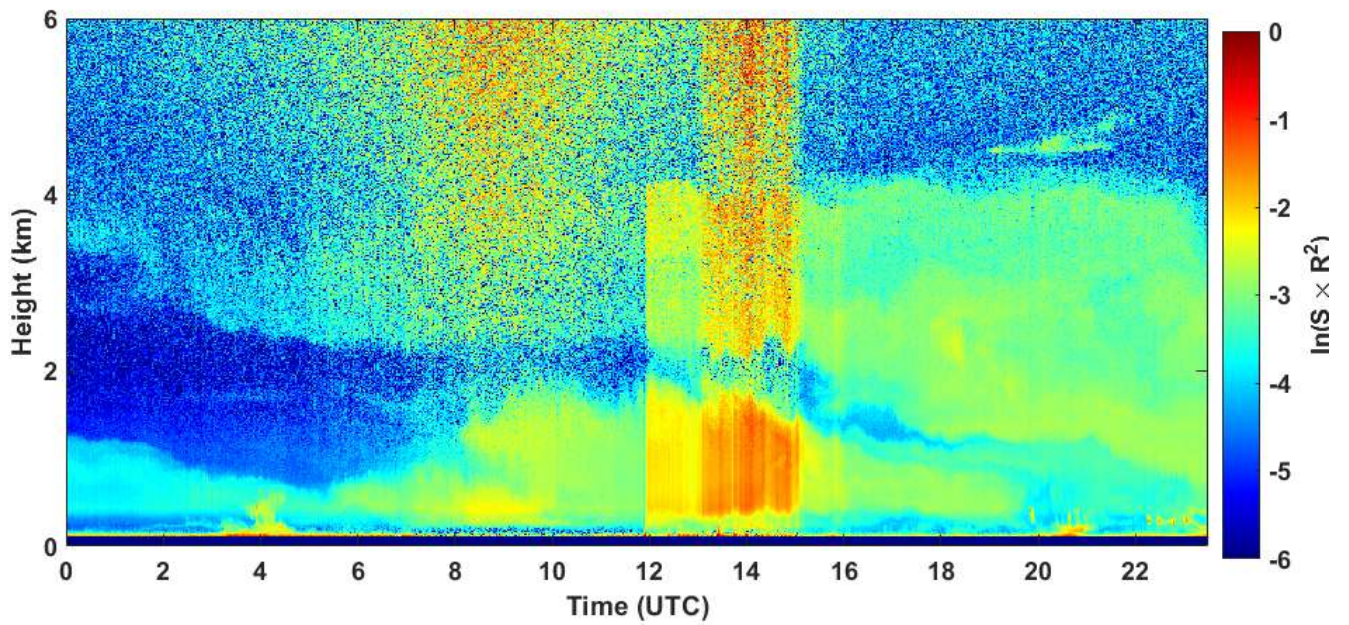
2020-07-30 RCS quick look CHM15k - ILVA LIDAR2 PARCHI
