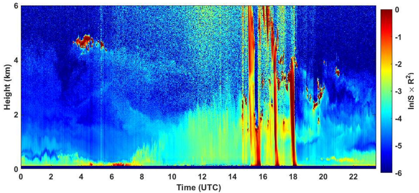
2020-07-26 RCS quick look CHM15k - ILVA LIDAR3 AGGLOMERATO
