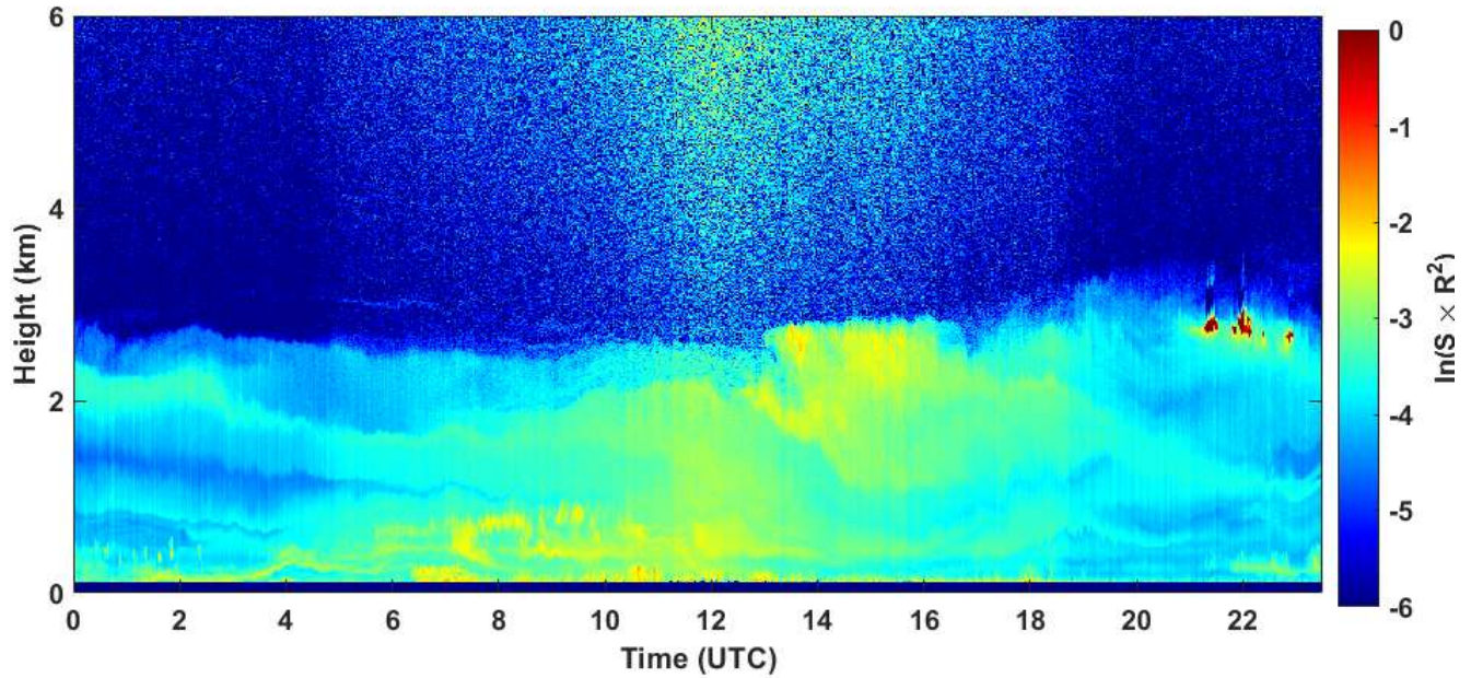
2020-07-02 RCS quick look CHM15k - ILVA LIDAR3 AGGLOMERATO
