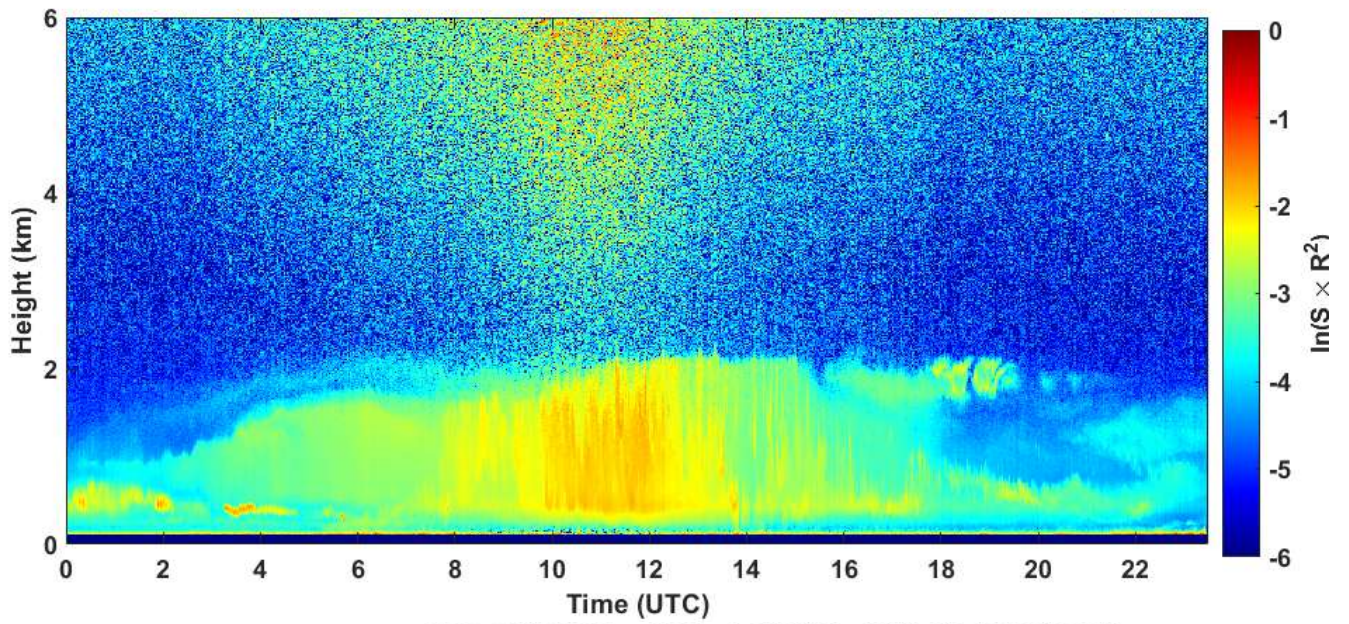
2020-07-10 RCS quick look CHM15k - ILVA LIDAR2 PARCHI
