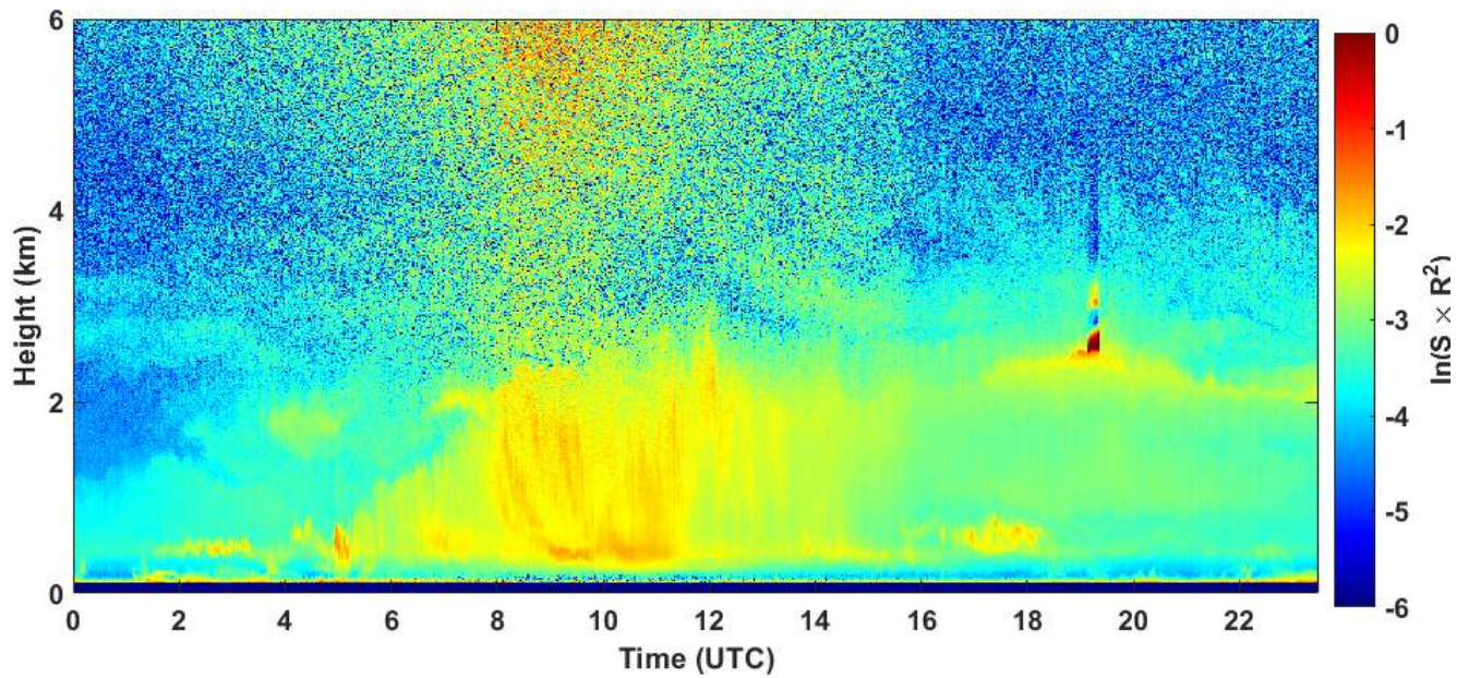
2020-07-24 RCS quick look CHM15k - ILVA LIDAR2 PARCHI
