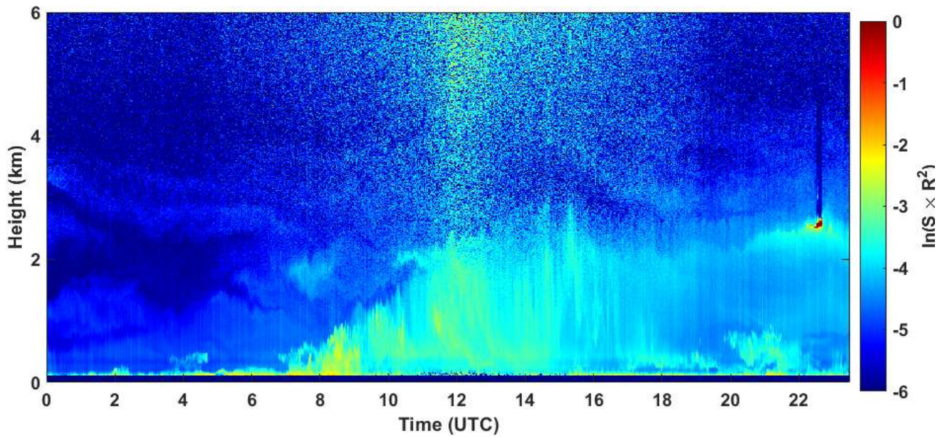
2020-07-24 RCS quick look CHM15k - ILVA LIDAR3 AGGLOMERATO
