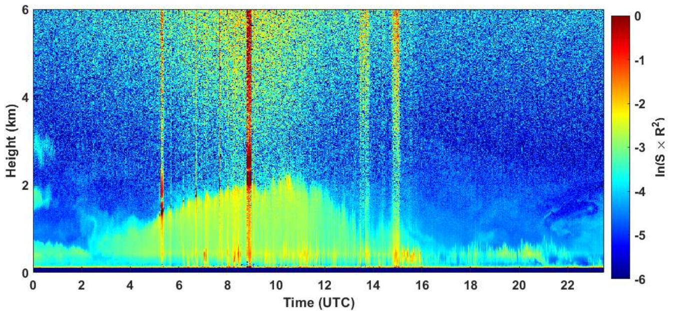
2020-07-26 RCS quick look CHM15k - ILVA LIDAR2 PARCHI
