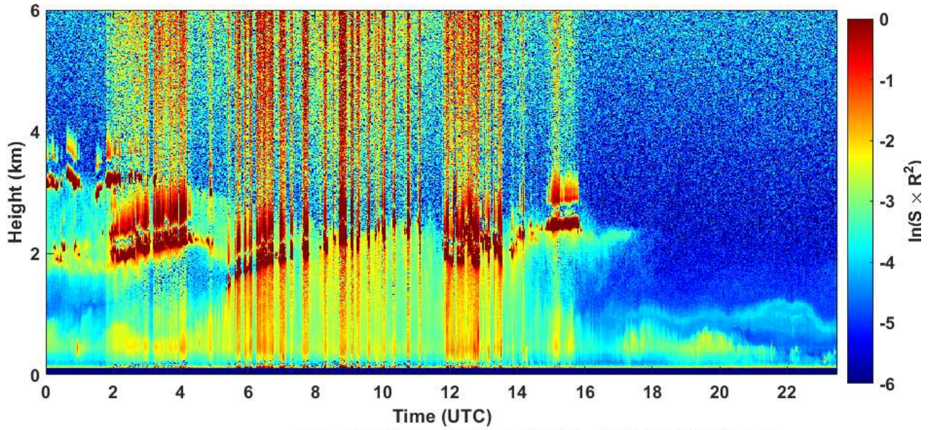
2020-07-20 RCS quick look CHM15k - ILVA LIDAR2 PARCHI
