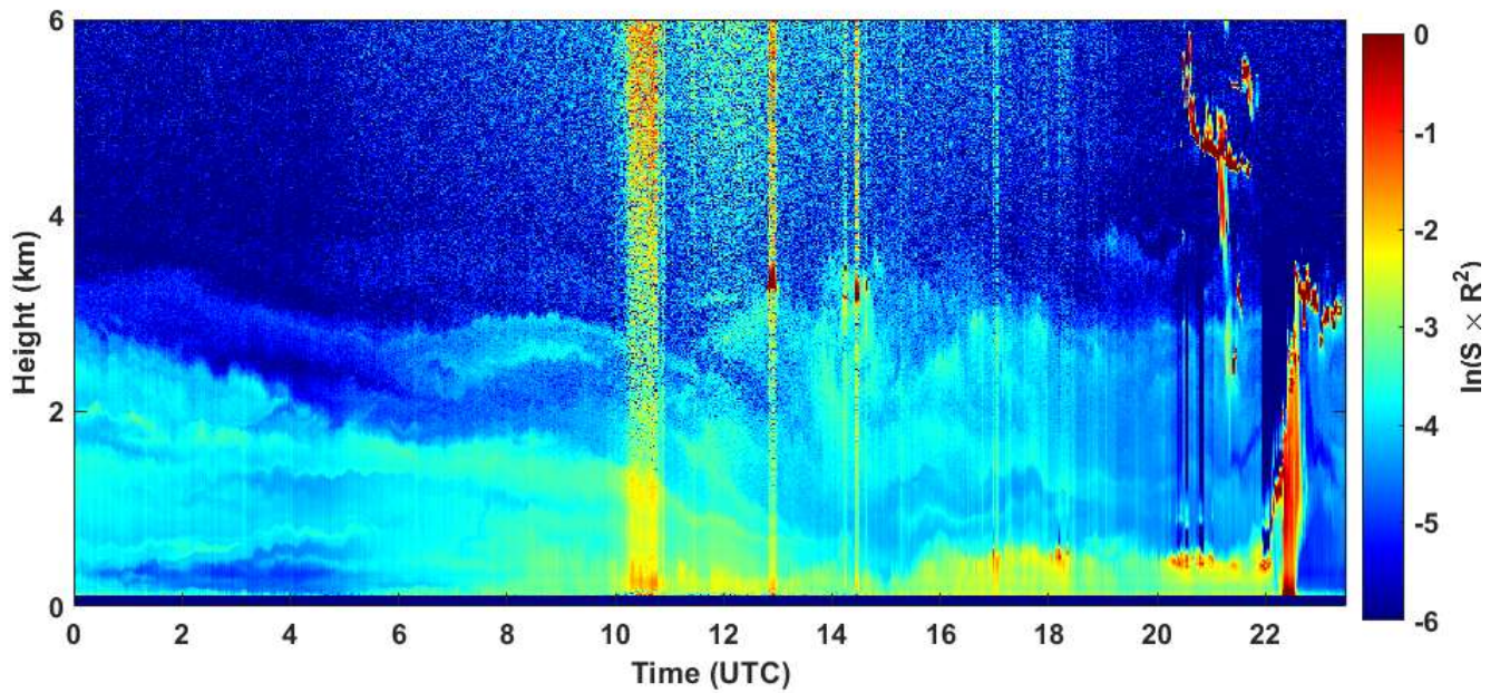
2020-07-16 RCS quick look CHM15k - ILVA LIDAR3 AGGLOMERATO
