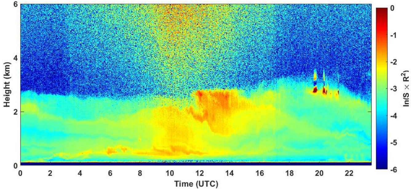
2020-07-02 RCS quick look CHM15k - ILVA LIDAR2 PARCHI
