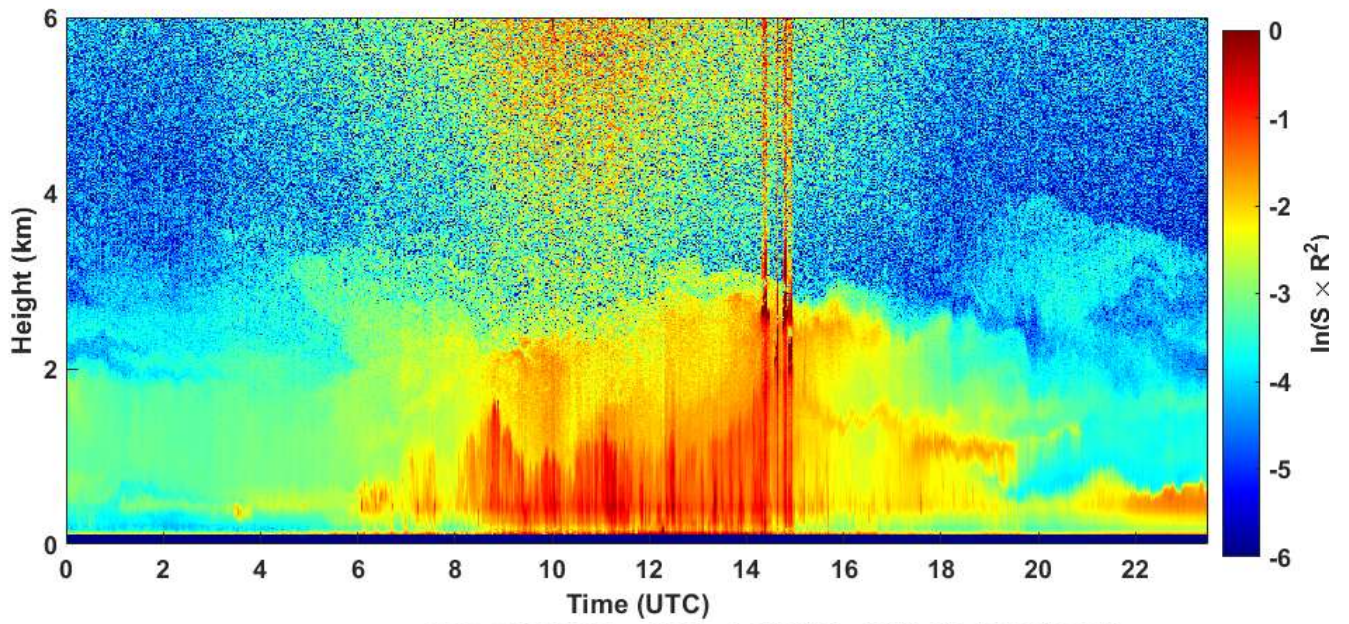
2020-07-08 RCS quick look CHM15k - ILVA LIDAR2 PARCHI
