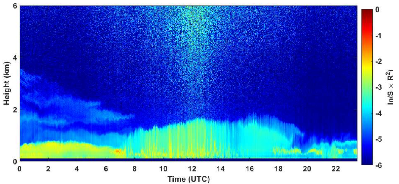
2020-07-08 RCS quick look CHM15k - ILVA LIDAR3 AGGLOMERATO
