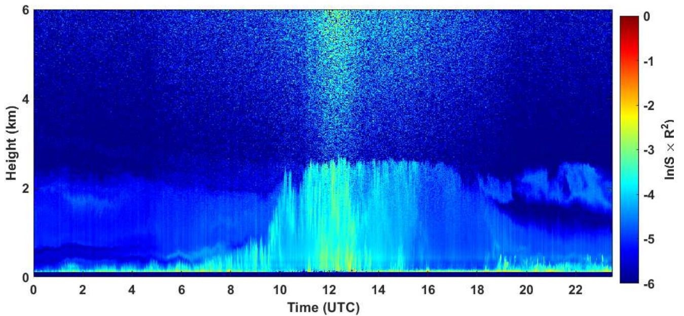
2020-07-28 RCS quick look CHM15k - ILVA LIDAR3 AGGLOMERATO
