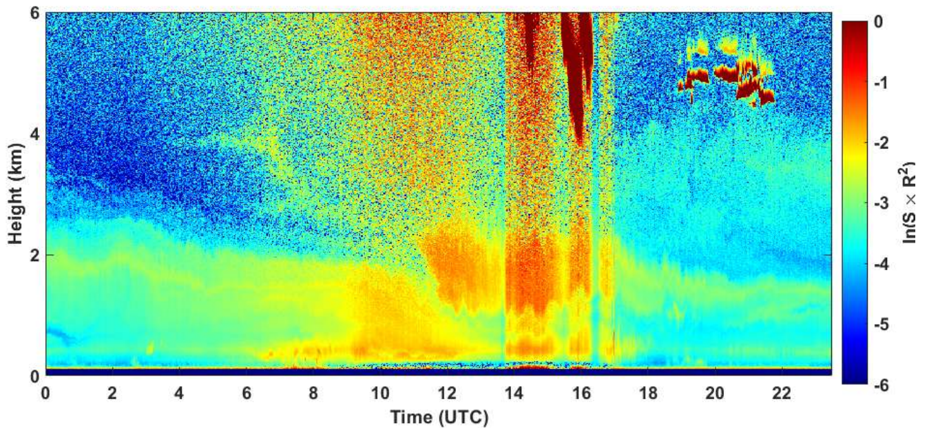
2020-07-02 RCS quick look CHM15k - ILVA LIDAR2 PARCHI
