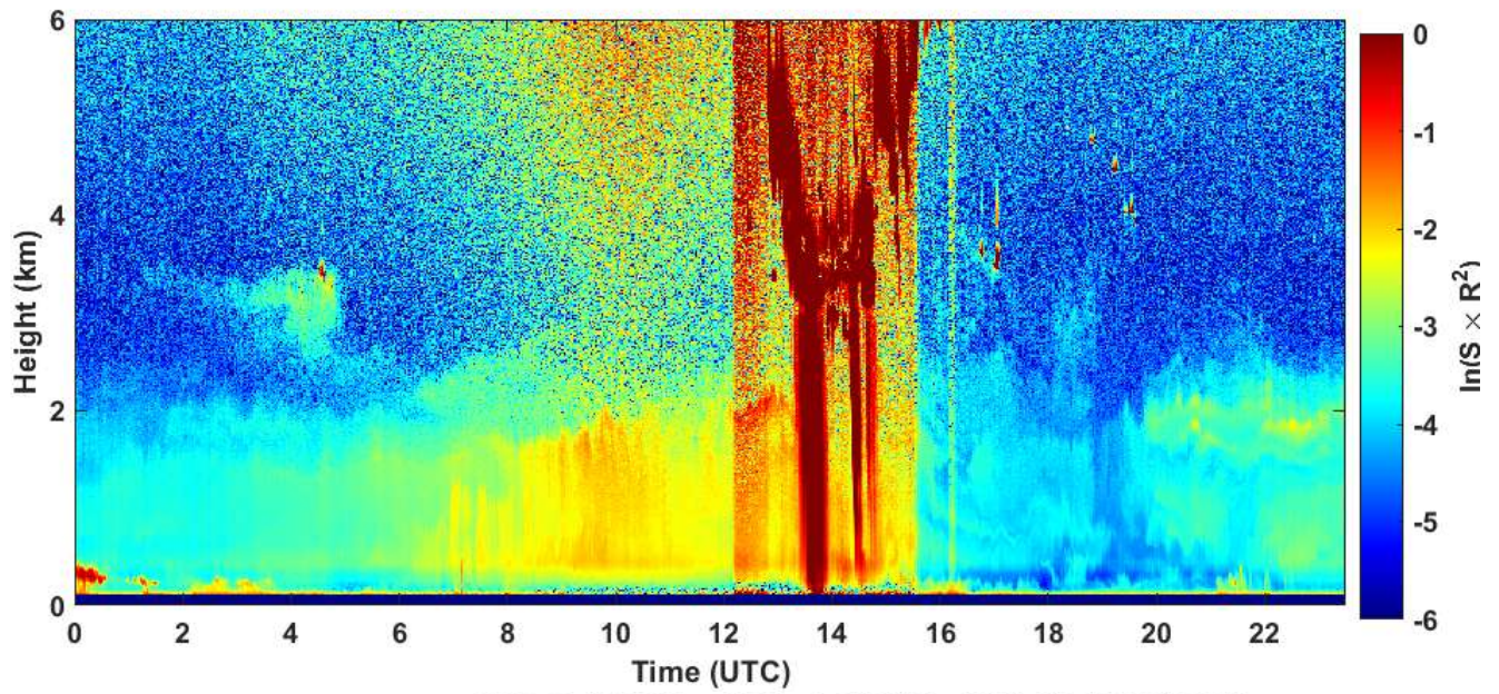
2020-06-10 RCS quick look CHM15k - ILVA LIDAR2 PARCHI
