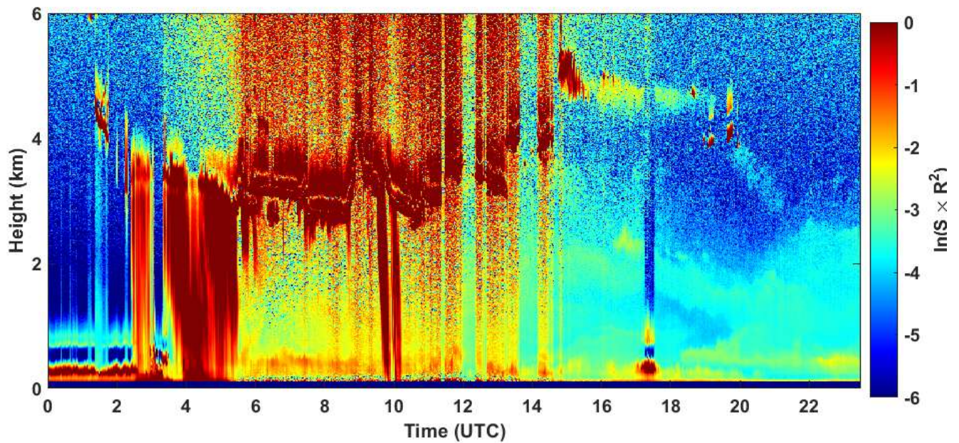
2020-06-08 RCS quick look CHM15k - ILVA LIDAR2 PARCHI
