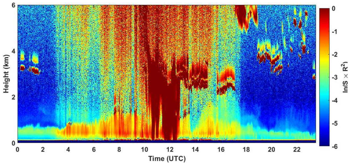
2020-06-22 RCS quick look CHM15k - ILVA LIDAR2 PARCHI
