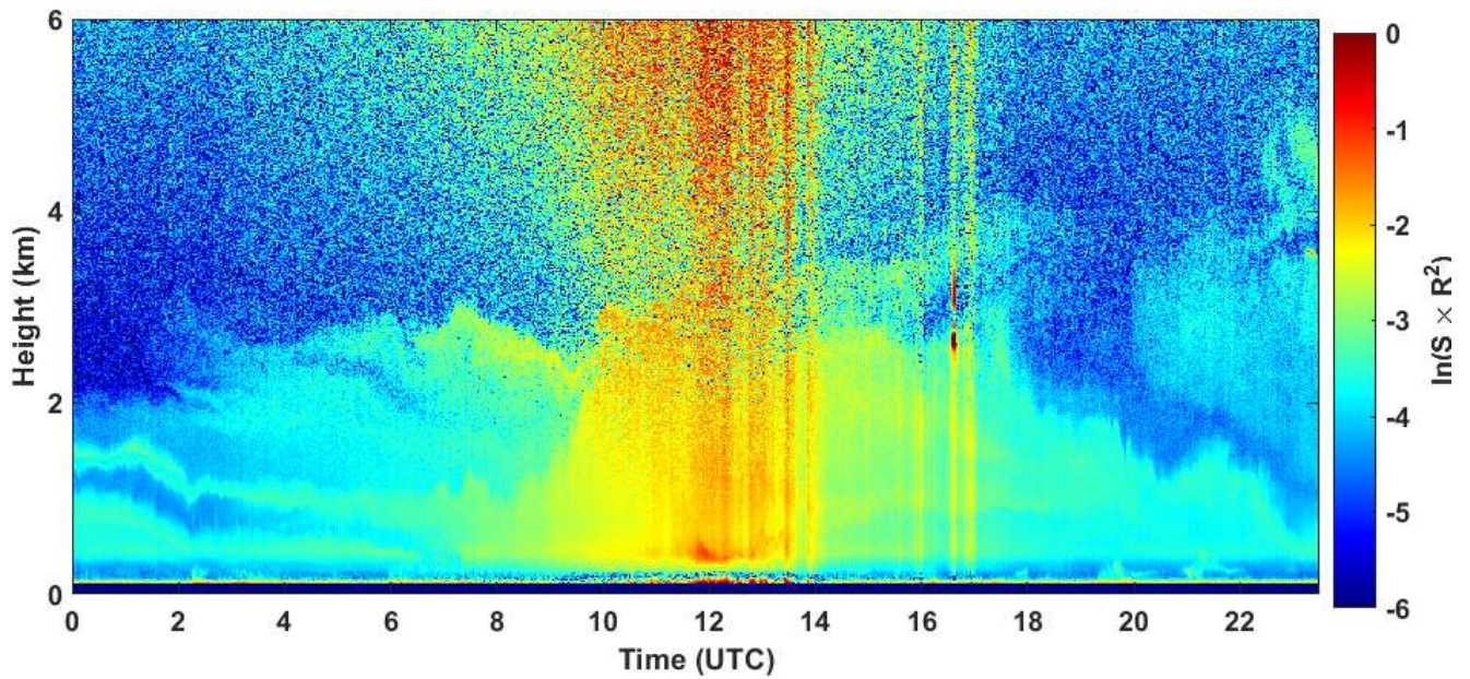
2020-06-14 RCS quick look CHM15k - ILVA LIDAR2 PARCHI
