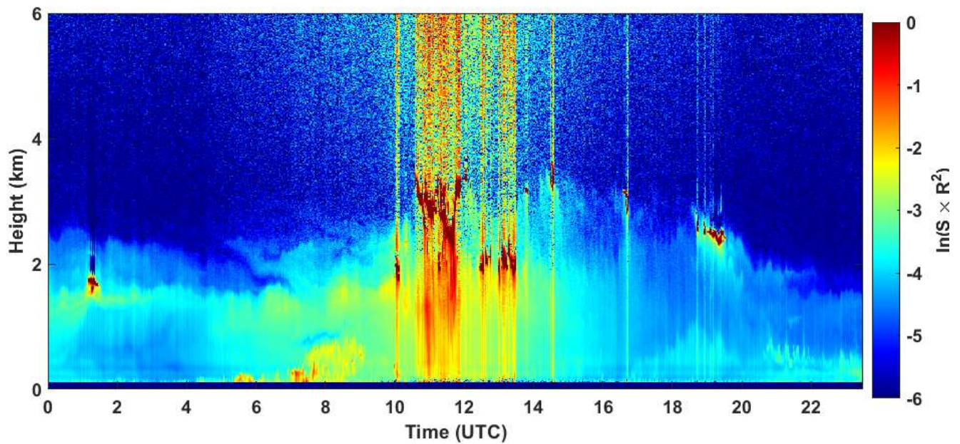
2020-06-18 RCS quick look CHM15k - ILVA LIDAR3 AGGLOMERATO
