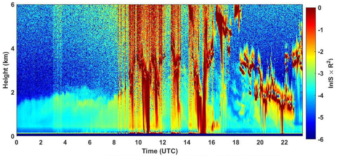
2020-06-16 RCS quick look CHM15k - ILVA LIDAR2 PARCHI
