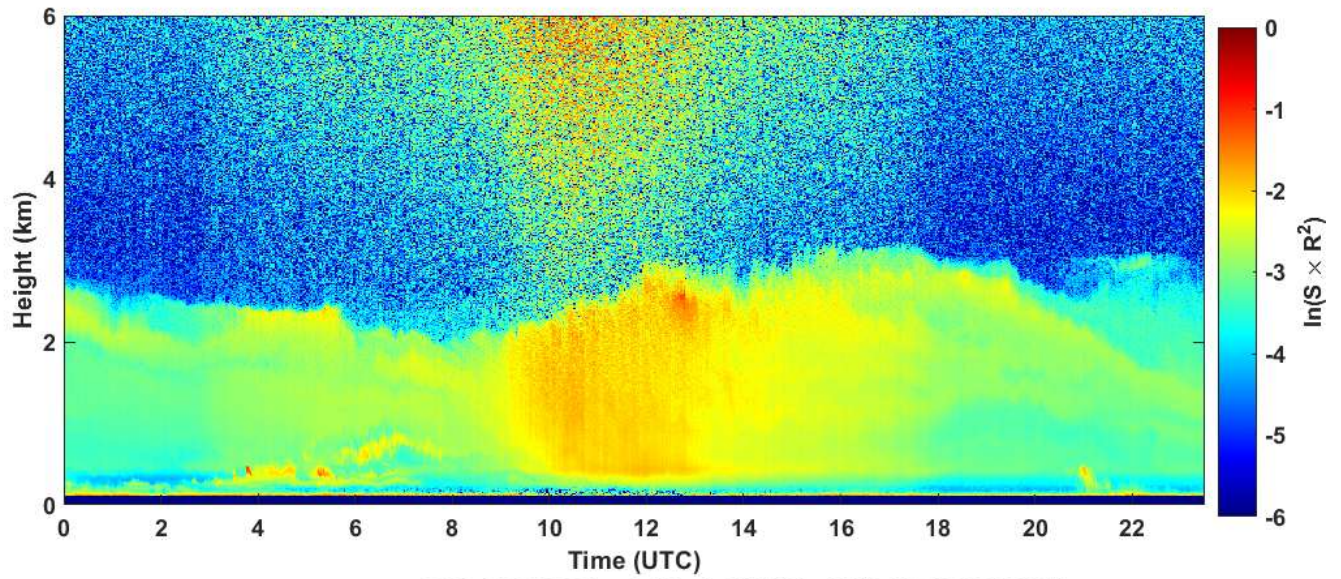
2020-06-30 RCS quick look CHM15k - ILVA LIDAR2 PARCHI
