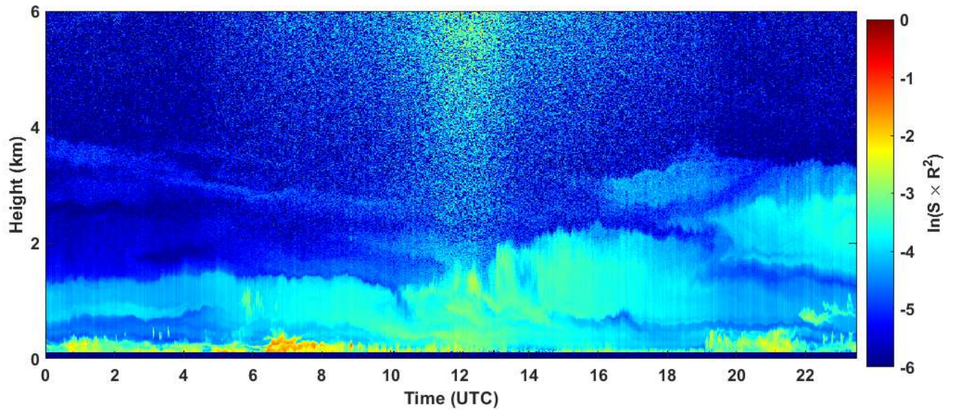
2020-06-28 RCS quick look CHM15k - ILVA LIDAR3 AGGLOMERATO
