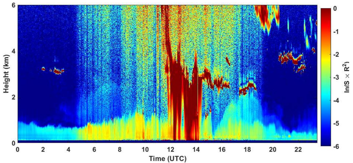
2020-06-22 RCS quick look CHM15k - ILVA LIDAR3 AGGLOMERATO
