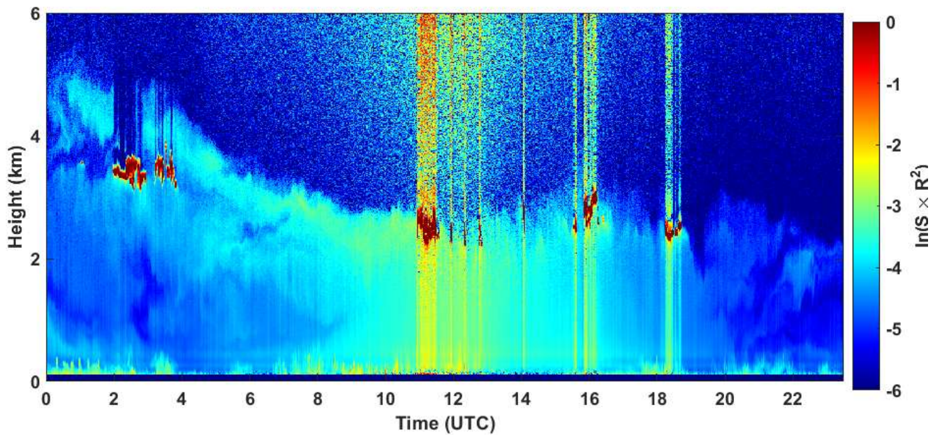
2020-06-14 RCS quick look CHM15k - ILVA LIDAR3 AGGLOMERATO
