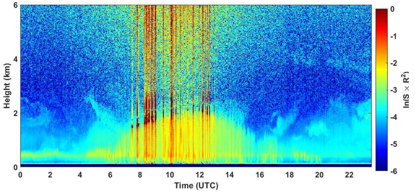
2020-06-02 RCS quick look CHM15k - ILVA LIDAR2 PARCHI
