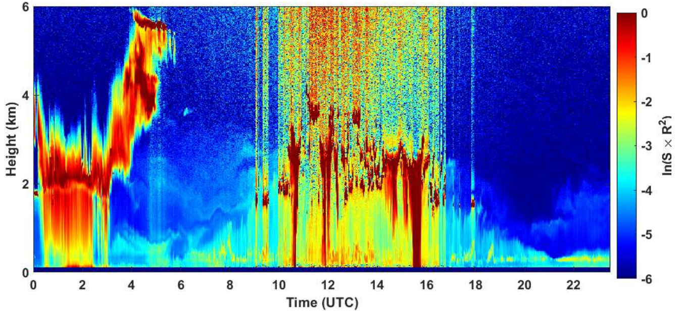
2020-06-02 RCS quick look CHM15k - ILVA LIDAR3 AGGLOMERATO
