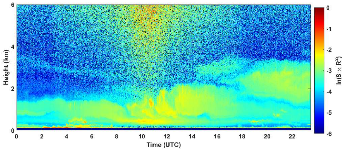
2020-06-28 RCS quick look CHM15k - ILVA LIDAR2 PARCHI
