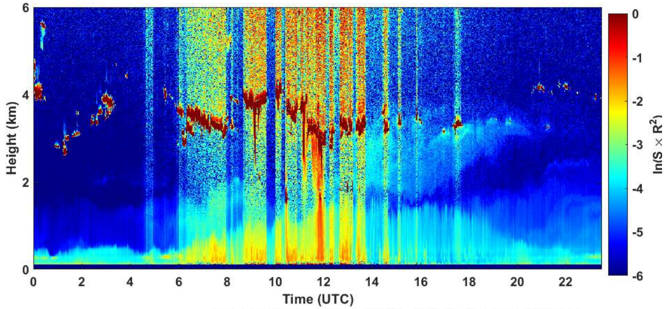
2020-06-24 RCS quick look CHM15k - ILVA LIDAR3 AGGLOMERATO
