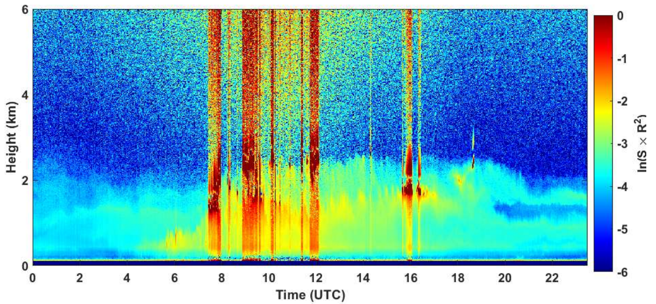
2020-06-12 RCS quick look CHM15k - ILVA LIDAR2 PARCHI
