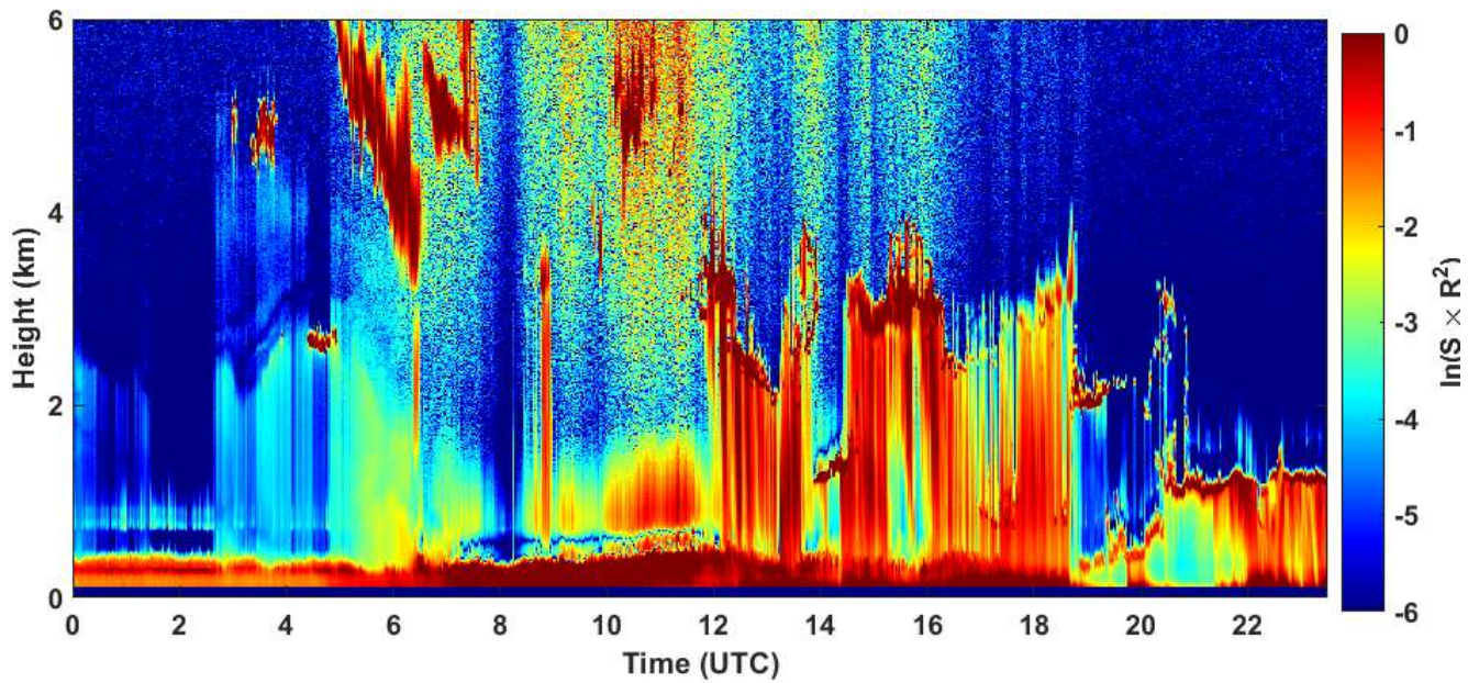
2020-06-06 RCS quick look CHM15k - ILVA LIDAR3 AGGLOMERATO
