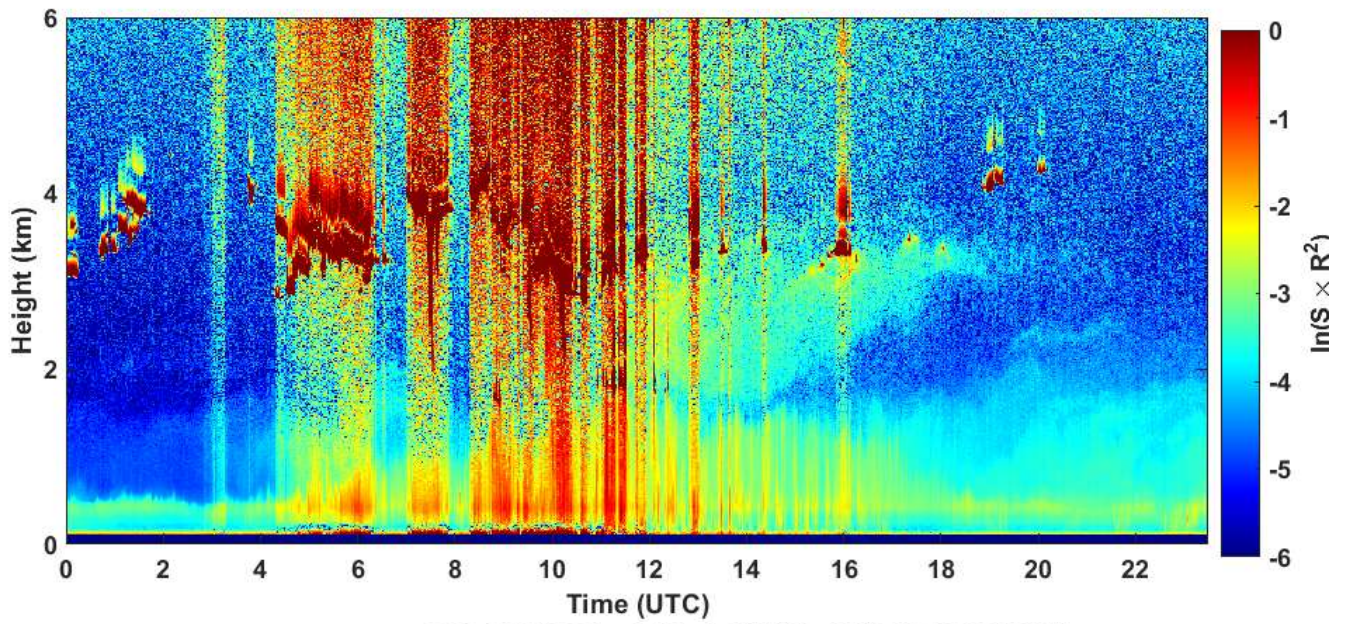
2020-06-24 RCS quick look CHM15k - ILVA LIDAR2 PARCHI
