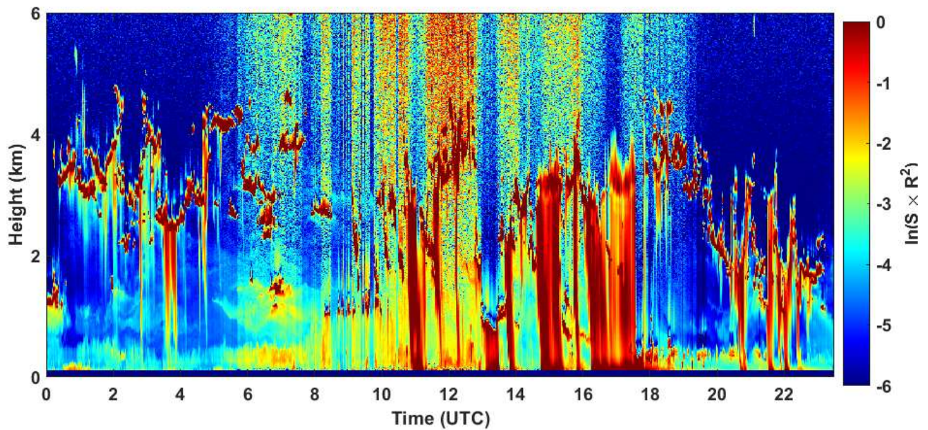
2020-06-16 RCS quick look CHM15k - ILVA LIDAR3 AGGLOMERATO
