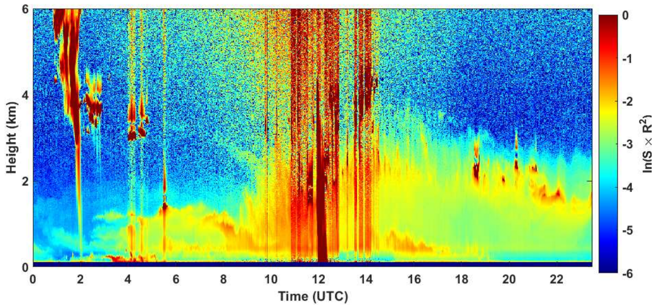
2020-06-18 RCS quick look CHM15k - ILVA LIDAR2 PARCHI
