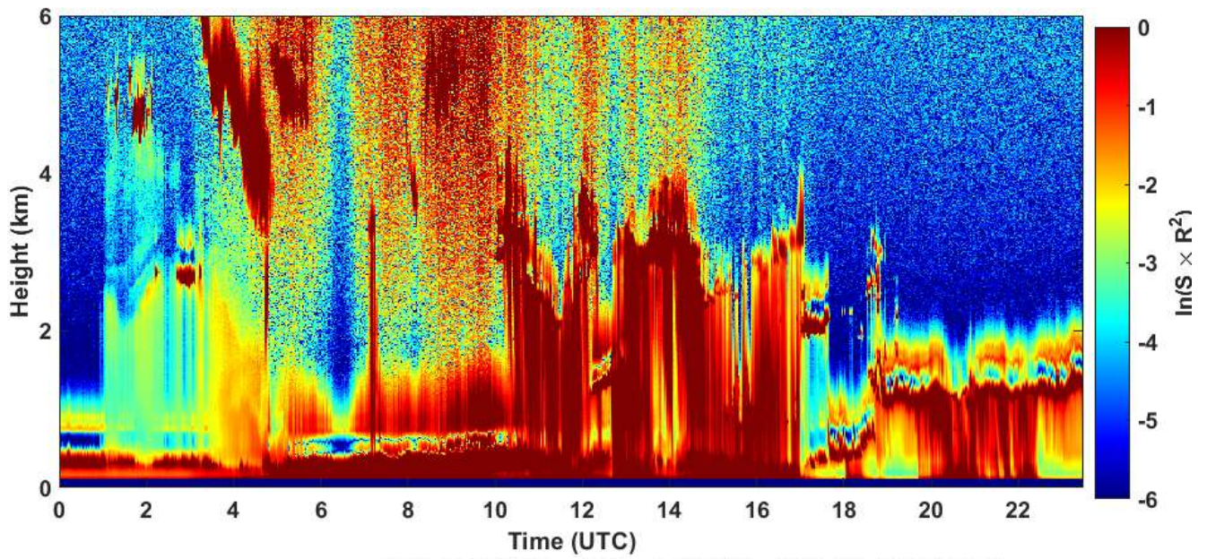
2020-06-06 RCS quick look CHM15k - ILVA LIDAR2 PARCHI
