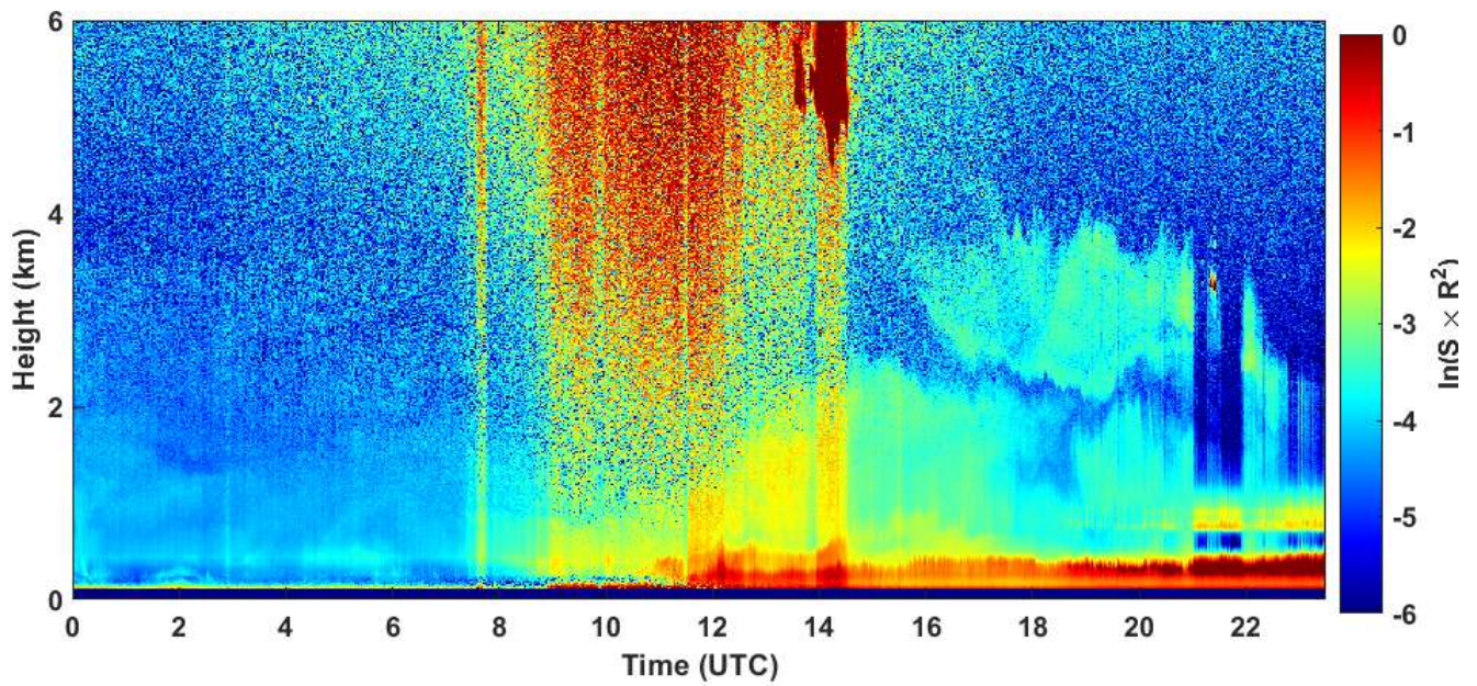
2020-06-04 RCS quick look CHM15k - ILVA LIDAR2 PARCHI
