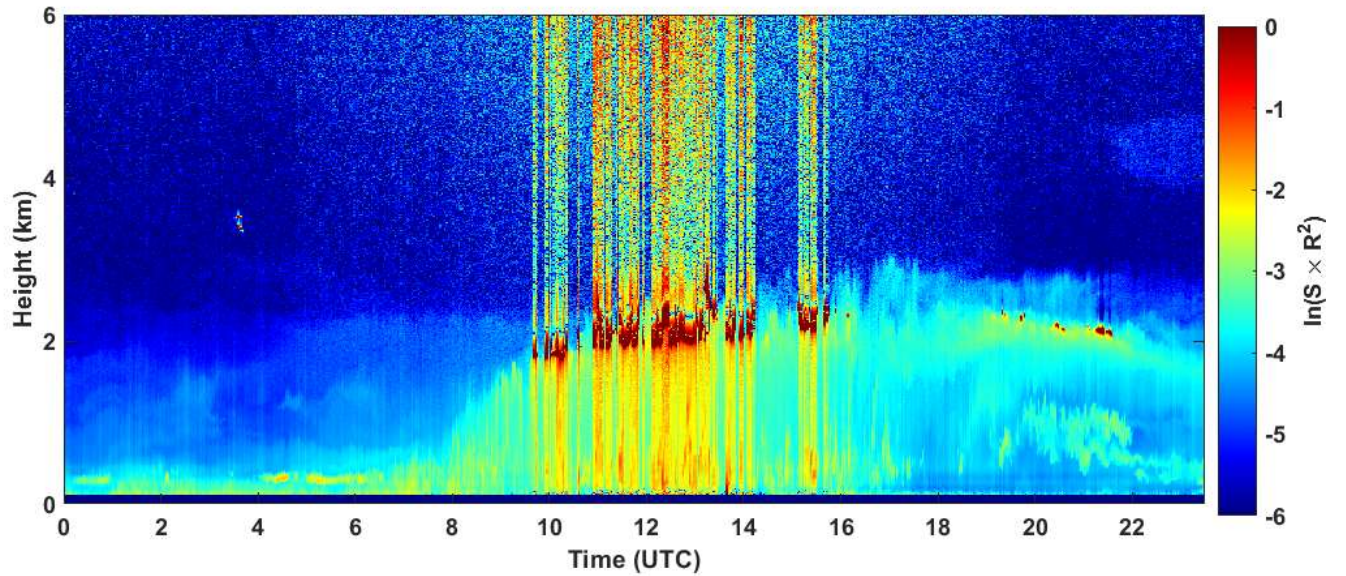
2020-06-24 RCS quick look CHM15k - ILVA LIDAR3 AGGLOMERATO
