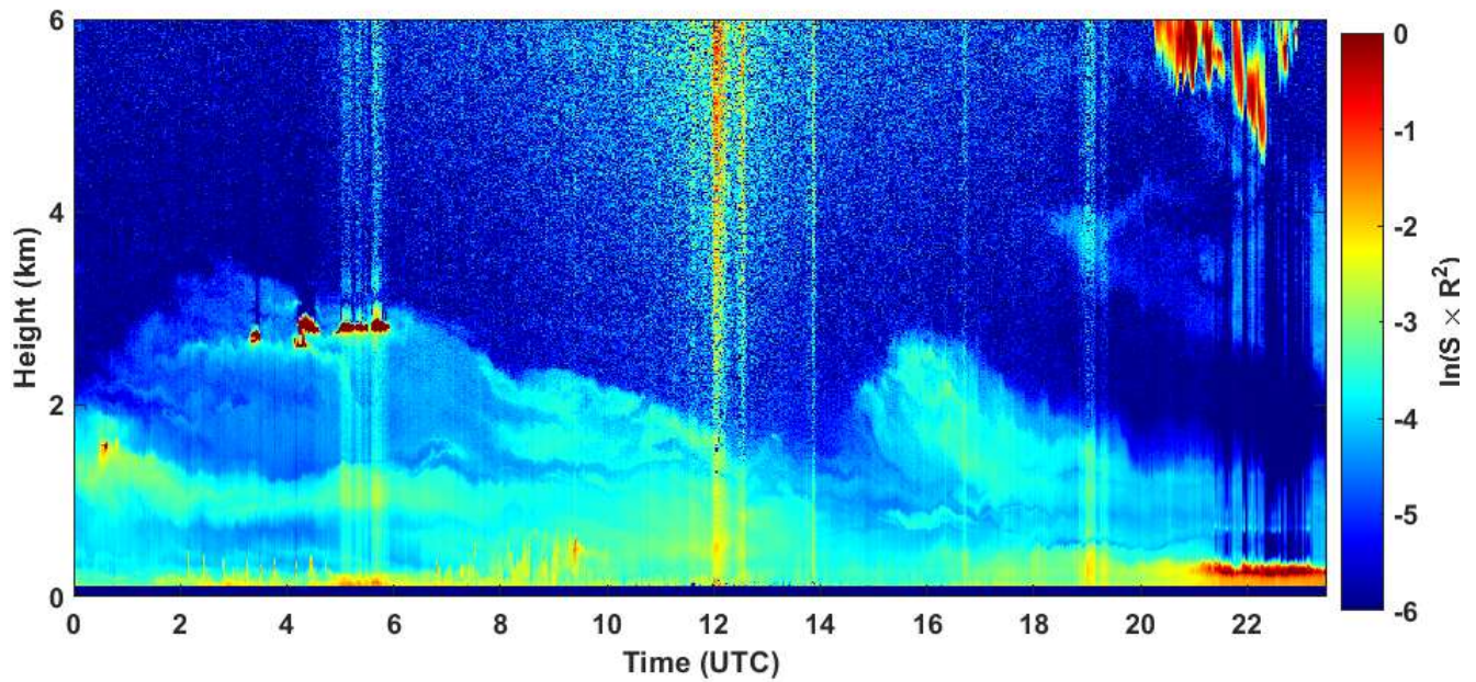
2020-06-08 RCS quick look CHM15k - ILVA LIDAR3 AGGLOMERATO
