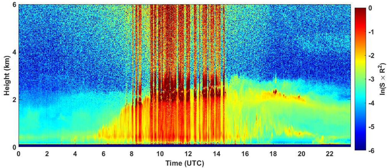
2020-06-24 RCS quick look CHM15k - ILVA LIDAR2 PARCHI
