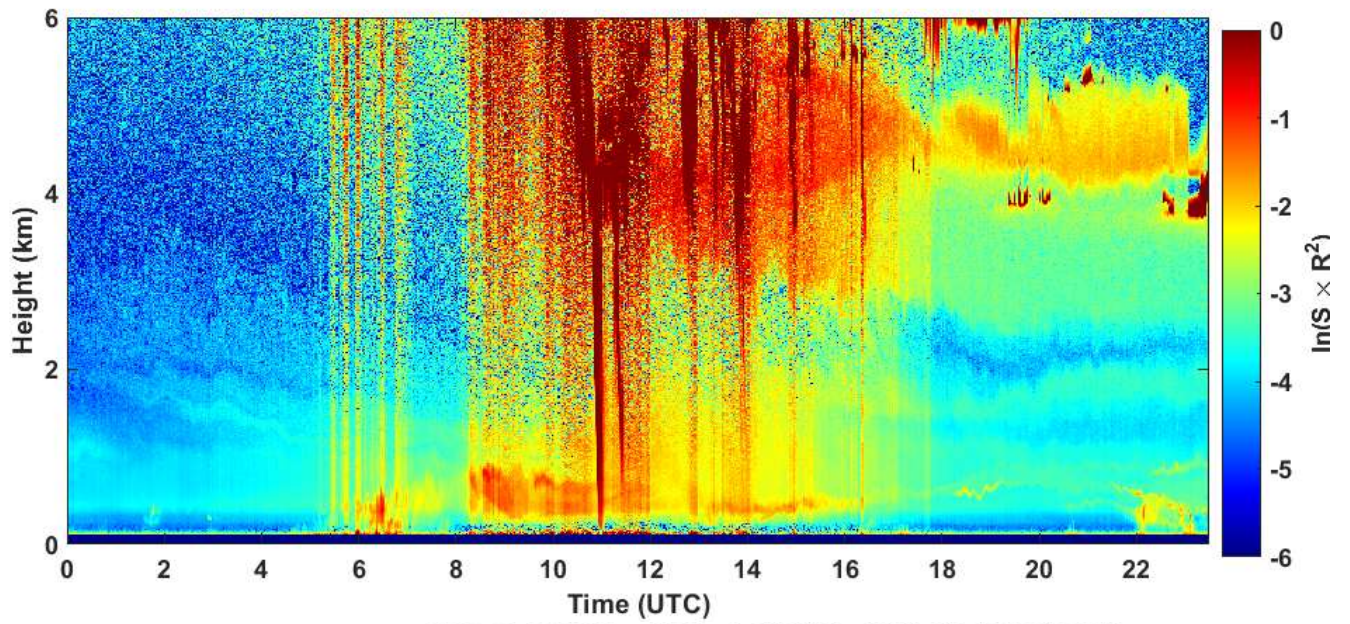
2020-06-20 RCS quick look CHM15k - ILVA LIDAR2 PARCHI
