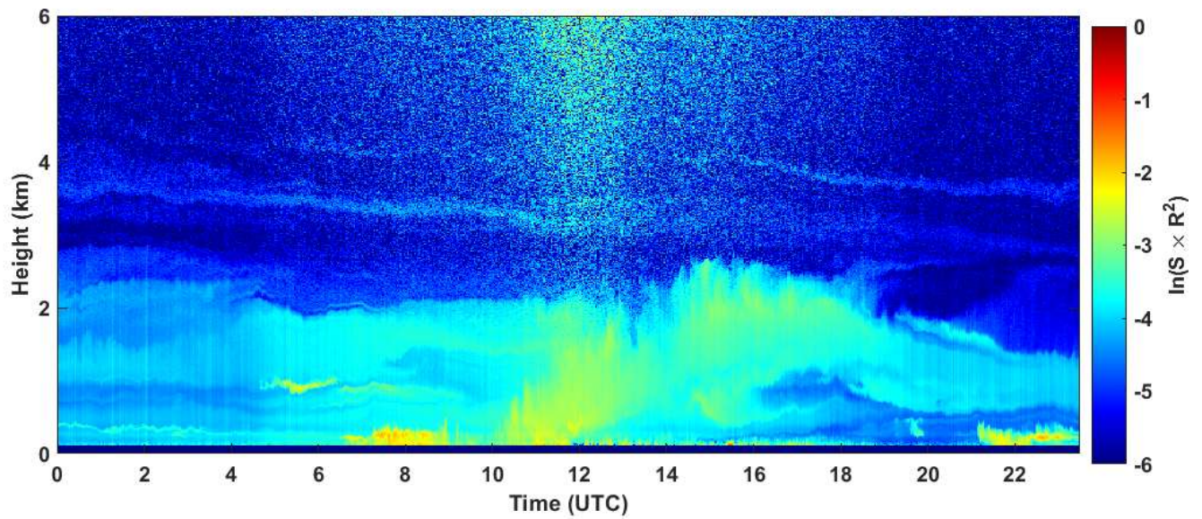
2020-06-26 RCS quick look CHM15k - ILVA LIDAR3 AGGLOMERATO
