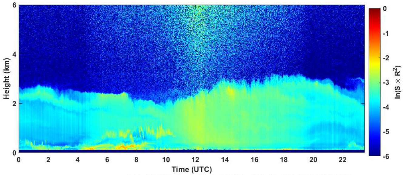
2020-06-30 RCS quick look CHM15k - ILVA LIDAR3 AGGLOMERATO
