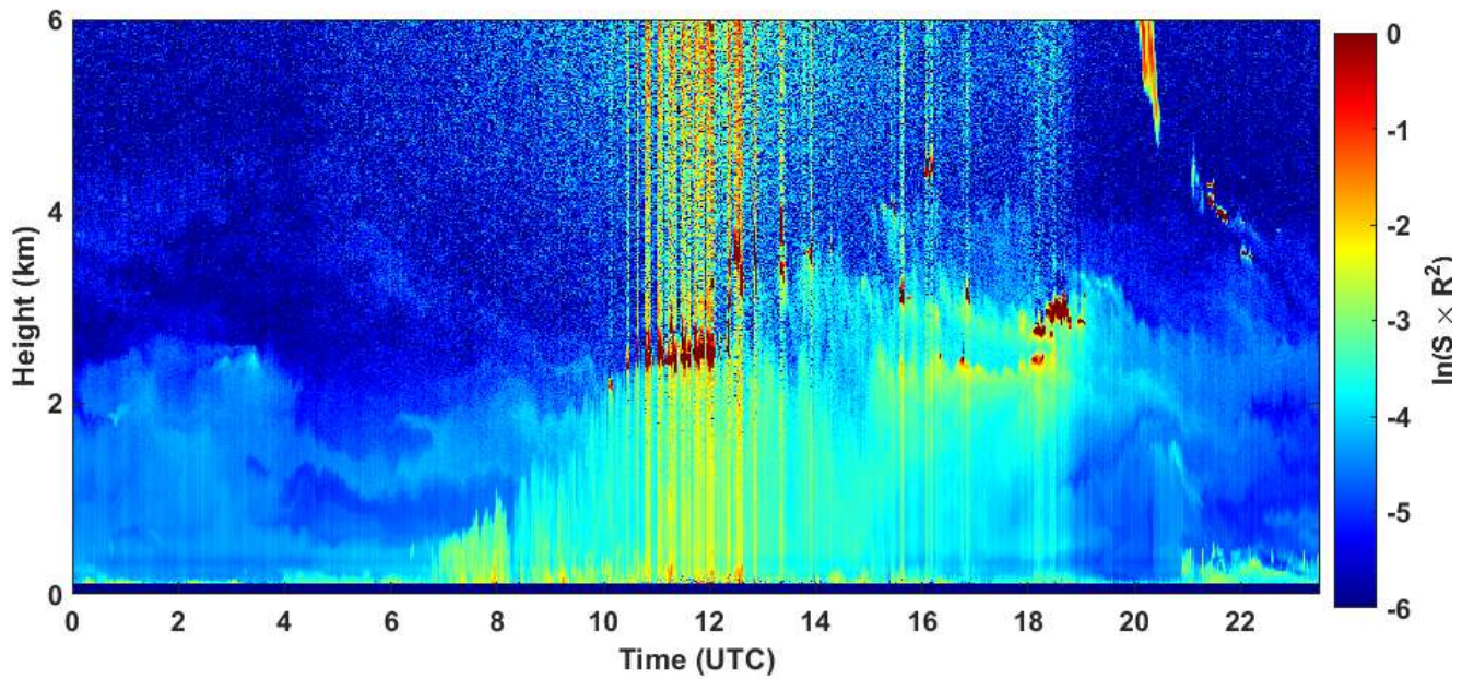
2020-06-04 RCS quick look CHM15k - ILVA LIDAR3 AGGLOMERATO
