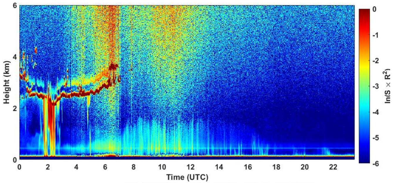
2020-05-26 RCS quick look CHM15k - ILVA LIDAR2 PARCHI
