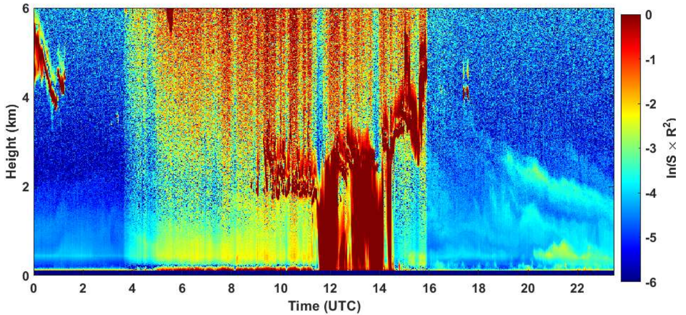
2020-05-02 RCS quick look CHM15k - ILVA LIDAR2 PARCHI
