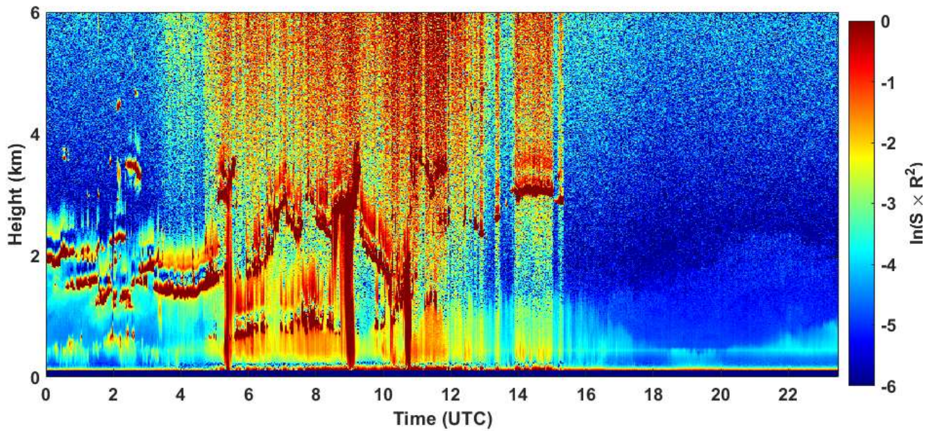
2020-05-22 RCS quick look CHM15k - ILVA LIDAR2 PARCHI
