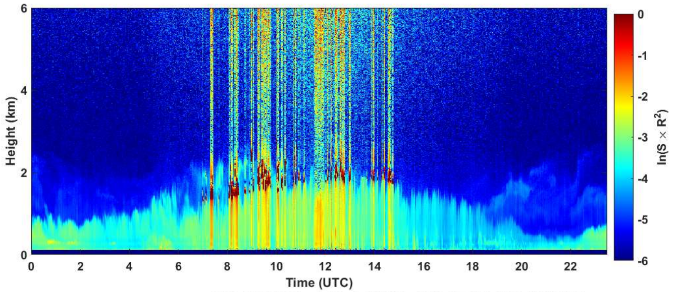
2020-05-28 RCS quick look CHM15k - ILVA LIDAR3 AGGLOMERATO
