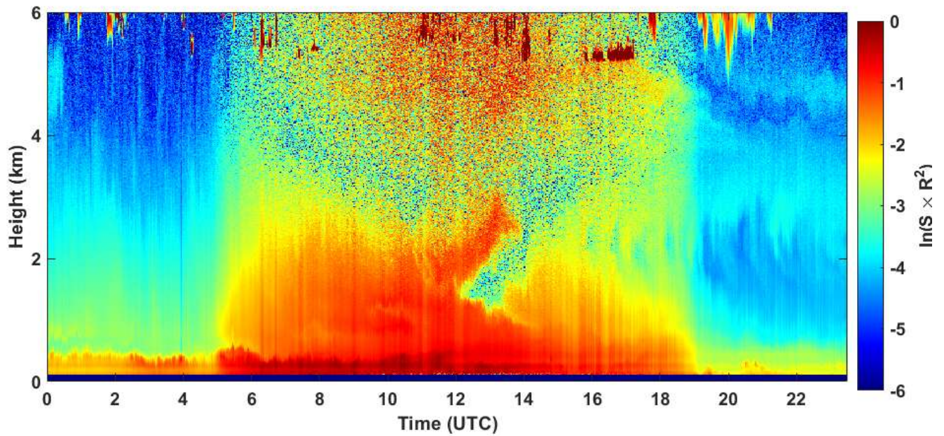
2020-05-16 RCS quick look CHM15k - ILVA LIDAR3 AGGLOMERATO
