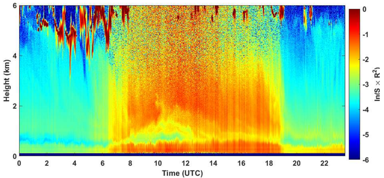
2020-05-14 RCS quick look CHM15k - ILVA LIDAR3 AGGLOMERATO
