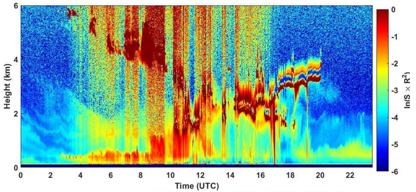
2020-05-04 RCS quick look CHM15k - ILVA LIDAR2 PARCHI
