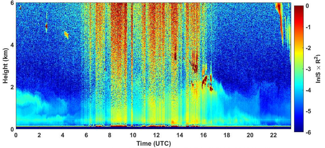
2020-05-02 RCS quick look CHM15k - ILVA LIDAR2 PARCHI
