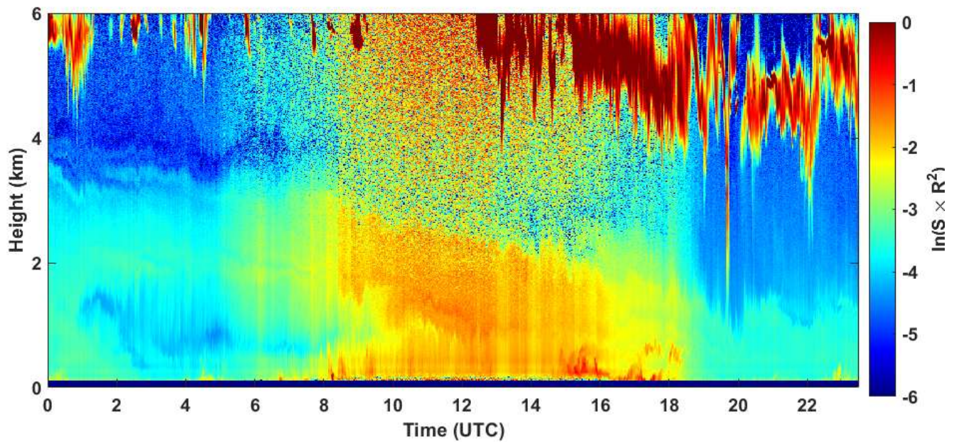
2020-05-18 RCS quick look CHM15k - ILVA LIDAR3 AGGLOMERATO
