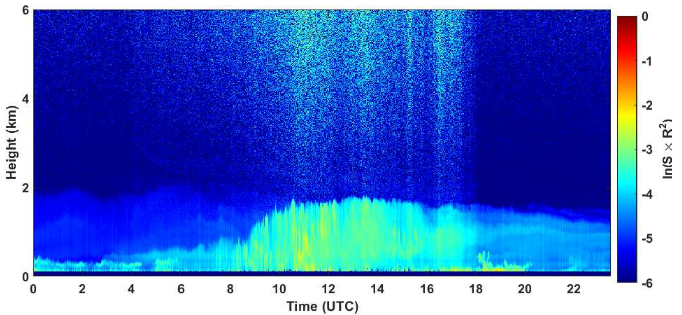
2020-05-08 RCS quick look CHM15k - ILVA LIDAR3 AGGLOMERATO
