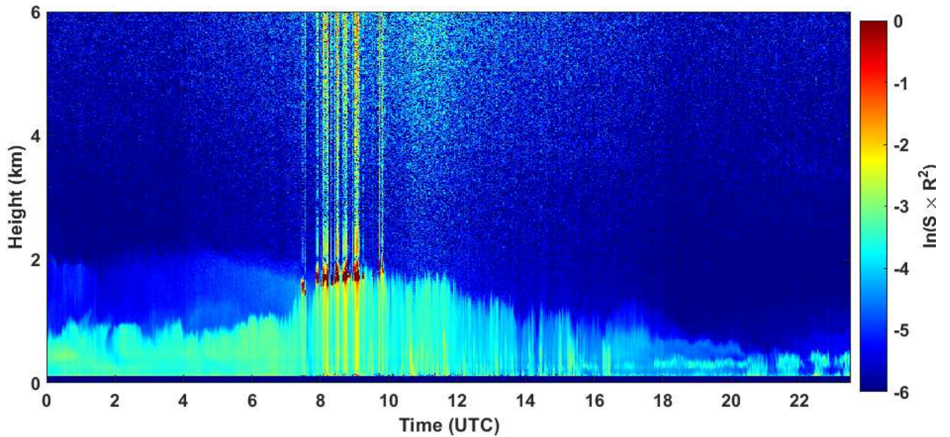
2020-05-04 RCS quick look CHM15k - ILVA LIDAR3 AGGLOMERATO
