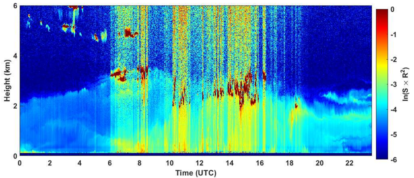
2020-05-30 RCS quick look CHM15k - ILVA LIDAR3 AGGLOMERATO
