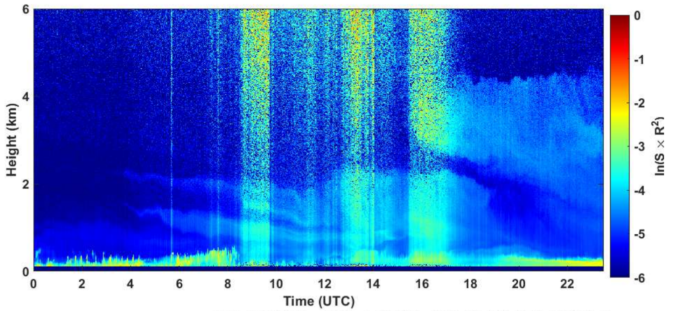
2020-05-06 RCS quick look CHM15k - ILVA LIDAR3 AGGLOMERATO
