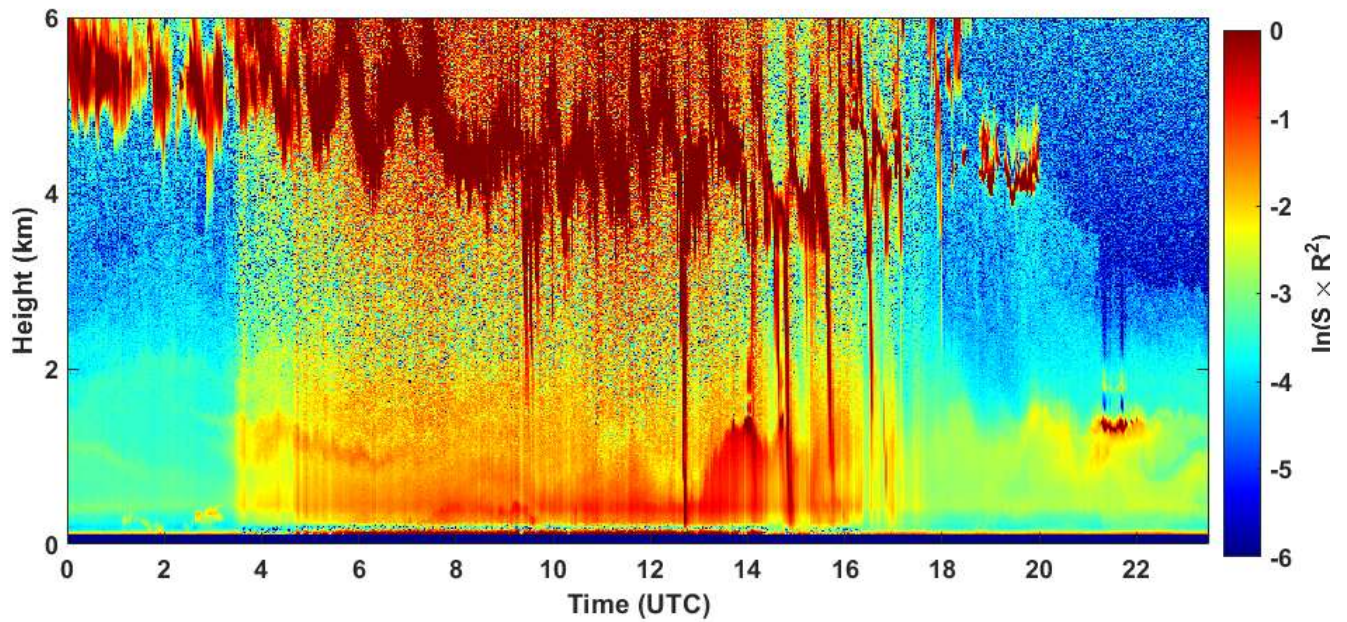
2020-05-20 RCS quick look CHM15k - ILVA LIDAR2 PARCHI
