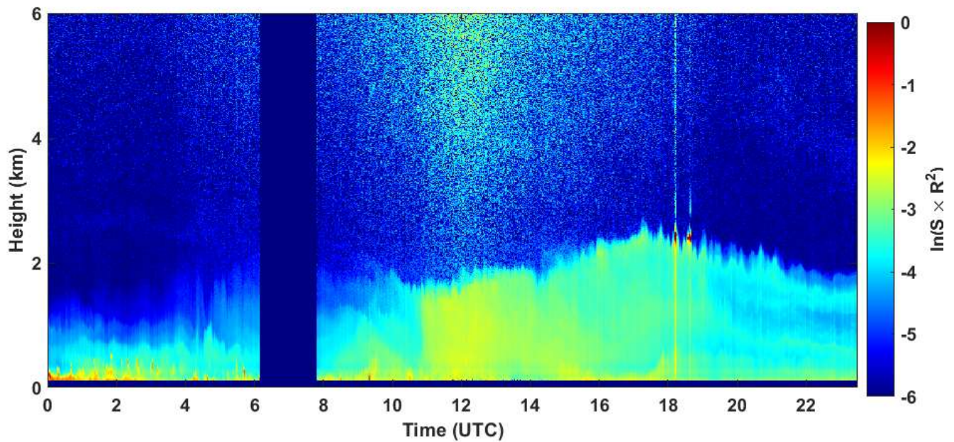
2020-05-12 RCS quick look CHM15k - ILVA LIDAR3 AGGLOMERATO
