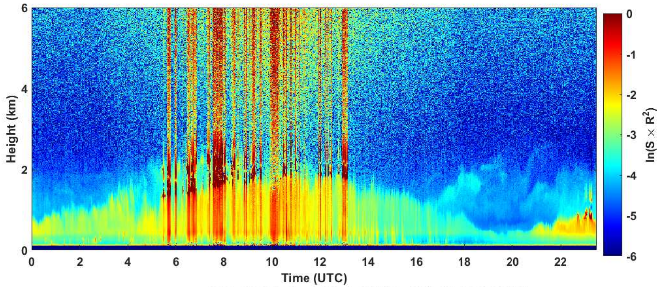
2020-05-28 RCS quick look CHM15k - ILVA LIDAR2 PARCHI
