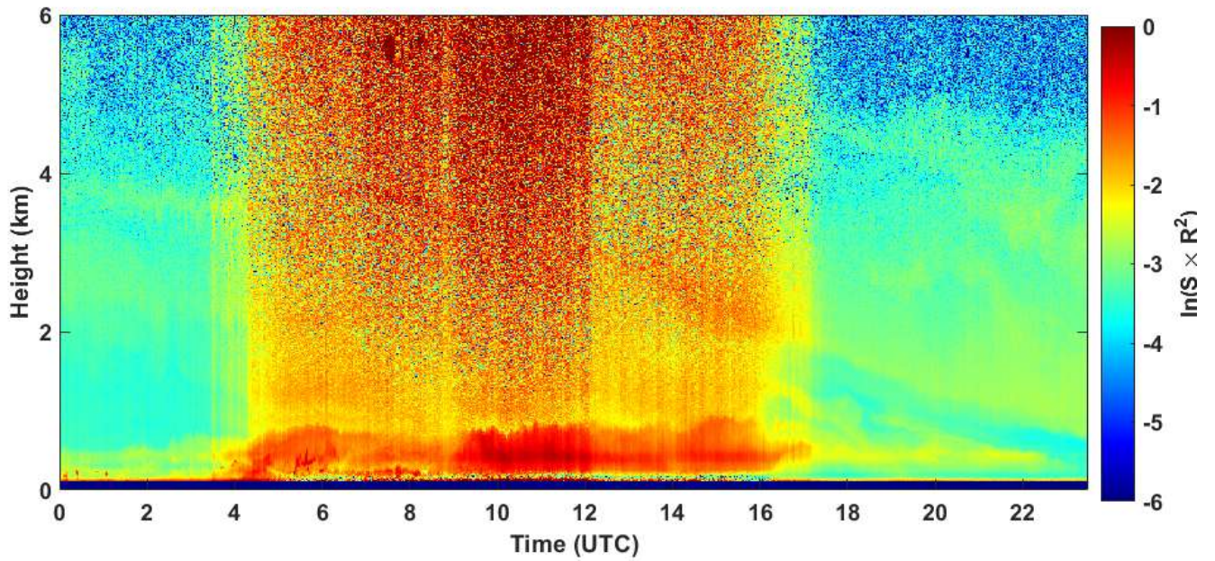
2020-05-16 RCS quick look CHM15k - ILVA LIDAR2 PARCHI
