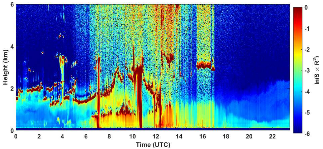
2020-05-22 RCS quick look CHM15k - ILVA LIDAR3 AGGLOMERATO
