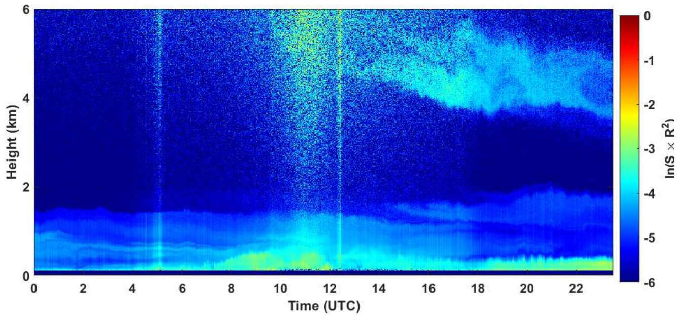
2020-05-10 RCS quick look CHM15k - ILVA LIDAR3 AGGLOMERATO
