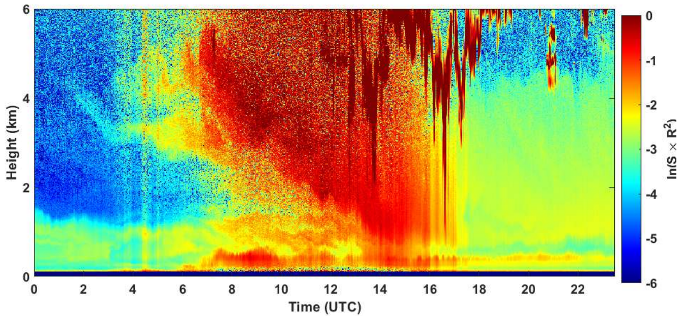
2020-05-14 RCS quick look CHM15k - ILVA LIDAR2 PARCHI
