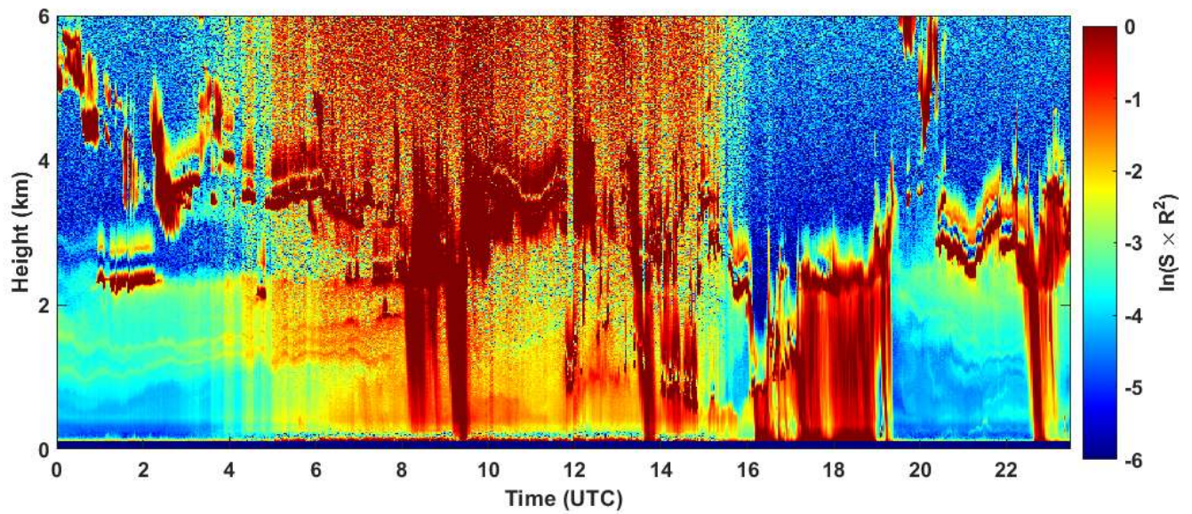
2020-05-30 RCS quick look CHM15k - ILVA LIDAR2 PARCHI
