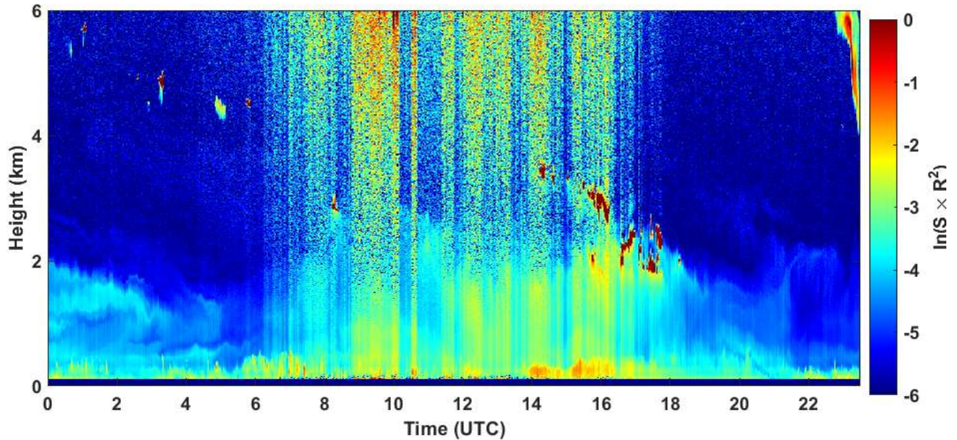
2020-05-02 RCS quick look CHM15k - ILVA LIDAR3 AGGLOMERATO
