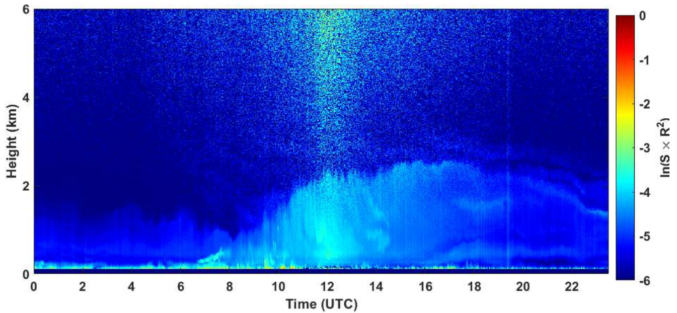
2020-05-24 RCS quick look CHM15k - ILVA LIDAR3 AGGLOMERATO
