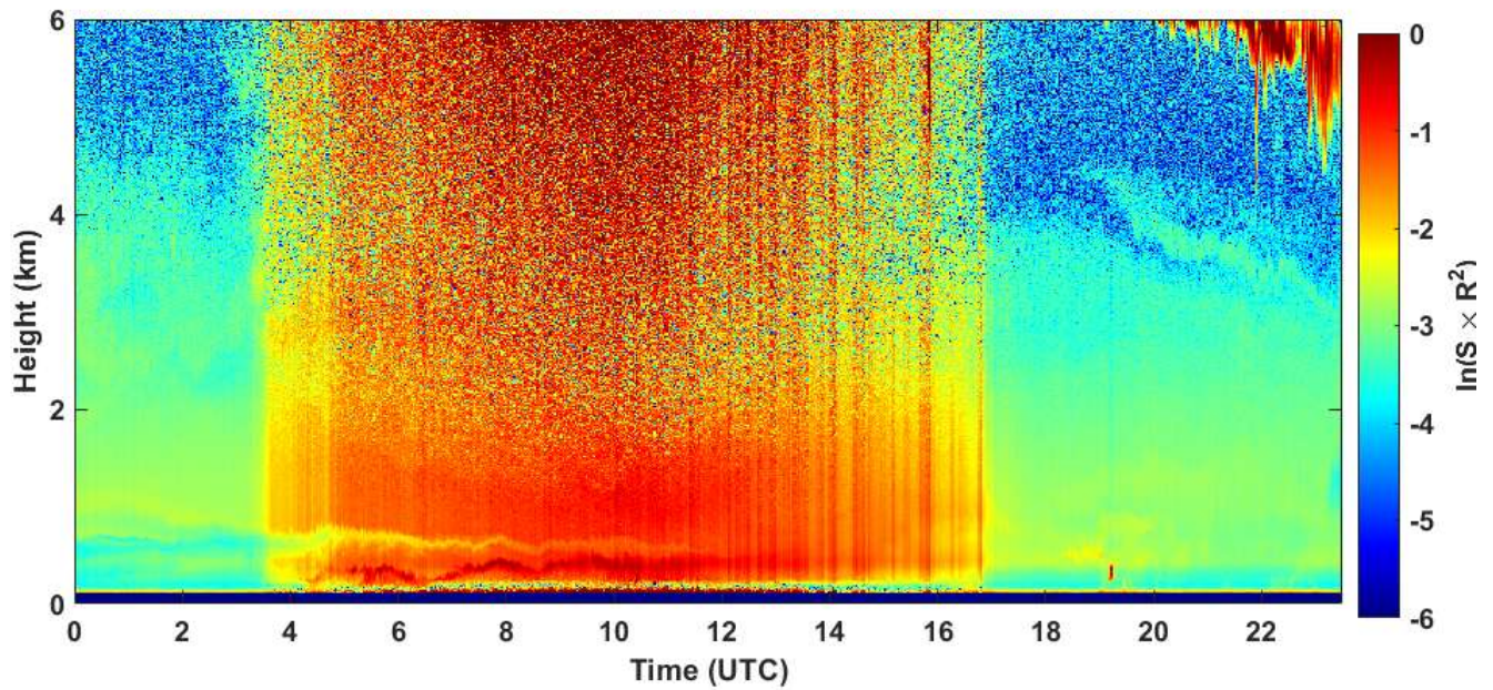
2020-05-18 RCS quick look CHM15k - ILVA LIDAR2 PARCHI
