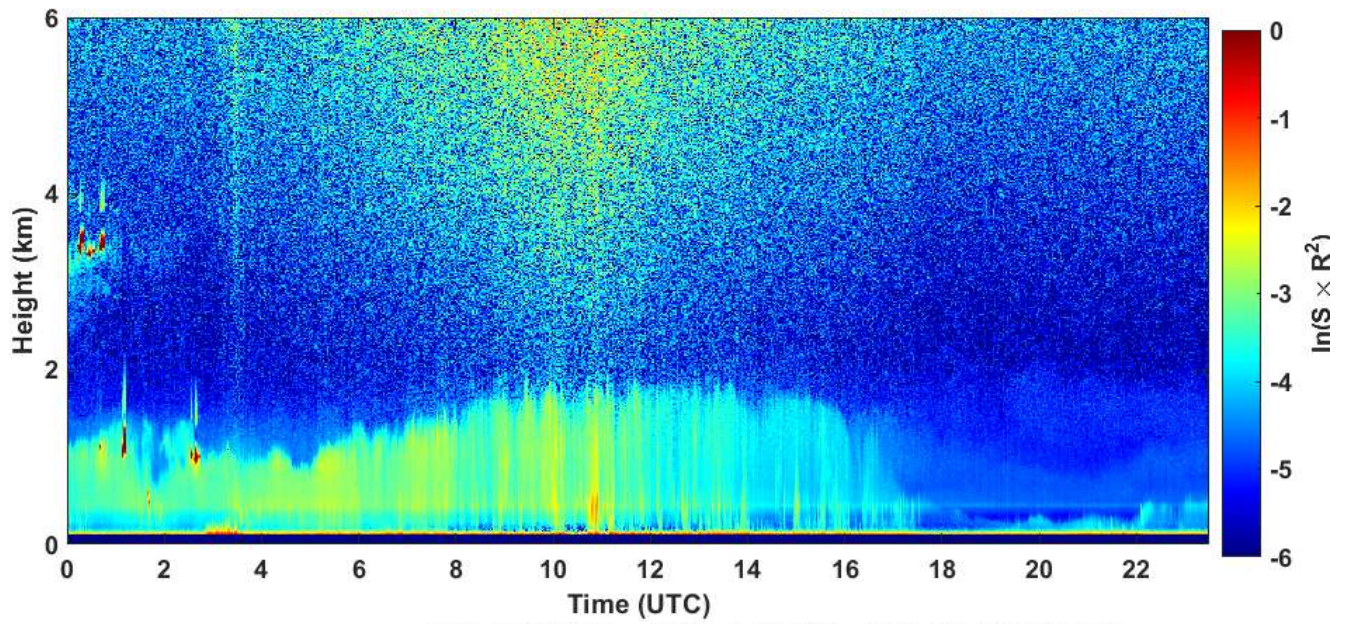
2020-05-08 RCS quick look CHM15k - ILVA LIDAR2 PARCHI
