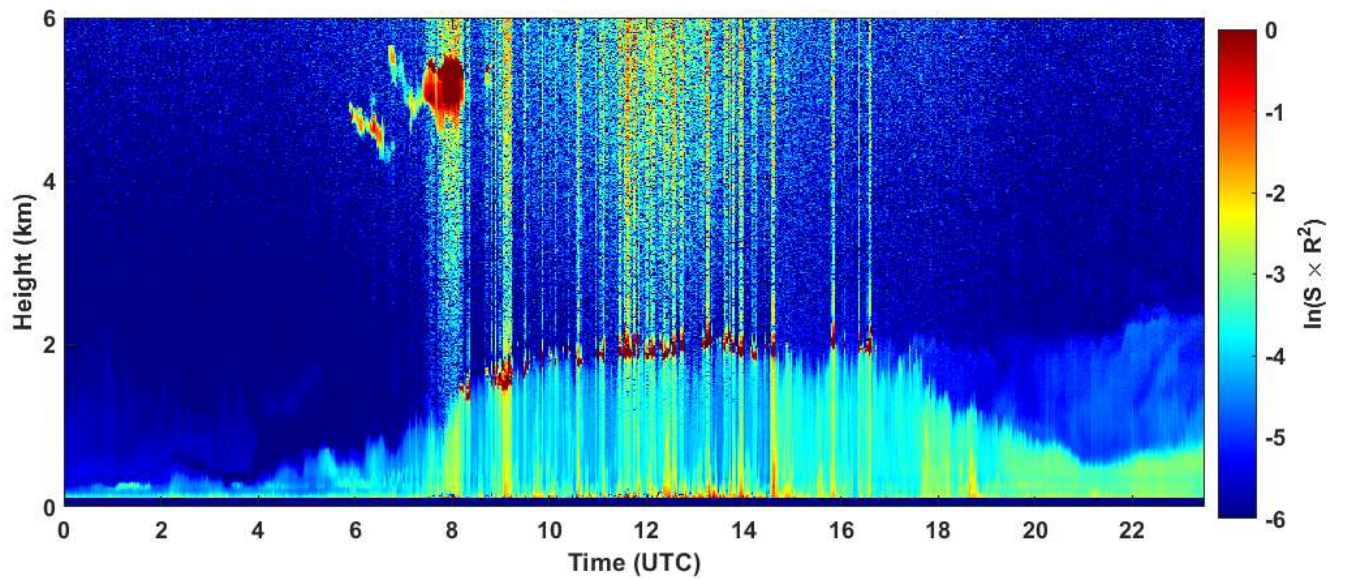
2020-05-26 RCS quick look CHM15k - ILVA LIDAR3 AGGLOMERATO
