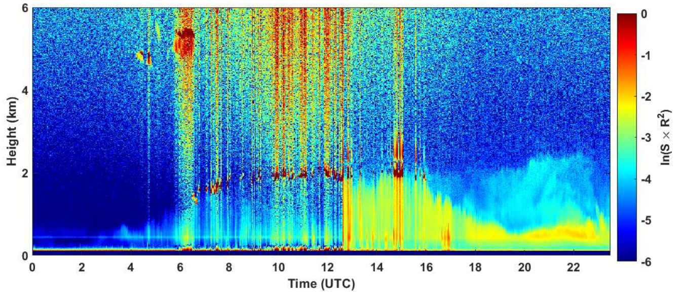
2020-05-26 RCS quick look CHM15k - ILVA LIDAR2 PARCHI
