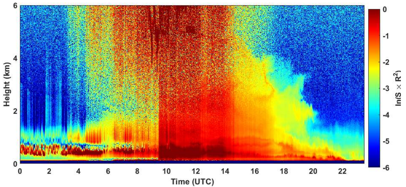
2020-05-12 RCS quick look CHM15k - ILVA LIDAR2 PARCHI
