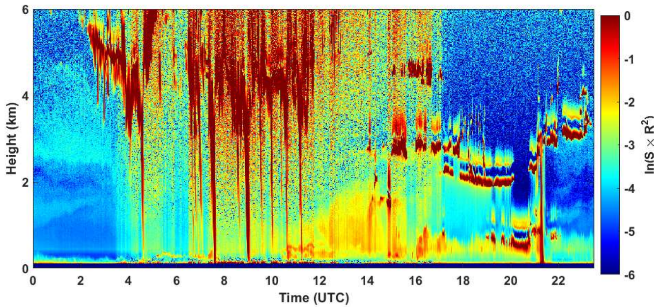
2020-05-06 RCS quick look CHM15k - ILVA LIDAR2 PARCHI
