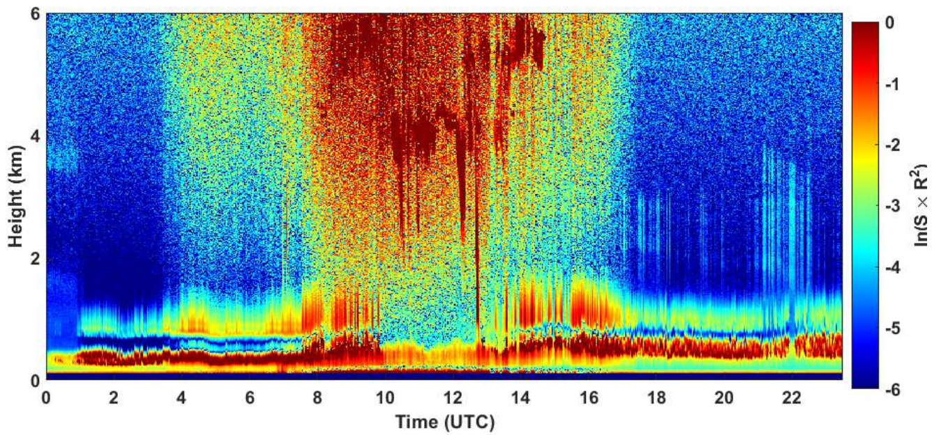
2020-05-10 RCS quick look CHM15k - ILVA LIDAR2 PARCHI
