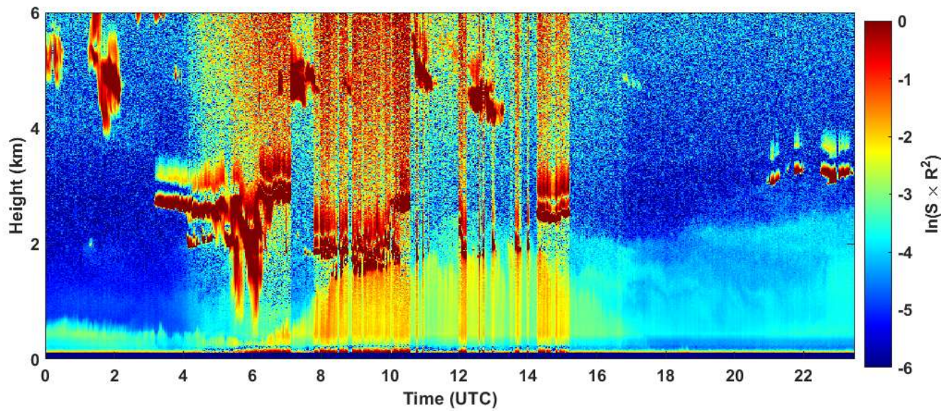
2020-04-06 RCS quick look CHM15k - ILVA LIDAR2 PARCHI
