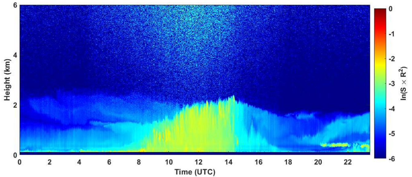
2020-04-10 RCS quick look CHM15k - ILVA LIDAR3 AGGLOMERATO
