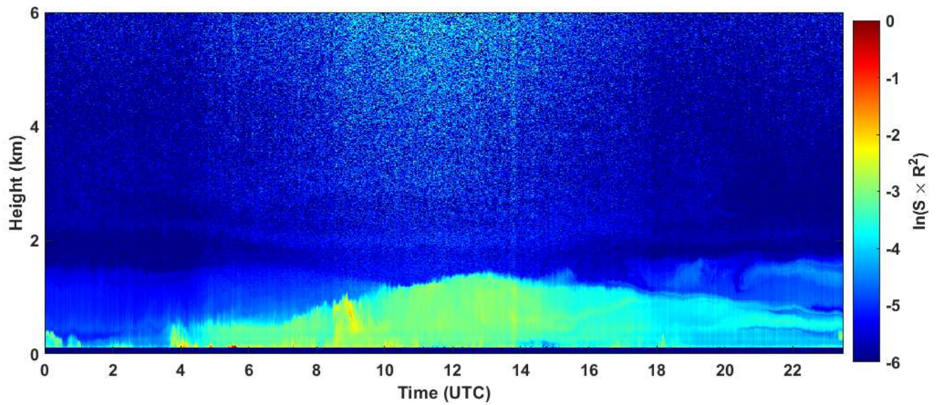
2020-04-16 RCS quick look CHM15k - ILVA LIDAR3 AGGLOMERATO
