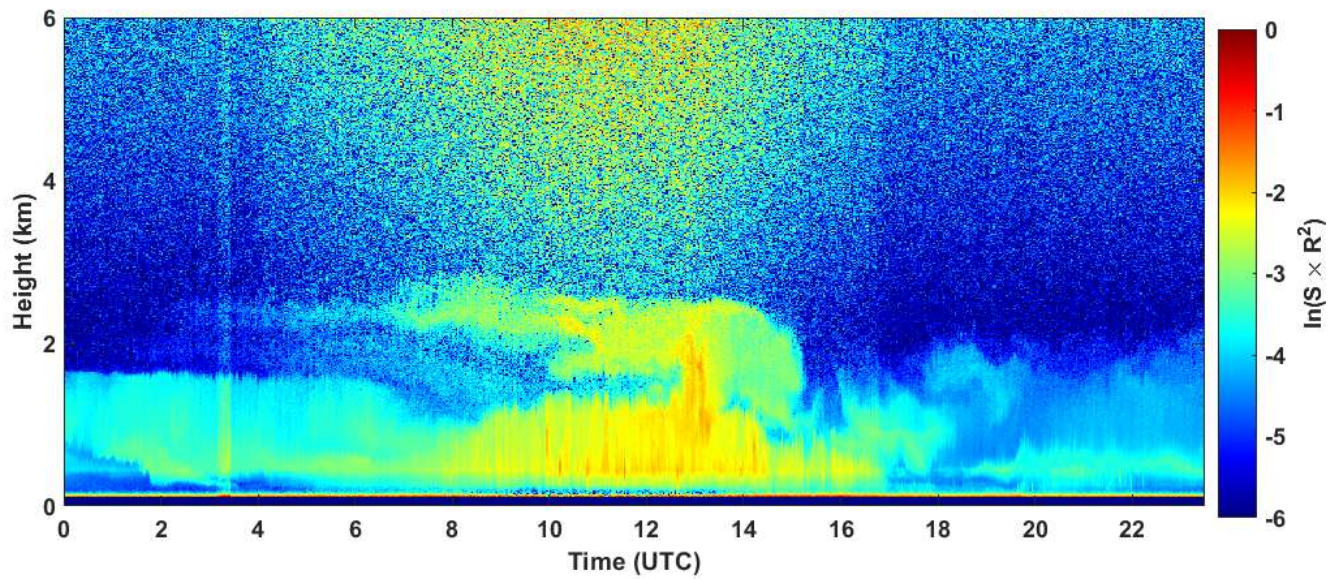
2020-04-10 RCS quick look CHM15k - ILVA LIDAR2 PARCHI
