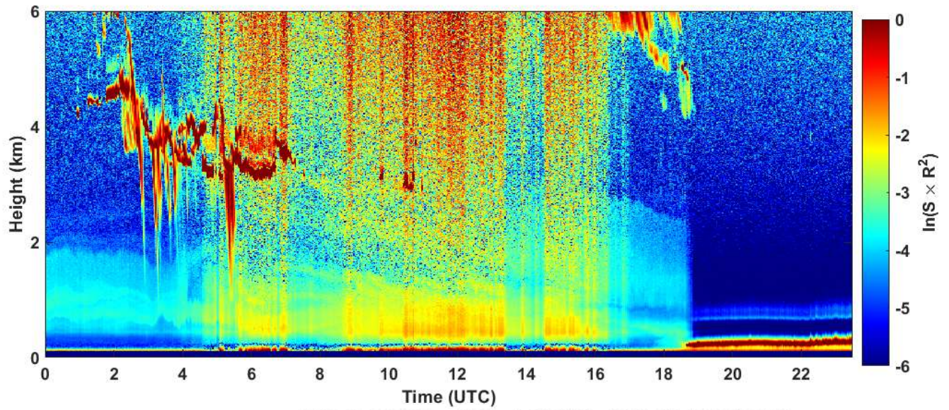
2020-04-20 RCS quick look CHM15k - ILVA LIDAR2 PARCHI
