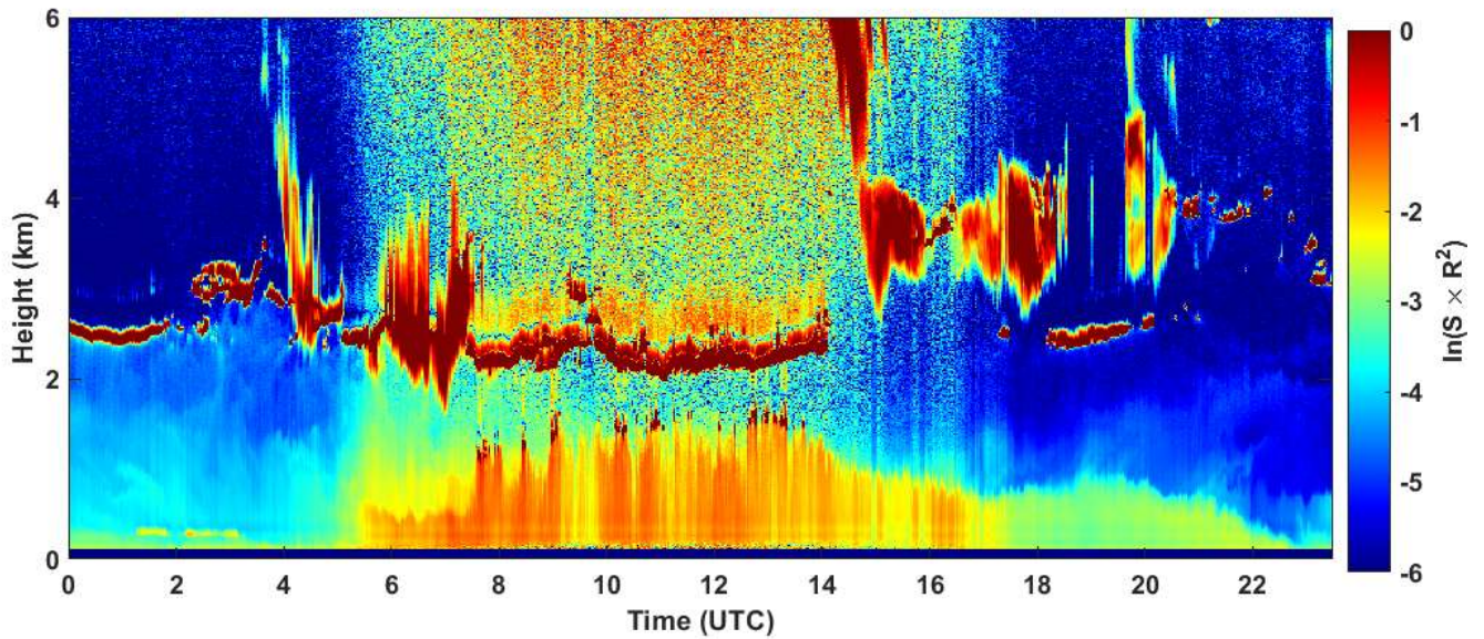
2020-04-06 RCS quick look CHM15k - ILVA LIDAR3 AGGLOMERATO
