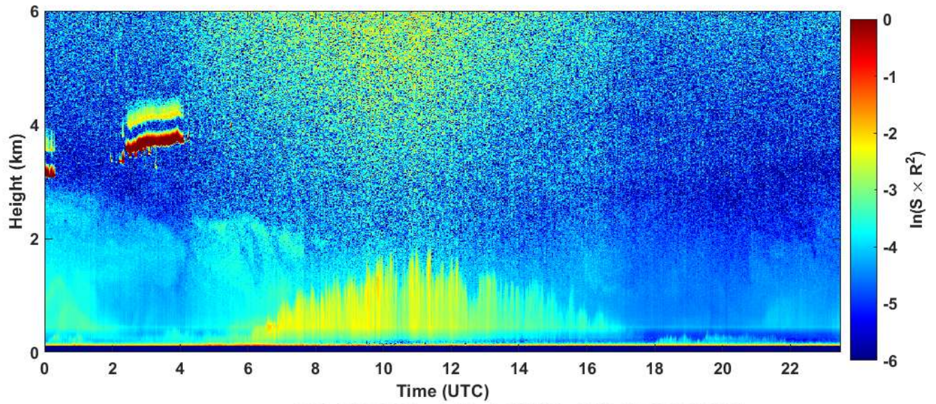
2020-04-08 RCS quick look CHM15k - ILVA LIDAR2 PARCHI
