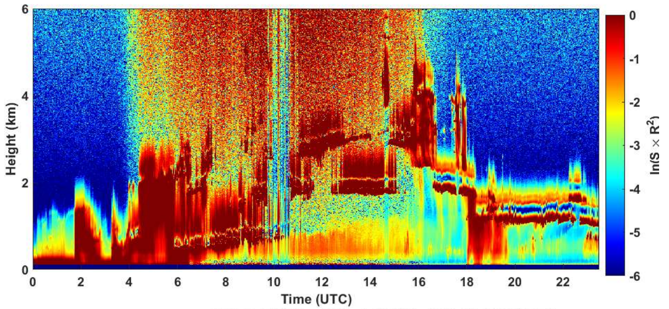
2020-04-24 RCS quick look CHM15k - ILVA LIDAR2 PARCHI
