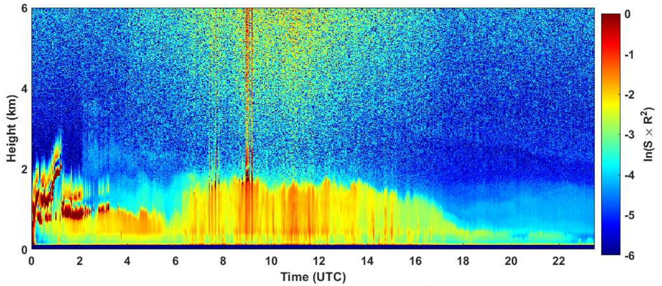
2020-04-16 RCS quick look CHM15k - ILVA LIDAR2 PARCHI
