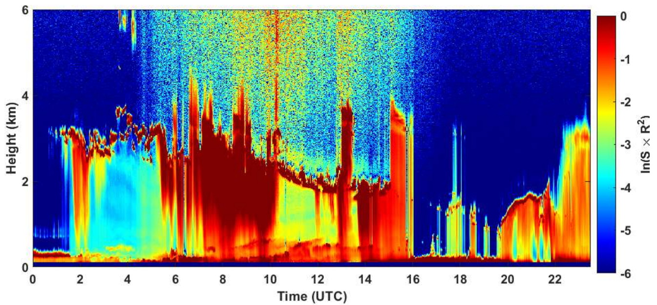
2020-04-20 RCS quick look CHM15k - ILVA LIDAR3 AGGLOMERATO
