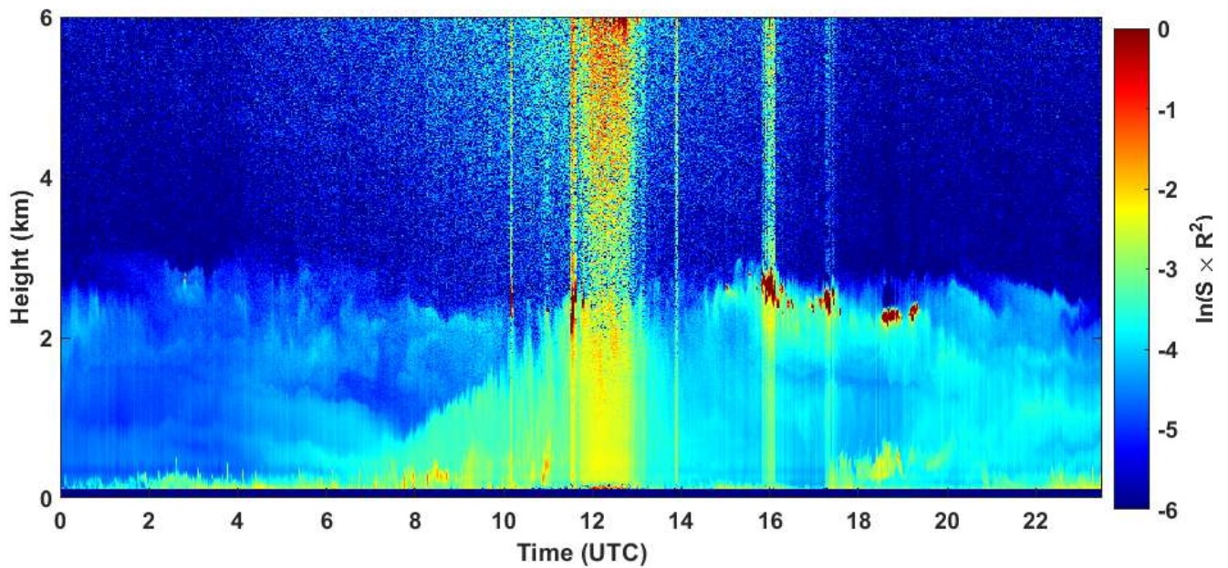
2020-04-30 RCS quick look CHM15k - ILVA LIDAR3 AGGLOMERATO
