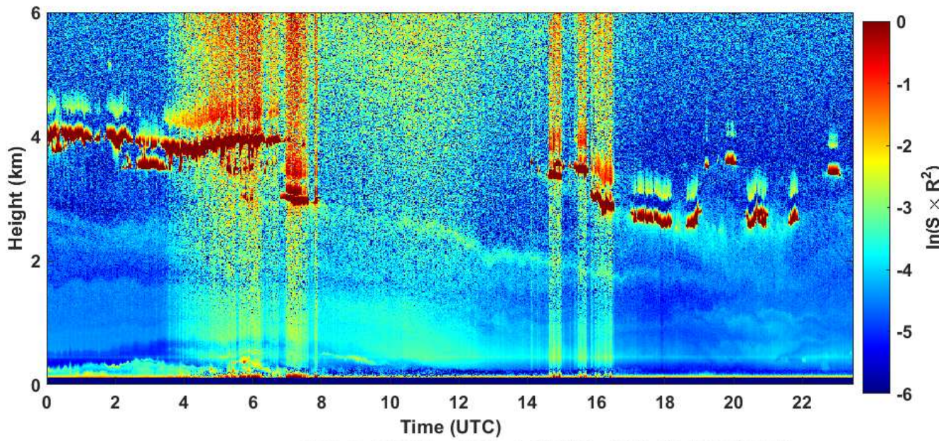
2020-04-28 RCS quick look CHM15k - ILVA LIDAR2 PARCHI
