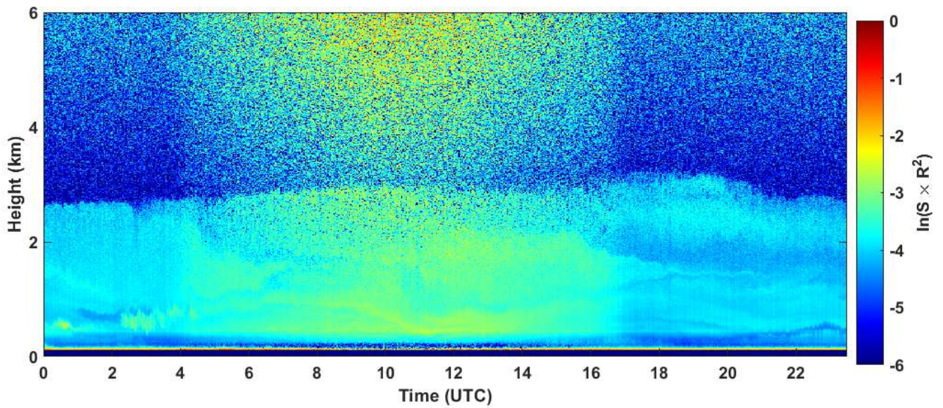
2020-04-12 RCS quick look CHM15k - ILVA LIDAR2 PARCHI
