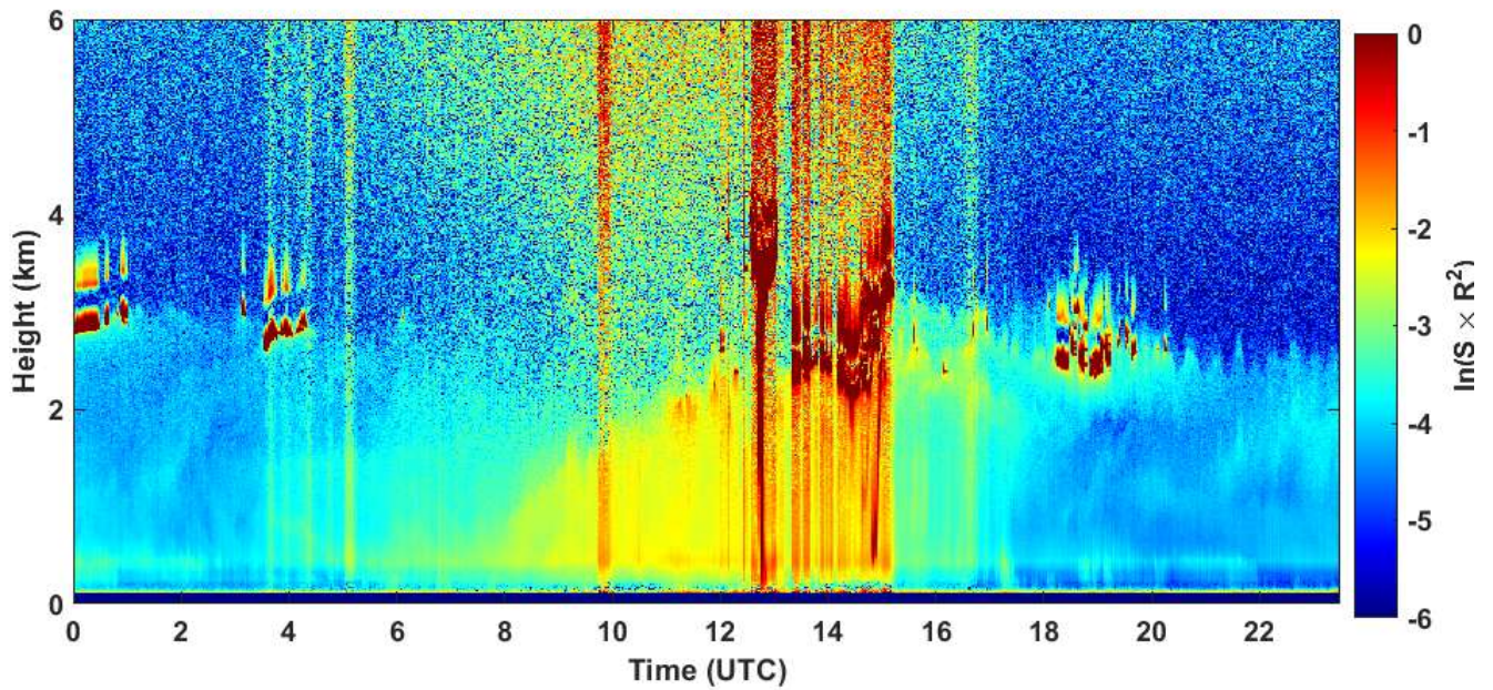
2020-04-30 RCS quick look CHM15k - ILVA LIDAR2 PARCHI
