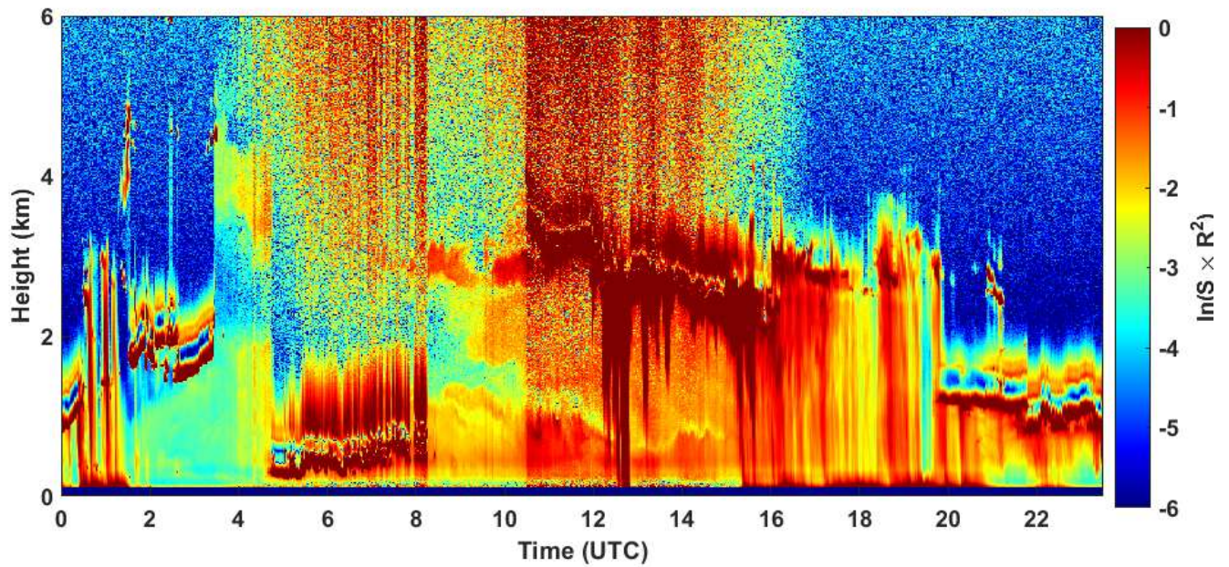
2020-04-22 RCS quick look CHM15k - ILVA LIDAR2 PARCHI
