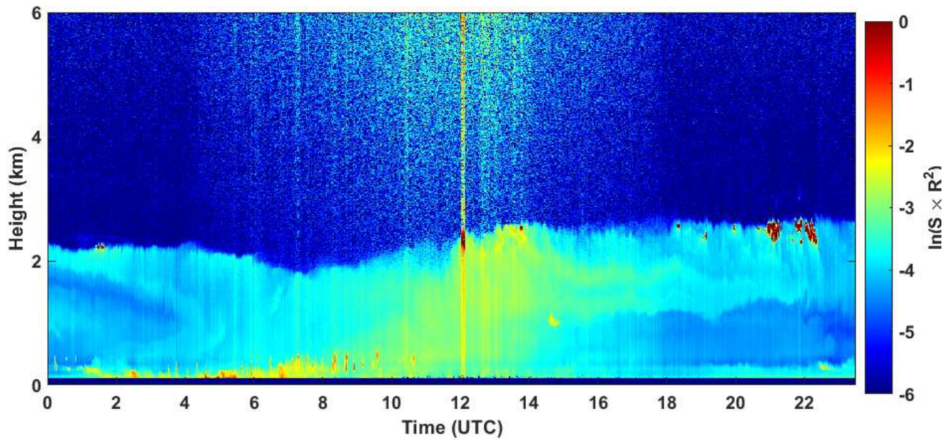
2020-04-26 RCS quick look CHM15k - ILVA LIDAR3 AGGLOMERATO
