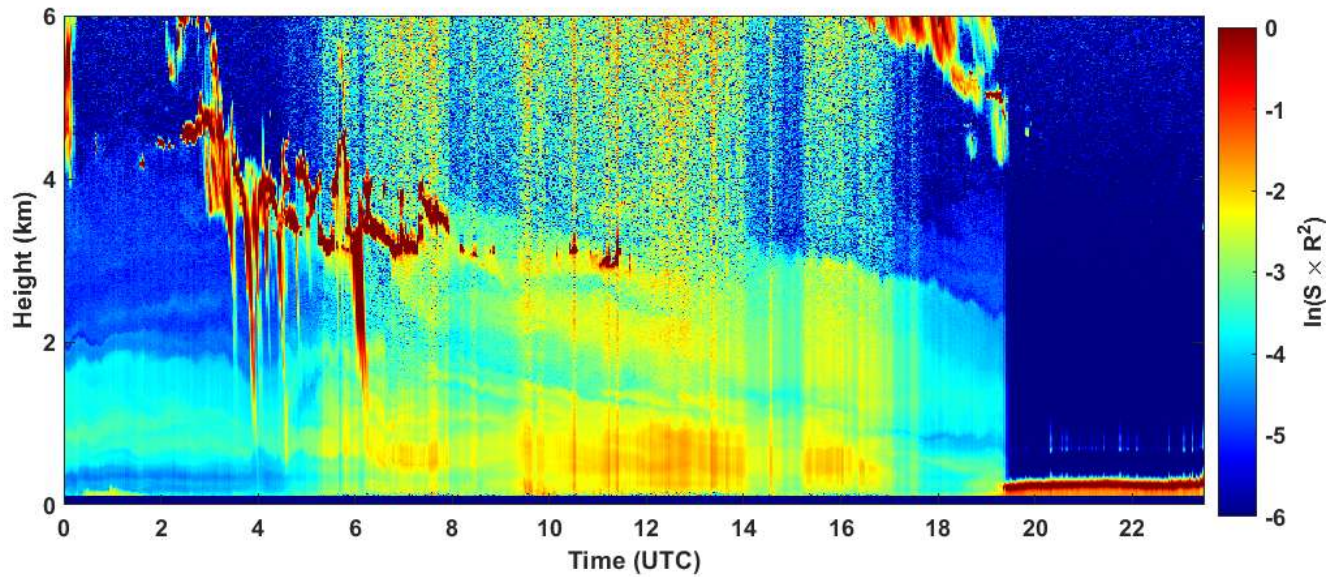
2020-04-20 RCS quick look CHM15k - ILVA LIDAR3 AGGLOMERATO
