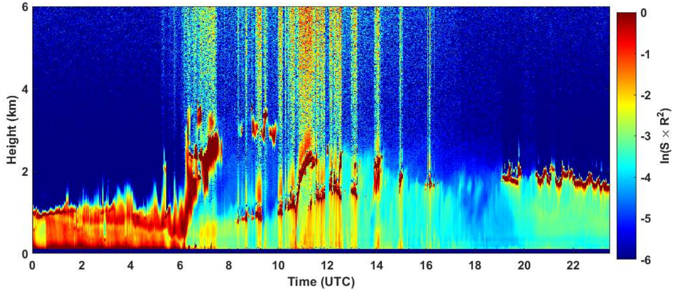
2020-04-02 RCS quick look CHM15k - ILVA LIDAR3 AGGLOMERATO
