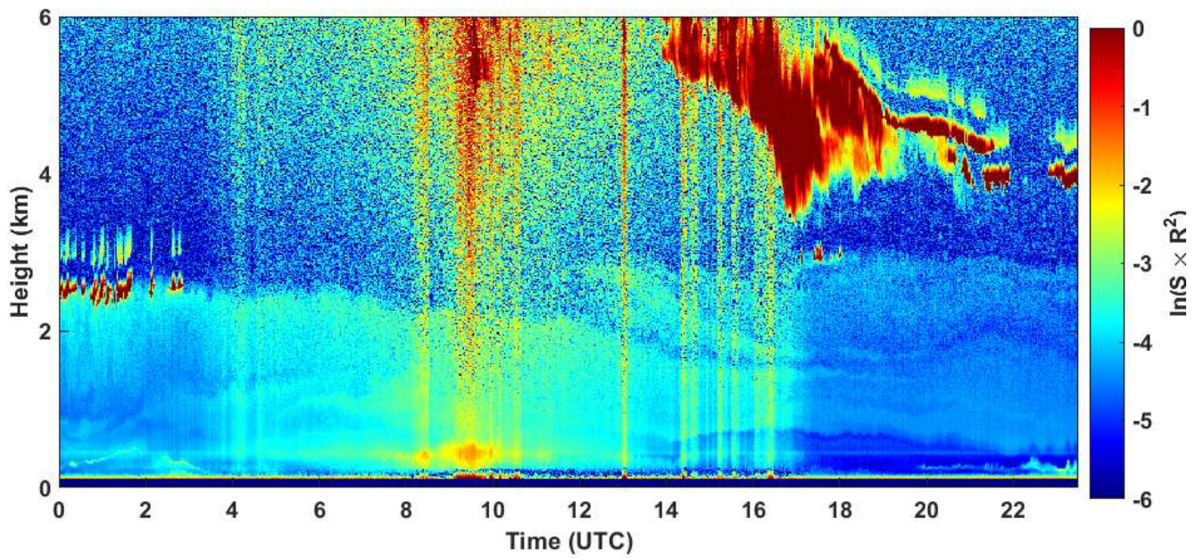
2020-04-26 RCS quick look CHM15k - ILVA LIDAR2 PARCHI
