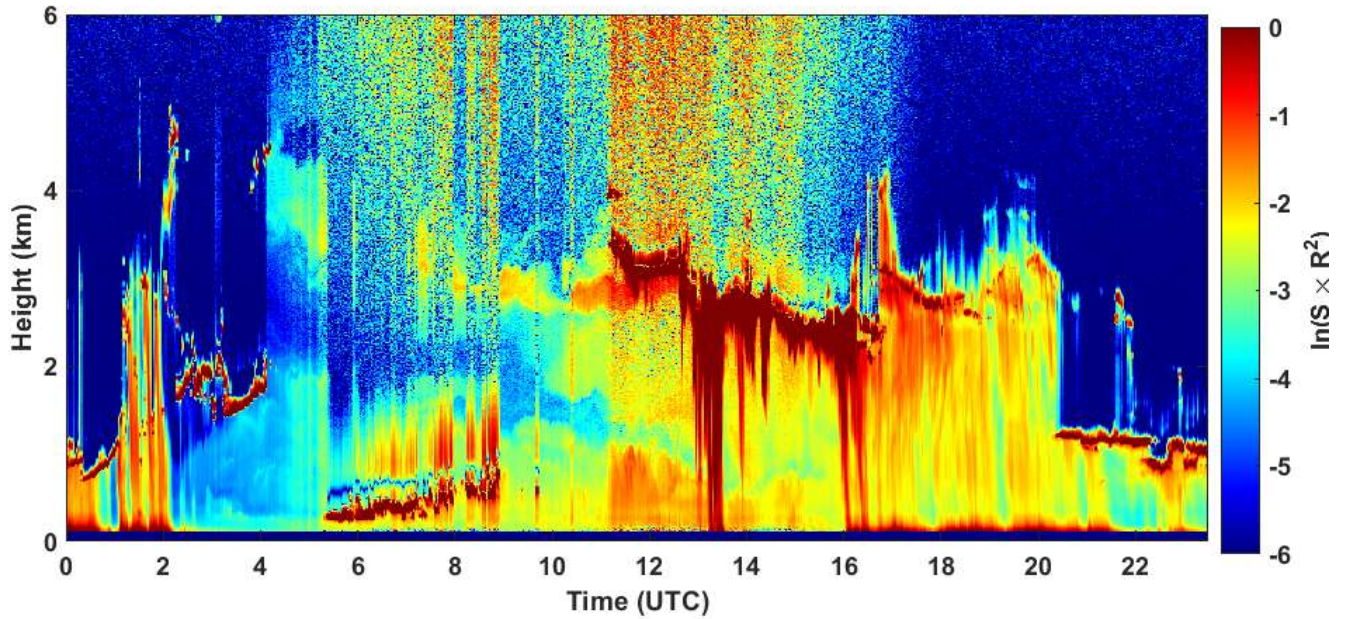
2020-04-22 RCS quick look CHM15k - ILVA LIDAR3 AGGLOMERATO
