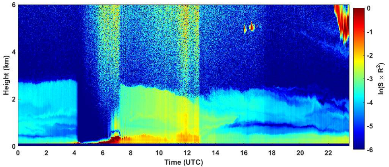
2020-04-14 RCS quick look CHM15k - ILVA LIDAR3 AGGLOMERATO
