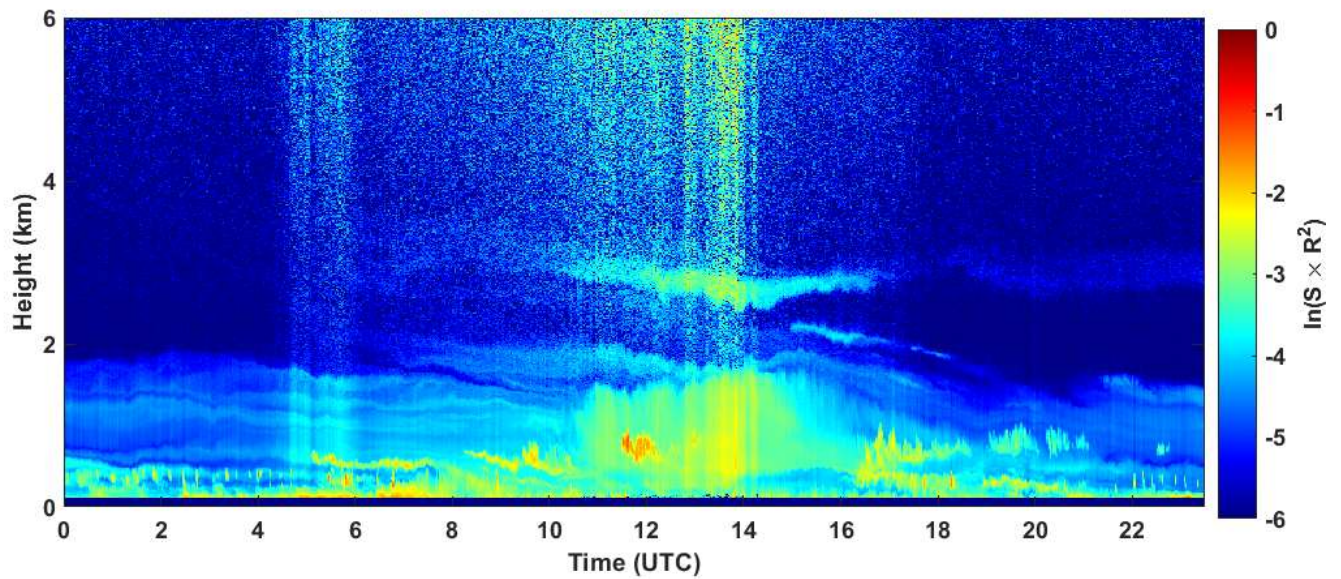
2020-04-18 RCS quick look CHM15k - ILVA LIDAR3 AGGLOMERATO
