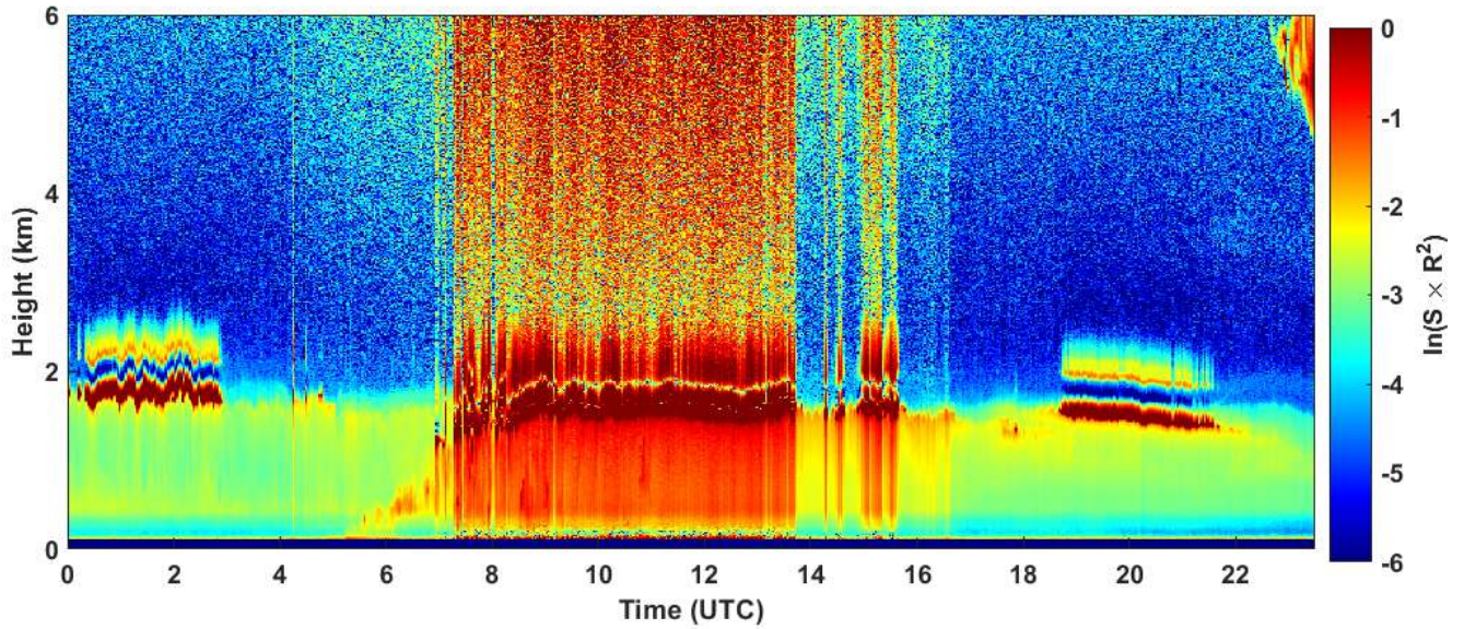
2020-04-02 RCS quick look CHM15k - ILVA LIDAR2 PARCHI
