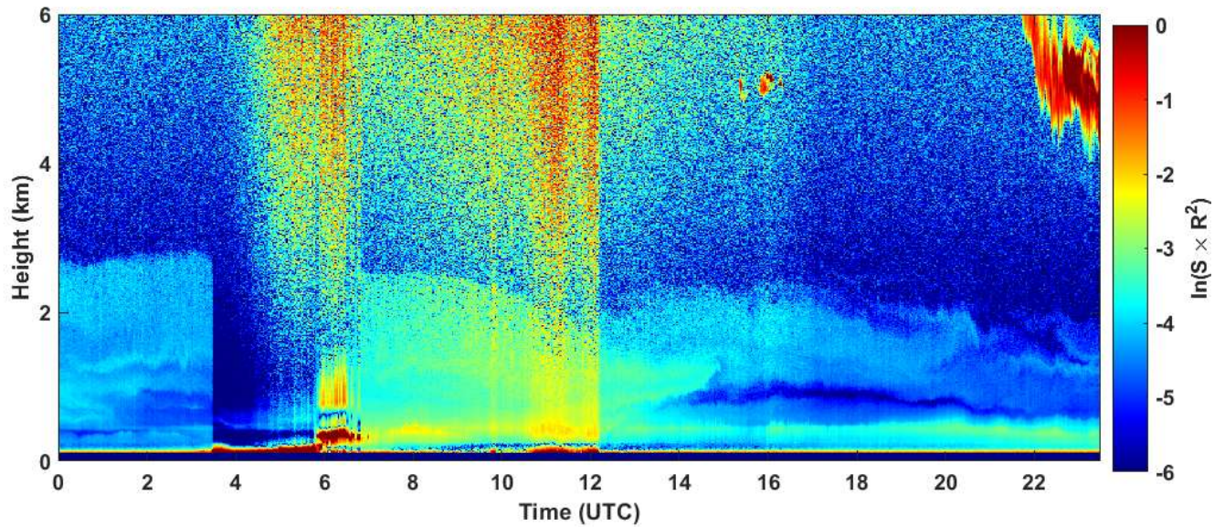
2020-04-14 RCS quick look CHM15k - ILVA LIDAR2 PARCHI
