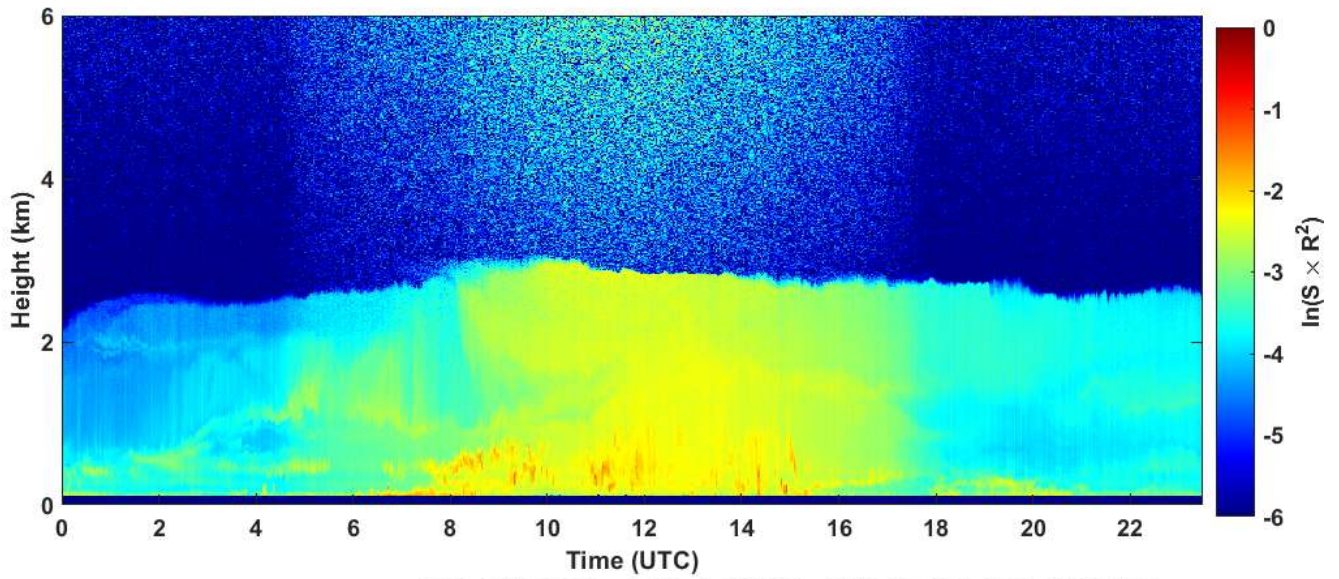
2020-04-12 RCS quick look CHM15k - ILVA LIDAR3 AGGLOMERATO
