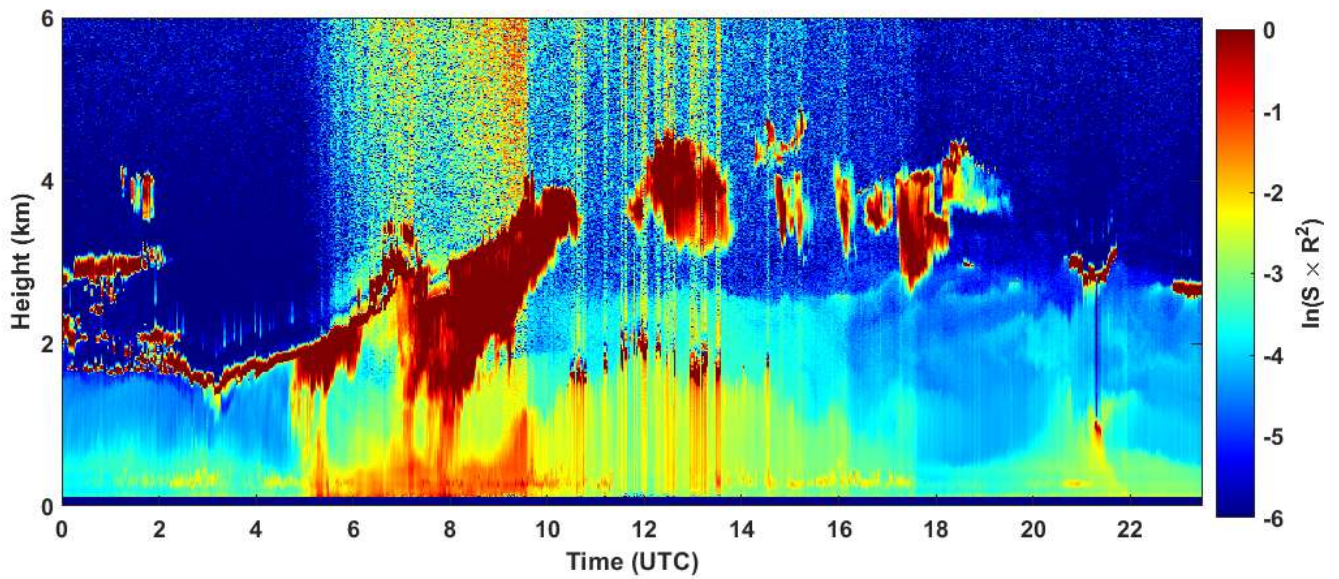
2020-04-04 RCS quick look CHM15k - ILVA LIDAR3 AGGLOMERATO
