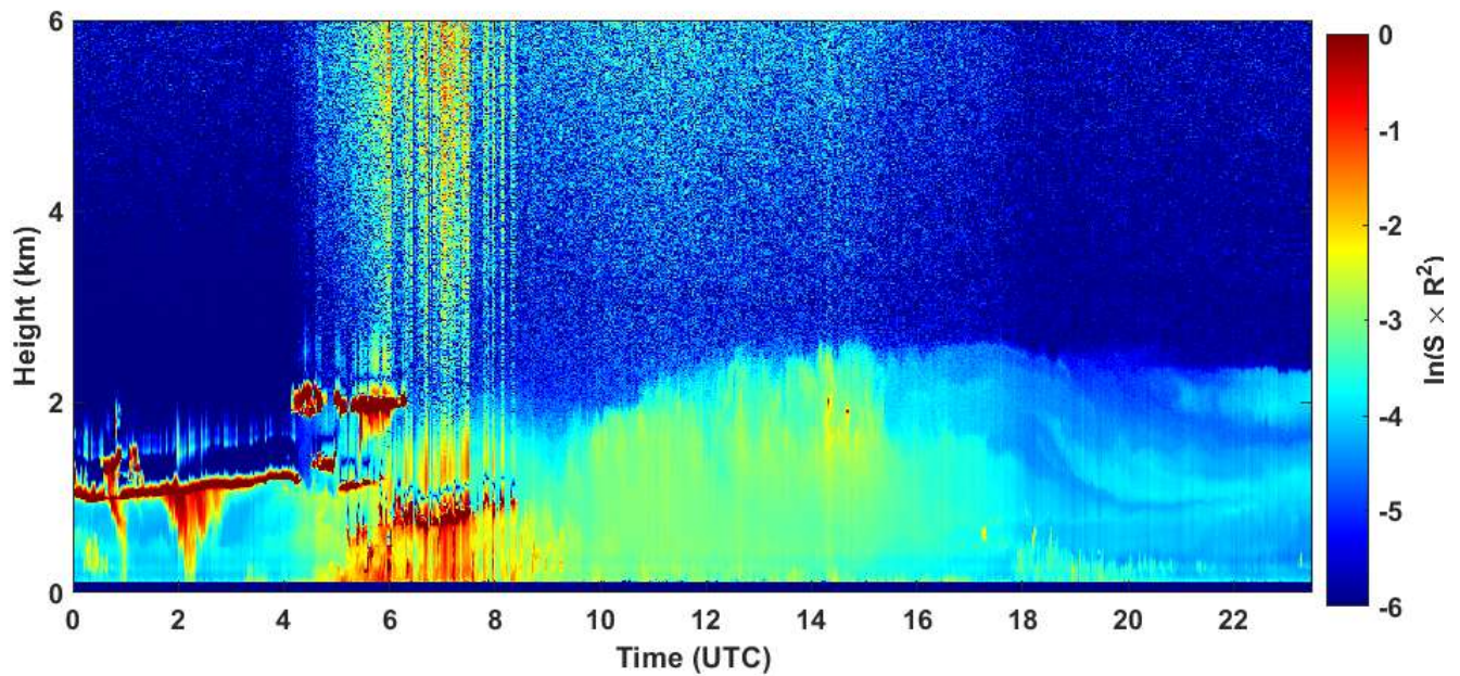
2020-04-24 RCS quick look CHM15k - ILVA LIDAR3 AGGLOMERATO
