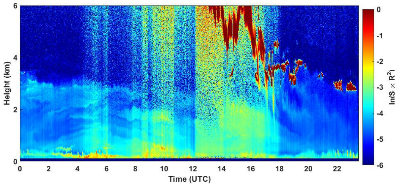
2020-04-28 RCS quick look CHM15k - ILVA LIDAR3 AGGLOMERATO
