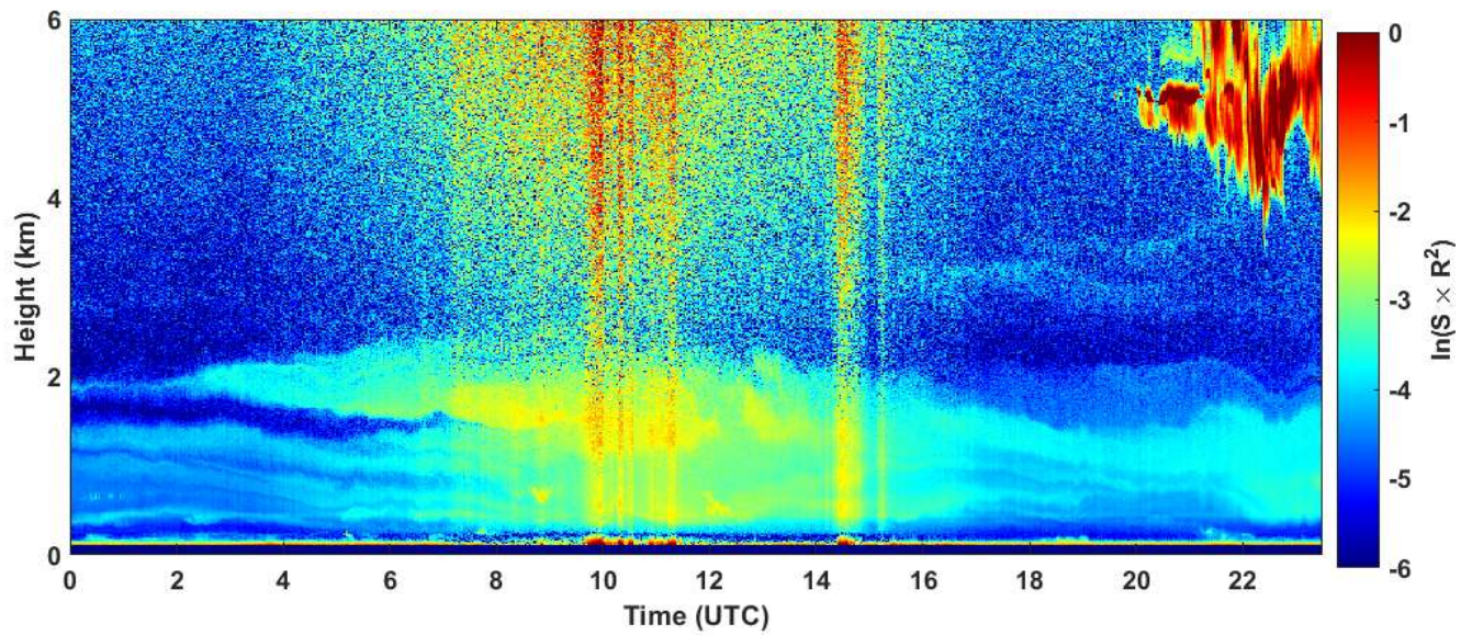
2020-04-18 RCS quick look CHM15k - ILVA LIDAR2 PARCHI
