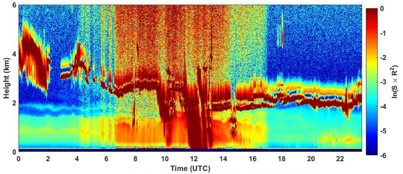
2020-04-04 RCS quick look CHM15k - ILVA LIDAR2 PARCHI
