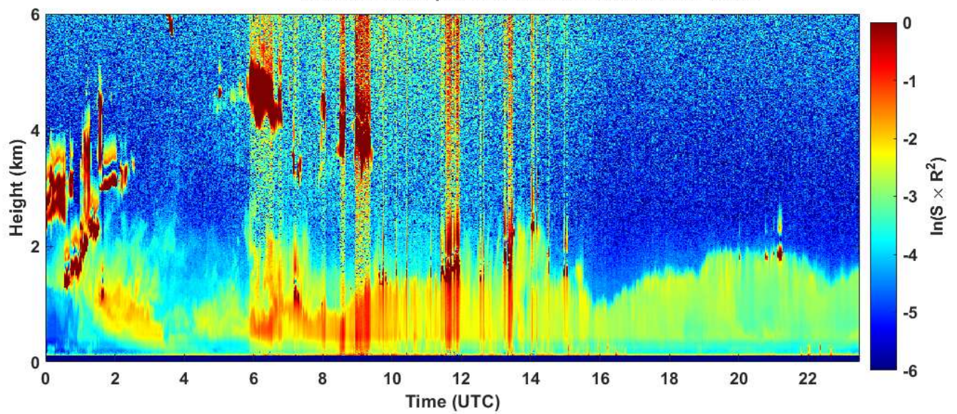
2020-02-20 RCS quick look CHM15k - ILVA LIDAR2 PARCHI
