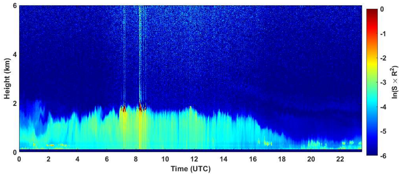
2020-02-22 RCS quick look CHM15k - ILVA LIDAR3 AGGLOMERATO
