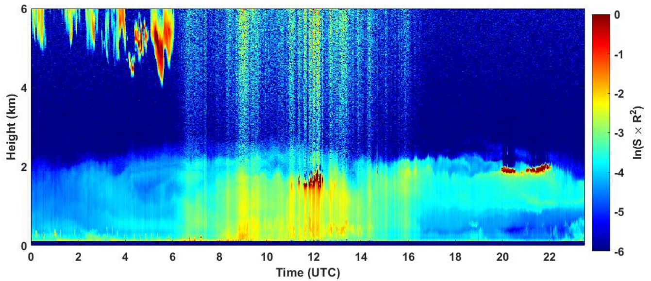
2020-02-12 RCS quick look CHM15k - ILVA LIDAR3 AGGLOMERATO
