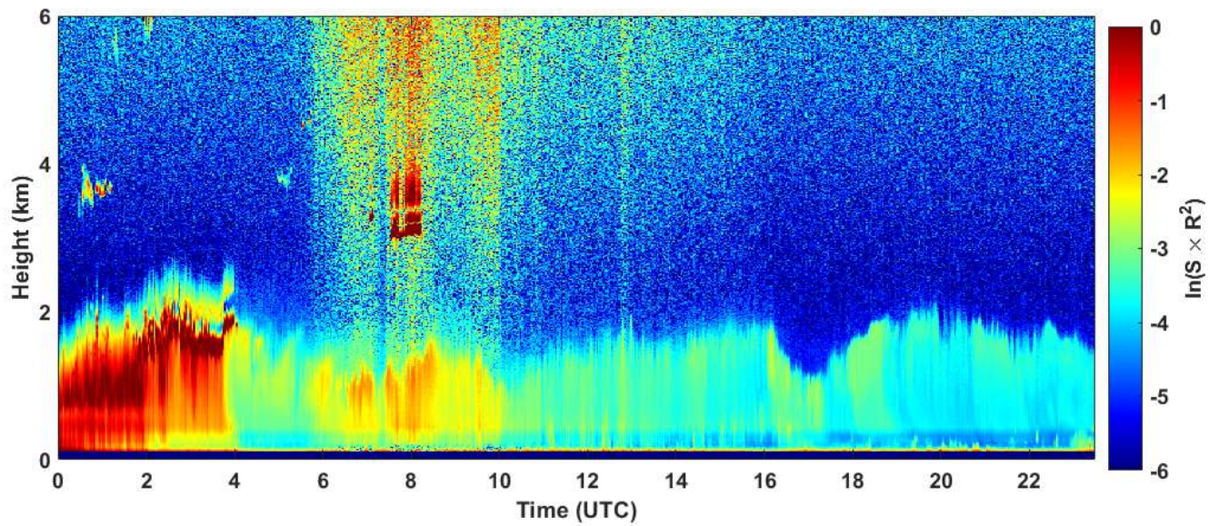
2020-02-06 RCS quick look CHM15k - ILVA LIDAR2 PARCHI
