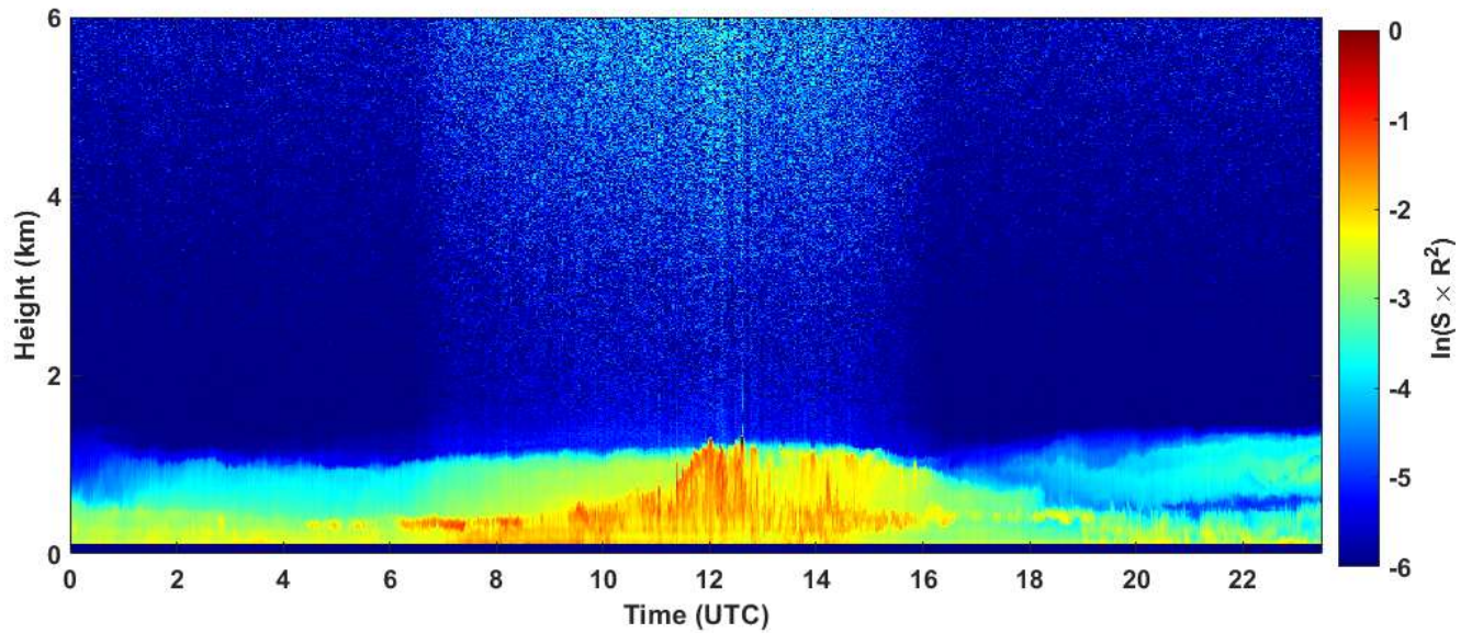
2020-01-18 RCS quick look CHM15k - ILVA LIDAR3 AGGLOMERATO
