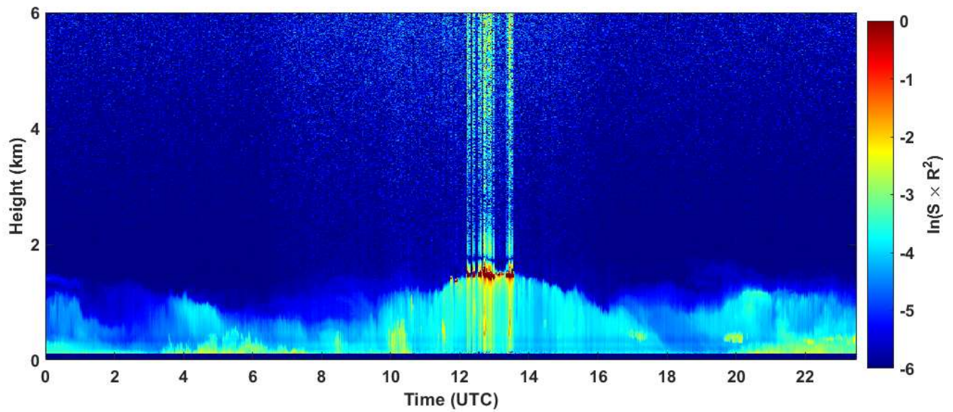
2020-01-08 RCS quick look CHM15k - ILVA LIDAR3 AGGLOMERATO
