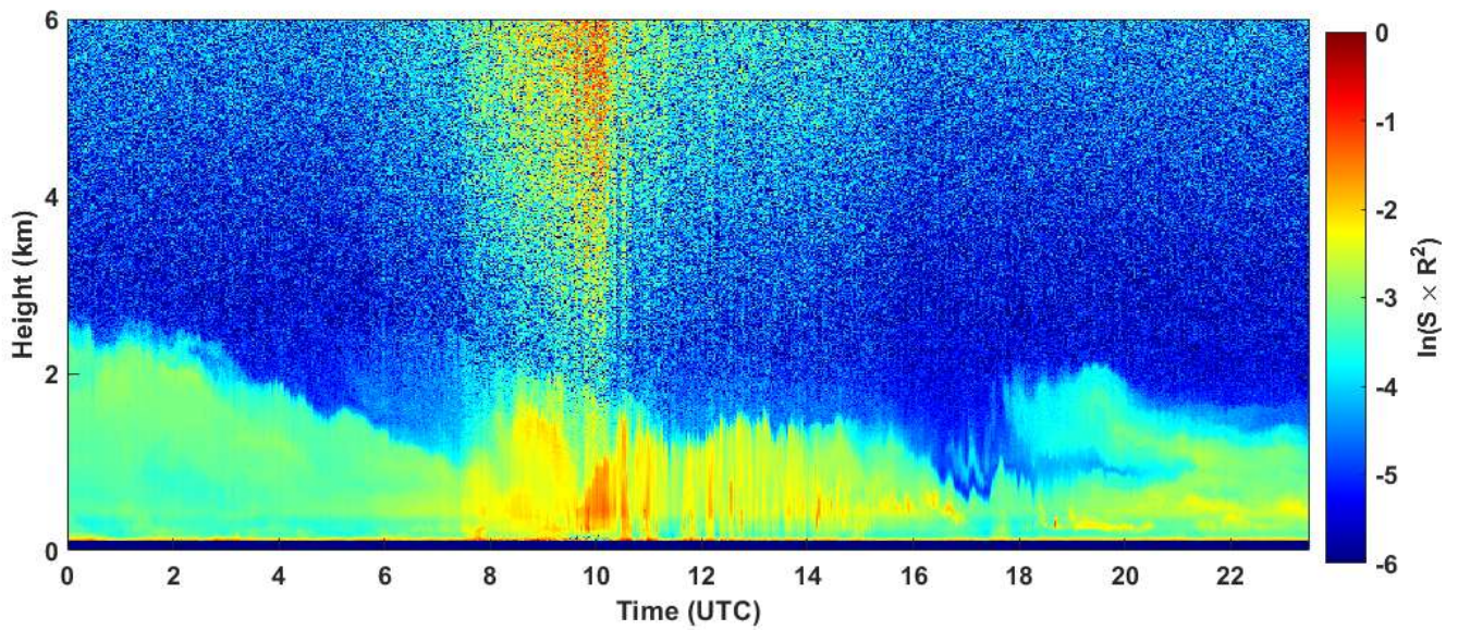
2020-01-30 RCS quick look CHM15k - ILVA LIDAR2 PARCHI
