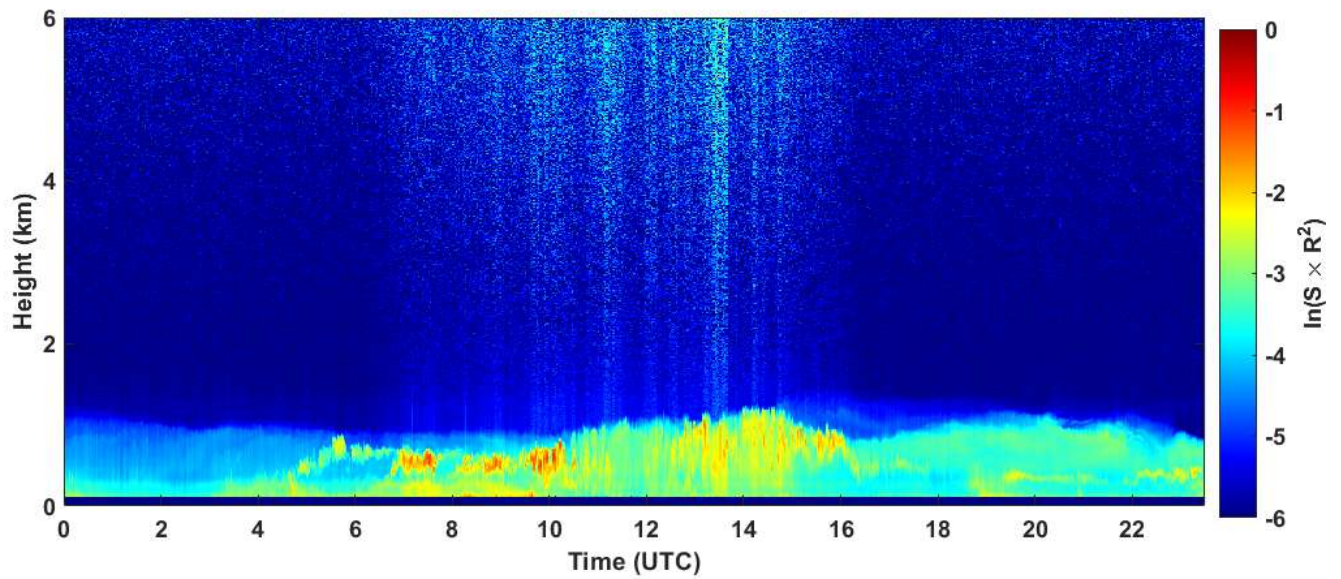
2020-01-22 RCS quick look CHM15k - ILVA LIDAR3 AGGLOMERATO
