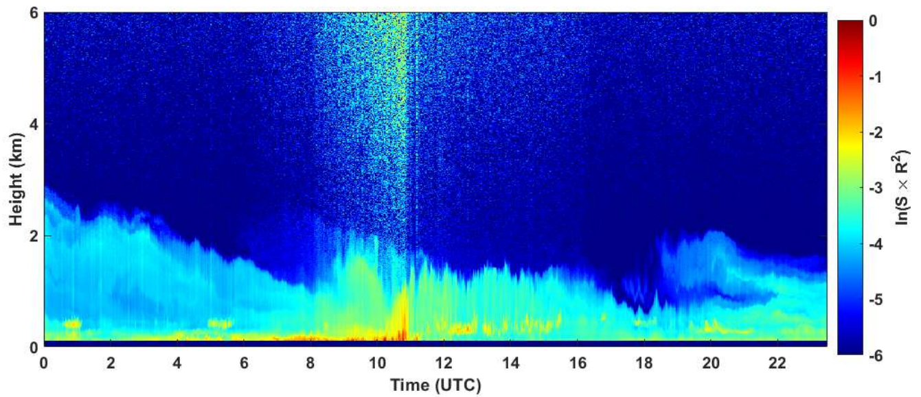
2020-01-30 RCS quick look CHM15k - ILVA LIDAR3 AGGLOMERATO
