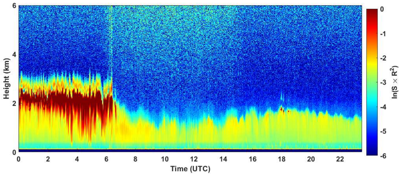
2020-01-06 RCS quick look CHM15k - ILVA LIDAR2 PARCHI
