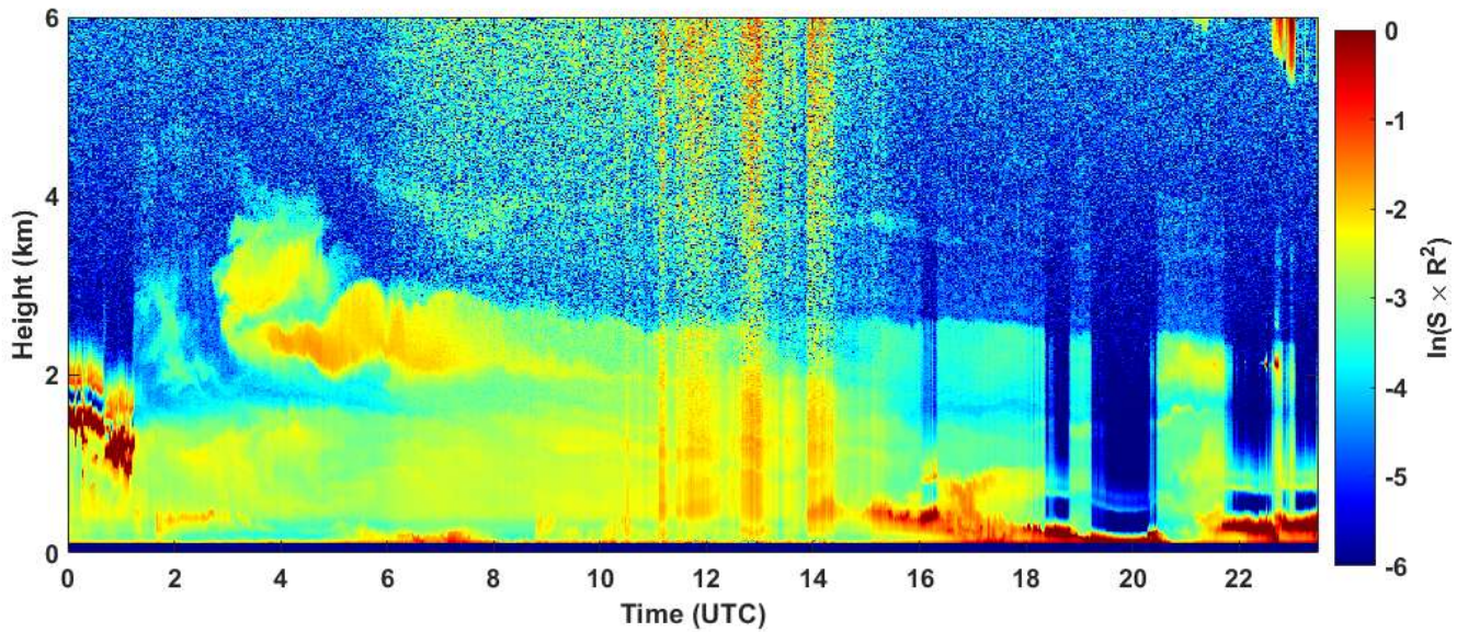
2020-01-26 RCS quick look CHM15k - ILVA LIDAR2 PARCHI
