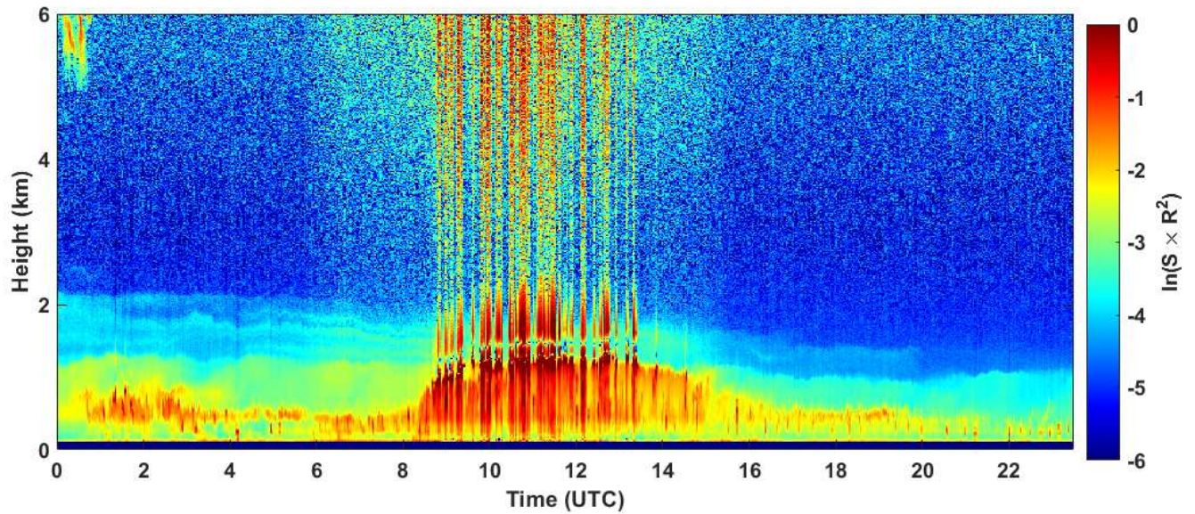
2020-01-22 RCS quick look CHM15k - ILVA LIDAR2 PARCHI
