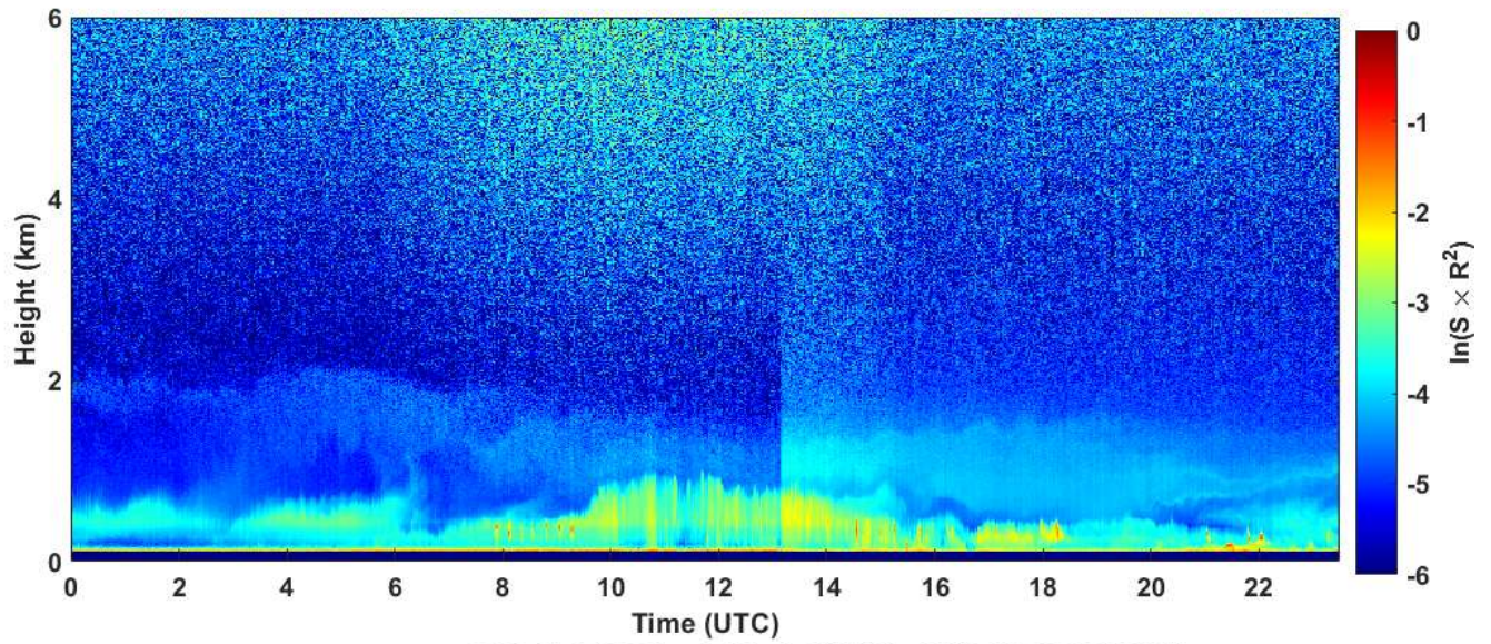
2020-01-04 RCS quick look CHM15k - ILVA LIDAR2 PARCHI
