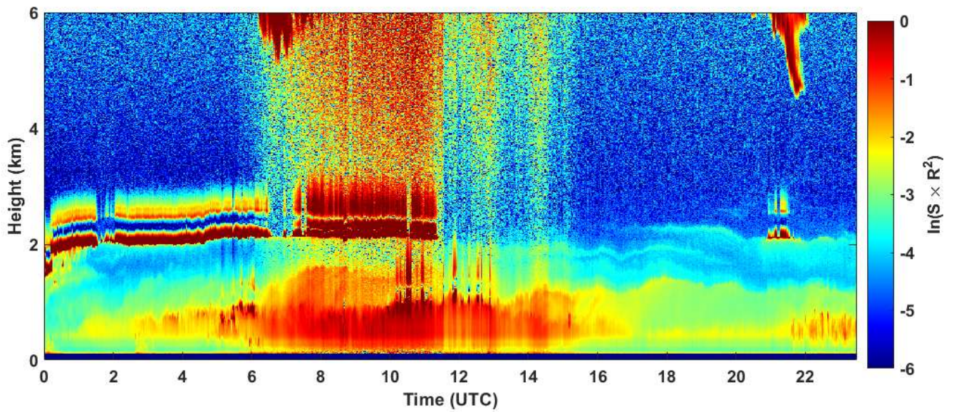
2020-01-20 RCS quick look CHM15k - ILVA LIDAR2 PARCHI
