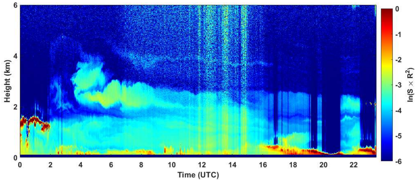
2020-01-26 RCS quick look CHM15k - ILVA LIDAR3 AGGLOMERATO
