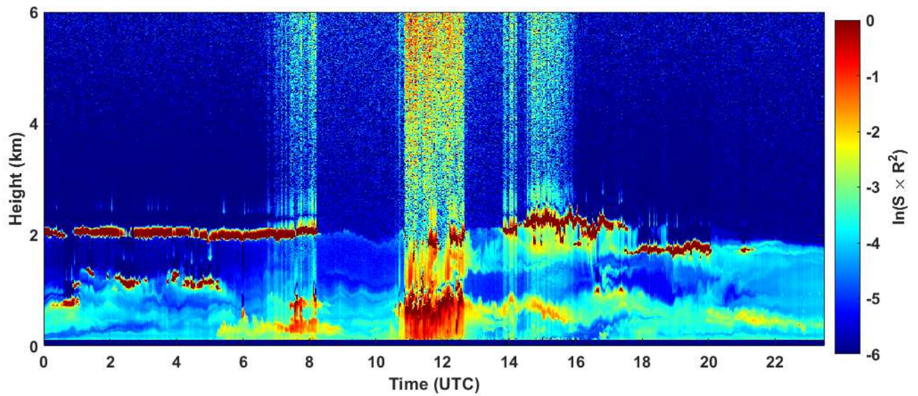
2020-01-14 RCS quick look CHM15k - ILVA LIDAR3 AGGLOMERATO
