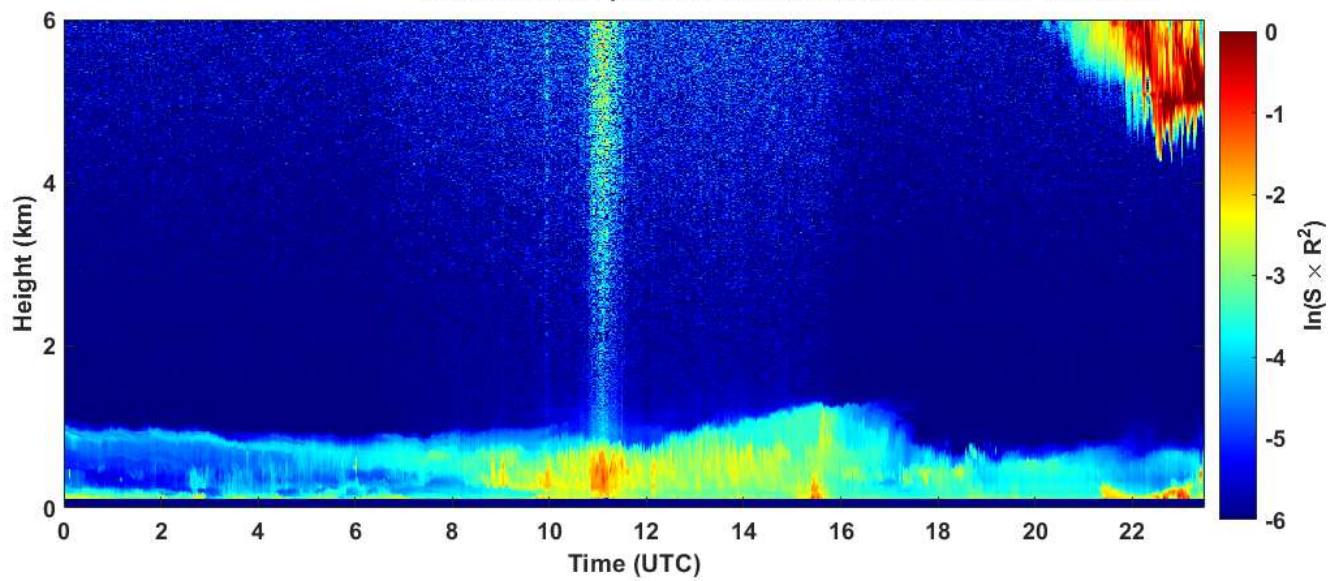
2020-01-10 RCS quick look CHM15k - ILVA LIDAR3 AGGLOMERATO
