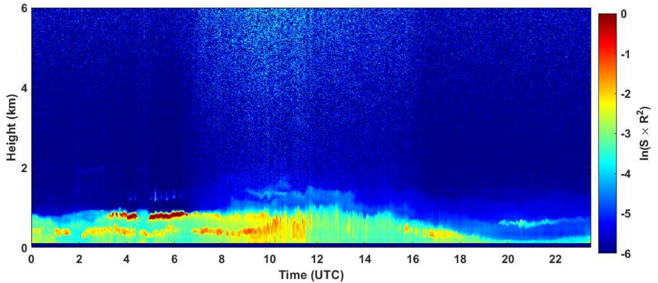
2020-01-24 RCS quick look CHM15k - ILVA LIDAR3 AGGLOMERATO
