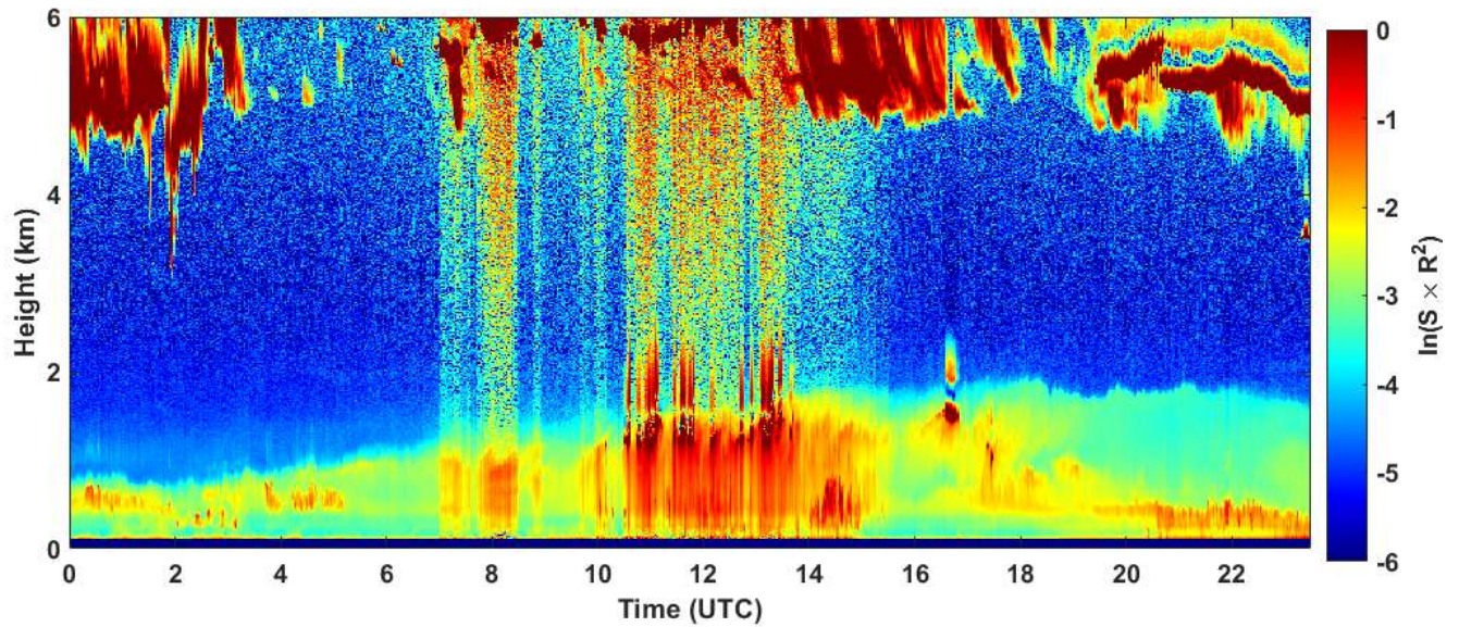
2020-01-12 RCS quick look CHM15k - ILVA LIDAR2 PARCHI
