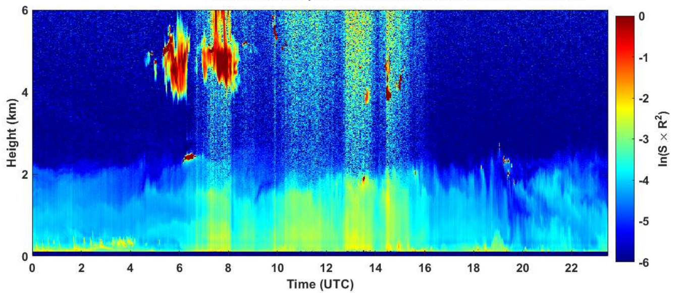
2020-01-28 RCS quick look CHM15k - ILVA LIDAR3 AGGLOMERATO
