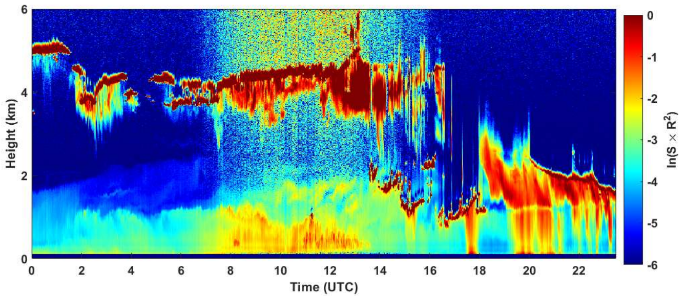
2020-01-12 RCS quick look CHM15k - ILVA LIDAR3 AGGLOMERATO
