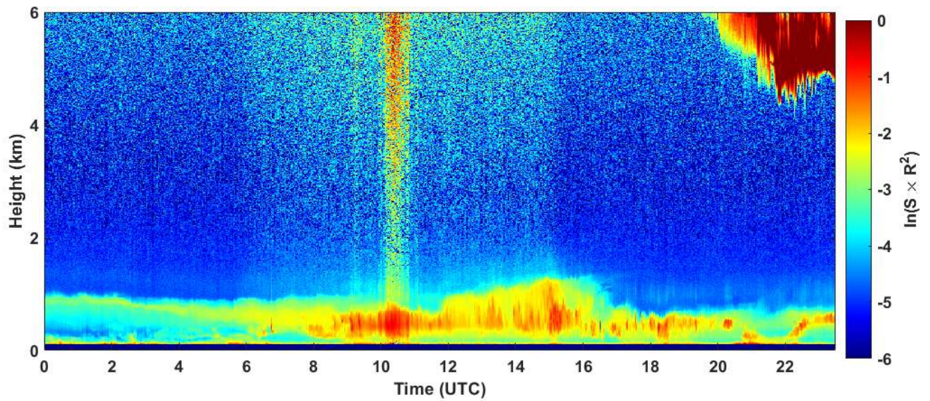
2020-01-10 RCS quick look CHM15k - ILVA LIDAR2 PARCHI
