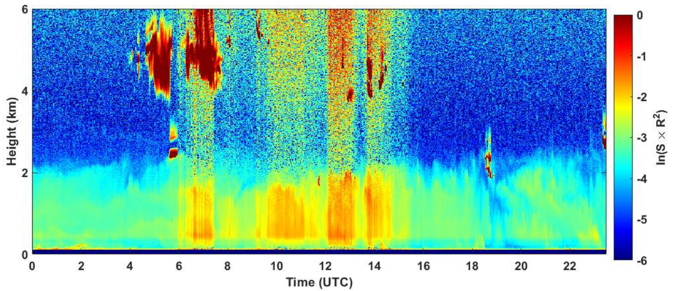
2020-01-28 RCS quick look CHM15k - ILVA LIDAR2 PARCHI
