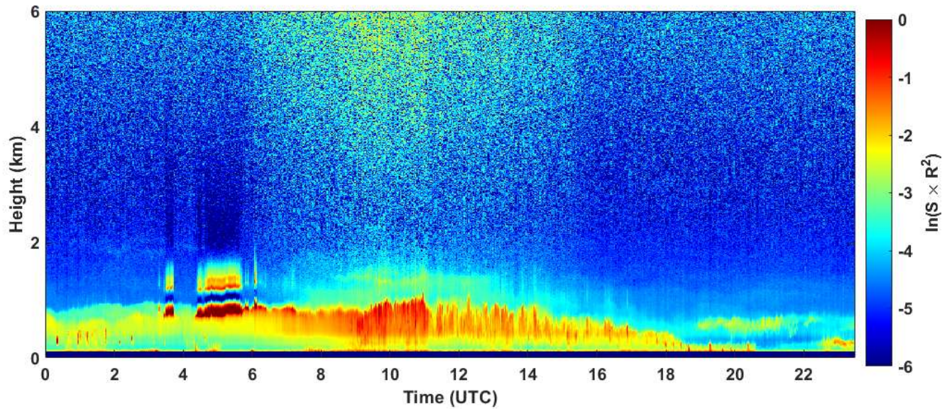
2020-01-24 RCS quick look CHM15k - ILVA LIDAR2 PARCHI
