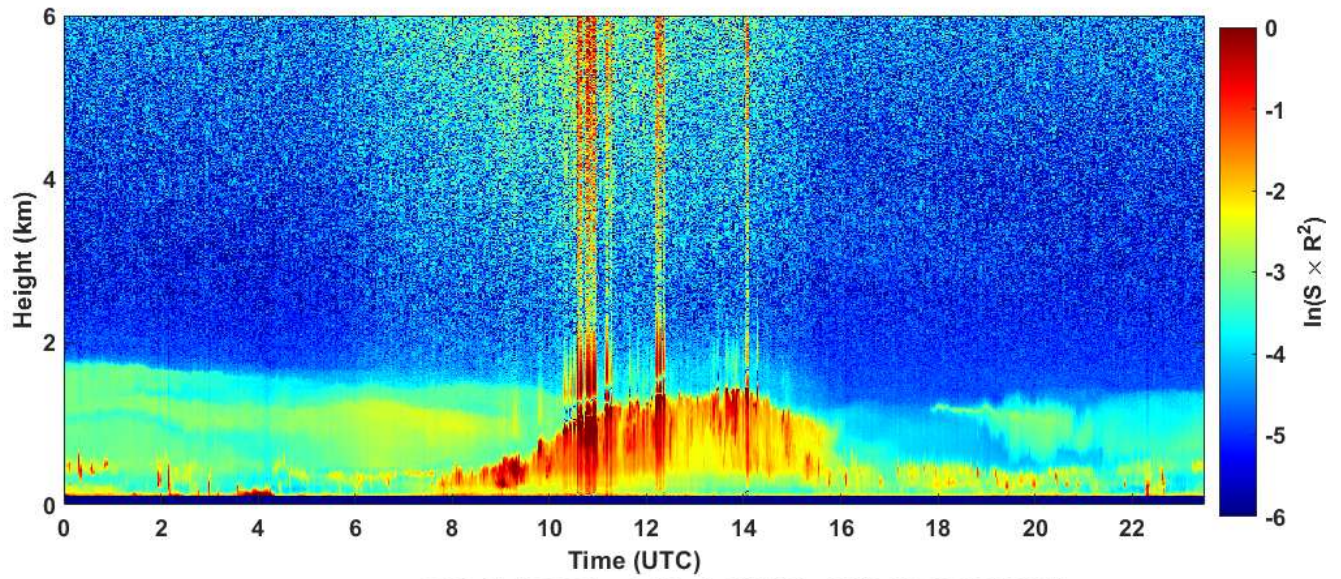
2020-01-16 RCS quick look CHM15k - ILVA LIDAR2 PARCHI
