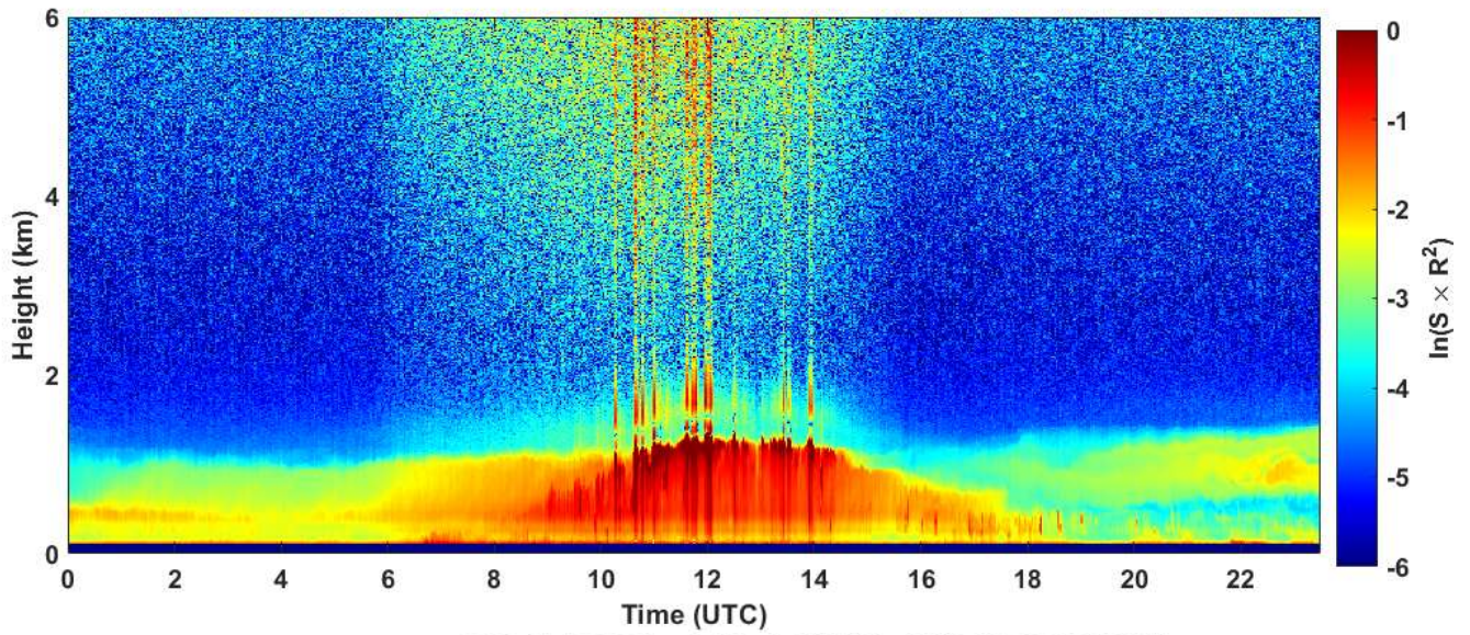
2020-01-18 RCS quick look CHM15k - ILVA LIDAR2 PARCHI
