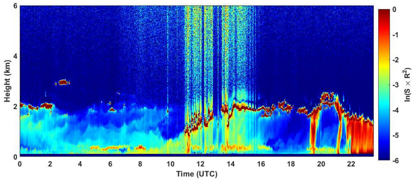
2020-01-20 RCS quick look CHM15k - ILVA LIDAR3 AGGLOMERATO
