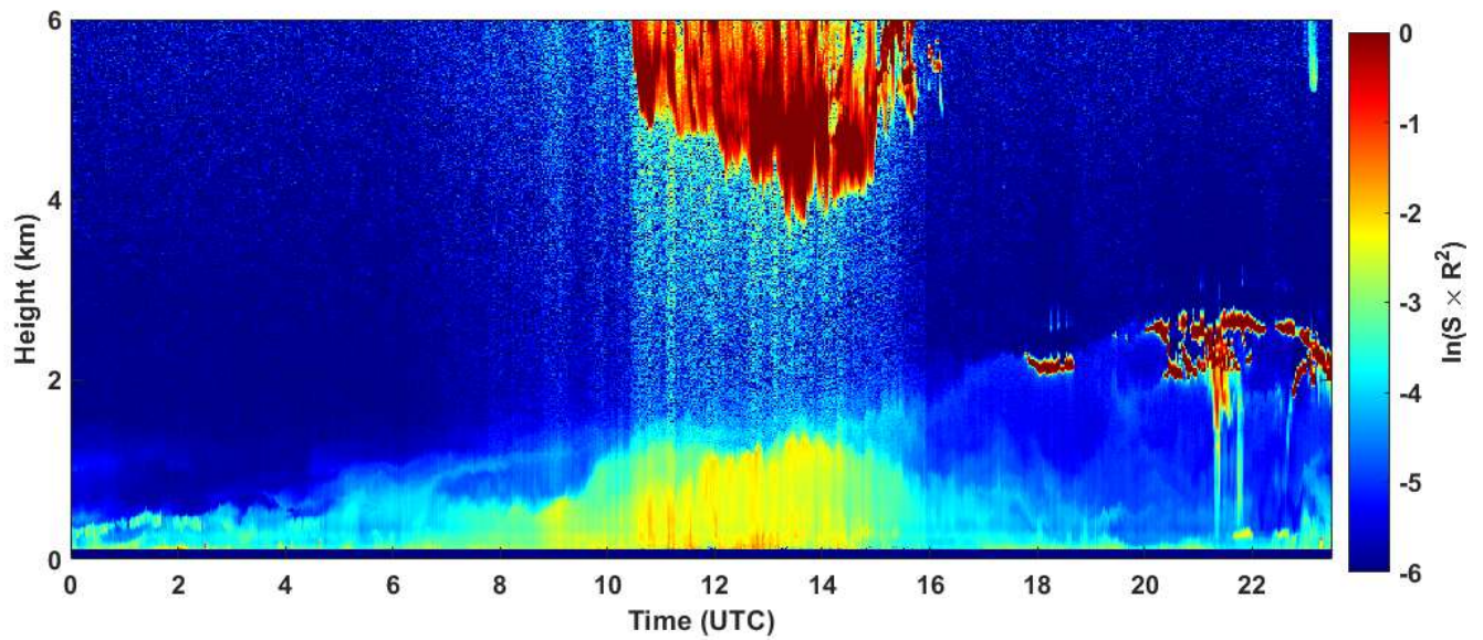
2020-01-04 RCS quick look CHM15k - ILVA LIDAR3 AGGLOMERATO
