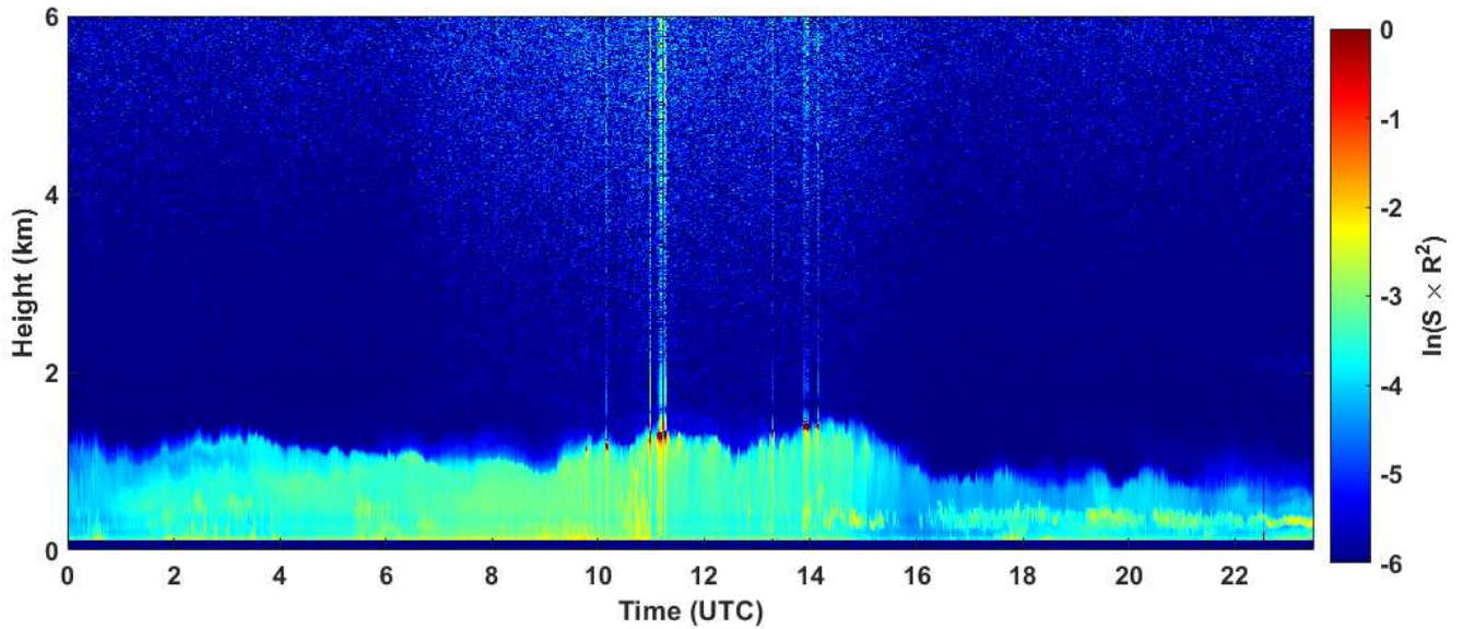
2020-01-02 RCS quick look CHM15k - ILVA LIDAR3 AGGLOMERATO
