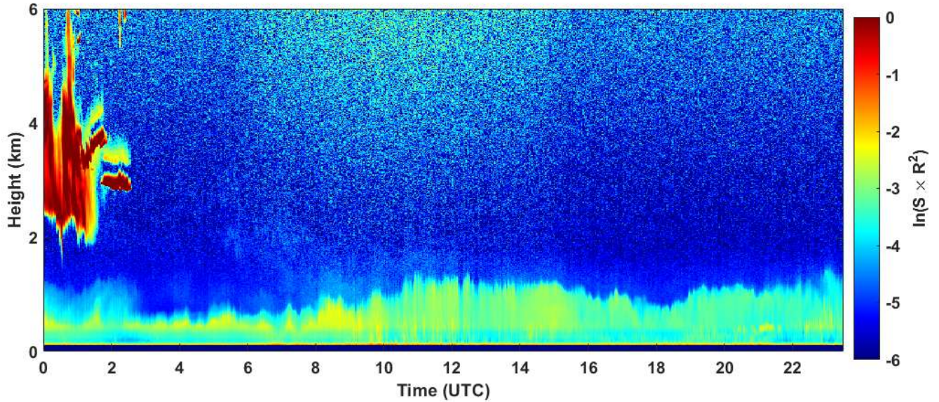
2020-01-02 RCS quick look CHM15k - ILVA LIDAR2 PARCHI
