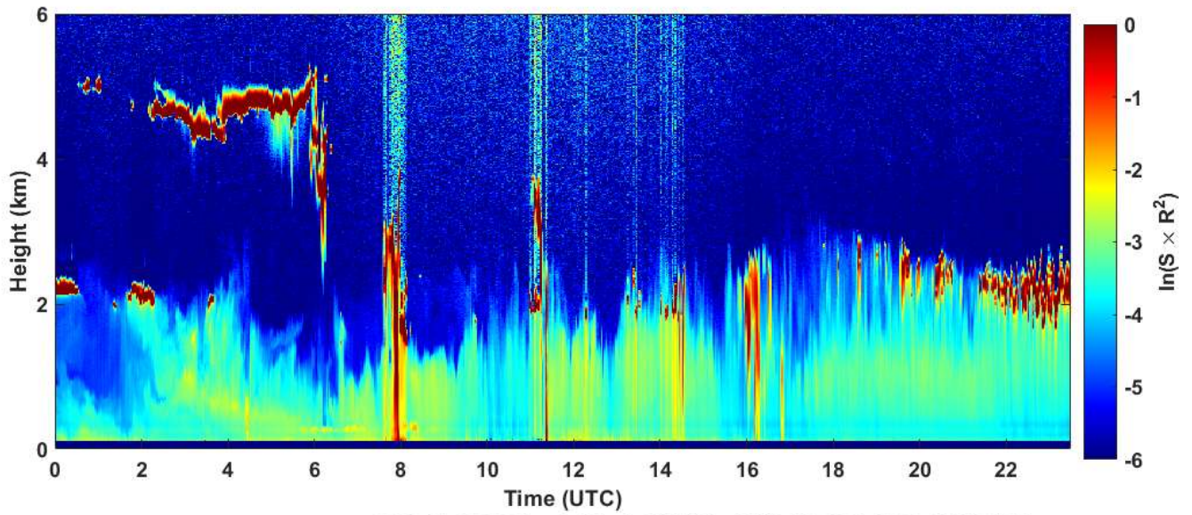
2020-01-06 RCS quick look CHM15k - ILVA LIDAR3 AGGLOMERATO
