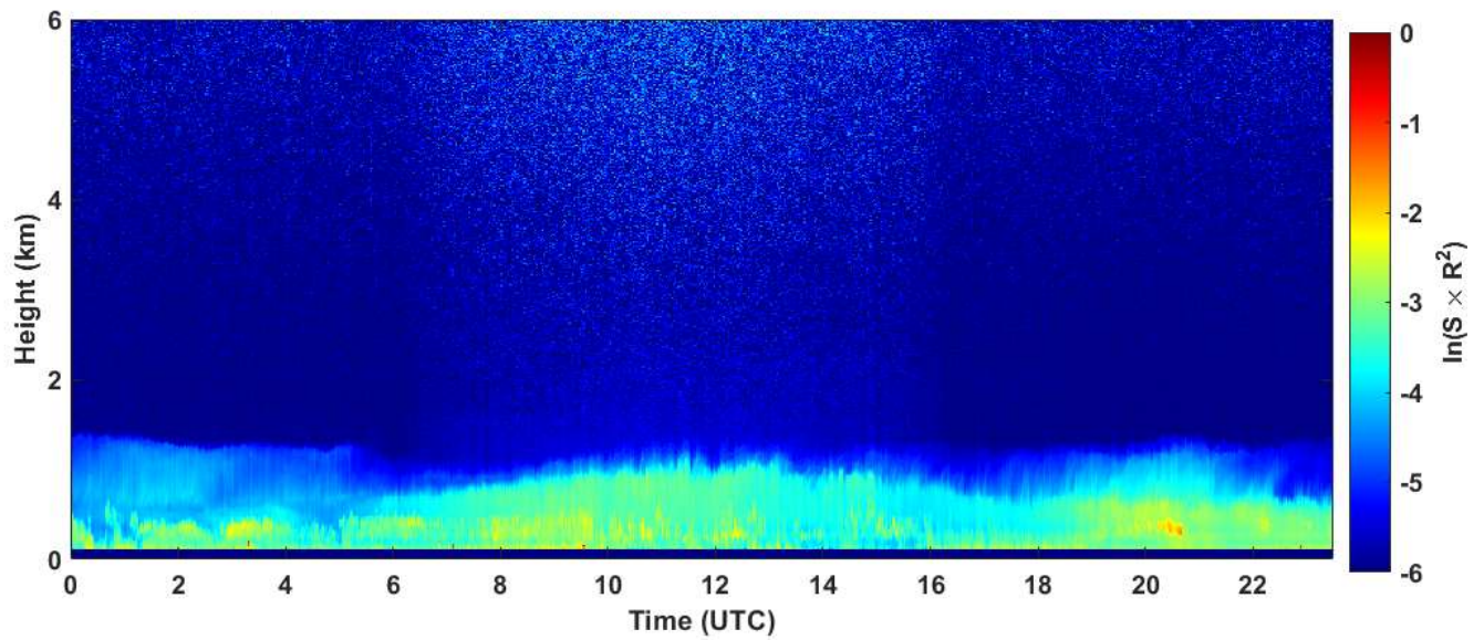
2020-01-16 RCS quick look CHM15k - ILVA LIDAR3 AGGLOMERATO
