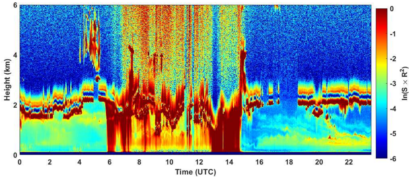
2020-01-14 RCS quick look CHM15k - ILVA LIDAR2 PARCHI
