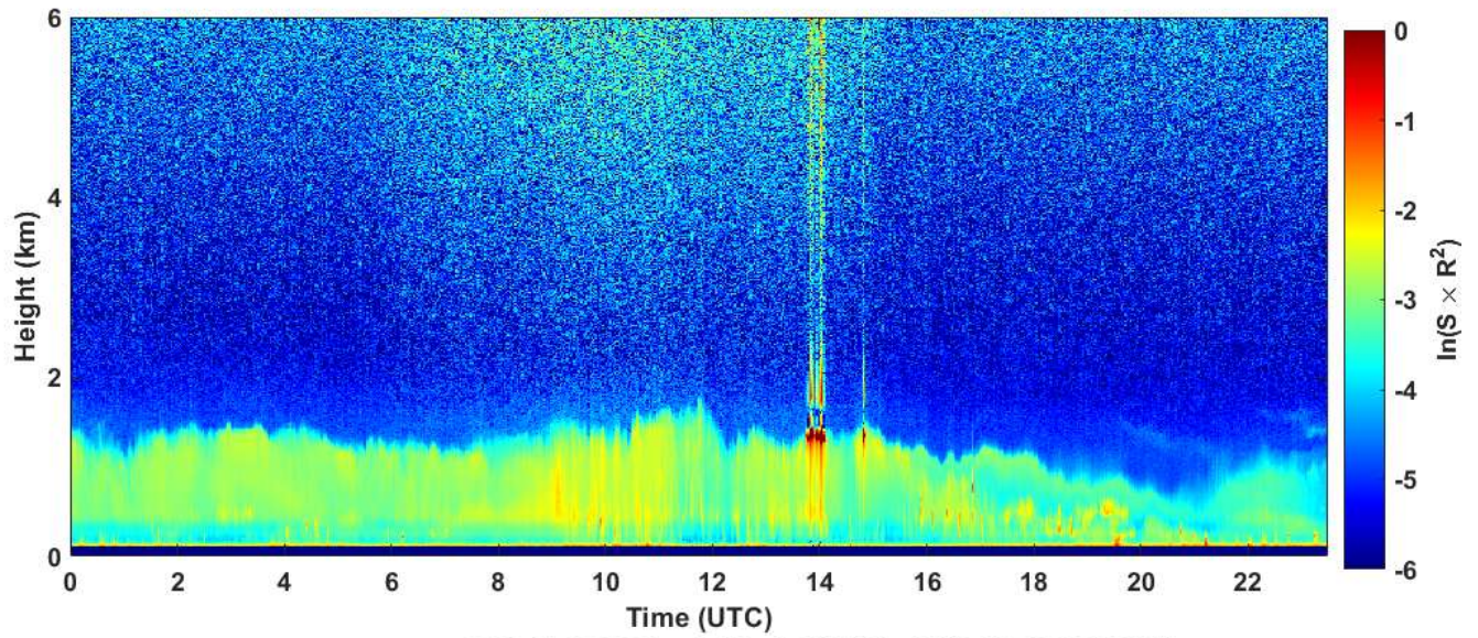
2020-01-08 RCS quick look CHM15k - ILVA LIDAR2 PARCHI
