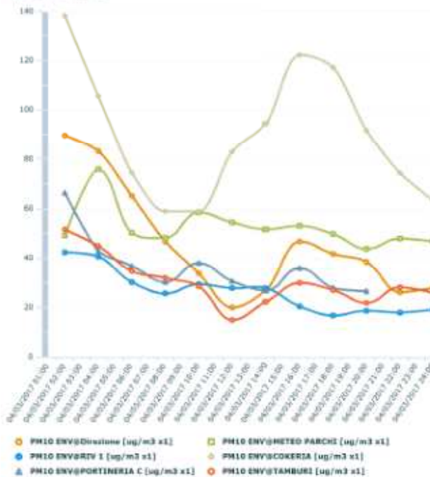
PM10
