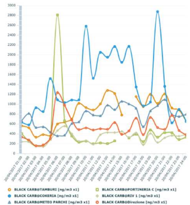
BLACK CARBON
